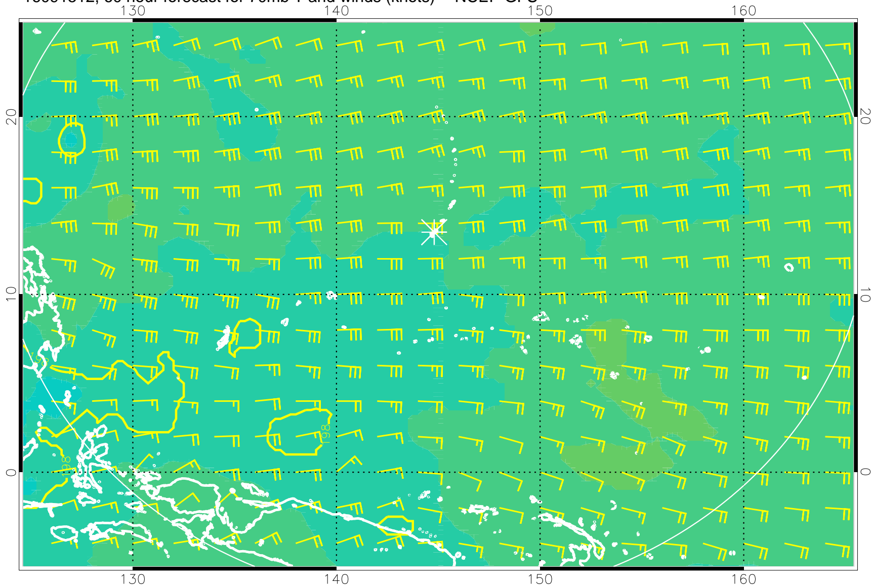
16091512, 60 hour forecast for 70mb T and winds (knots) -- NCEP GFS
