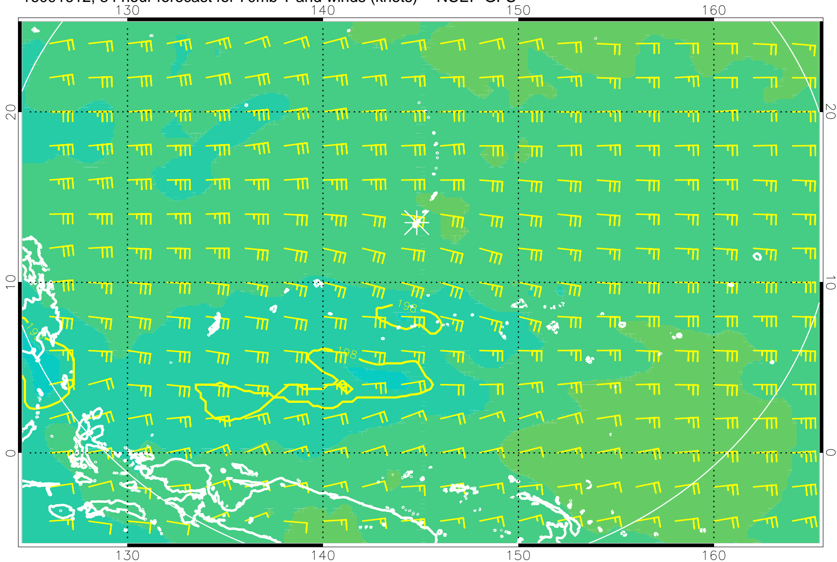
16091612, 84 hour forecast for 70mb T and winds (knots) -- NCEP GFS
