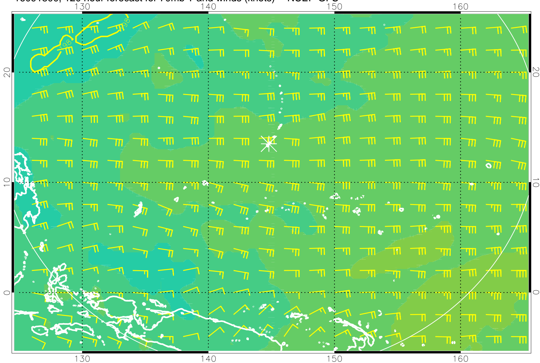
16091800, 120 hour forecast for 70mb T and winds (knots) -- NCEP GFS
