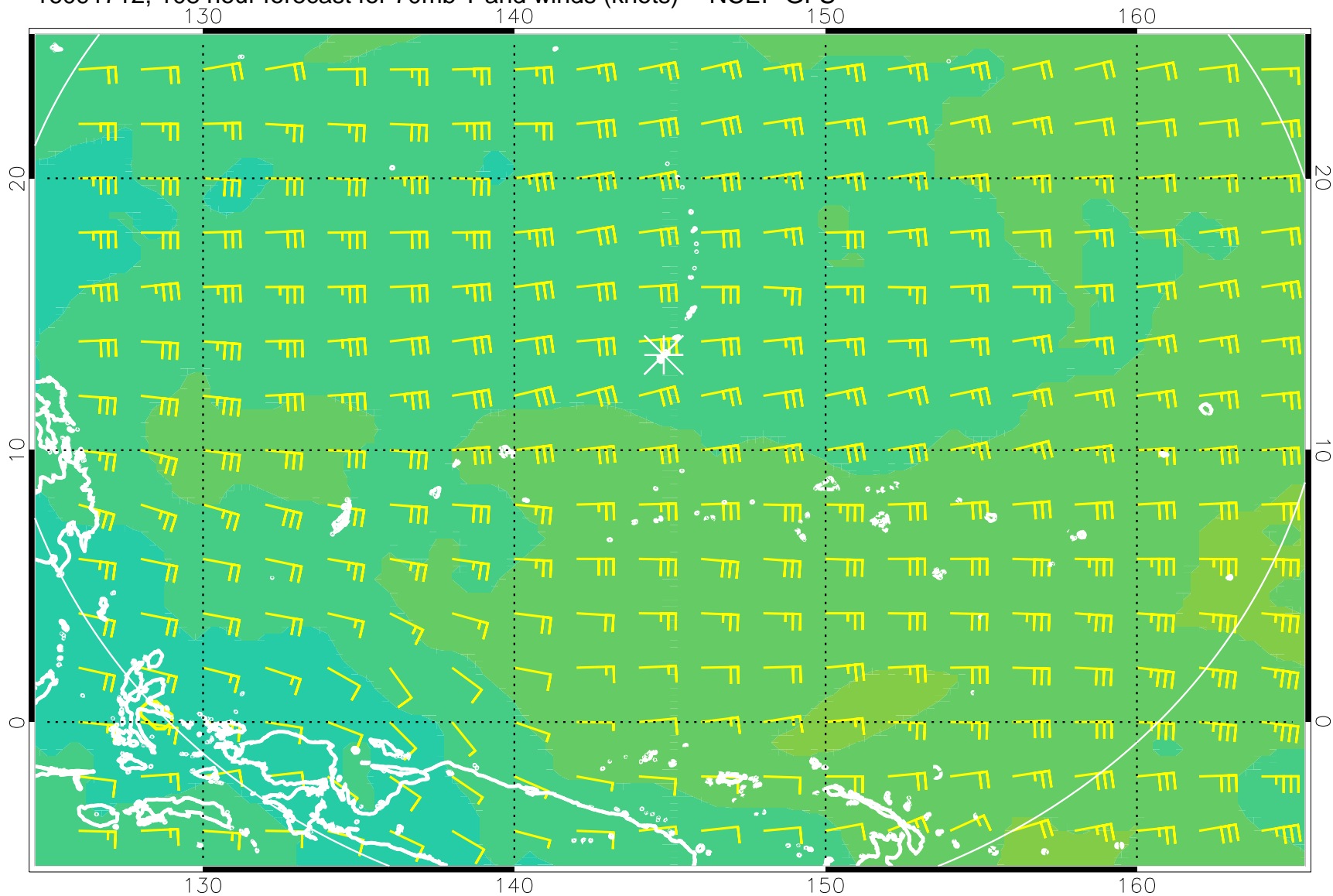
16091712, 108 hour forecast for 70mb T and winds (knots) -- NCEP GFS
