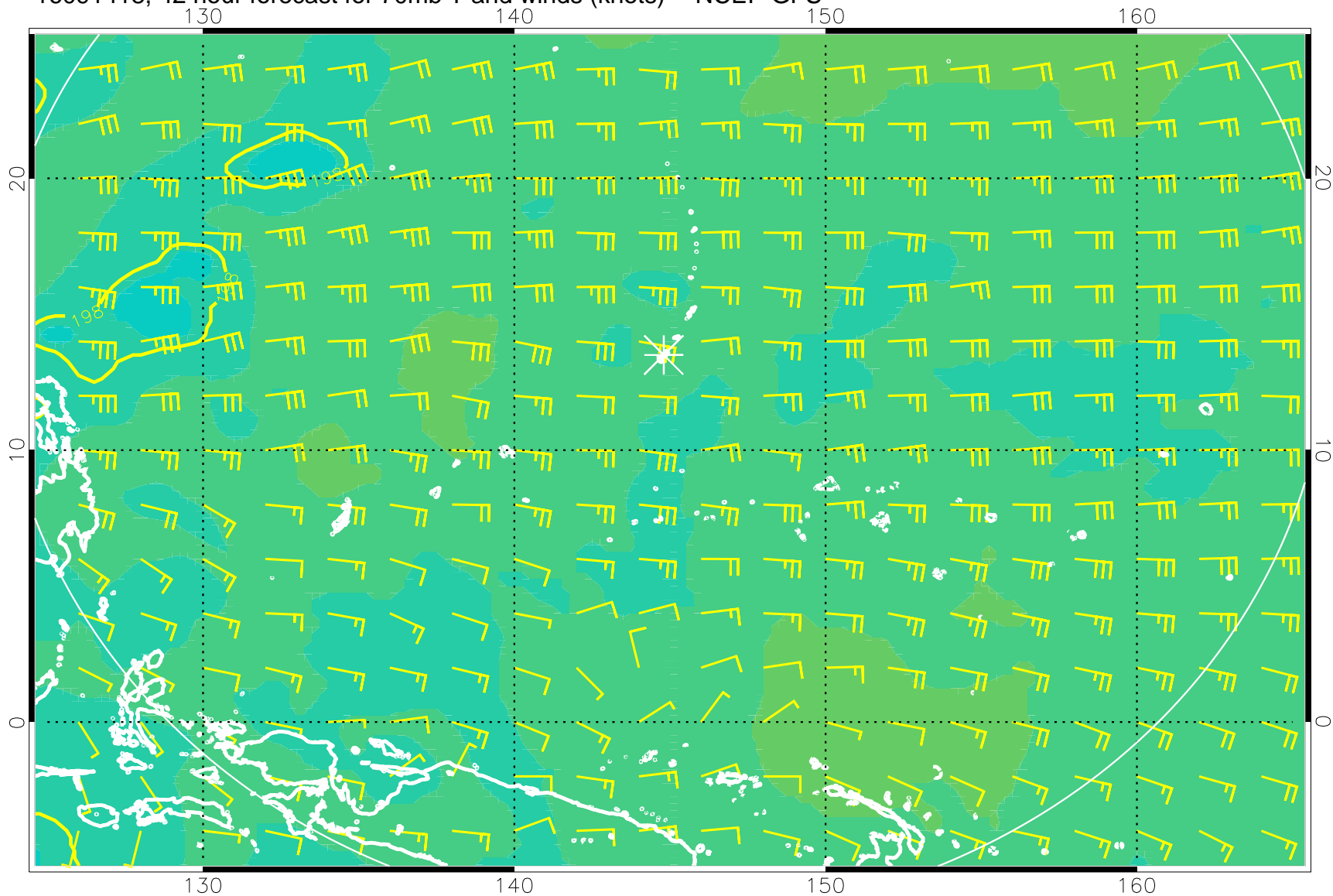
16091418, 42 hour forecast for 70mb T and winds (knots) -- NCEP GFS
