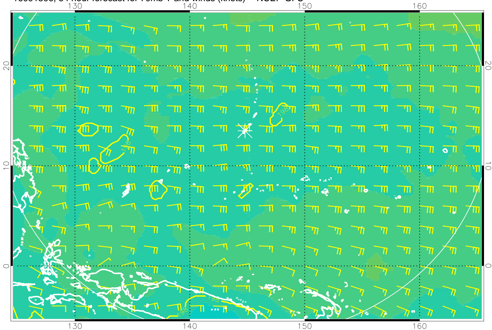
16091506, 54 hour forecast for 70mb T and winds (knots) -- NCEP GFS
