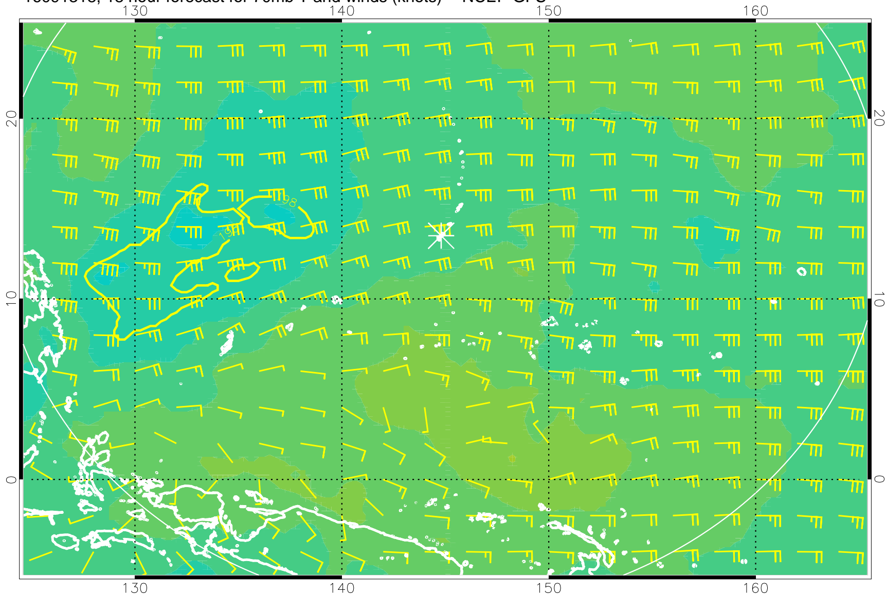
16091318, 18 hour forecast for 70mb T and winds (knots) -- NCEP GFS
