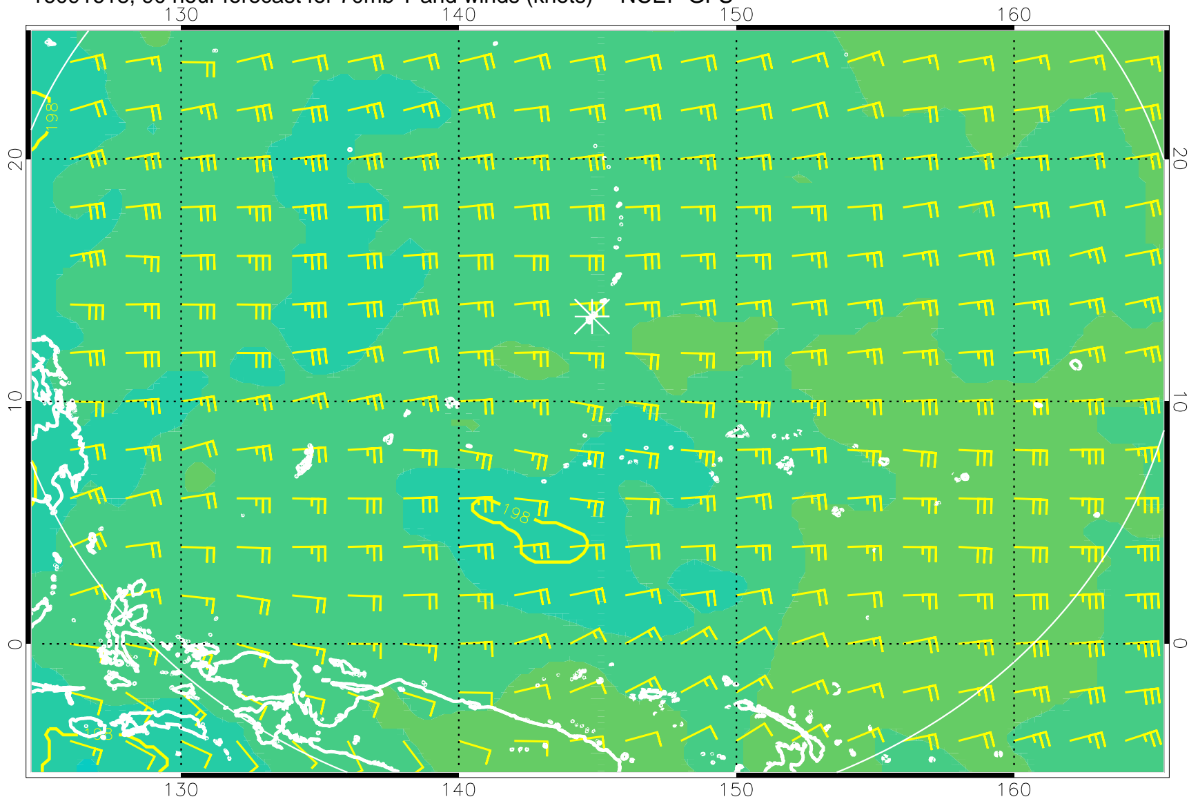
16091618, 90 hour forecast for 70mb T and winds (knots) -- NCEP GFS
