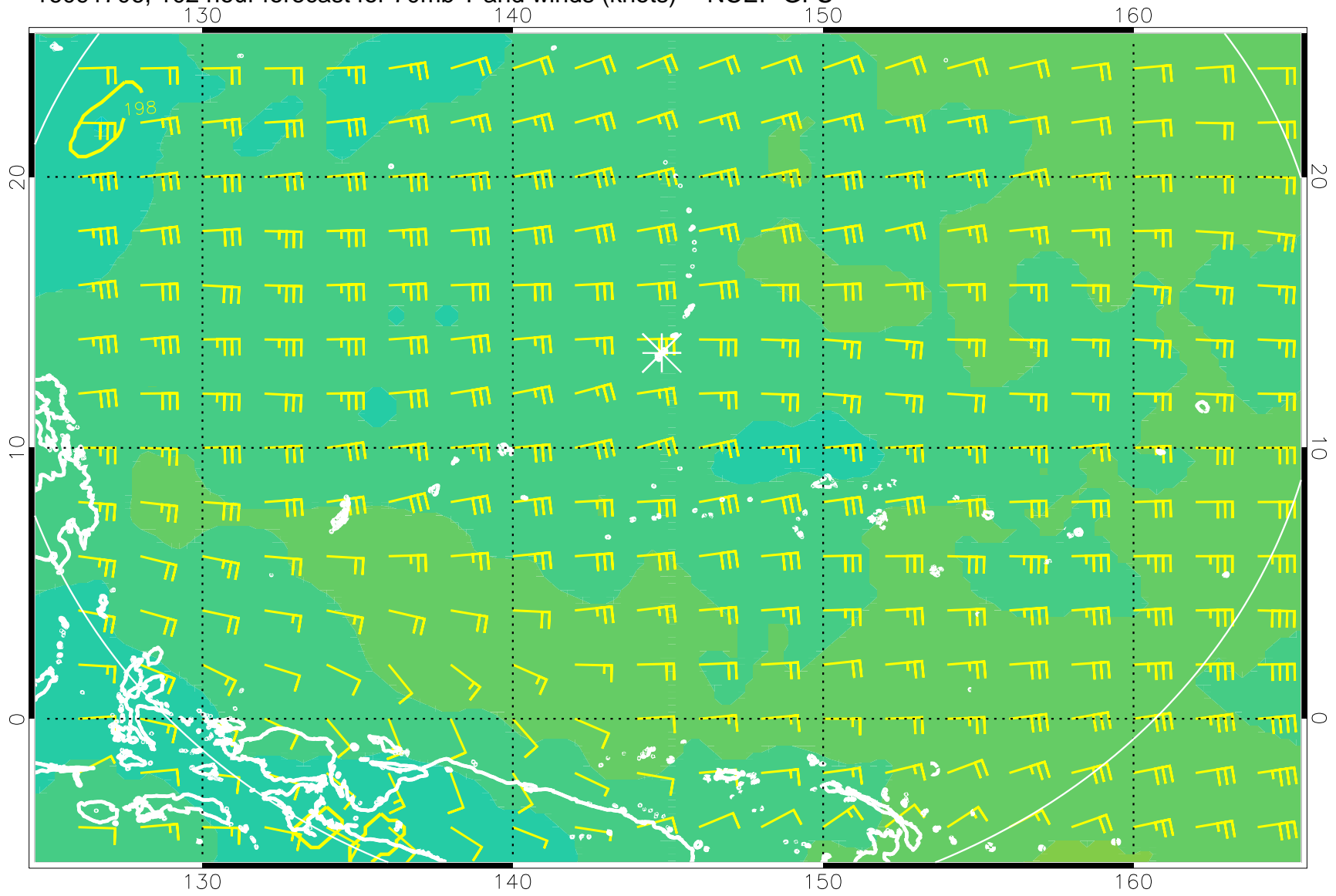
16091706, 102 hour forecast for 70mb T and winds (knots) -- NCEP GFS
