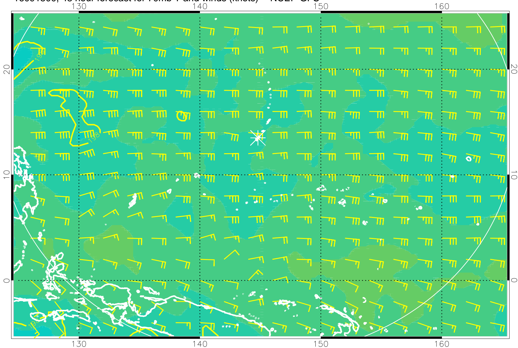
16091500, 48 hour forecast for 70mb T and winds (knots) -- NCEP GFS
