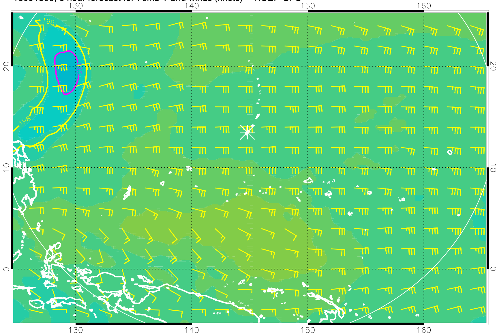
16091306, 6 hour forecast for 70mb T and winds (knots) -- NCEP GFS
