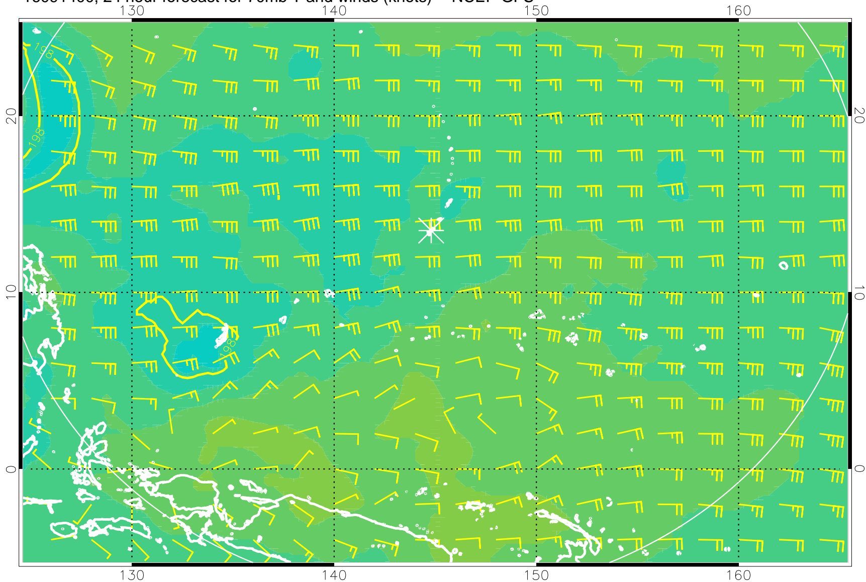
16091400, 24 hour forecast for 70mb T and winds (knots) -- NCEP GFS
