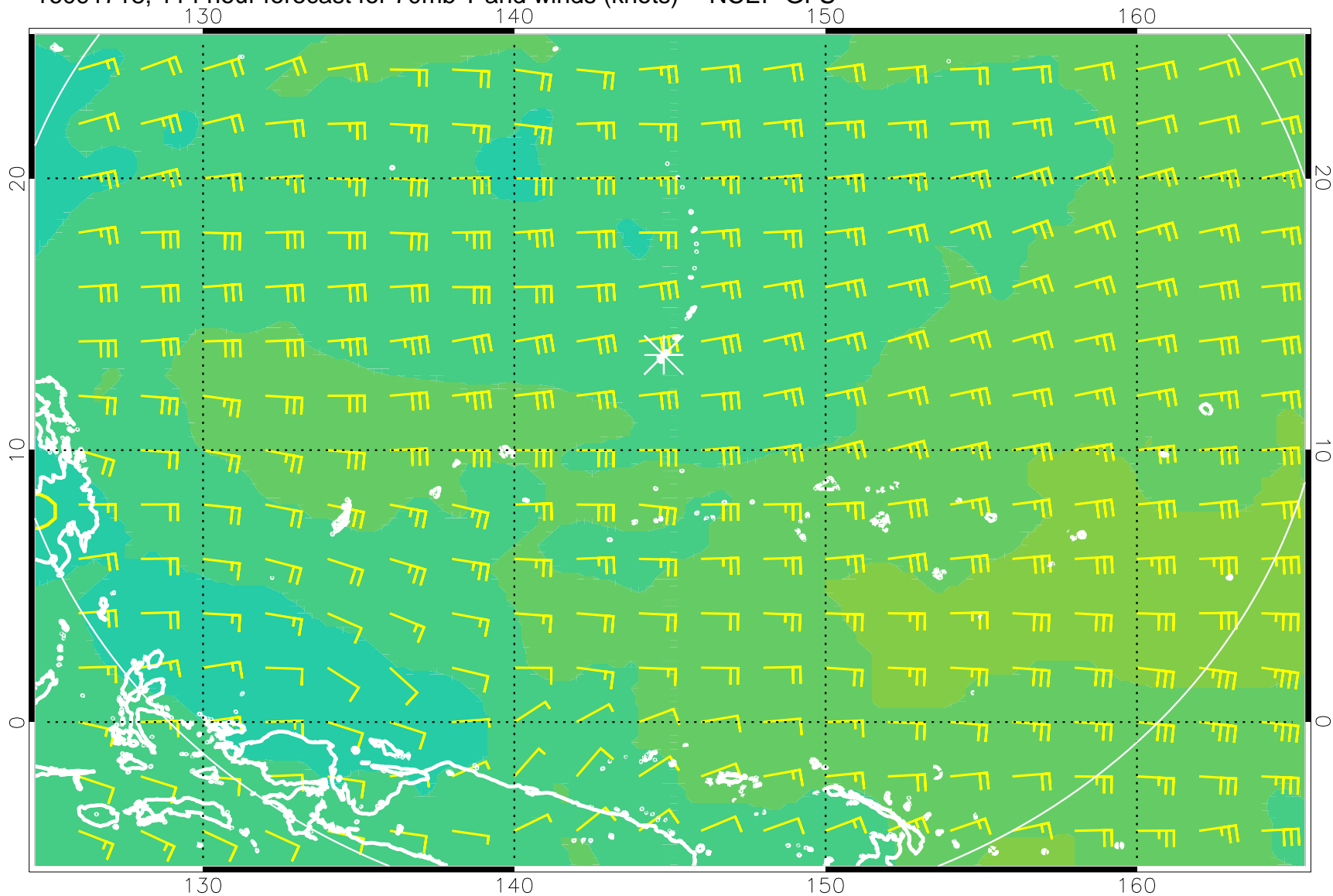
16091718, 114 hour forecast for 70mb T and winds (knots) -- NCEP GFS
