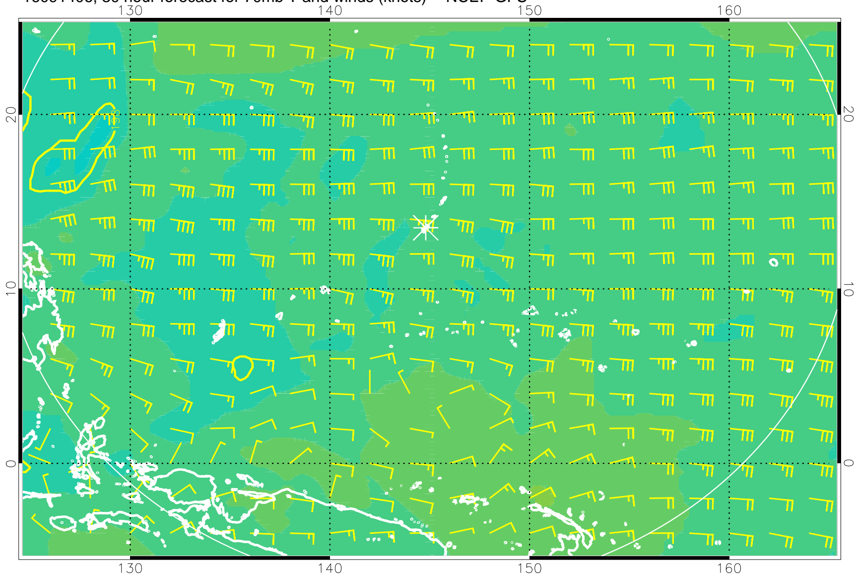
16091406, 30 hour forecast for 70mb T and winds (knots) -- NCEP GFS
