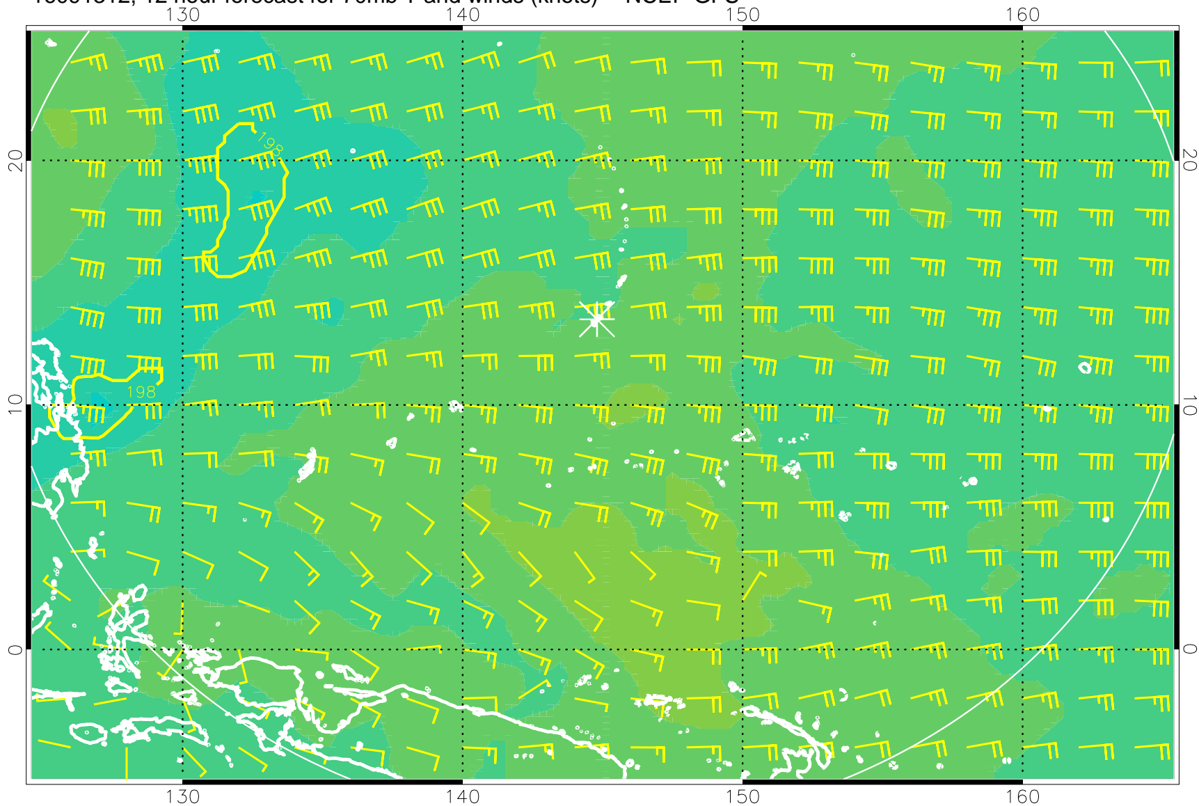
16091312, 12 hour forecast for 70mb T and winds (knots) -- NCEP GFS
