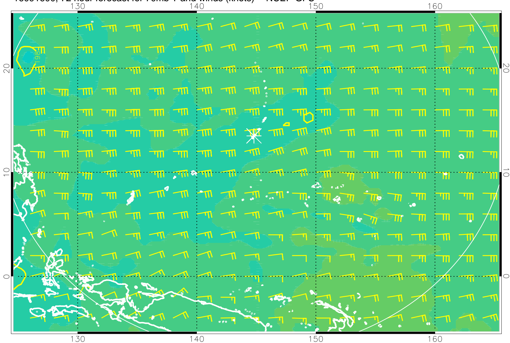
16091600, 72 hour forecast for 70mb T and winds (knots) -- NCEP GFS
