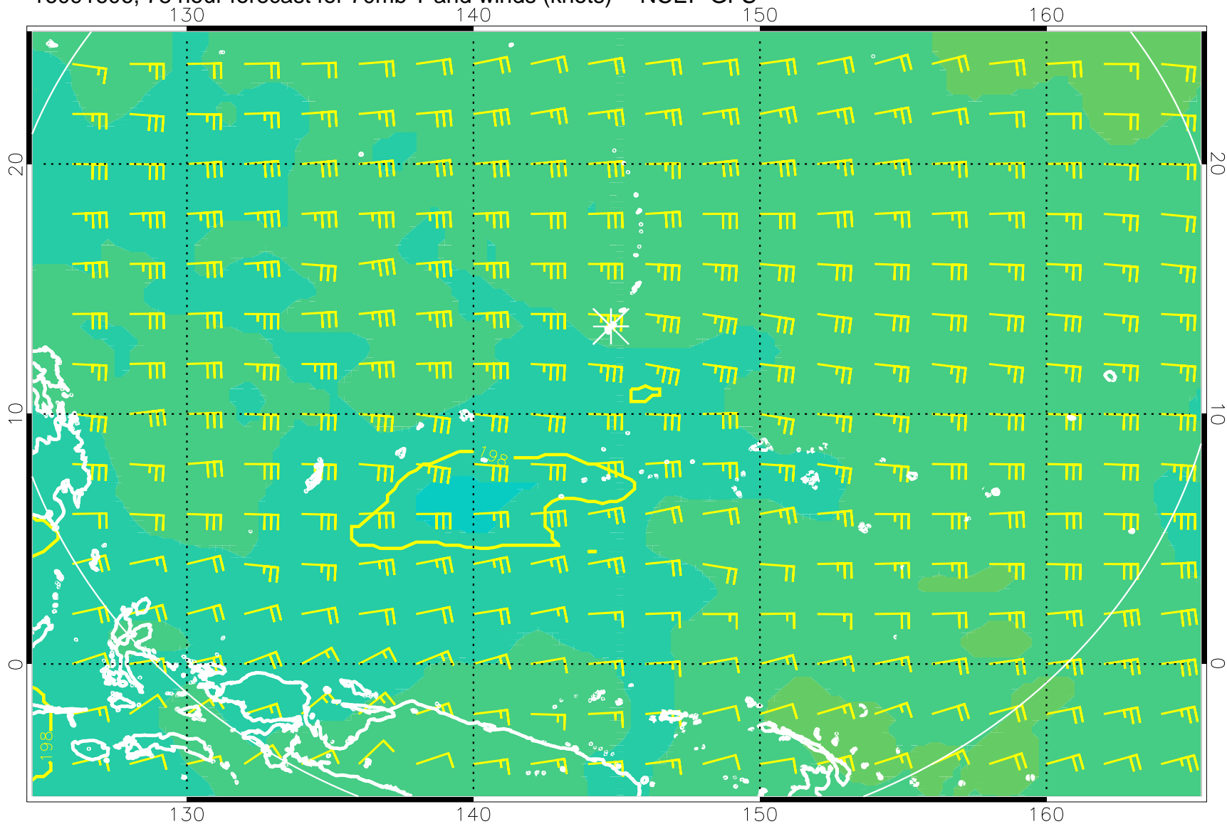
16091606, 78 hour forecast for 70mb T and winds (knots) -- NCEP GFS
