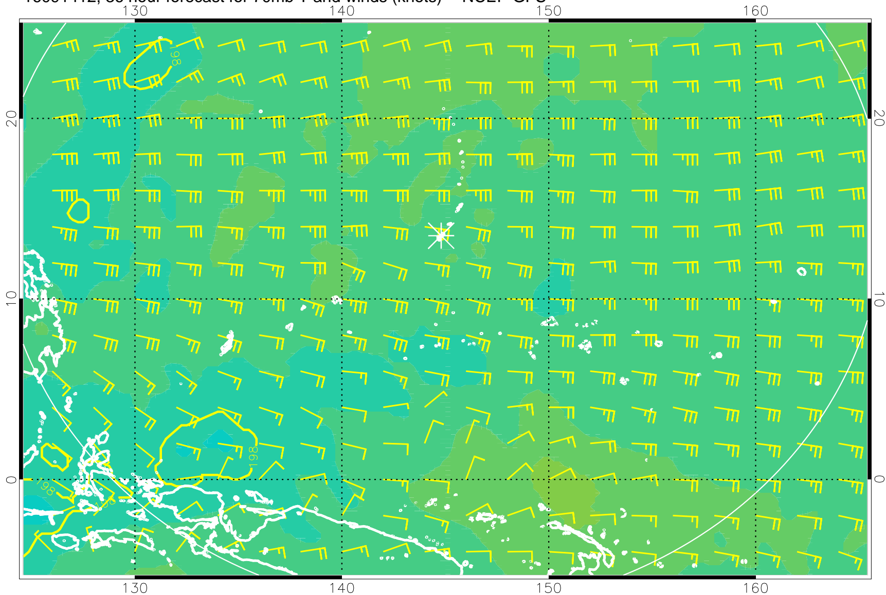
16091412, 36 hour forecast for 70mb T and winds (knots) -- NCEP GFS
