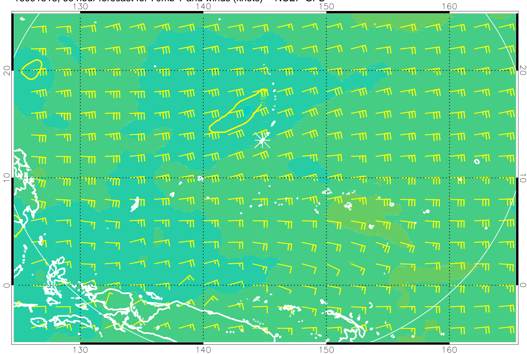
16091518, 66 hour forecast for 70mb T and winds (knots) -- NCEP GFS
