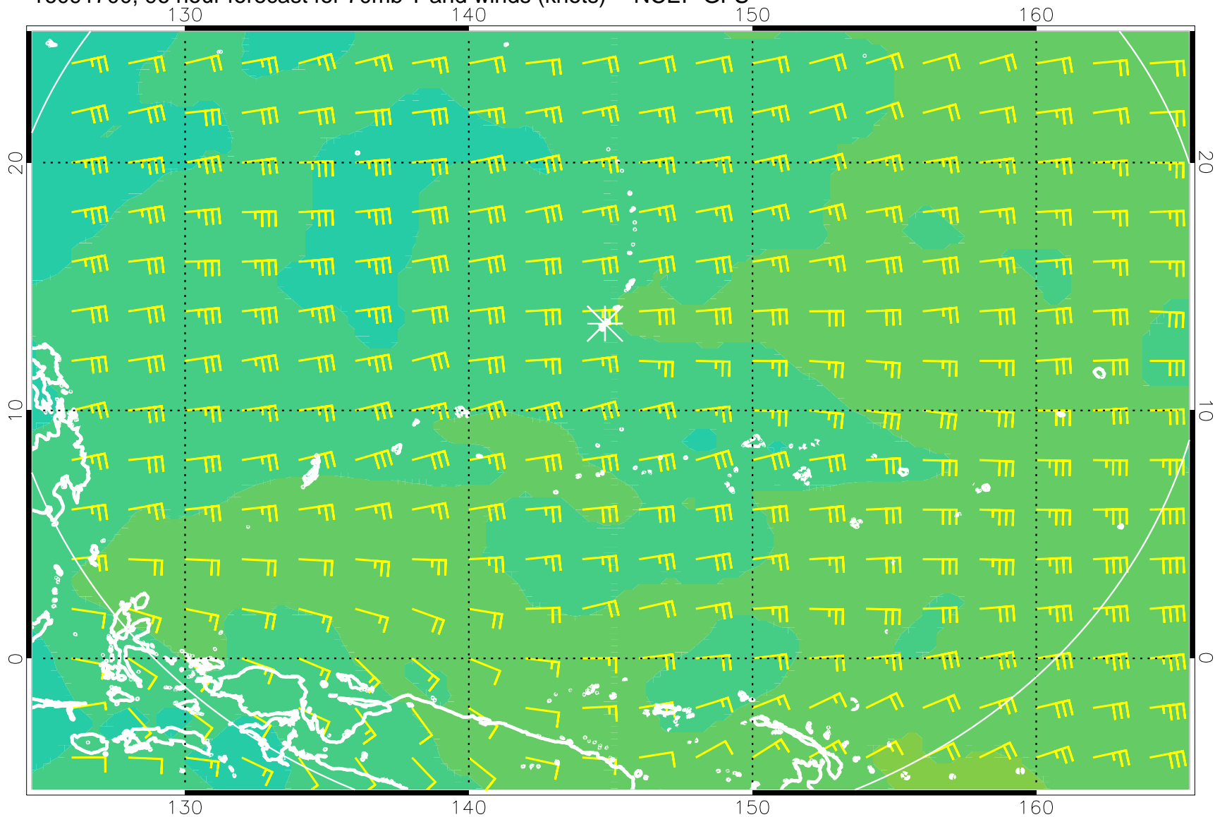
16091700, 96 hour forecast for 70mb T and winds (knots) -- NCEP GFS
