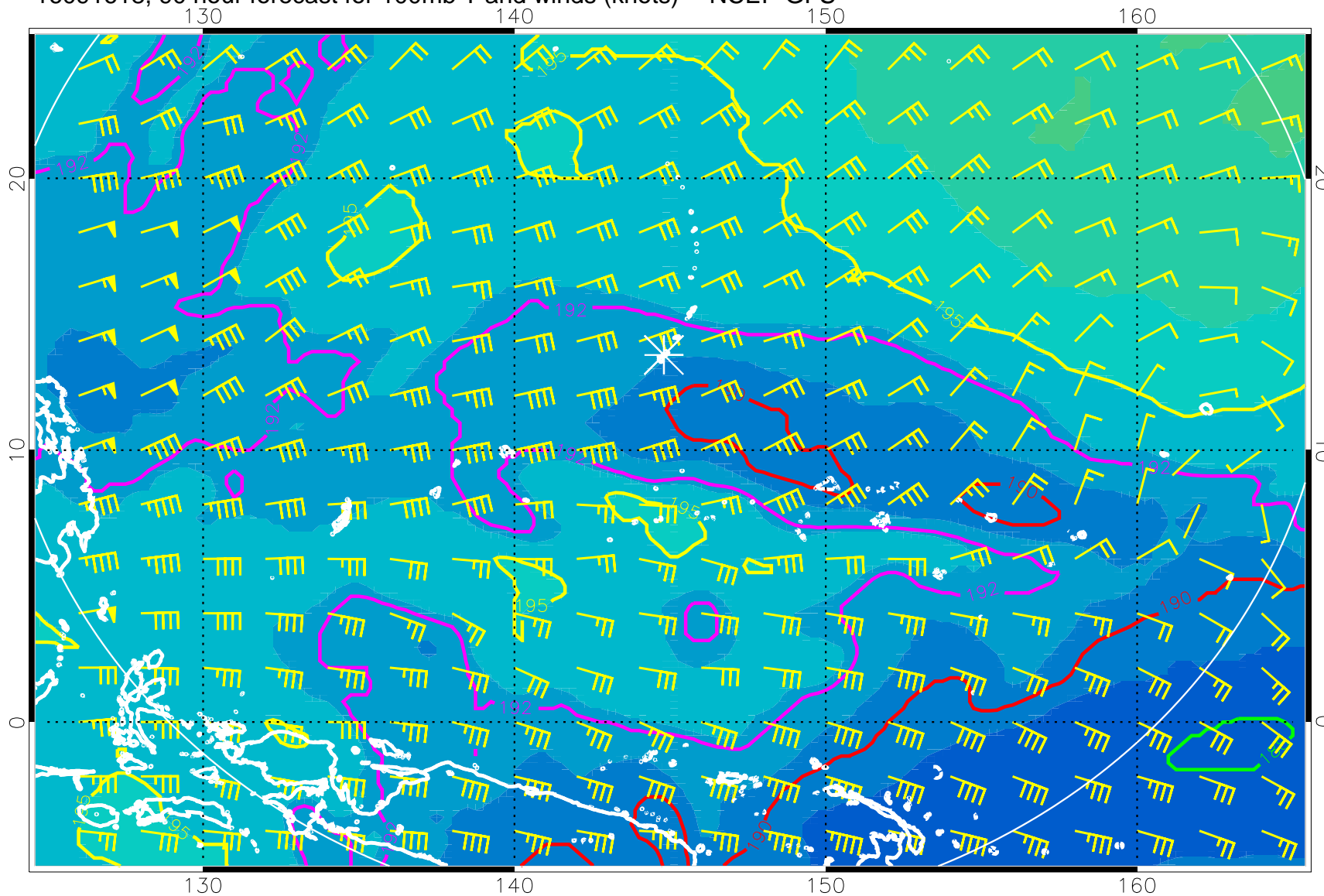
16091618, 90 hour forecast for 100mb T and winds (knots) -- NCEP GFS
