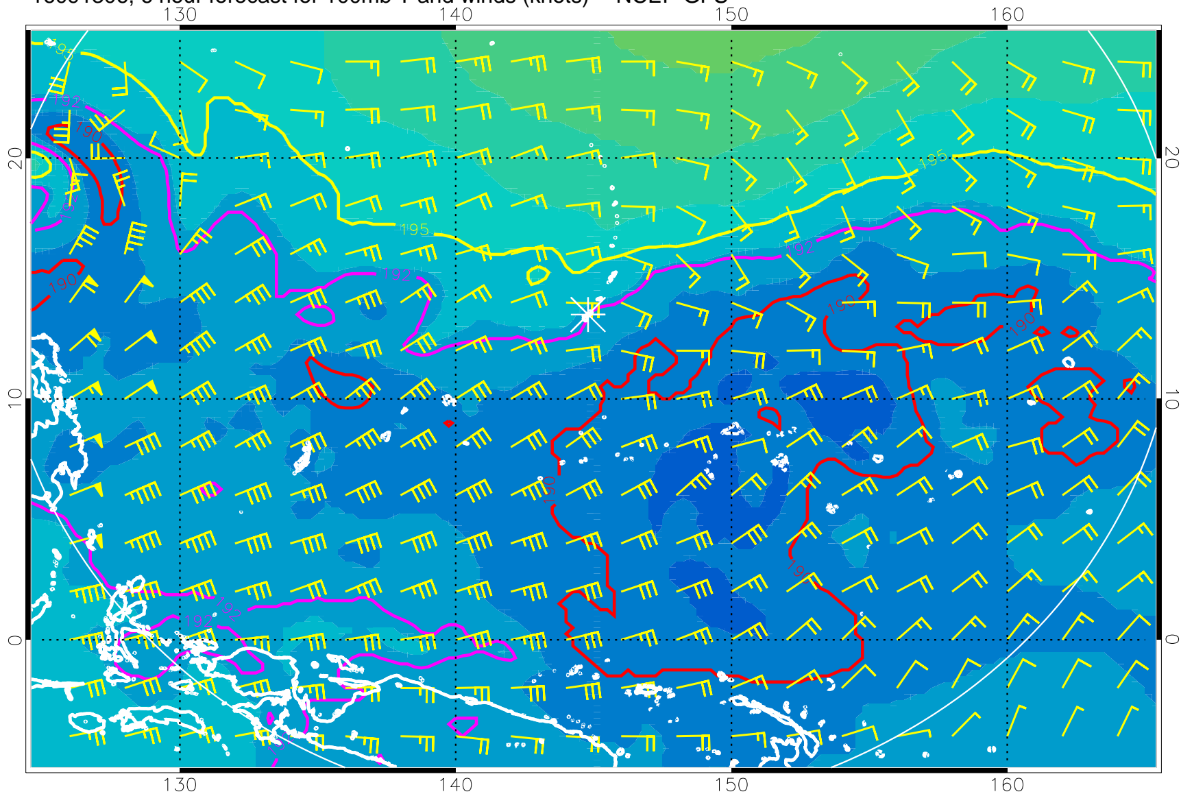
16091306, 6 hour forecast for 100mb T and winds (knots) -- NCEP GFS
