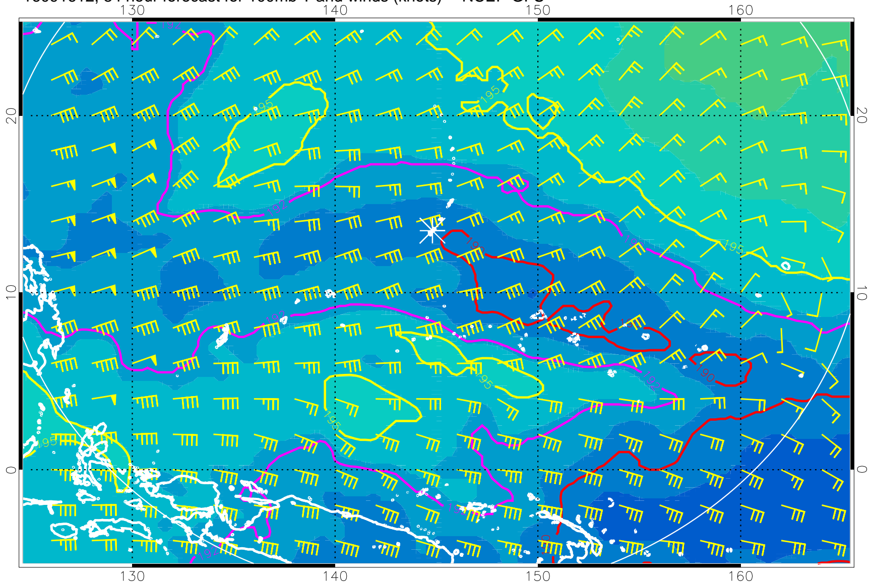
16091612, 84 hour forecast for 100mb T and winds (knots) -- NCEP GFS
