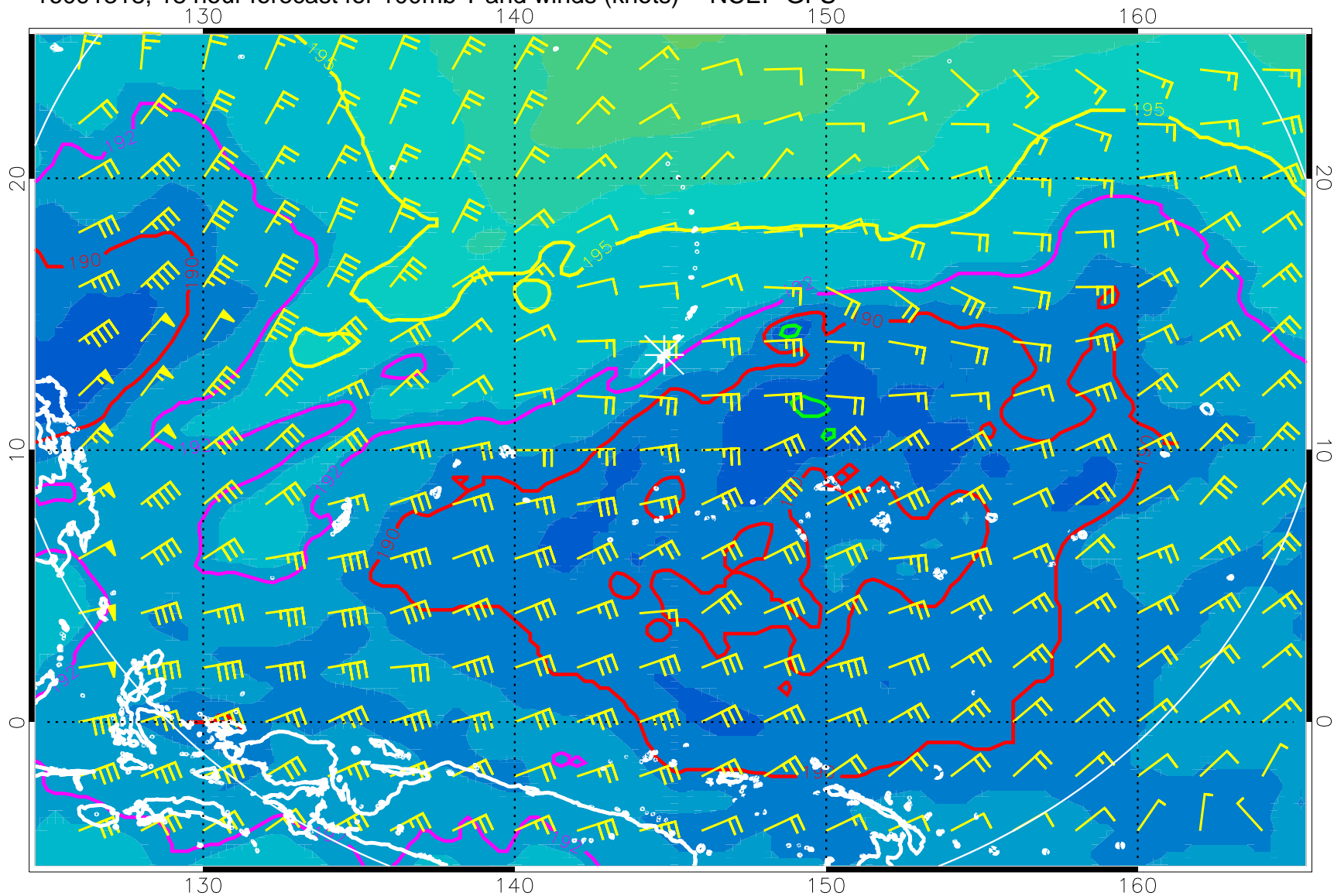
16091318, 18 hour forecast for 100mb T and winds (knots) -- NCEP GFS
