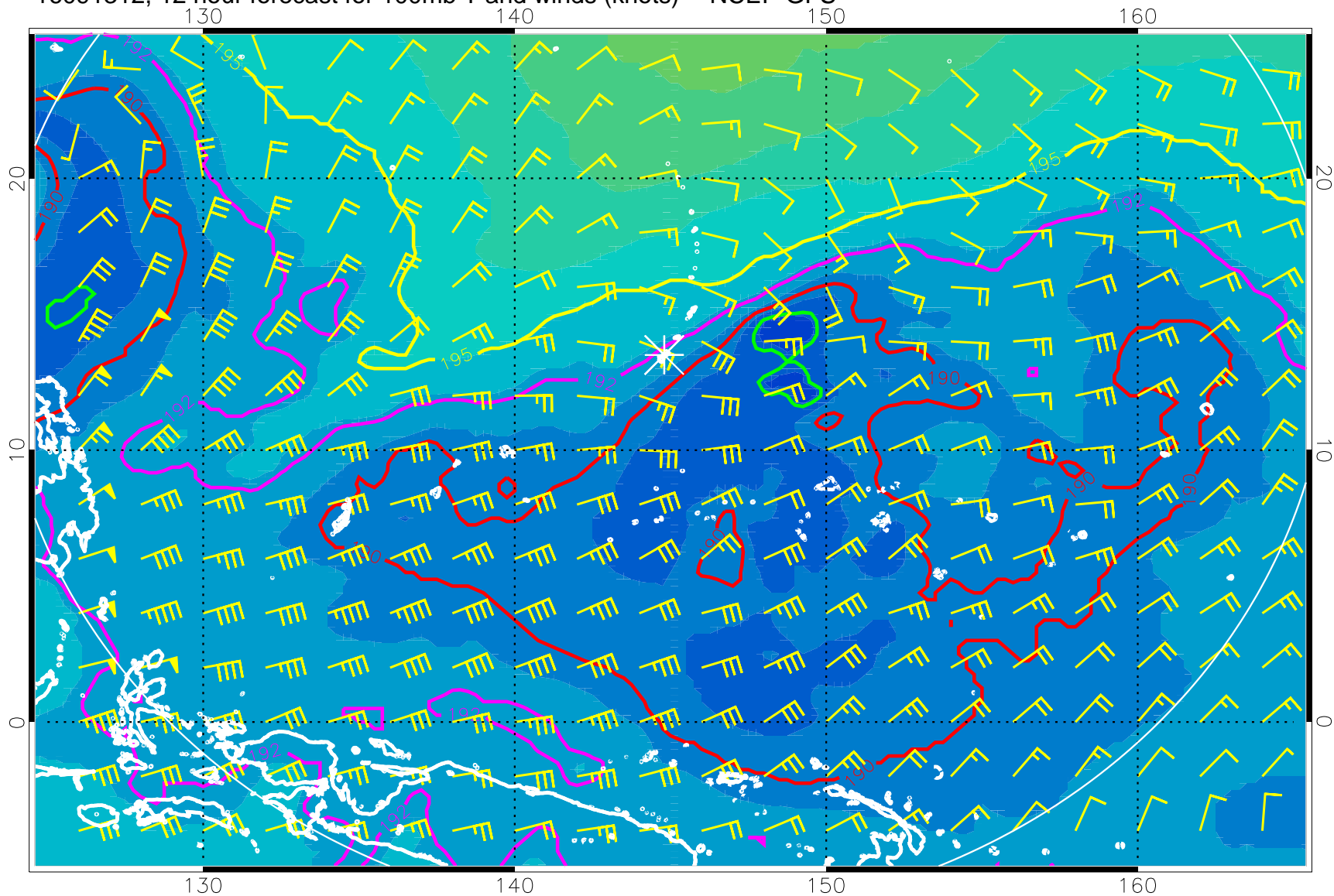
16091312, 12 hour forecast for 100mb T and winds (knots) -- NCEP GFS
