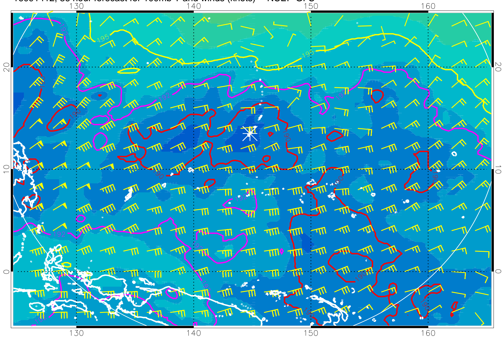
16091412, 36 hour forecast for 100mb T and winds (knots) -- NCEP GFS
