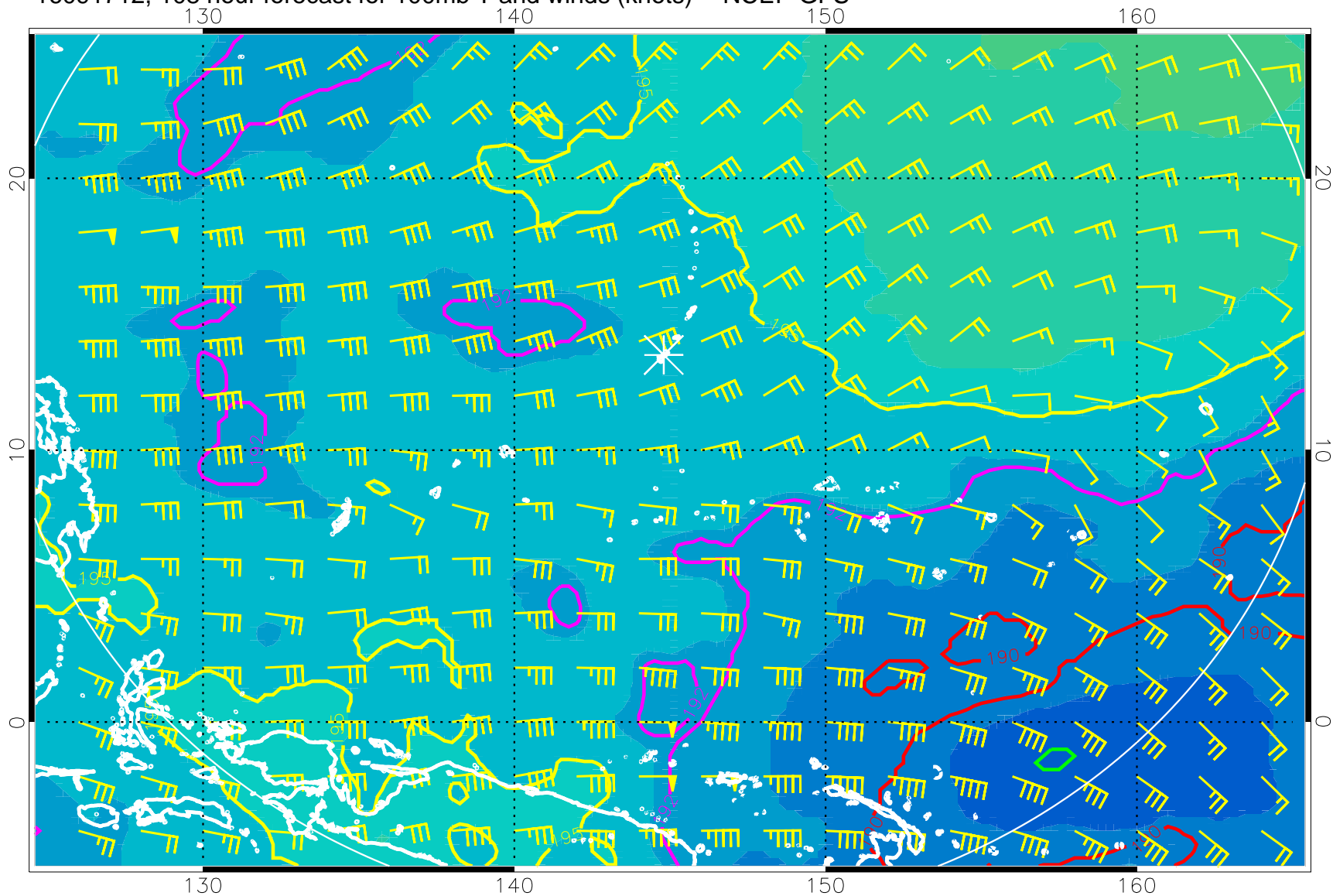
16091712, 108 hour forecast for 100mb T and winds (knots) -- NCEP GFS
