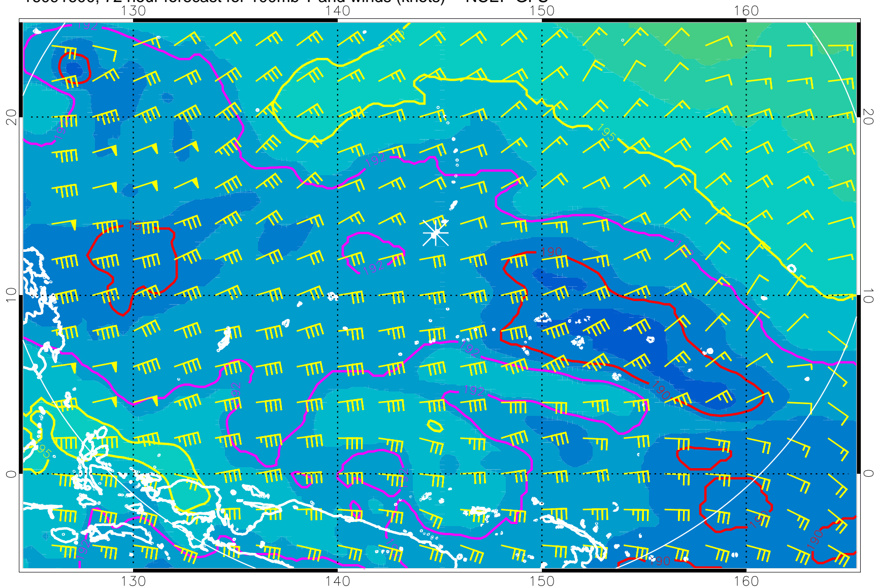
16091600, 72 hour forecast for 100mb T and winds (knots) -- NCEP GFS
