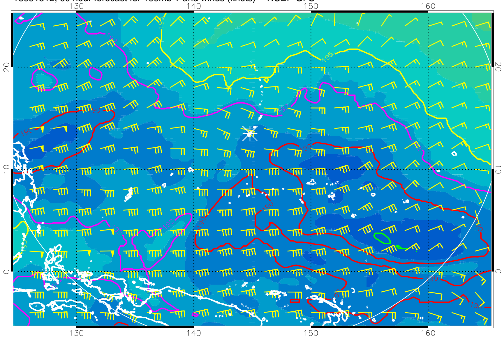
16091512, 60 hour forecast for 100mb T and winds (knots) -- NCEP GFS
