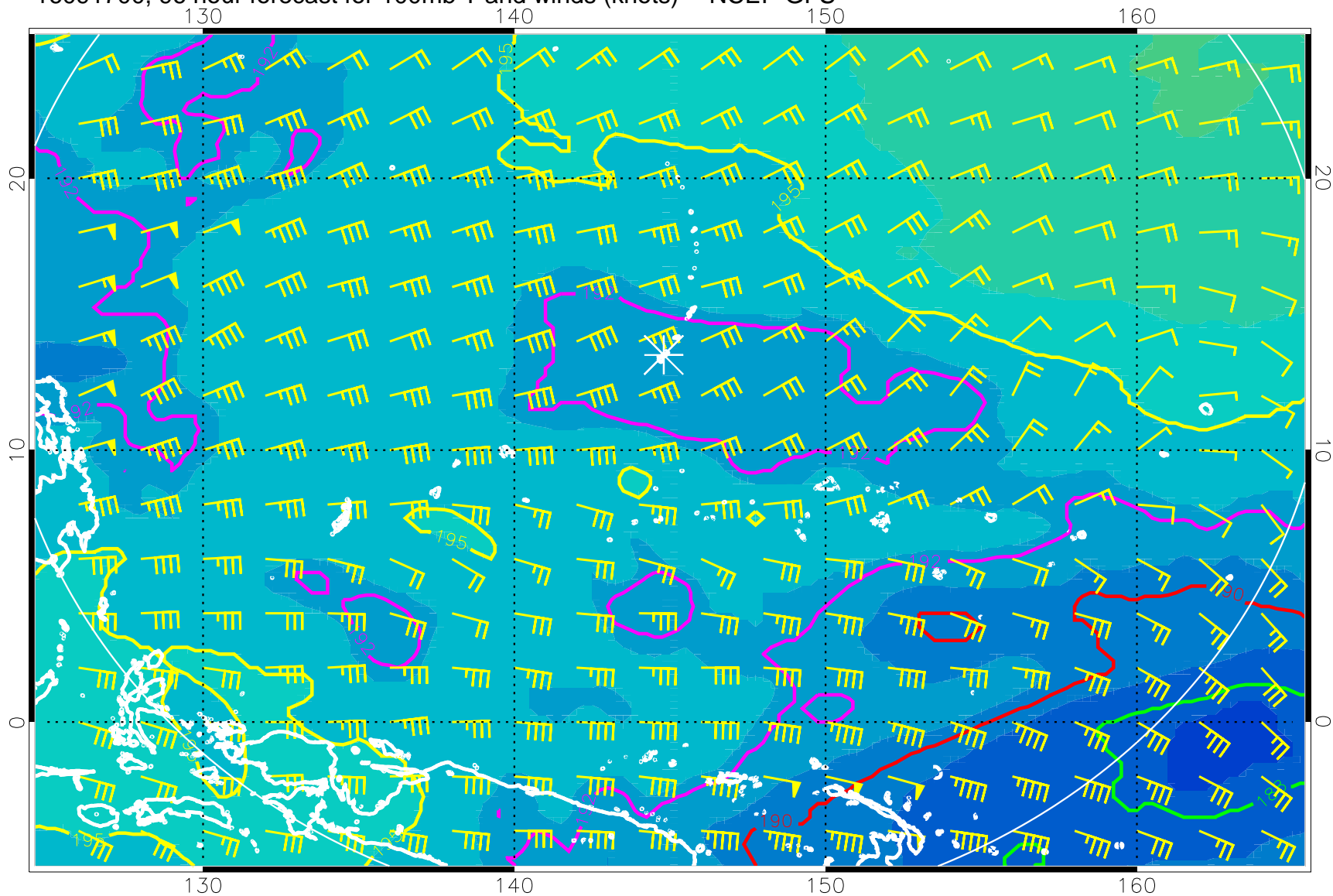
16091700, 96 hour forecast for 100mb T and winds (knots) -- NCEP GFS
