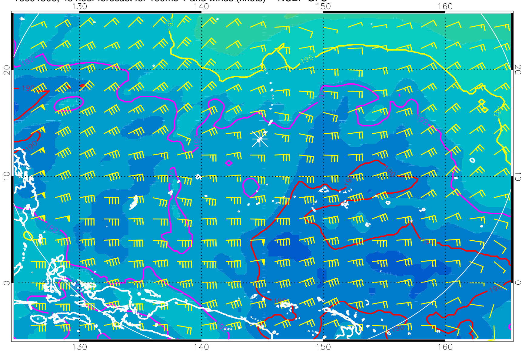
16091500, 48 hour forecast for 100mb T and winds (knots) -- NCEP GFS
