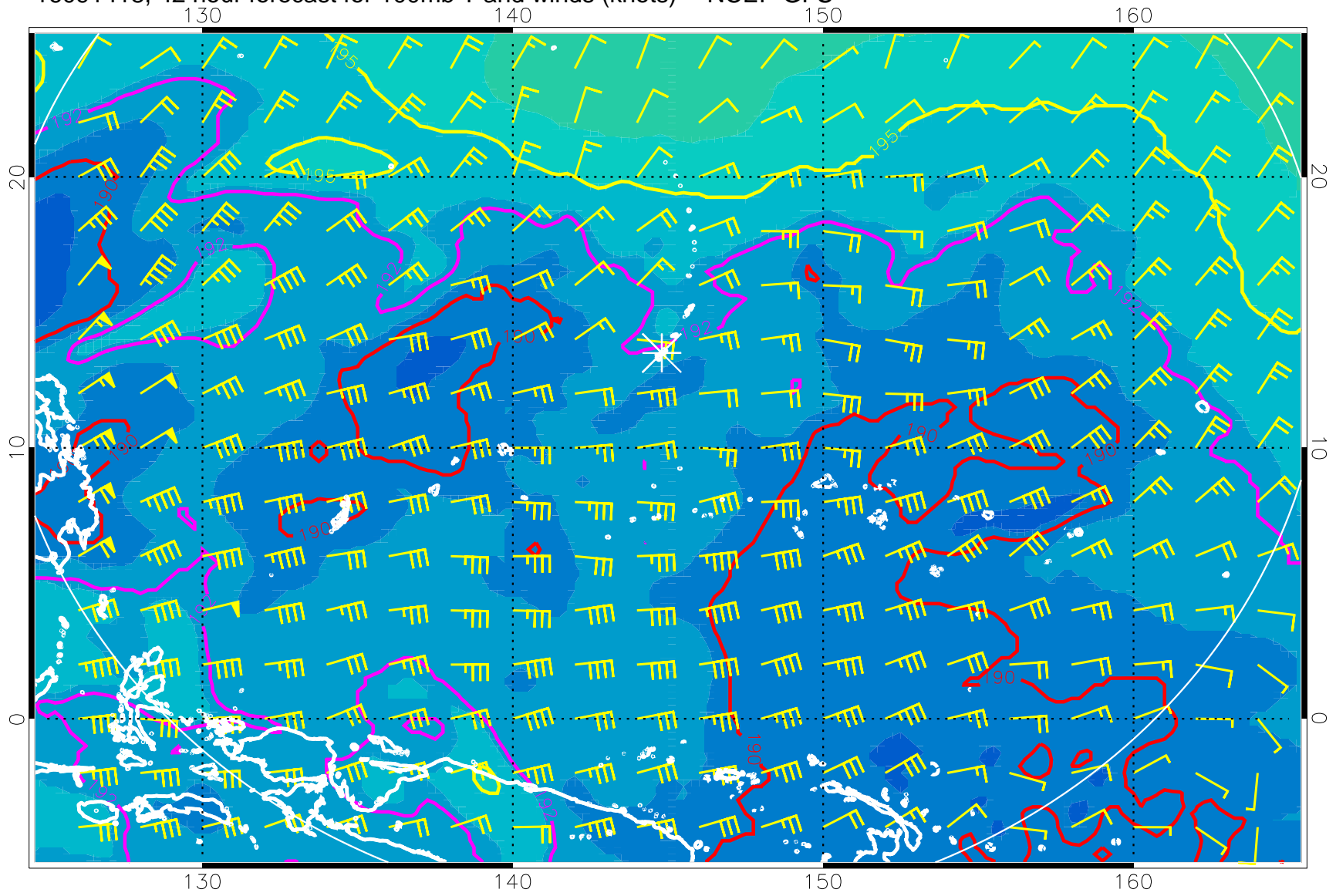
16091418, 42 hour forecast for 100mb T and winds (knots) -- NCEP GFS
