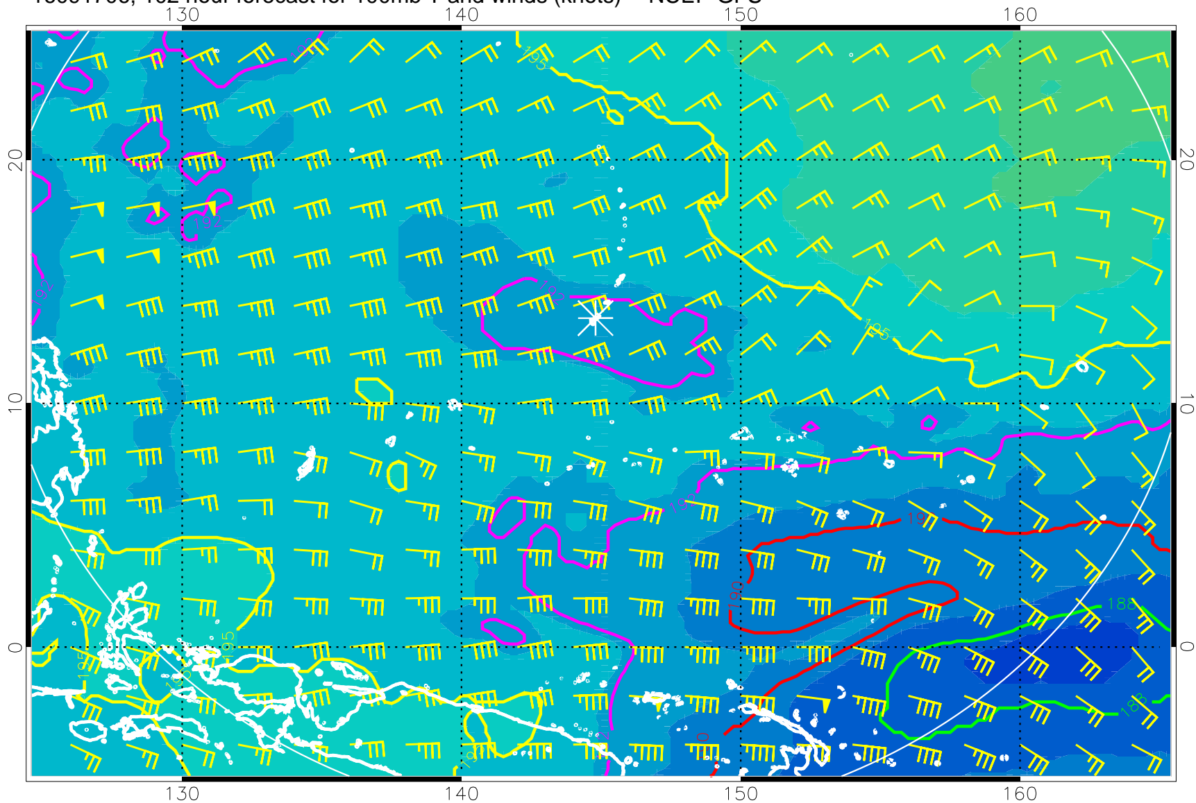
16091706, 102 hour forecast for 100mb T and winds (knots) -- NCEP GFS
