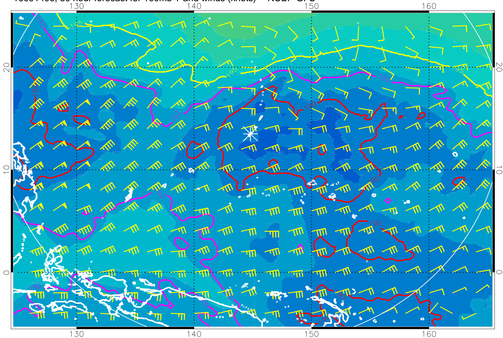
16091406, 30 hour forecast for 100mb T and winds (knots) -- NCEP GFS
