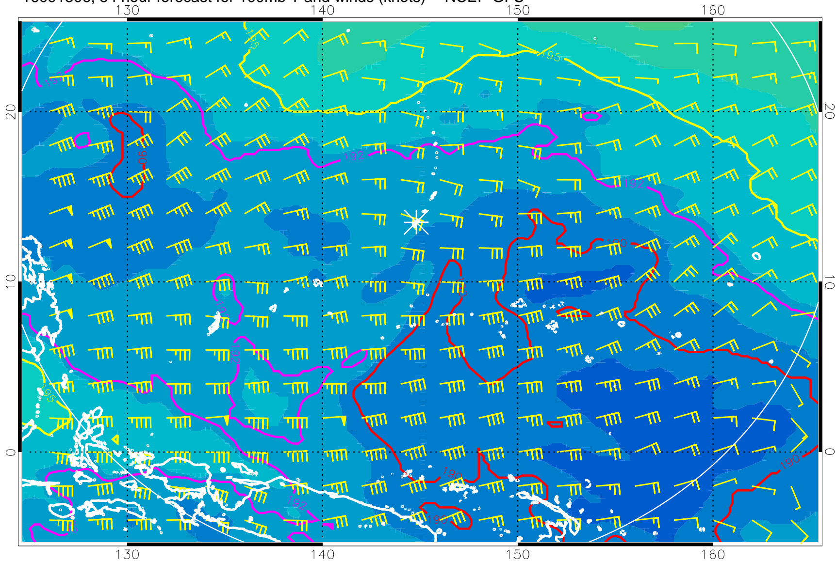
16091506, 54 hour forecast for 100mb T and winds (knots) -- NCEP GFS
