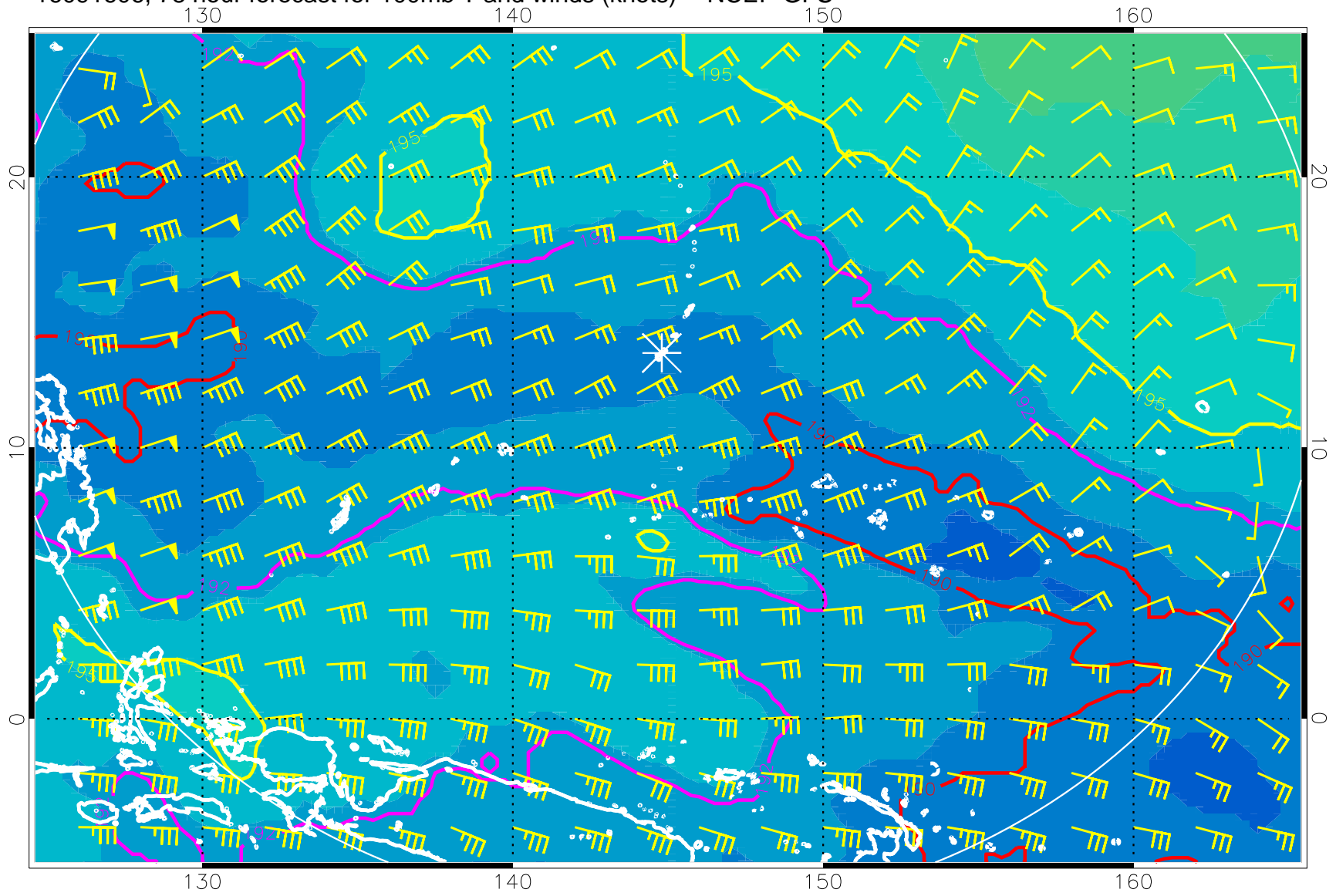
16091606, 78 hour forecast for 100mb T and winds (knots) -- NCEP GFS
