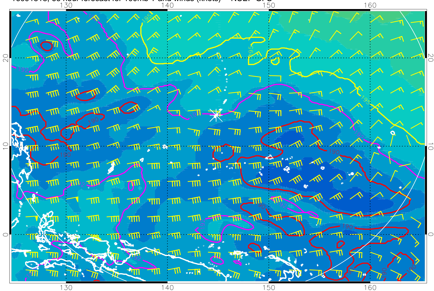
16091518, 66 hour forecast for 100mb T and winds (knots) -- NCEP GFS
