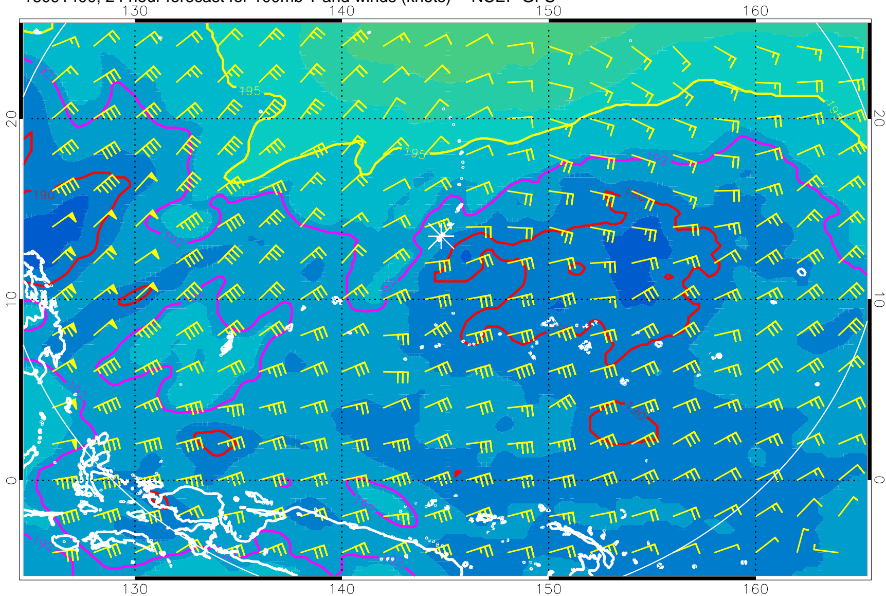
16091400, 24 hour forecast for 100mb T and winds (knots) -- NCEP GFS
