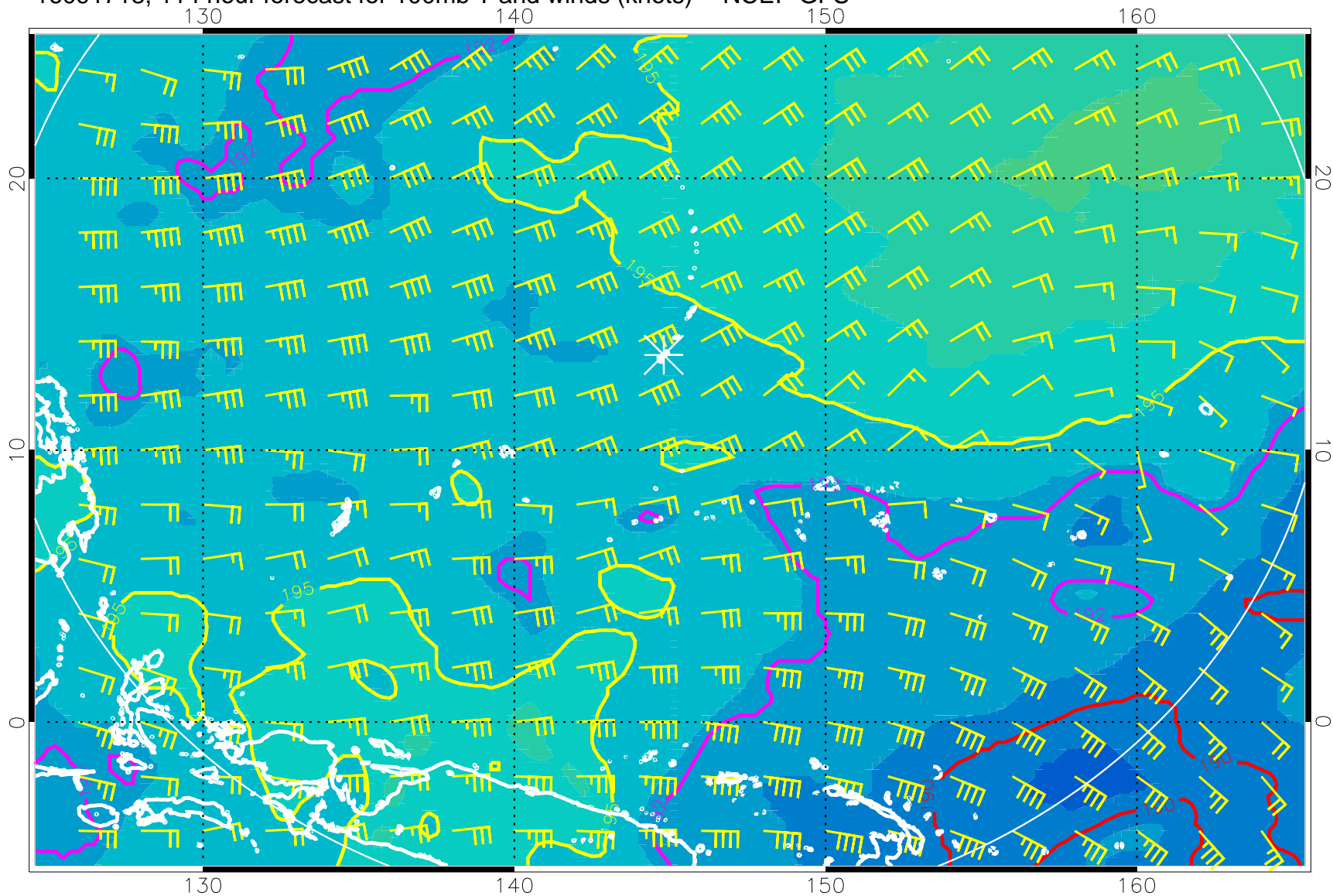
16091718, 114 hour forecast for 100mb T and winds (knots) -- NCEP GFS
