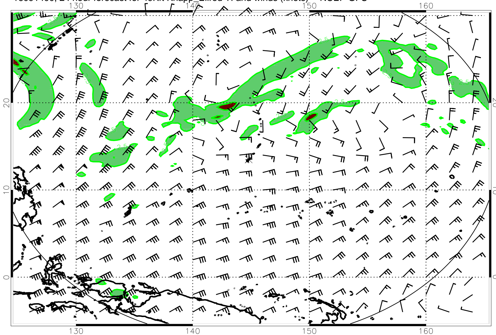
16091400, 24 hour forecast for 49Kft Knapp_Ellrod TI and winds (knots) -- NCEP GFS
