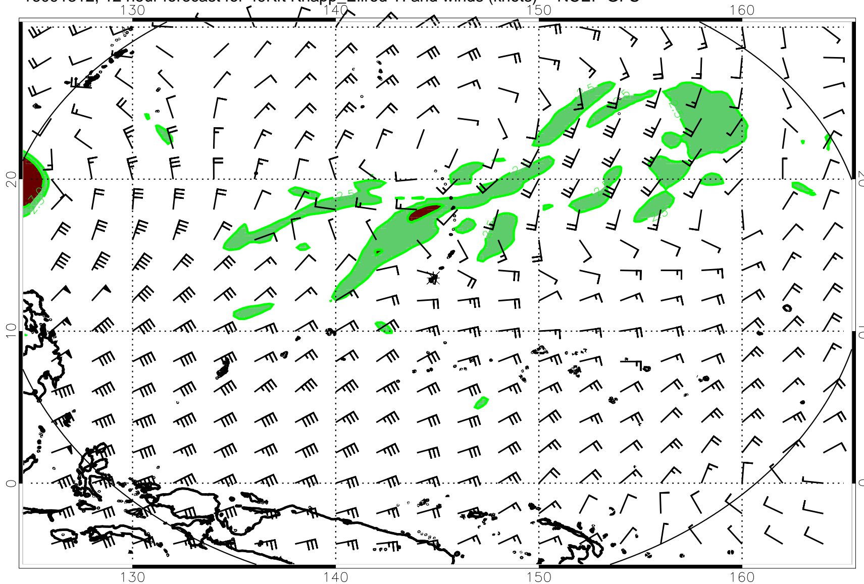
16091312, 12 hour forecast for 49Kft Knapp_Ellrod TI and winds (knots) -- NCEP GFS
