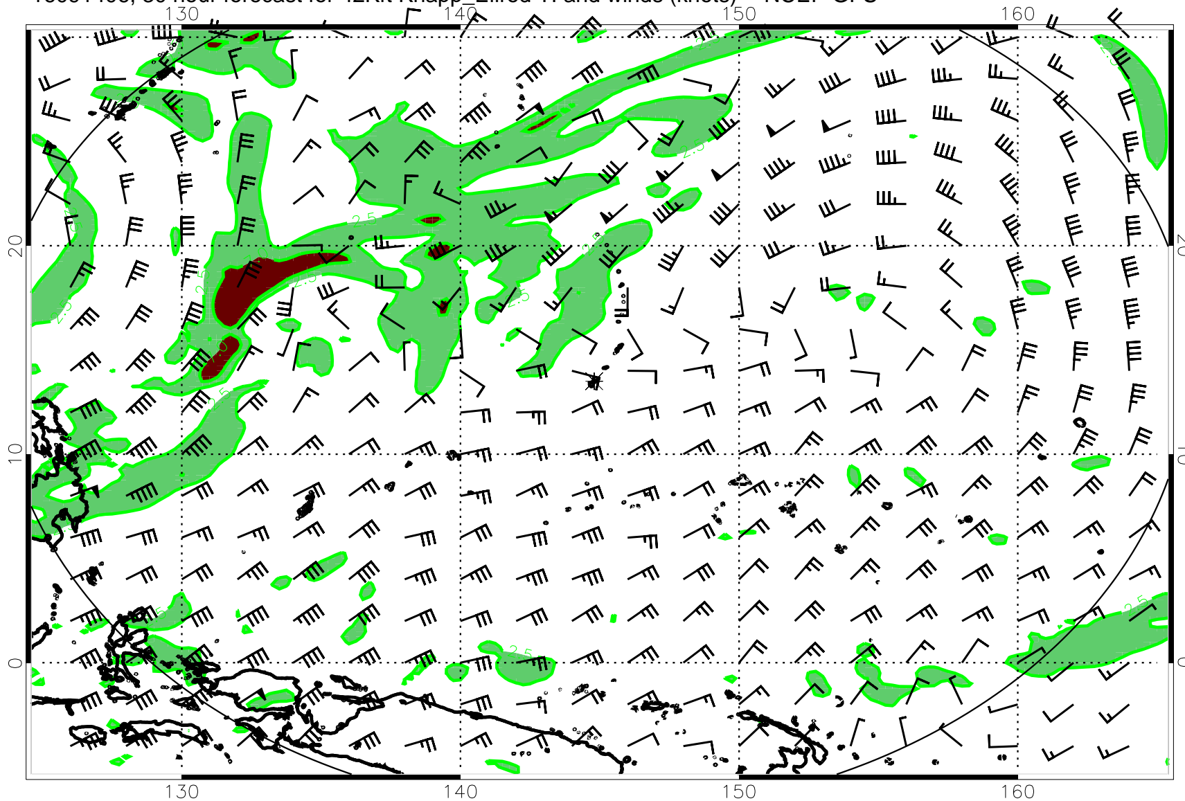
16091406, 30 hour forecast for 42Kft Knapp_Ellrod TI and winds (knots) -- NCEP GFS
