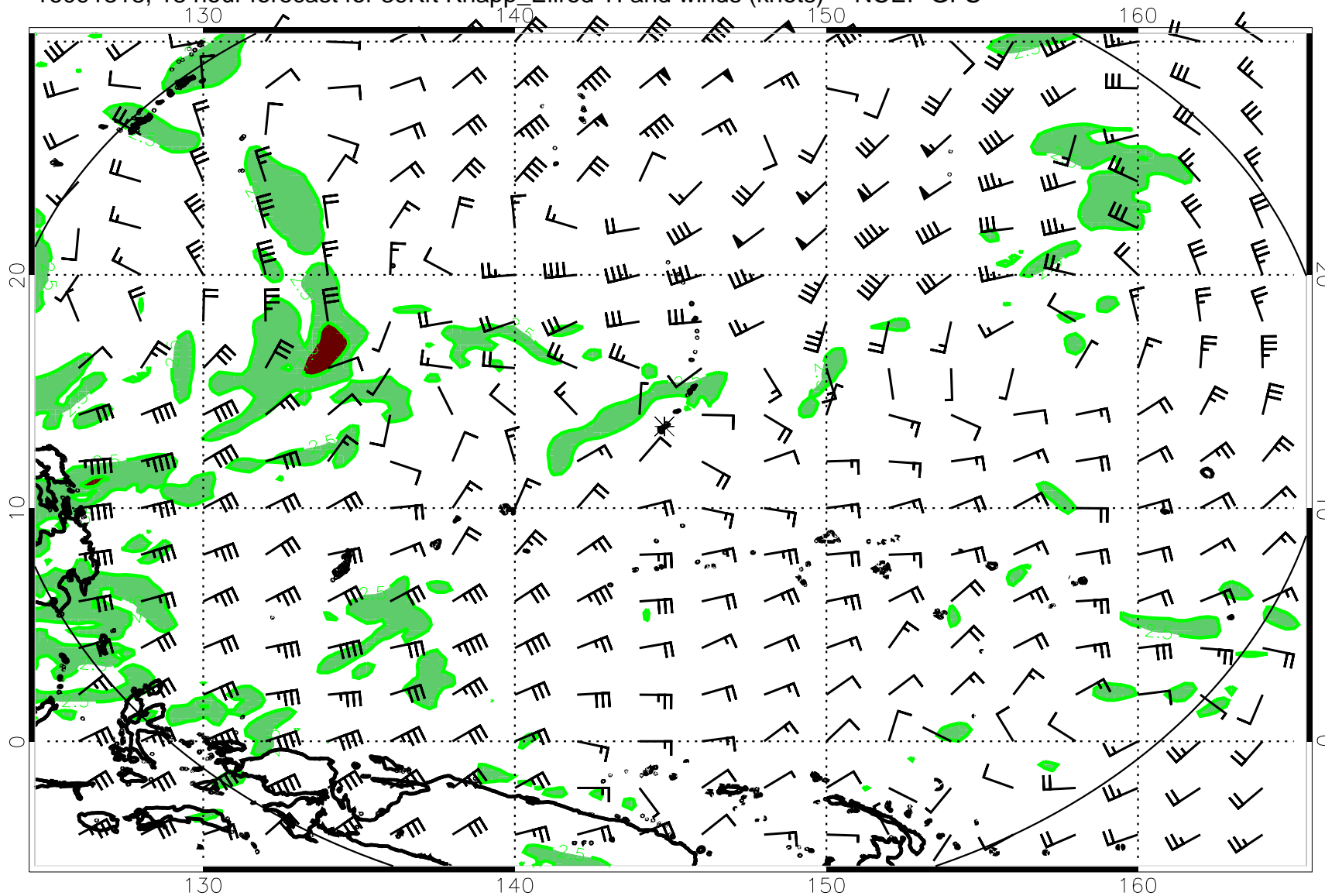
16091318, 18 hour forecast for 39Kft Knapp_Ellrod TI and winds (knots) -- NCEP GFS
