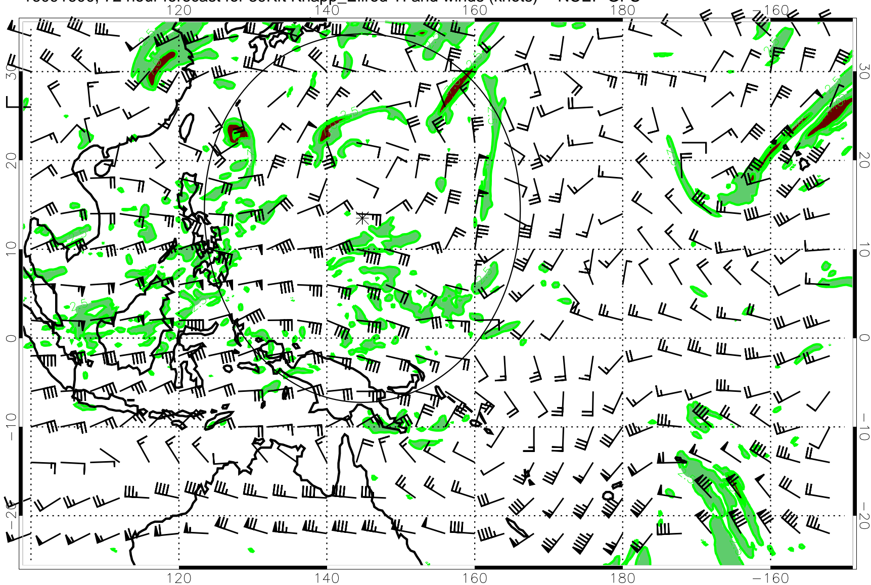
16091600, 72 hour forecast for 39Kft Knapp_Ellrod TI and winds (knots) -- NCEP GFS
