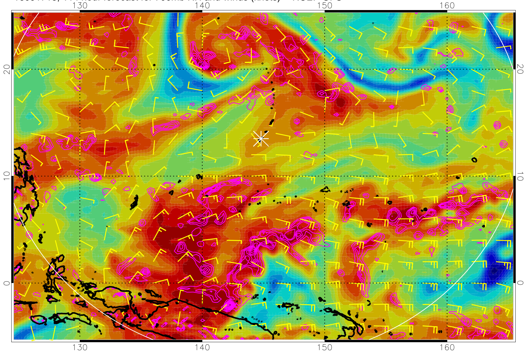
16091718, 114 hour forecast for 700mb RH and winds (knots) -- NCEP GFS
