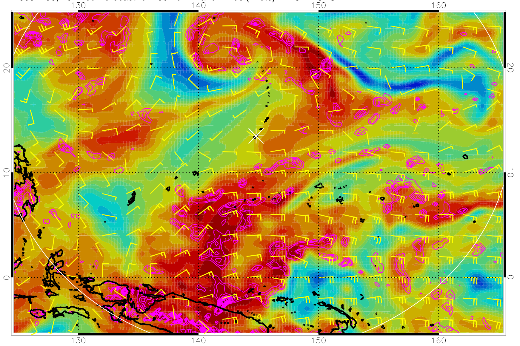
16091706, 102 hour forecast for 700mb RH and winds (knots) -- NCEP GFS
