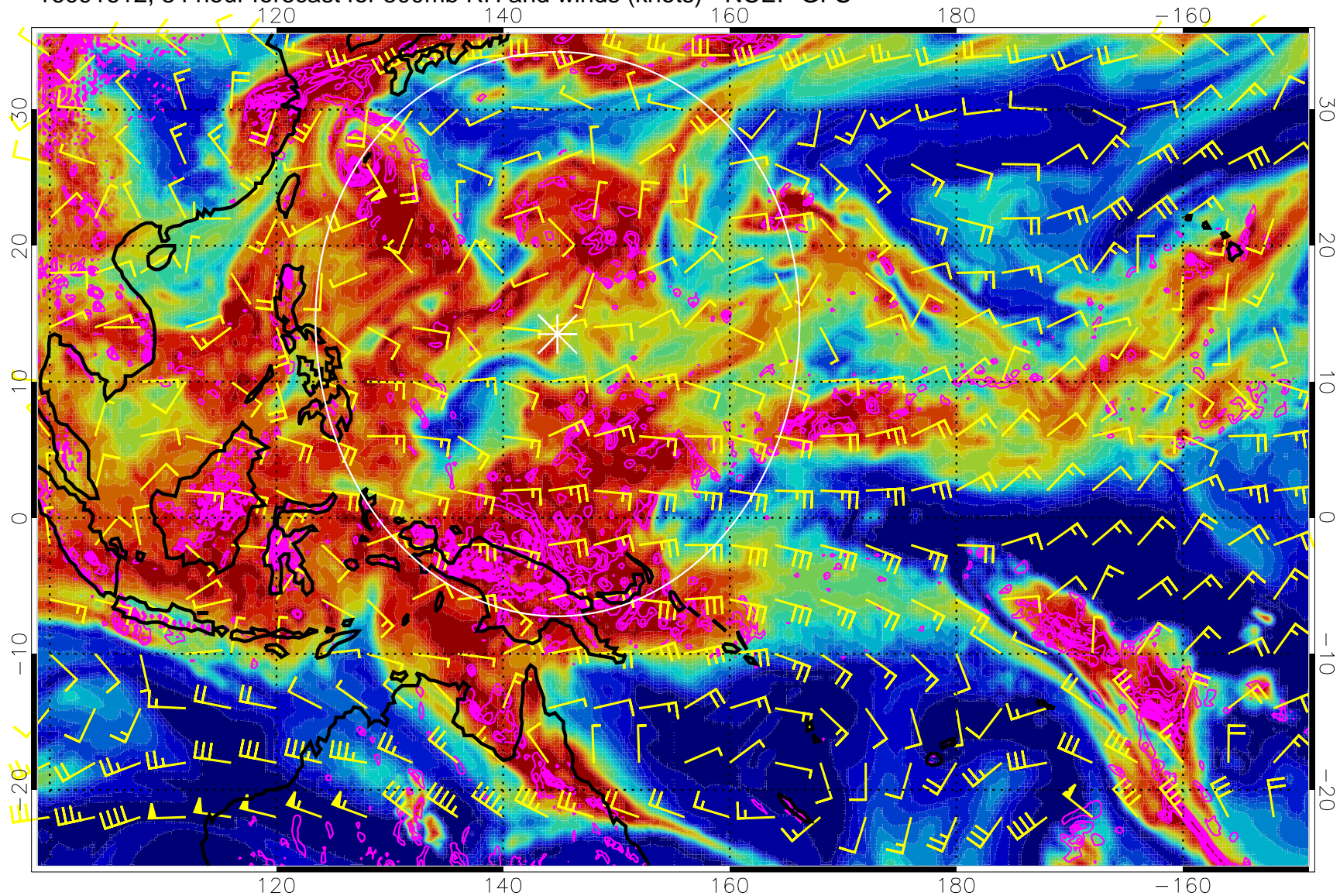
16091612, 84 hour forecast for 500mb RH and winds (knots) - NCEP GFS
