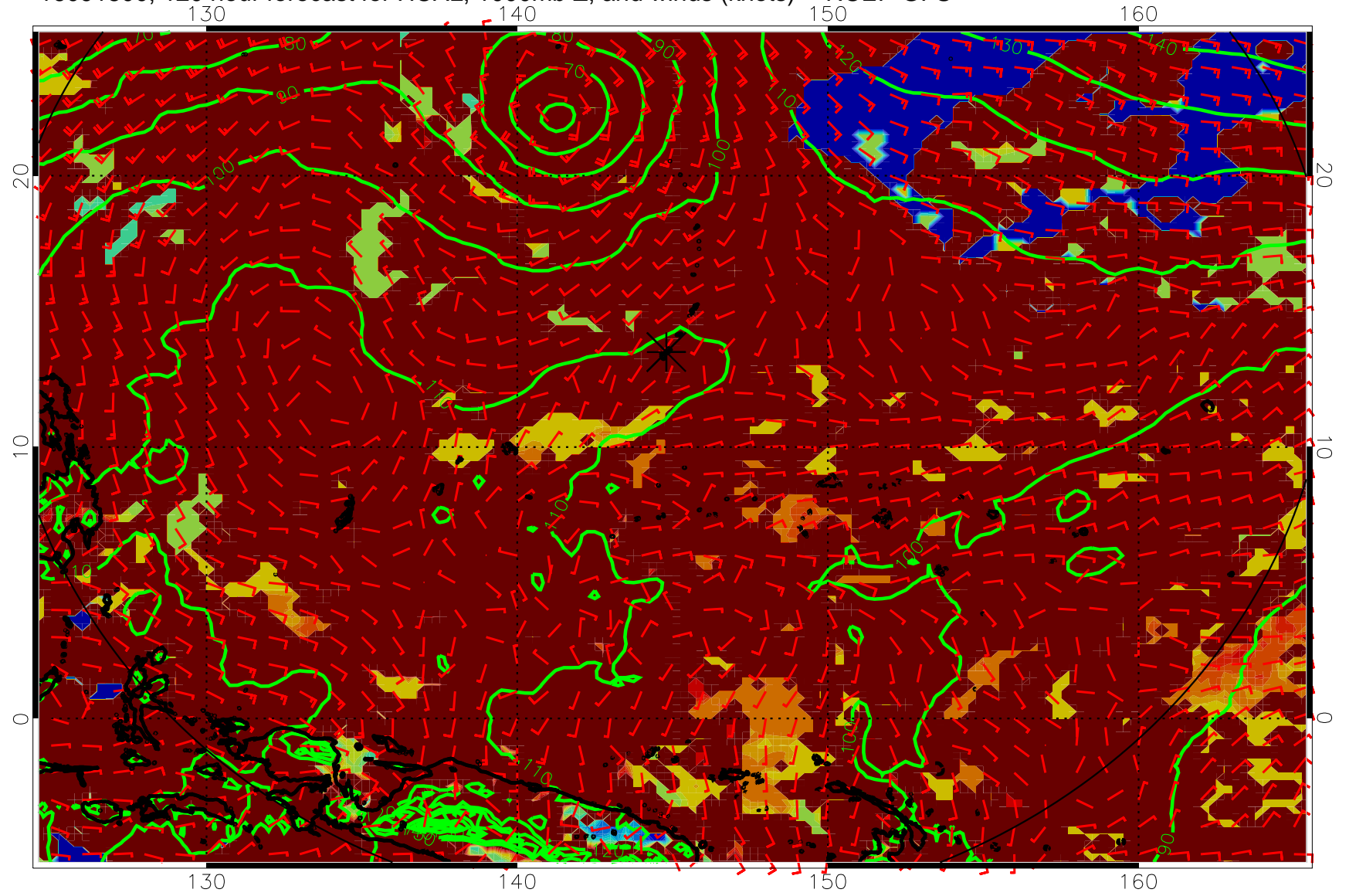
16091800, 120 hour forecast for HCAL, 1000mb Z, and winds (knots) -- NCEP GFS
