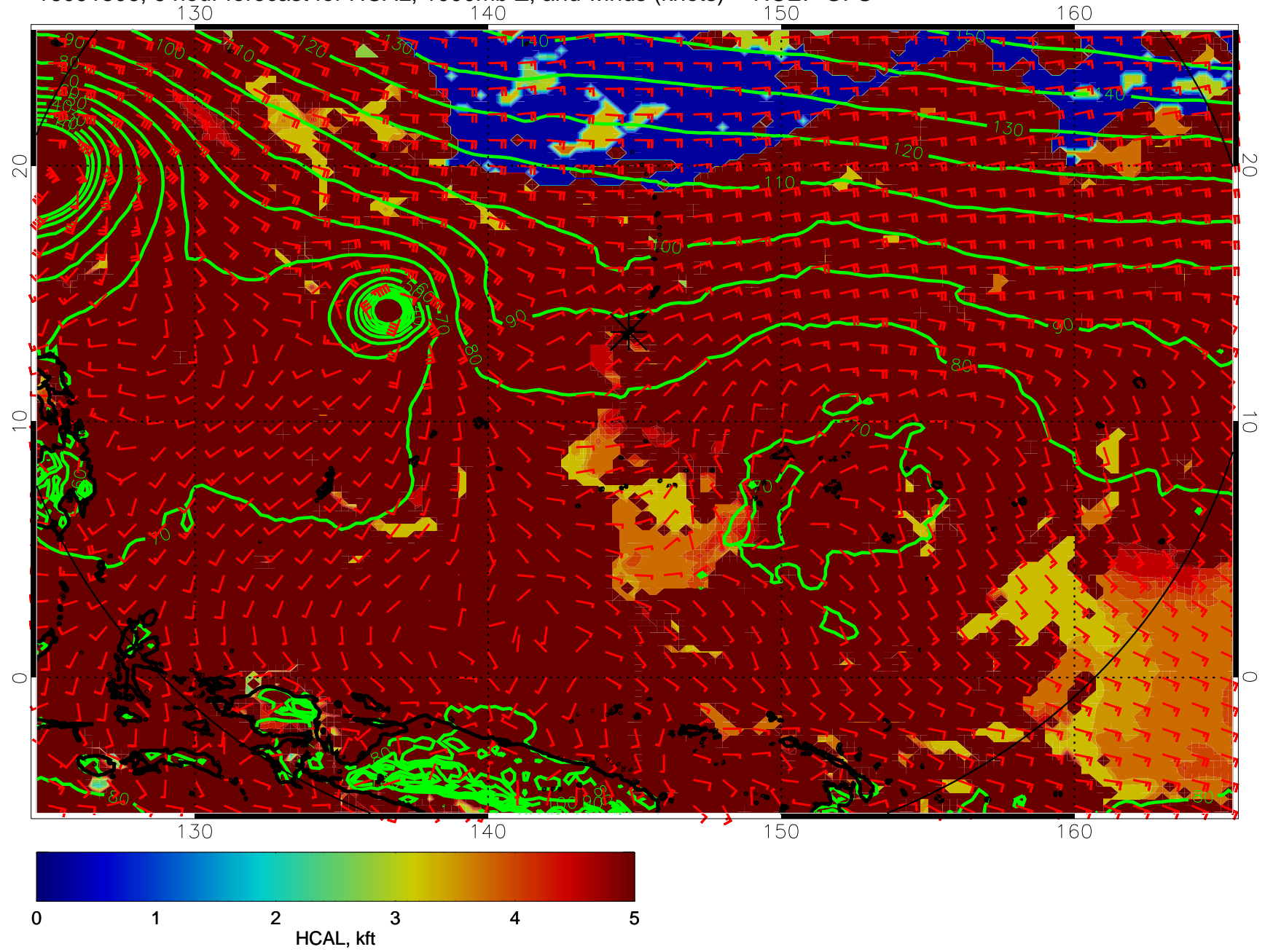
16091306, 6 hour forecast for HCAL, 1000mb Z, and winds (knots) -- NCEP GFS
