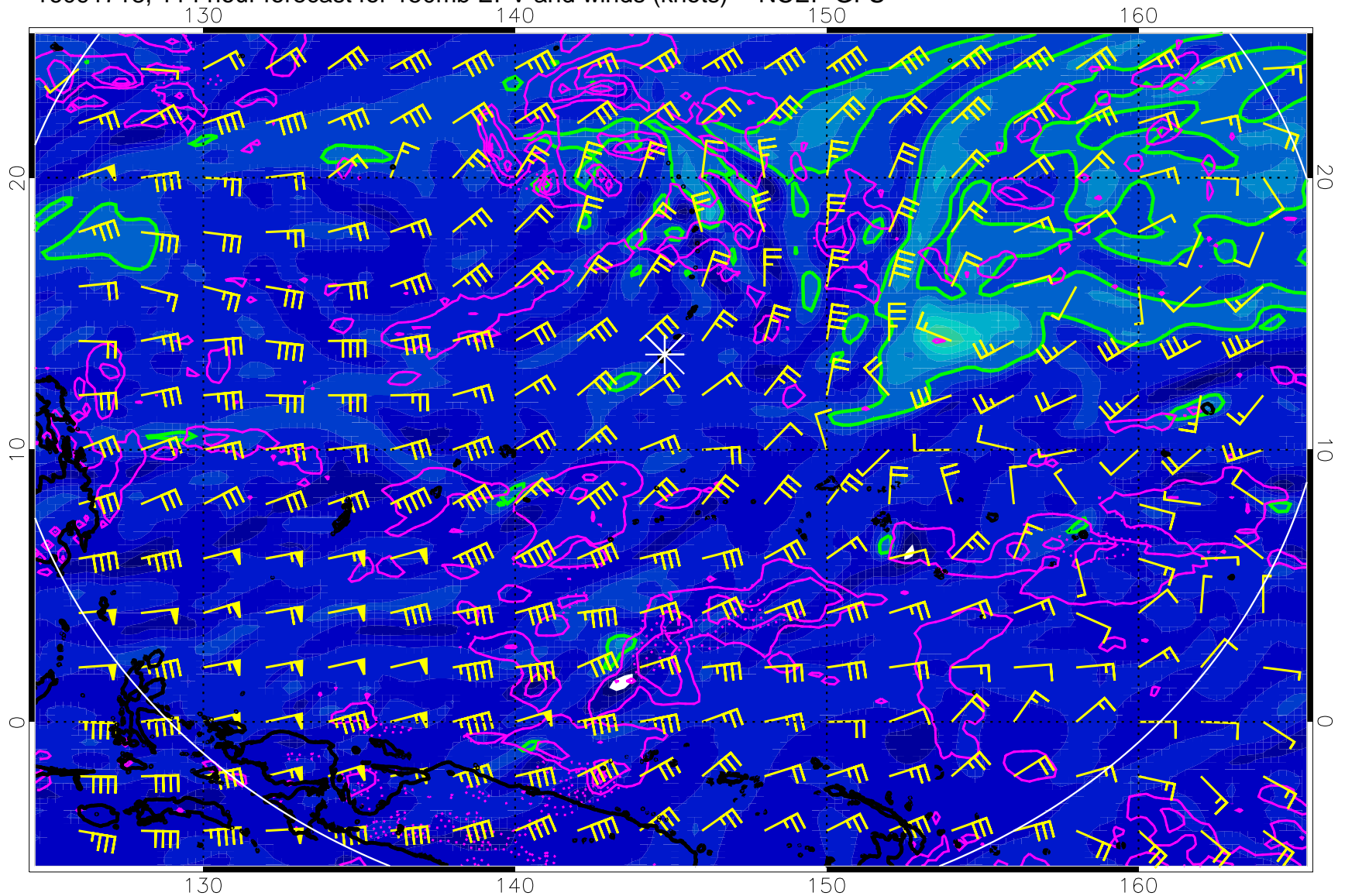
16091718, 114 hour forecast for 150mb EPV and winds (knots) -- NCEP GFS
