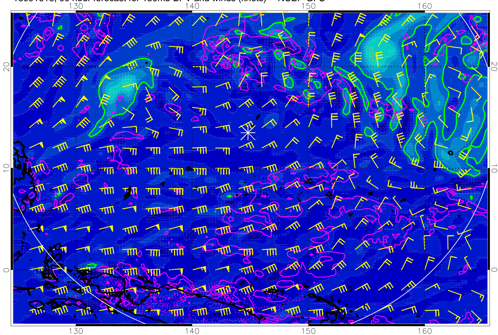
16091618, 90 hour forecast for 150mb EPV and winds (knots) -- NCEP GFS
