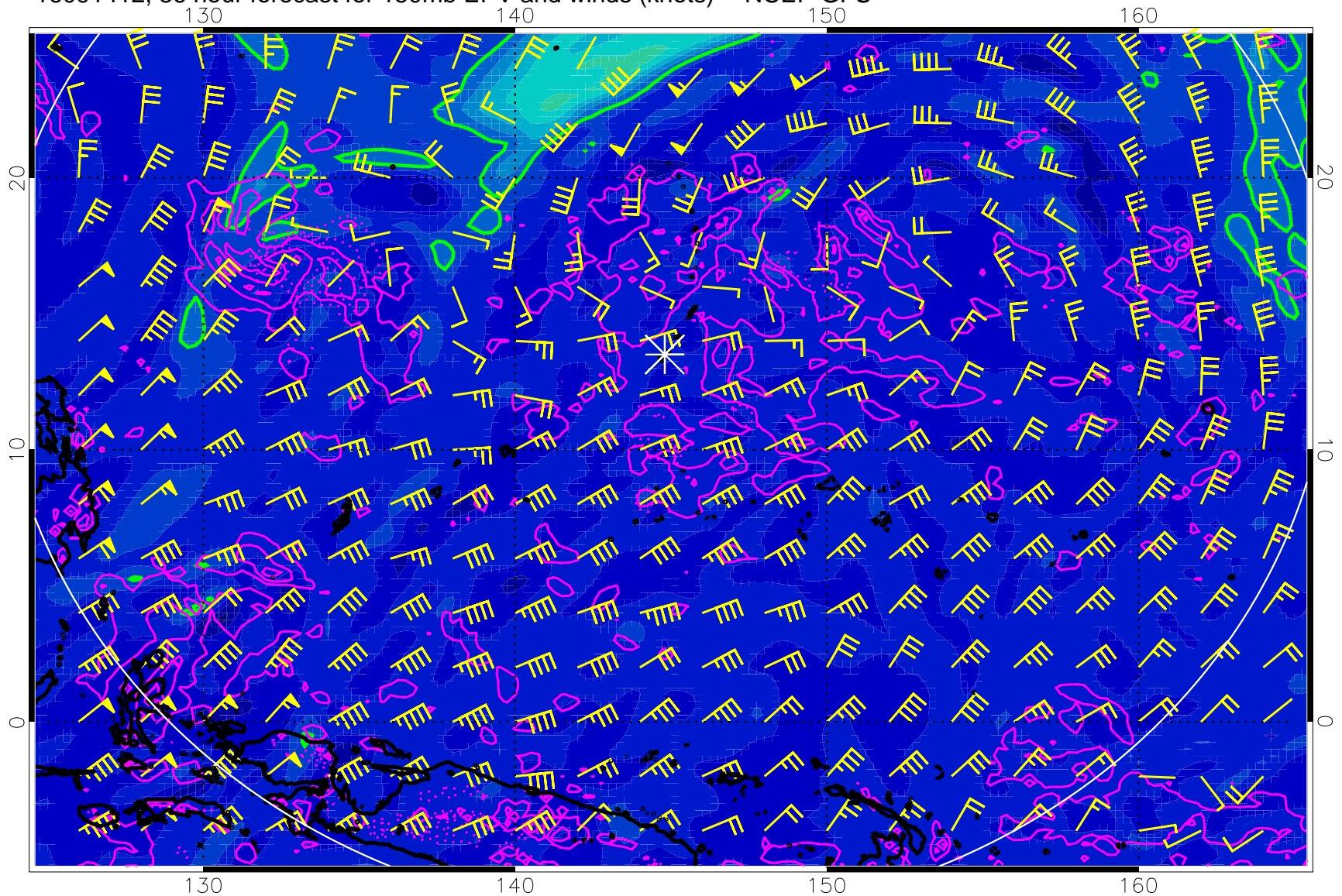
16091412, 36 hour forecast for 150mb EPV and winds (knots) -- NCEP GFS
