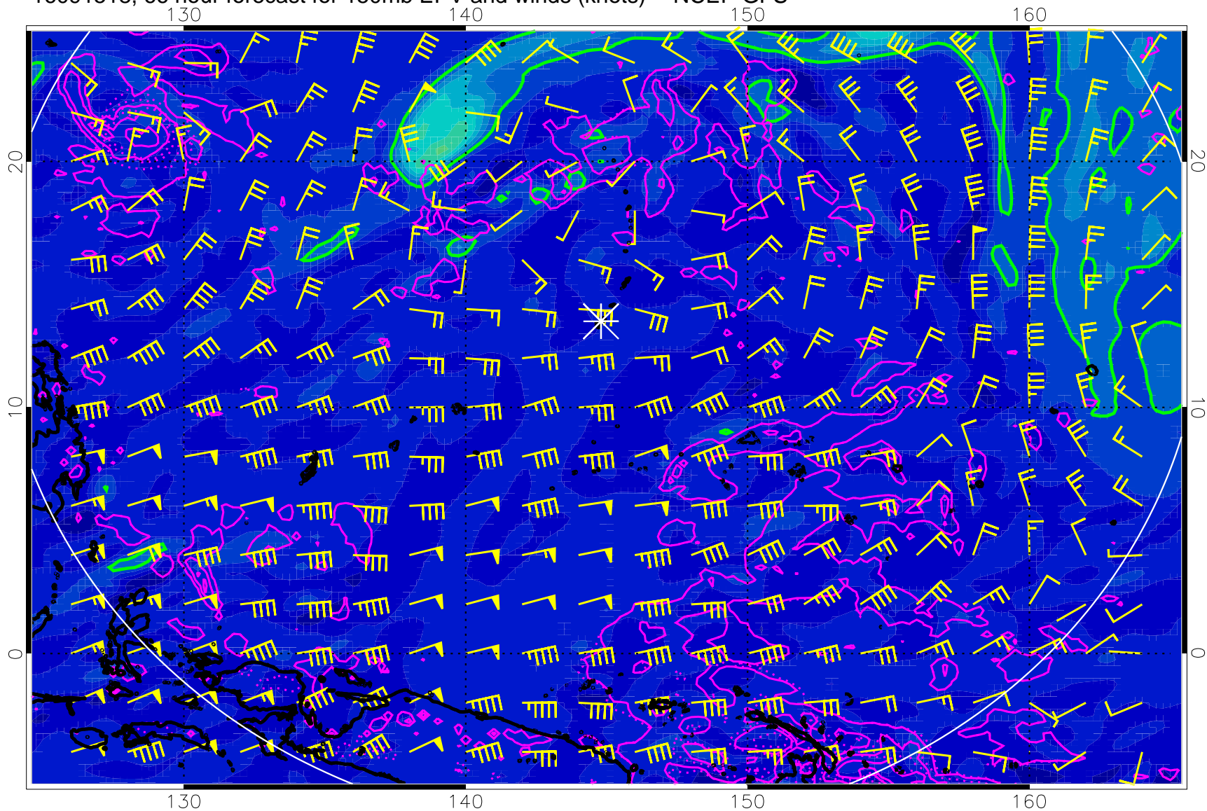
16091518, 66 hour forecast for 150mb EPV and winds (knots) -- NCEP GFS
