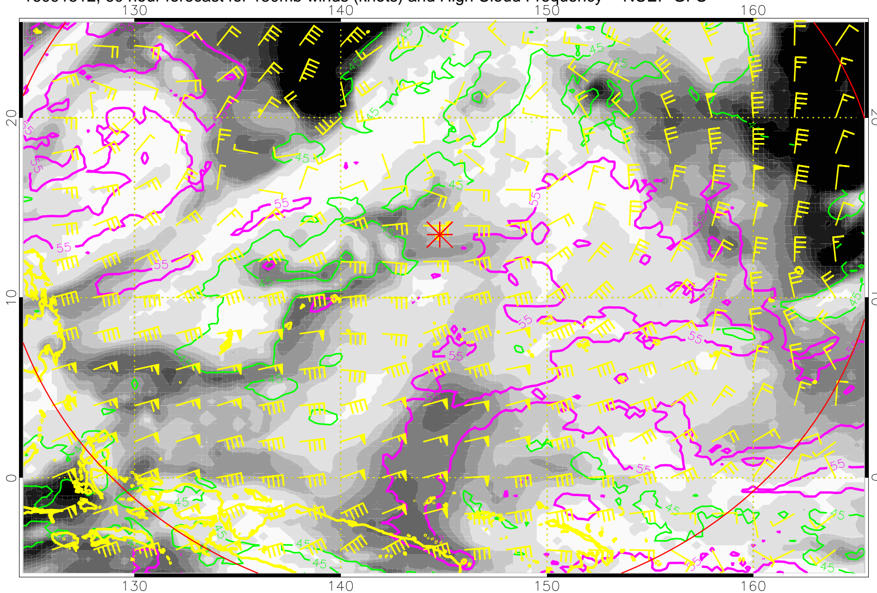
16091512, 60 hour forecast for 150mb winds (knots) and High Cloud Frequency -- NCEP GFS
