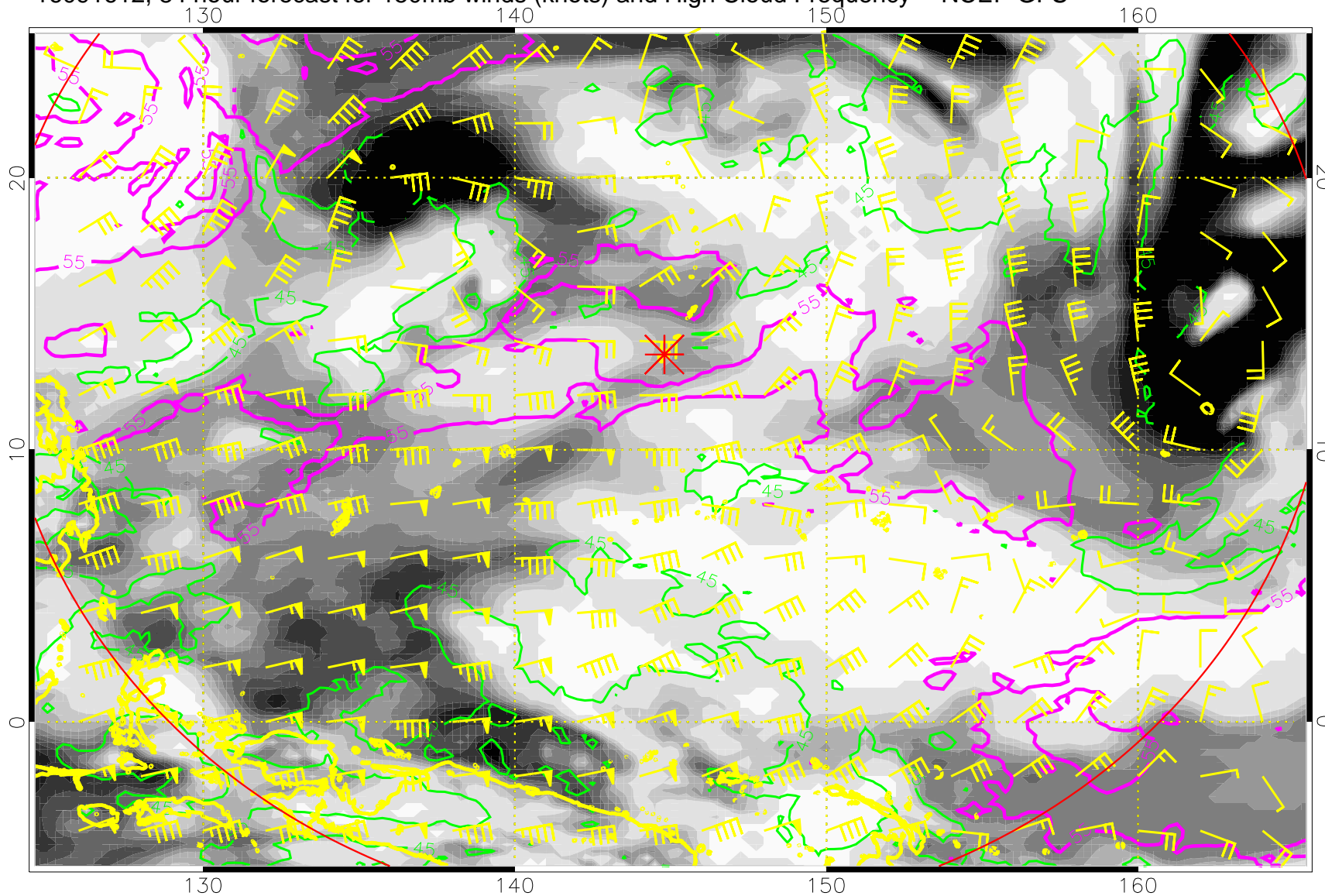
16091612, 84 hour forecast for 150mb winds (knots) and High Cloud Frequency -- NCEP GFS
