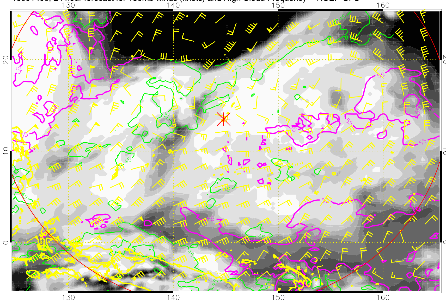
16091400, 24 hour forecast for 150mb winds (knots) and High Cloud Frequency -- NCEP GFS
