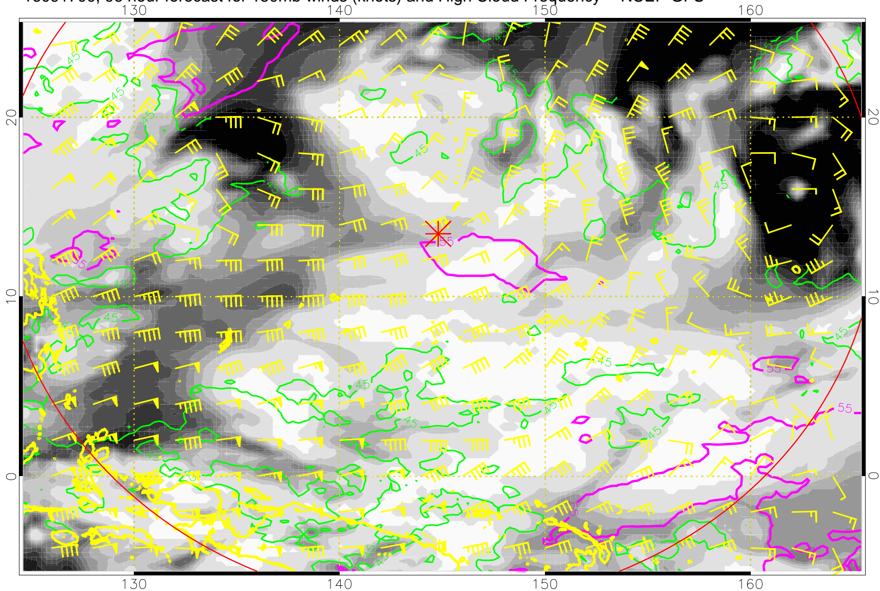
16091700, 96 hour forecast for 150mb winds (knots) and High Cloud Frequency -- NCEP GFS
