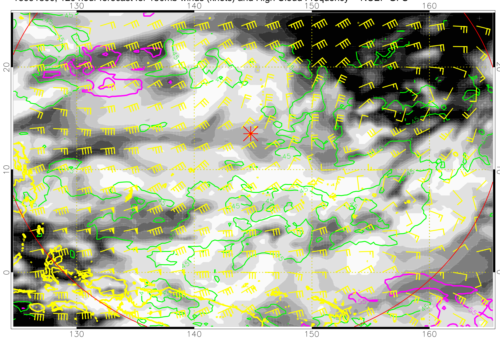
16091800, 120 hour forecast for 150mb winds (knots) and High Cloud Frequency -- NCEP GFS
