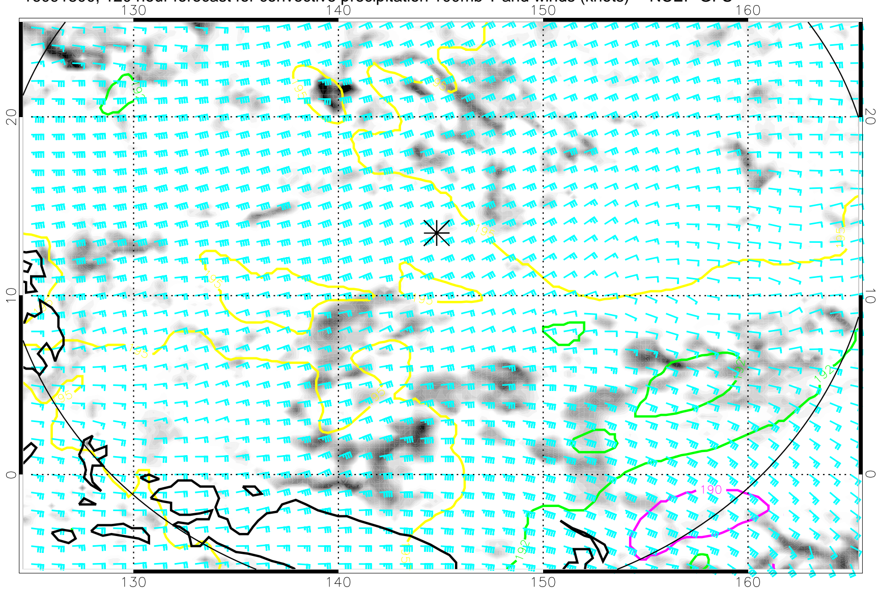
16091800, 120 hour forecast for convective precipitation 100mb T and winds (knots) -- NCEP GFS
