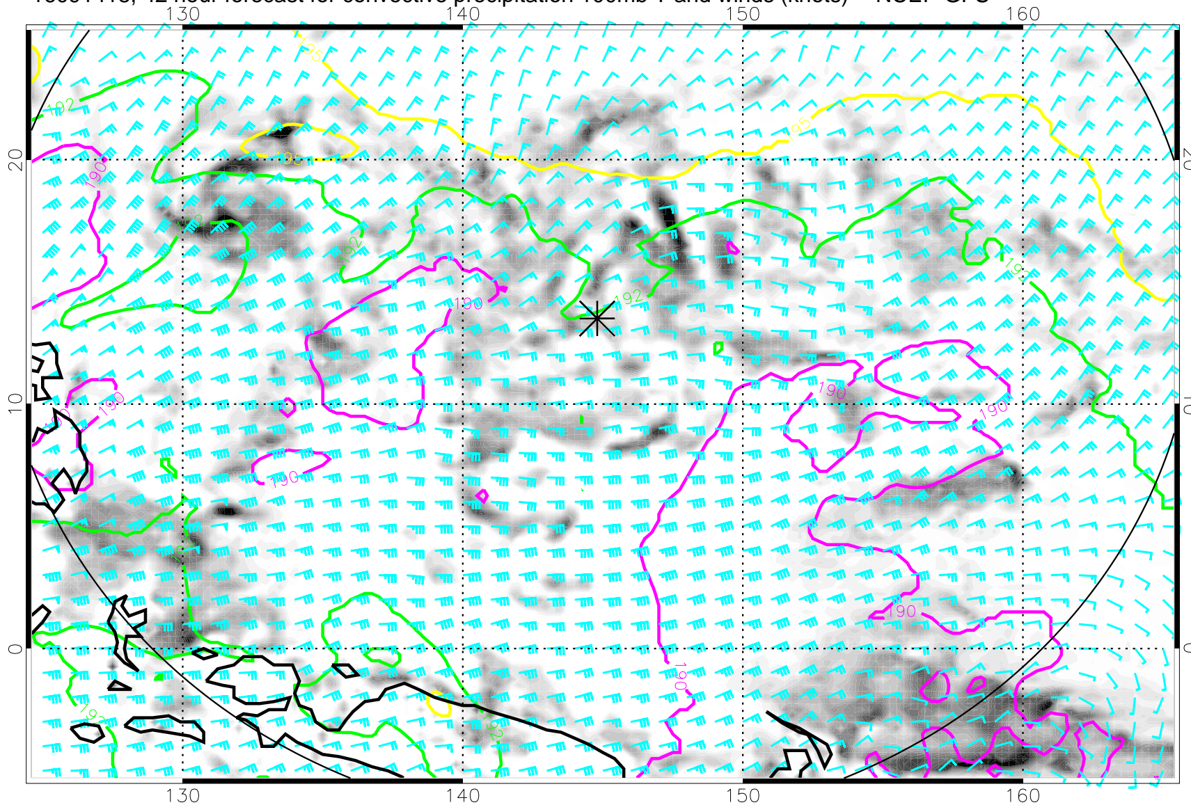
16091418, 42 hour forecast for convective precipitation 100mb T and winds (knots) -- NCEP GFS
