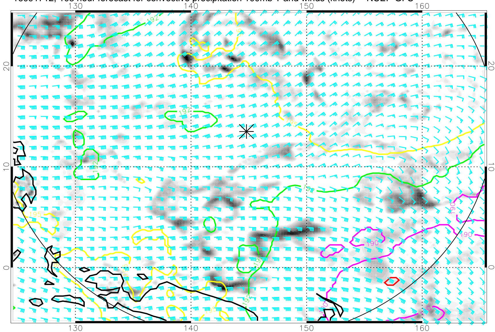
16091712, 108 hour forecast for convective precipitation 100mb T and winds (knots) -- NCEP GFS
