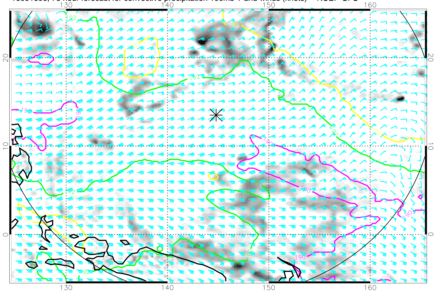
16091606, 78 hour forecast for convective precipitation 100mb T and winds (knots) -- NCEP GFS
