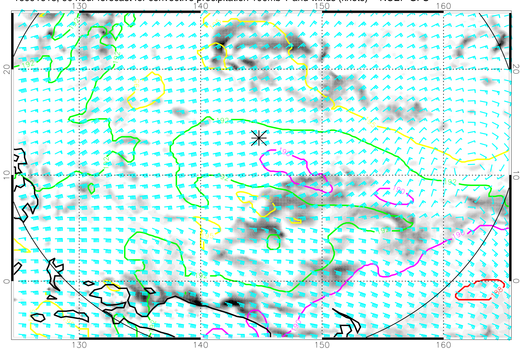
16091618, 90 hour forecast for convective precipitation 100mb T and winds (knots) -- NCEP GFS
