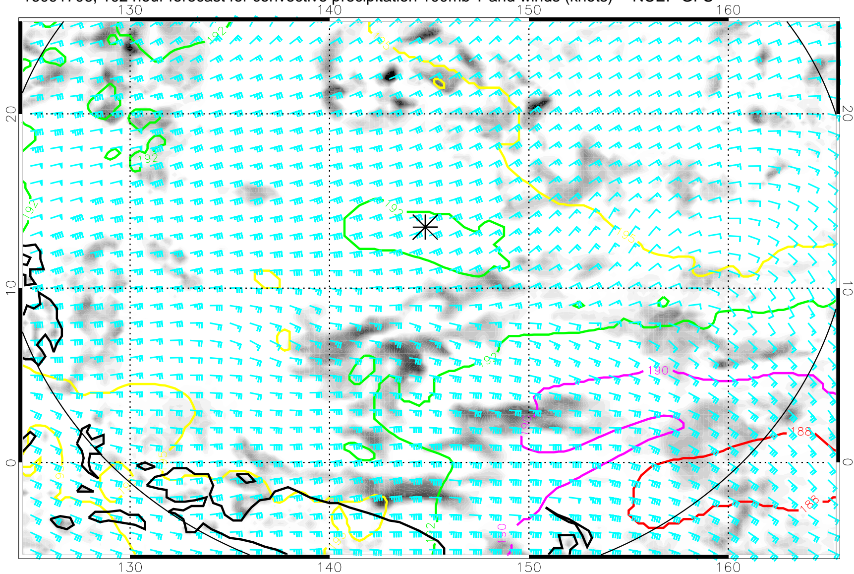
16091706, 102 hour forecast for convective precipitation 100mb T and winds (knots) -- NCEP GFS
