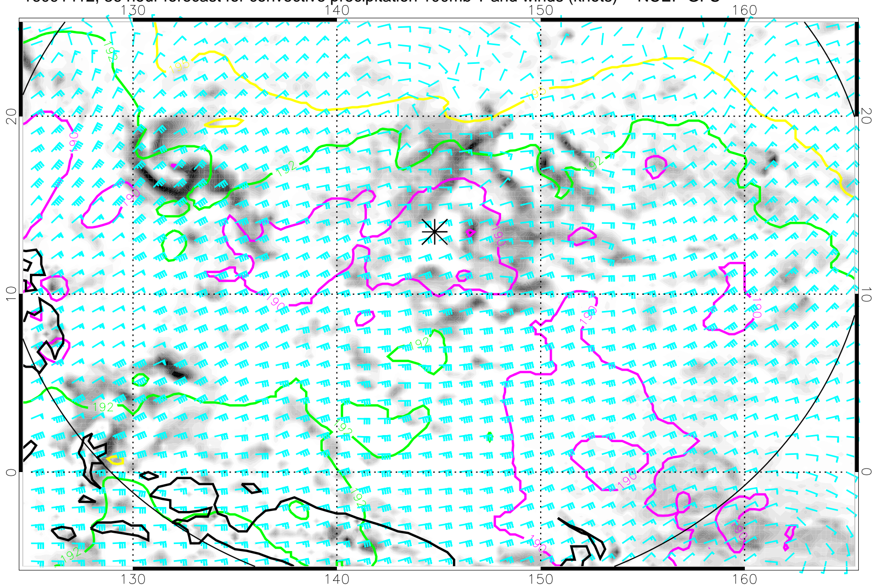
16091412, 36 hour forecast for convective precipitation 100mb T and winds (knots) -- NCEP GFS
