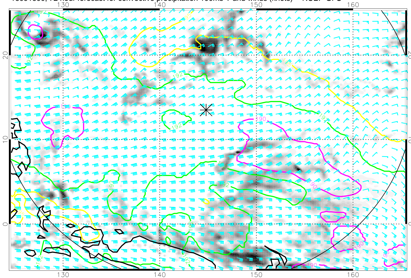
16091600, 72 hour forecast for convective precipitation 100mb T and winds (knots) -- NCEP GFS
