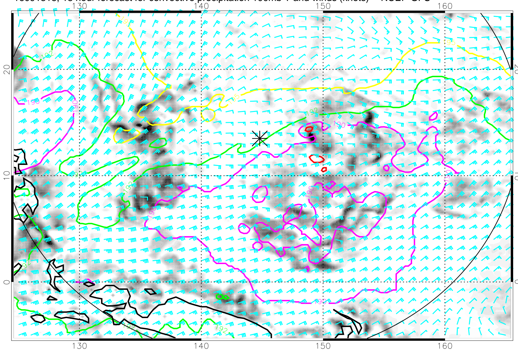
16091318, 18 hour forecast for convective precipitation 100mb T and winds (knots) -- NCEP GFS
