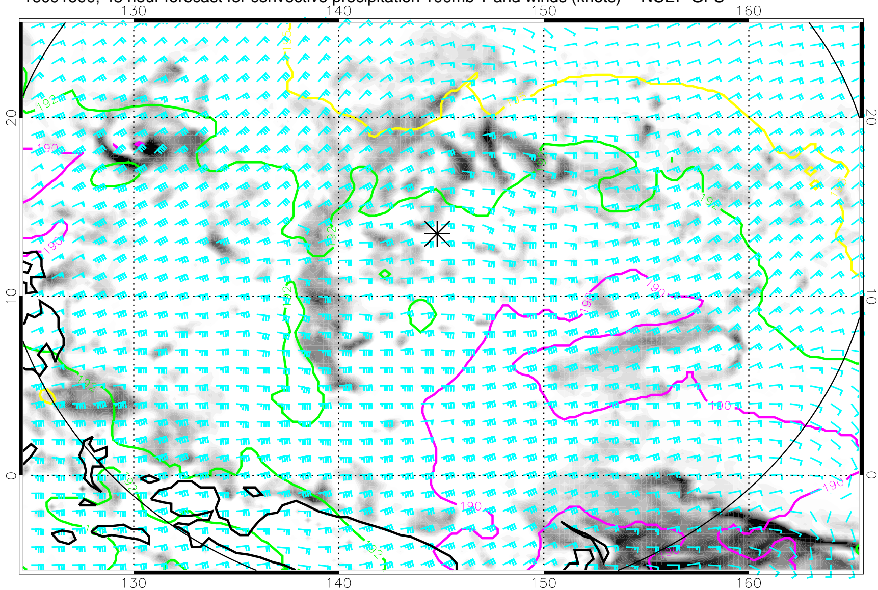
16091500, 48 hour forecast for convective precipitation 100mb T and winds (knots) -- NCEP GFS
