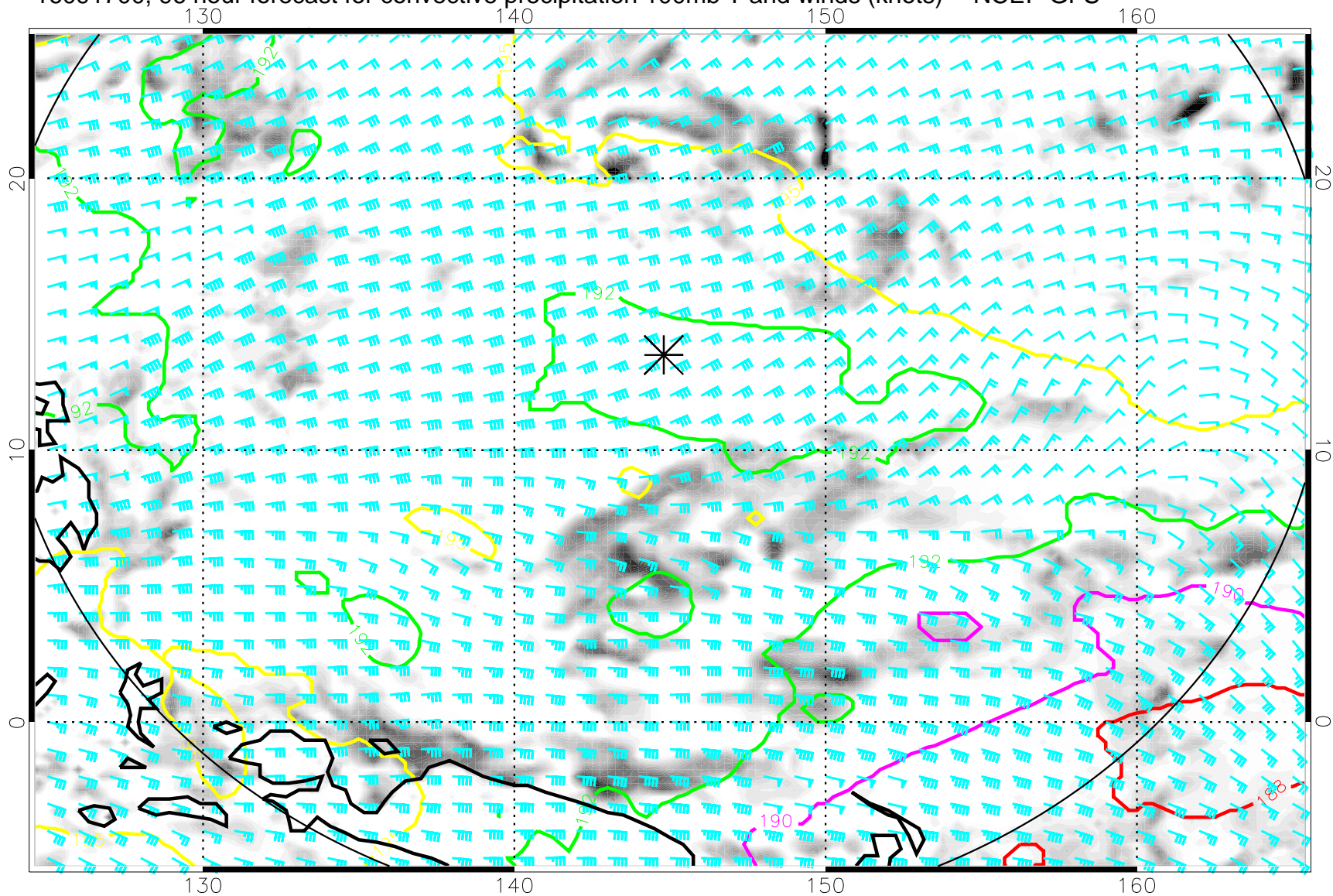
16091700, 96 hour forecast for convective precipitation 100mb T and winds (knots) -- NCEP GFS
