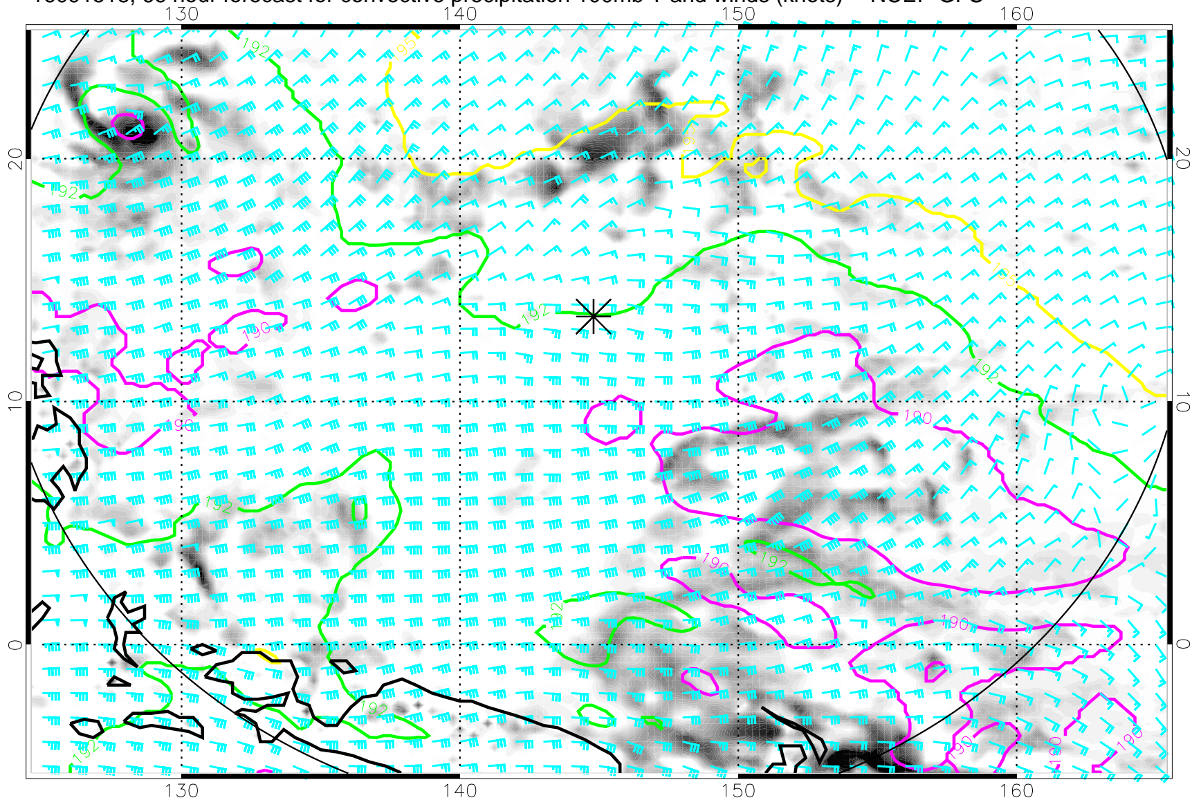
16091518, 66 hour forecast for convective precipitation 100mb T and winds (knots) -- NCEP GFS
