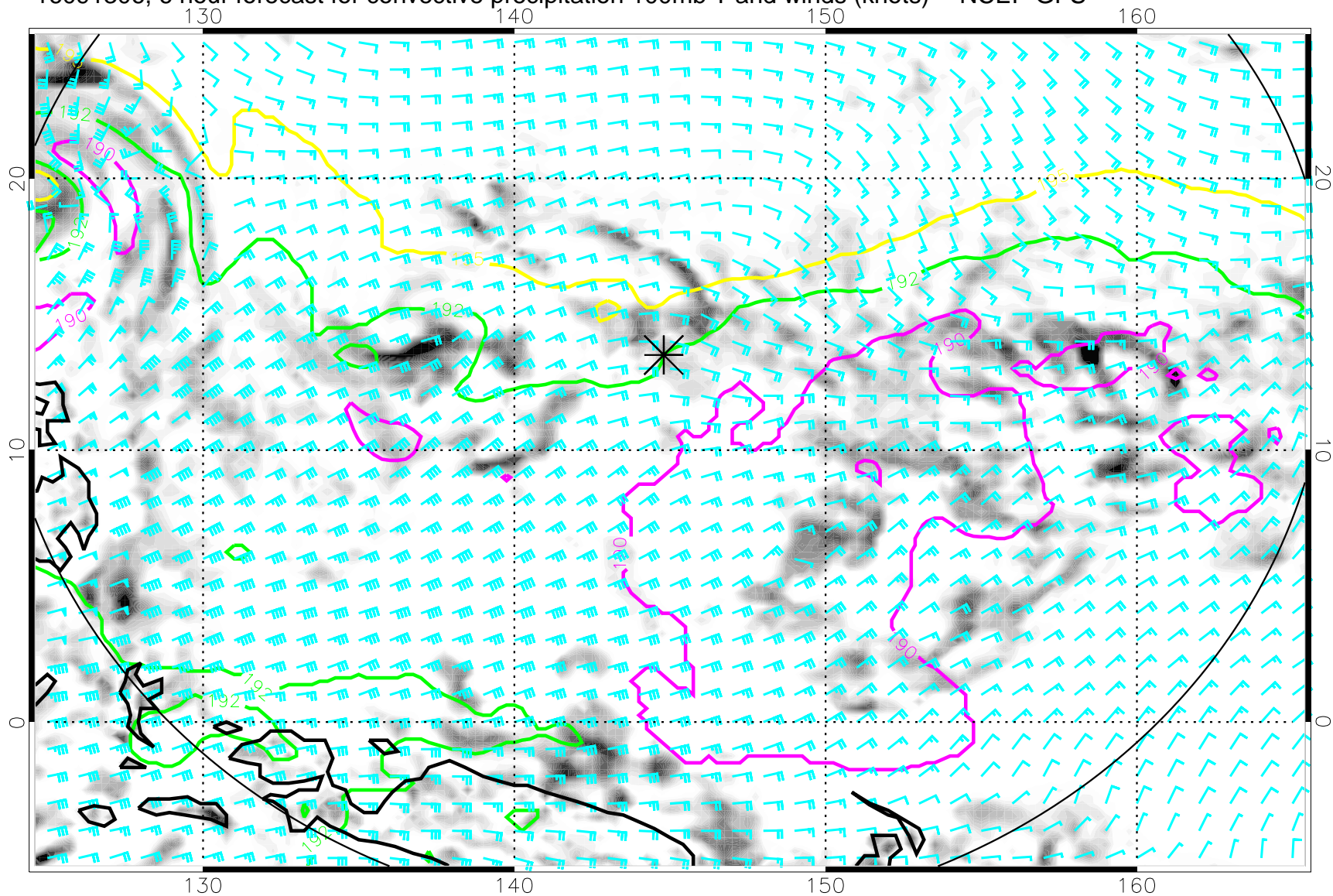
16091306, 6 hour forecast for convective precipitation 100mb T and winds (knots) -- NCEP GFS
