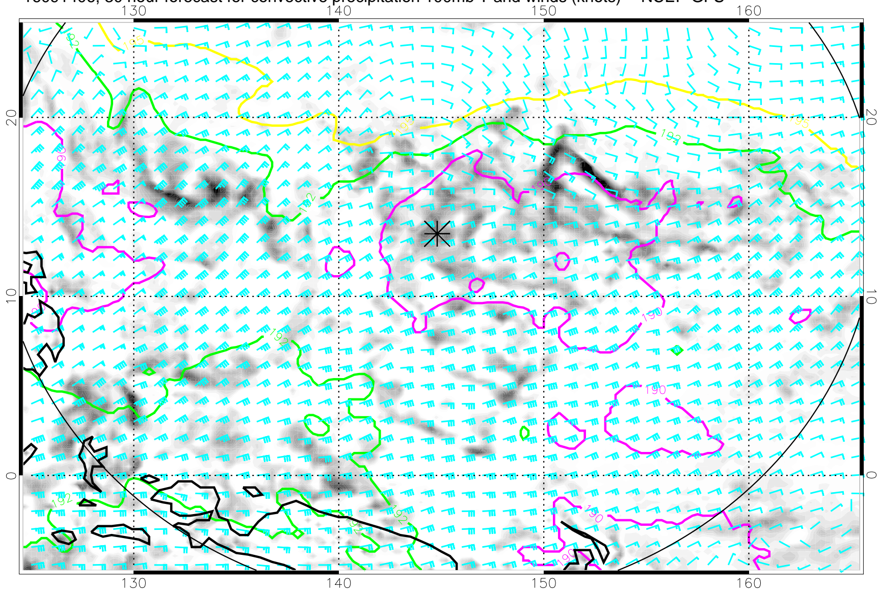
16091406, 30 hour forecast for convective precipitation 100mb T and winds (knots) -- NCEP GFS
