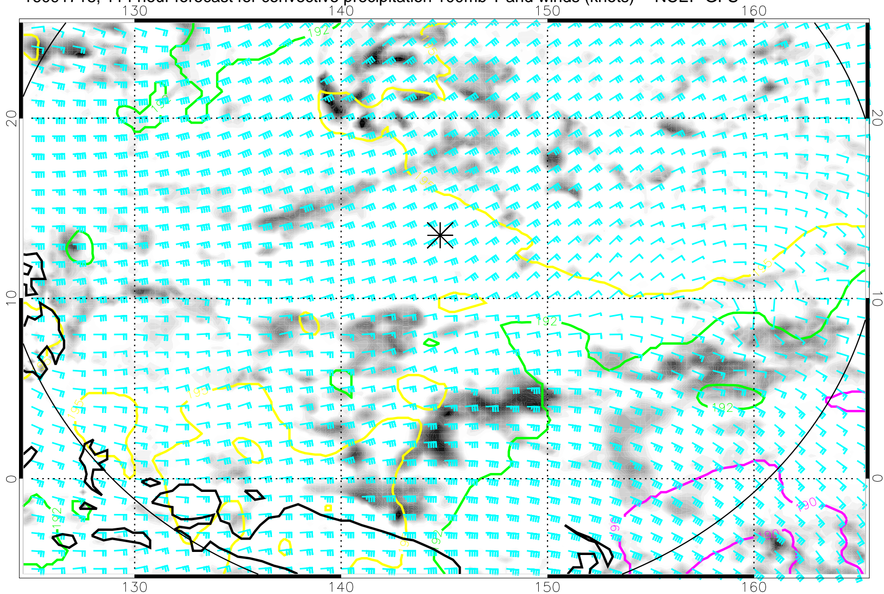
16091718, 114 hour forecast for convective precipitation 100mb T and winds (knots) -- NCEP GFS
