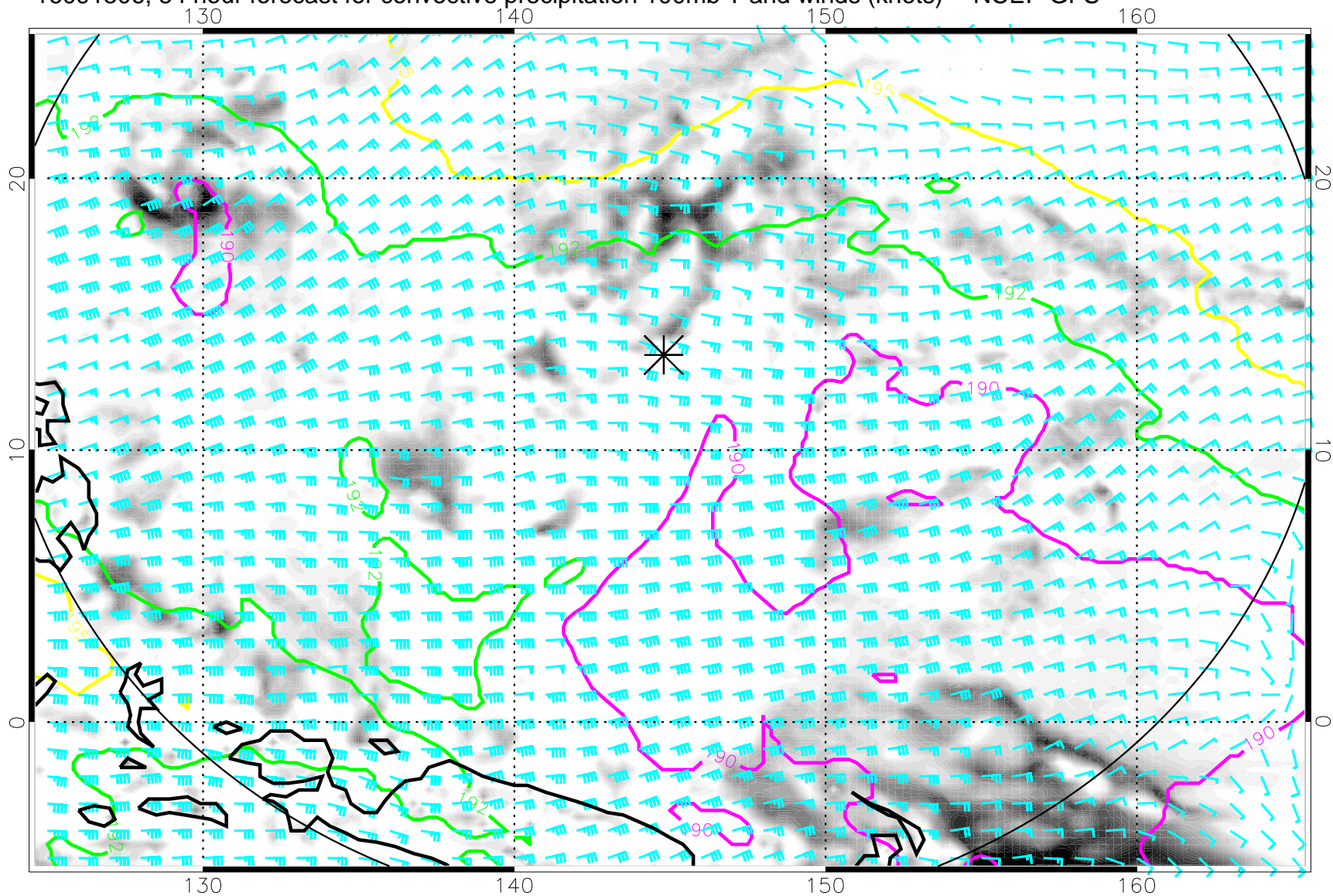
16091506, 54 hour forecast for convective precipitation 100mb T and winds (knots) -- NCEP GFS
