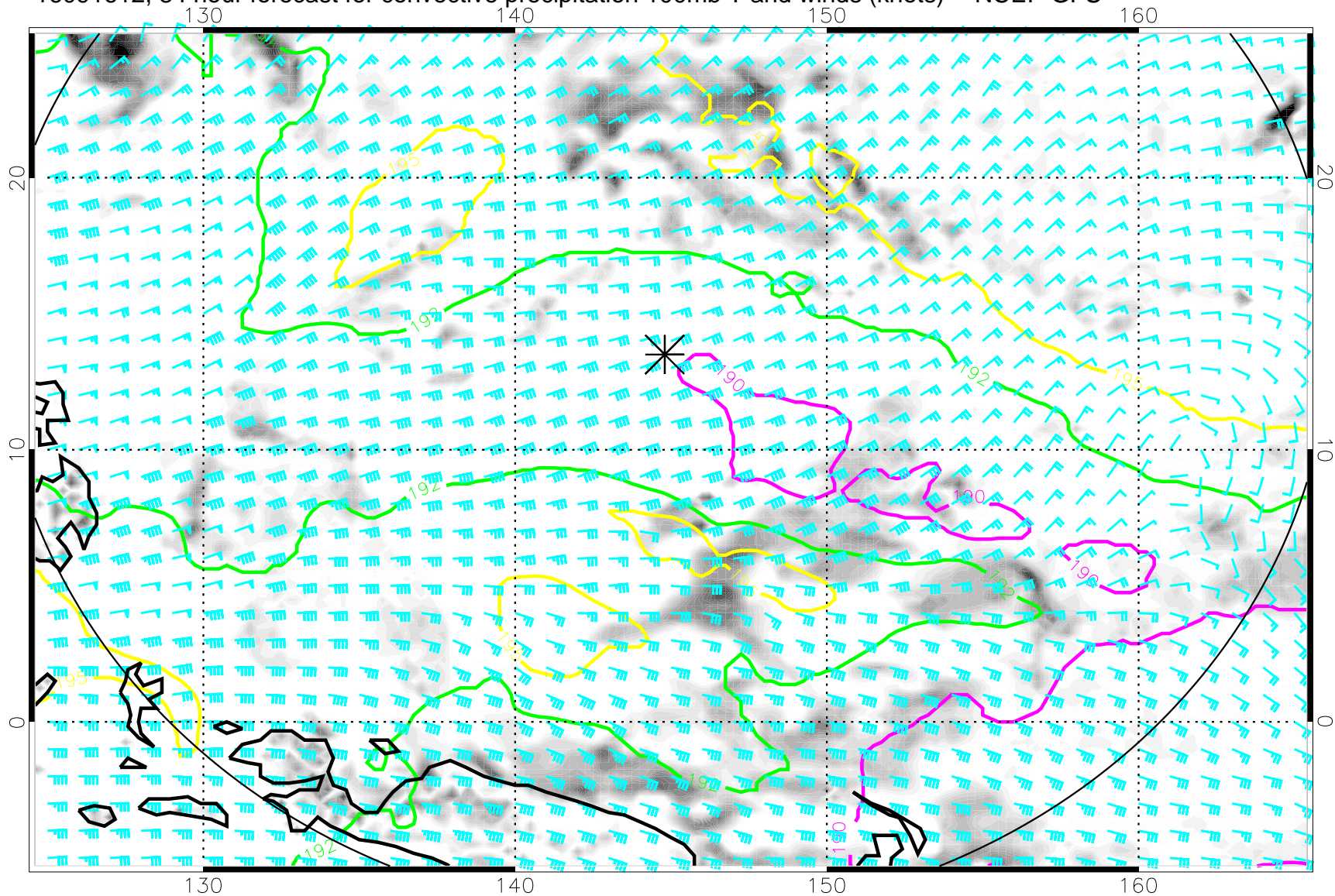
16091612, 84 hour forecast for convective precipitation 100mb T and winds (knots) -- NCEP GFS
