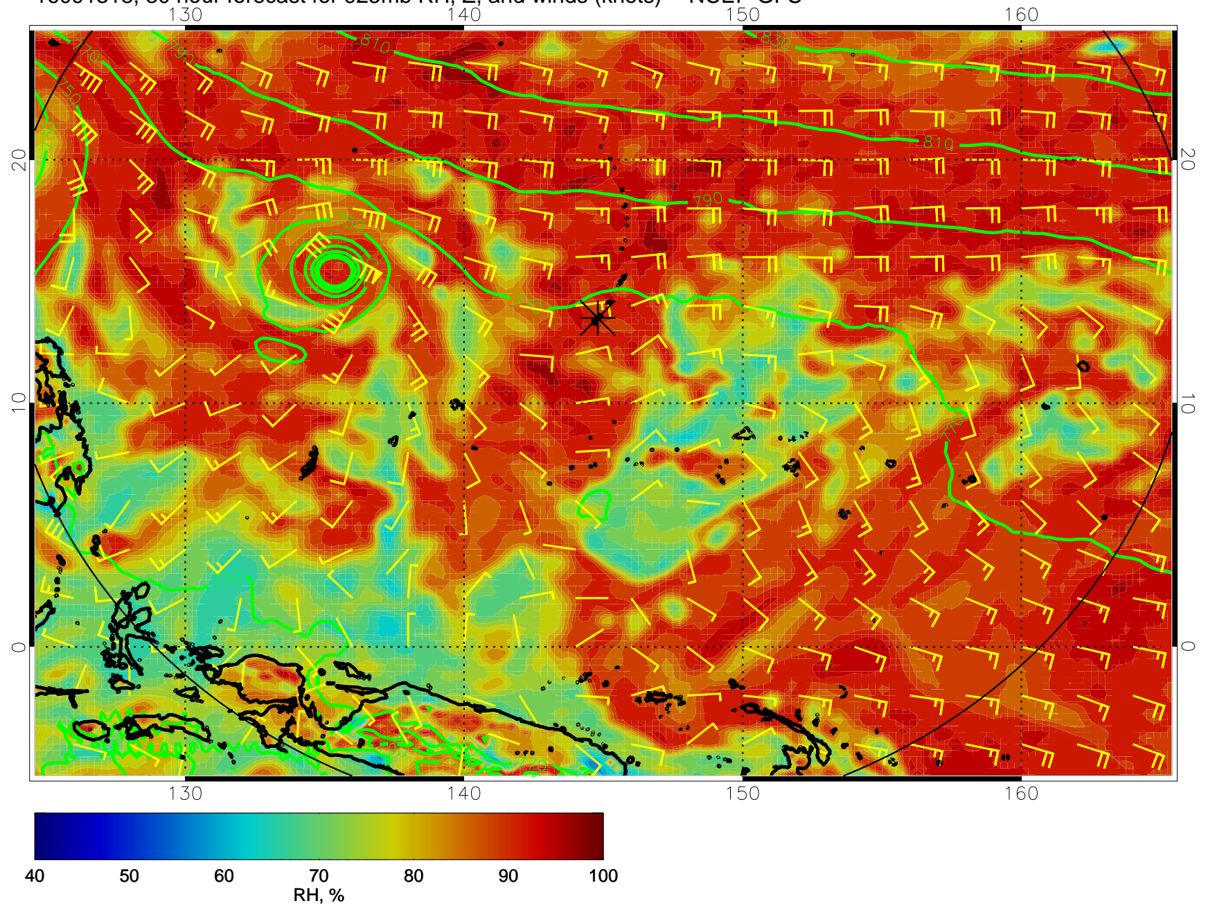
16091318, 30 hour forecast for 925mb RH, Z, and winds (knots) -- NCEP GFS
