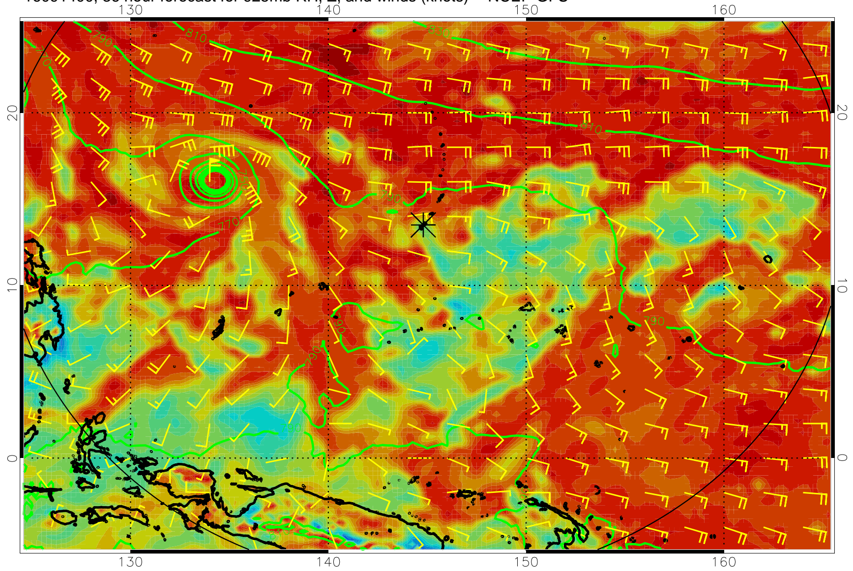
16091400, 36 hour forecast for 925mb RH, Z, and winds (knots) -- NCEP GFS
