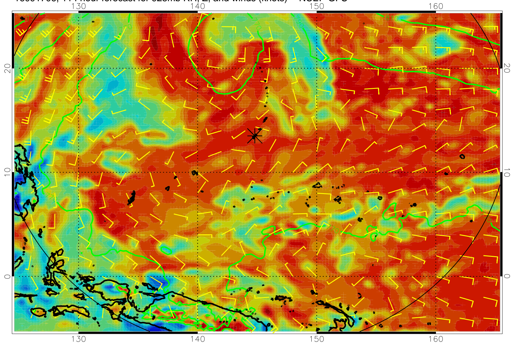
16091706, 114 hour forecast for 925mb RH, Z, and winds (knots) -- NCEP GFS
