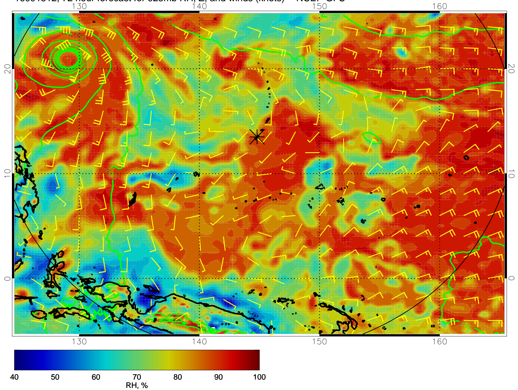
16091512, 72 hour forecast for 925mb RH, Z, and winds (knots) -- NCEP GFS
