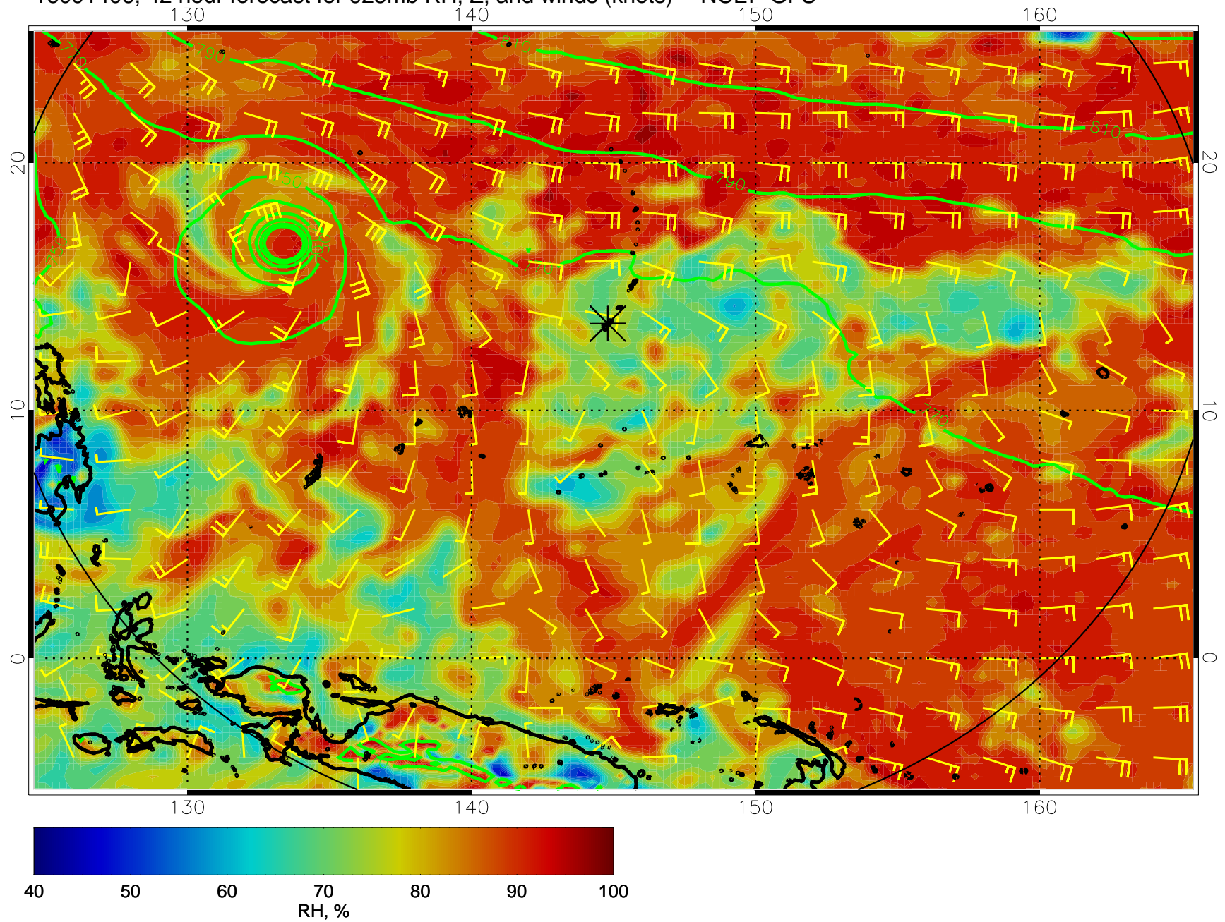
16091406, 42 hour forecast for 925mb RH, Z, and winds (knots) -- NCEP GFS
