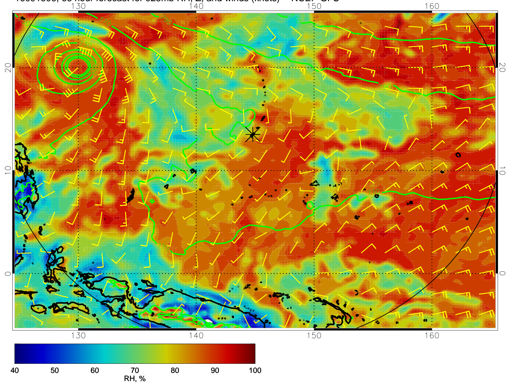
16091506, 66 hour forecast for 925mb RH, Z, and winds (knots) -- NCEP GFS
