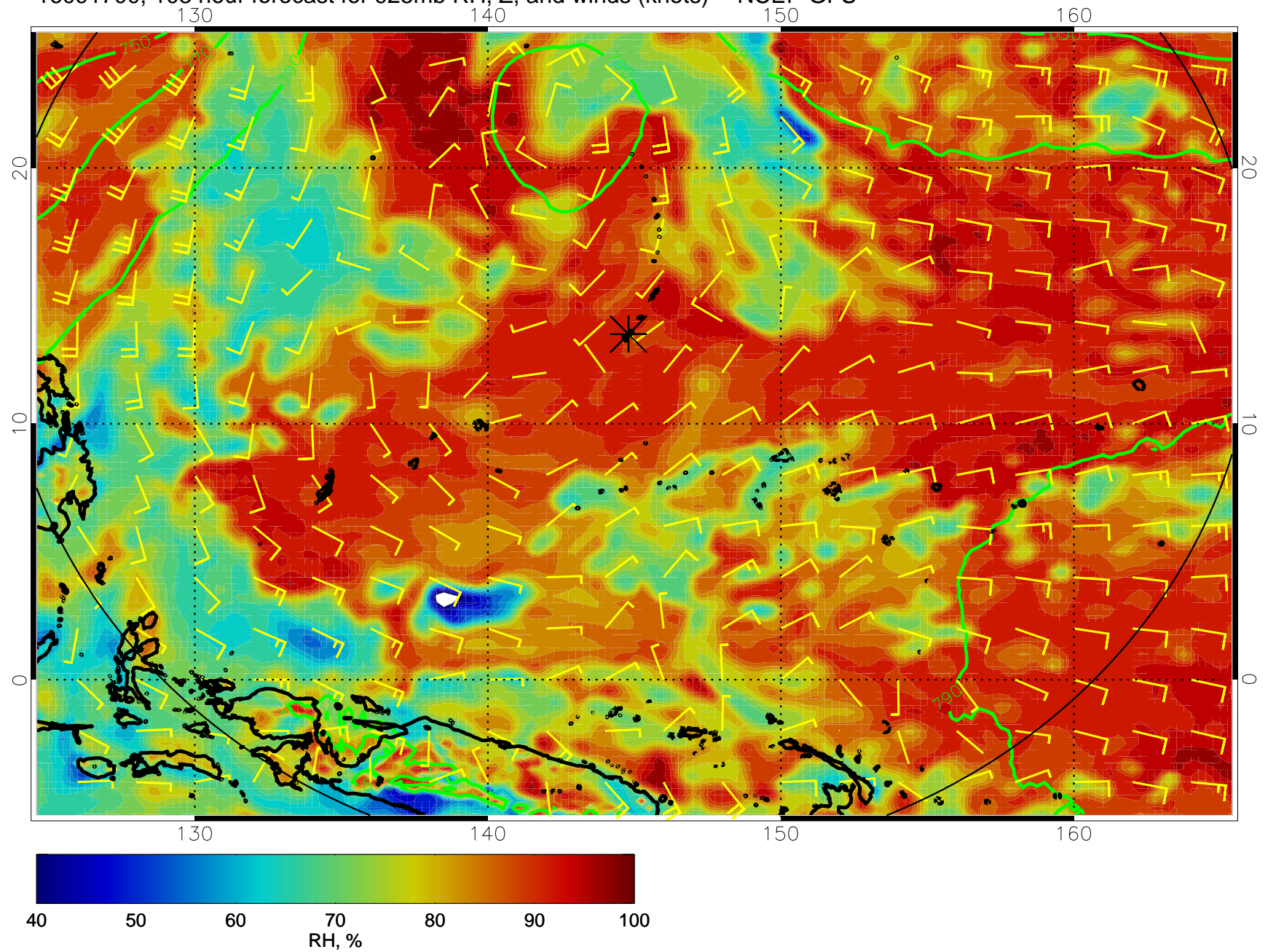
16091700, 108 hour forecast for 925mb RH, Z, and winds (knots) -- NCEP GFS
