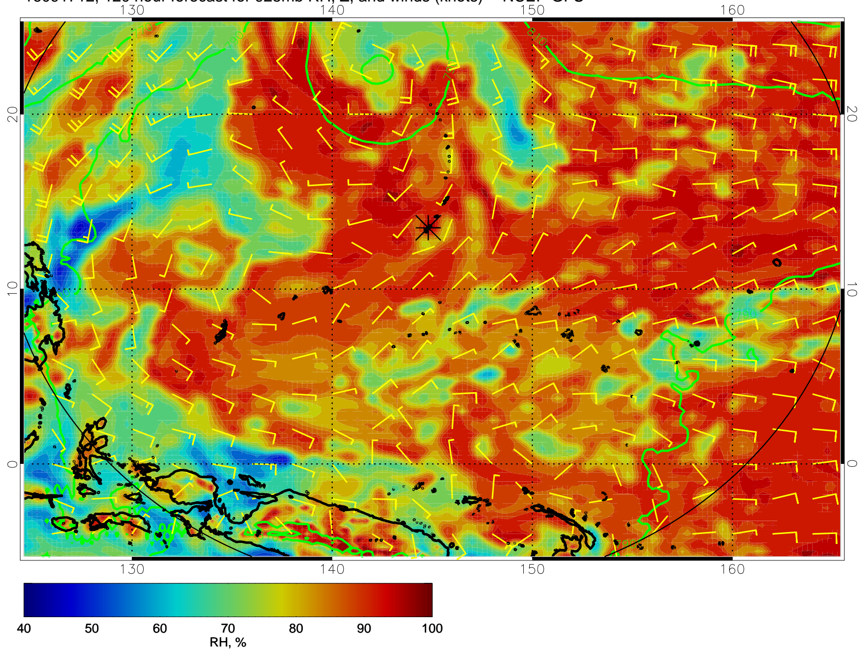
16091712, 120 hour forecast for 925mb RH, Z, and winds (knots) -- NCEP GFS
