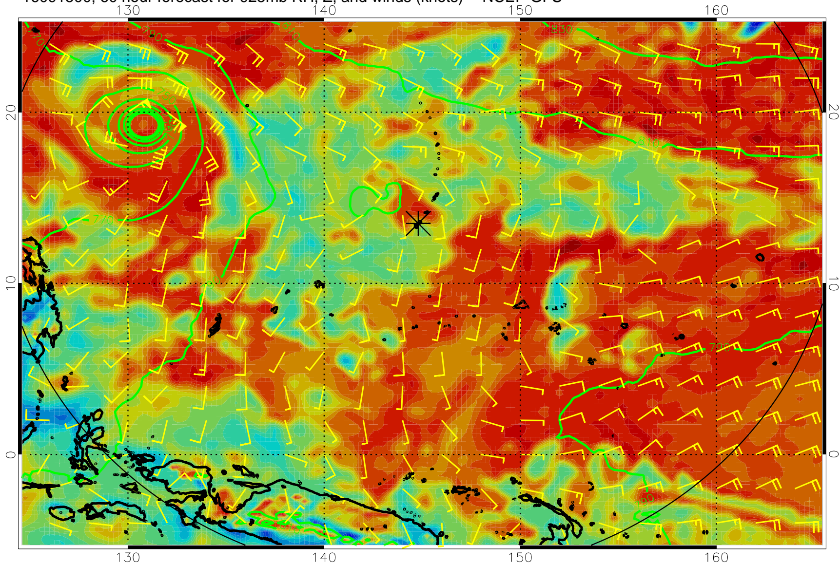
16091500, 60 hour forecast for 925mb RH, Z, and winds (knots) -- NCEP GFS
