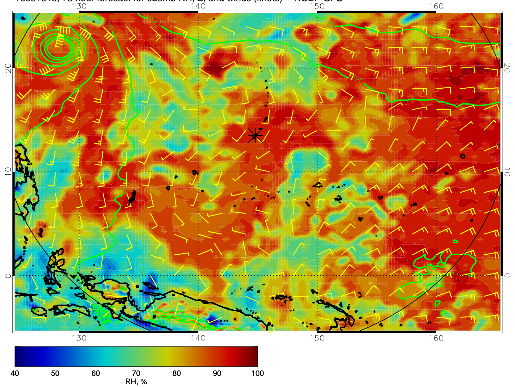
16091518, 78 hour forecast for 925mb RH, Z, and winds (knots) -- NCEP GFS
