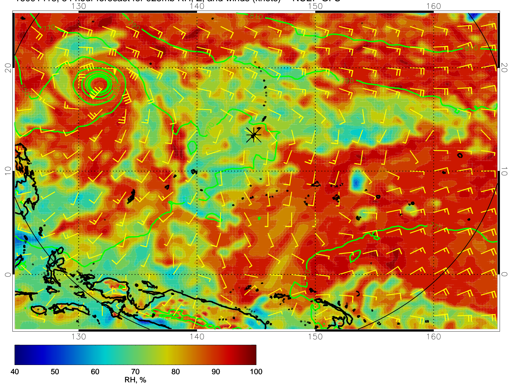
16091418, 54 hour forecast for 925mb RH, Z, and winds (knots) -- NCEP GFS
