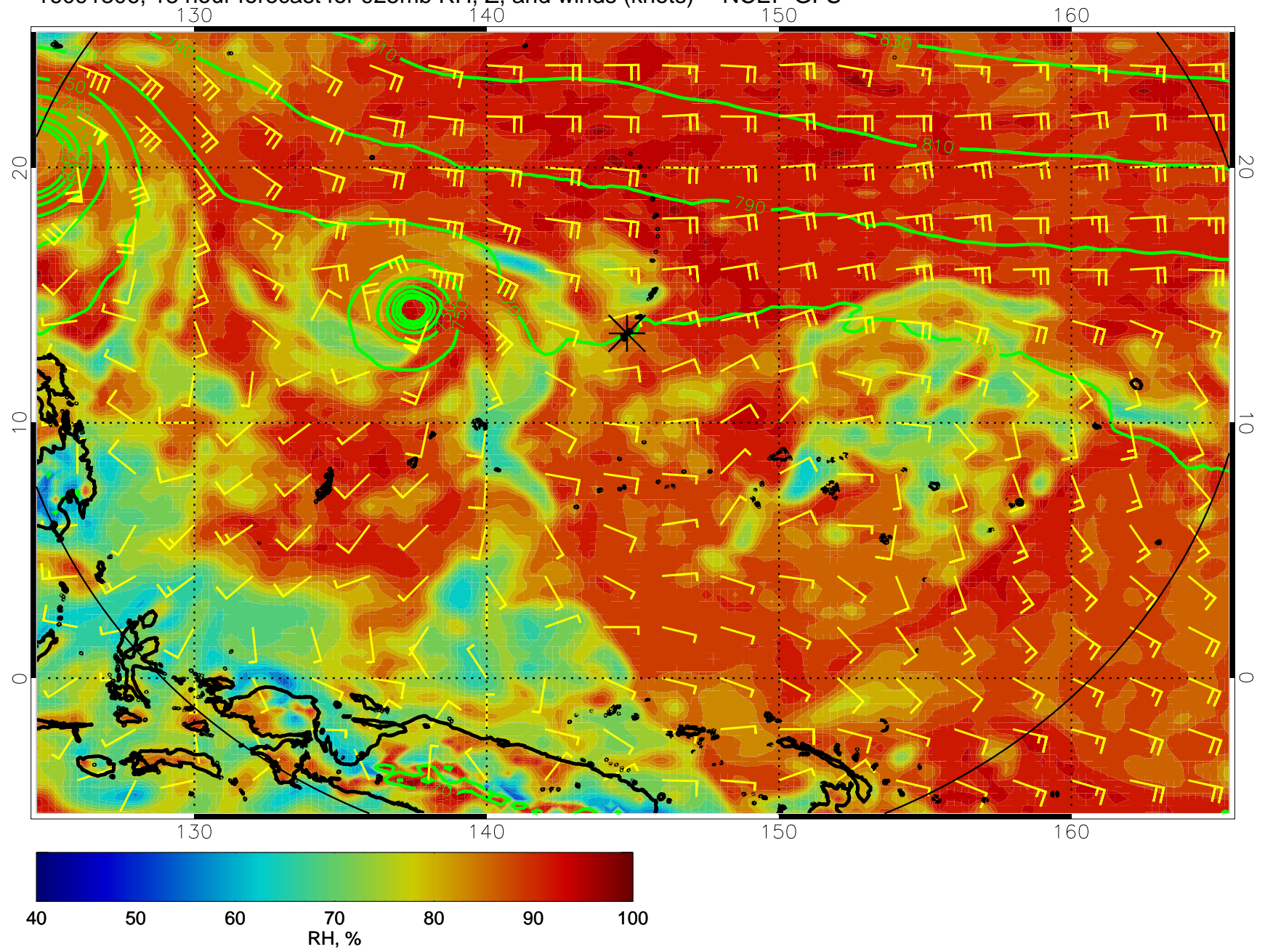
16091306, 18 hour forecast for 925mb RH, Z, and winds (knots) -- NCEP GFS
