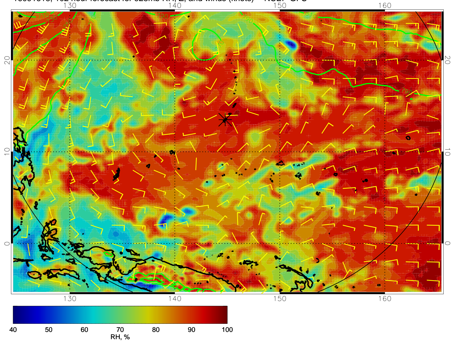
16091618, 102 hour forecast for 925mb RH, Z, and winds (knots) -- NCEP GFS
