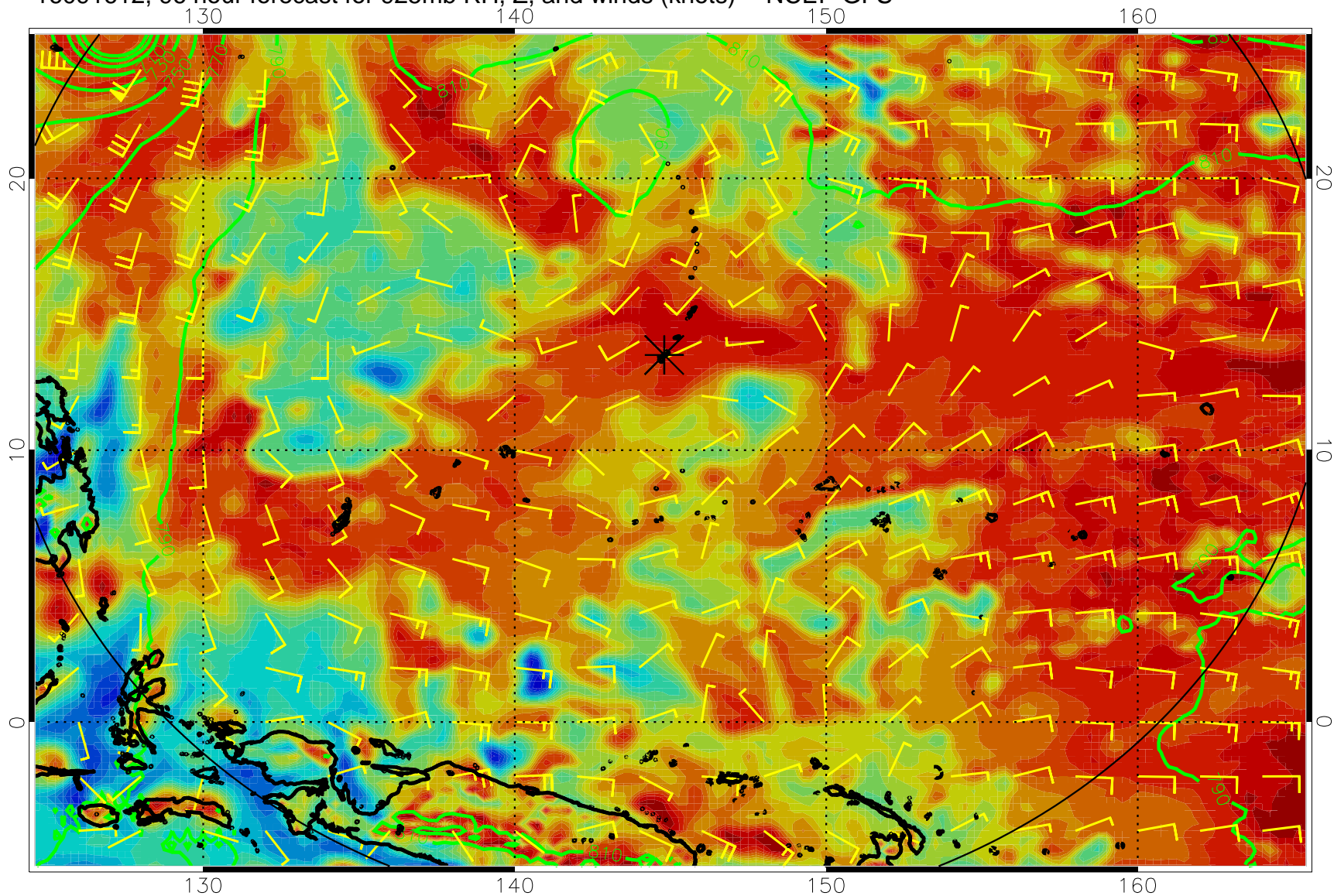
16091612, 96 hour forecast for 925mb RH, Z, and winds (knots) -- NCEP GFS
