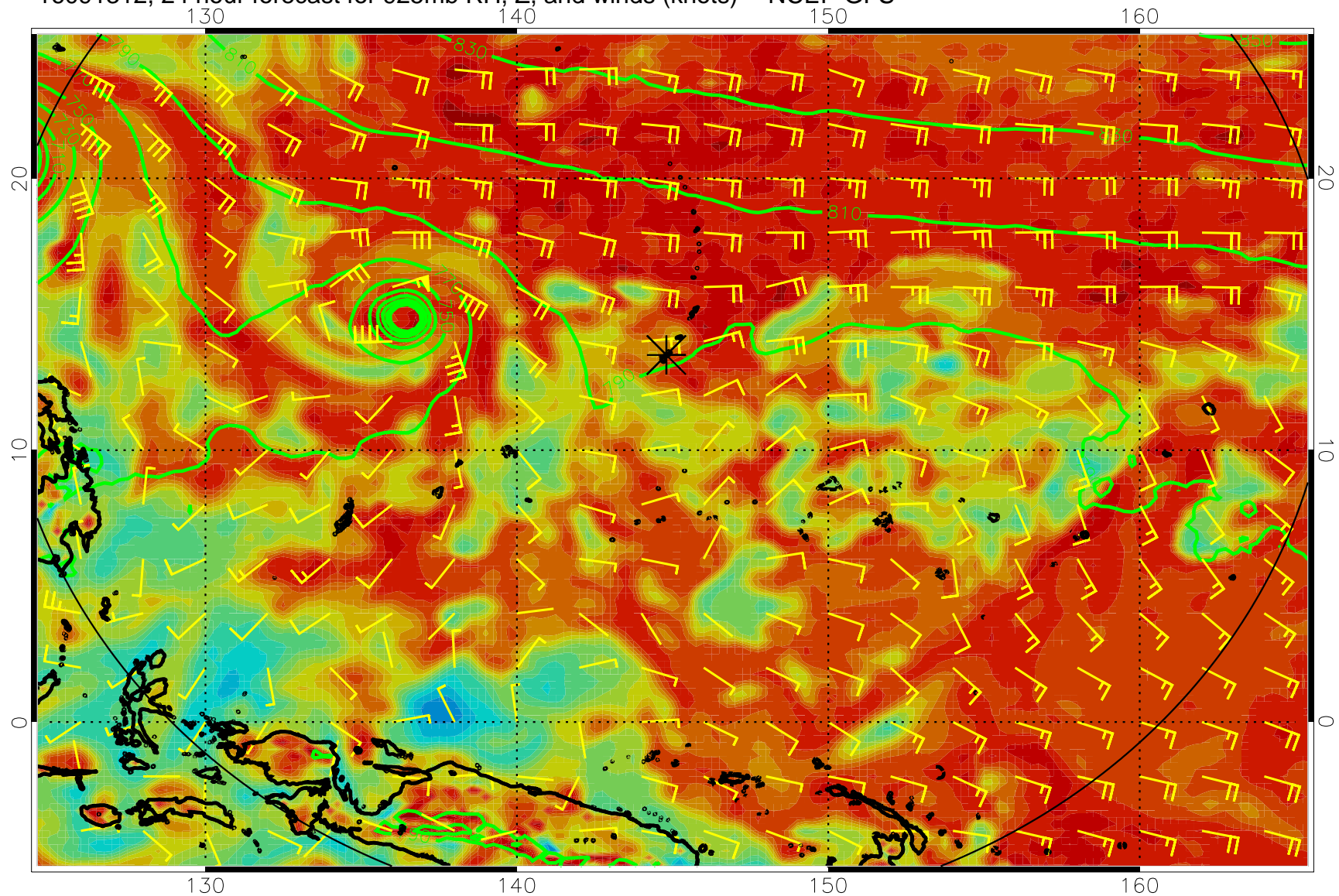
16091312, 24 hour forecast for 925mb RH, Z, and winds (knots) -- NCEP GFS
