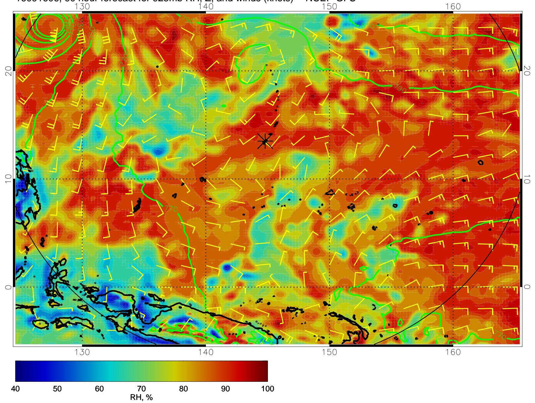
16091606, 90 hour forecast for 925mb RH, Z, and winds (knots) -- NCEP GFS
