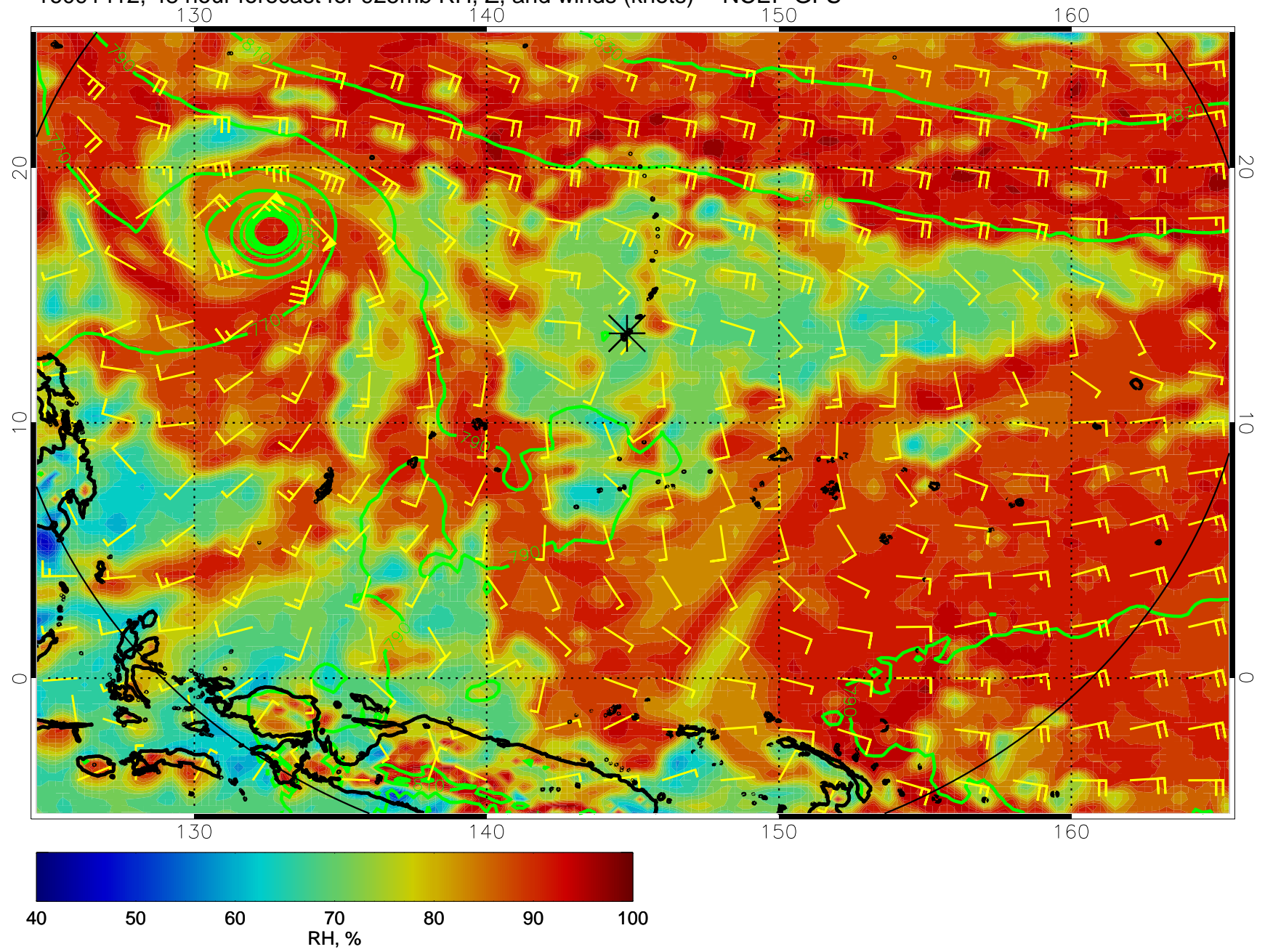
16091412, 48 hour forecast for 925mb RH, Z, and winds (knots) -- NCEP GFS
