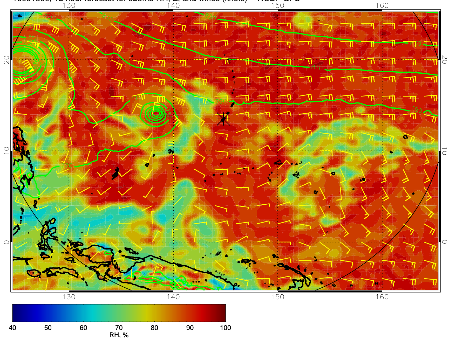
16091300, 12 hour forecast for 925mb RH, Z, and winds (knots) -- NCEP GFS
