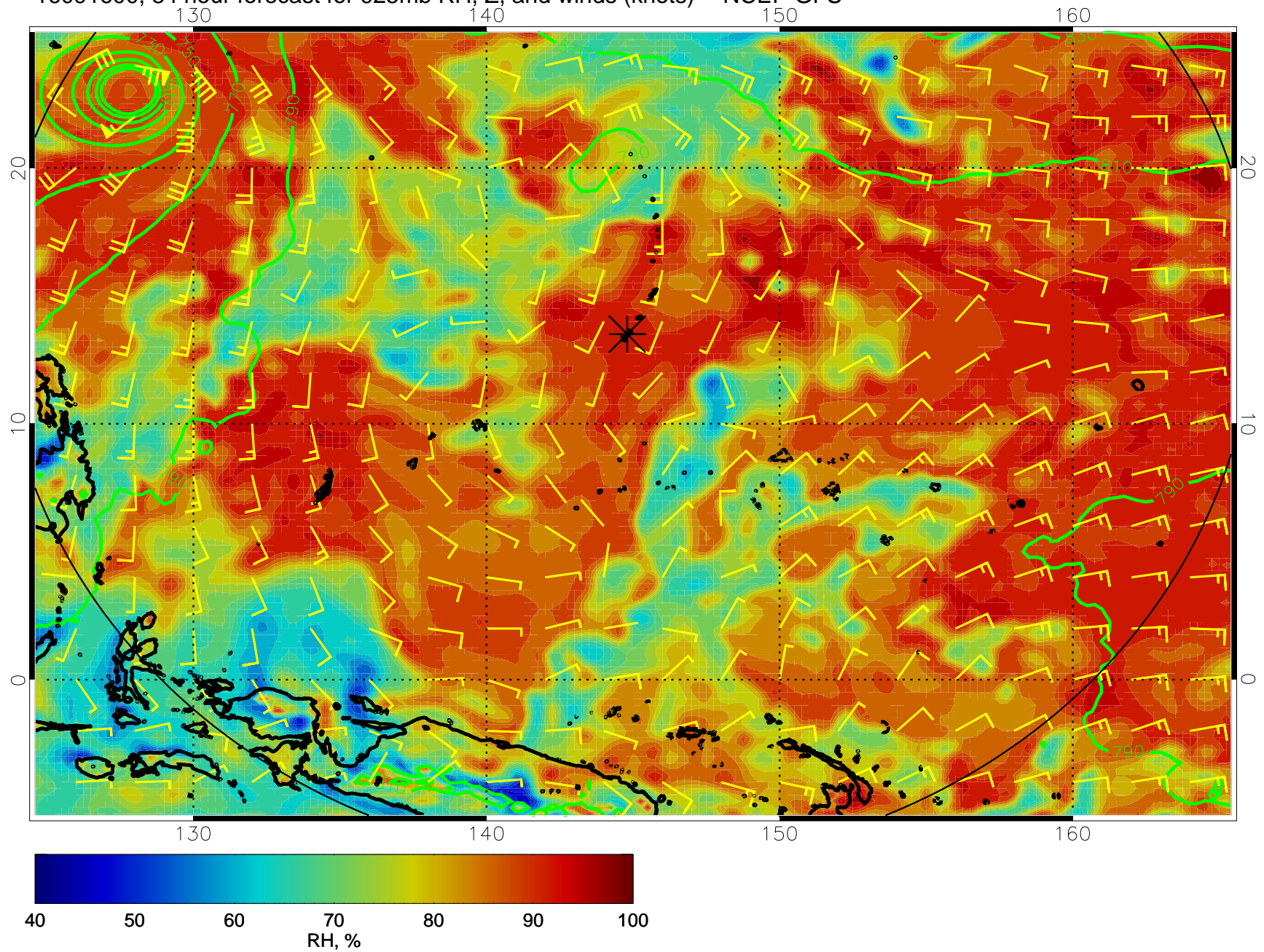
16091600, 84 hour forecast for 925mb RH, Z, and winds (knots) -- NCEP GFS
