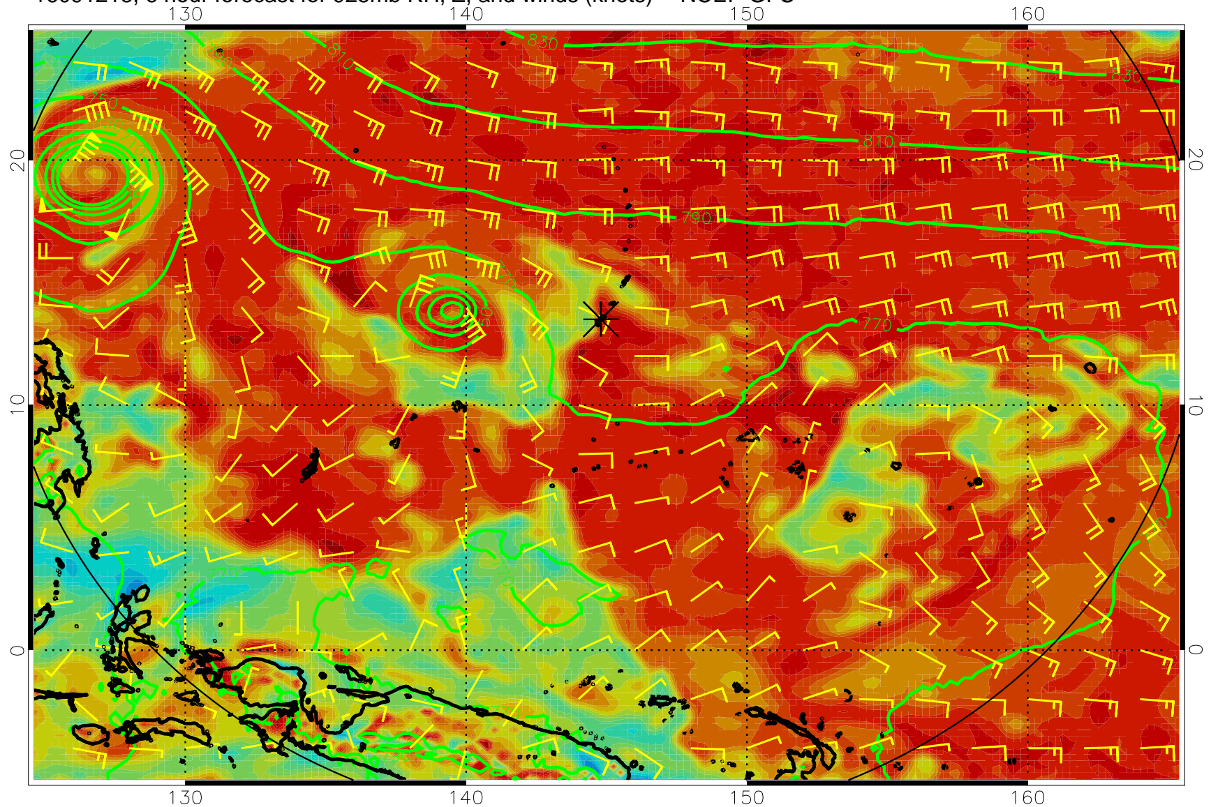
16091218, 6 hour forecast for 925mb RH, Z, and winds (knots) -- NCEP GFS
