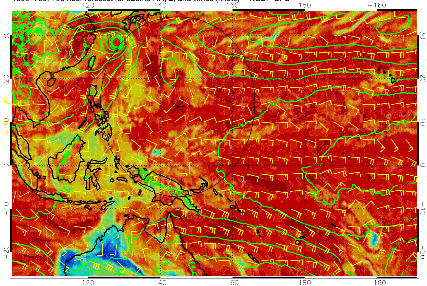
16091700, 108 hour forecast for 925mb RH, Z, and winds (knots) -- NCEP GFS
