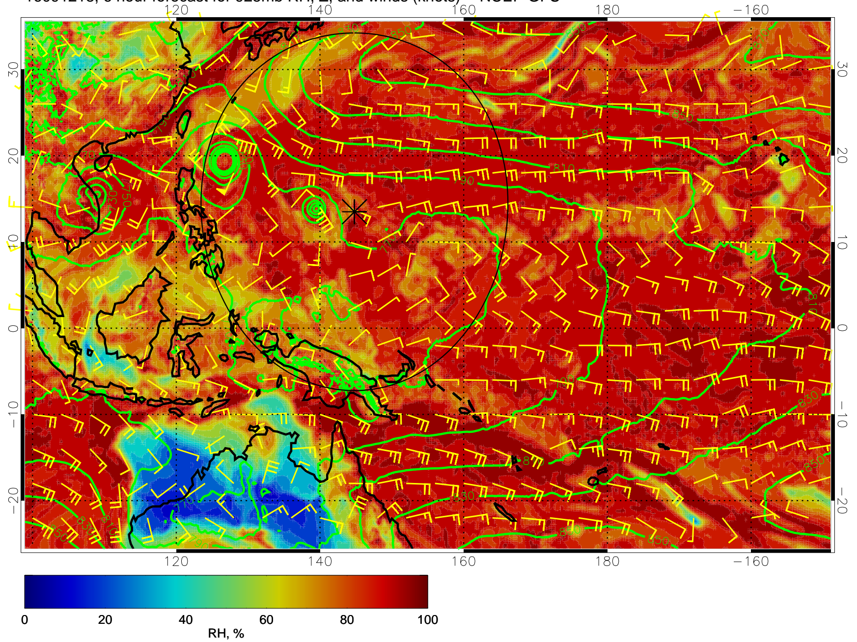
16091218, 6 hour forecast for 925mb RH, Z, and winds (knots) -- NCEP GFS
