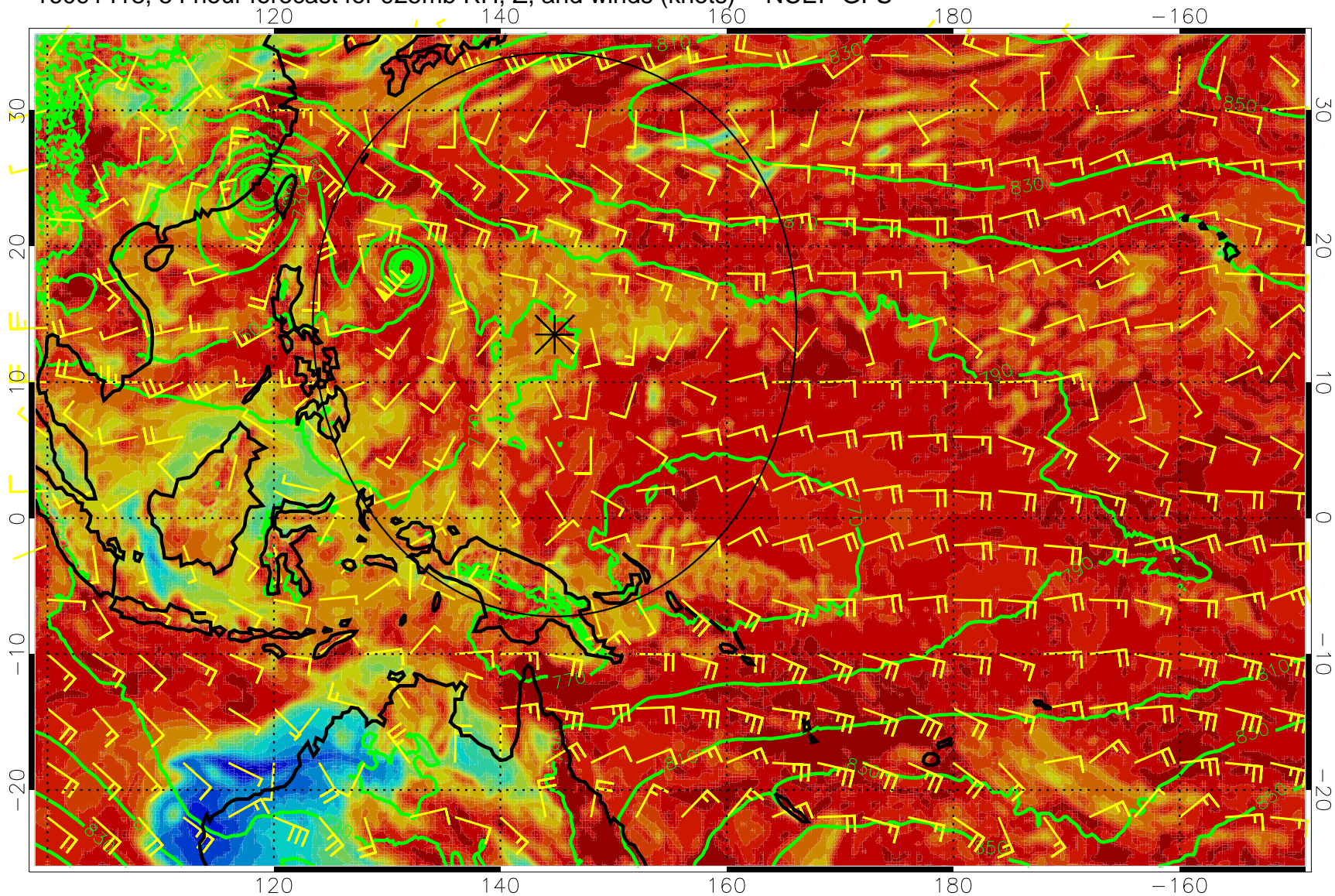
16091418, 54 hour forecast for 925mb RH, Z, and winds (knots) -- NCEP GFS
