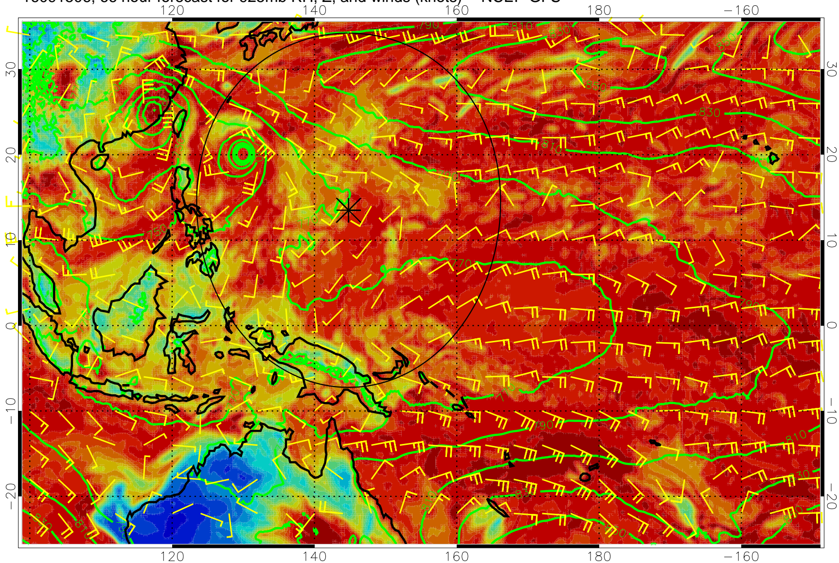
16091506, 66 hour forecast for 925mb RH, Z, and winds (knots) -- NCEP GFS
