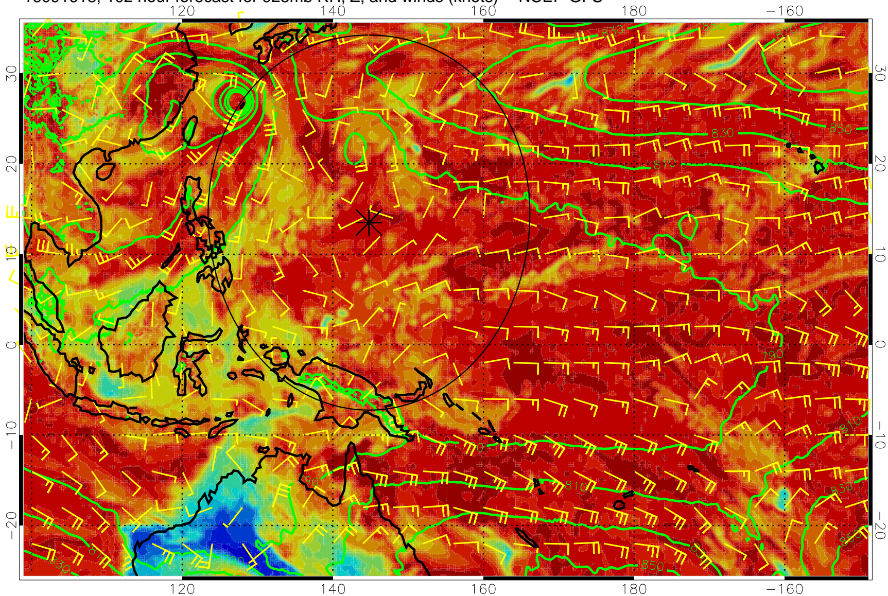
16091618, 102 hour forecast for 925mb RH, Z, and winds (knots) -- NCEP GFS
