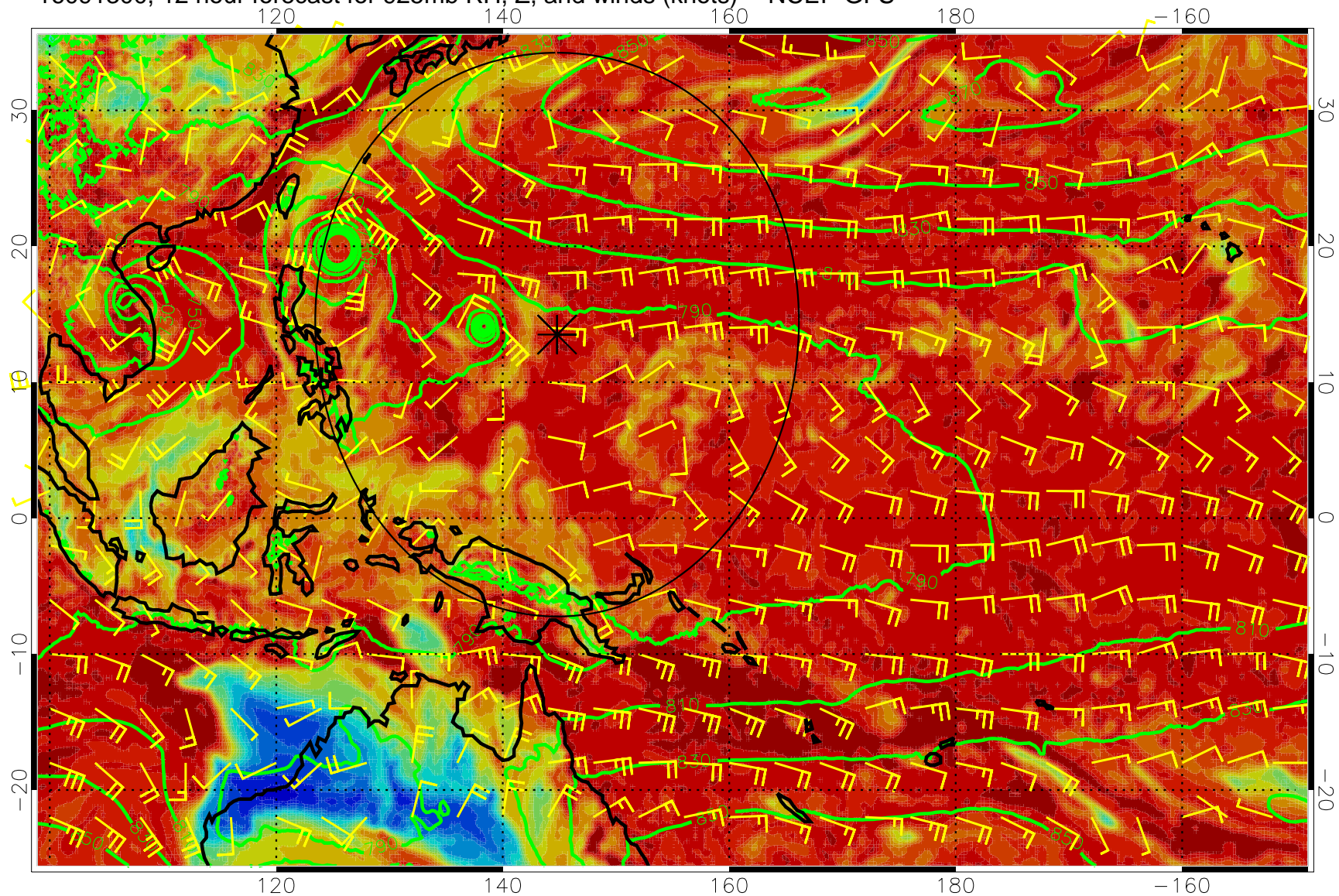
16091300, 12 hour forecast for 925mb RH, Z, and winds (knots) -- NCEP GFS
