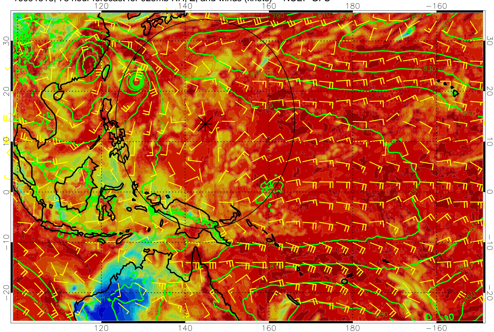
16091518, 78 hour forecast for 925mb RH, Z, and winds (knots) -- NCEP GFS
