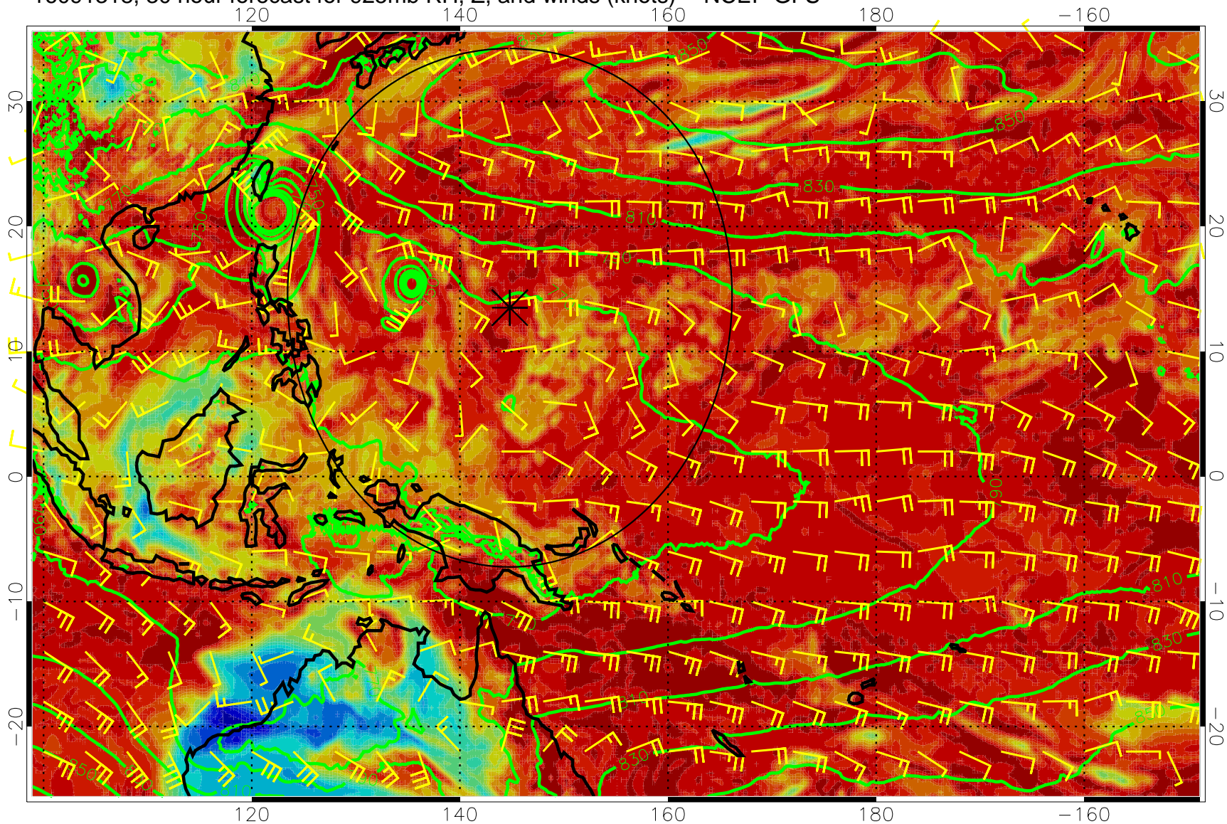
16091318, 30 hour forecast for 925mb RH, Z, and winds (knots) -- NCEP GFS
