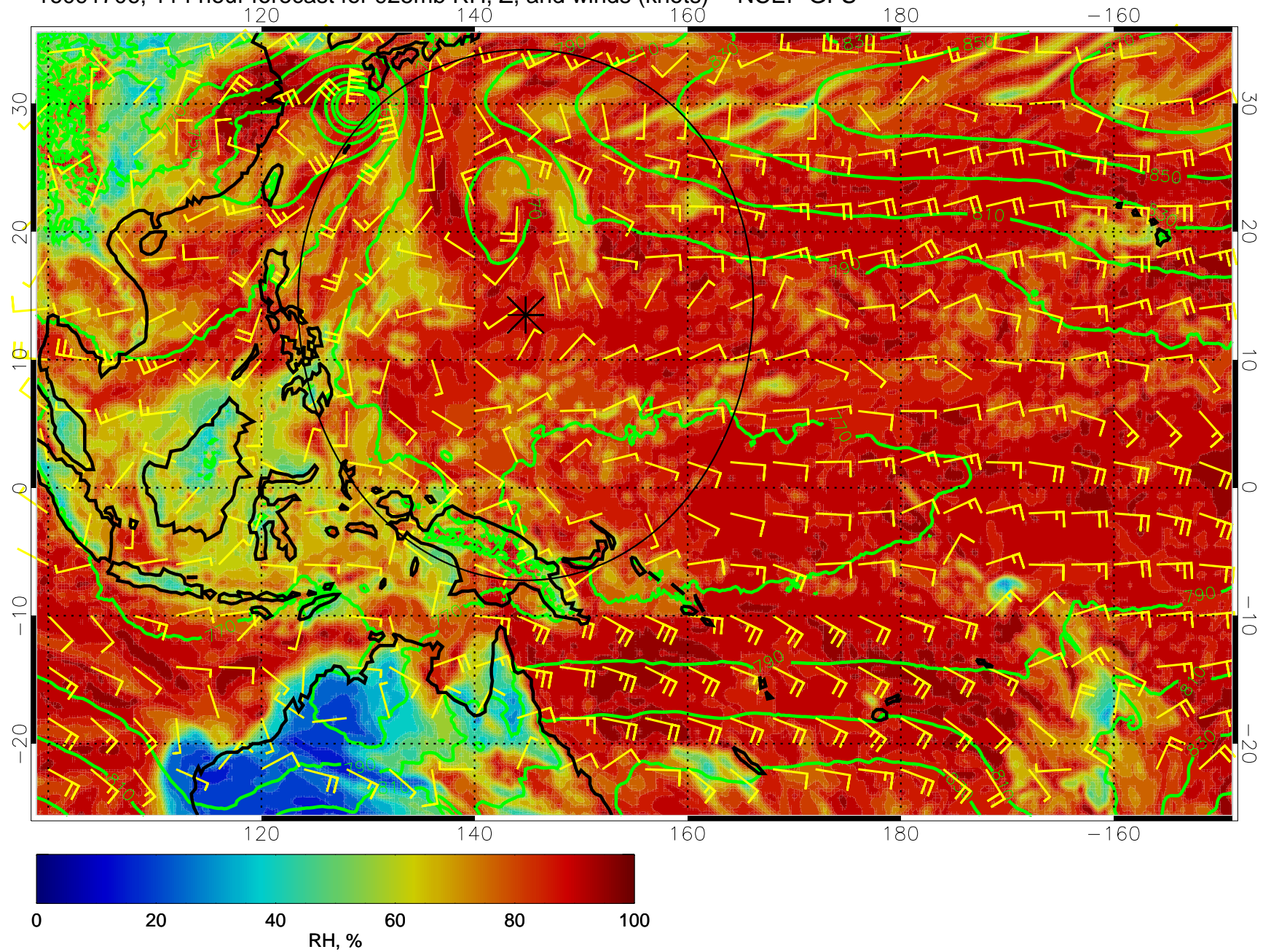
16091706, 114 hour forecast for 925mb RH, Z, and winds (knots) -- NCEP GFS
