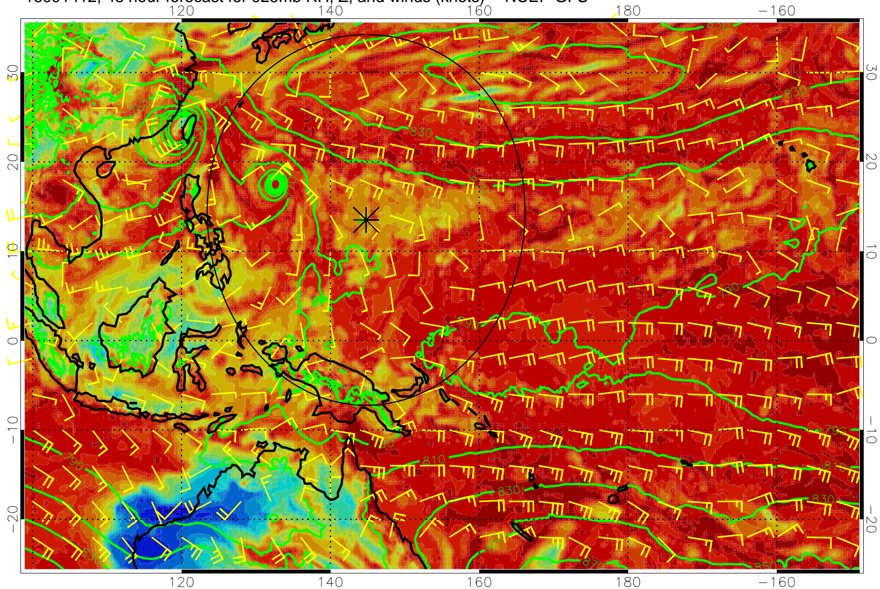
16091412, 48 hour forecast for 925mb RH, Z, and winds (knots) -- NCEP GFS
