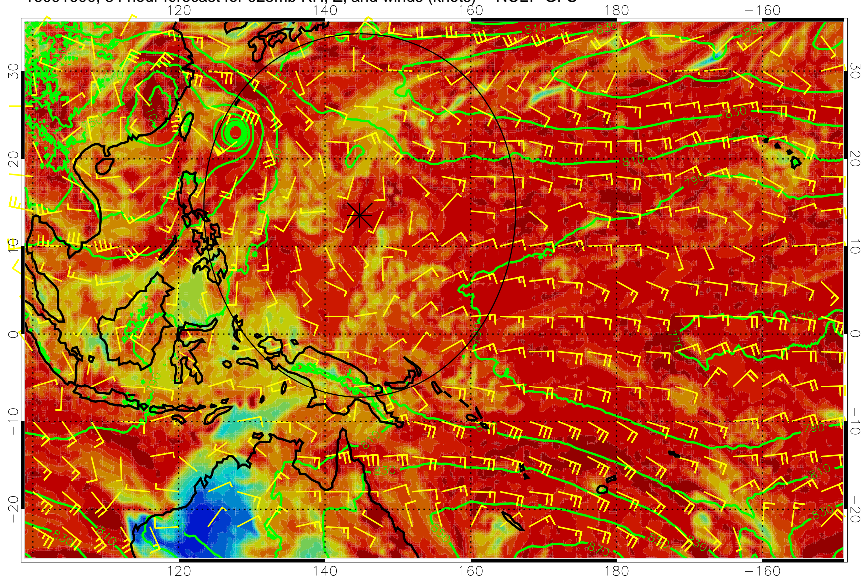
16091600, 84 hour forecast for 925mb RH, Z, and winds (knots) -- NCEP GFS
