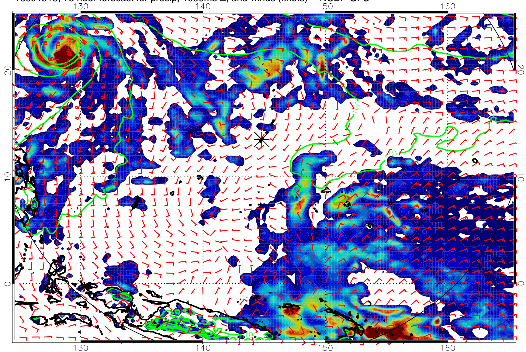
16091518, 78 hour forecast for precip, 1000mb Z, and winds (knots) -- NCEP GFS
