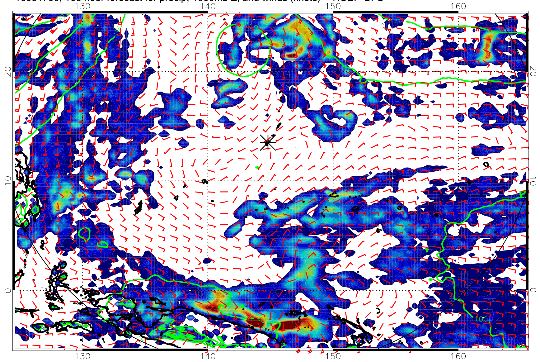
16091700, 108 hour forecast for precip, 1000mb Z, and winds (knots) -- NCEP GFS
