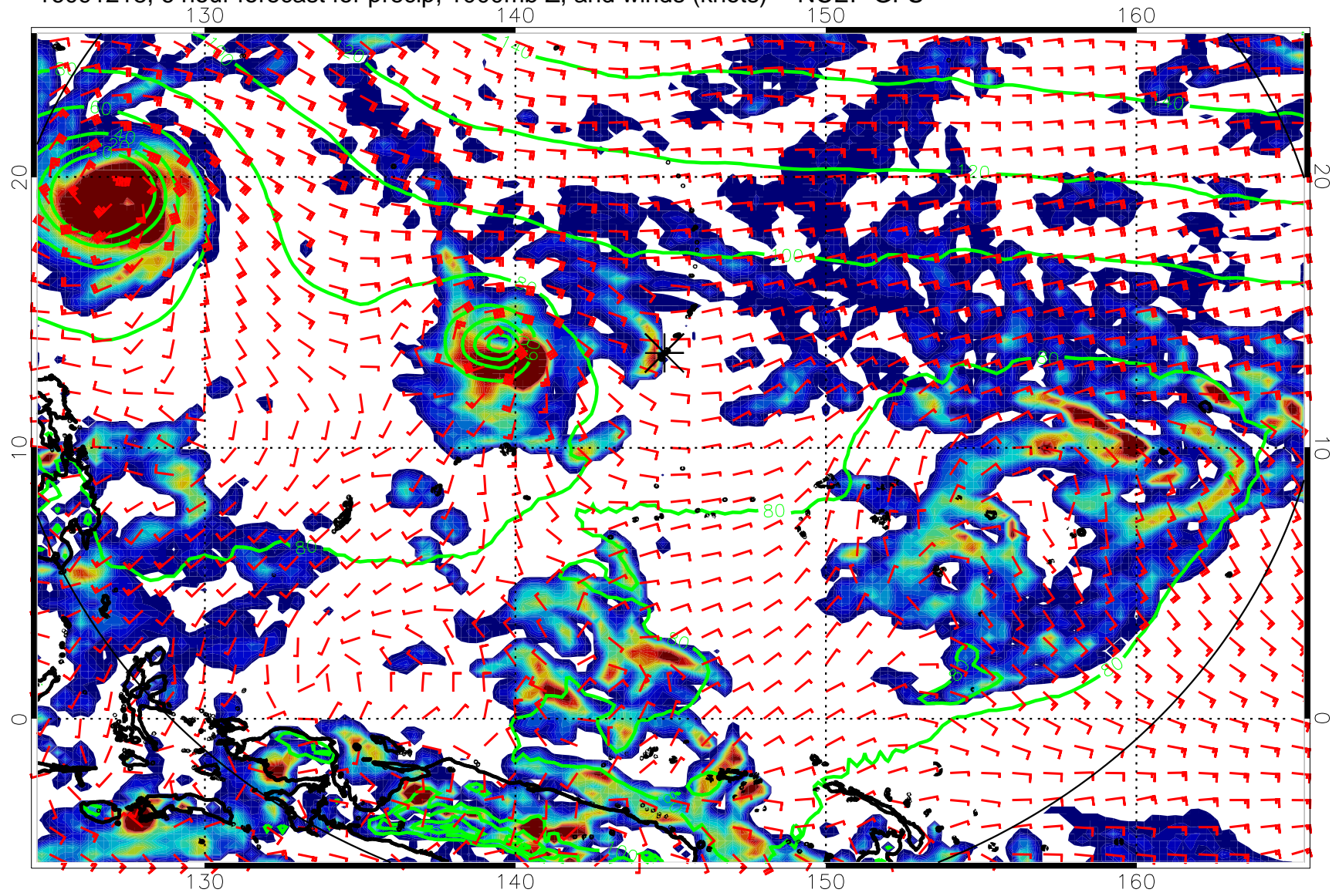
16091218, 6 hour forecast for precip, 1000mb Z, and winds (knots) -- NCEP GFS
