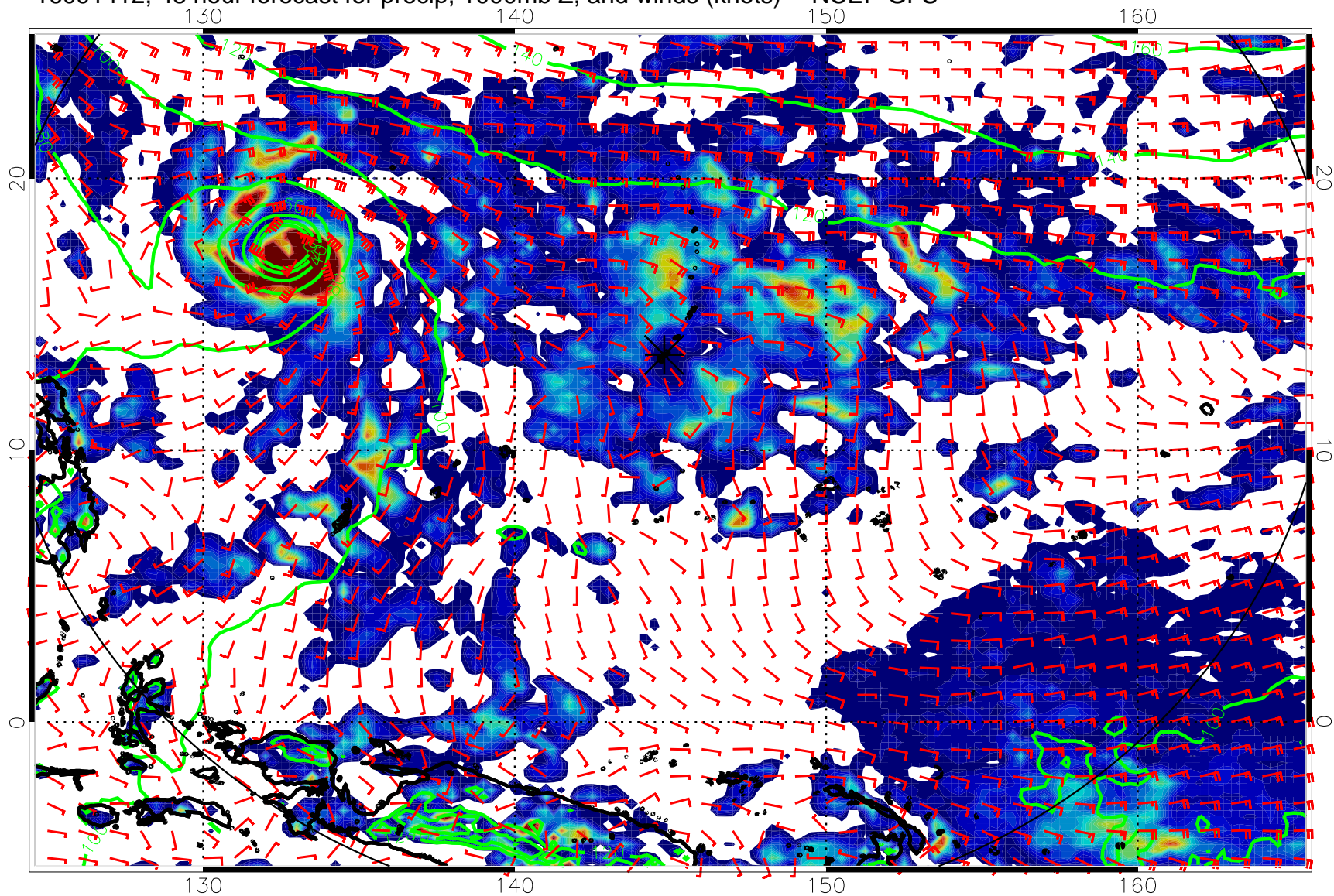
16091412, 48 hour forecast for precip, 1000mb Z, and winds (knots) -- NCEP GFS
