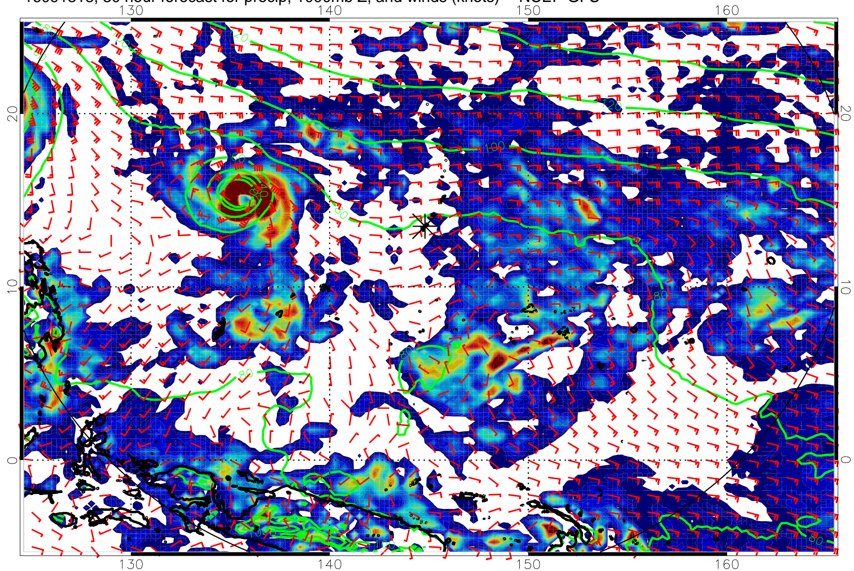
16091318, 30 hour forecast for precip, 1000mb Z, and winds (knots) -- NCEP GFS
