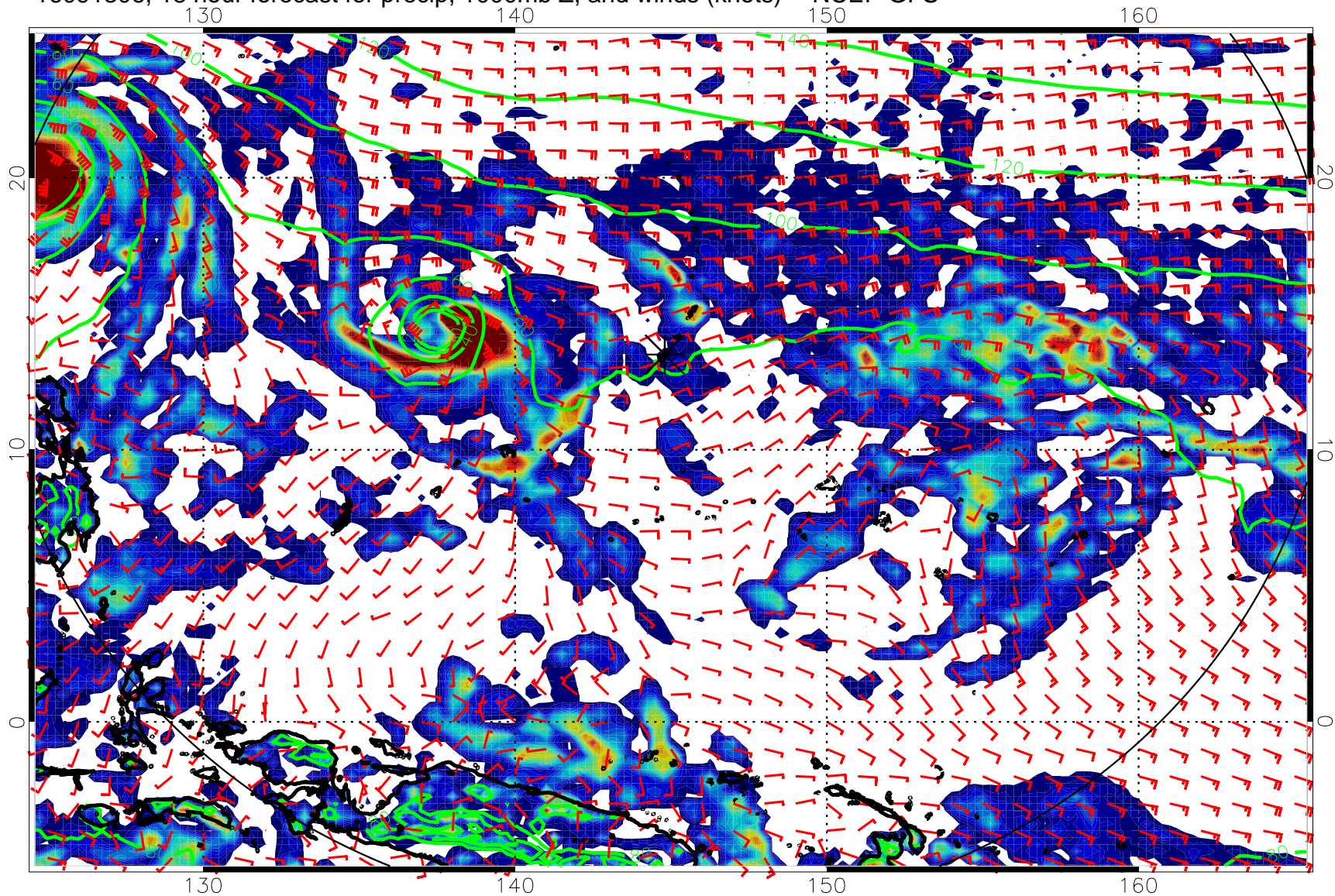
16091306, 18 hour forecast for precip, 1000mb Z, and winds (knots) -- NCEP GFS
