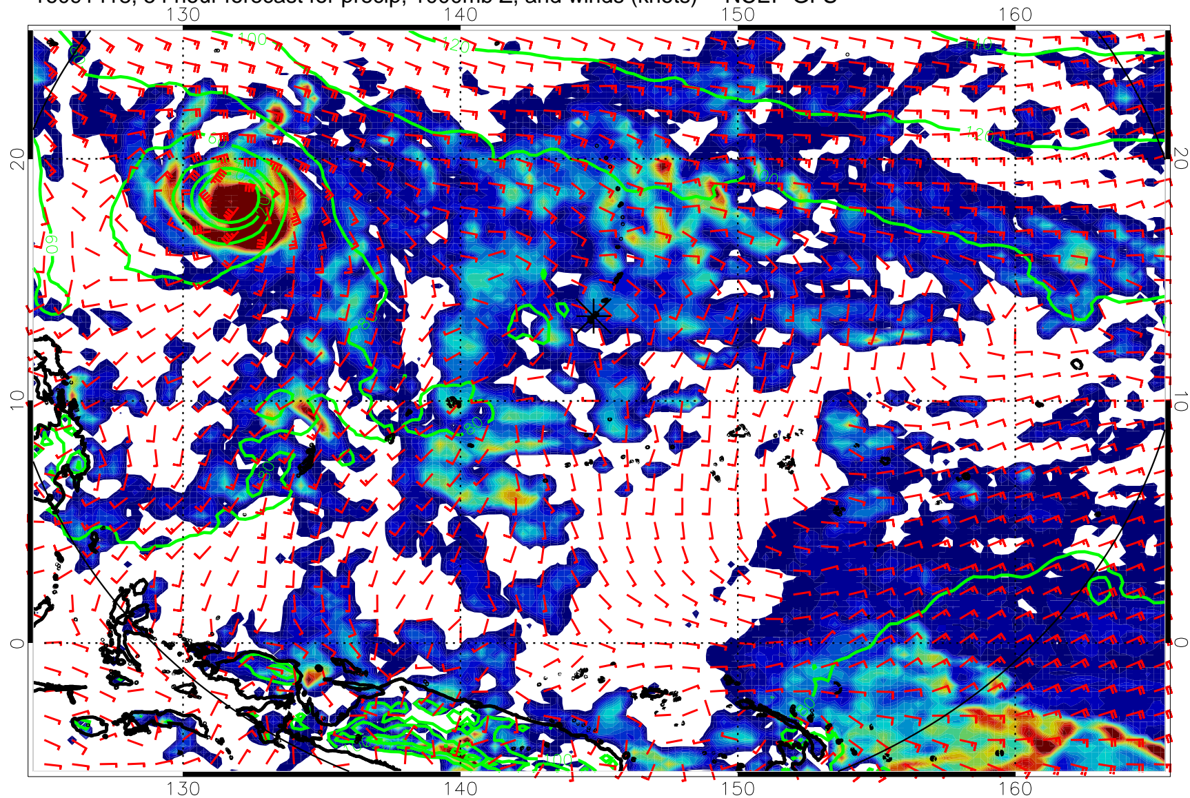
16091418, 54 hour forecast for precip, 1000mb Z, and winds (knots) -- NCEP GFS
