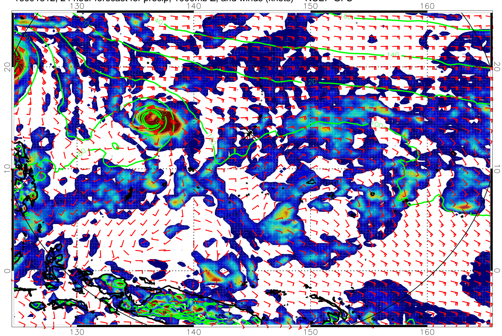
16091312, 24 hour forecast for precip, 1000mb Z, and winds (knots) -- NCEP GFS
