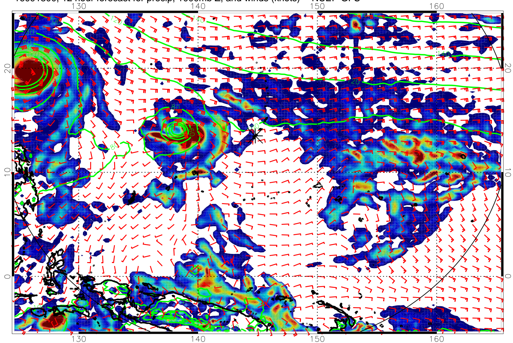
16091300, 12 hour forecast for precip, 1000mb Z, and winds (knots) -- NCEP GFS
