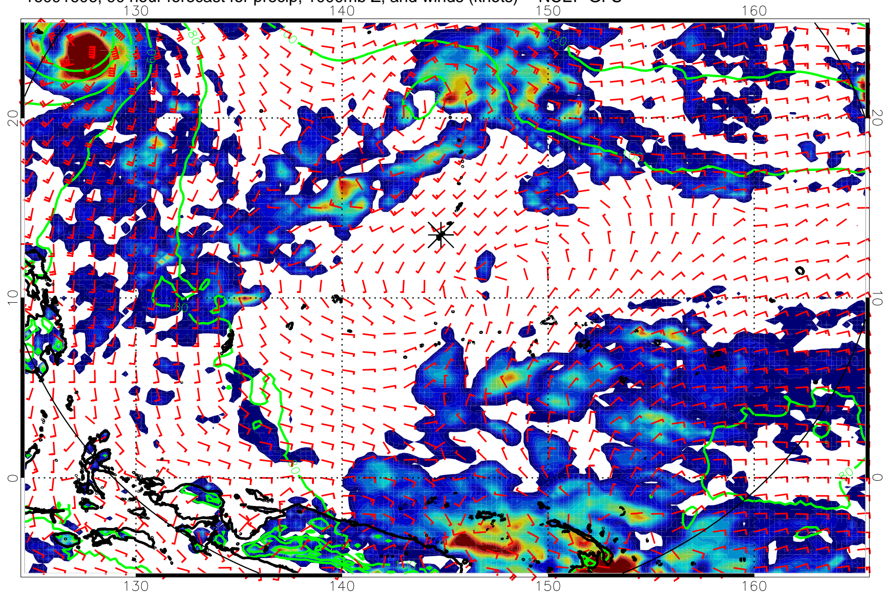
16091606, 90 hour forecast for precip, 1000mb Z, and winds (knots) -- NCEP GFS
