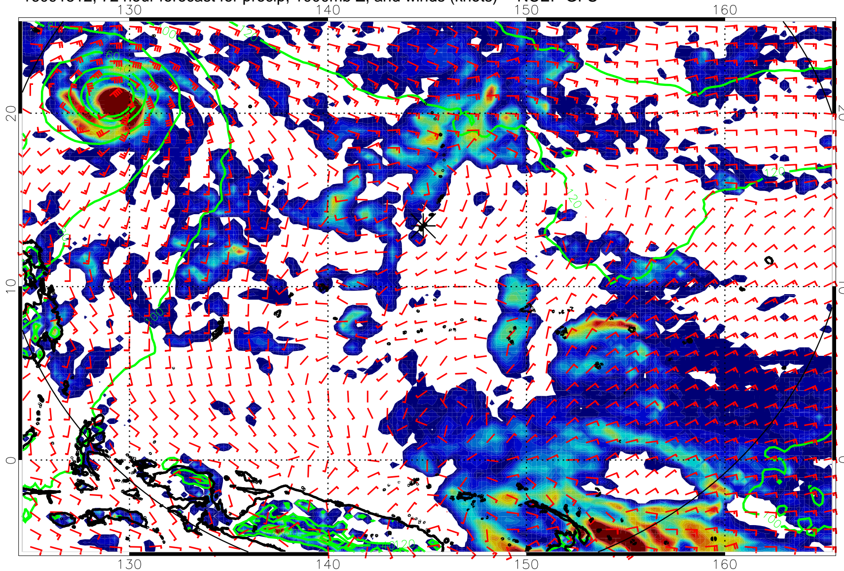
16091512, 72 hour forecast for precip, 1000mb Z, and winds (knots) -- NCEP GFS
