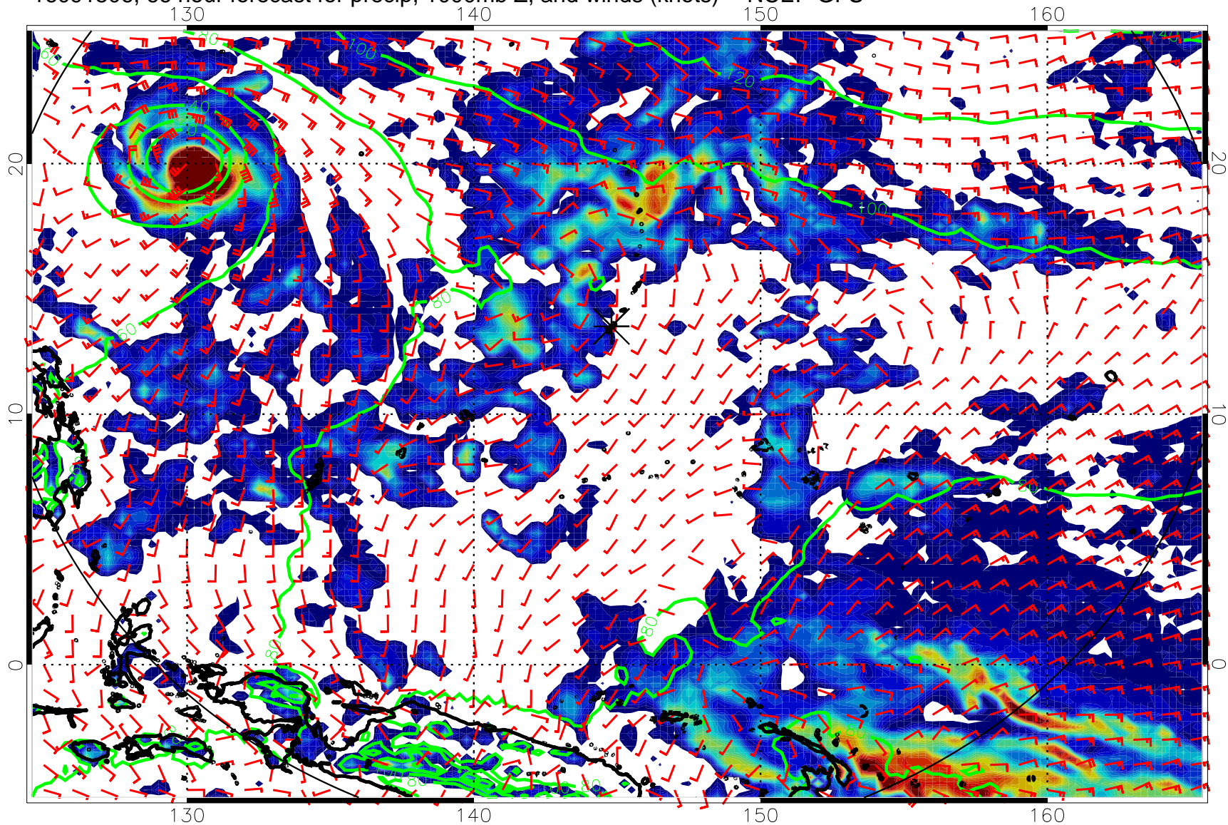
16091506, 66 hour forecast for precip, 1000mb Z, and winds (knots) -- NCEP GFS
