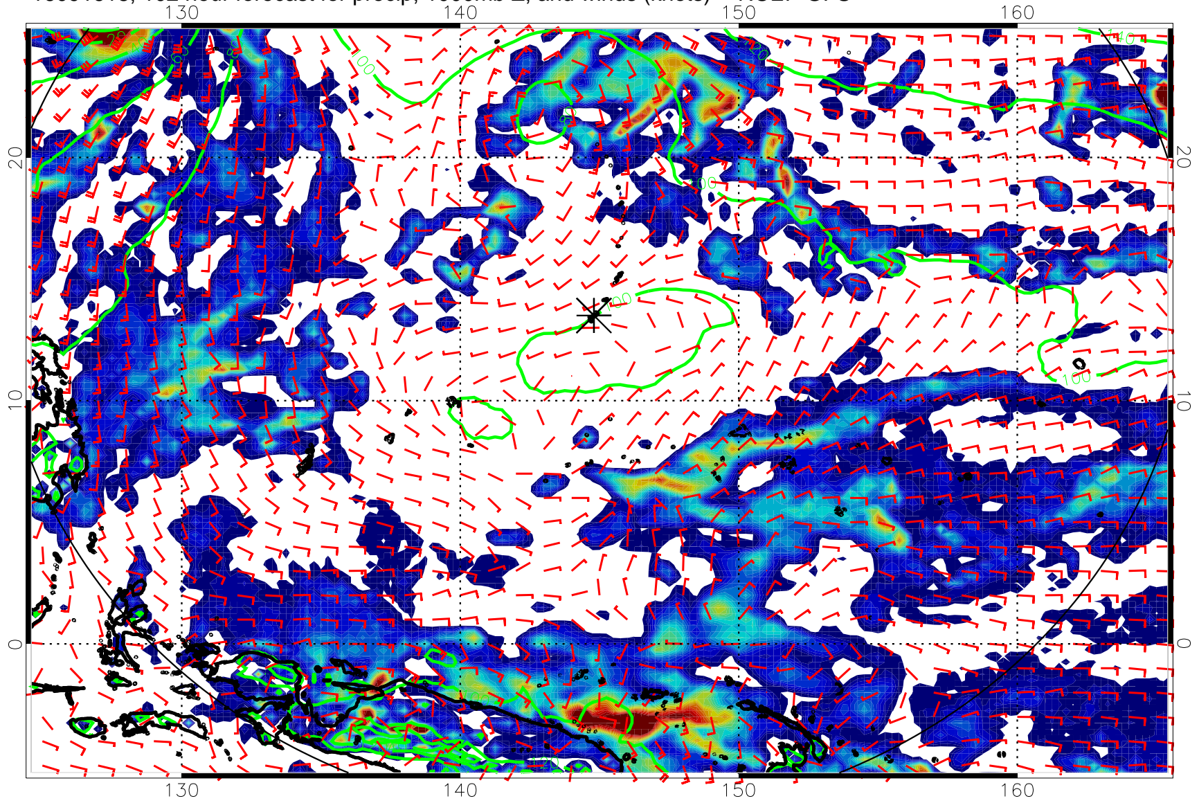
16091618, 102 hour forecast for precip, 1000mb Z, and winds (knots) -- NCEP GFS
