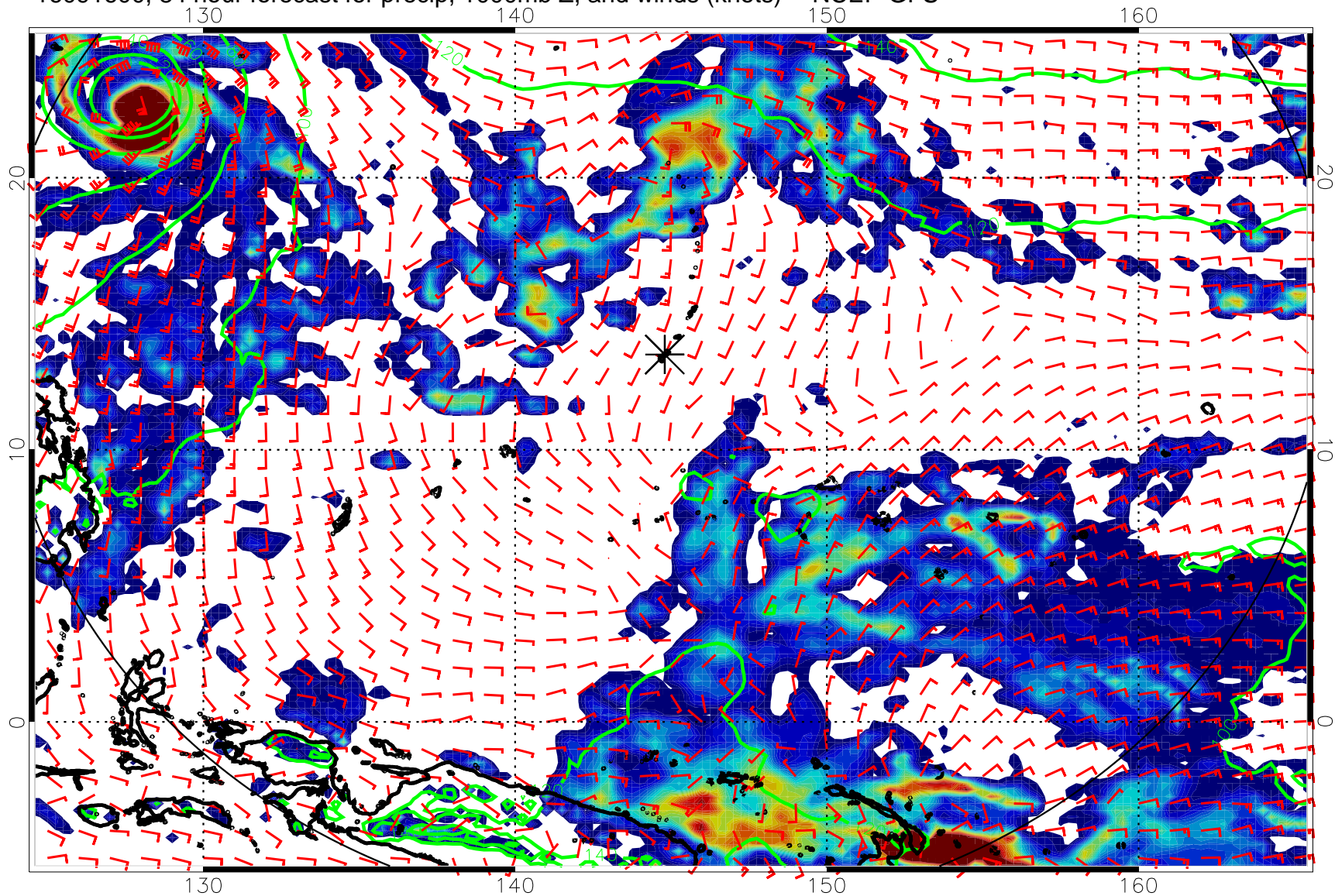
16091600, 84 hour forecast for precip, 1000mb Z, and winds (knots) -- NCEP GFS
