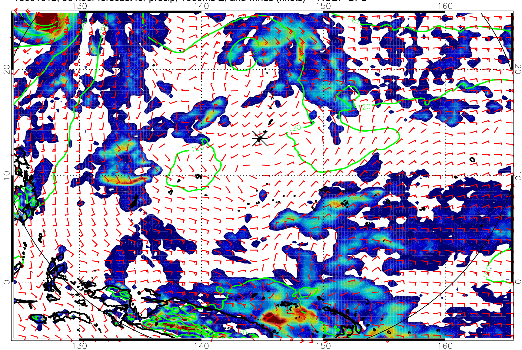
16091612, 96 hour forecast for precip, 1000mb Z, and winds (knots) -- NCEP GFS
