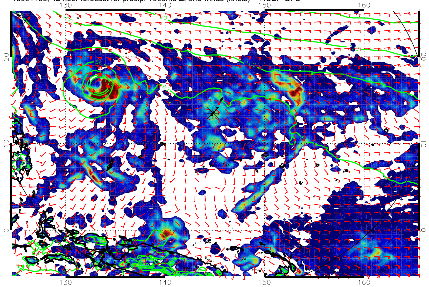
16091406, 42 hour forecast for precip, 1000mb Z, and winds (knots) -- NCEP GFS
