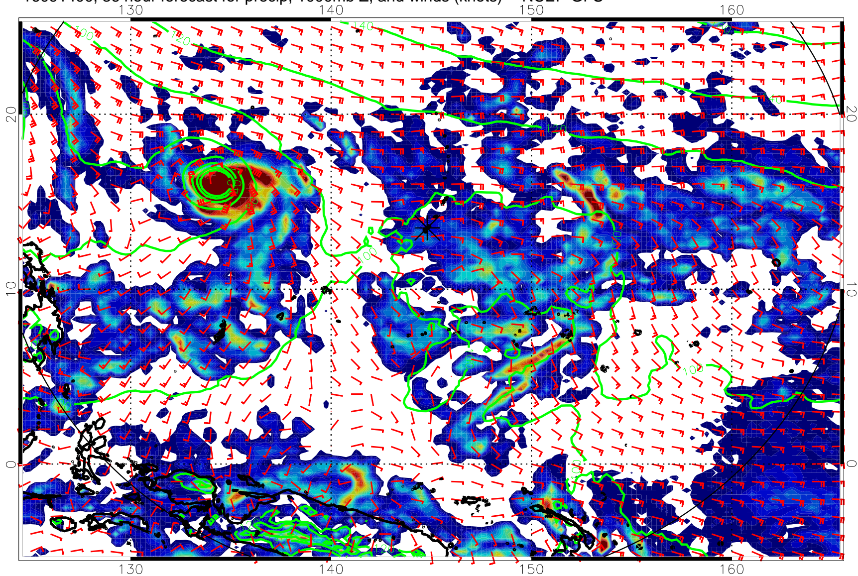
16091400, 36 hour forecast for precip, 1000mb Z, and winds (knots) -- NCEP GFS
