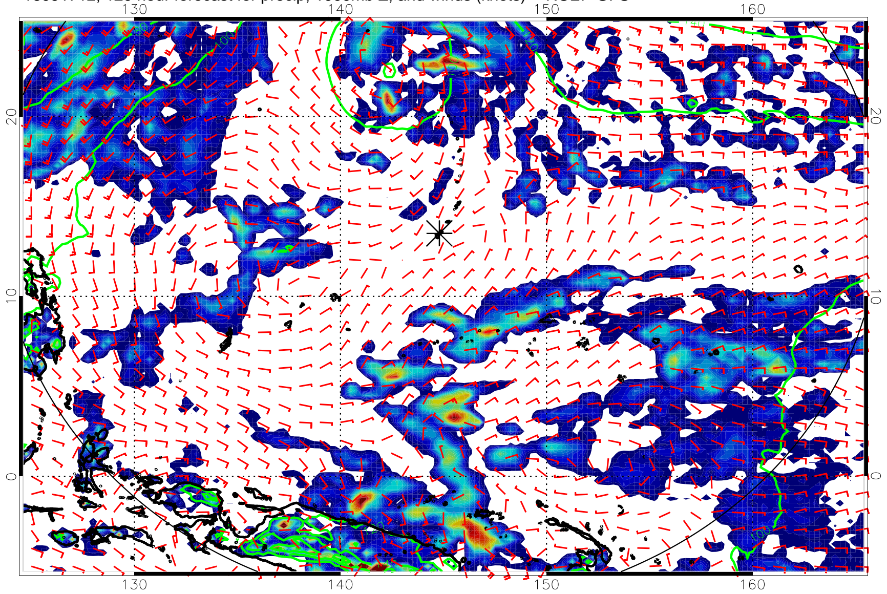
16091712, 120 hour forecast for precip, 1000mb Z, and winds (knots) -- NCEP GFS
