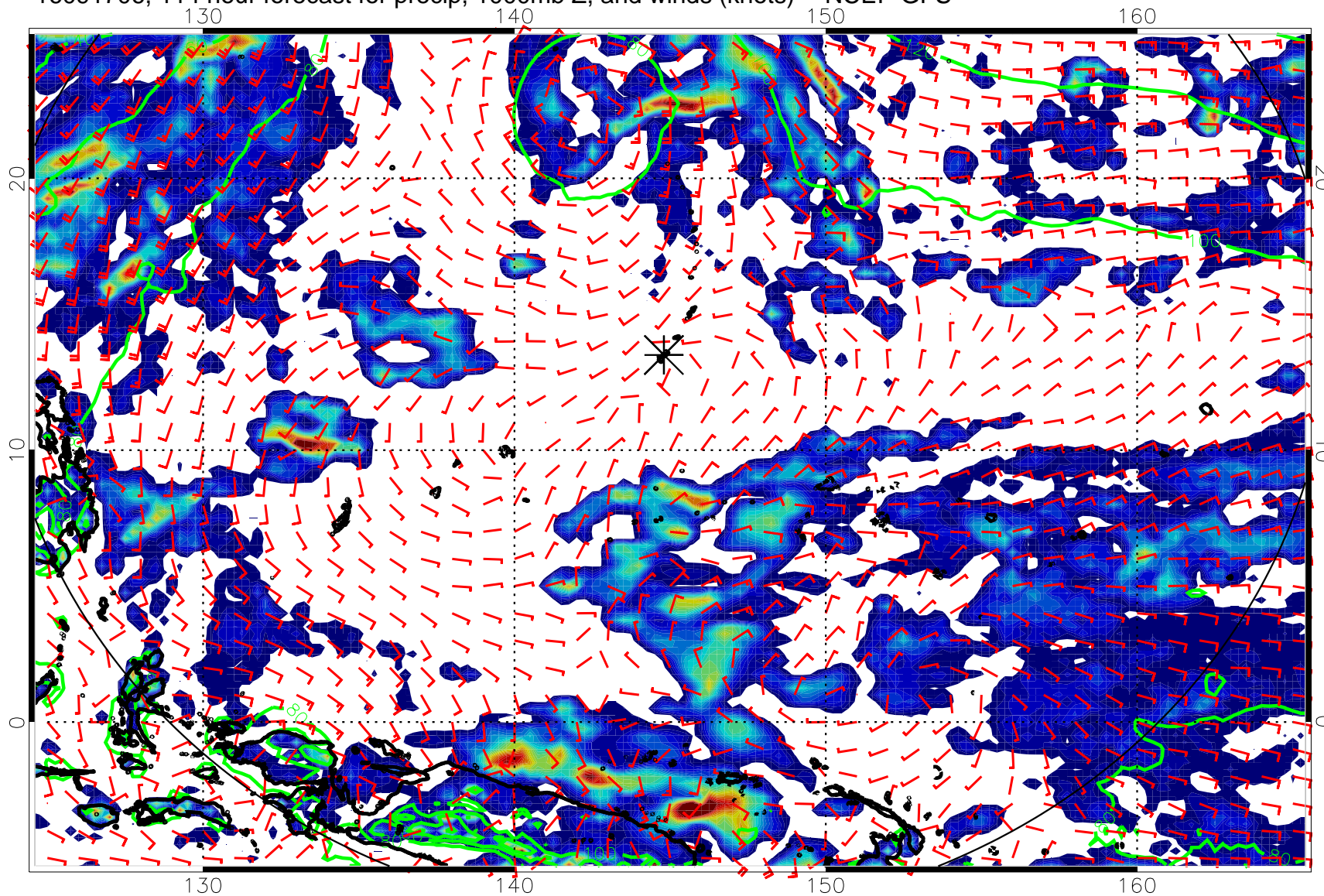
16091706, 114 hour forecast for precip, 1000mb Z, and winds (knots) -- NCEP GFS
