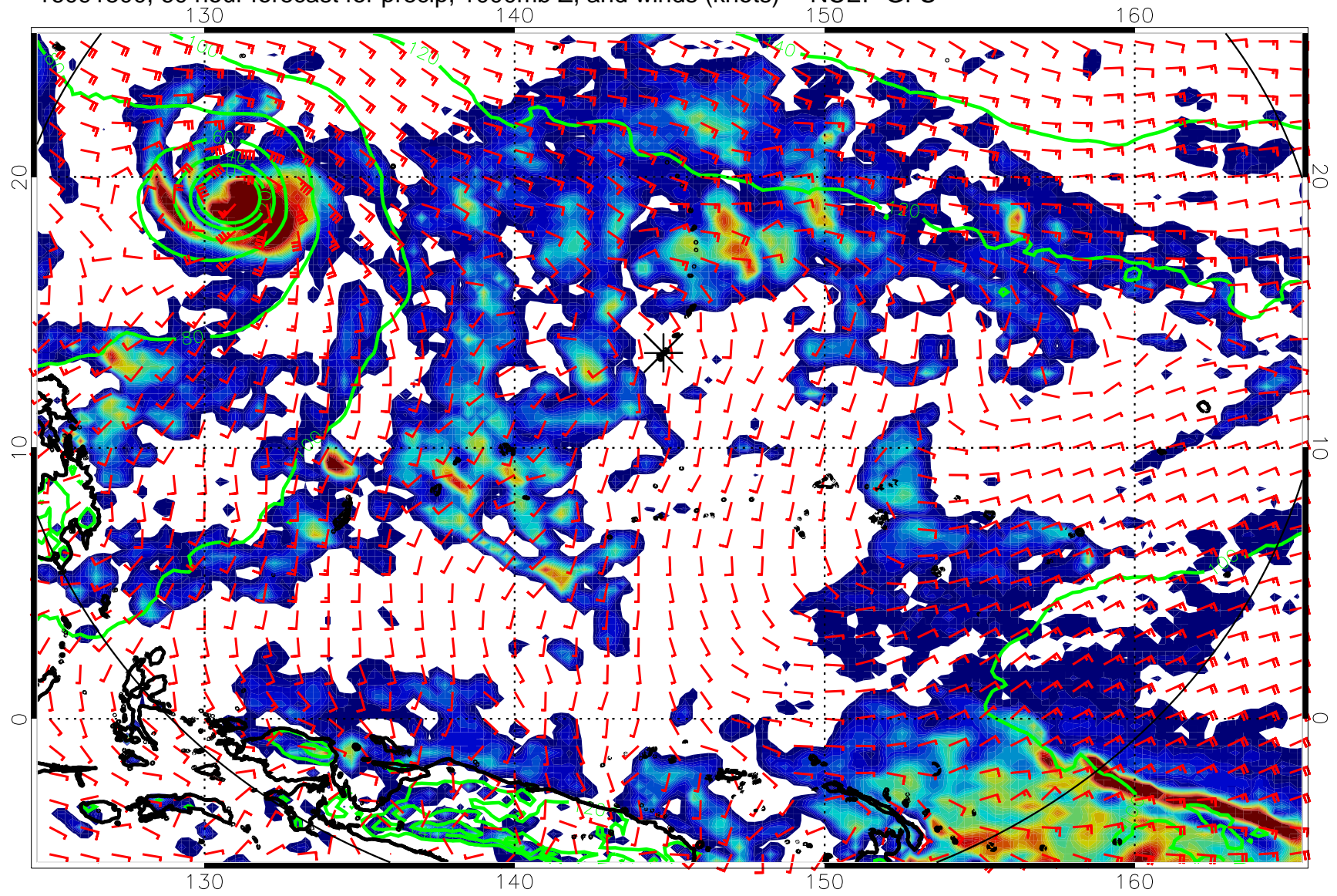
16091500, 60 hour forecast for precip, 1000mb Z, and winds (knots) -- NCEP GFS
