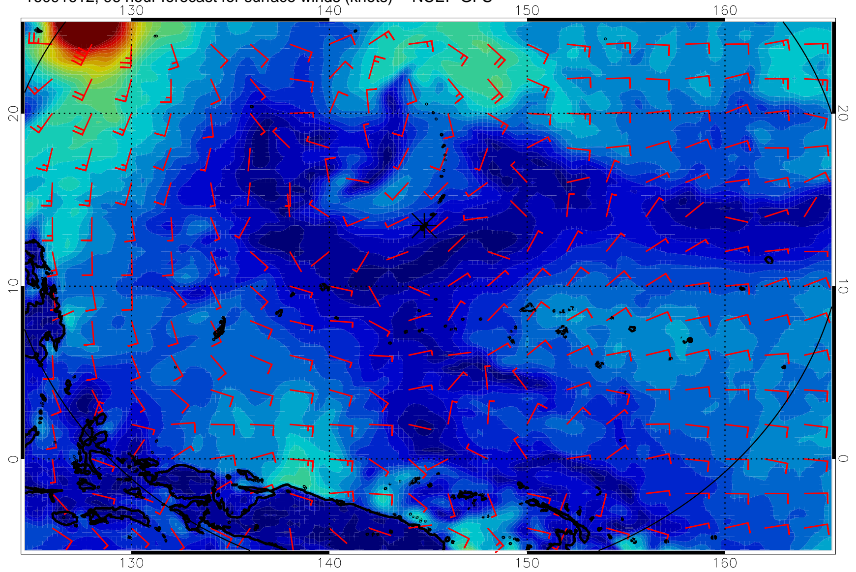
16091612, 96 hour forecast for surface winds (knots) -- NCEP GFS
