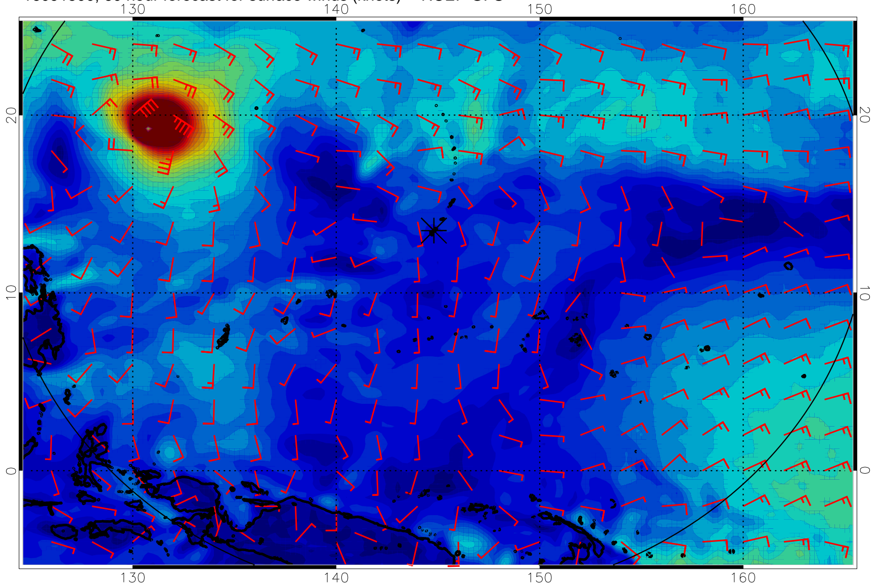
16091500, 60 hour forecast for surface winds (knots) -- NCEP GFS
