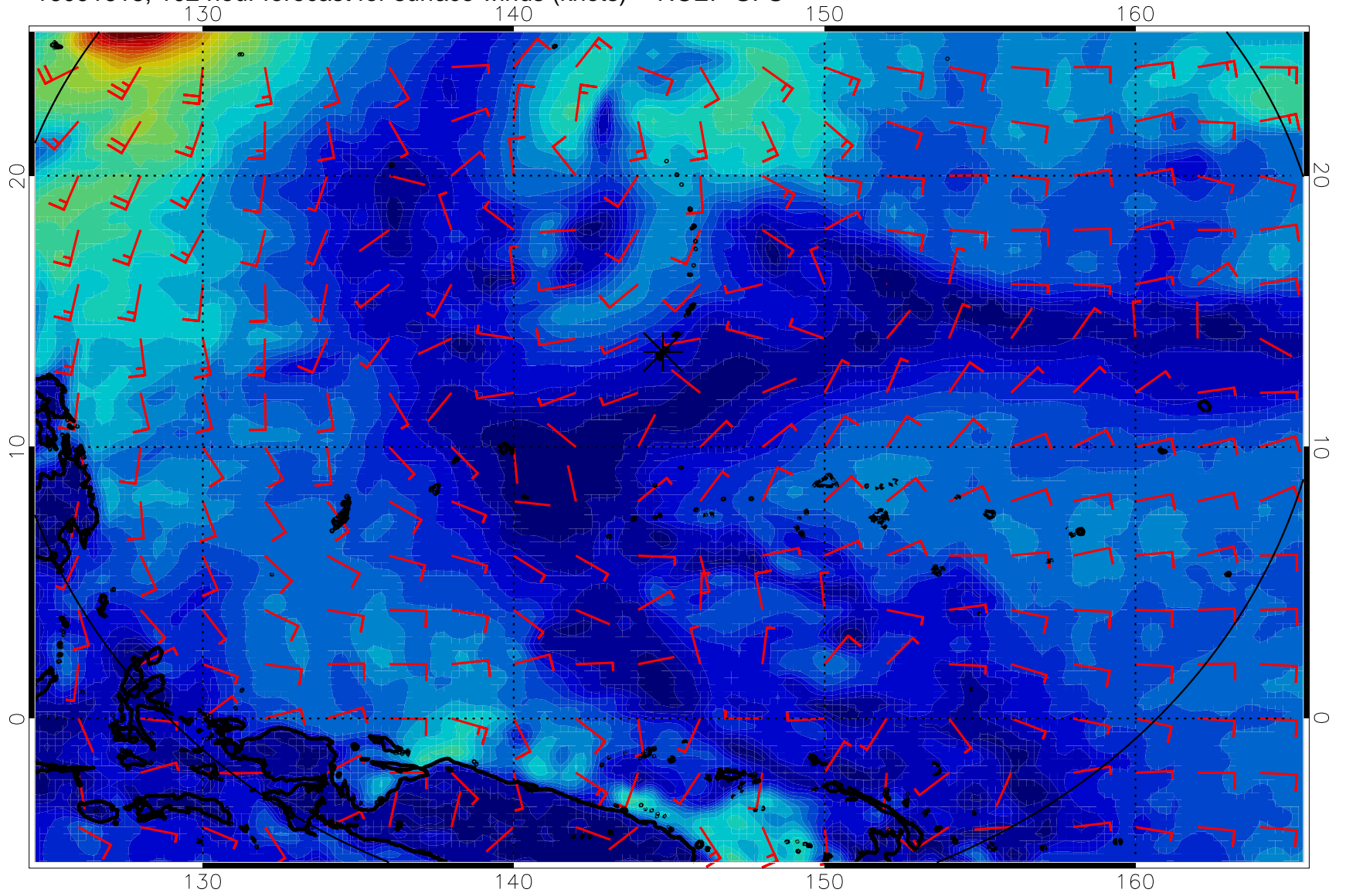
16091618, 102 hour forecast for surface winds (knots) -- NCEP GFS
