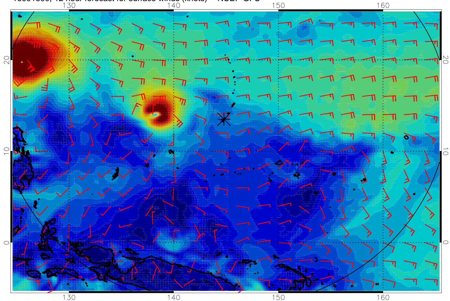
16091300, 12 hour forecast for surface winds (knots) -- NCEP GFS
