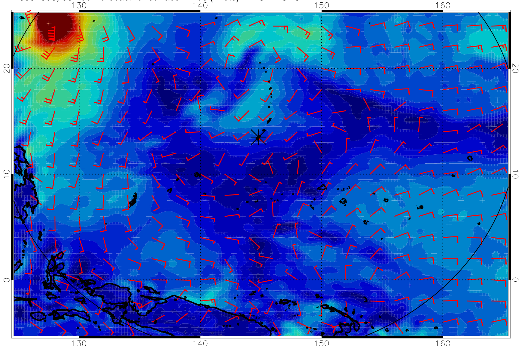
16091606, 90 hour forecast for surface winds (knots) -- NCEP GFS
