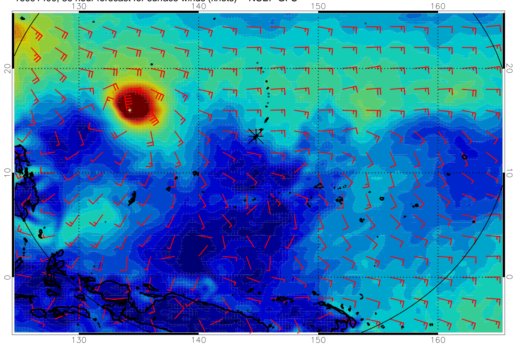
16091400, 36 hour forecast for surface winds (knots) -- NCEP GFS
