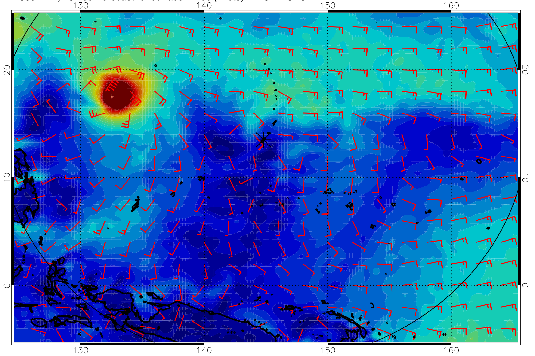
16091412, 48 hour forecast for surface winds (knots) -- NCEP GFS
