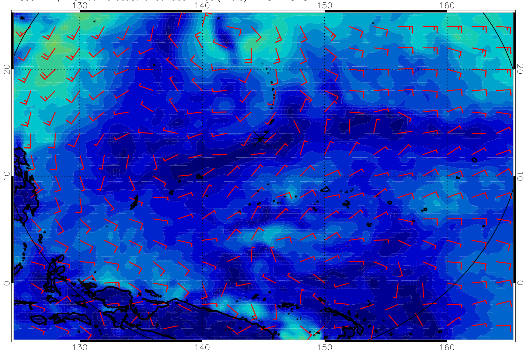
16091712, 120 hour forecast for surface winds (knots) -- NCEP GFS
