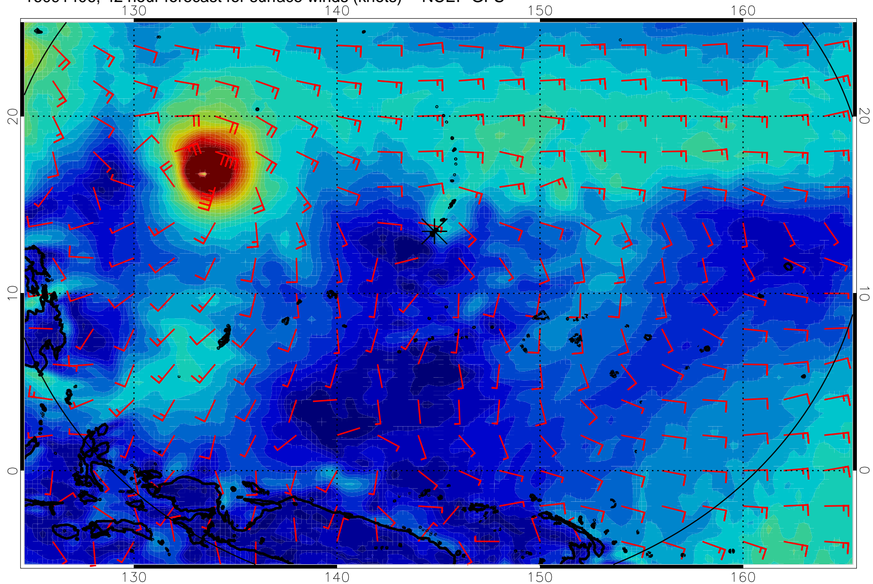
16091406, 42 hour forecast for surface winds (knots) -- NCEP GFS
