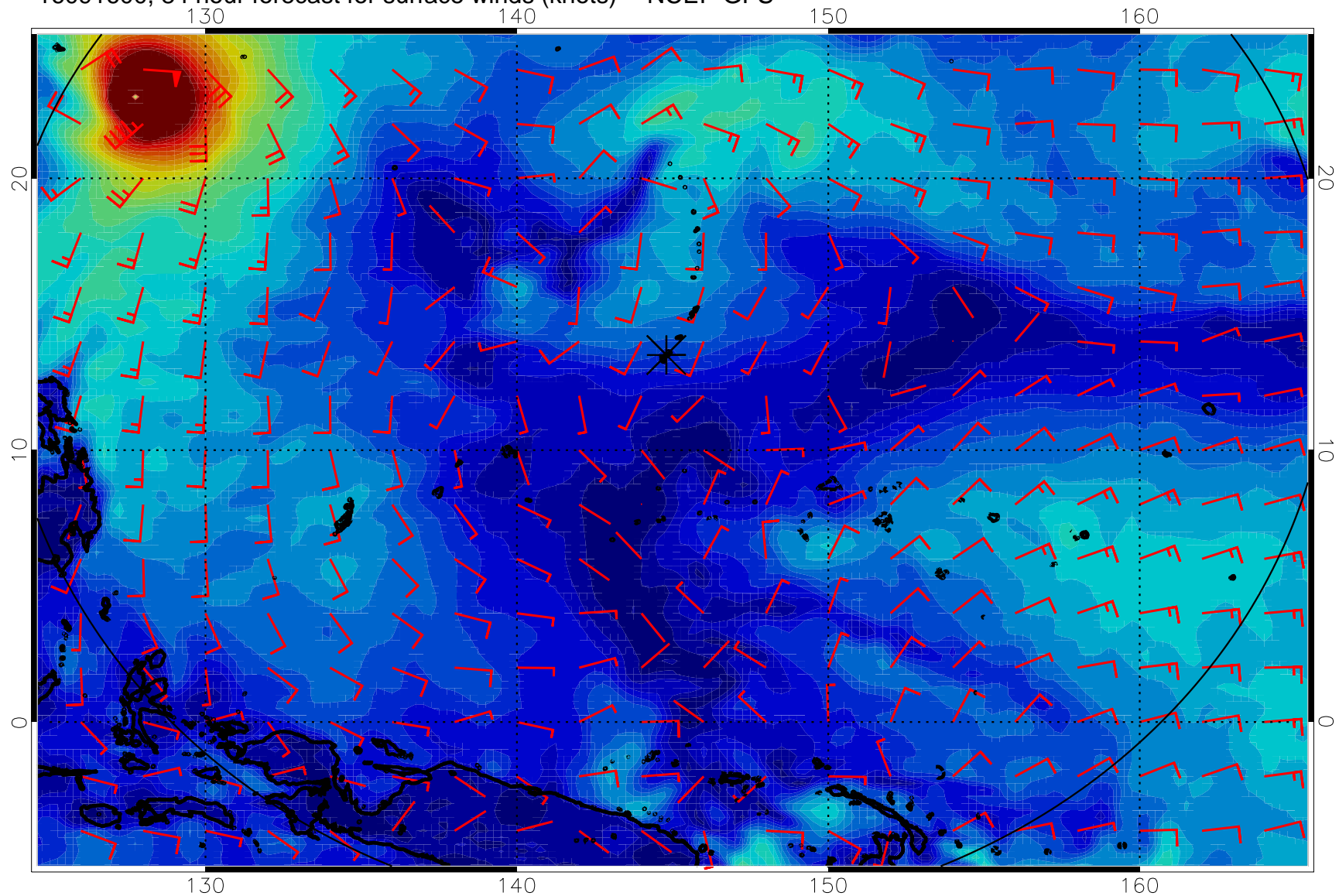
16091600, 84 hour forecast for surface winds (knots) -- NCEP GFS
