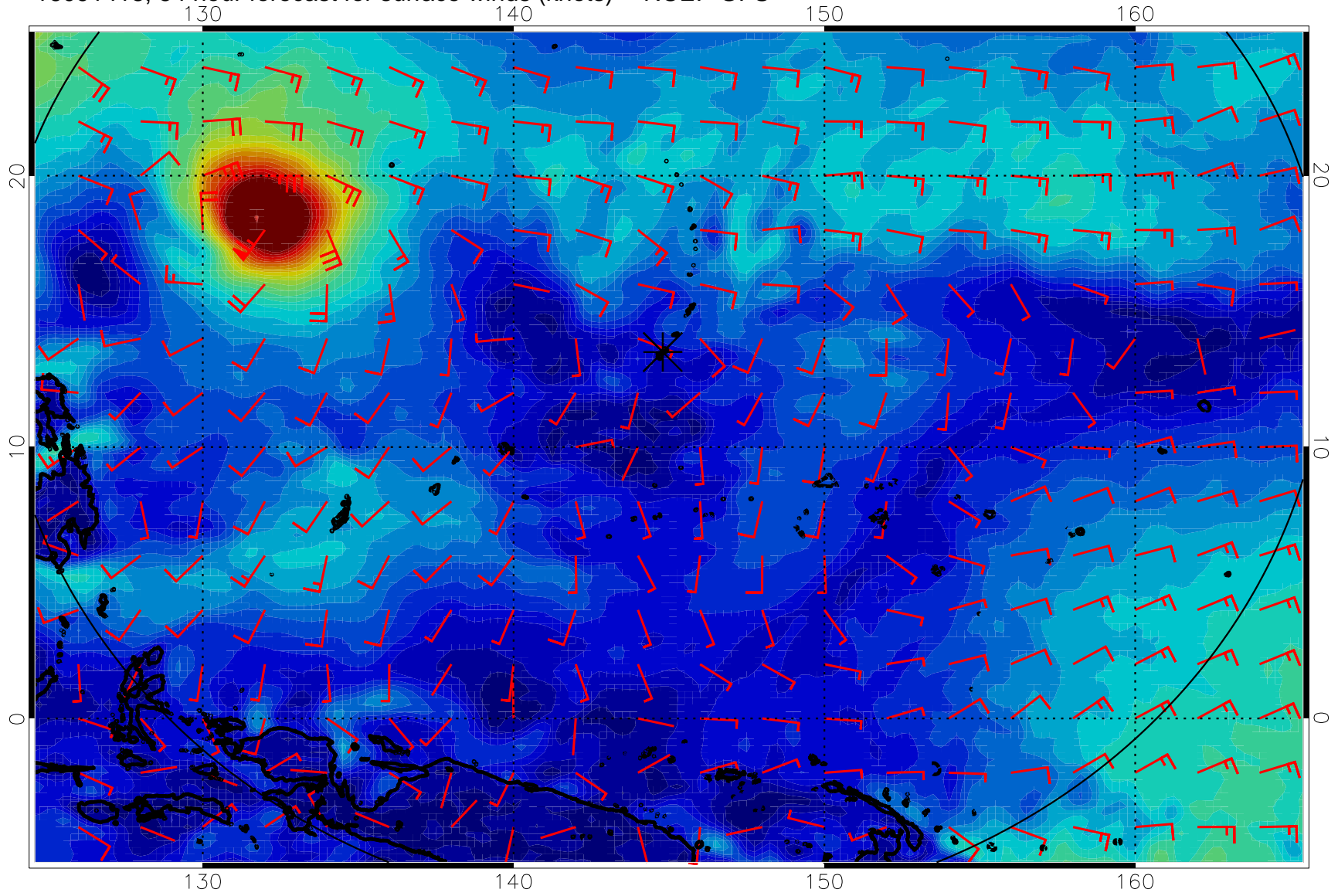
16091418, 54 hour forecast for surface winds (knots) -- NCEP GFS
