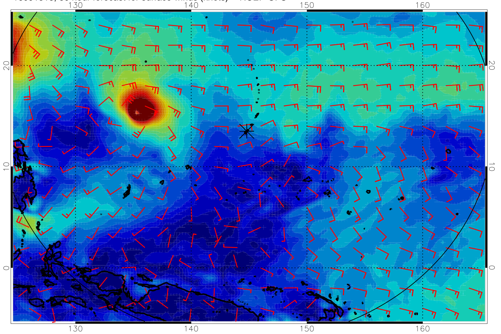
16091318, 30 hour forecast for surface winds (knots) -- NCEP GFS
