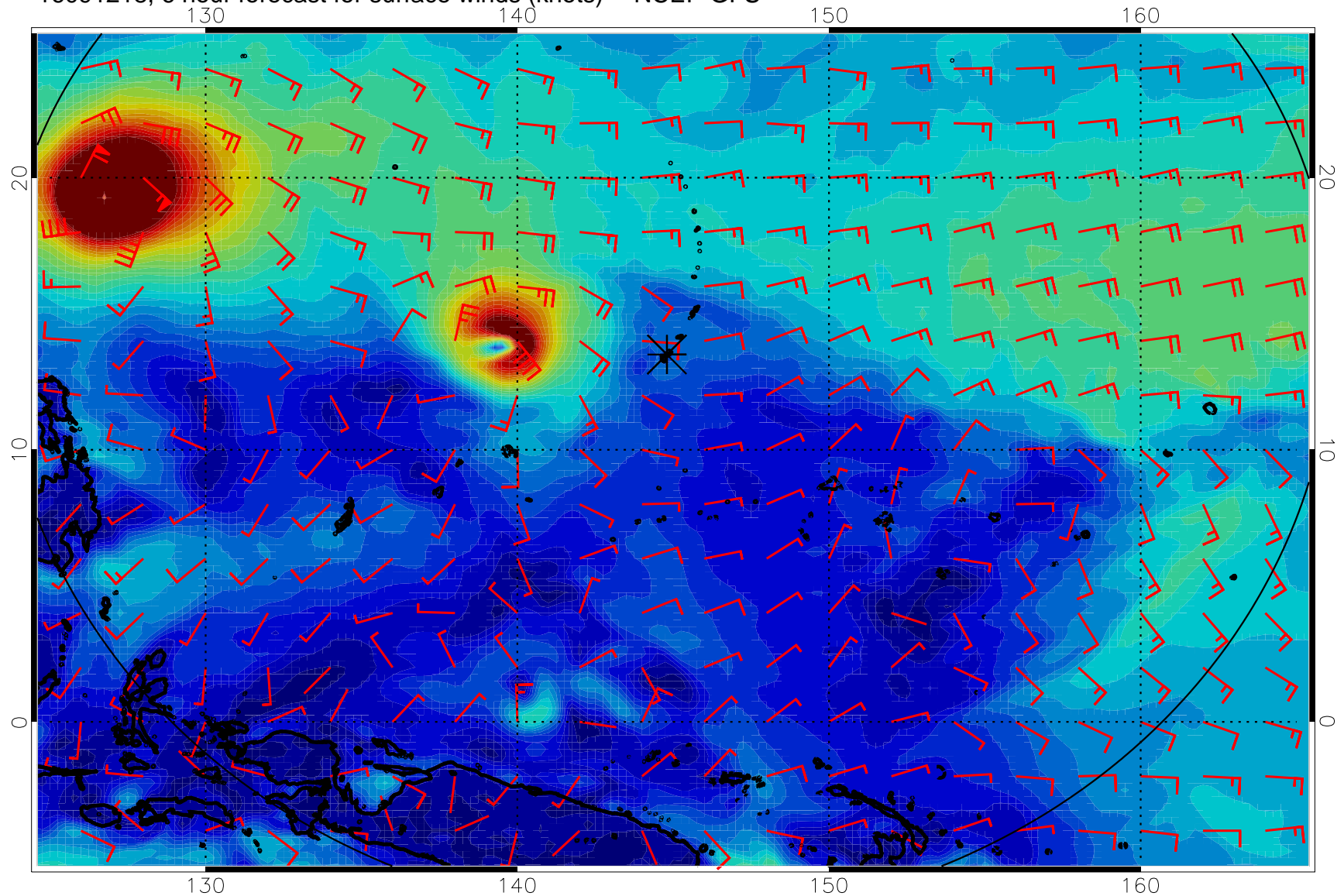
16091218, 6 hour forecast for surface winds (knots) -- NCEP GFS
