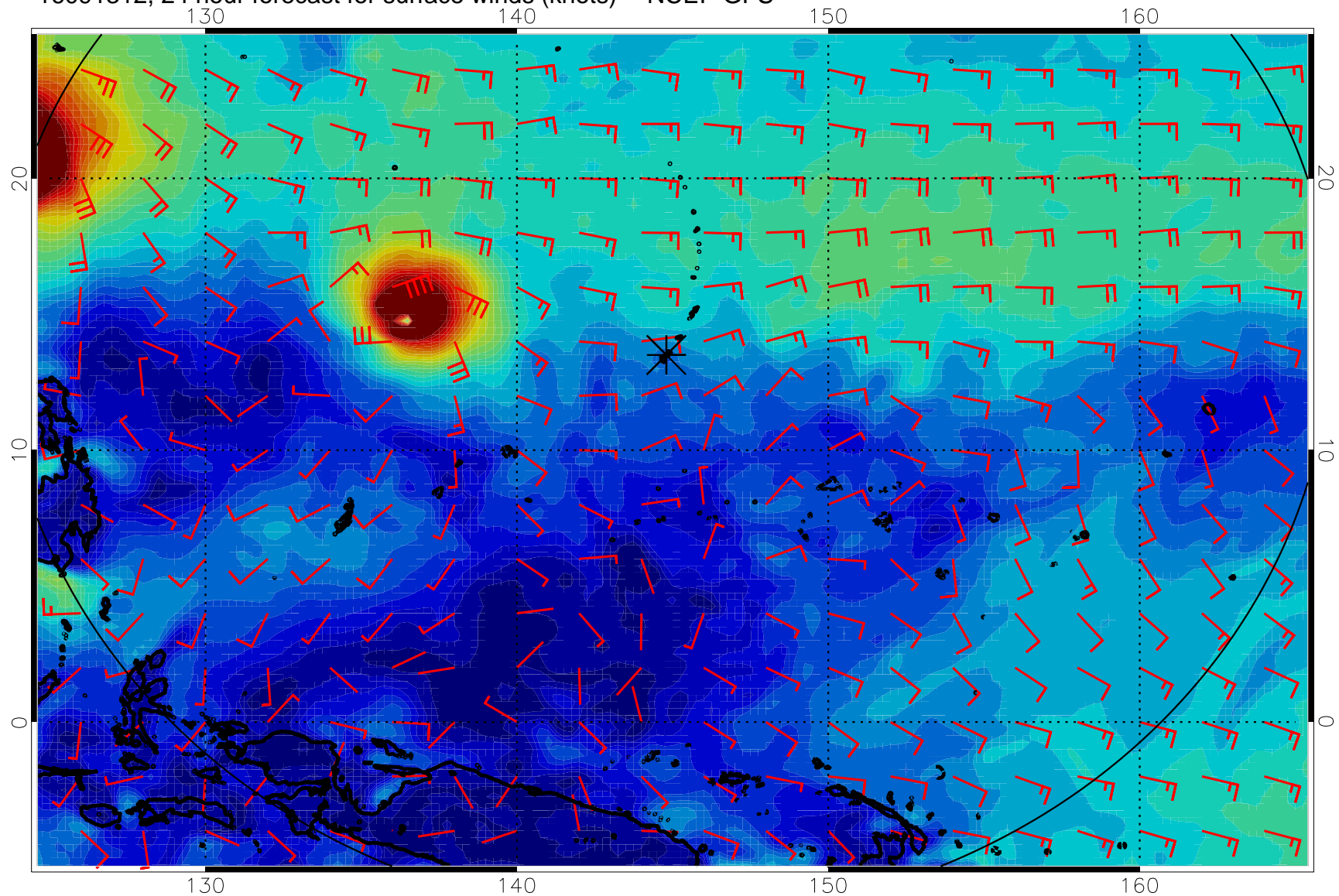
16091312, 24 hour forecast for surface winds (knots) -- NCEP GFS
