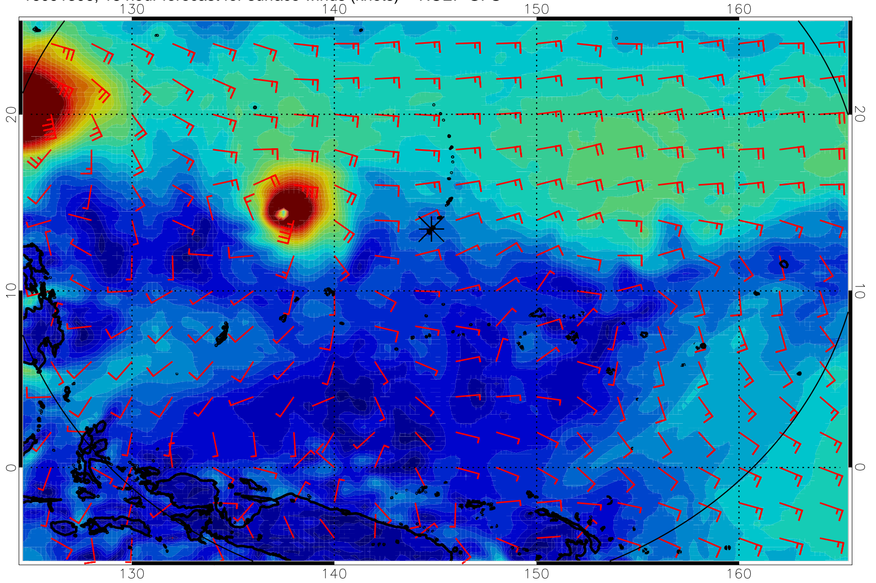
16091306, 18 hour forecast for surface winds (knots) -- NCEP GFS
