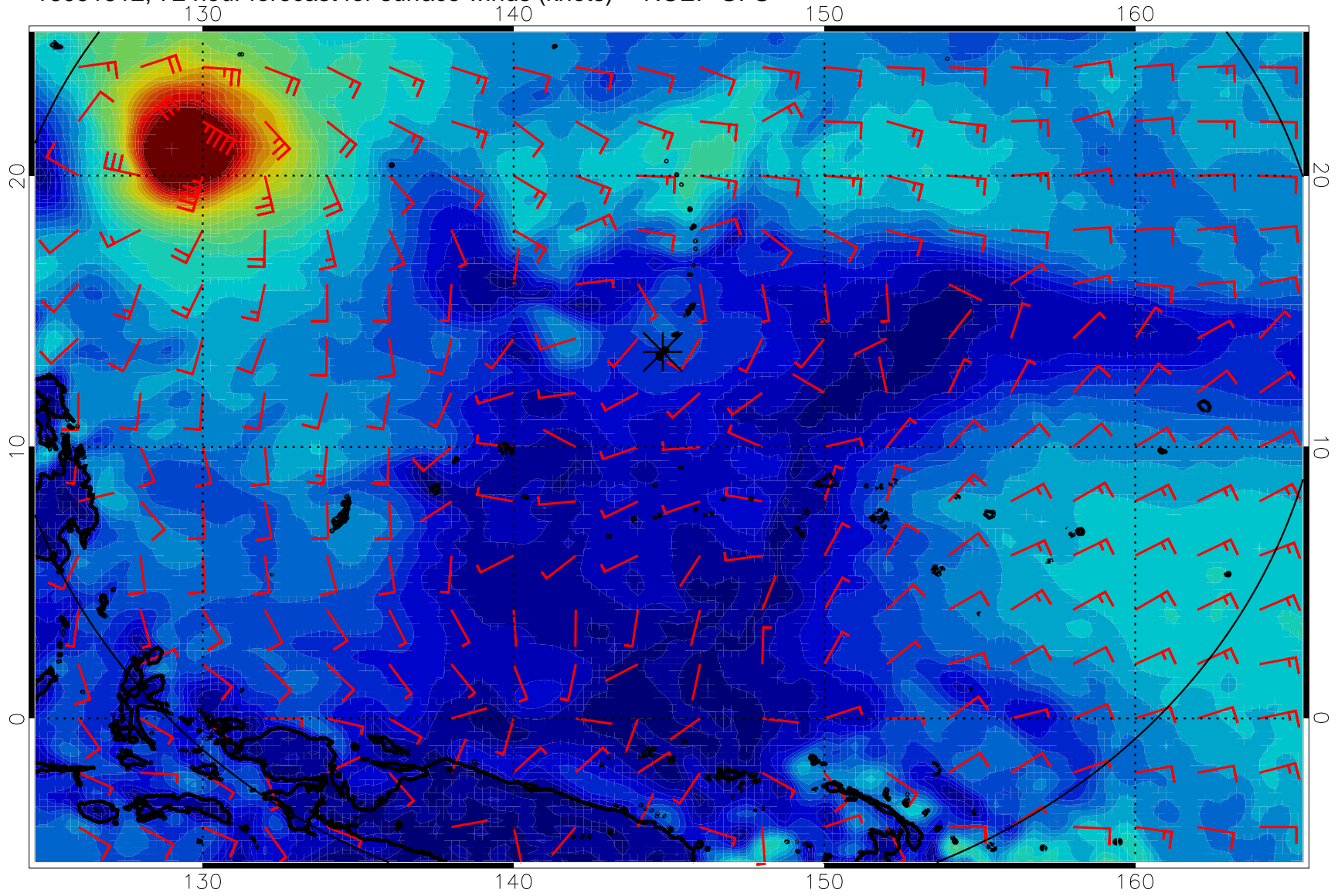
16091512, 72 hour forecast for surface winds (knots) -- NCEP GFS
