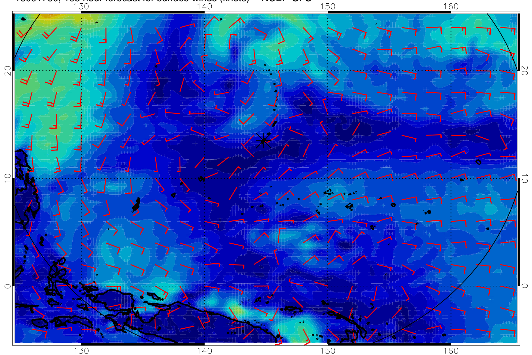
16091700, 108 hour forecast for surface winds (knots) -- NCEP GFS
