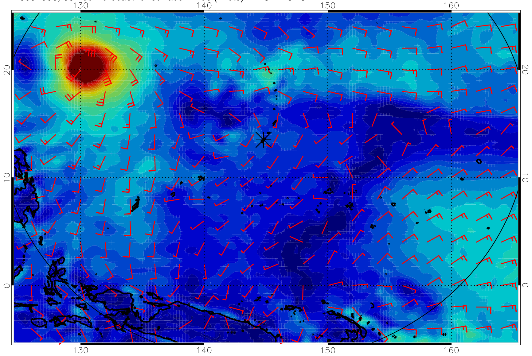
16091506, 66 hour forecast for surface winds (knots) -- NCEP GFS
