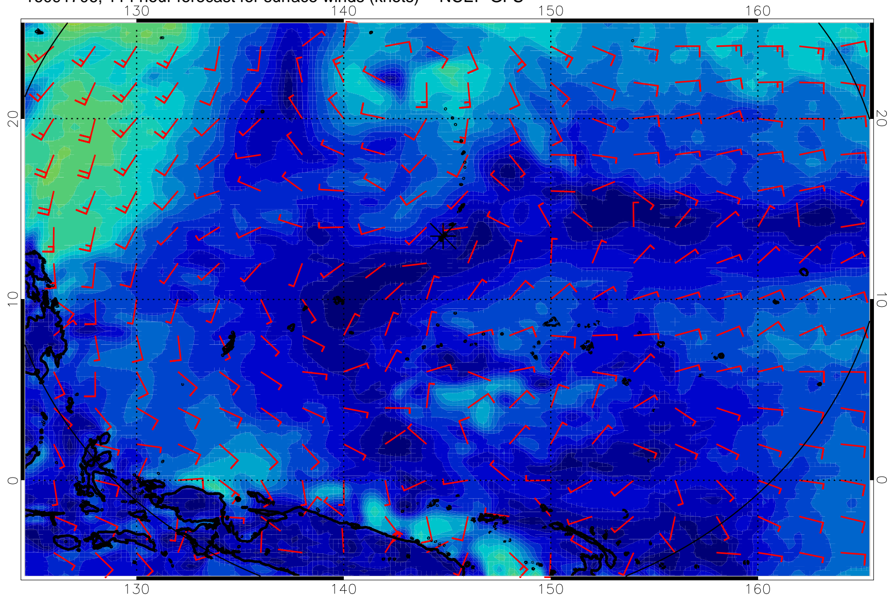
16091706, 114 hour forecast for surface winds (knots) -- NCEP GFS
