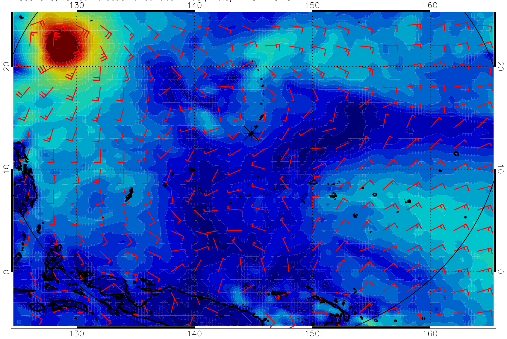
16091518, 78 hour forecast for surface winds (knots) -- NCEP GFS
