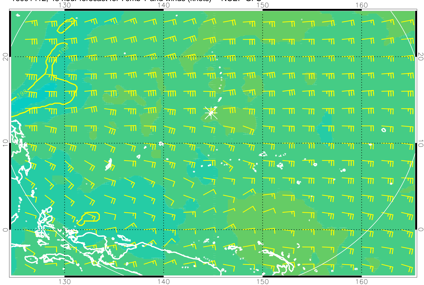
16091412, 48 hour forecast for 70mb T and winds (knots) -- NCEP GFS
