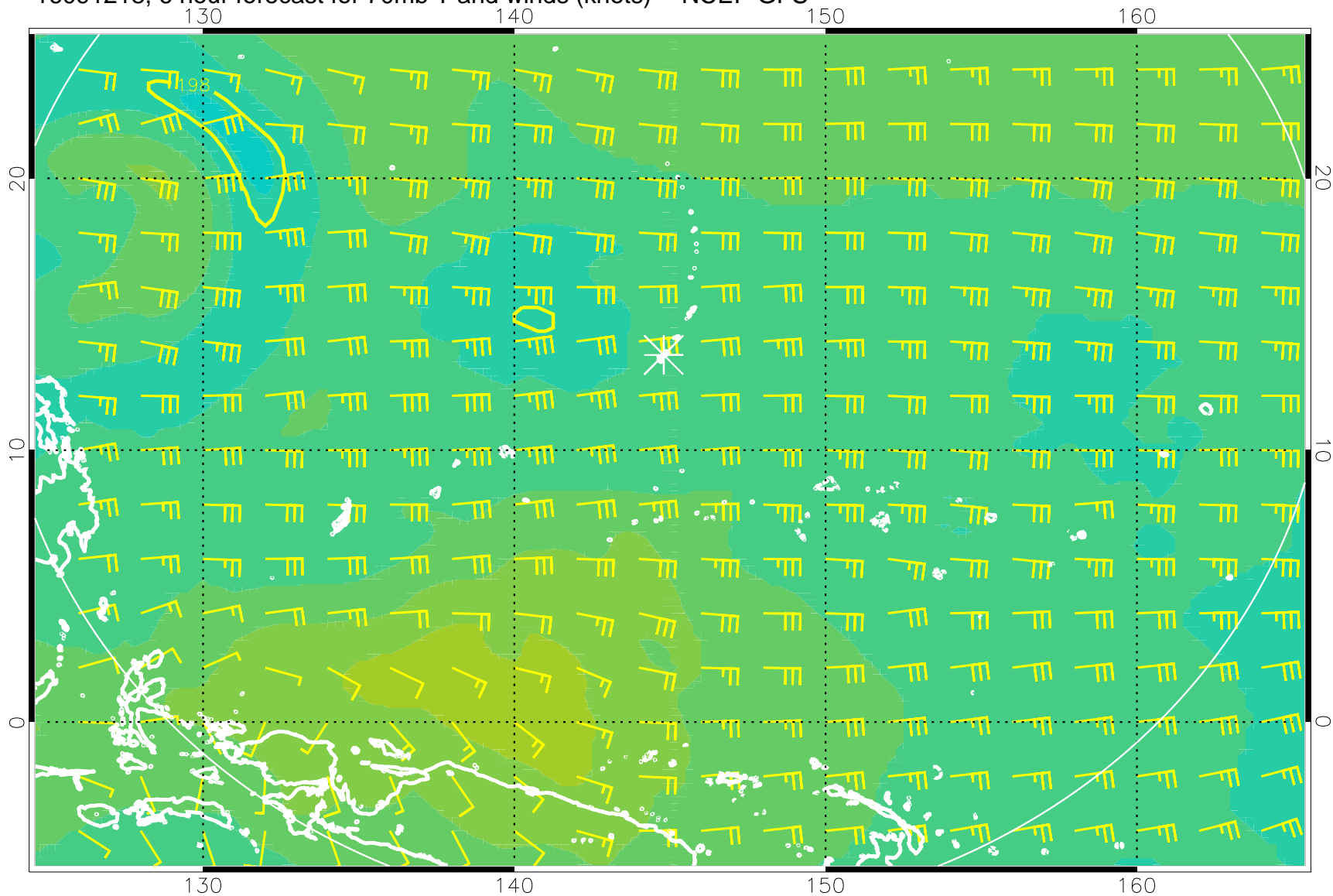
16091218, 6 hour forecast for 70mb T and winds (knots) -- NCEP GFS
