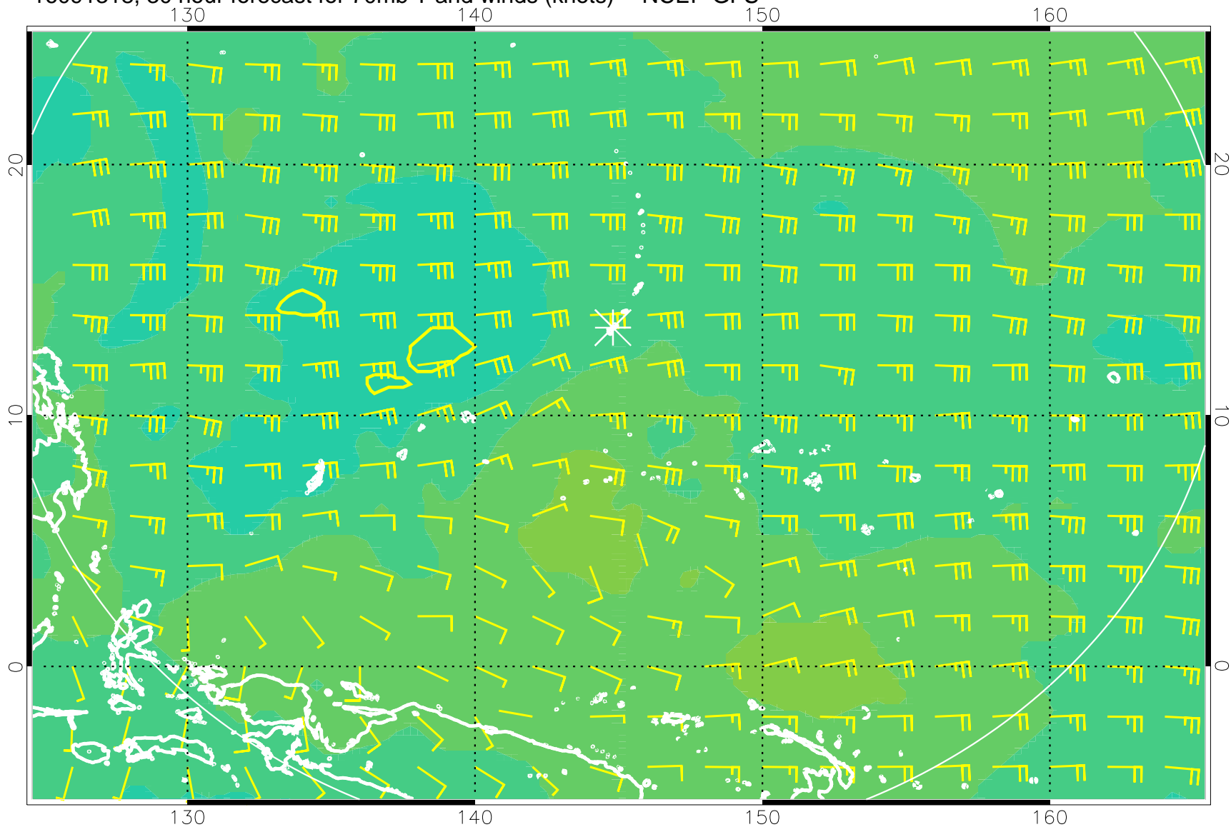
16091318, 30 hour forecast for 70mb T and winds (knots) -- NCEP GFS
