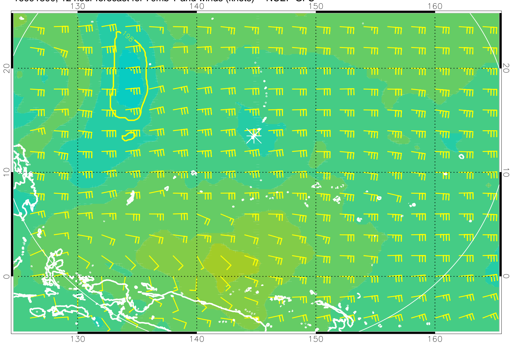
16091300, 12 hour forecast for 70mb T and winds (knots) -- NCEP GFS
