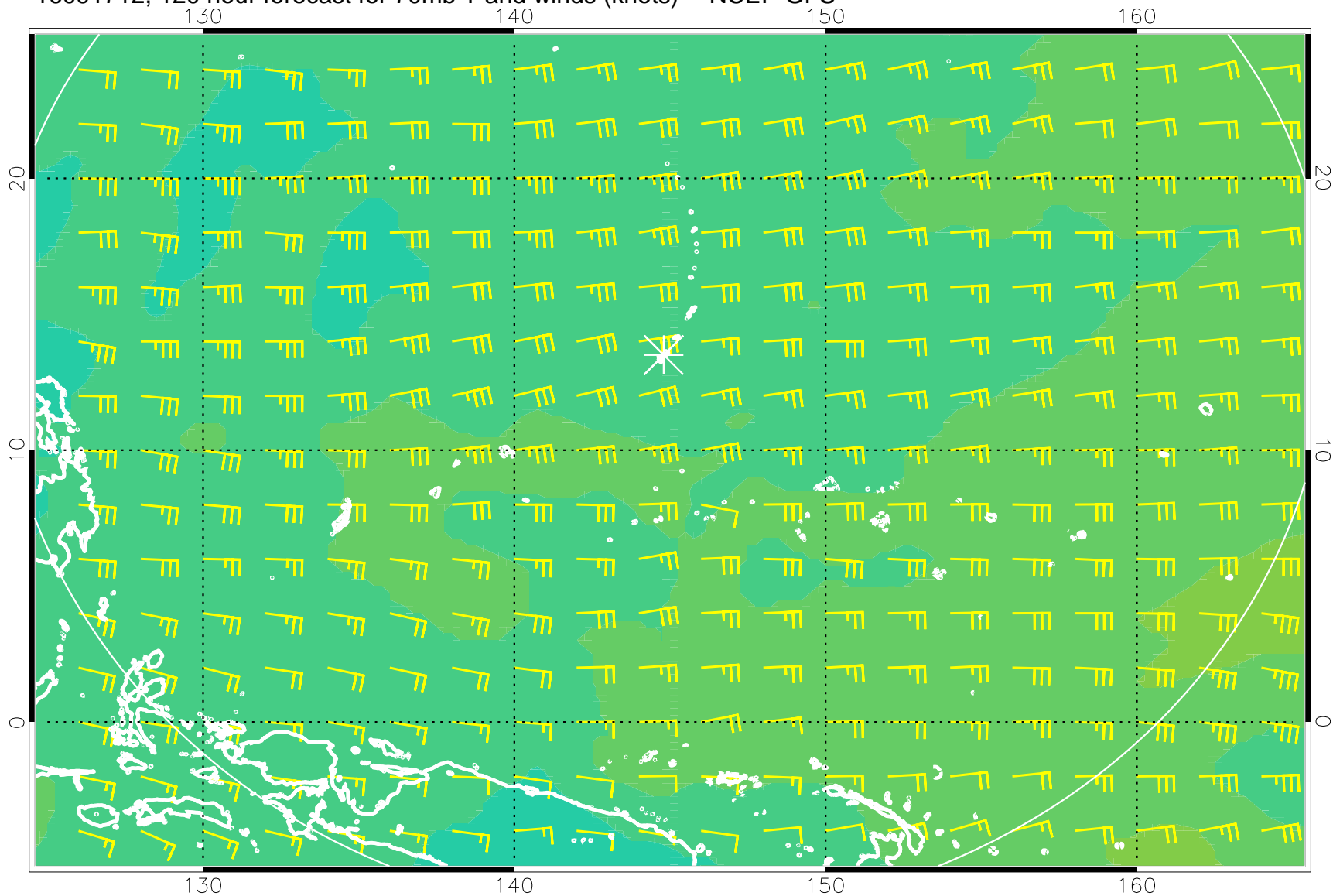
16091712, 120 hour forecast for 70mb T and winds (knots) -- NCEP GFS
