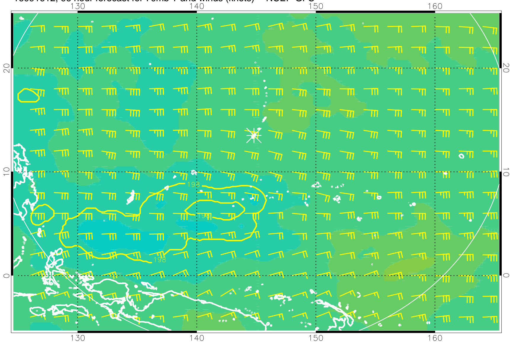
16091612, 96 hour forecast for 70mb T and winds (knots) -- NCEP GFS
