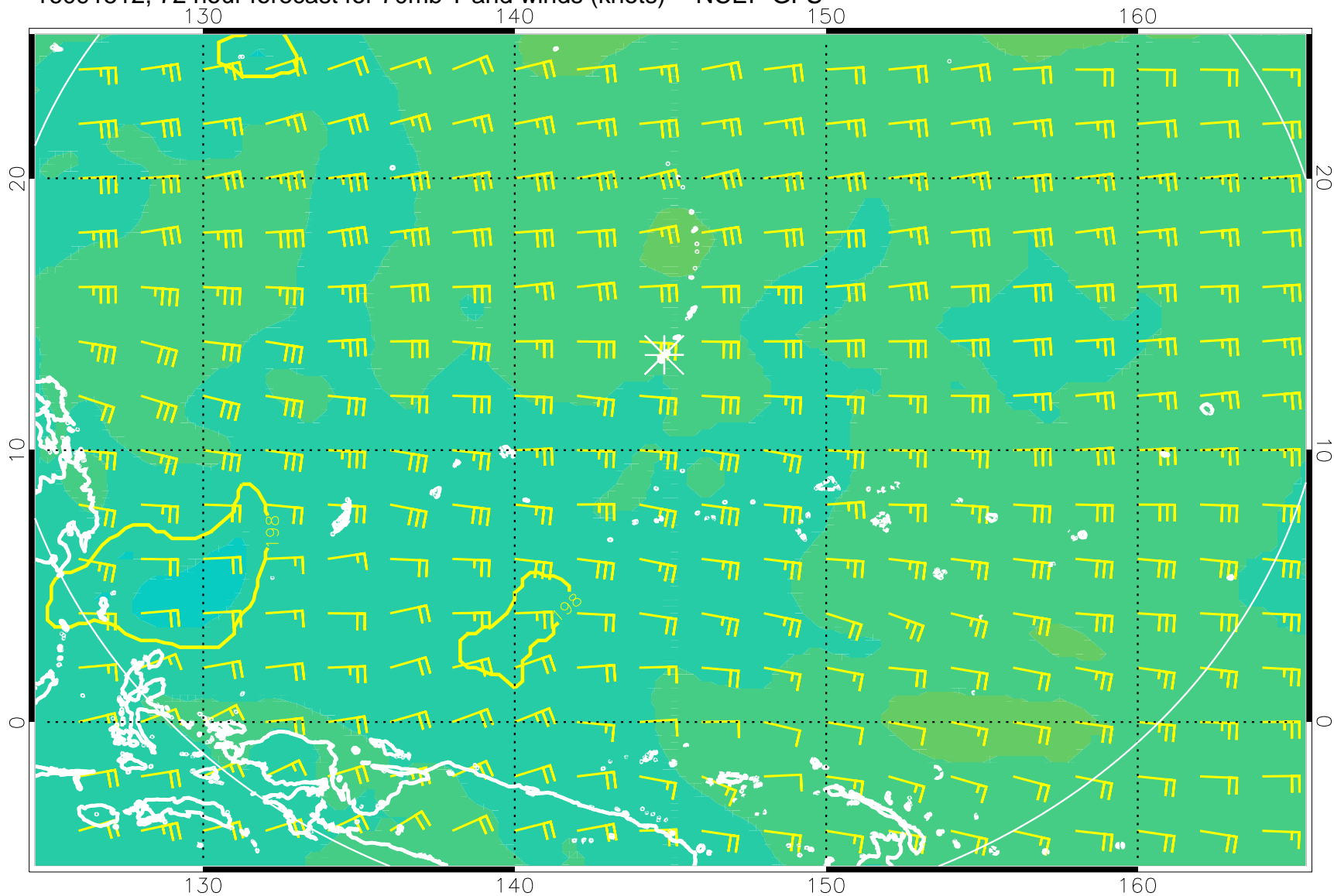
16091512, 72 hour forecast for 70mb T and winds (knots) -- NCEP GFS
