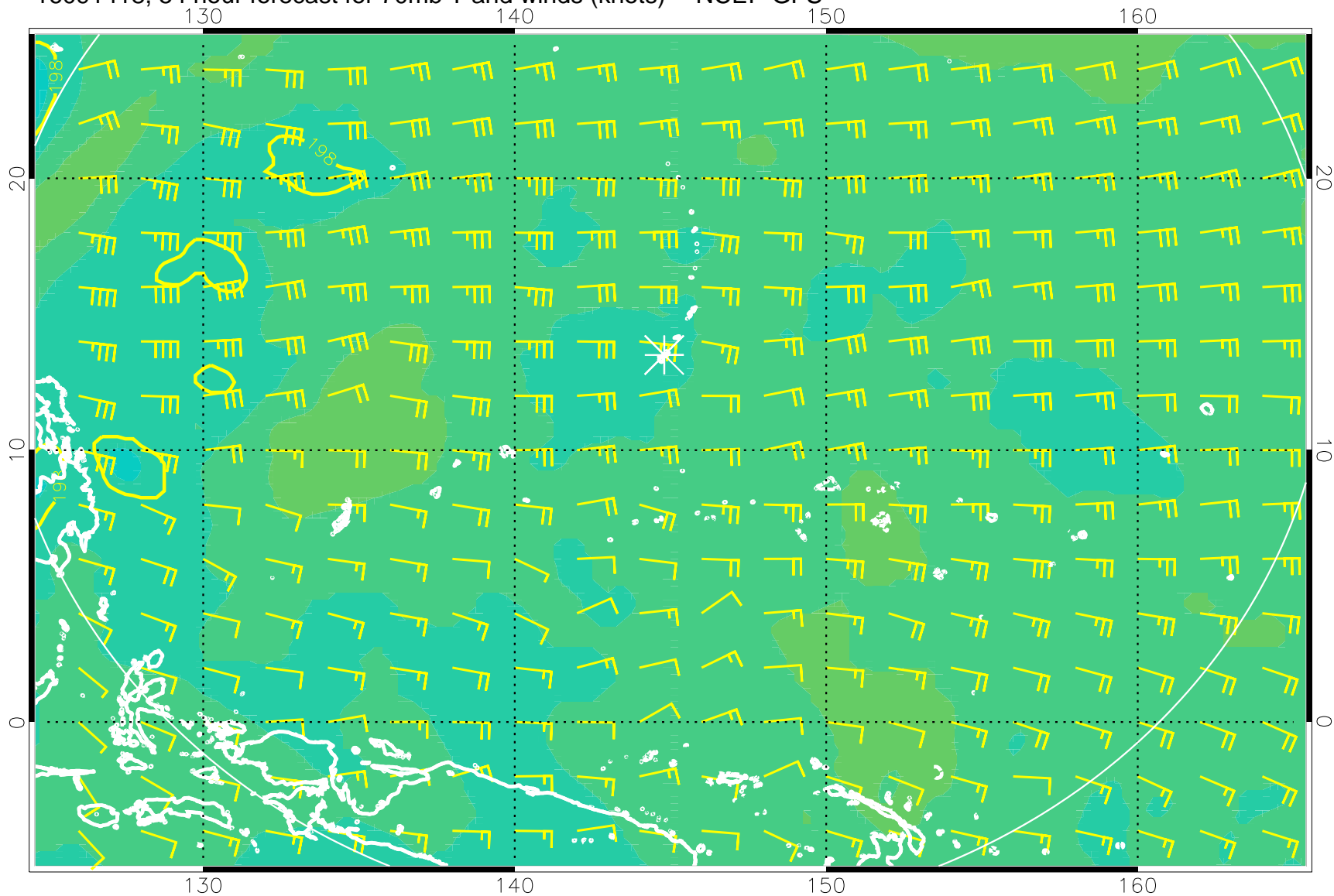
16091418, 54 hour forecast for 70mb T and winds (knots) -- NCEP GFS
