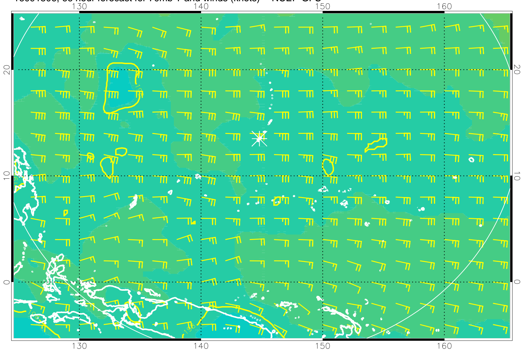
16091506, 66 hour forecast for 70mb T and winds (knots) -- NCEP GFS
