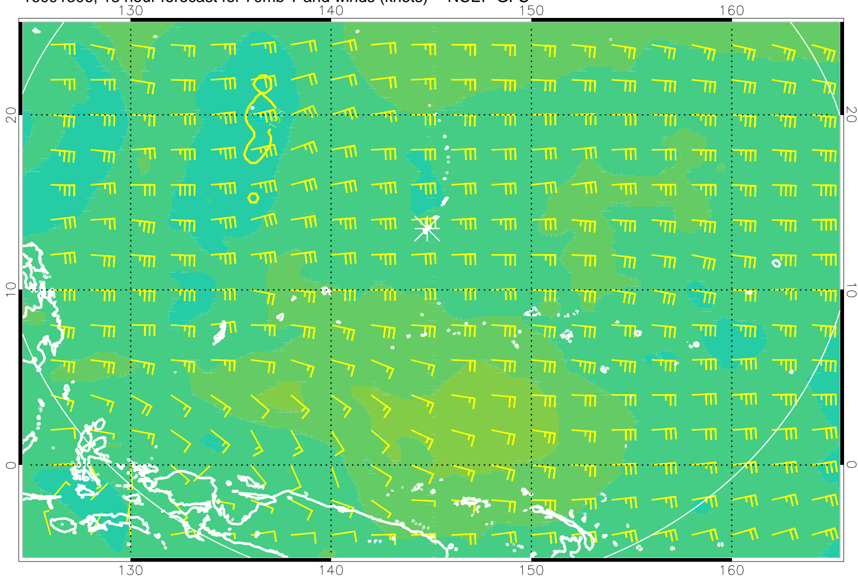
16091306, 18 hour forecast for 70mb T and winds (knots) -- NCEP GFS
