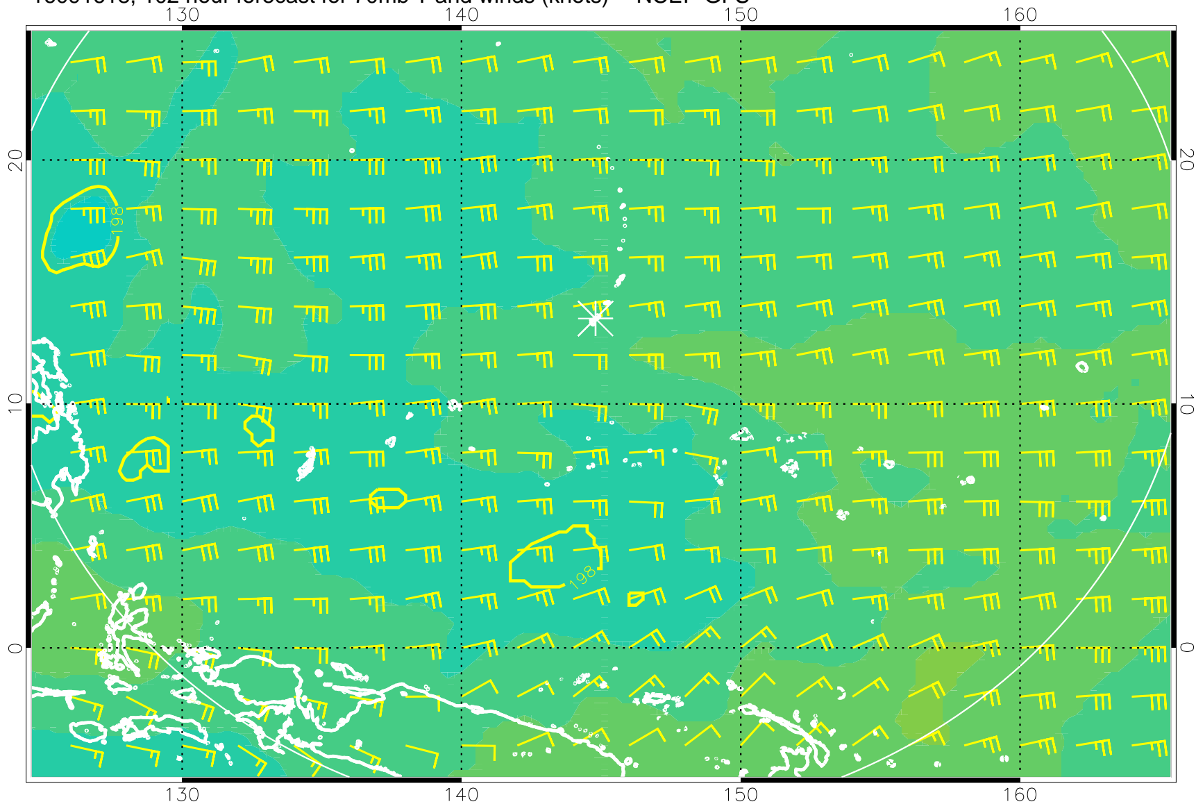
16091618, 102 hour forecast for 70mb T and winds (knots) -- NCEP GFS
