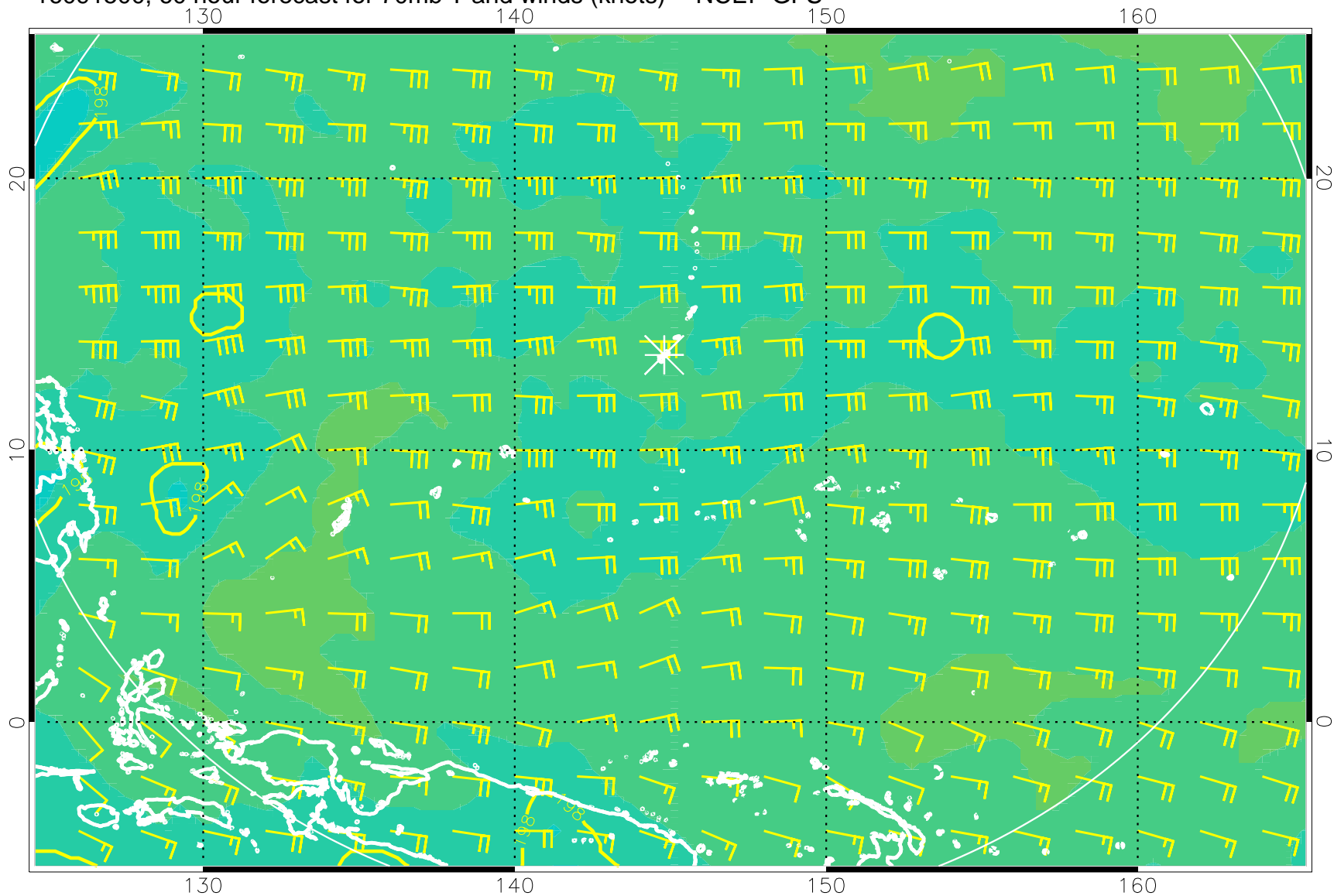
16091500, 60 hour forecast for 70mb T and winds (knots) -- NCEP GFS
