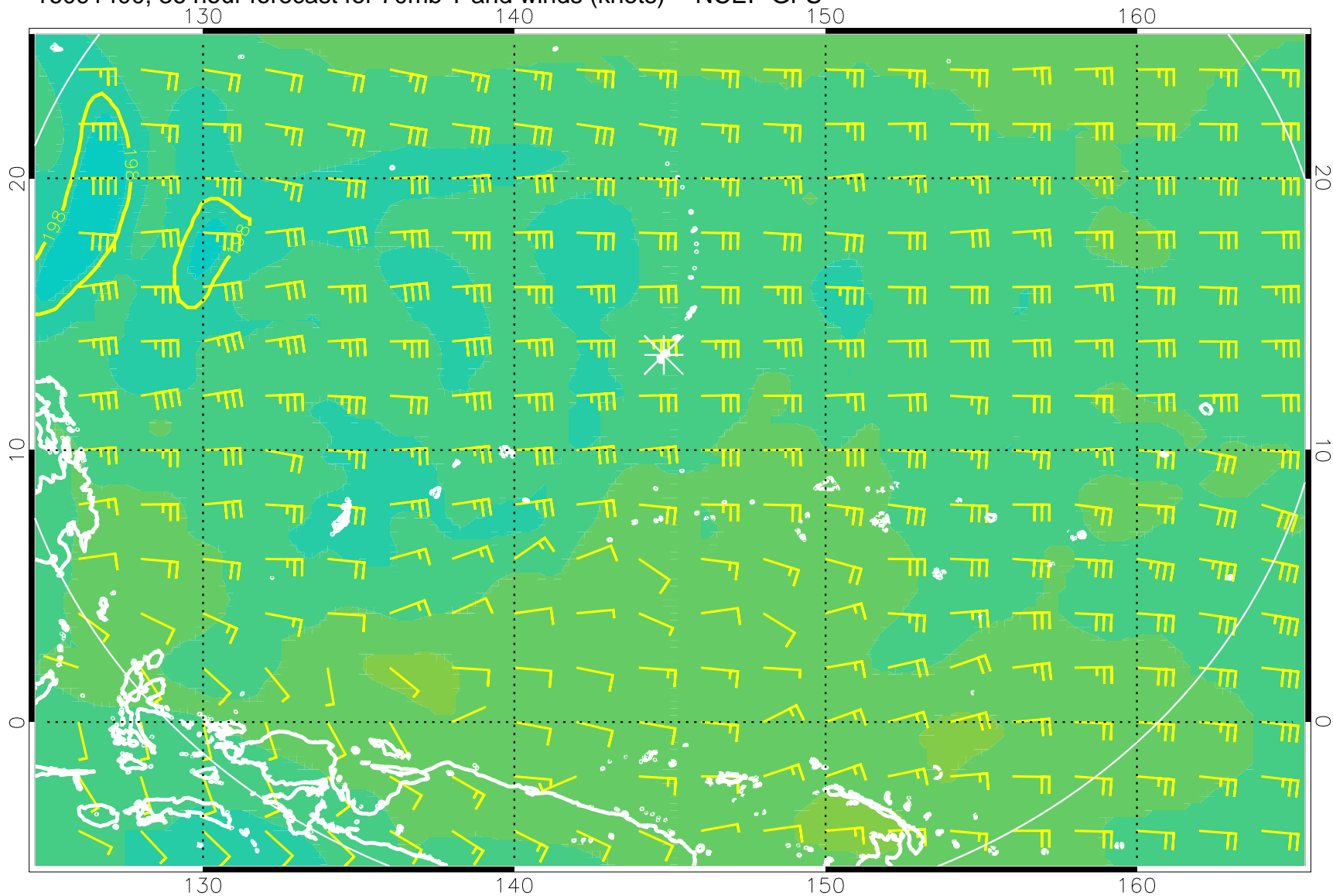
16091400, 36 hour forecast for 70mb T and winds (knots) -- NCEP GFS
