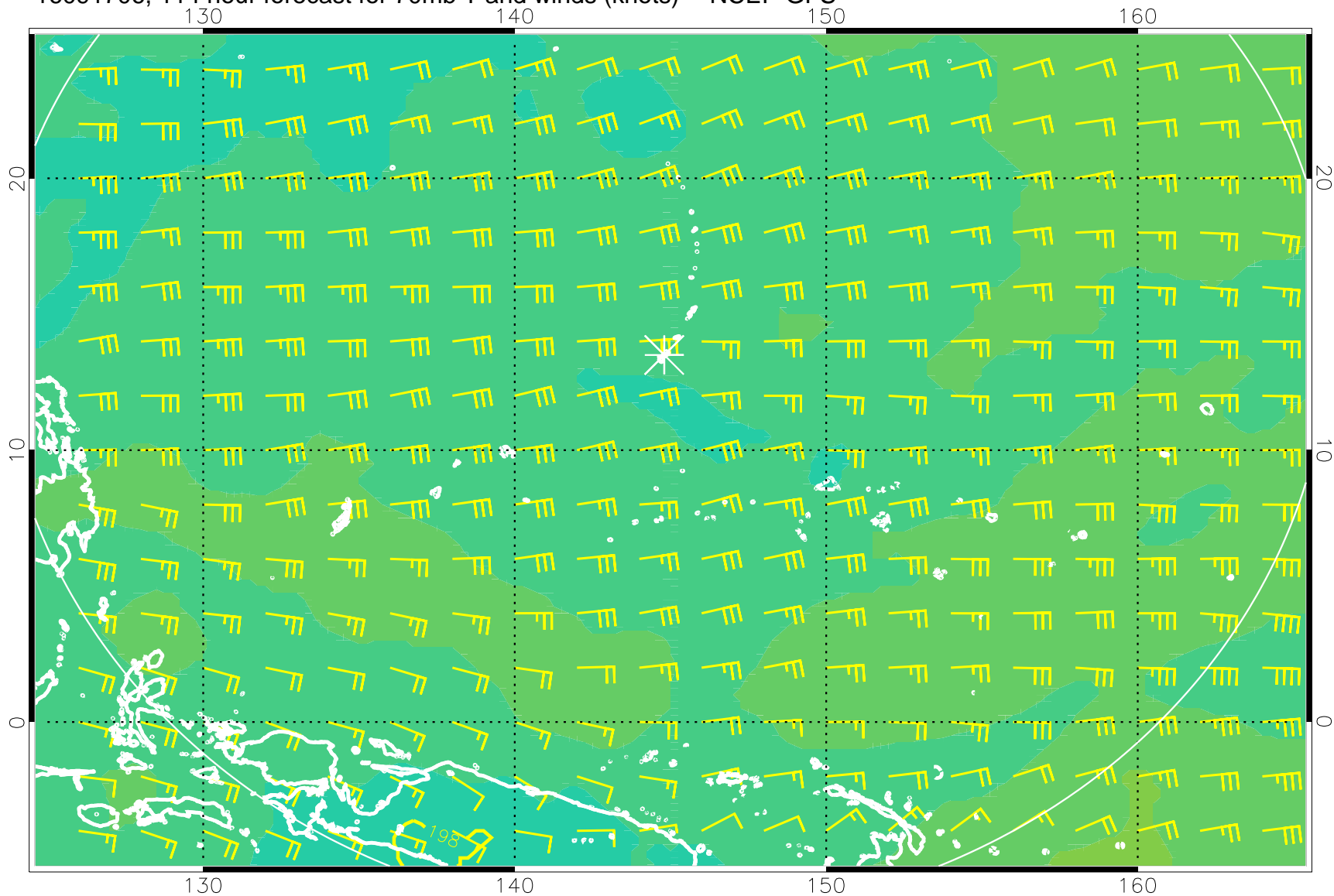
16091706, 114 hour forecast for 70mb T and winds (knots) -- NCEP GFS
