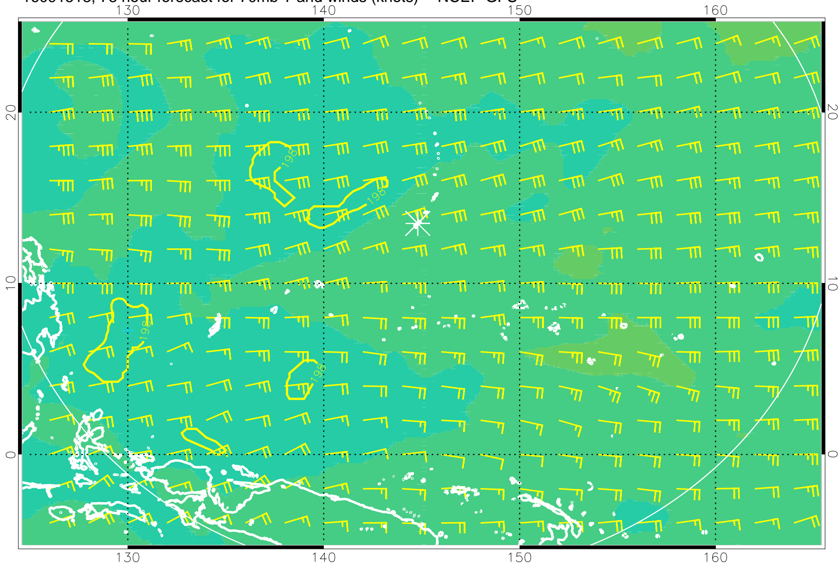
16091518, 78 hour forecast for 70mb T and winds (knots) -- NCEP GFS
