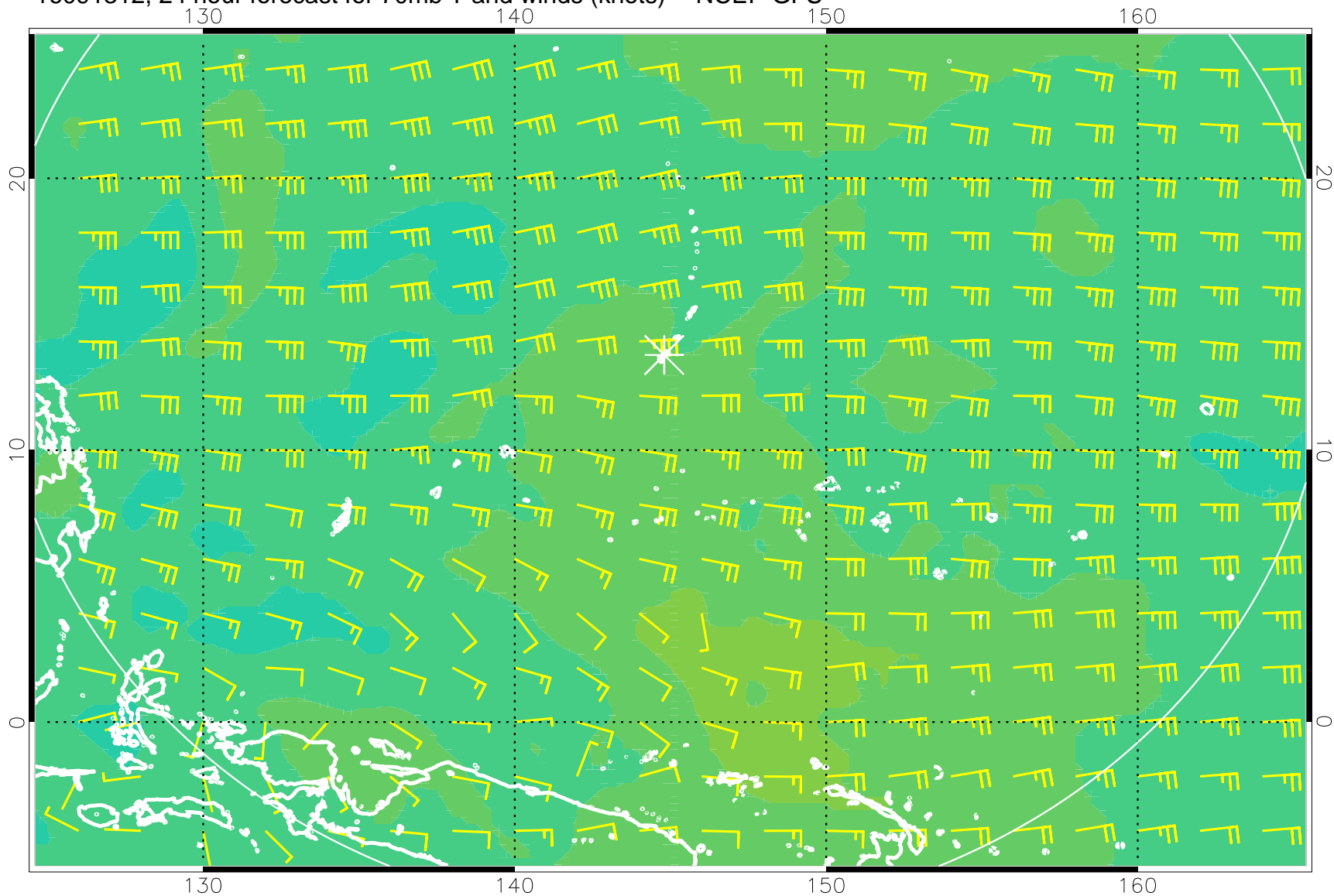
16091312, 24 hour forecast for 70mb T and winds (knots) -- NCEP GFS
