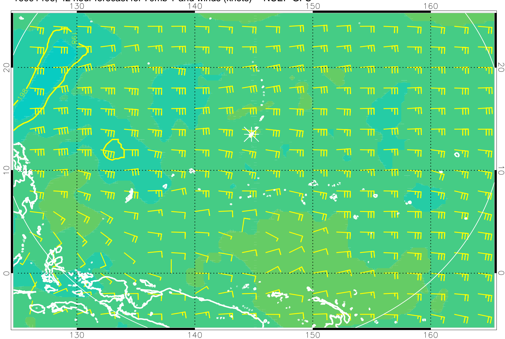
16091406, 42 hour forecast for 70mb T and winds (knots) -- NCEP GFS
