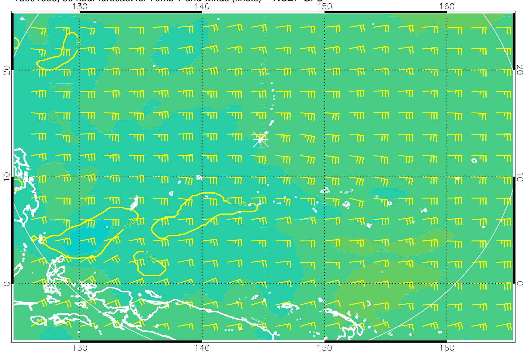
16091606, 90 hour forecast for 70mb T and winds (knots) -- NCEP GFS
