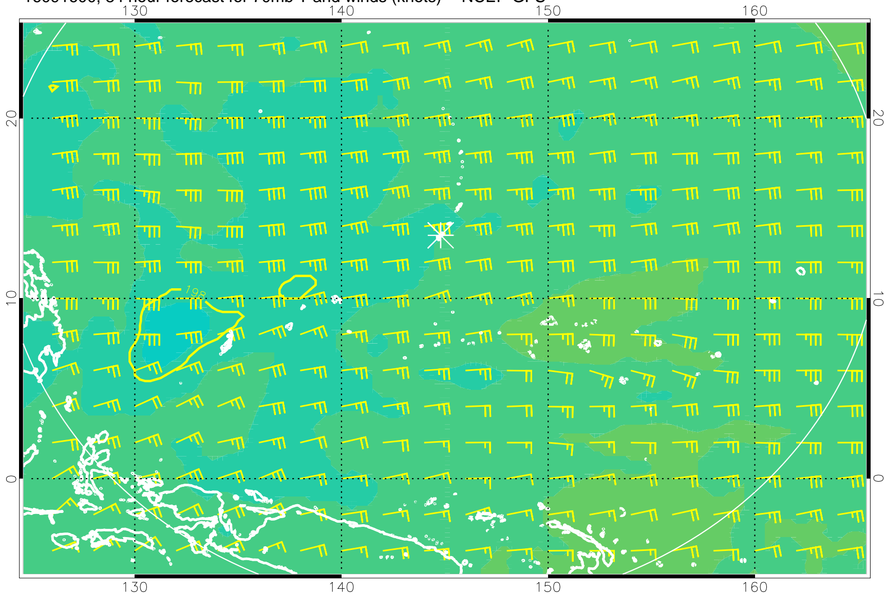
16091600, 84 hour forecast for 70mb T and winds (knots) -- NCEP GFS
