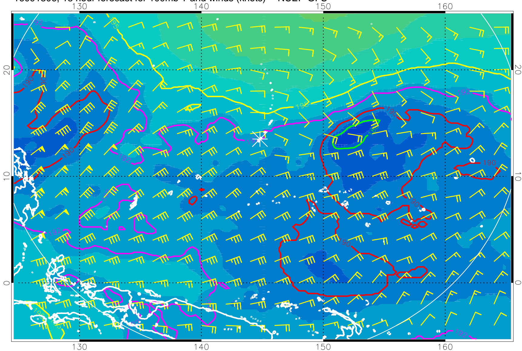
16091306, 18 hour forecast for 100mb T and winds (knots) -- NCEP GFS
