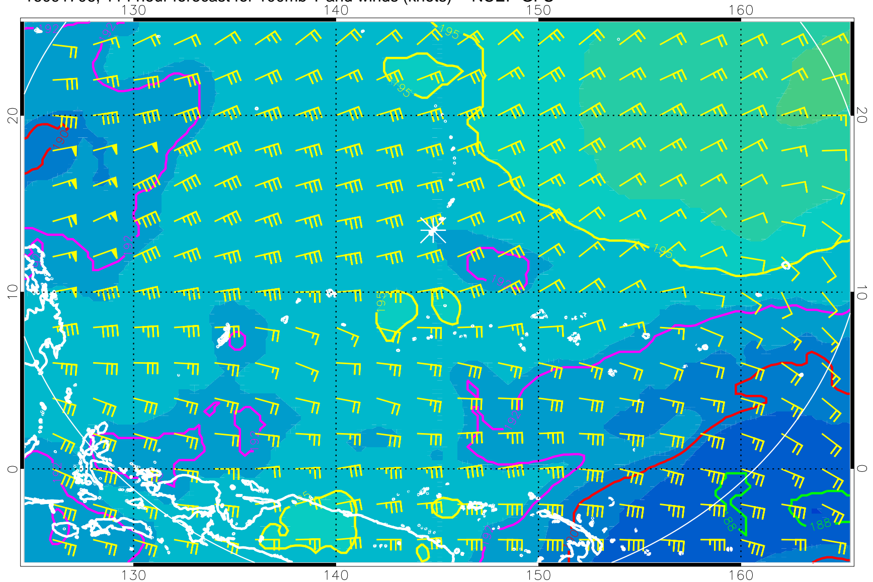
16091706, 114 hour forecast for 100mb T and winds (knots) -- NCEP GFS
