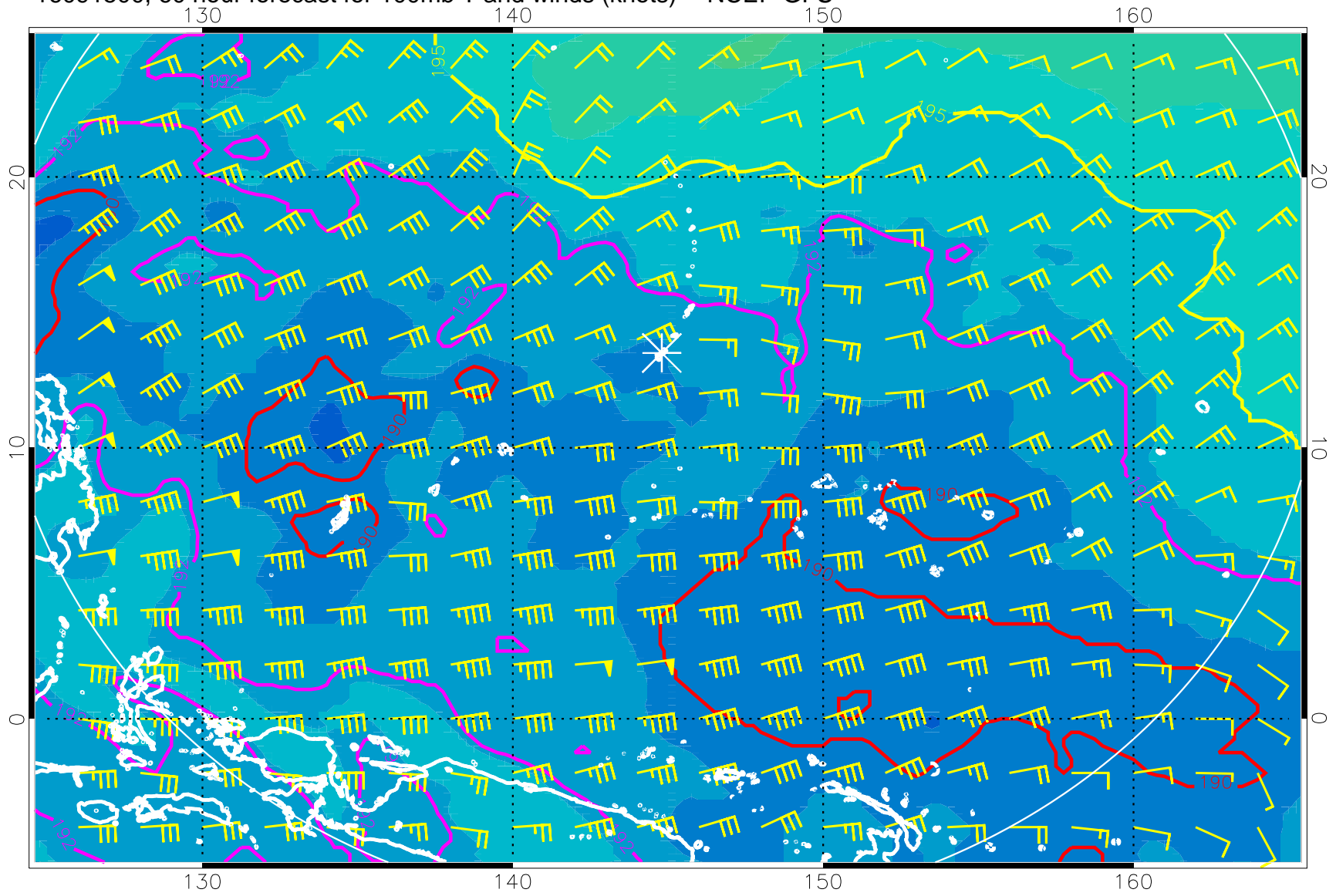
16091500, 60 hour forecast for 100mb T and winds (knots) -- NCEP GFS
