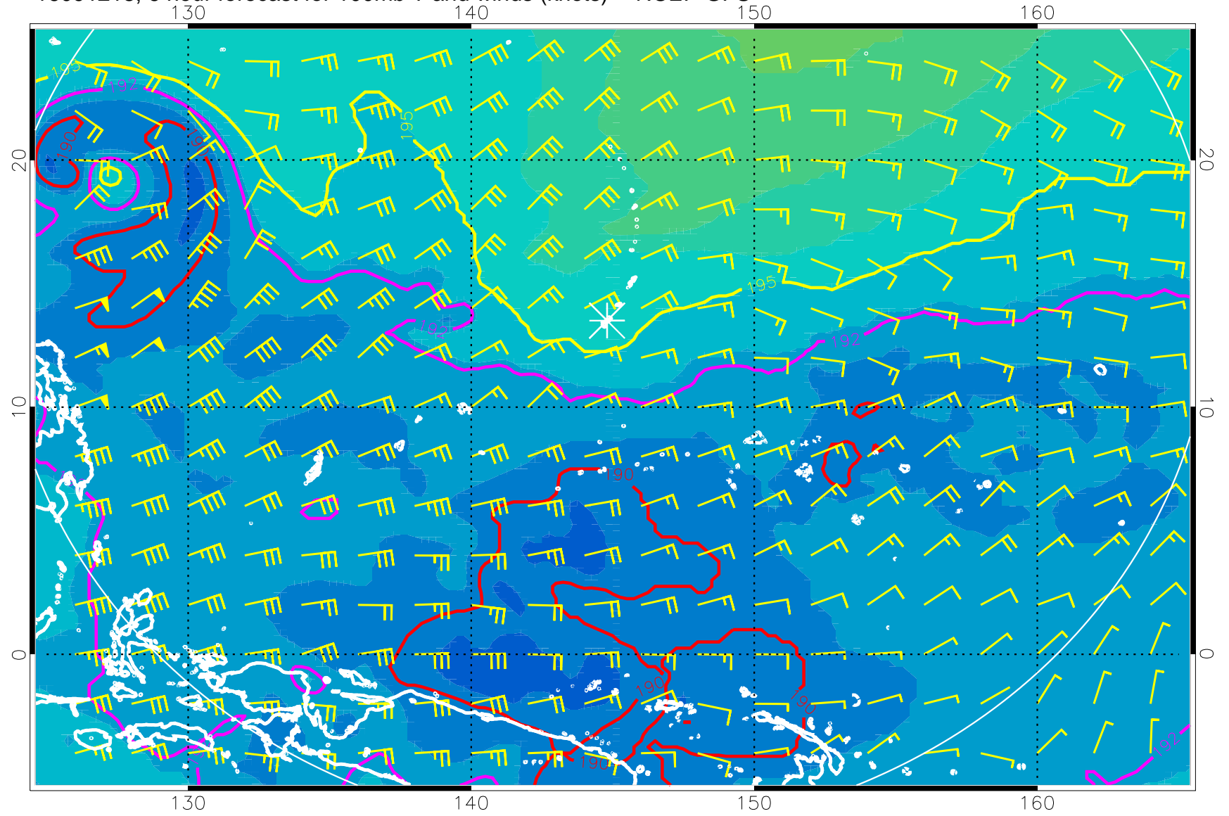
16091218, 6 hour forecast for 100mb T and winds (knots) -- NCEP GFS
