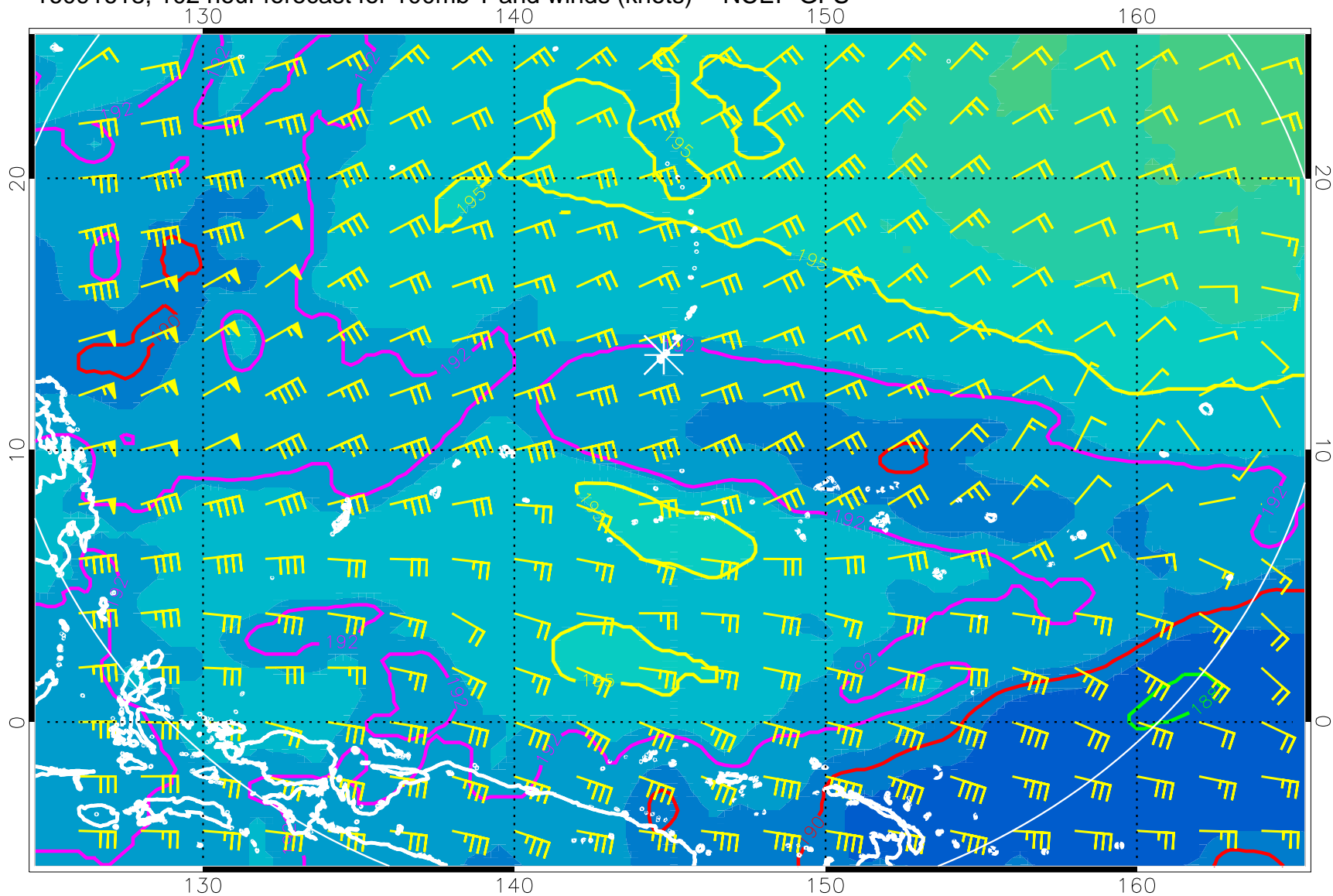
16091618, 102 hour forecast for 100mb T and winds (knots) -- NCEP GFS
