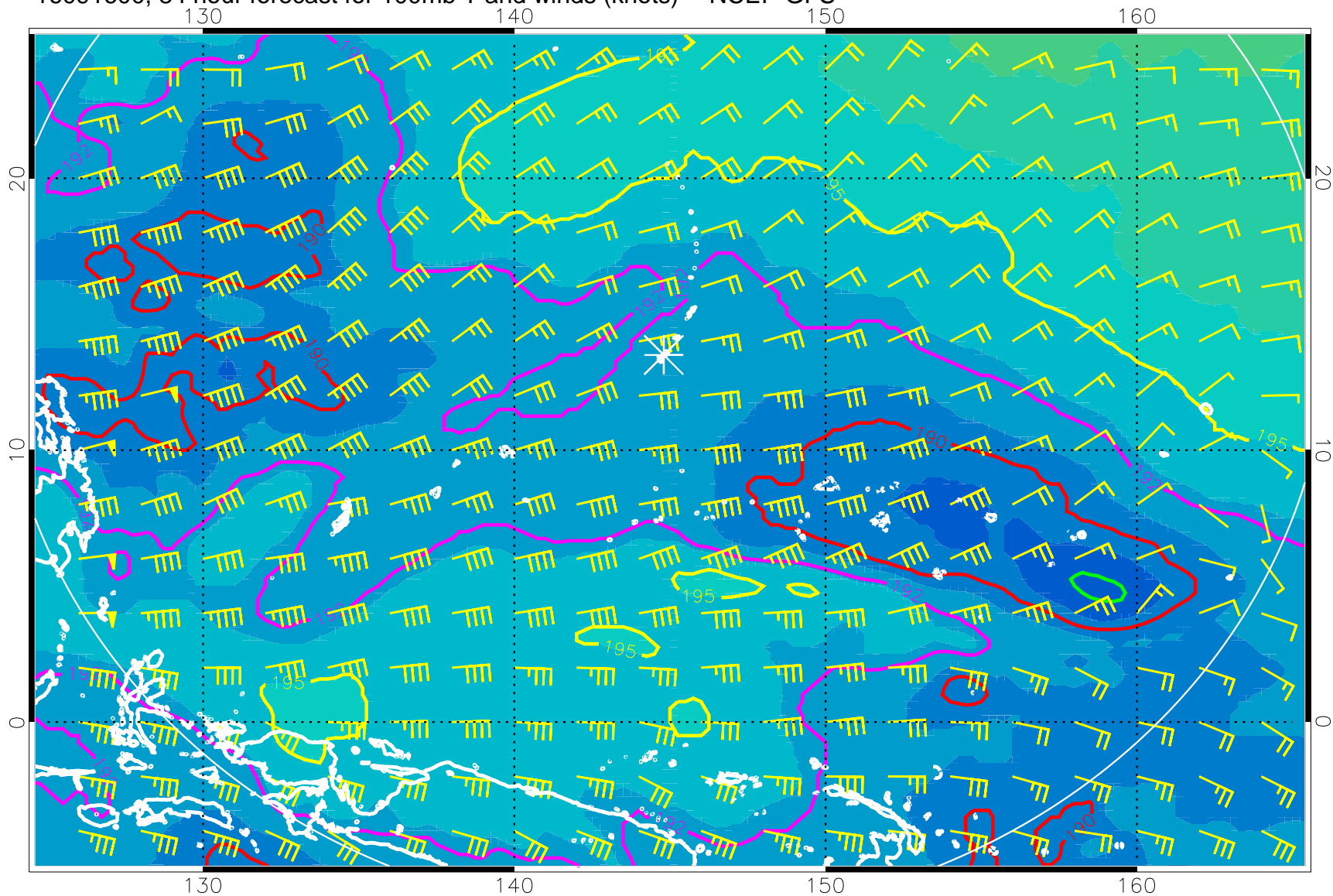
16091600, 84 hour forecast for 100mb T and winds (knots) -- NCEP GFS
