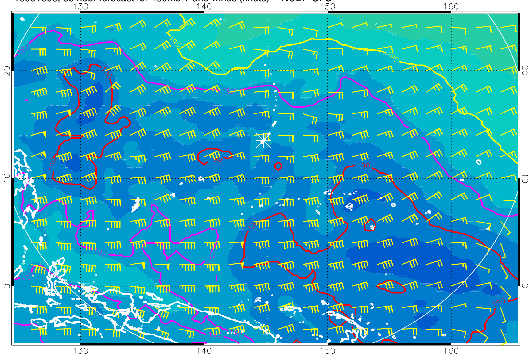
16091506, 66 hour forecast for 100mb T and winds (knots) -- NCEP GFS
