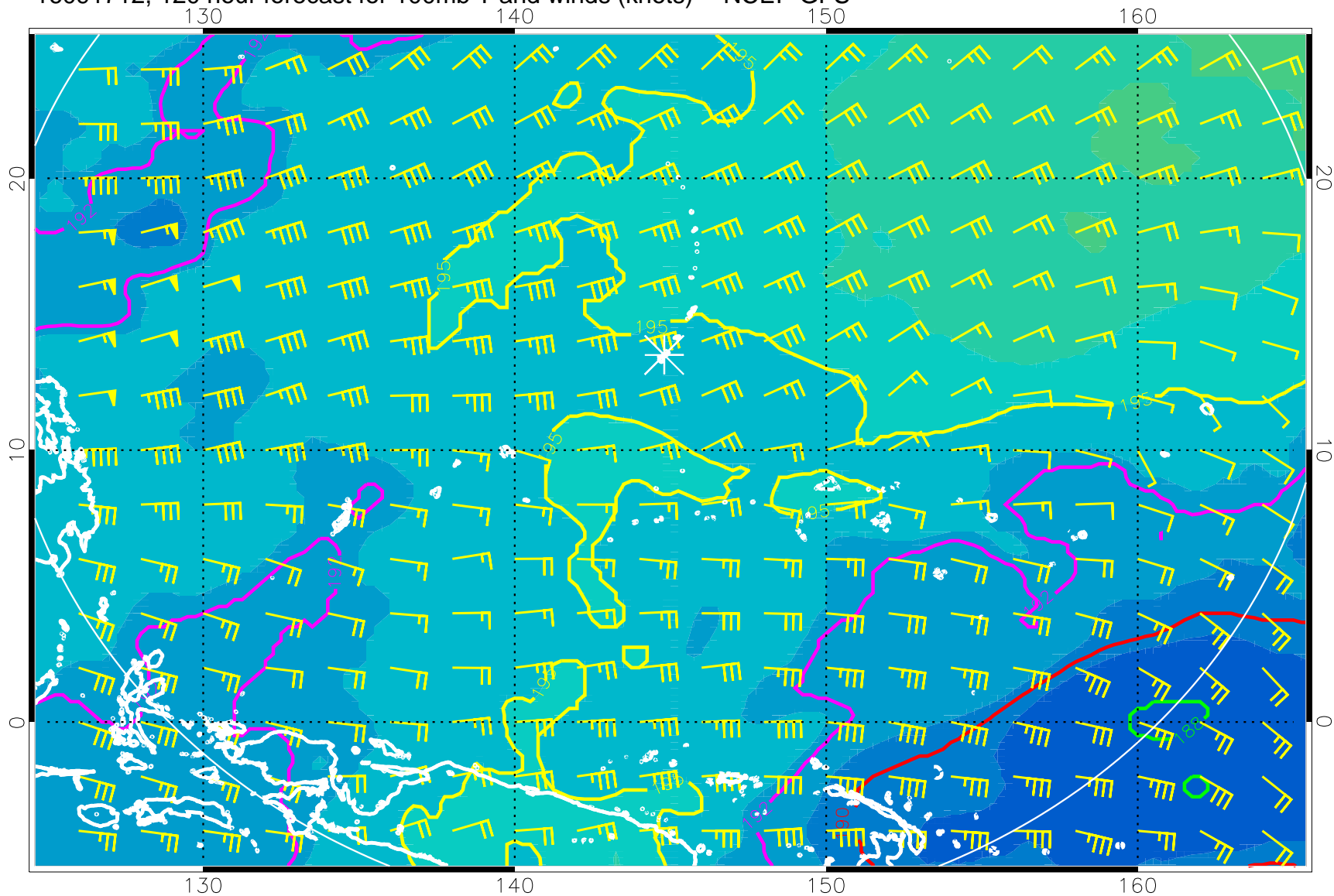
16091712, 120 hour forecast for 100mb T and winds (knots) -- NCEP GFS
