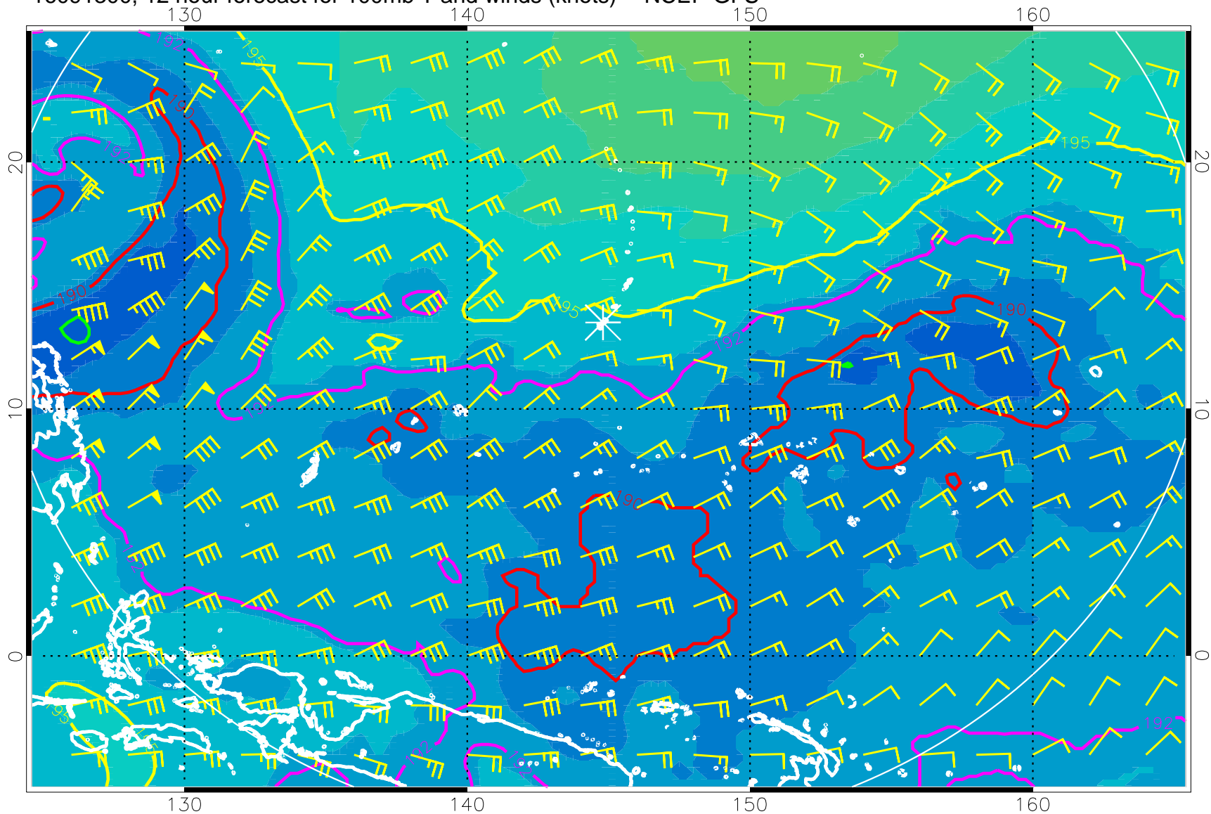
16091300, 12 hour forecast for 100mb T and winds (knots) -- NCEP GFS
