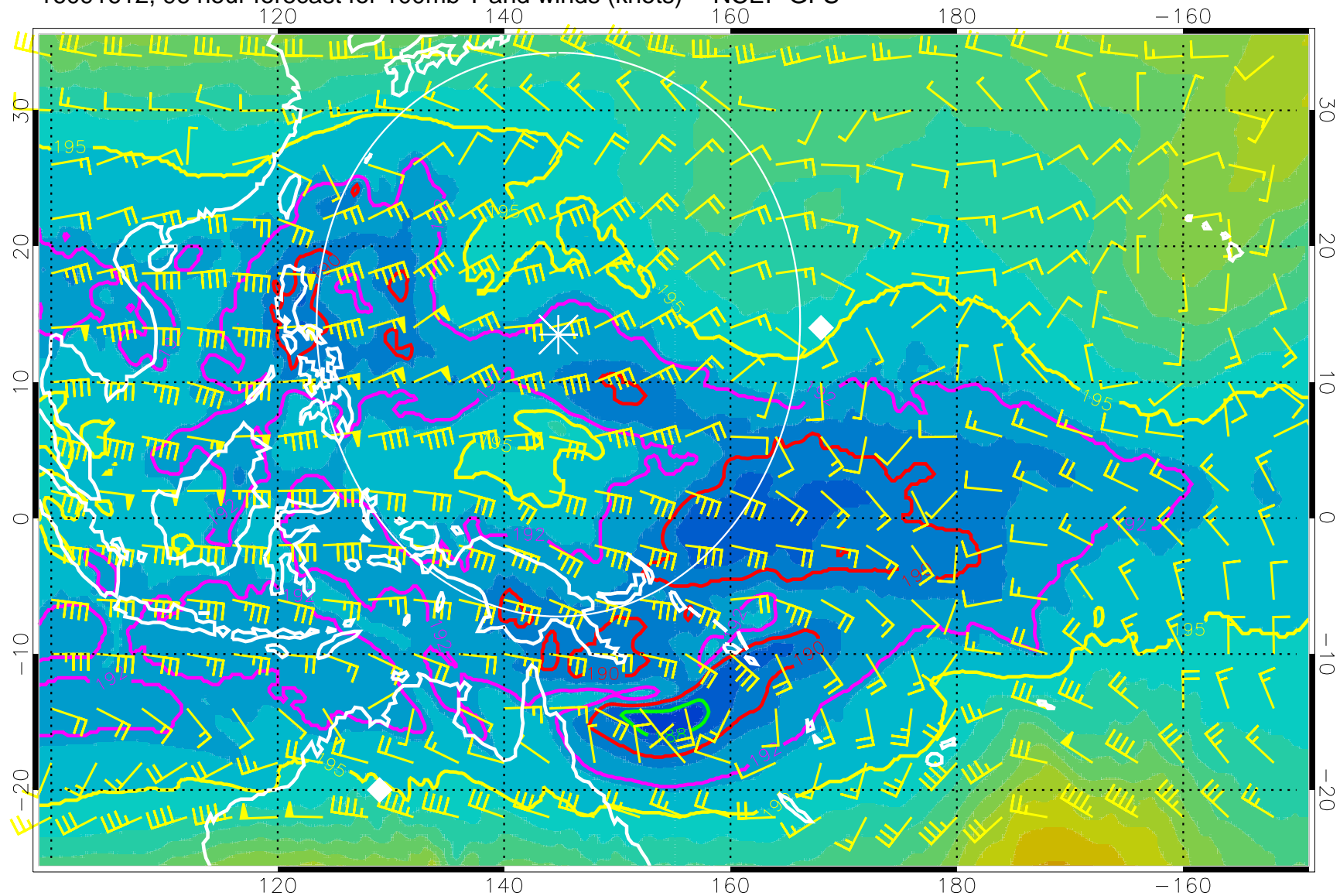
16091612, 96 hour forecast for 100mb T and winds (knots) -- NCEP GFS
