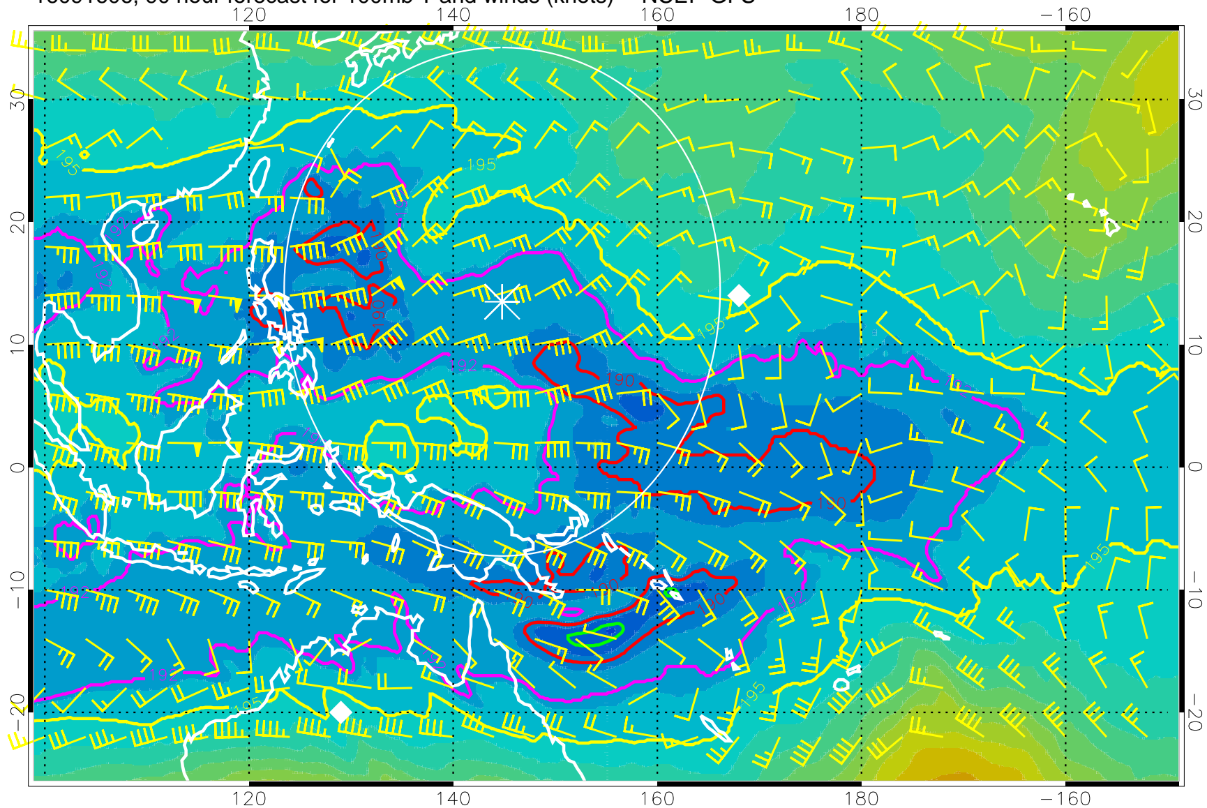
16091606, 90 hour forecast for 100mb T and winds (knots) -- NCEP GFS
