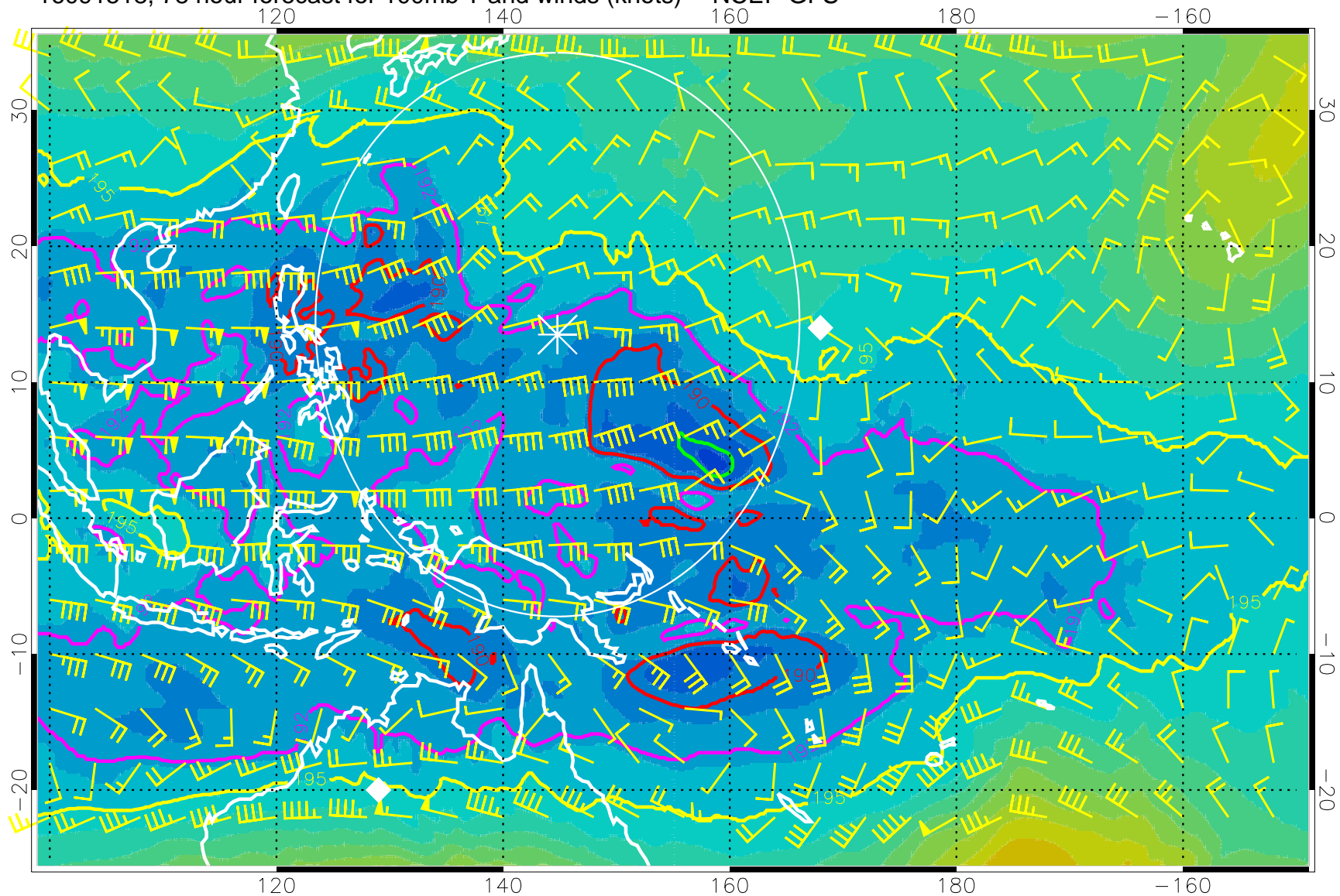
16091518, 78 hour forecast for 100mb T and winds (knots) -- NCEP GFS
