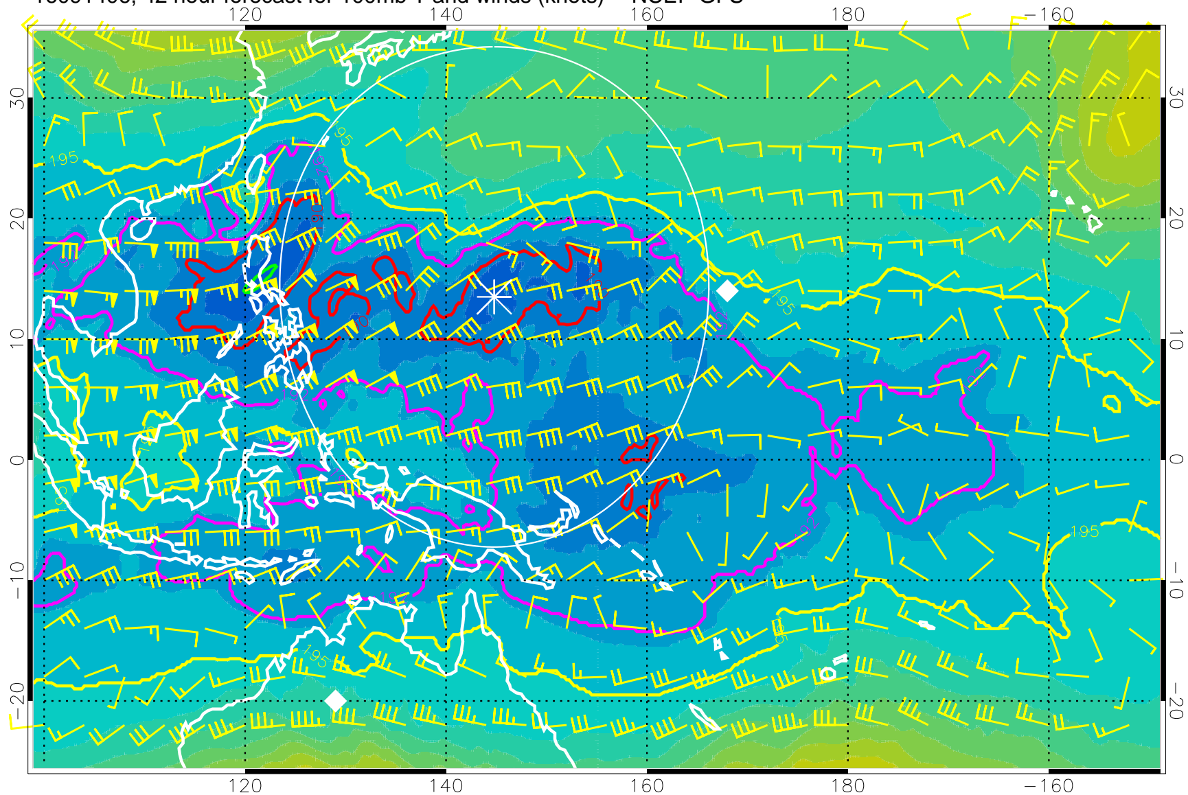
16091406, 42 hour forecast for 100mb T and winds (knots) -- NCEP GFS
