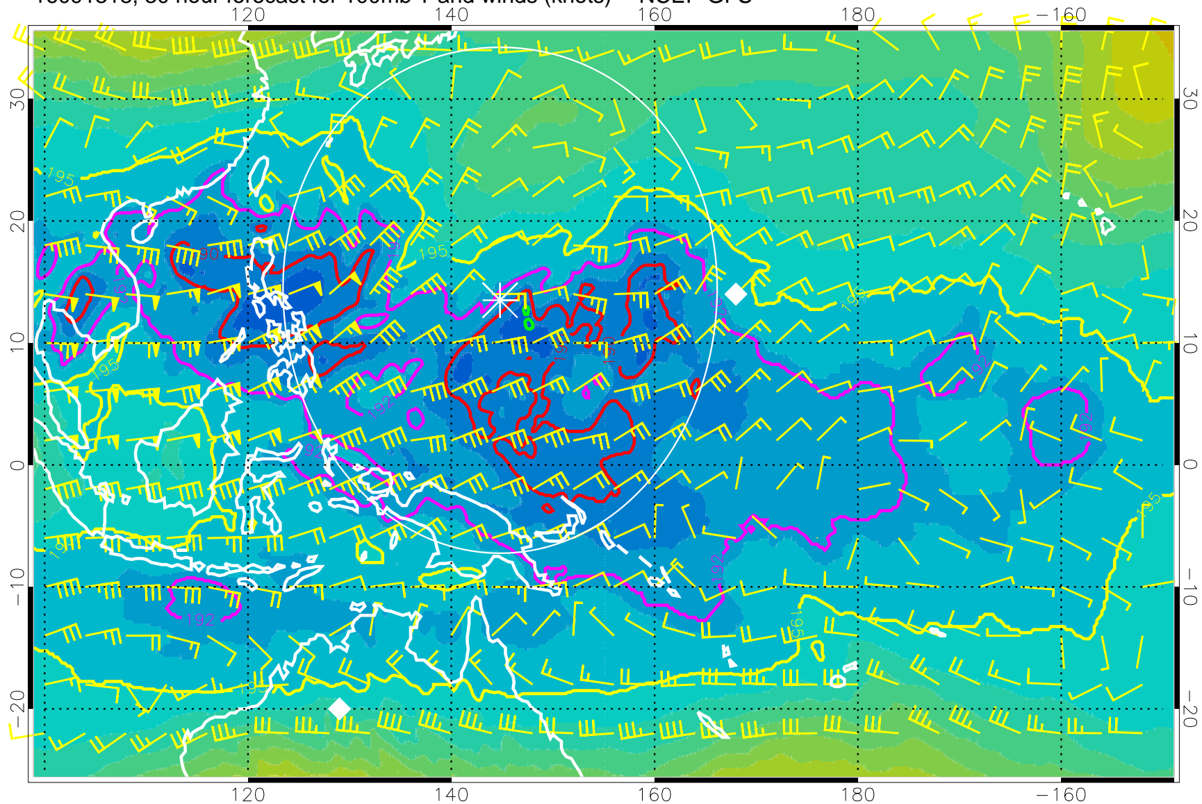
16091318, 30 hour forecast for 100mb T and winds (knots) -- NCEP GFS
