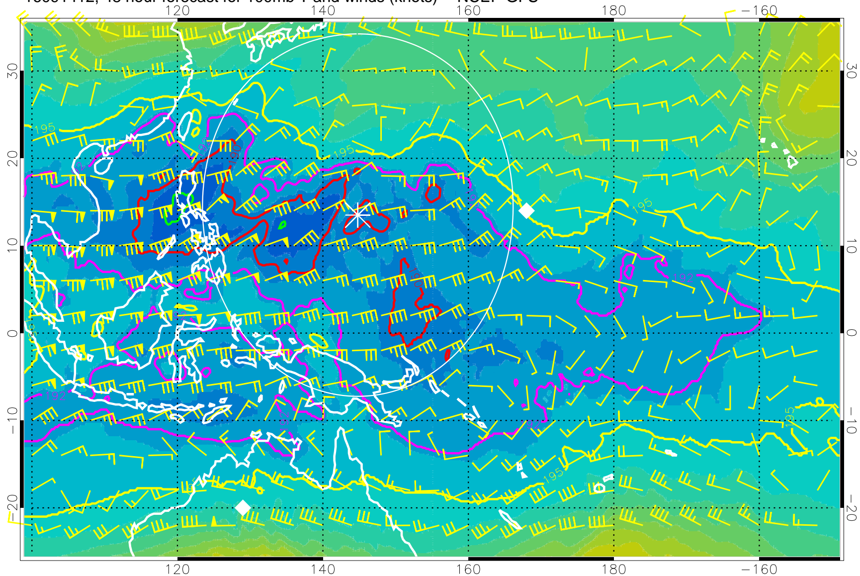
16091412, 48 hour forecast for 100mb T and winds (knots) -- NCEP GFS
