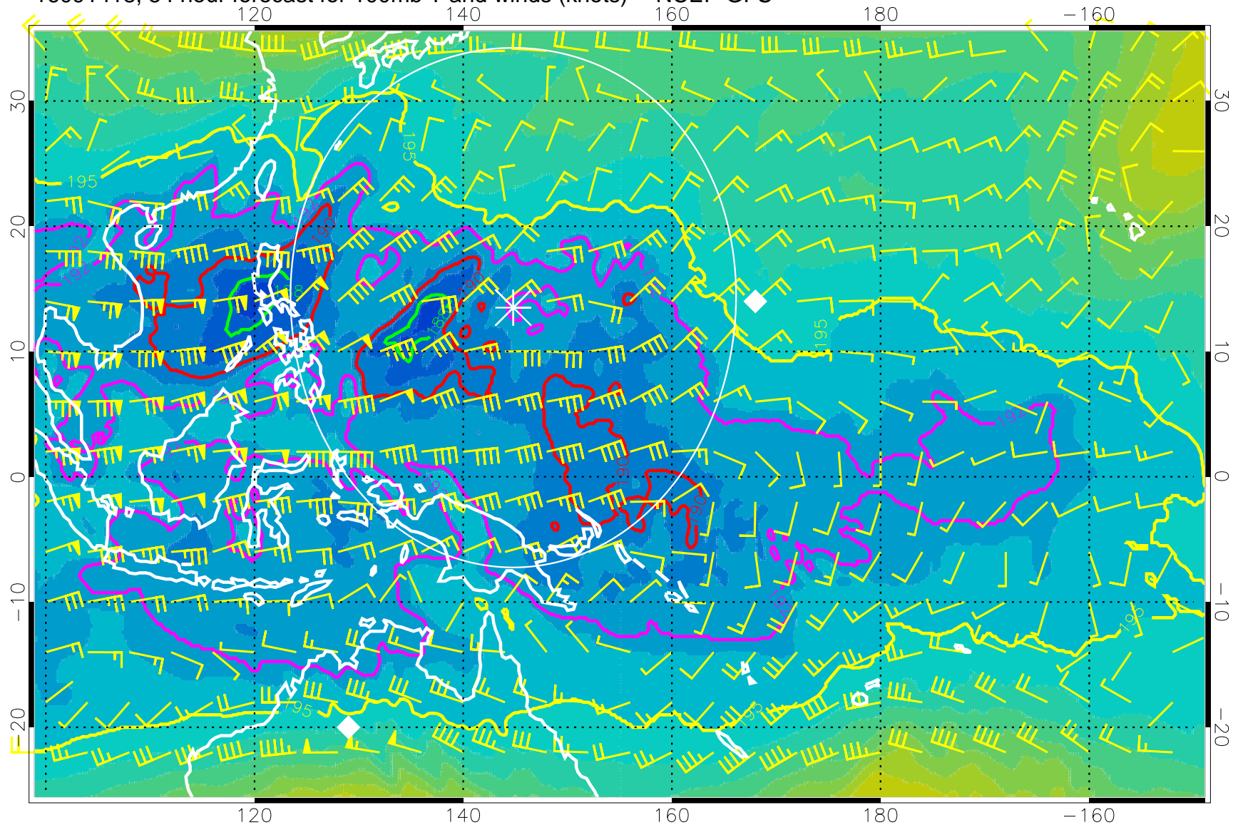
16091418, 54 hour forecast for 100mb T and winds (knots) -- NCEP GFS
