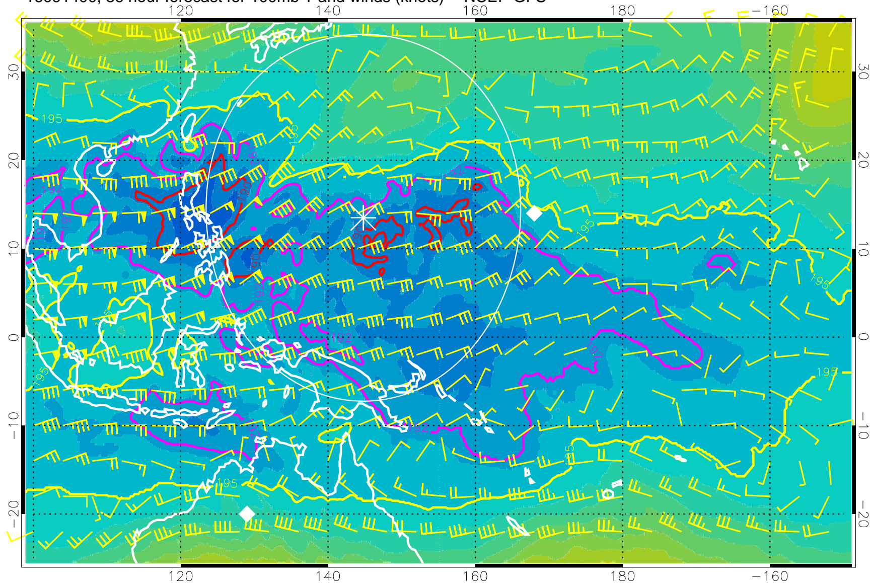
16091400, 36 hour forecast for 100mb T and winds (knots) -- NCEP GFS
