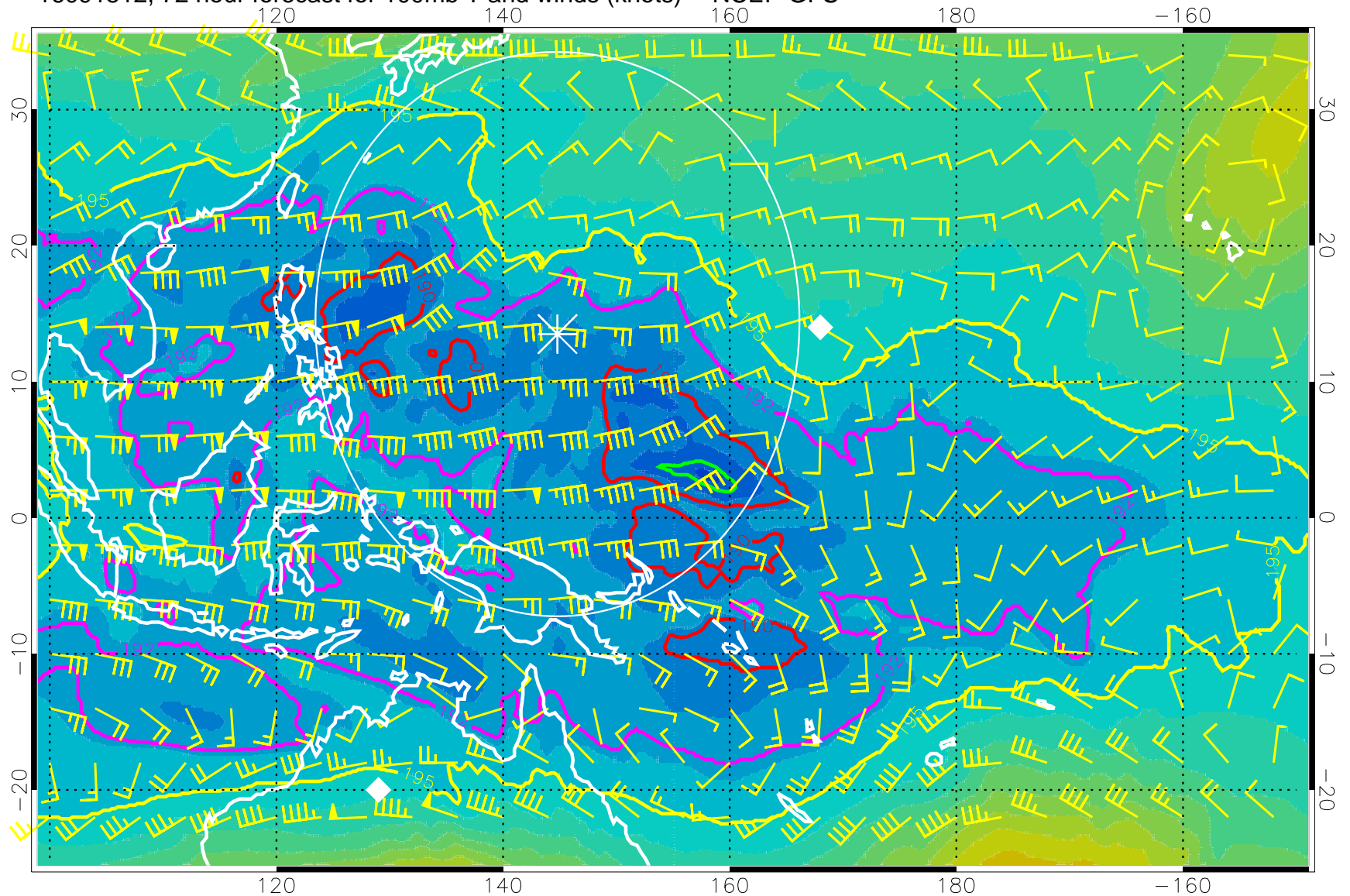
16091512, 72 hour forecast for 100mb T and winds (knots) -- NCEP GFS
