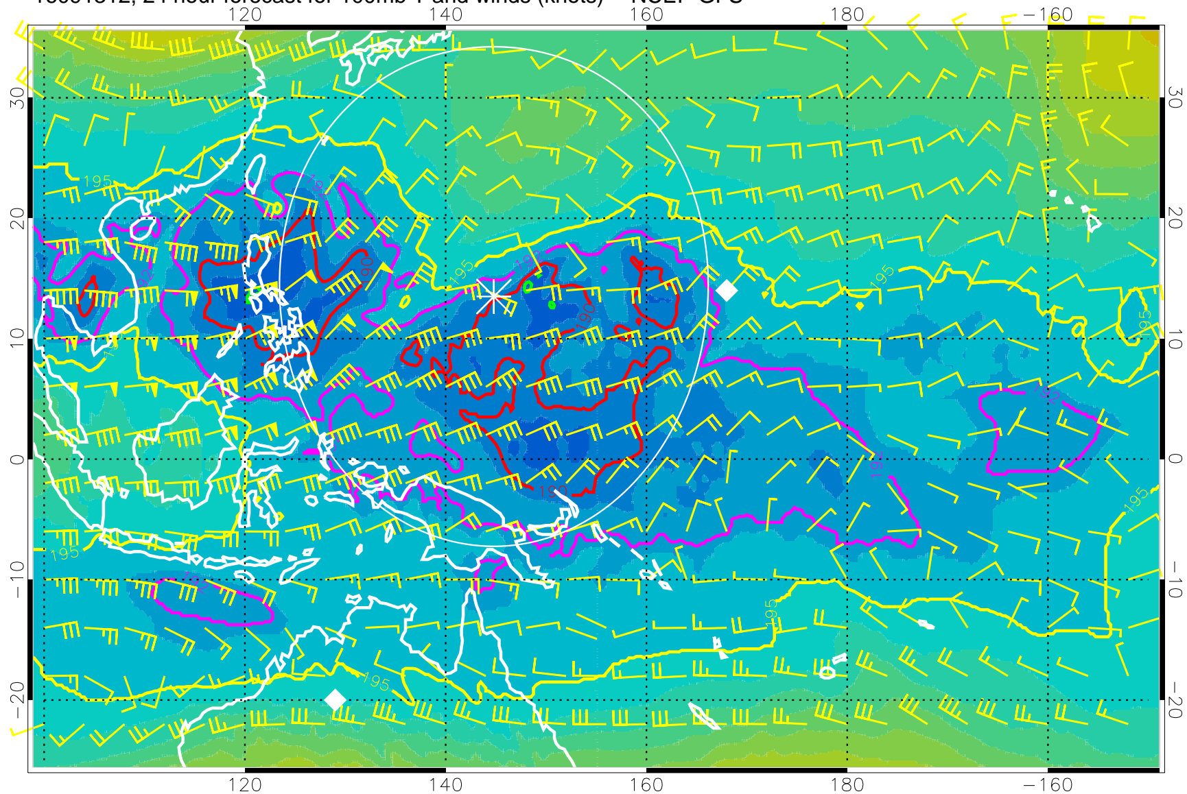
16091312, 24 hour forecast for 100mb T and winds (knots) -- NCEP GFS
