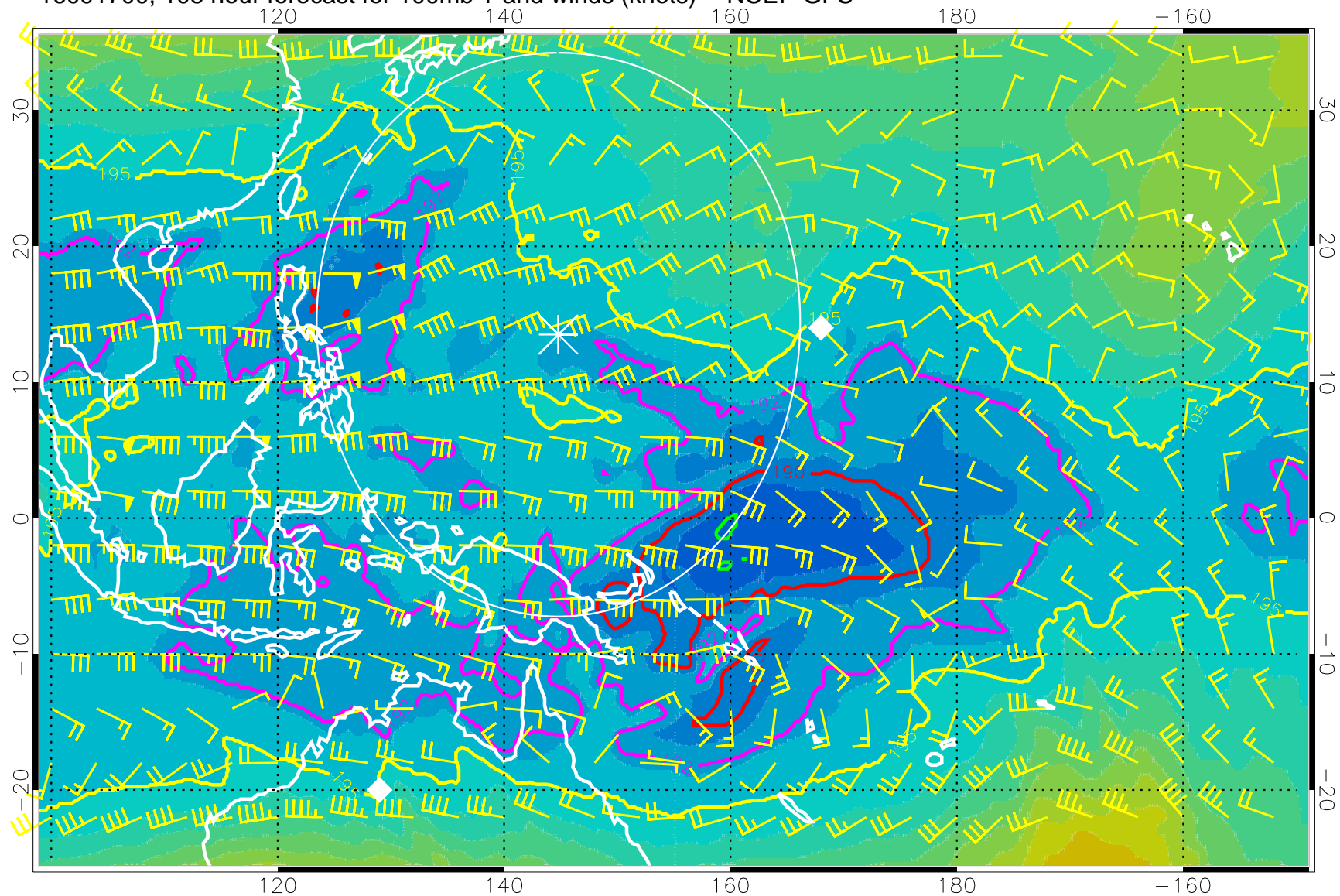
16091700, 108 hour forecast for 100mb T and winds (knots) -- NCEP GFS
