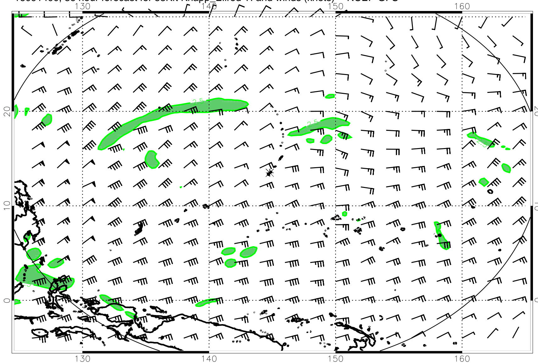
16091400, 36 hour forecast for 53Kft Knapp_Ellrod TI and winds (knots) -- NCEP GFS
