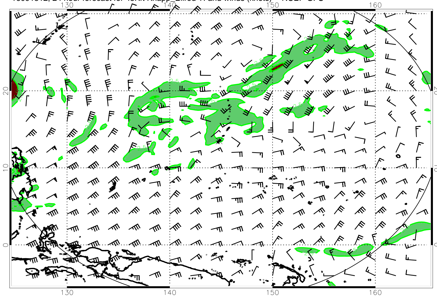
16091312, 24 hour forecast for 45Kft Knapp_Ellrod TI and winds (knots) -- NCEP GFS
