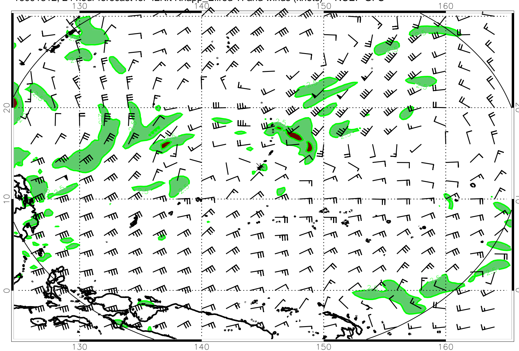
16091312, 24 hour forecast for 42Kft Knapp_Ellrod TI and winds (knots) -- NCEP GFS
