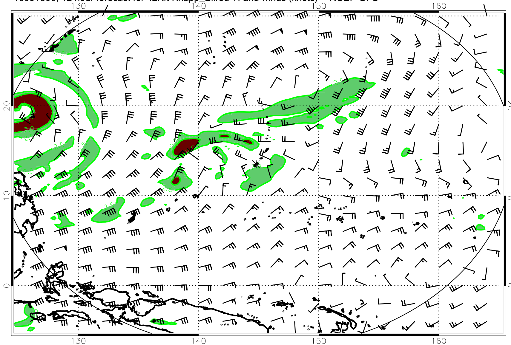
16091300, 12 hour forecast for 42Kft Knapp_Ellrod TI and winds (knots) -- NCEP GFS
