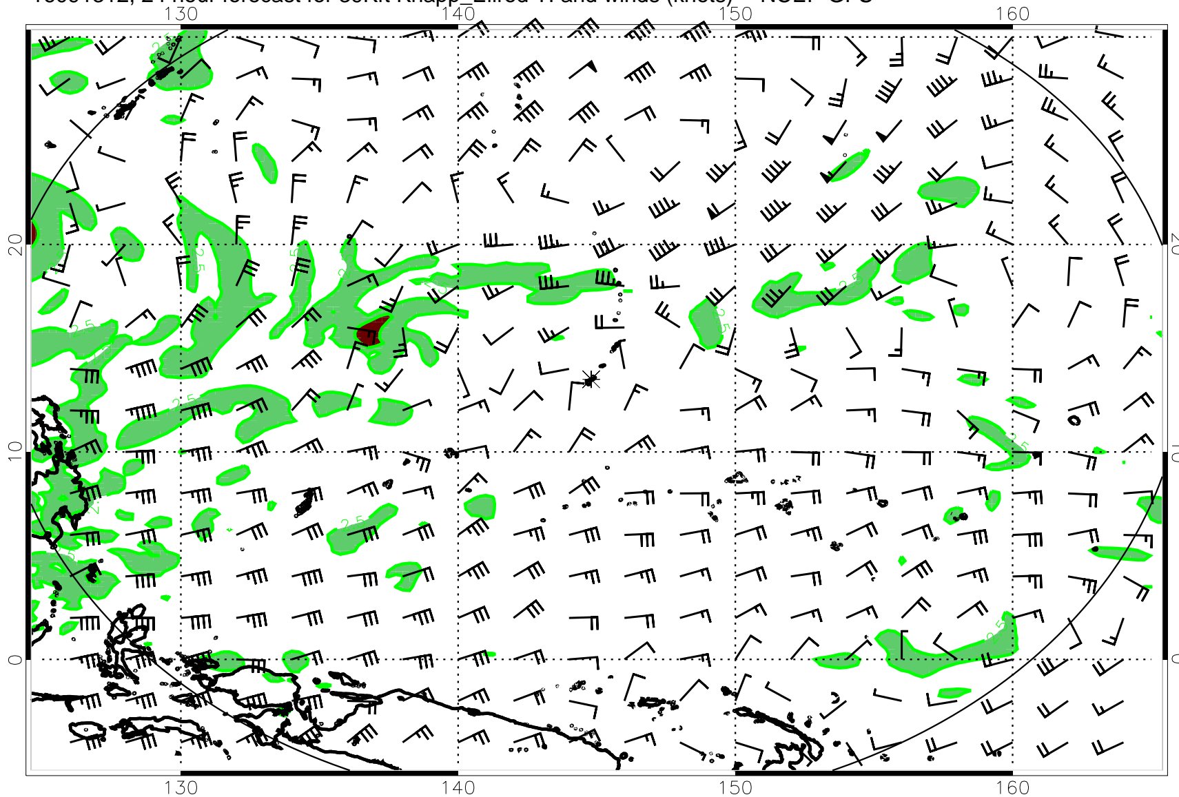
16091312, 24 hour forecast for 39Kft Knapp_Ellrod TI and winds (knots) -- NCEP GFS
