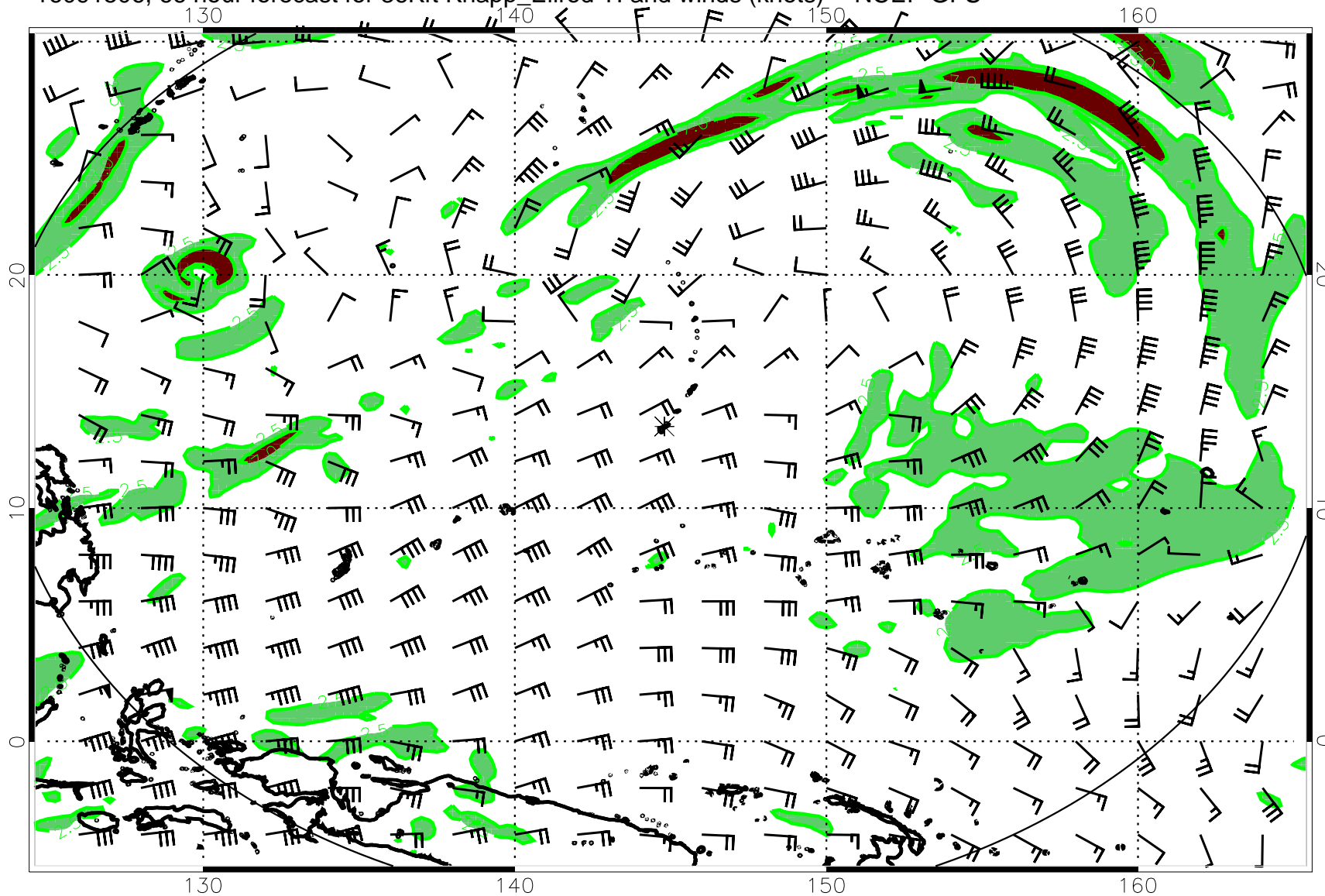
16091506, 66 hour forecast for 36Kft Knapp_Ellrod TI and winds (knots) -- NCEP GFS
