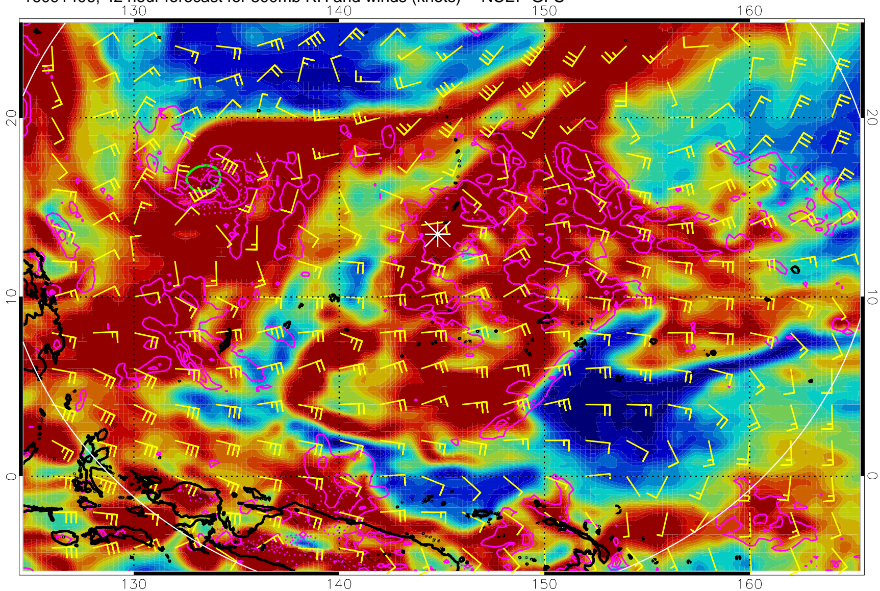
16091406, 42 hour forecast for 300mb RH and winds (knots) -- NCEP GFS
