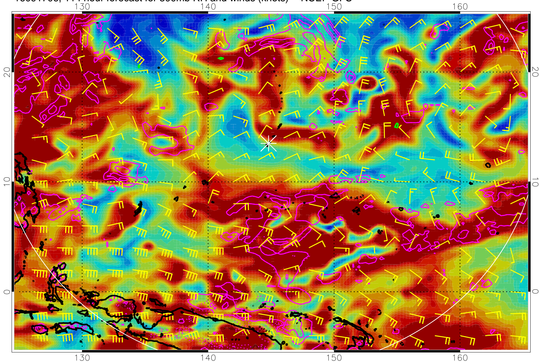
16091706, 114 hour forecast for 300mb RH and winds (knots) -- NCEP GFS
