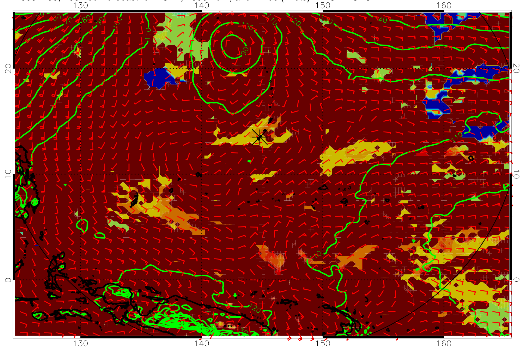
16091700, 108 hour forecast for HCAL, 1000mb Z, and winds (knots) -- NCEP GFS
