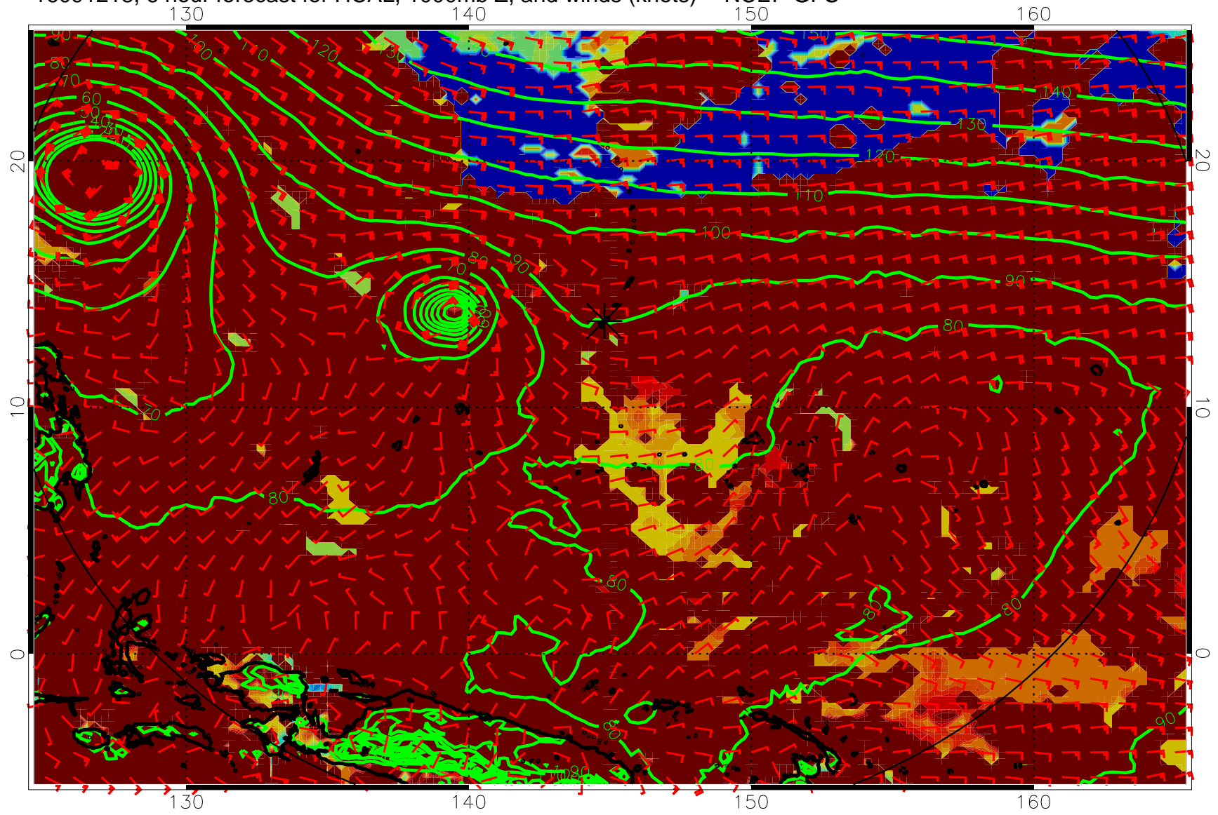
16091218, 6 hour forecast for HCAL, 1000mb Z, and winds (knots) -- NCEP GFS
