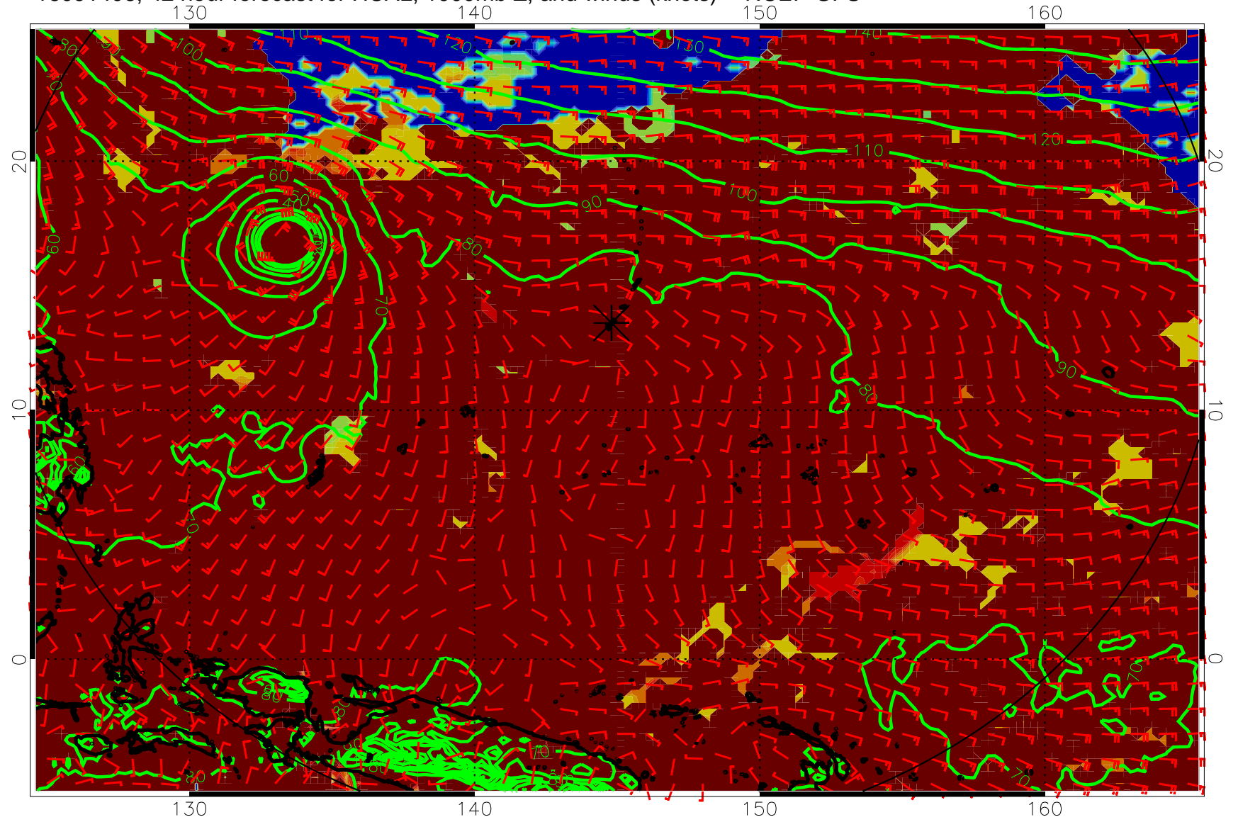
16091406, 42 hour forecast for HCAL, 1000mb Z, and winds (knots) -- NCEP GFS
