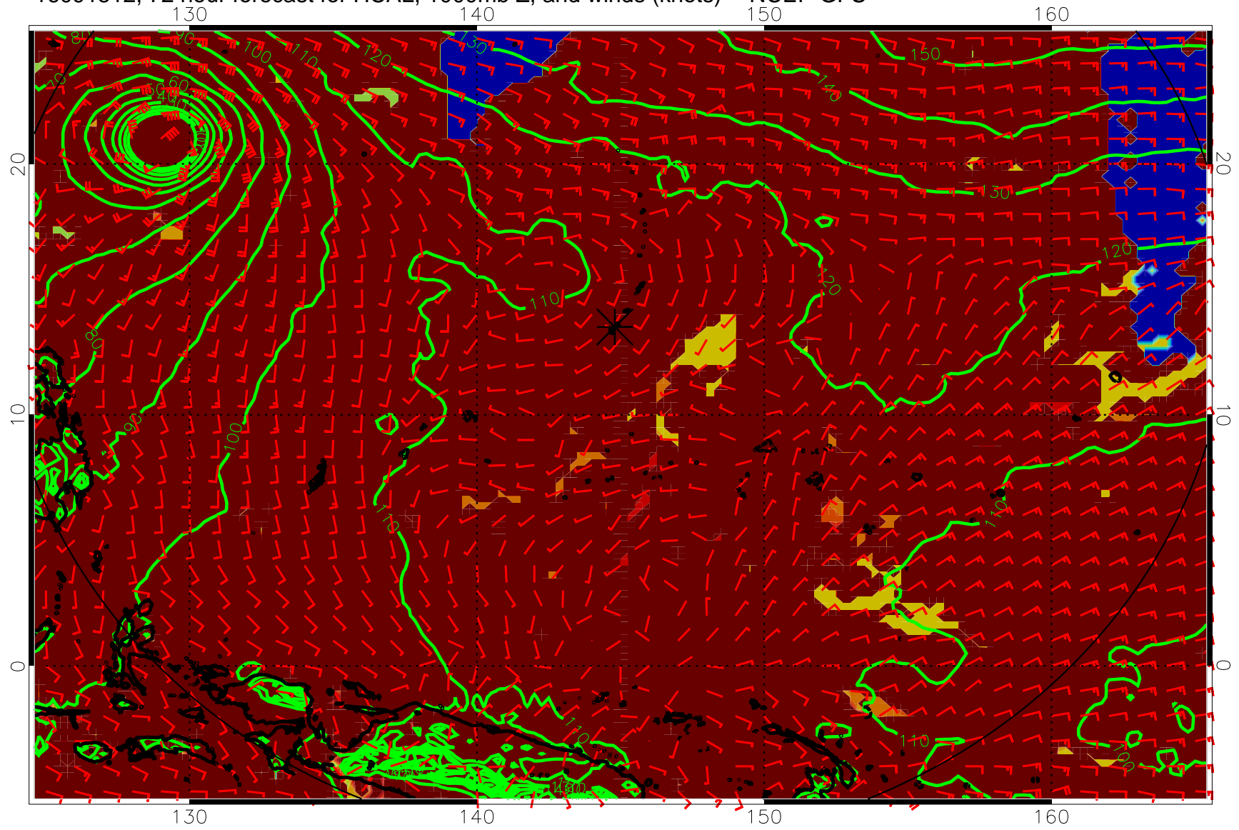
16091512, 72 hour forecast for HCAL, 1000mb Z, and winds (knots) -- NCEP GFS
