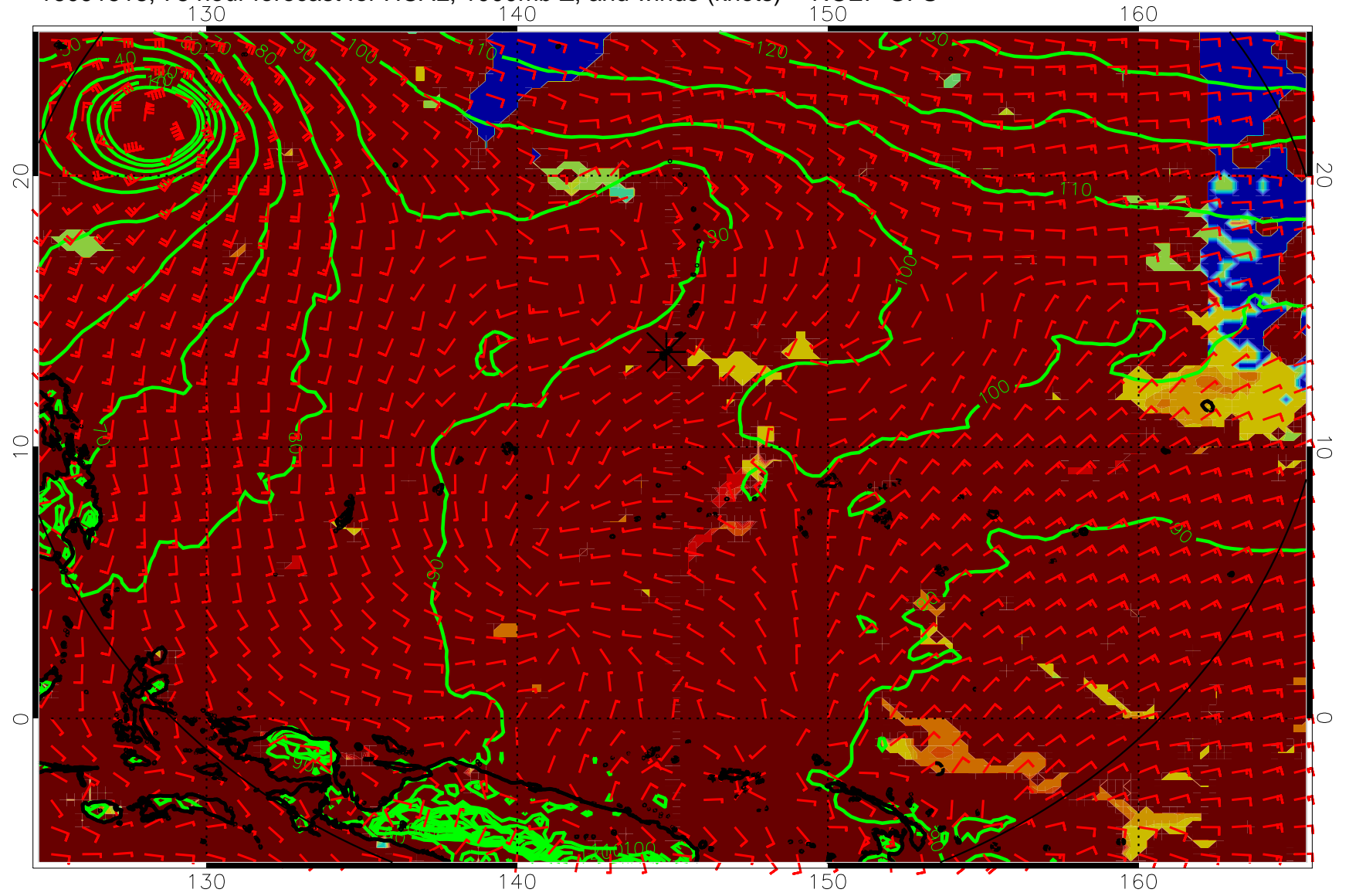
16091518, 78 hour forecast for HCAL, 1000mb Z, and winds (knots) -- NCEP GFS
