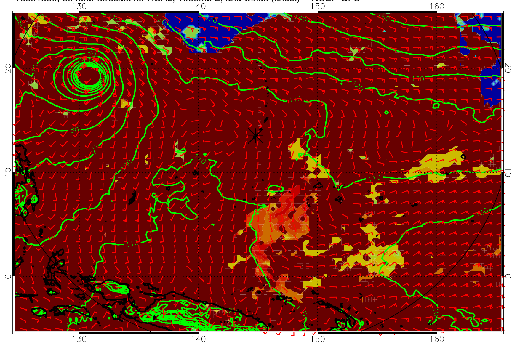
16091500, 60 hour forecast for HCAL, 1000mb Z, and winds (knots) -- NCEP GFS
