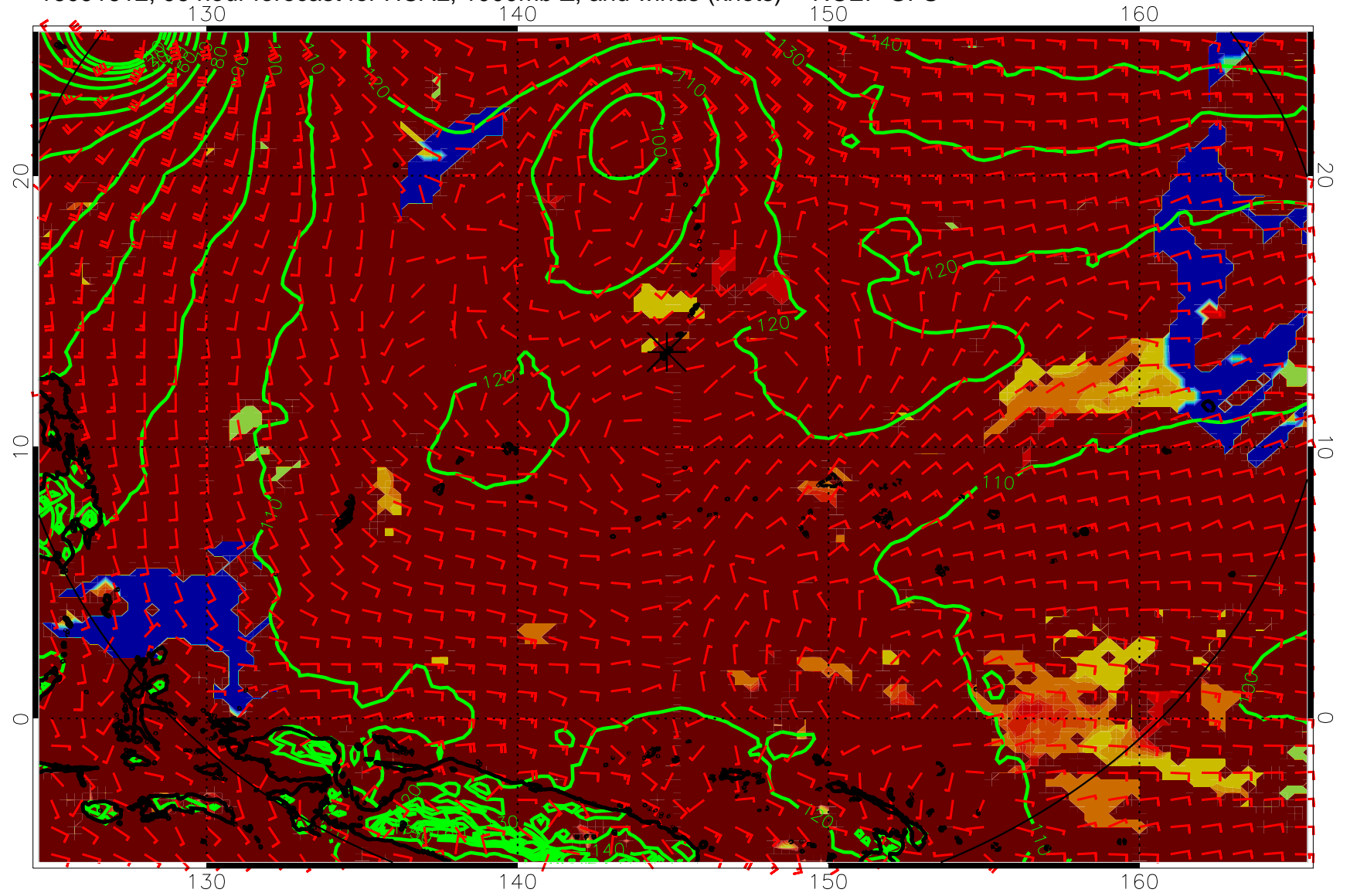
16091612, 96 hour forecast for HCAL, 1000mb Z, and winds (knots) -- NCEP GFS
