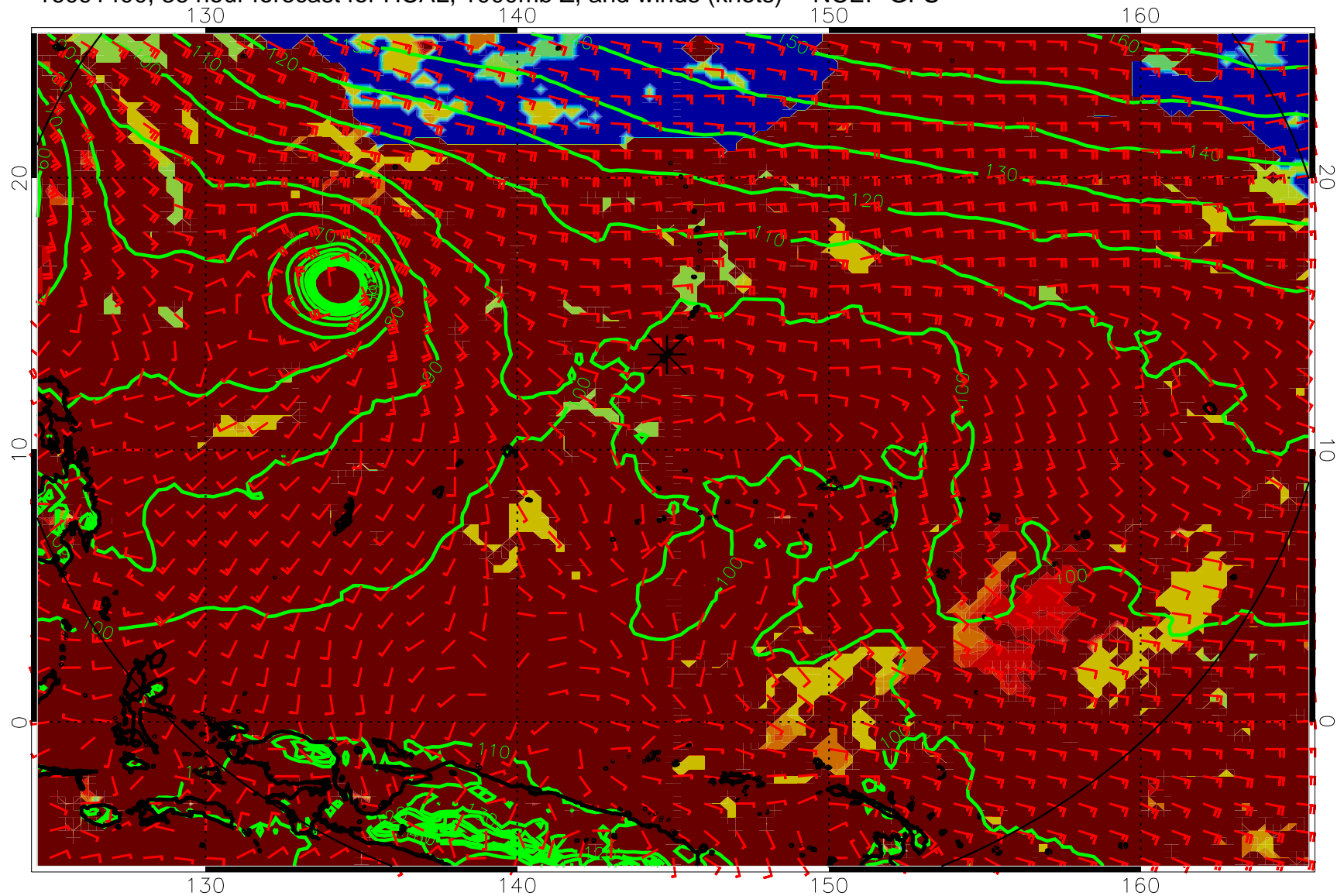
16091400, 36 hour forecast for HCAL, 1000mb Z, and winds (knots) -- NCEP GFS
