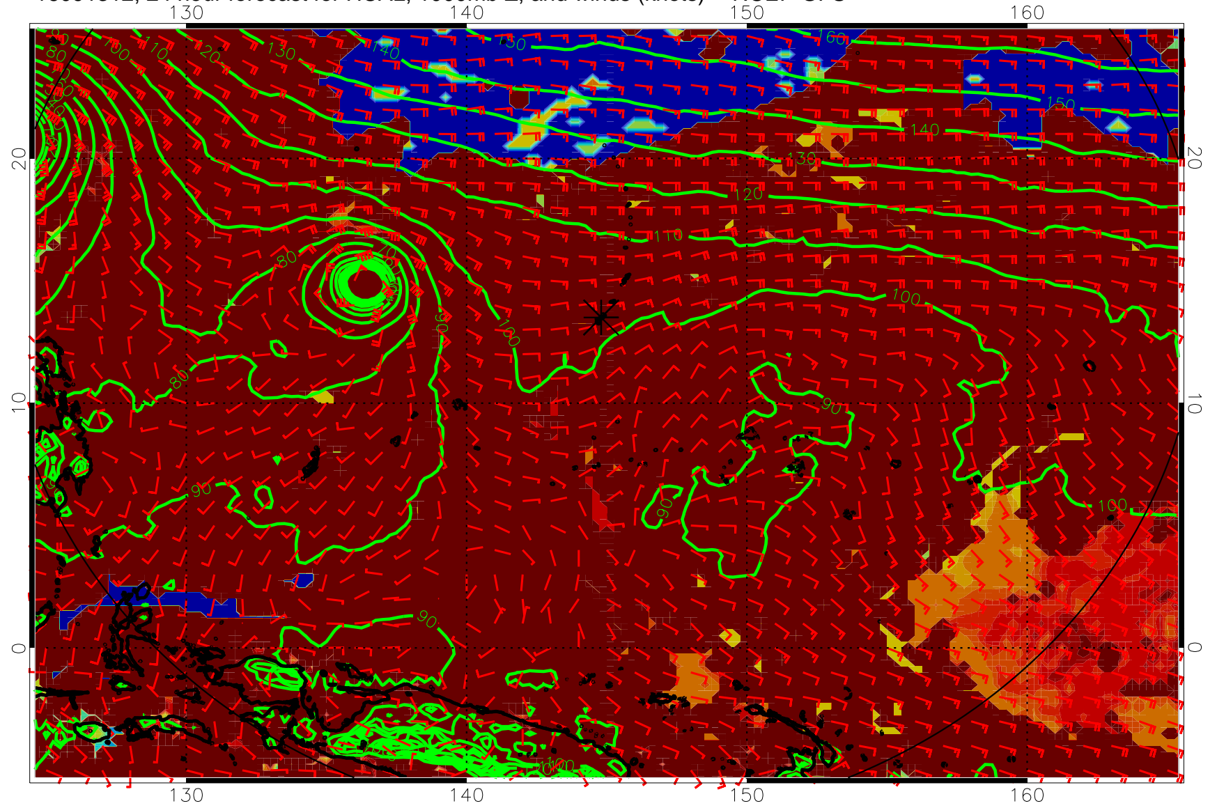
16091312, 24 hour forecast for HCAL, 1000mb Z, and winds (knots) -- NCEP GFS
