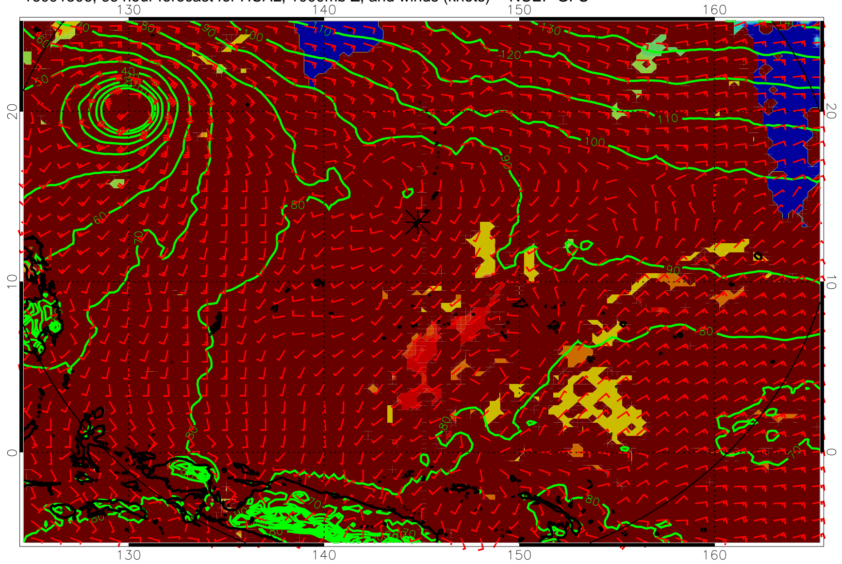
16091506, 66 hour forecast for HCAL, 1000mb Z, and winds (knots) -- NCEP GFS
