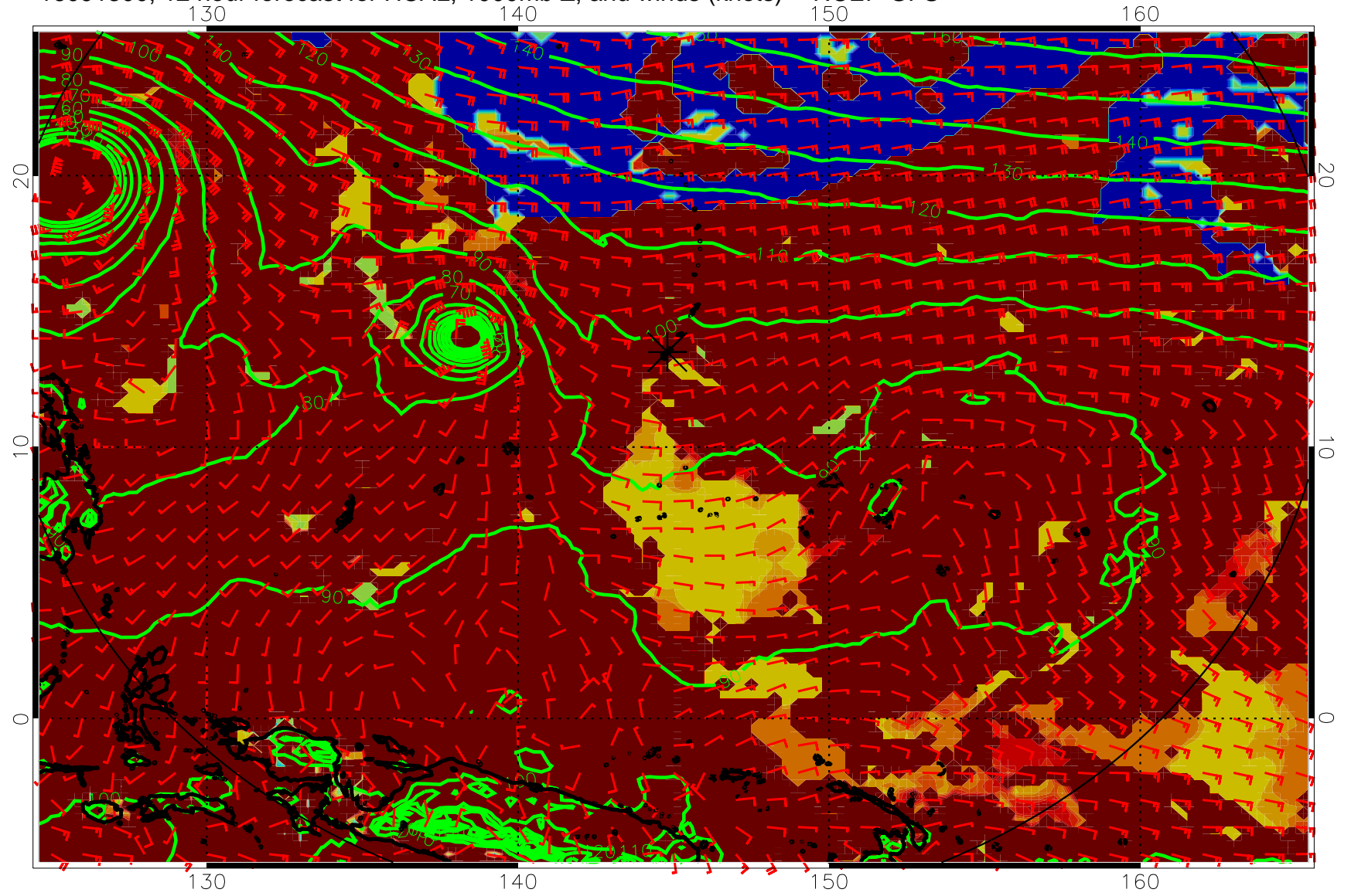
16091300, 12 hour forecast for HCAL, 1000mb Z, and winds (knots) -- NCEP GFS
