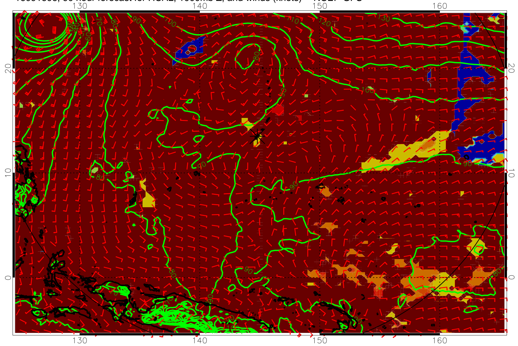
16091606, 90 hour forecast for HCAL, 1000mb Z, and winds (knots) -- NCEP GFS
