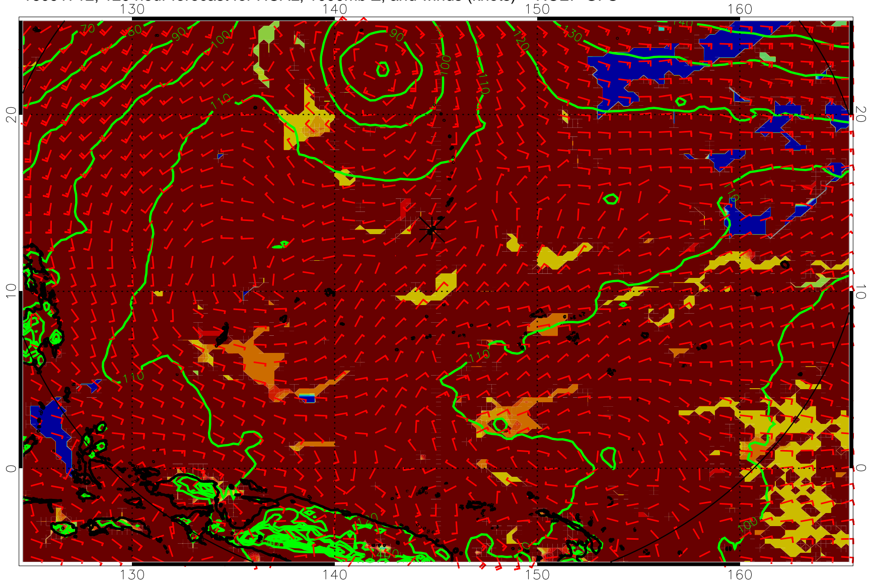
16091712, 120 hour forecast for HCAL, 1000mb Z, and winds (knots) -- NCEP GFS
