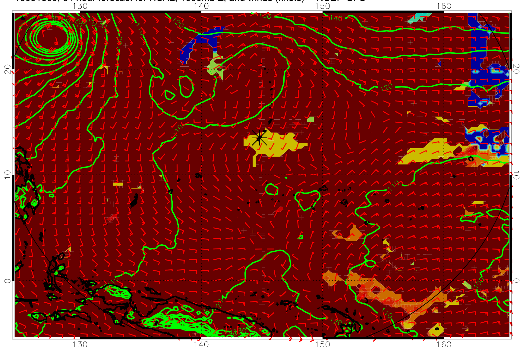
16091600, 84 hour forecast for HCAL, 1000mb Z, and winds (knots) -- NCEP GFS
