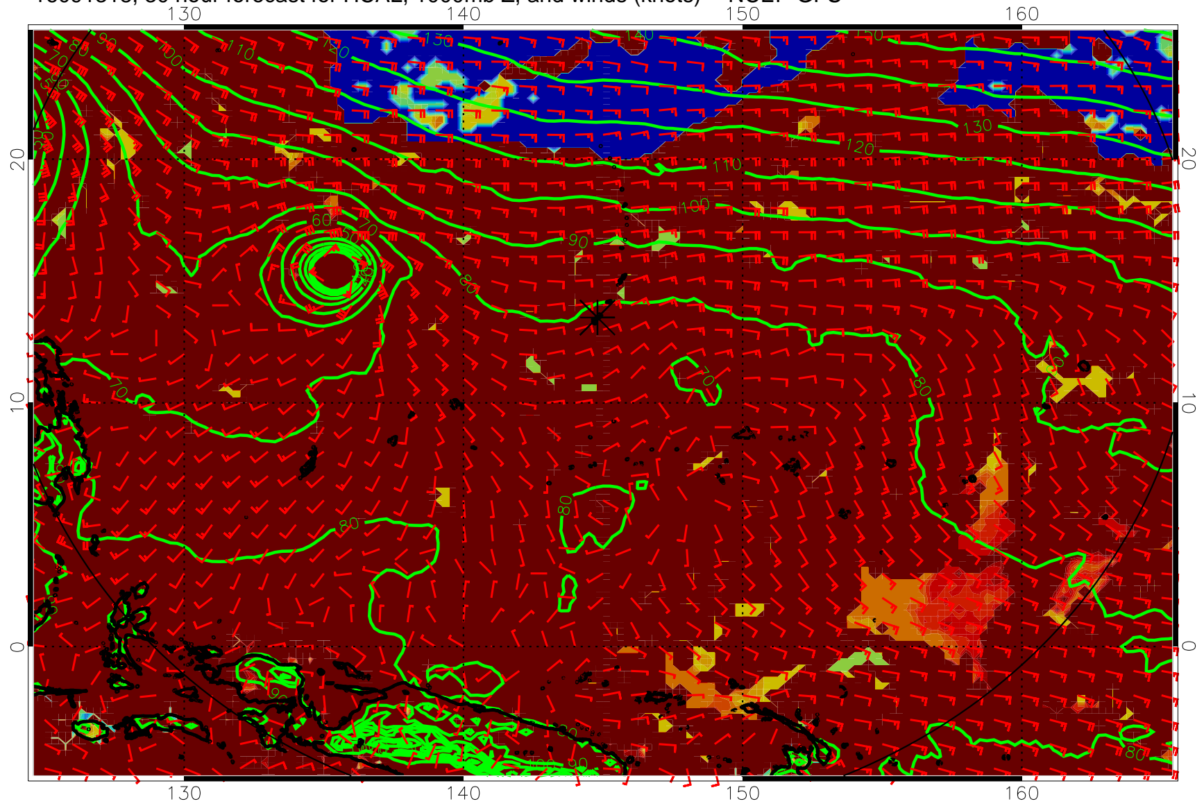
16091318, 30 hour forecast for HCAL, 1000mb Z, and winds (knots) -- NCEP GFS
