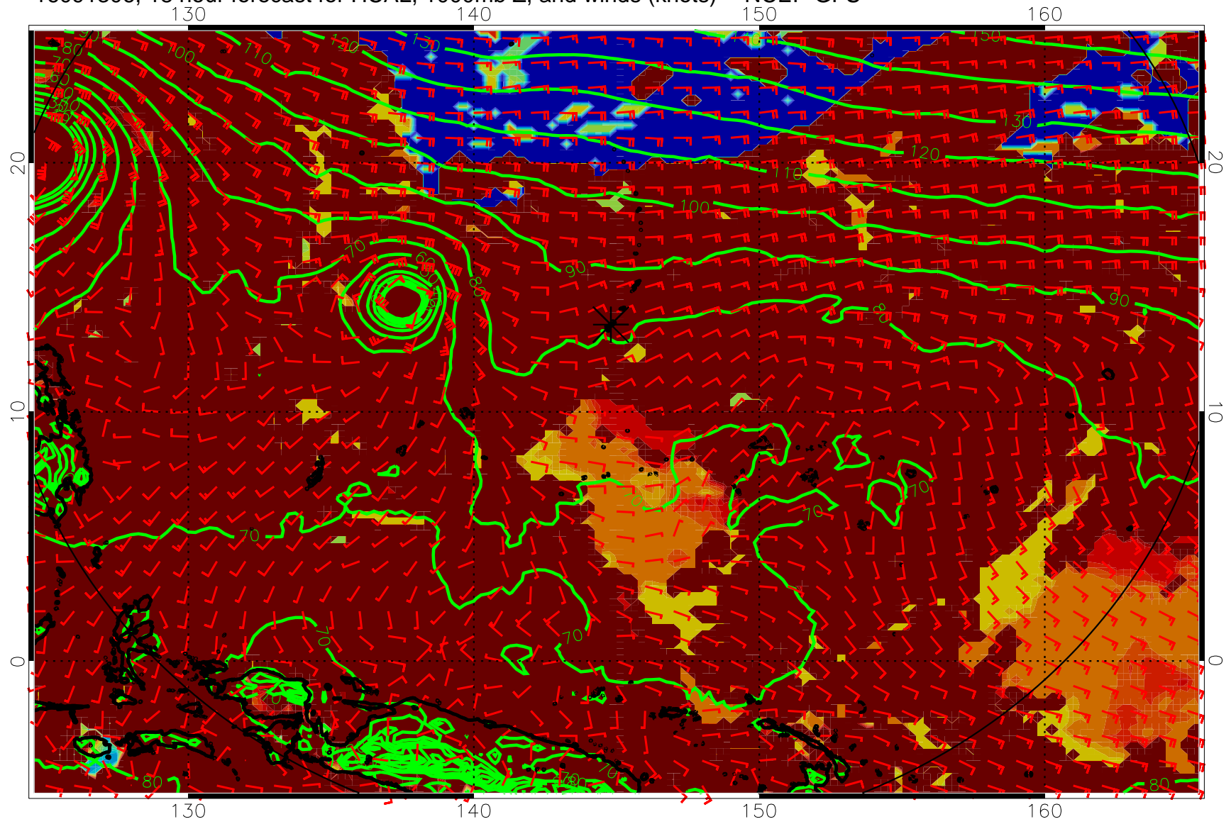
16091306, 18 hour forecast for HCAL, 1000mb Z, and winds (knots) -- NCEP GFS
