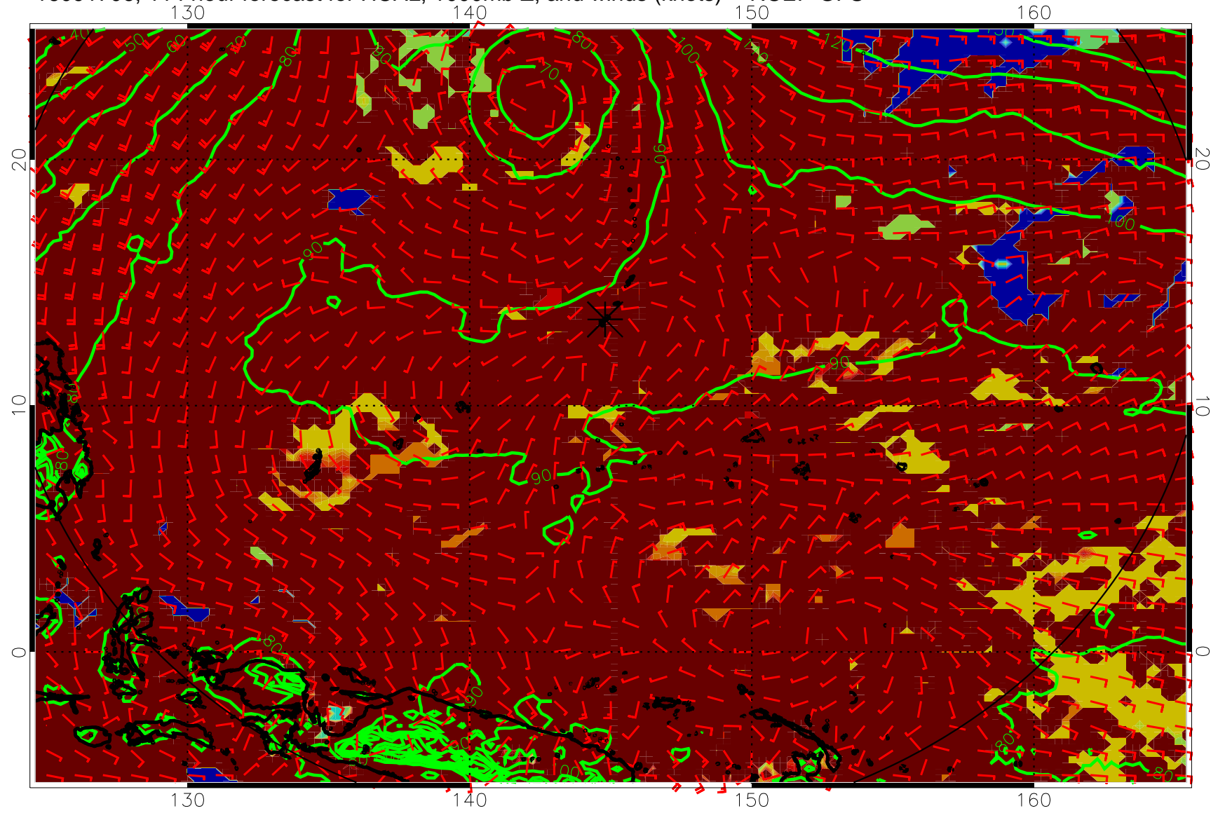
16091706, 114 hour forecast for HCAL, 1000mb Z, and winds (knots) -- NCEP GFS
