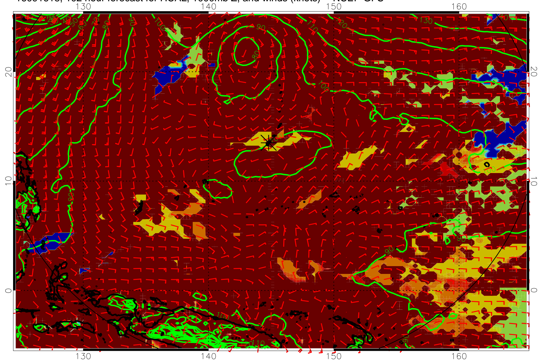
16091618, 102 hour forecast for HCAL, 1000mb Z, and winds (knots) -- NCEP GFS
