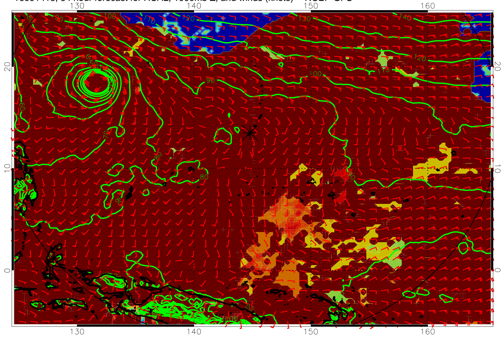
16091418, 54 hour forecast for HCAL, 1000mb Z, and winds (knots) -- NCEP GFS
