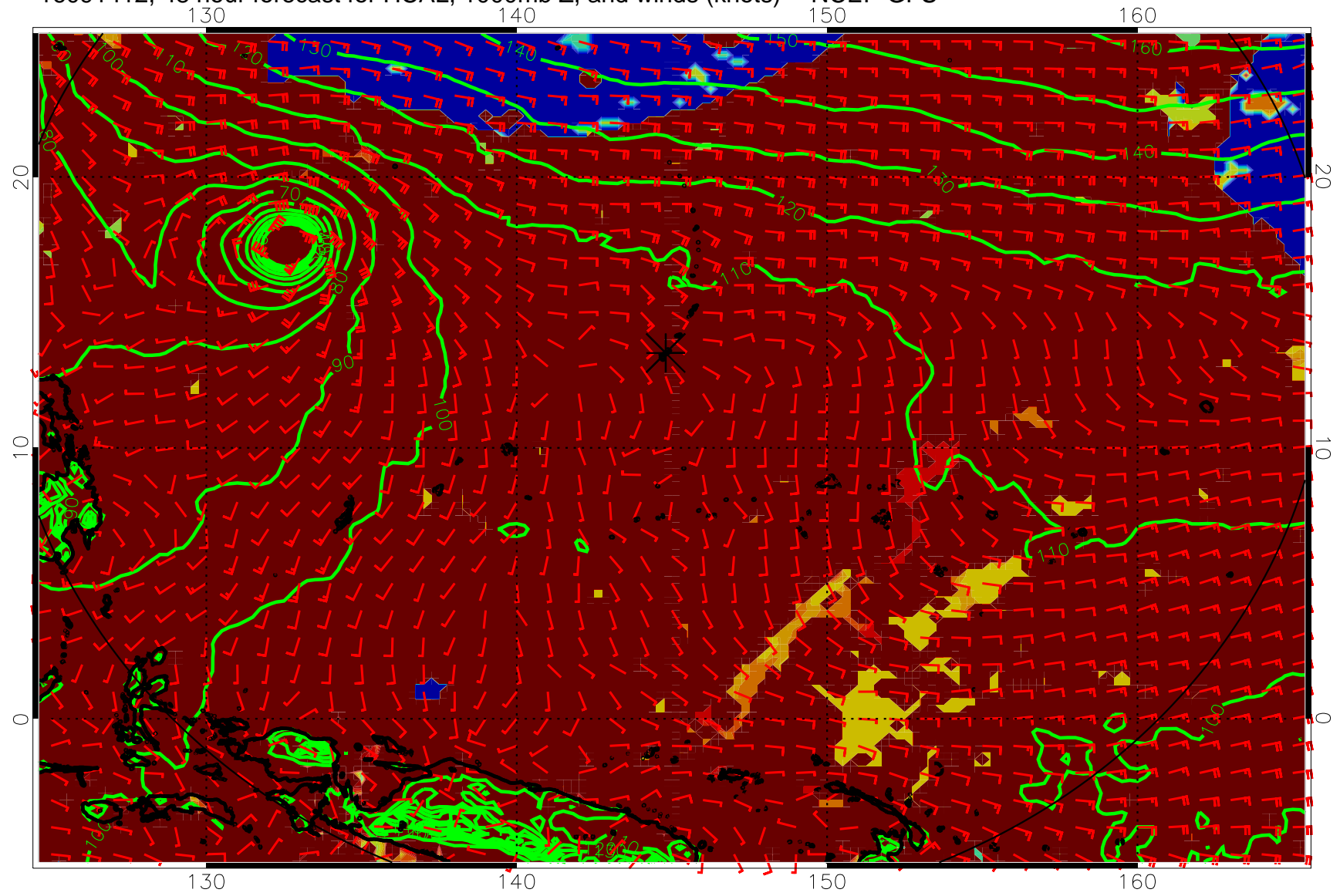
16091412, 48 hour forecast for HCAL, 1000mb Z, and winds (knots) -- NCEP GFS
