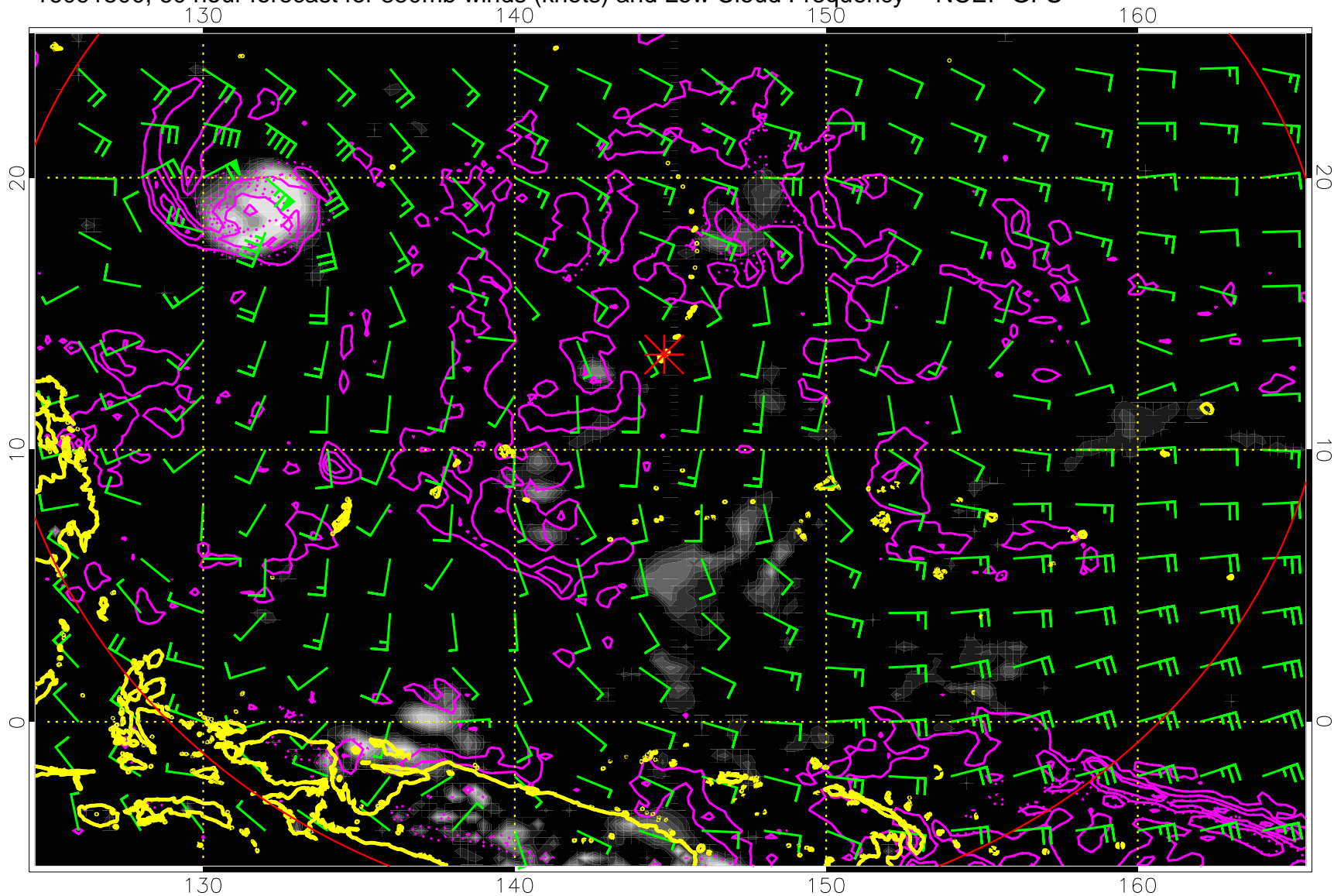
16091500, 60 hour forecast for 850mb winds (knots) and Low Cloud Frequency -- NCEP GFS
