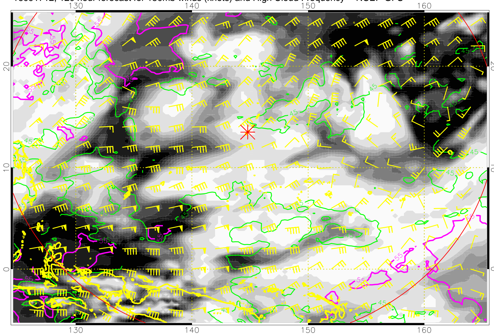
16091712, 120 hour forecast for 150mb winds (knots) and High Cloud Frequency -- NCEP GFS
