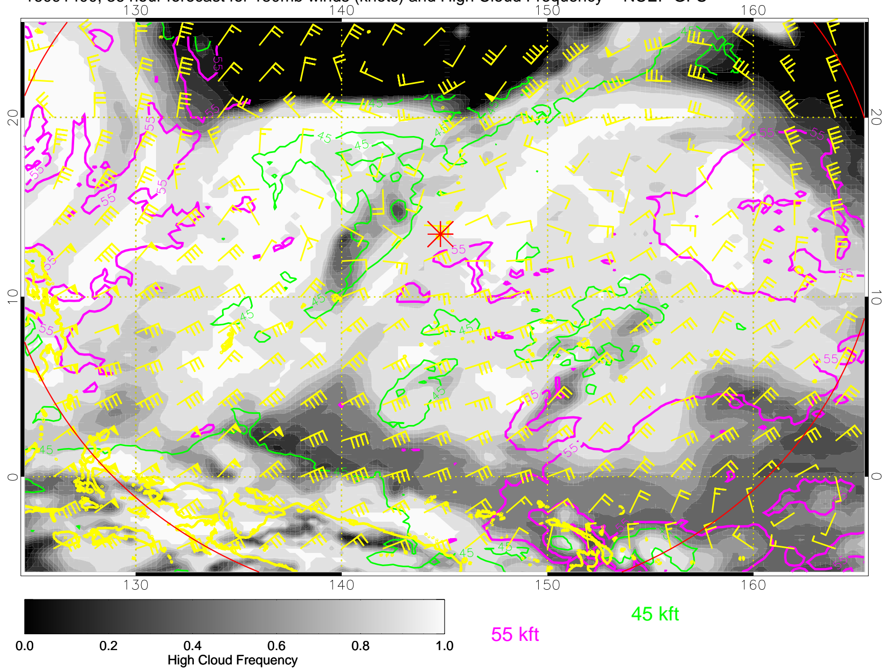
16091400, 36 hour forecast for 150mb winds (knots) and High Cloud Frequency -- NCEP GFS
