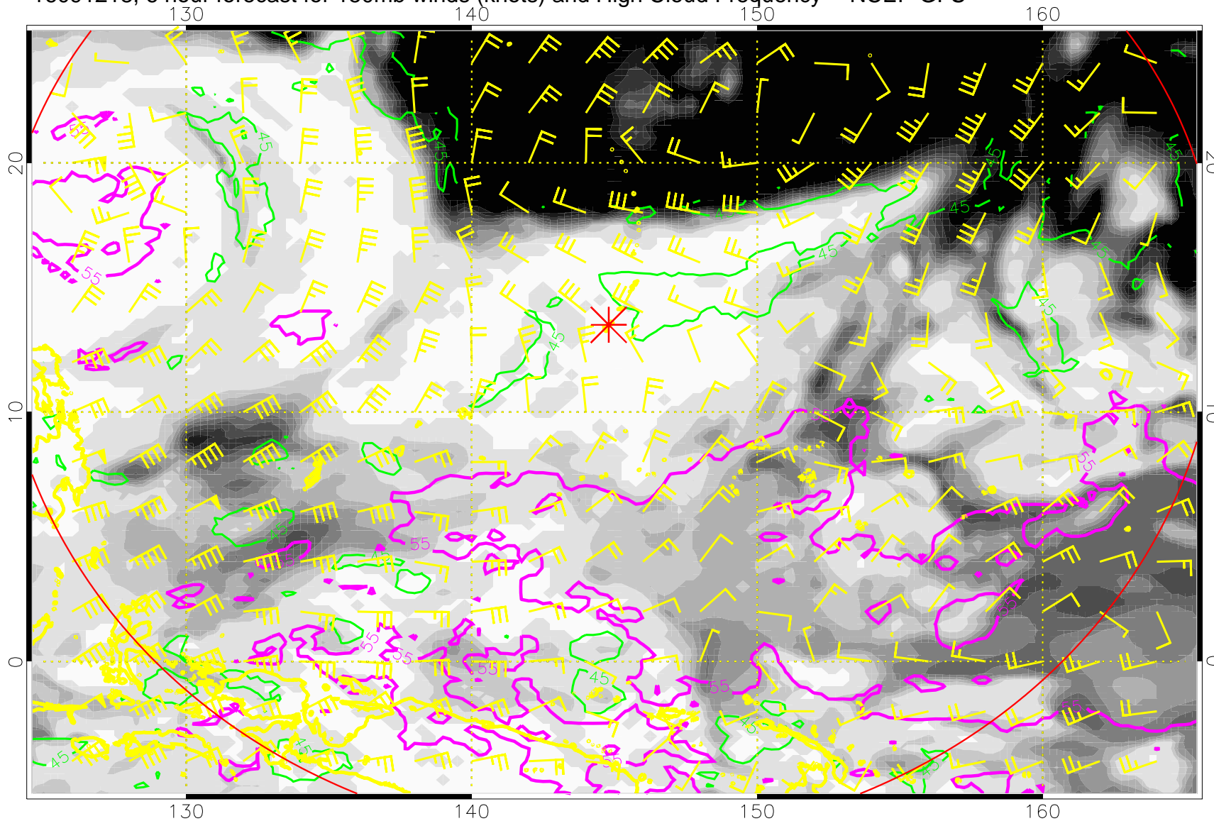
16091218, 6 hour forecast for 150mb winds (knots) and High Cloud Frequency -- NCEP GFS
