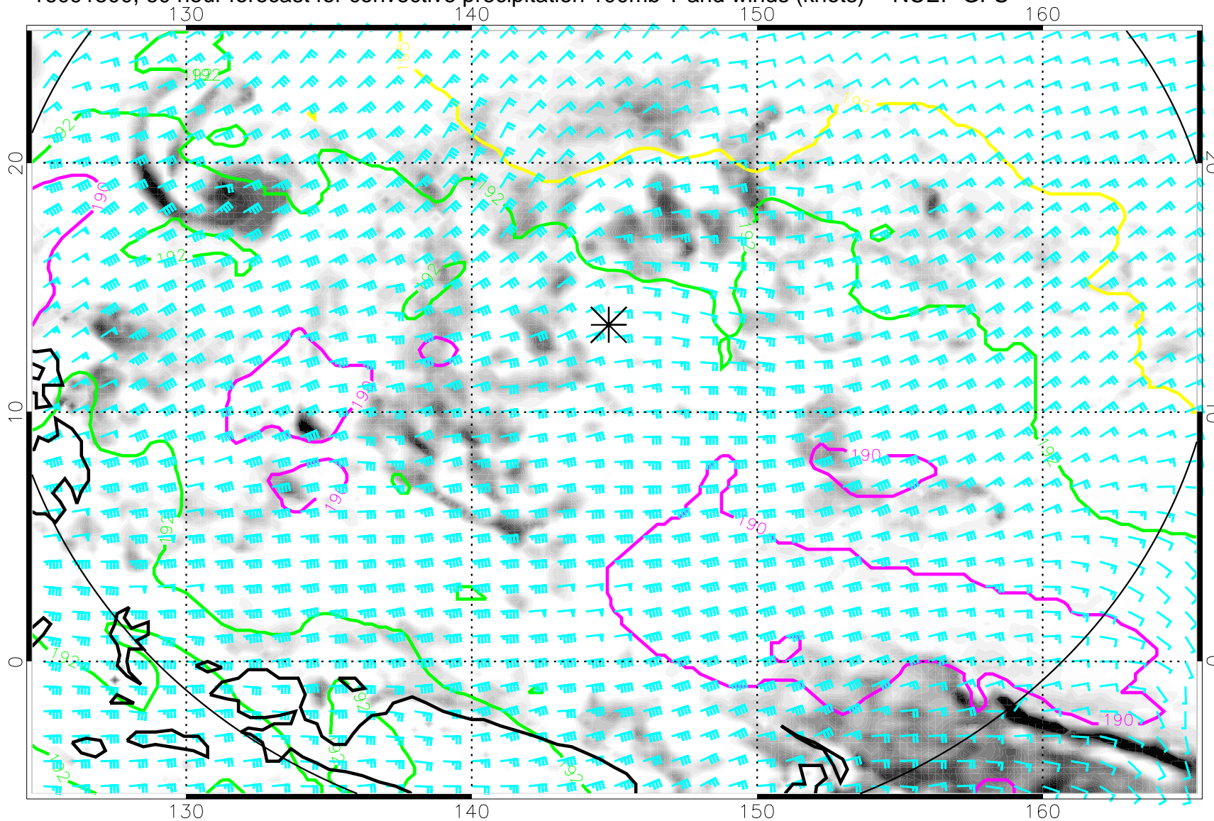
16091500, 60 hour forecast for convective precipitation 100mb T and winds (knots) -- NCEP GFS
