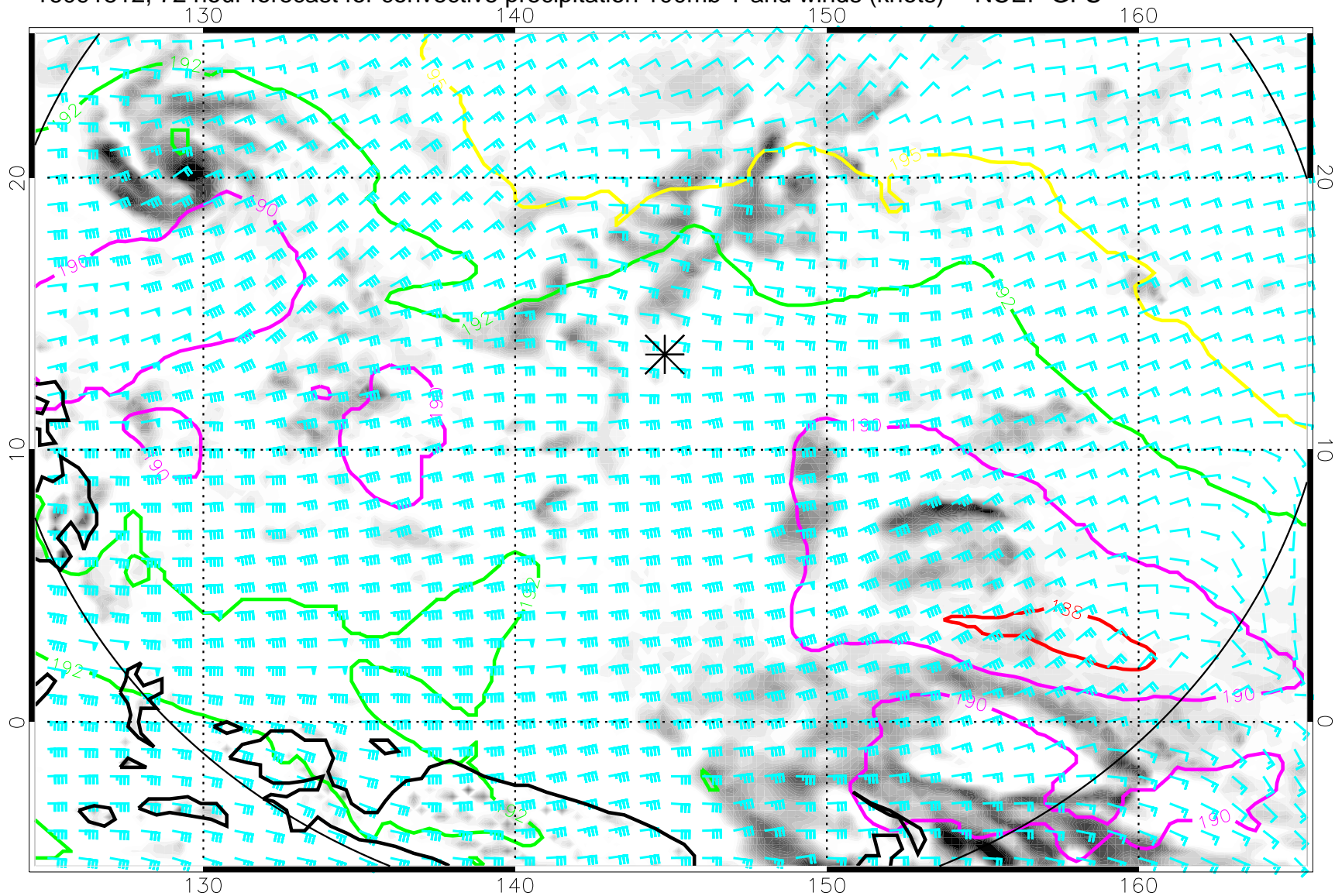
16091512, 72 hour forecast for convective precipitation 100mb T and winds (knots) -- NCEP GFS
