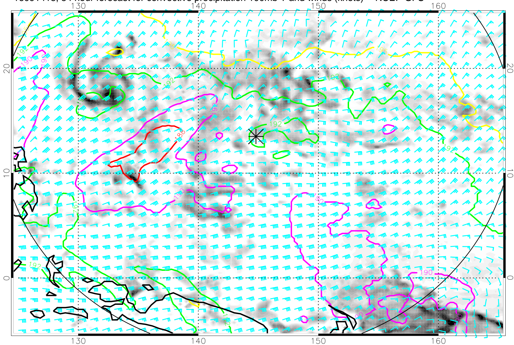
16091418, 54 hour forecast for convective precipitation 100mb T and winds (knots) -- NCEP GFS
