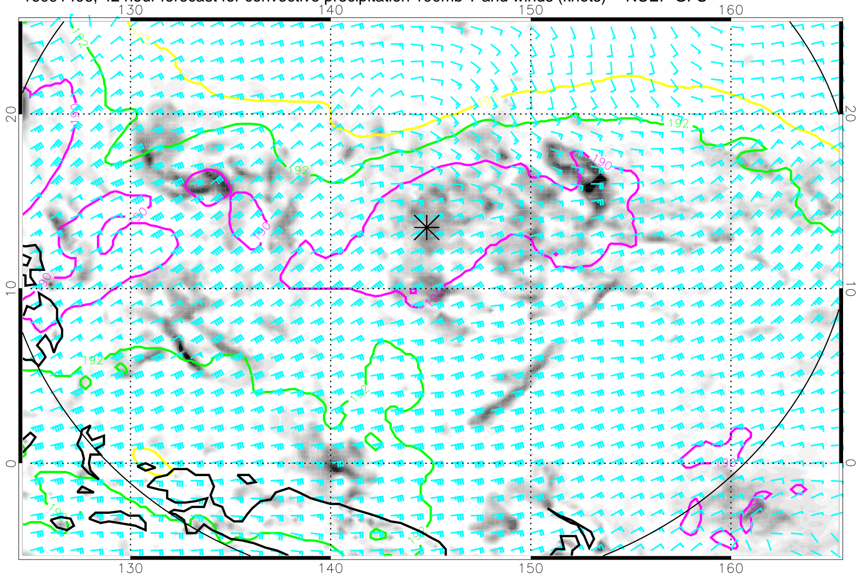
16091406, 42 hour forecast for convective precipitation 100mb T and winds (knots) -- NCEP GFS
