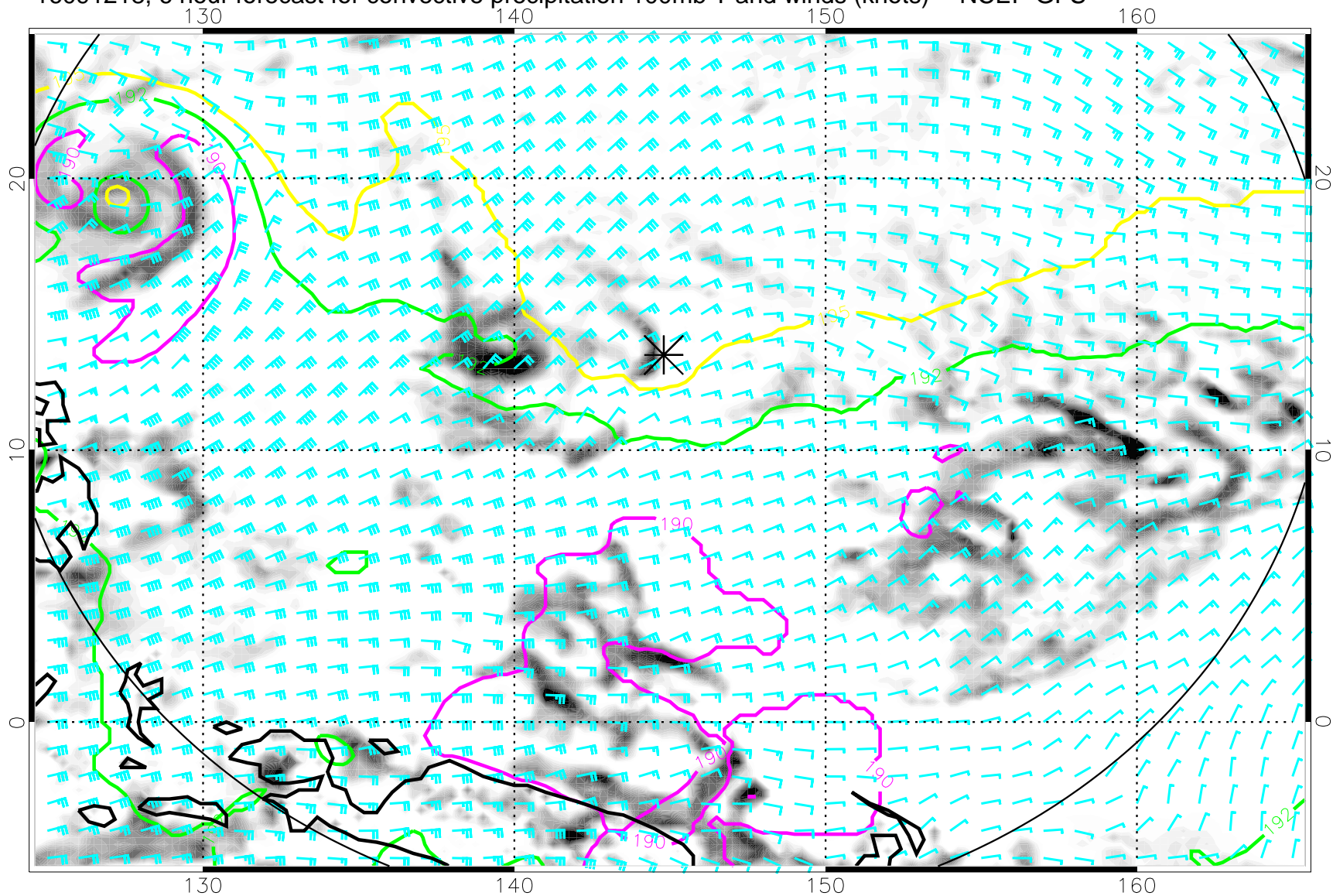
16091218, 6 hour forecast for convective precipitation 100mb T and winds (knots) -- NCEP GFS
