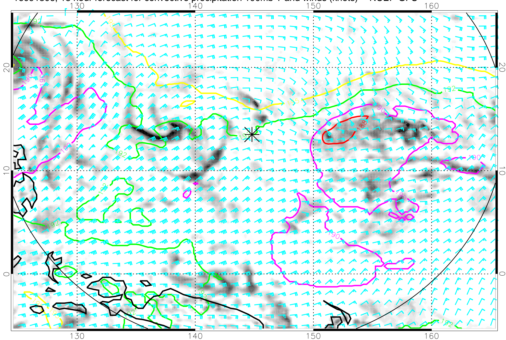
16091306, 18 hour forecast for convective precipitation 100mb T and winds (knots) -- NCEP GFS
