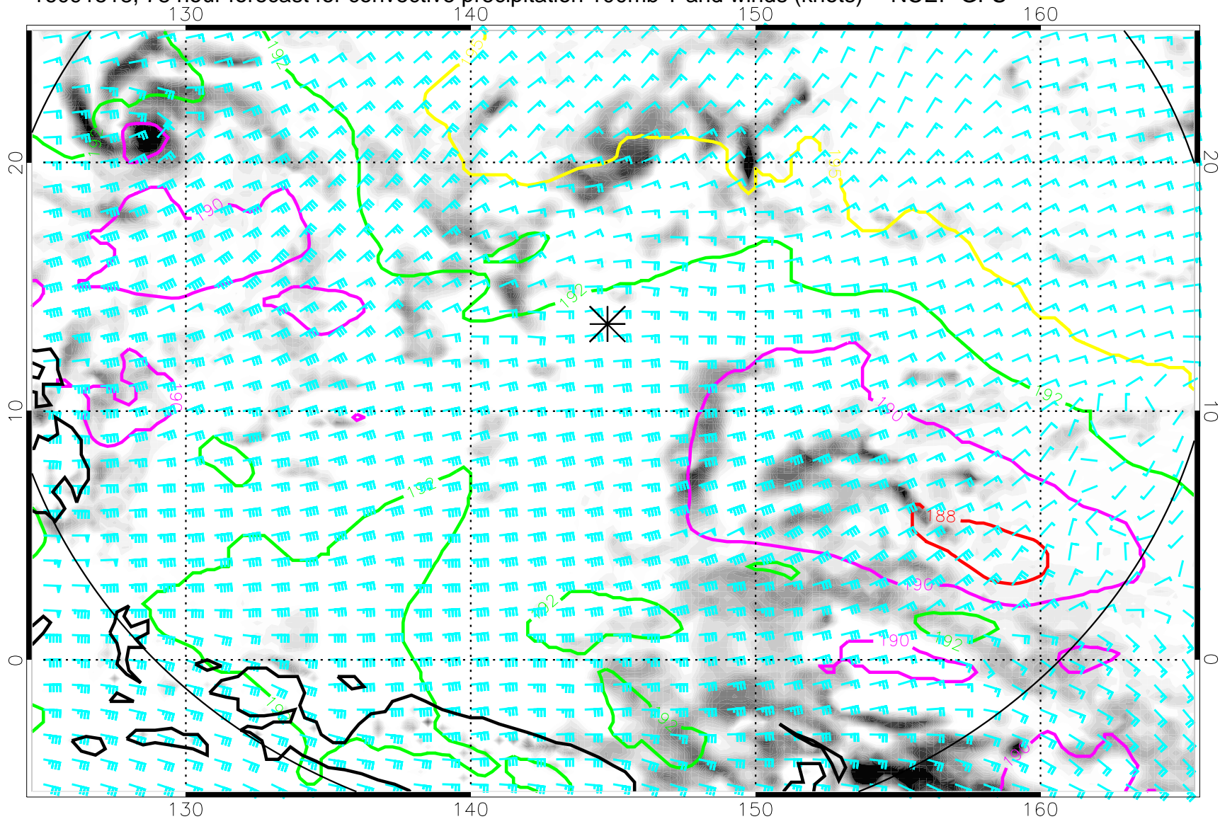
16091518, 78 hour forecast for convective precipitation 100mb T and winds (knots) -- NCEP GFS
