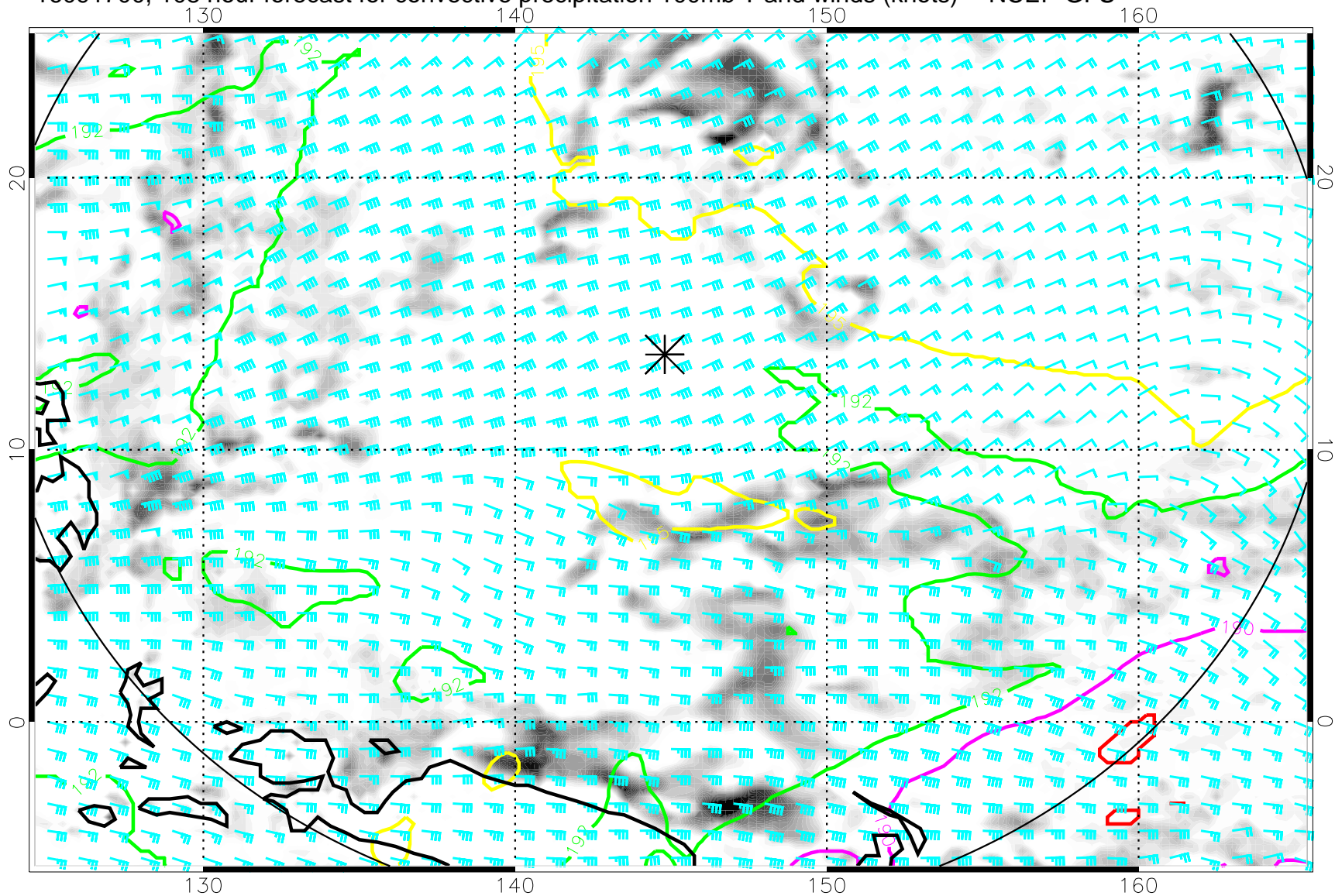
16091700, 108 hour forecast for convective precipitation 100mb T and winds (knots) -- NCEP GFS
