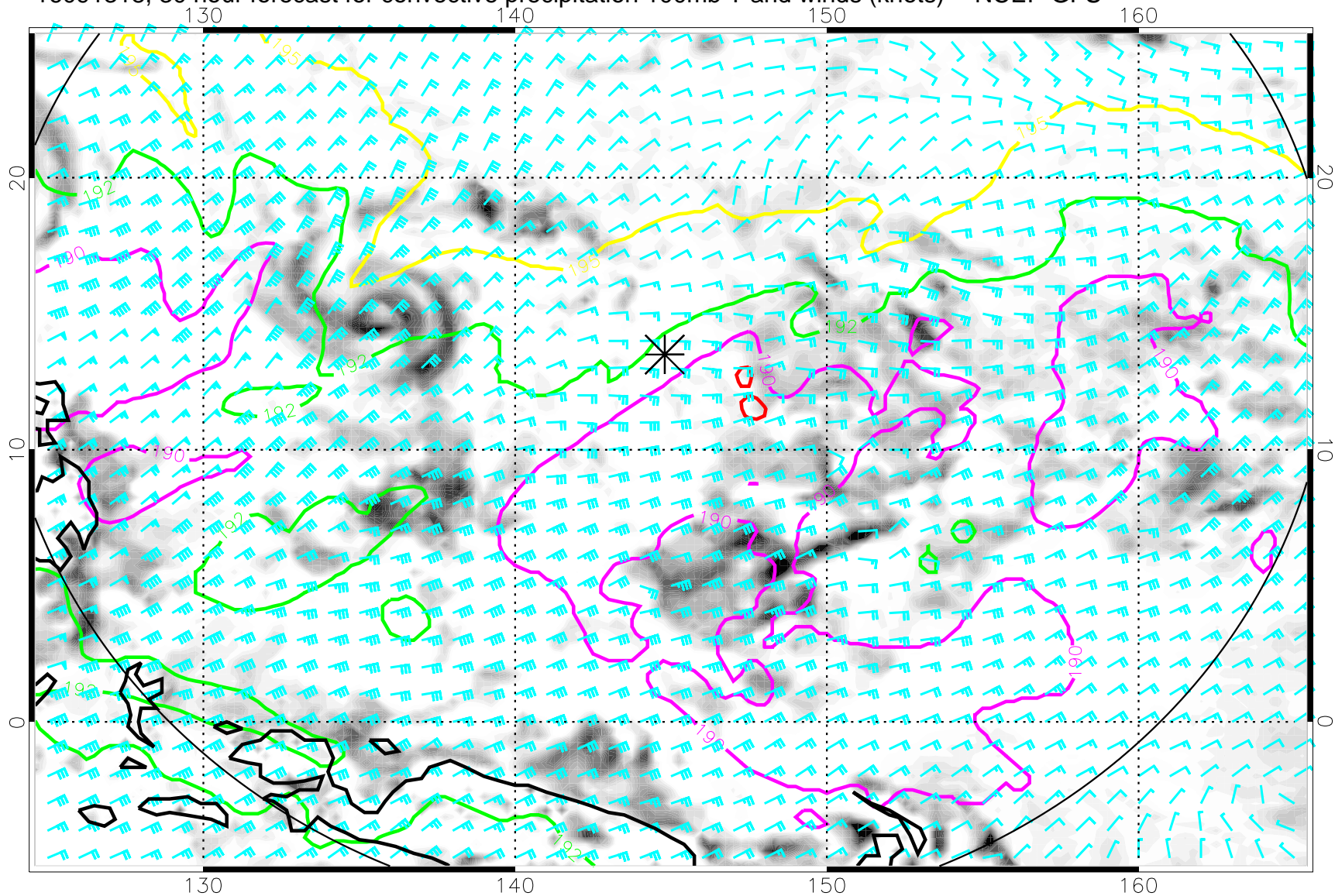
16091318, 30 hour forecast for convective precipitation 100mb T and winds (knots) -- NCEP GFS
