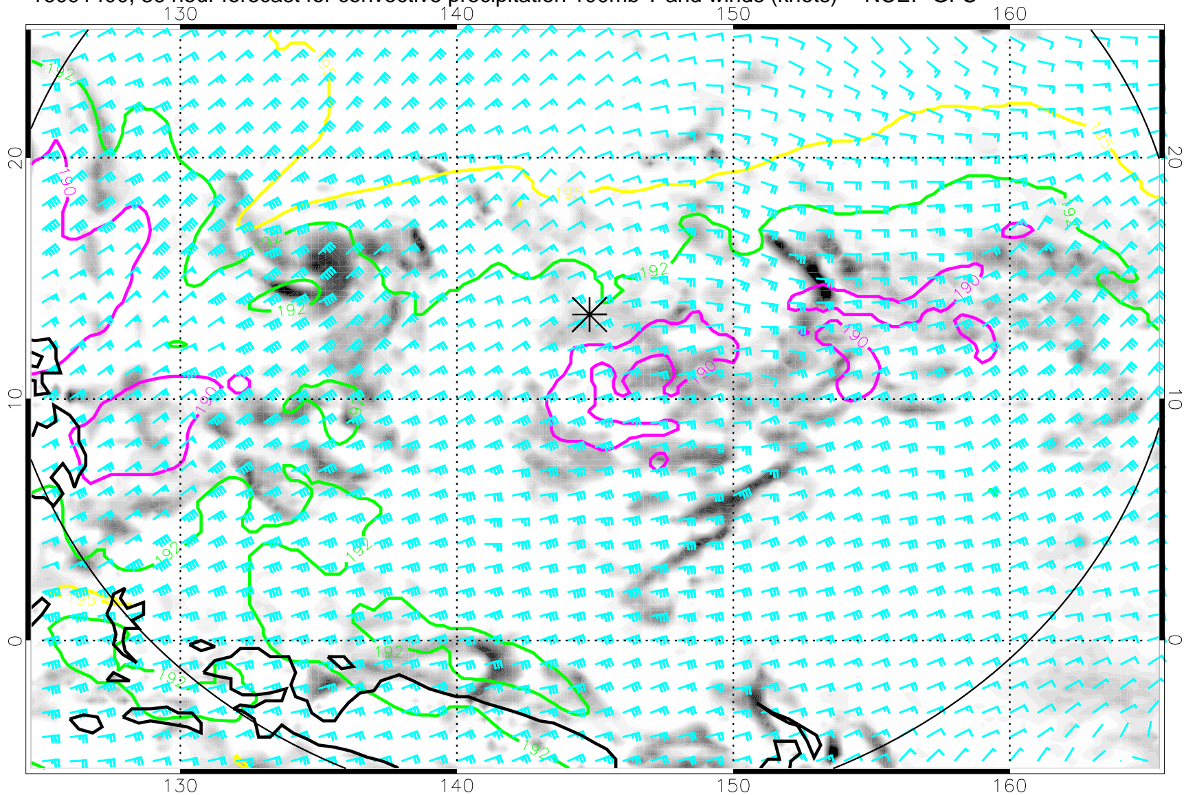
16091400, 36 hour forecast for convective precipitation 100mb T and winds (knots) -- NCEP GFS
