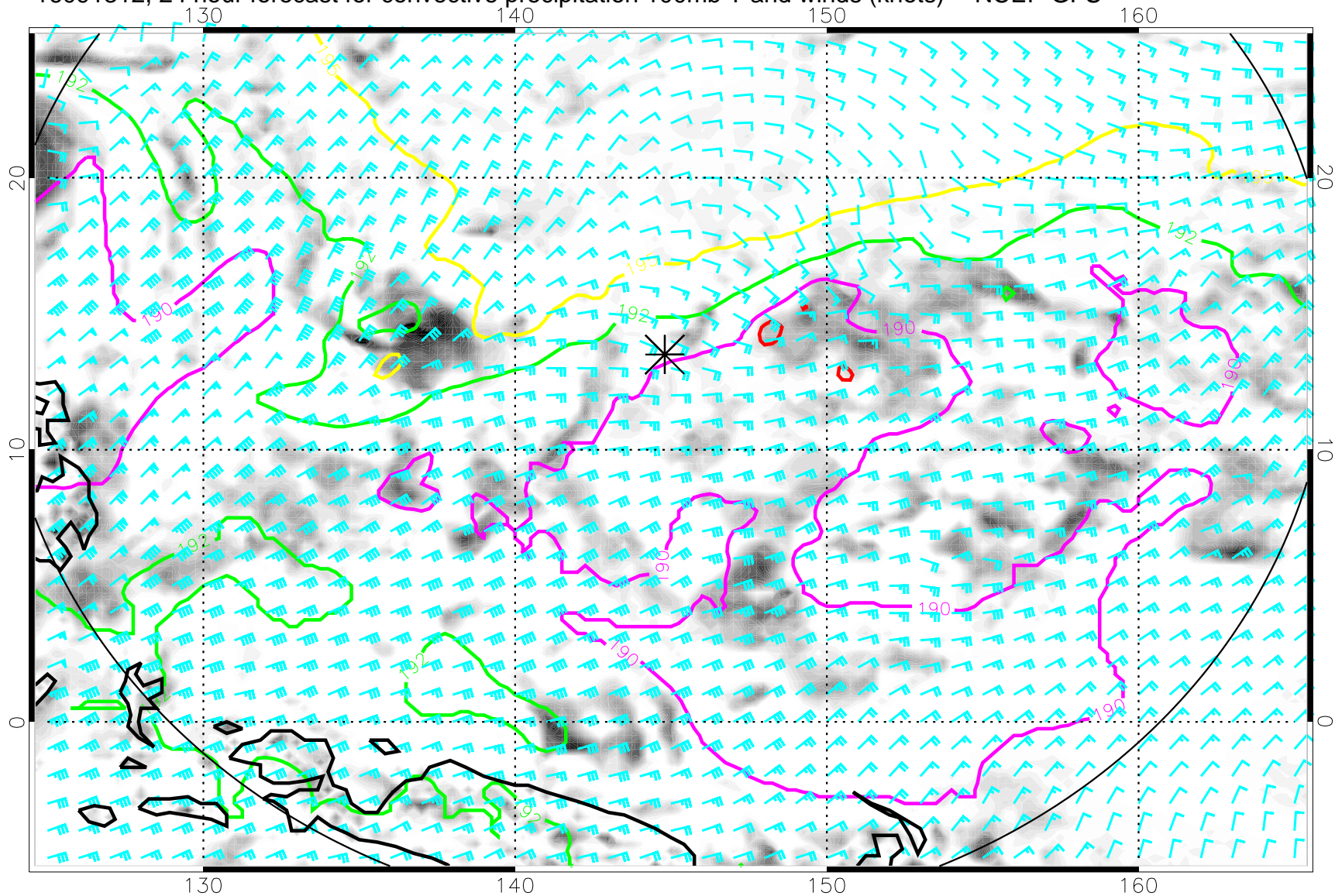
16091312, 24 hour forecast for convective precipitation 100mb T and winds (knots) -- NCEP GFS
