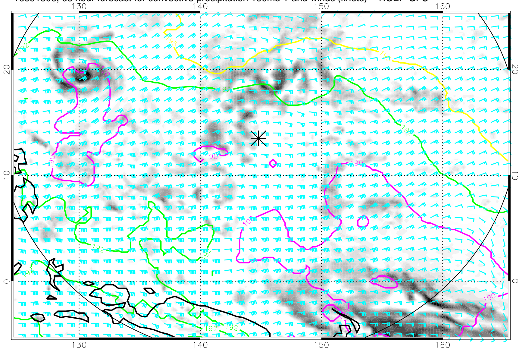
16091506, 66 hour forecast for convective precipitation 100mb T and winds (knots) -- NCEP GFS
