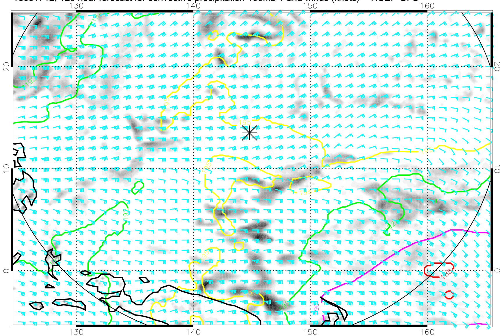
16091712, 120 hour forecast for convective precipitation 100mb T and winds (knots) -- NCEP GFS
