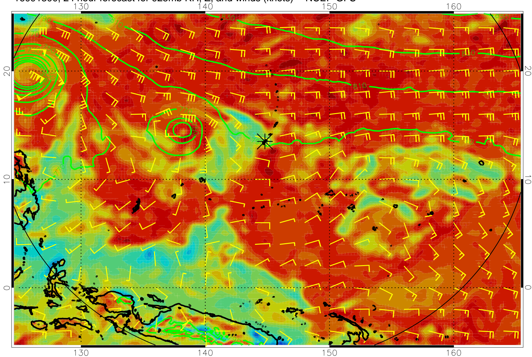
16091300, 24 hour forecast for 925mb RH, Z, and winds (knots) -- NCEP GFS
