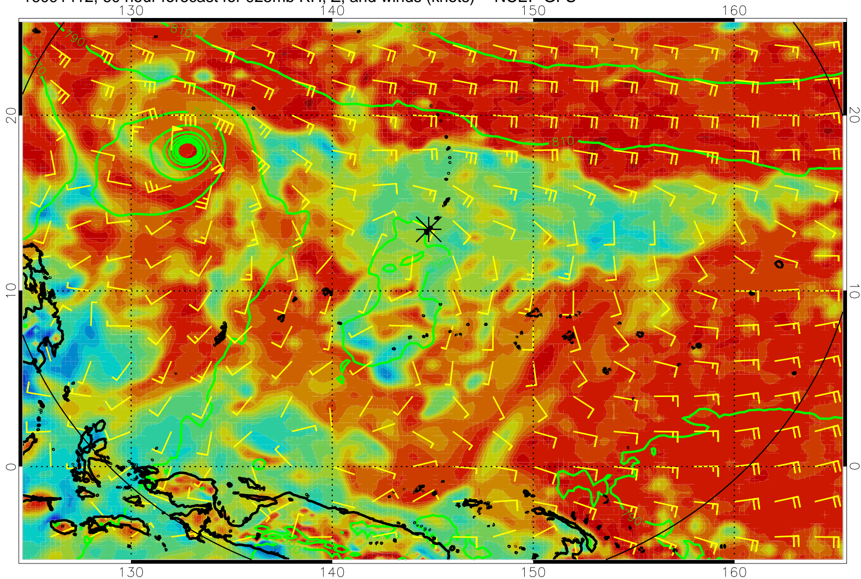
16091412, 60 hour forecast for 925mb RH, Z, and winds (knots) -- NCEP GFS
