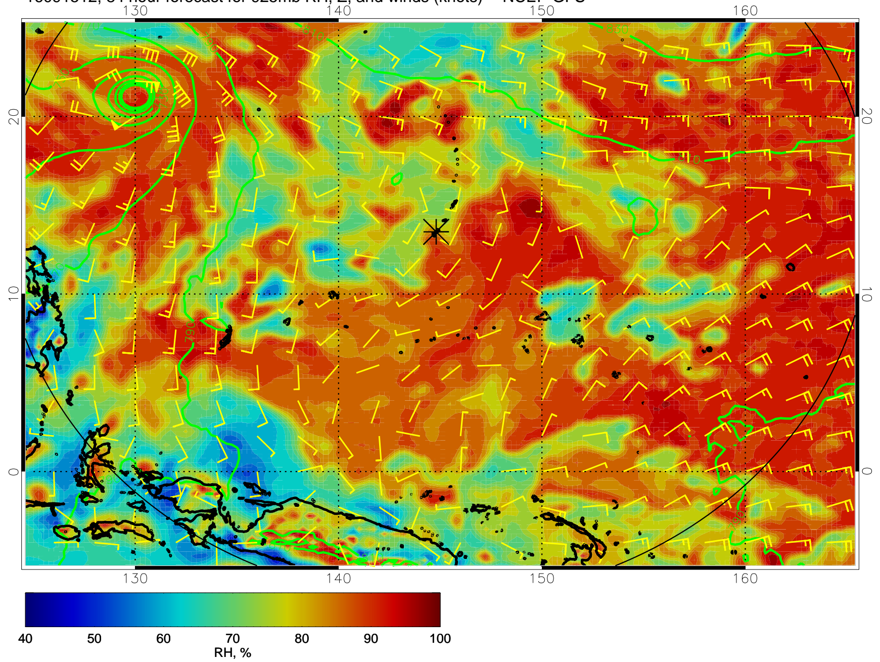
16091512, 84 hour forecast for 925mb RH, Z, and winds (knots) -- NCEP GFS
