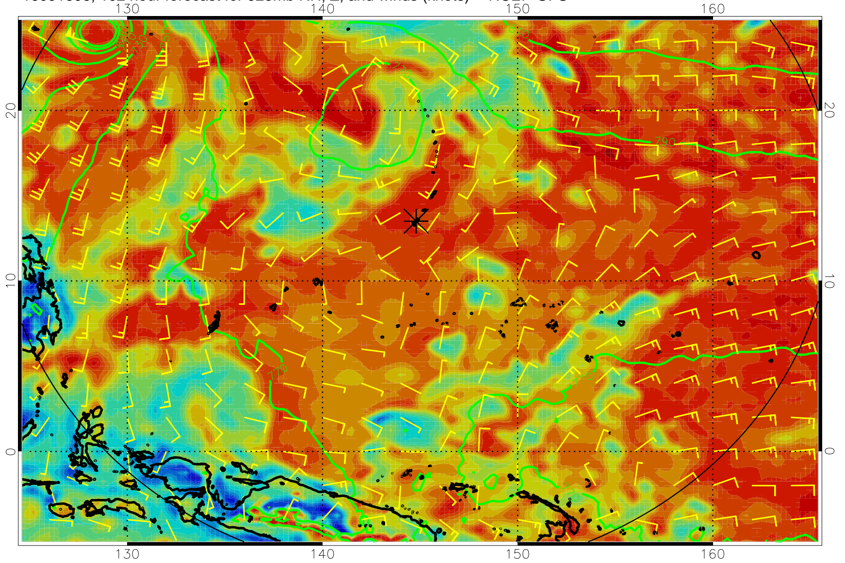
16091606, 102 hour forecast for 925mb RH, Z, and winds (knots) -- NCEP GFS
