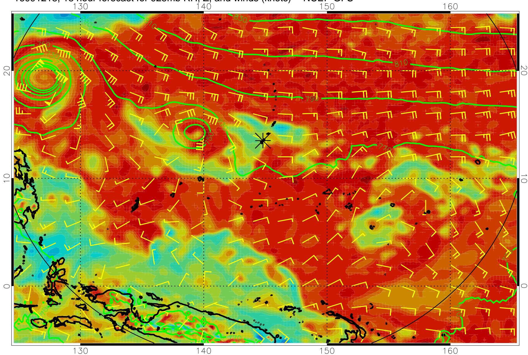
16091218, 18 hour forecast for 925mb RH, Z, and winds (knots) -- NCEP GFS
