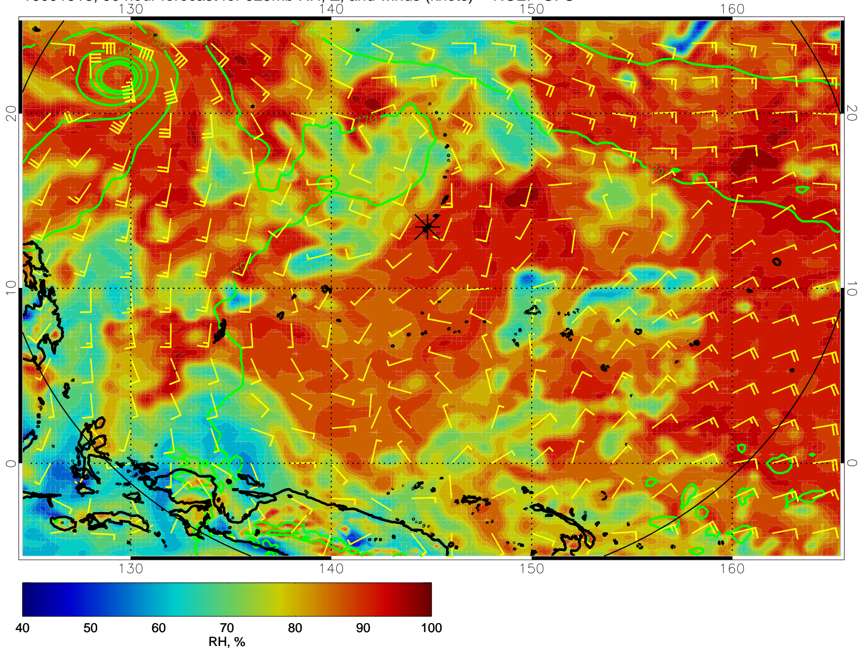
16091518, 90 hour forecast for 925mb RH, Z, and winds (knots) -- NCEP GFS
