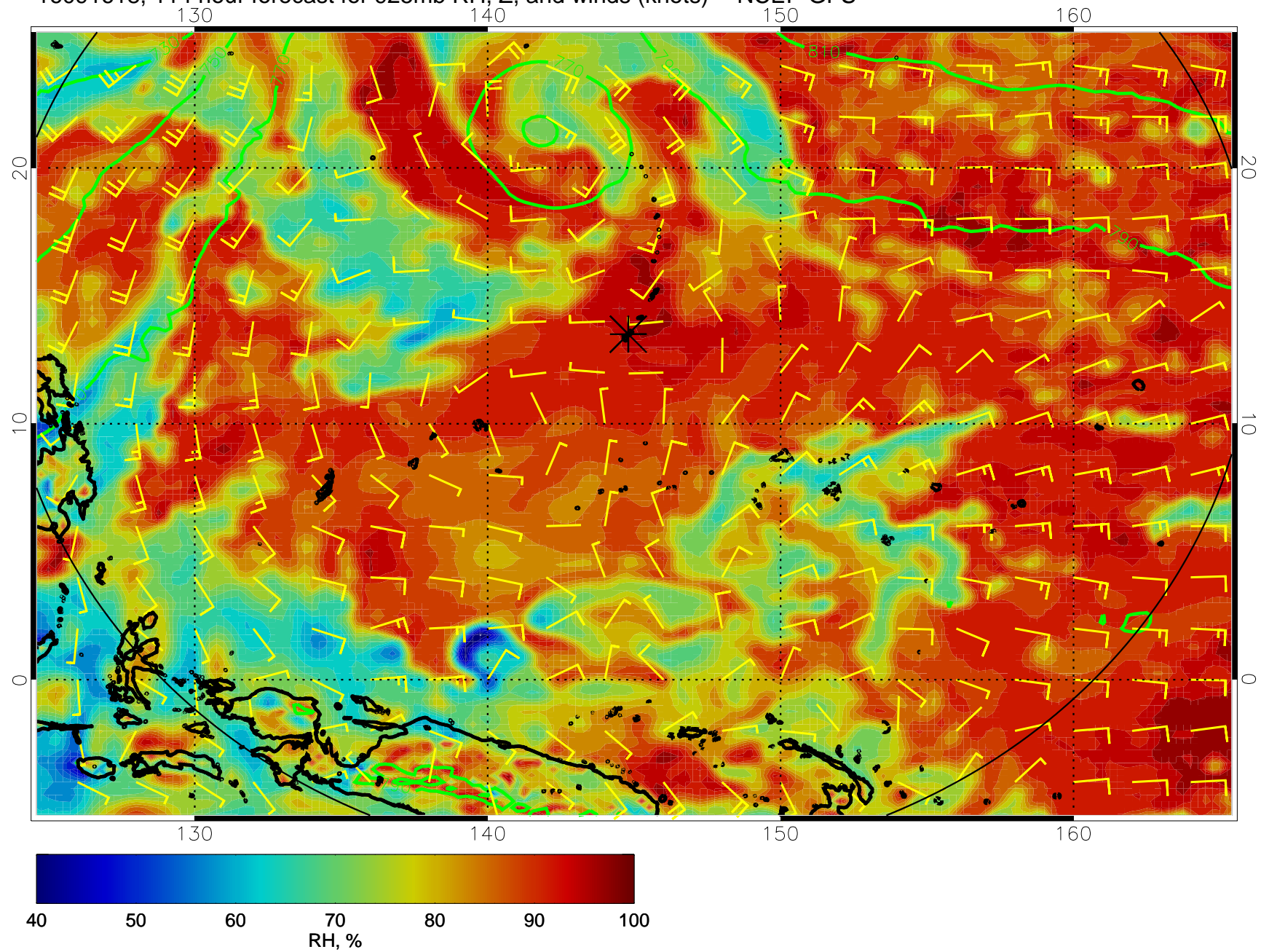
16091618, 114 hour forecast for 925mb RH, Z, and winds (knots) -- NCEP GFS
