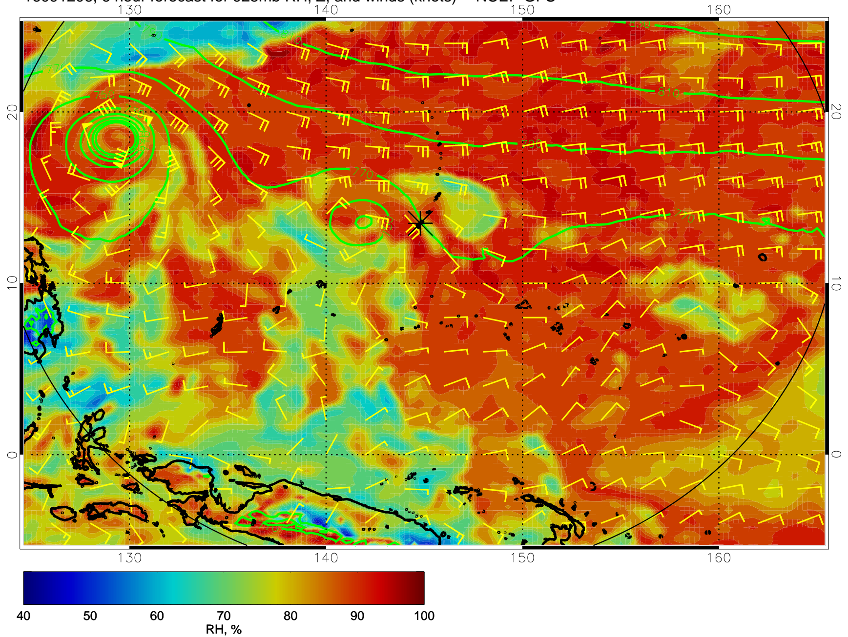
16091206, 6 hour forecast for 925mb RH, Z, and winds (knots) -- NCEP GFS
