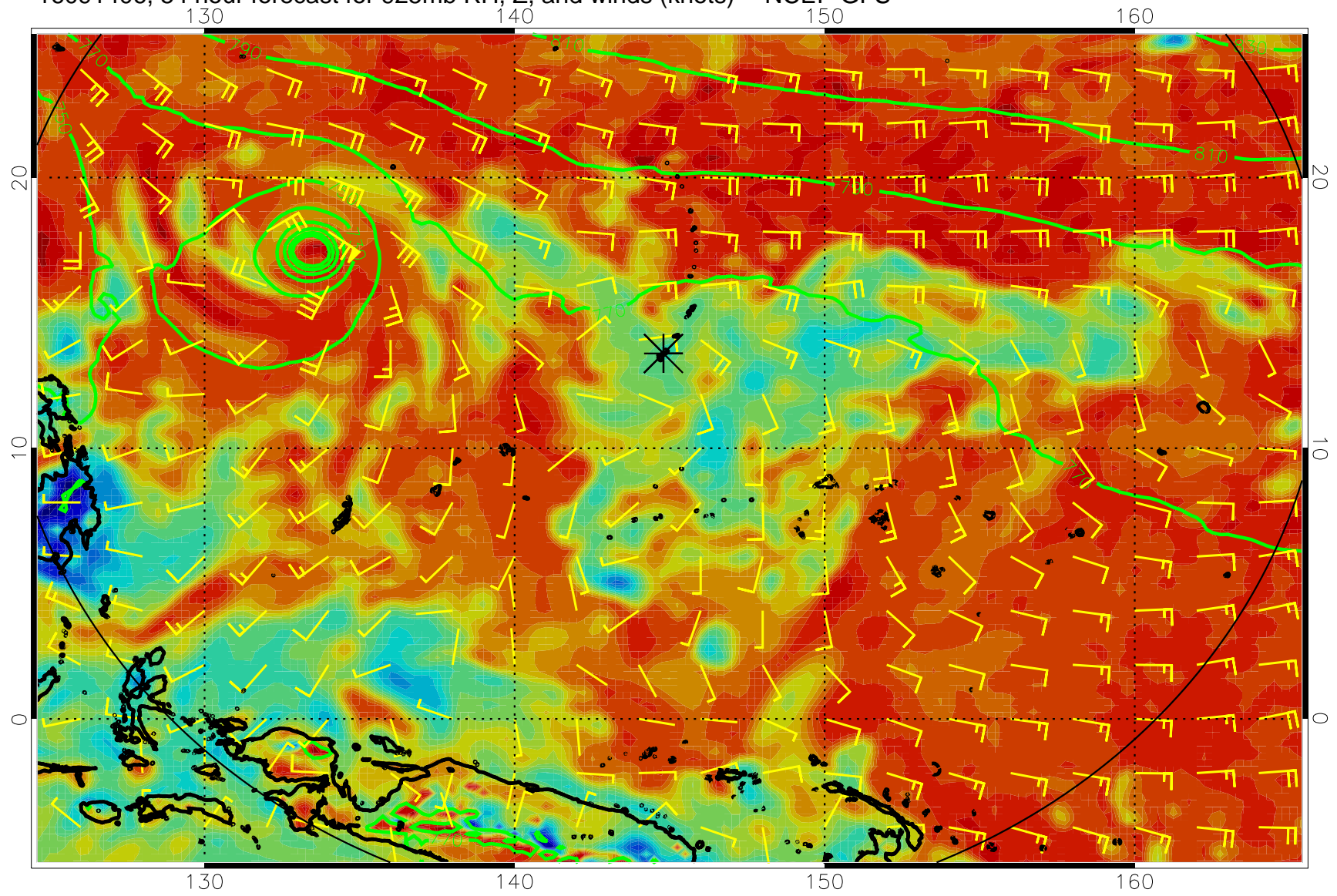
16091406, 54 hour forecast for 925mb RH, Z, and winds (knots) -- NCEP GFS
