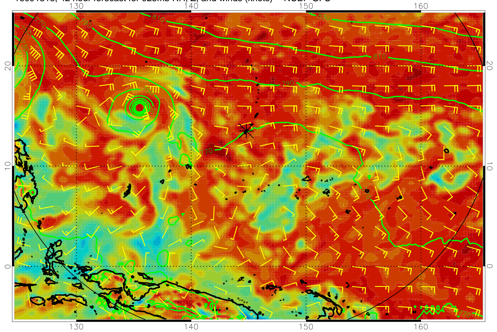
16091318, 42 hour forecast for 925mb RH, Z, and winds (knots) -- NCEP GFS
