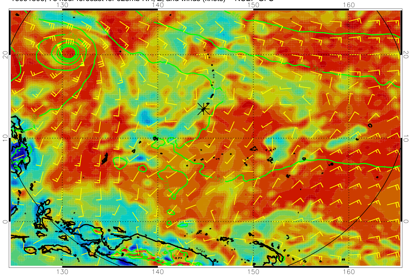
16091506, 78 hour forecast for 925mb RH, Z, and winds (knots) -- NCEP GFS
