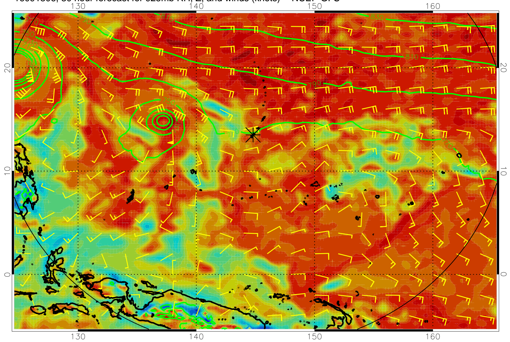
16091306, 30 hour forecast for 925mb RH, Z, and winds (knots) -- NCEP GFS
