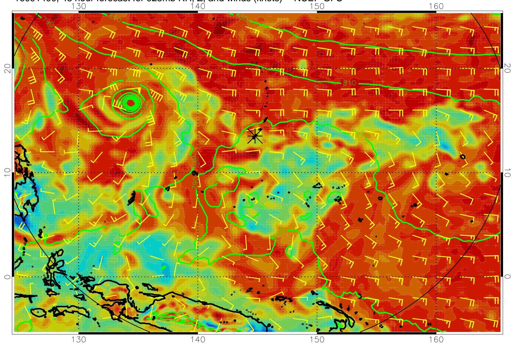
16091400, 48 hour forecast for 925mb RH, Z, and winds (knots) -- NCEP GFS
