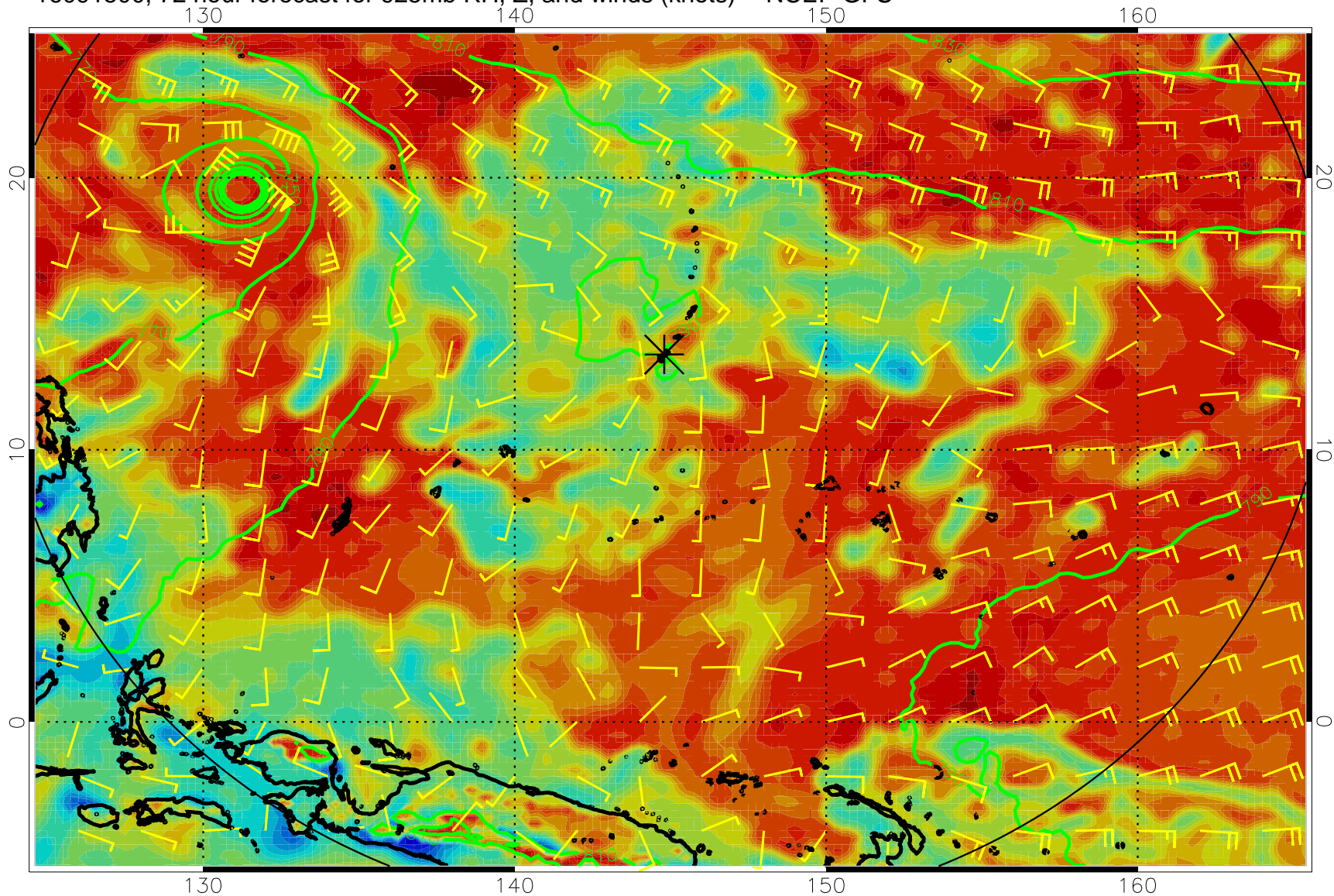
16091500, 72 hour forecast for 925mb RH, Z, and winds (knots) -- NCEP GFS
