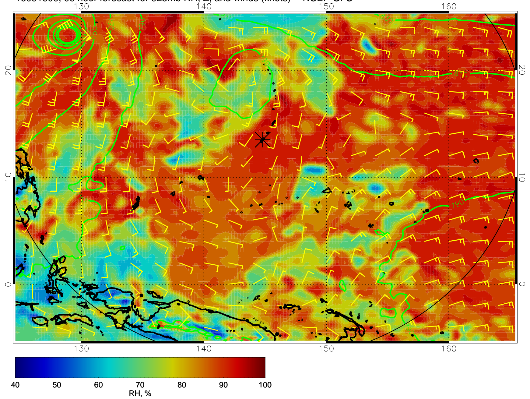
16091600, 96 hour forecast for 925mb RH, Z, and winds (knots) -- NCEP GFS
