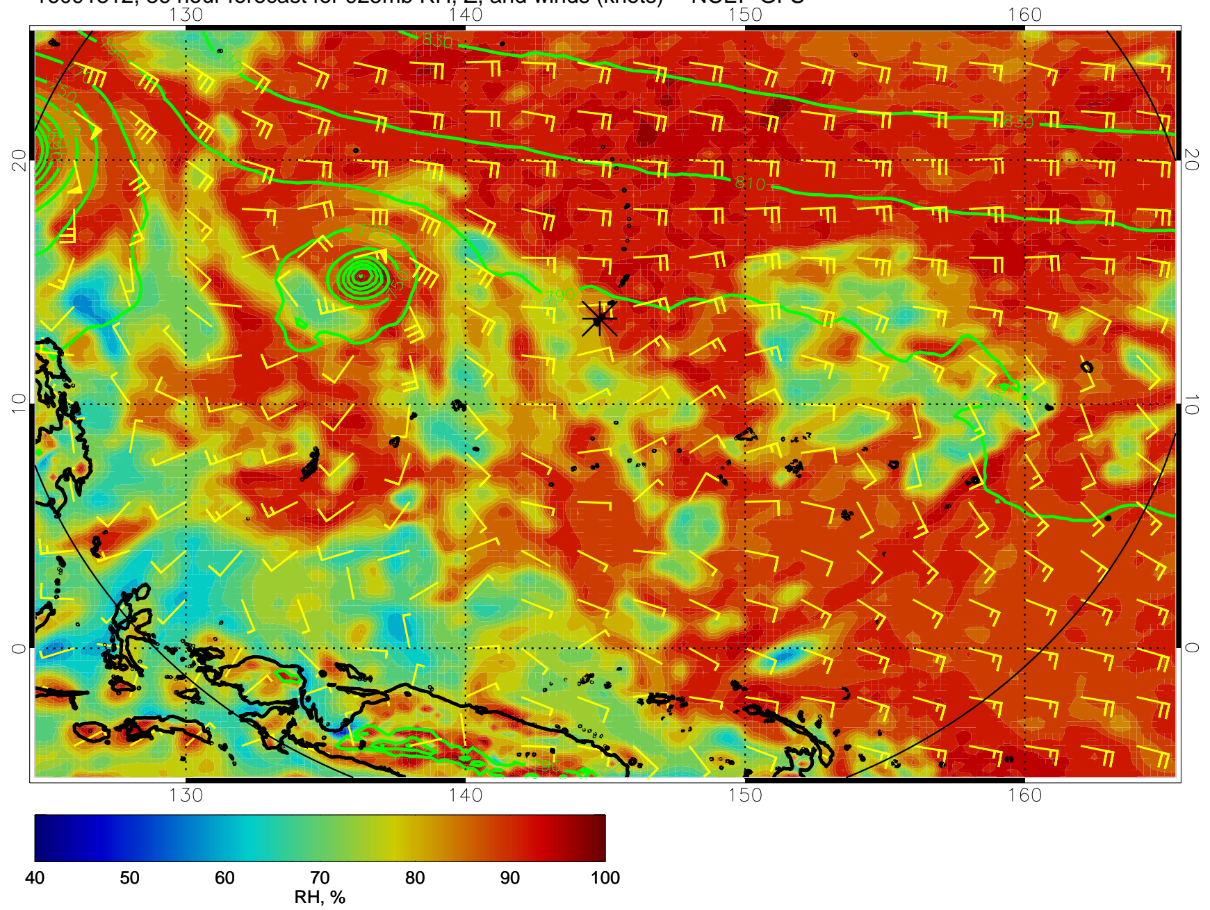
16091312, 36 hour forecast for 925mb RH, Z, and winds (knots) -- NCEP GFS
