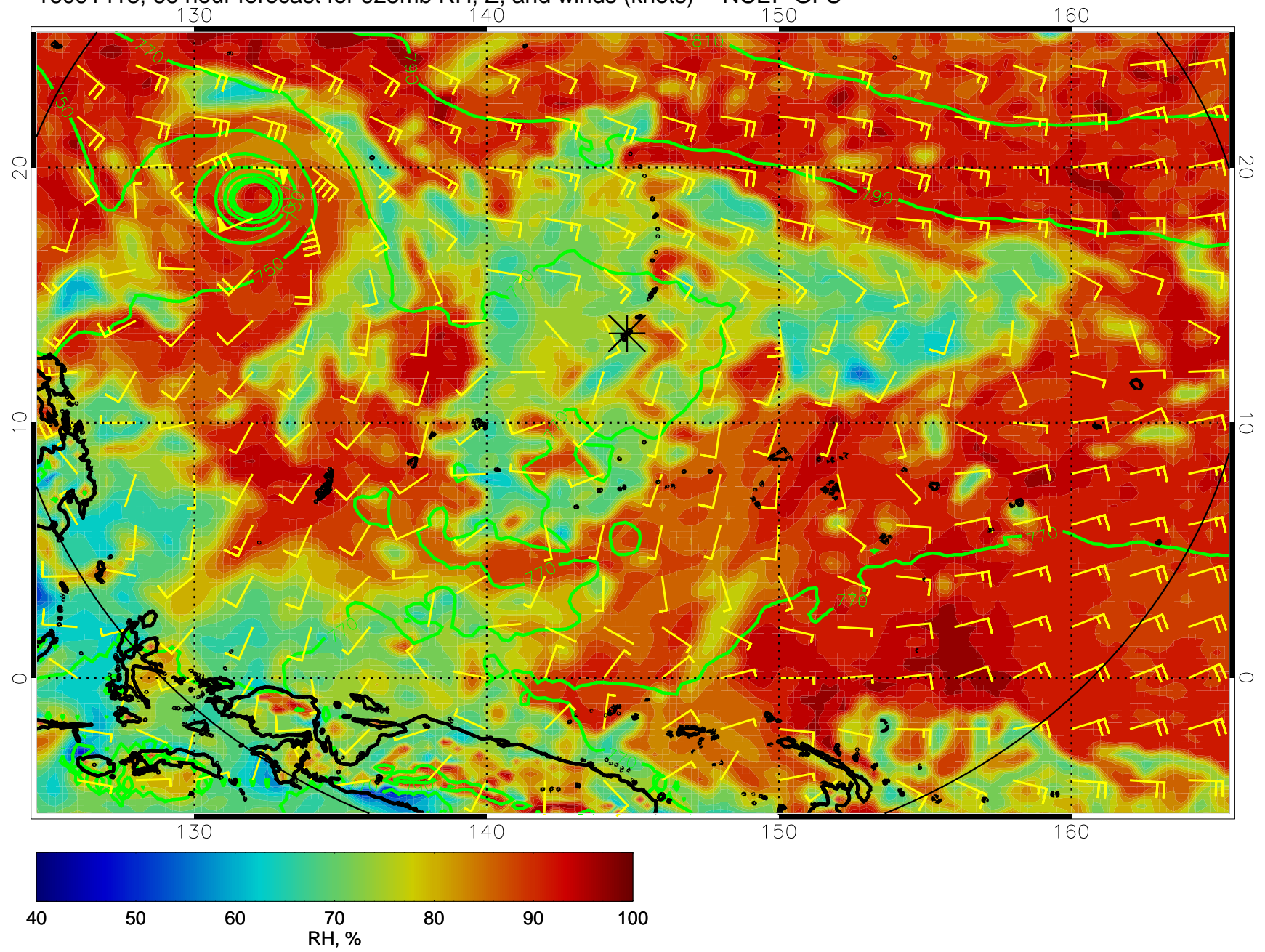
16091418, 66 hour forecast for 925mb RH, Z, and winds (knots) -- NCEP GFS
