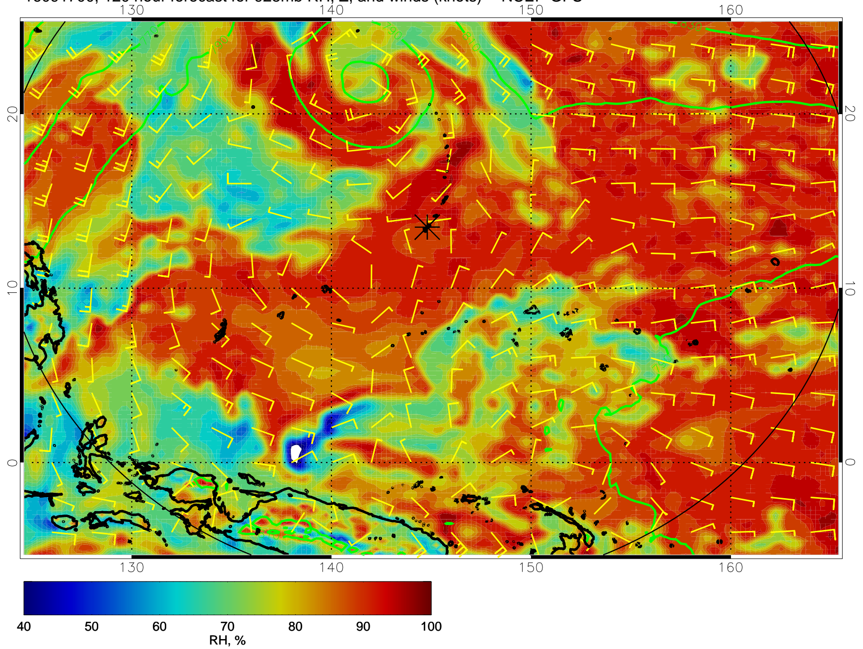
16091700, 120 hour forecast for 925mb RH, Z, and winds (knots) -- NCEP GFS
