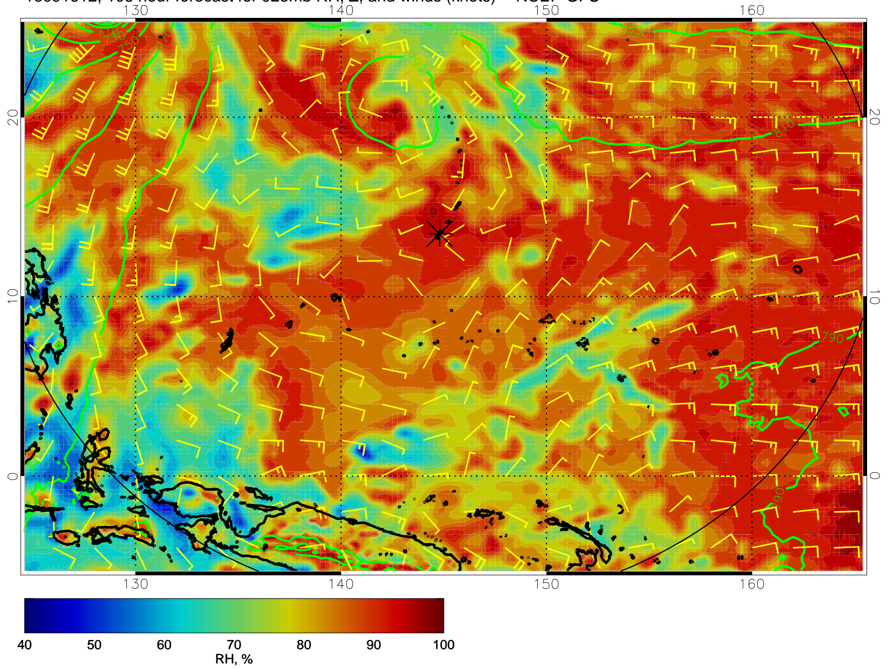
16091612, 108 hour forecast for 925mb RH, Z, and winds (knots) -- NCEP GFS
