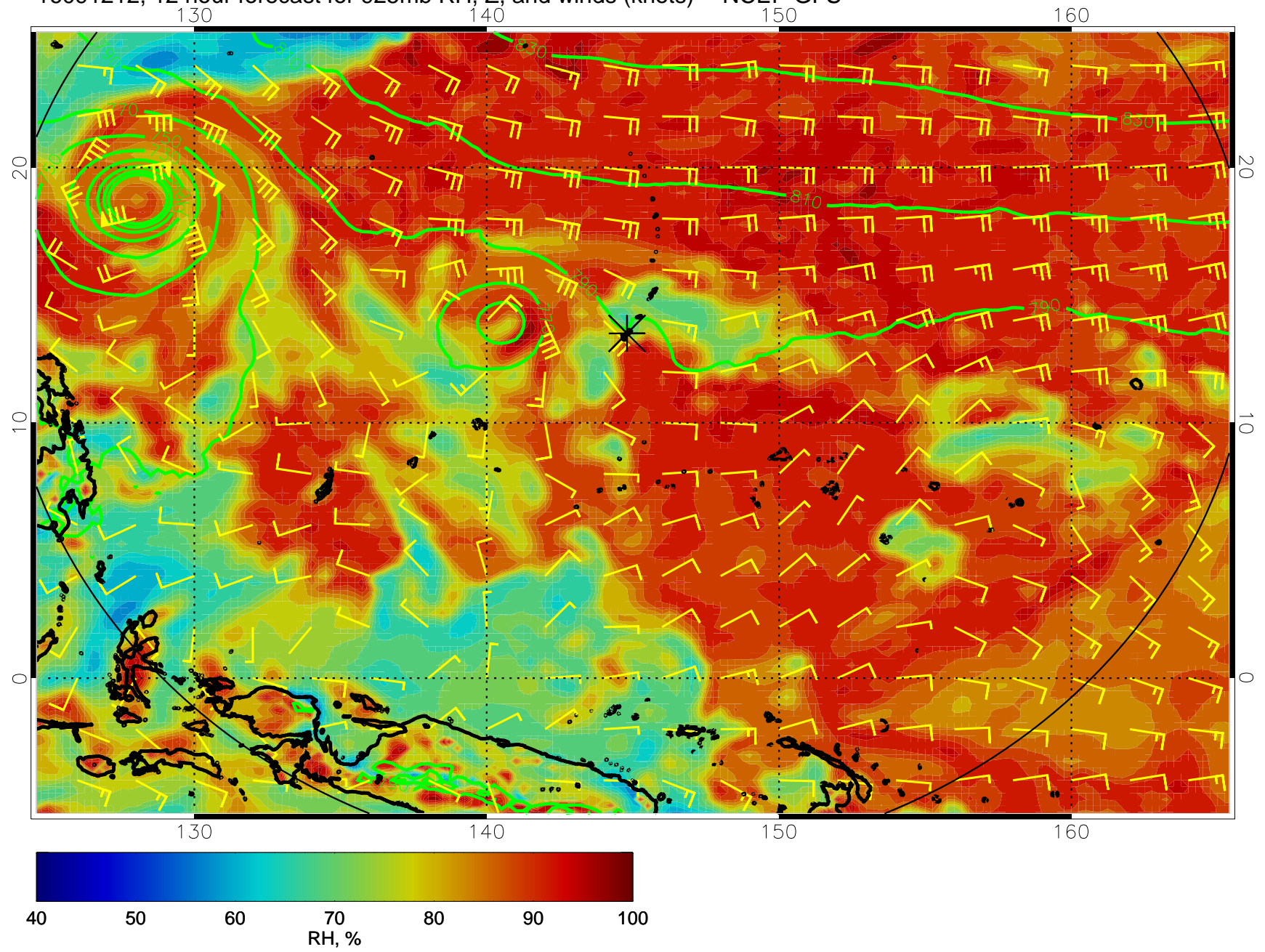
16091212, 12 hour forecast for 925mb RH, Z, and winds (knots) -- NCEP GFS
