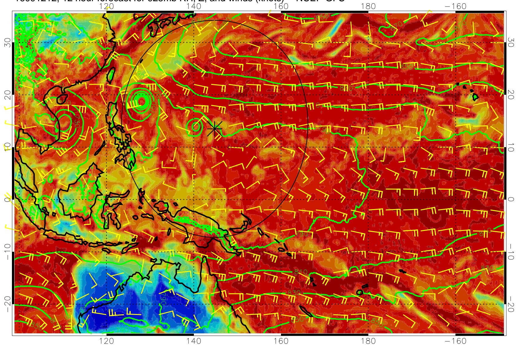
16091212, 12 hour forecast for 925mb RH, Z, and winds (knots) -- NCEP GFS
