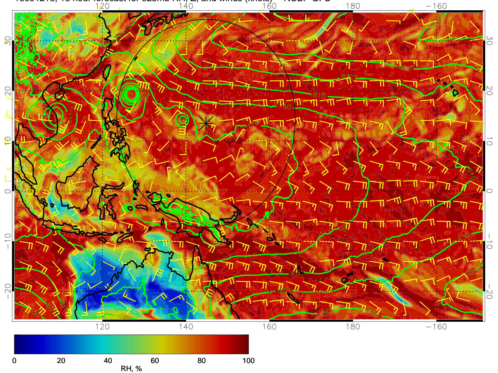
16091218, 18 hour forecast for 925mb RH, Z, and winds (knots) -- NCEP GFS
