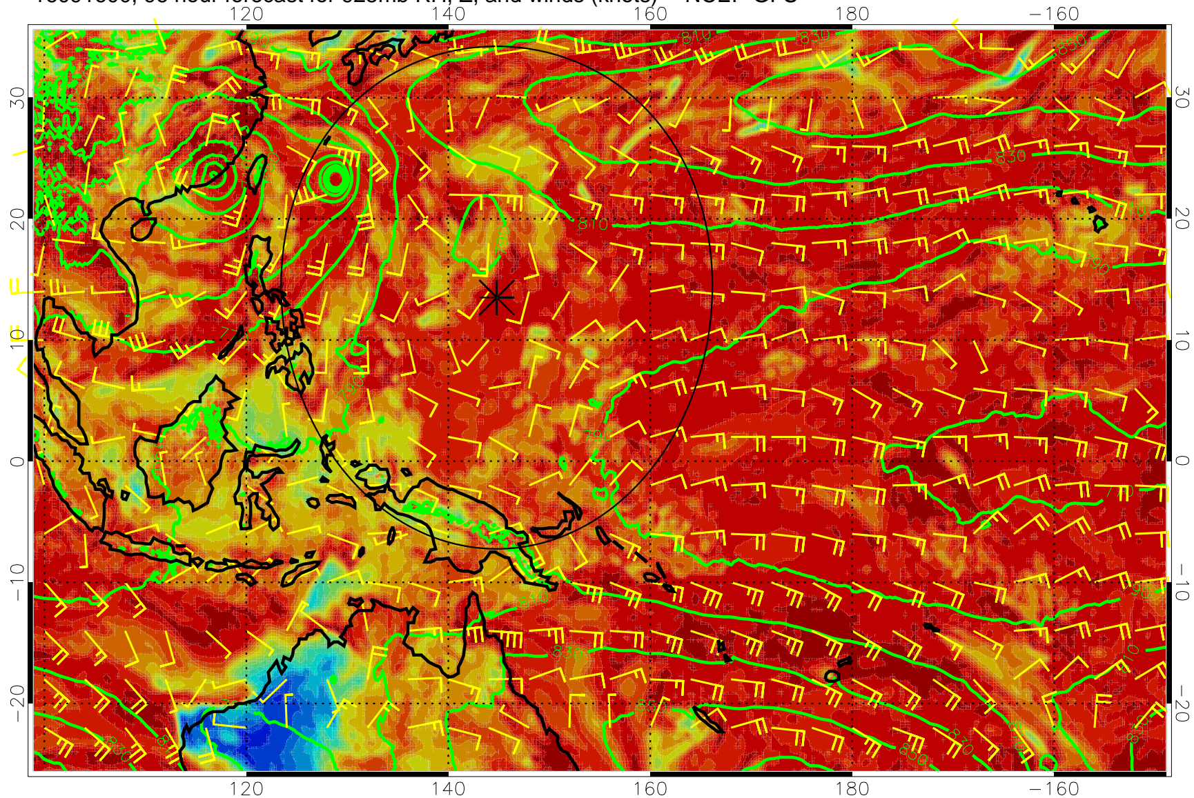
16091600, 96 hour forecast for 925mb RH, Z, and winds (knots) -- NCEP GFS
