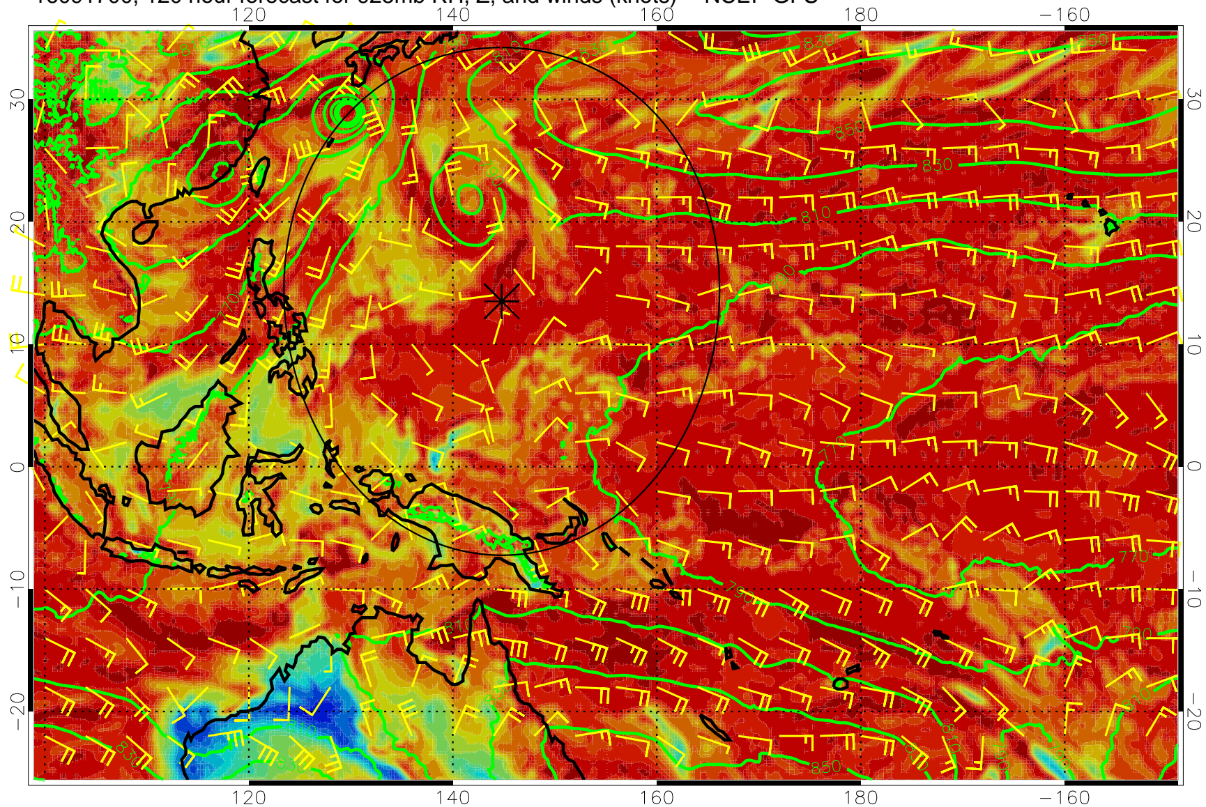
16091700, 120 hour forecast for 925mb RH, Z, and winds (knots) -- NCEP GFS
