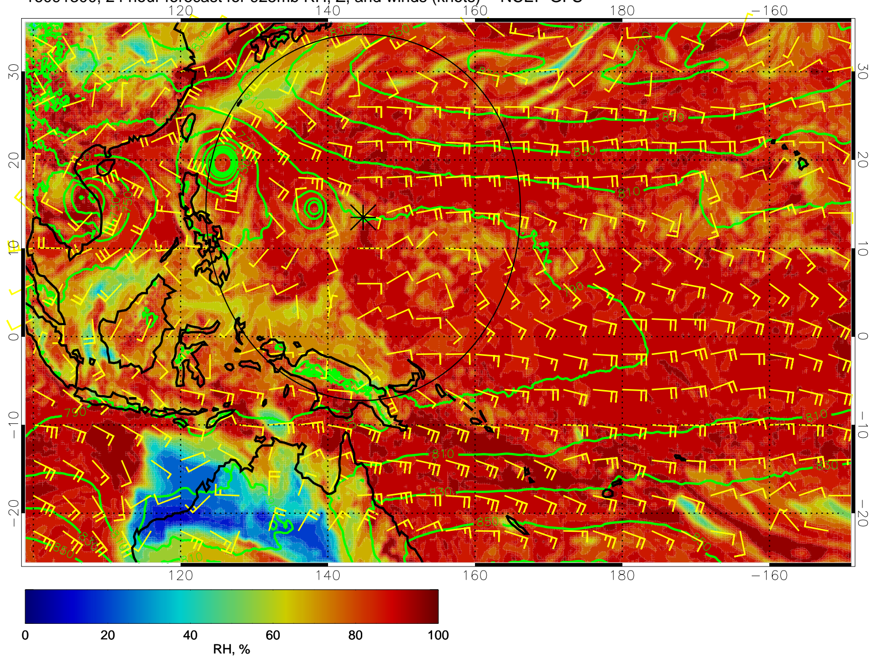
16091300, 24 hour forecast for 925mb RH, Z, and winds (knots) -- NCEP GFS
