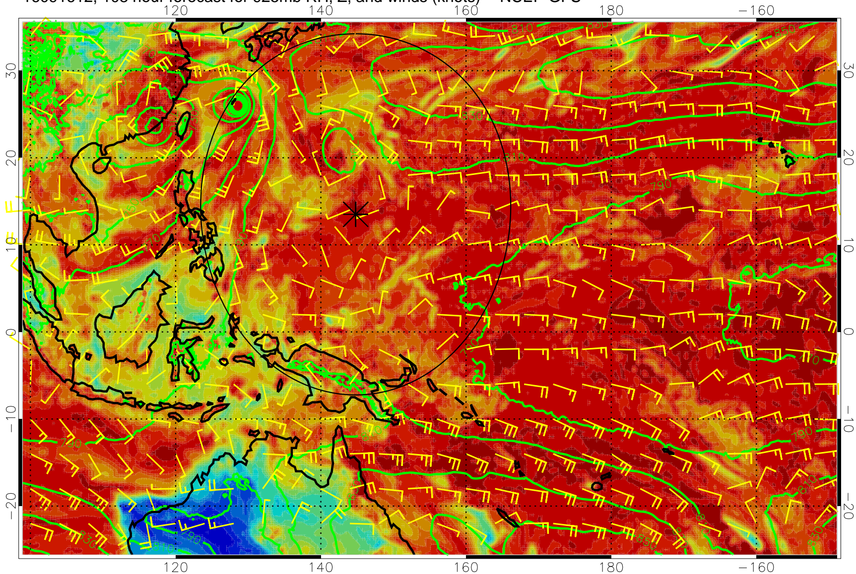
16091612, 108 hour forecast for 925mb RH, Z, and winds (knots) -- NCEP GFS
