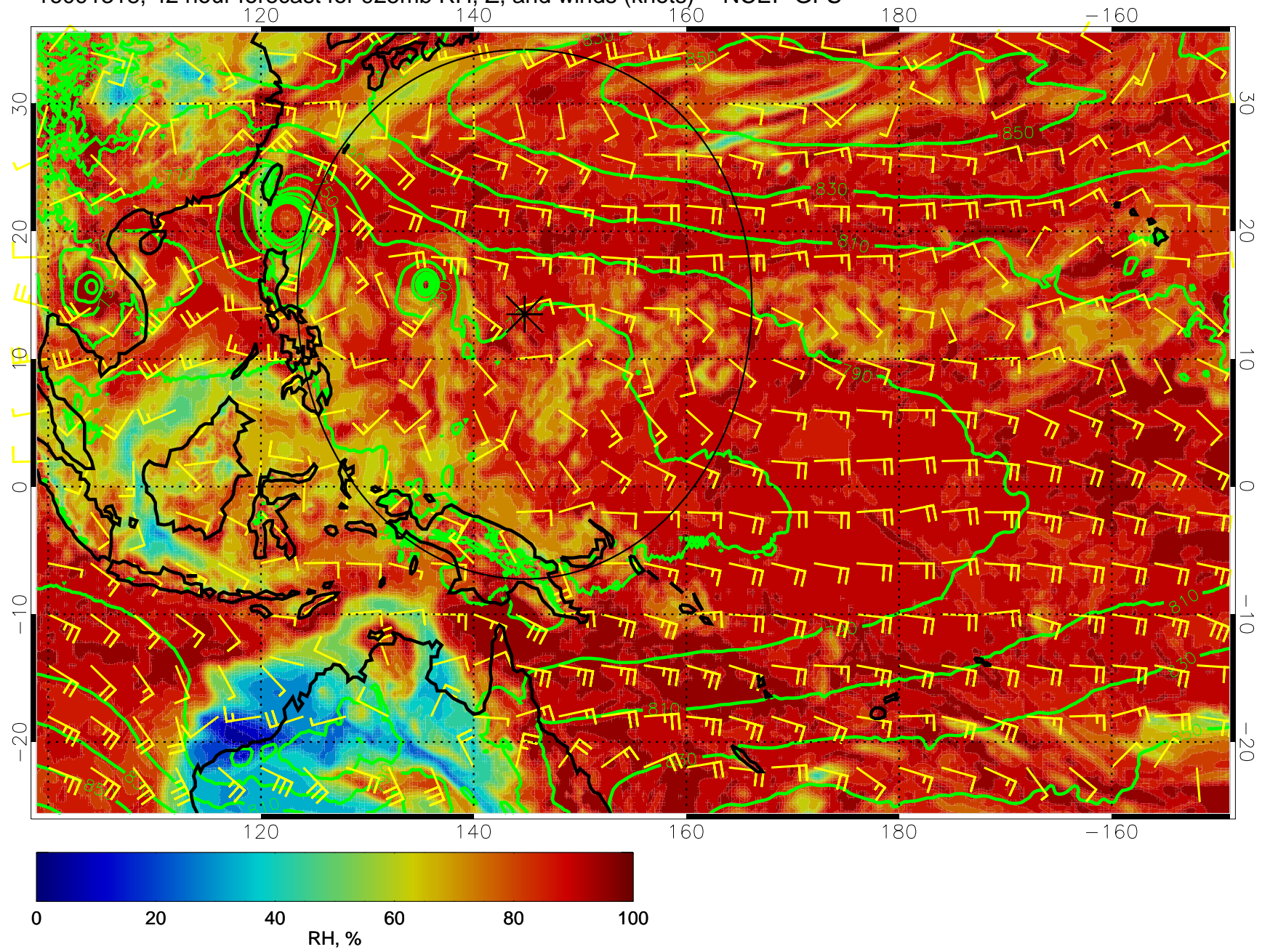
16091318, 42 hour forecast for 925mb RH, Z, and winds (knots) -- NCEP GFS
