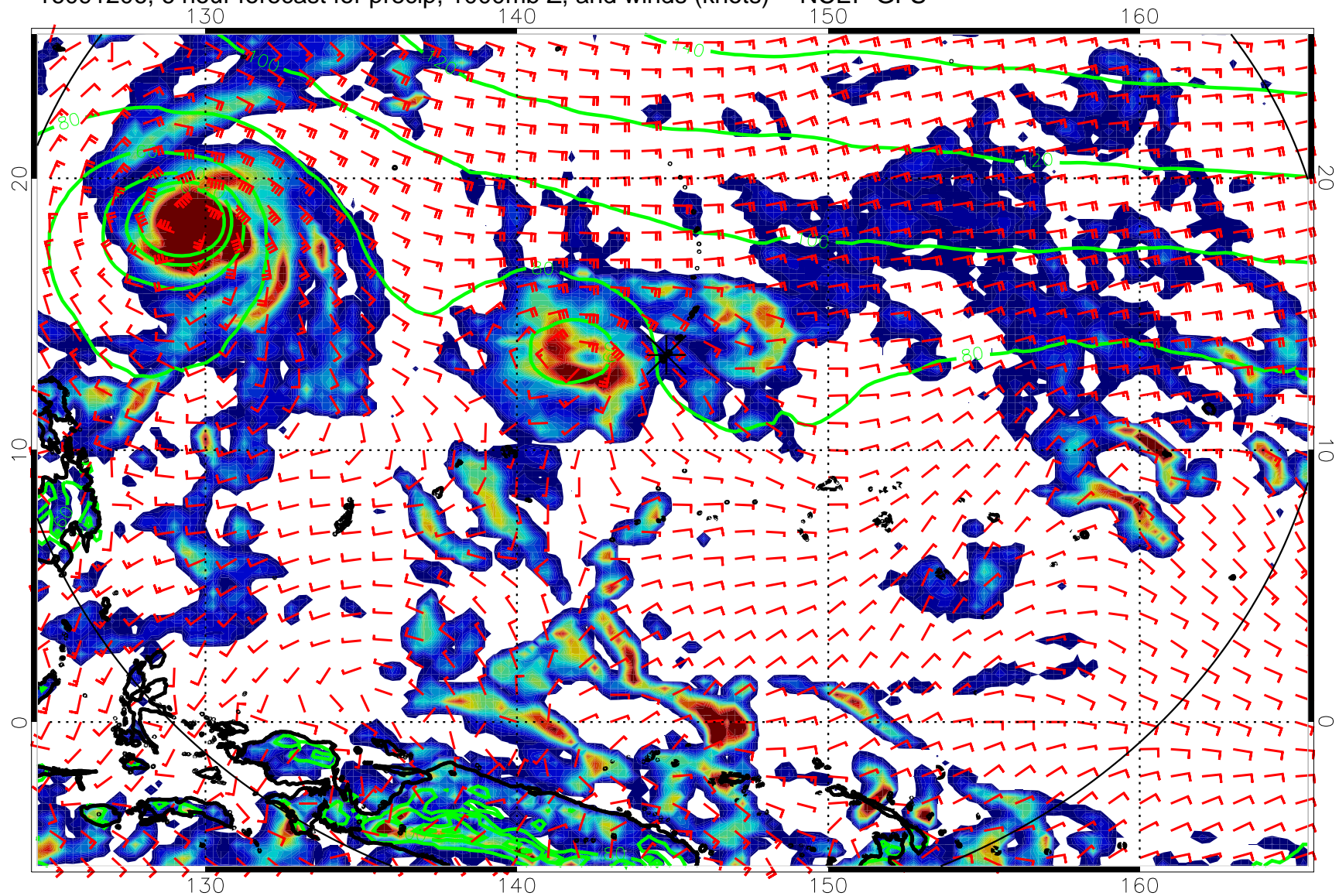
16091206, 6 hour forecast for precip, 1000mb Z, and winds (knots) -- NCEP GFS
