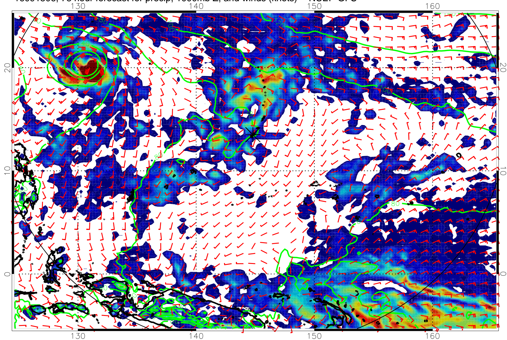
16091506, 78 hour forecast for precip, 1000mb Z, and winds (knots) -- NCEP GFS
