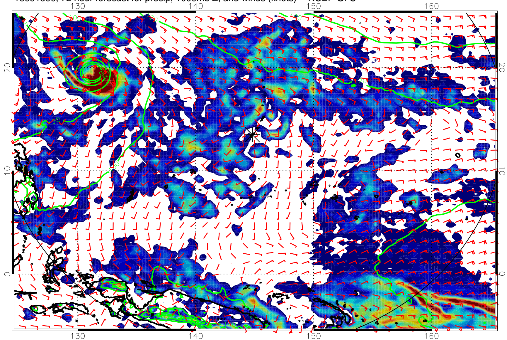
16091500, 72 hour forecast for precip, 1000mb Z, and winds (knots) -- NCEP GFS
