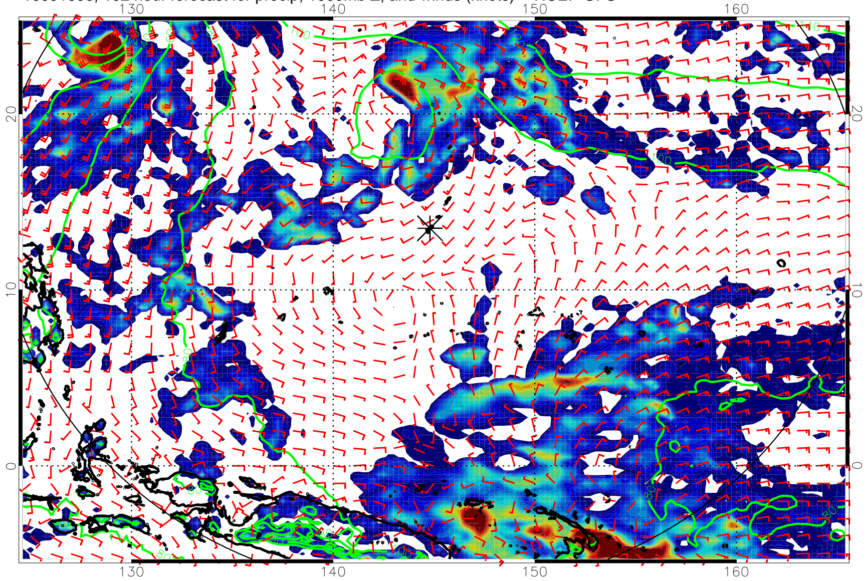
16091606, 102 hour forecast for precip, 1000mb Z, and winds (knots) -- NCEP GFS
