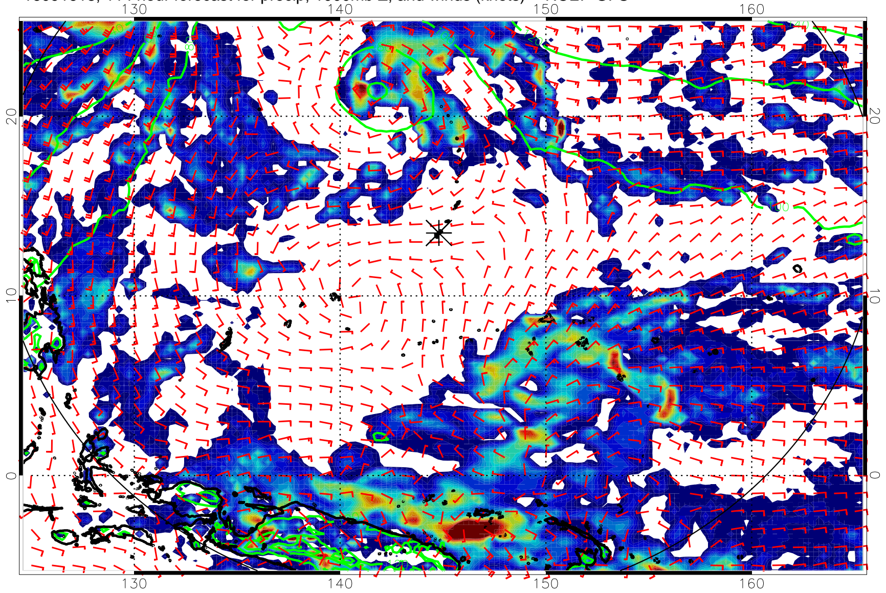
16091618, 114 hour forecast for precip, 1000mb Z, and winds (knots) -- NCEP GFS
