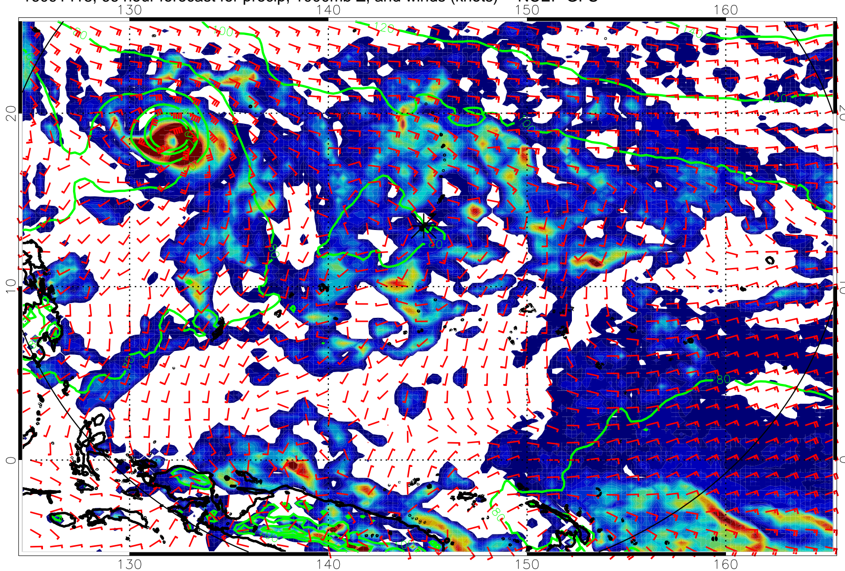
16091418, 66 hour forecast for precip, 1000mb Z, and winds (knots) -- NCEP GFS
