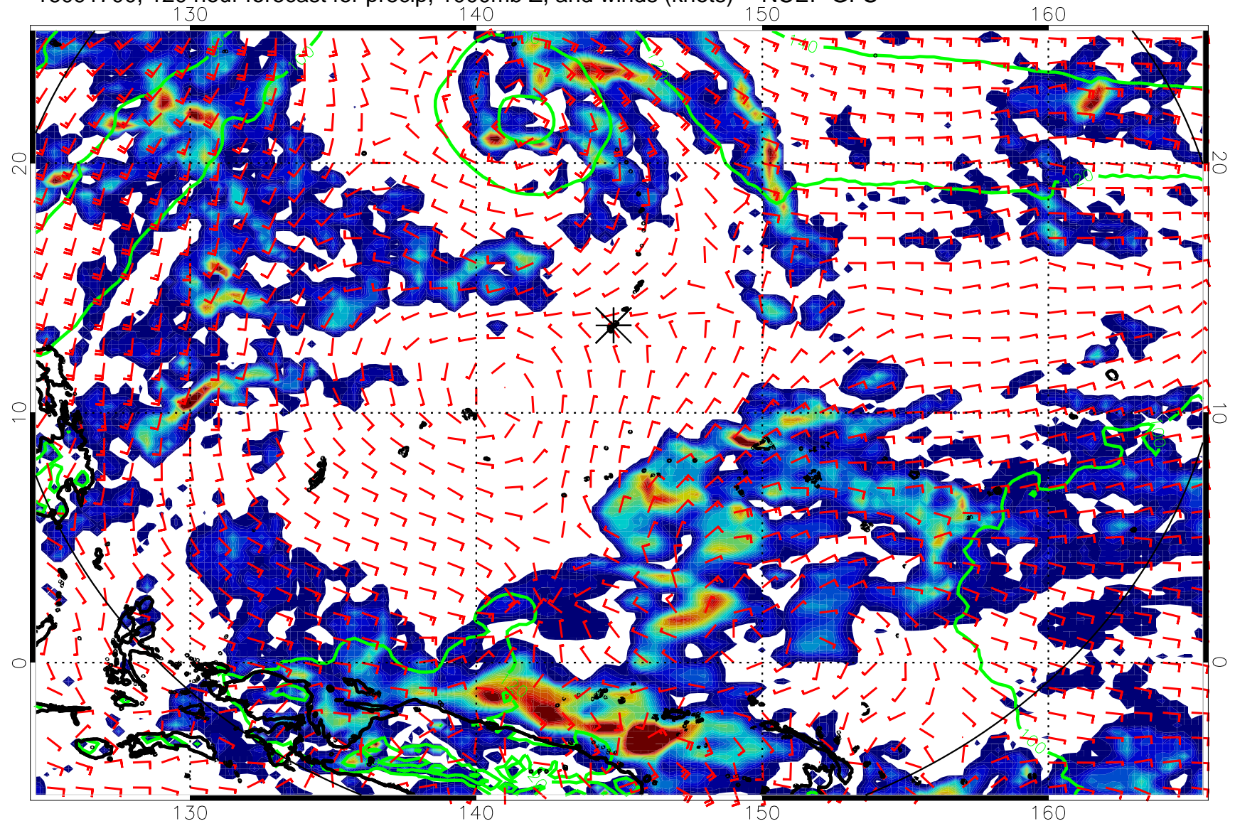
16091700, 120 hour forecast for precip, 1000mb Z, and winds (knots) -- NCEP GFS
