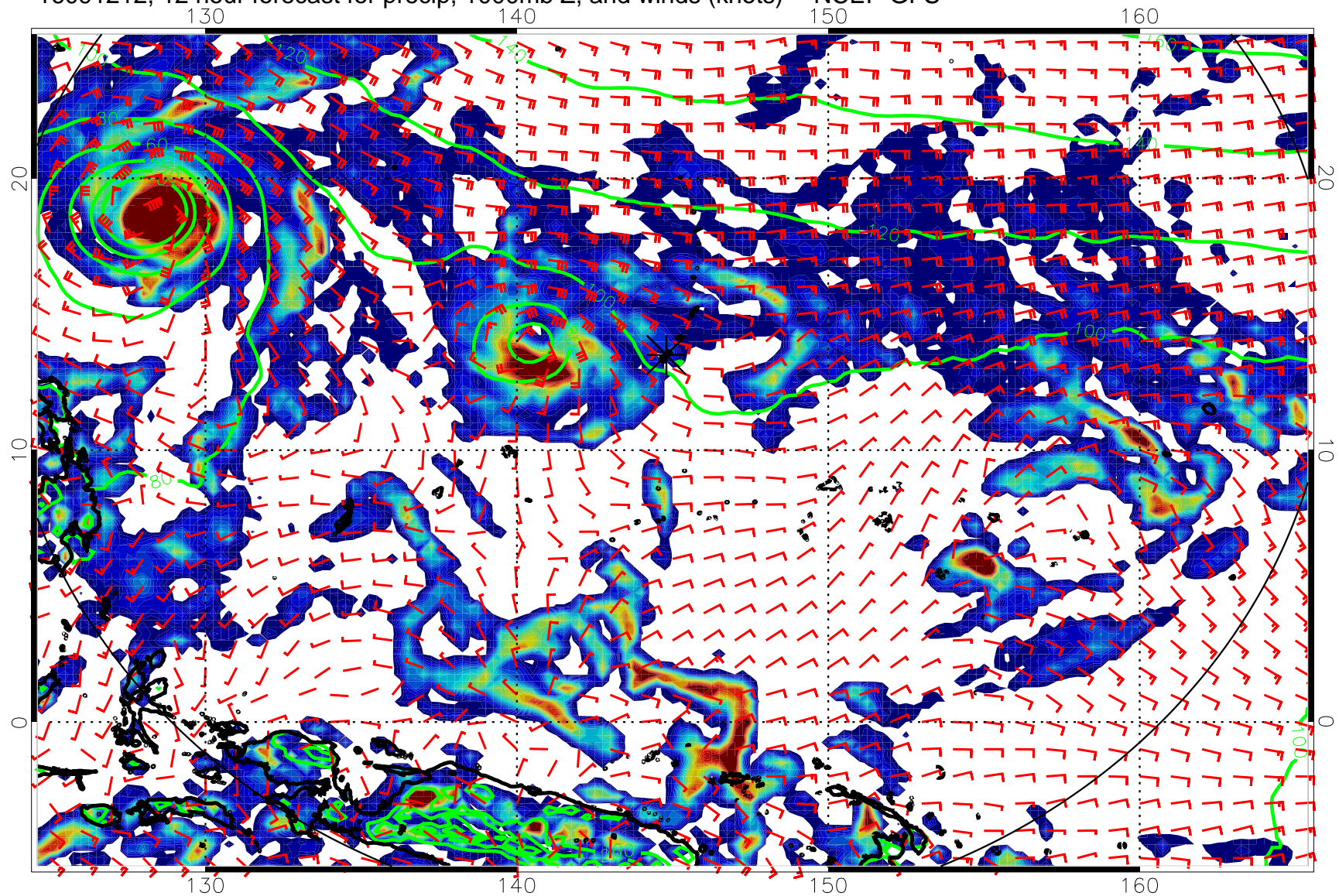
16091212, 12 hour forecast for precip, 1000mb Z, and winds (knots) -- NCEP GFS
