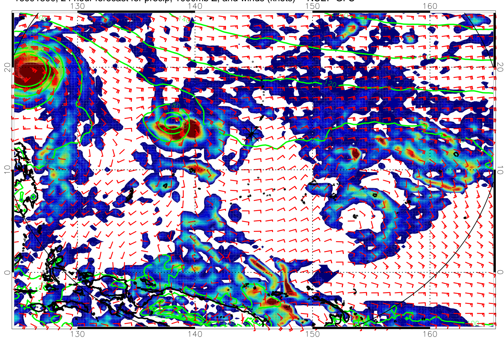
16091300, 24 hour forecast for precip, 1000mb Z, and winds (knots) -- NCEP GFS
