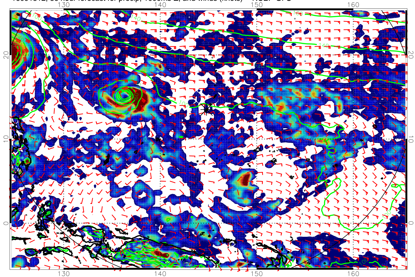
16091312, 36 hour forecast for precip, 1000mb Z, and winds (knots) -- NCEP GFS
