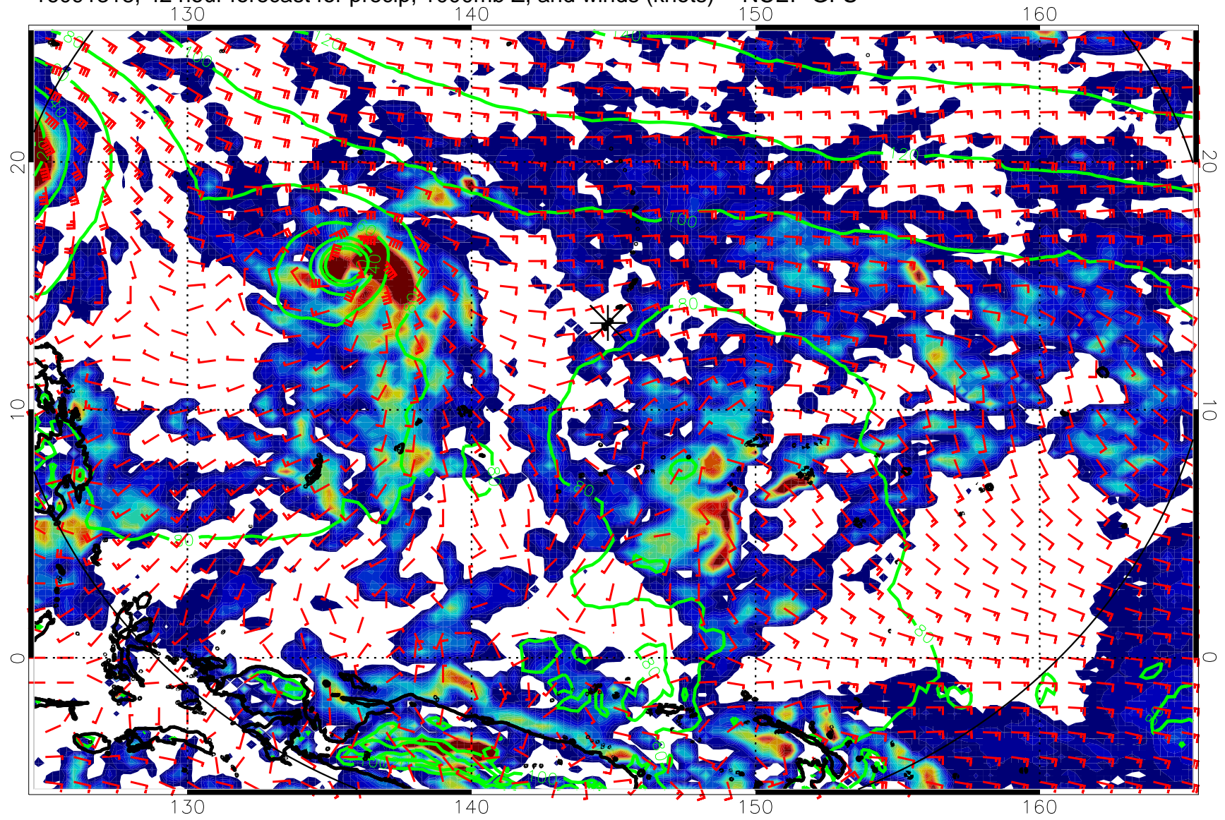
16091318, 42 hour forecast for precip, 1000mb Z, and winds (knots) -- NCEP GFS
