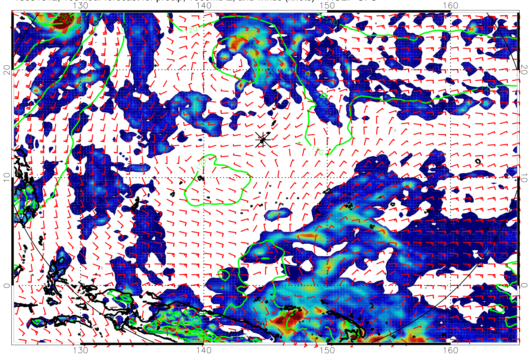
16091612, 108 hour forecast for precip, 1000mb Z, and winds (knots) -- NCEP GFS
