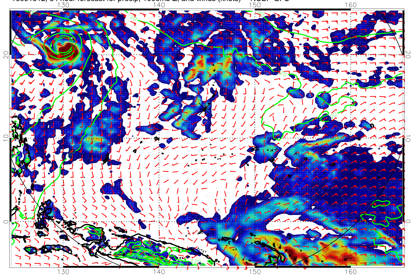
16091512, 84 hour forecast for precip, 1000mb Z, and winds (knots) -- NCEP GFS
