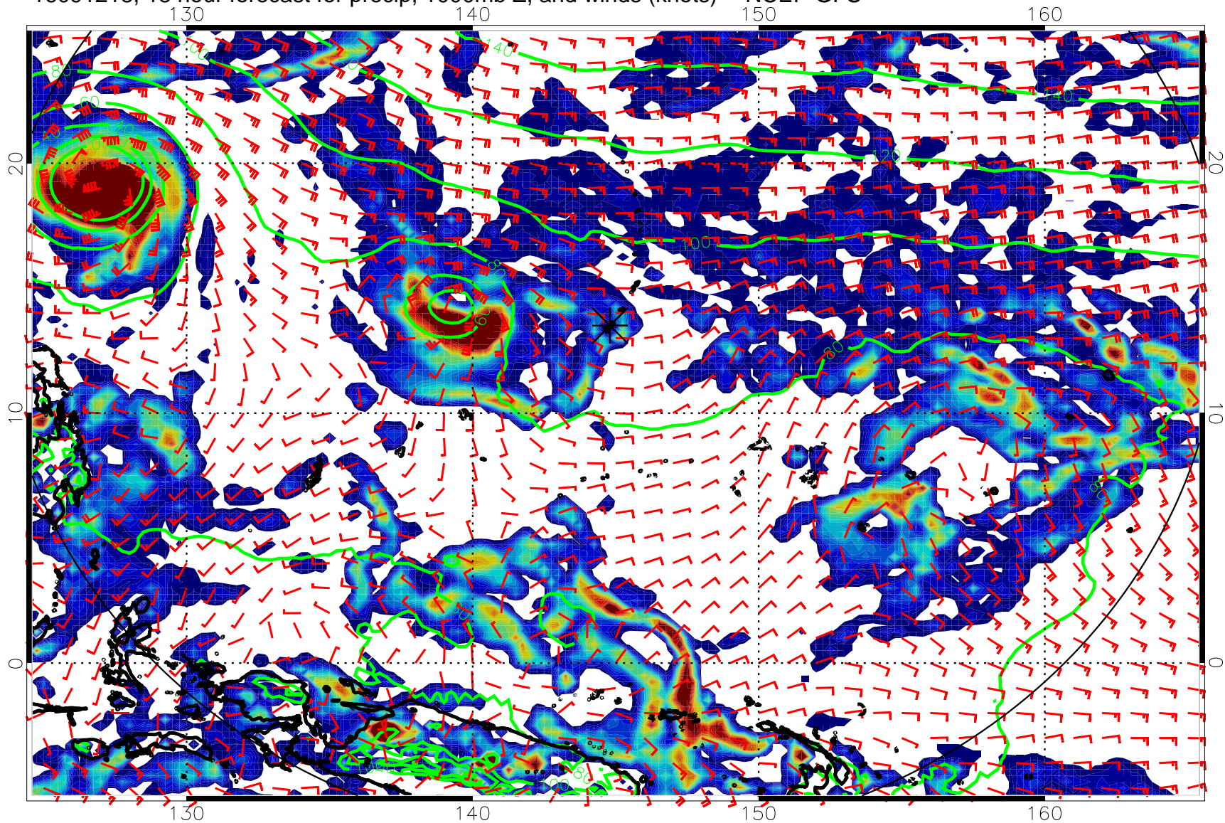
16091218, 18 hour forecast for precip, 1000mb Z, and winds (knots) -- NCEP GFS
