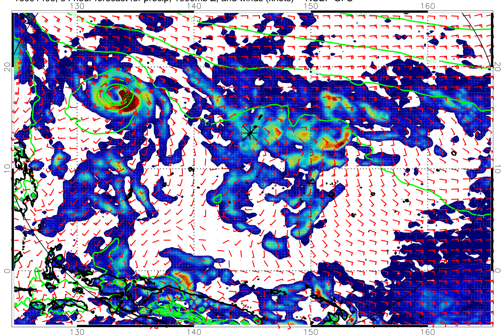
16091406, 54 hour forecast for precip, 1000mb Z, and winds (knots) -- NCEP GFS
