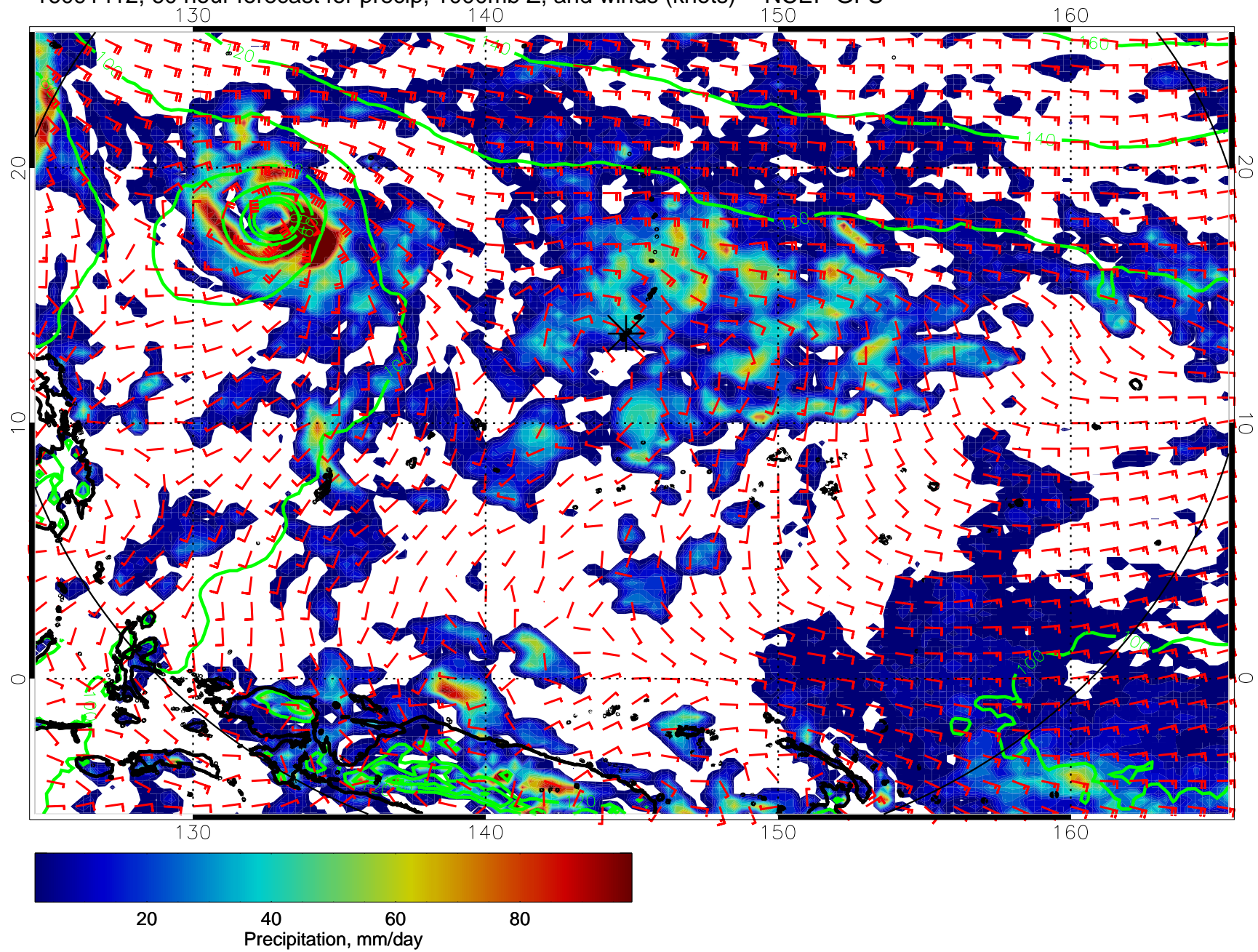
16091412, 60 hour forecast for precip, 1000mb Z, and winds (knots) -- NCEP GFS
