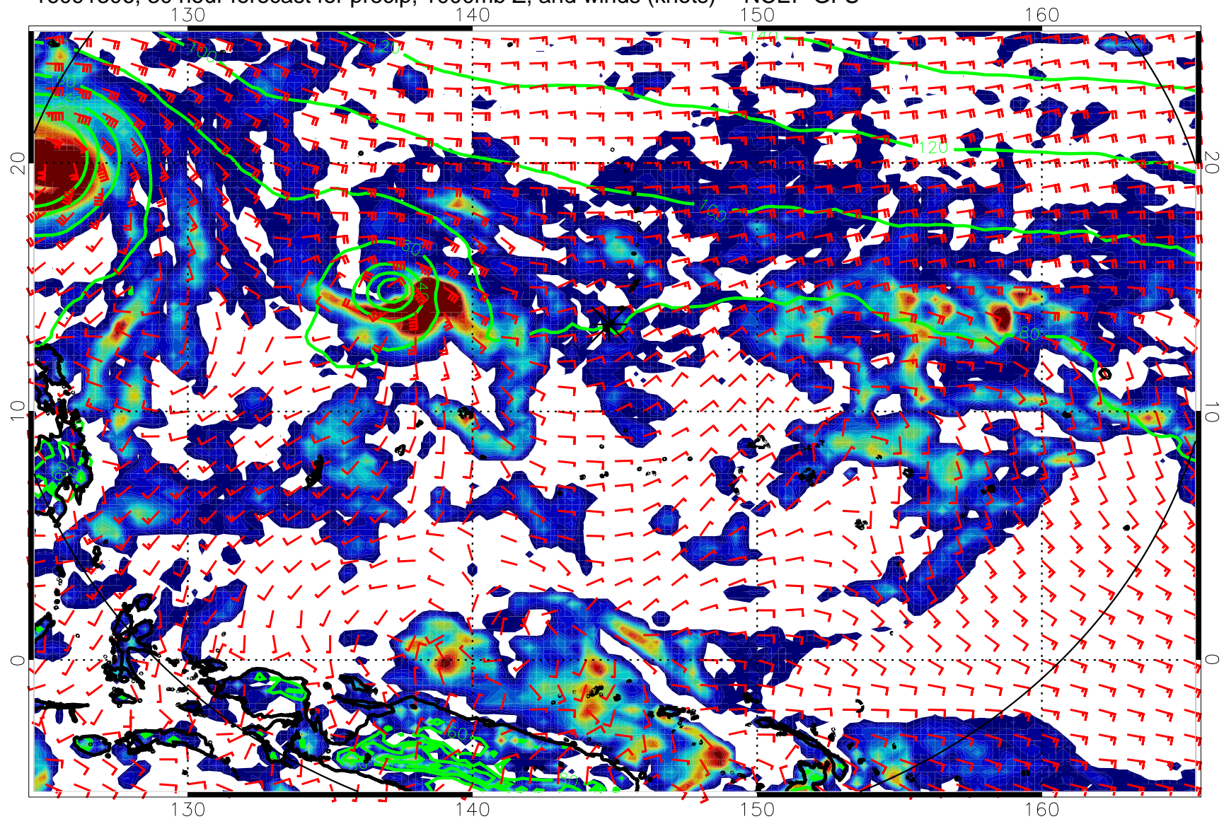
16091306, 30 hour forecast for precip, 1000mb Z, and winds (knots) -- NCEP GFS
