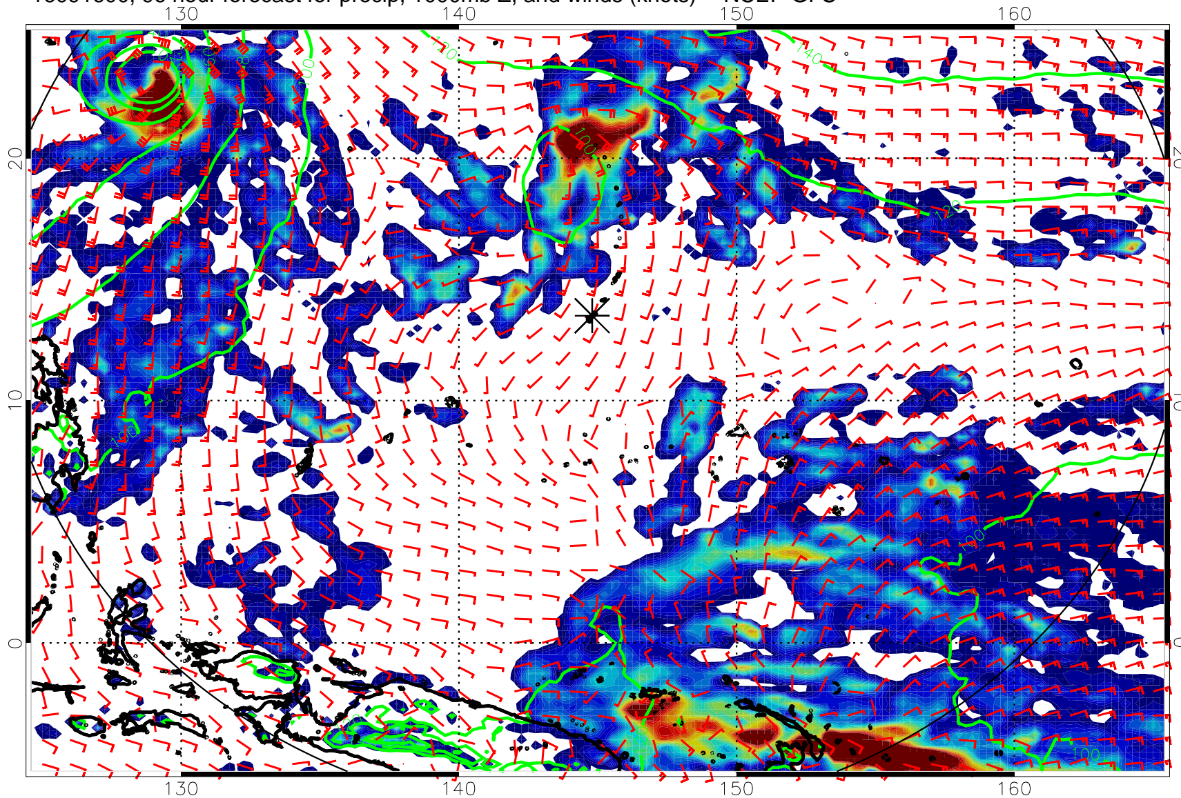
16091600, 96 hour forecast for precip, 1000mb Z, and winds (knots) -- NCEP GFS
