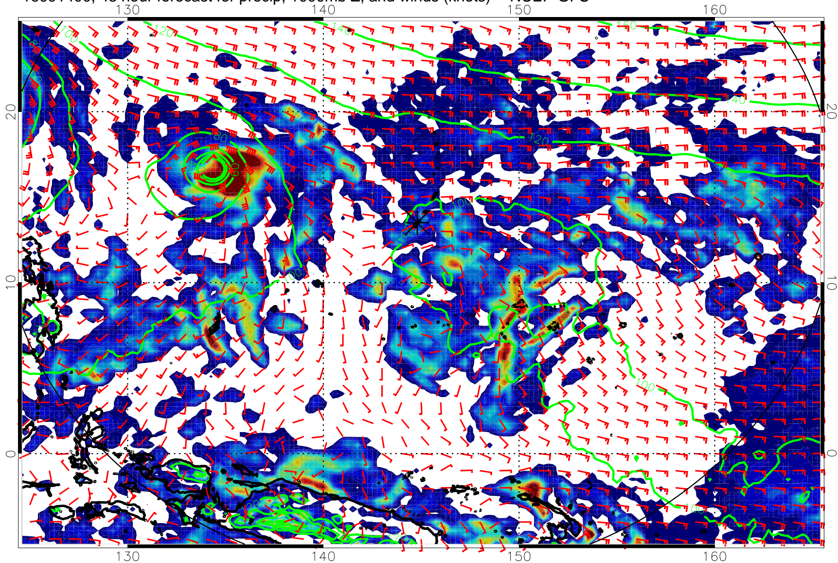
16091400, 48 hour forecast for precip, 1000mb Z, and winds (knots) -- NCEP GFS
