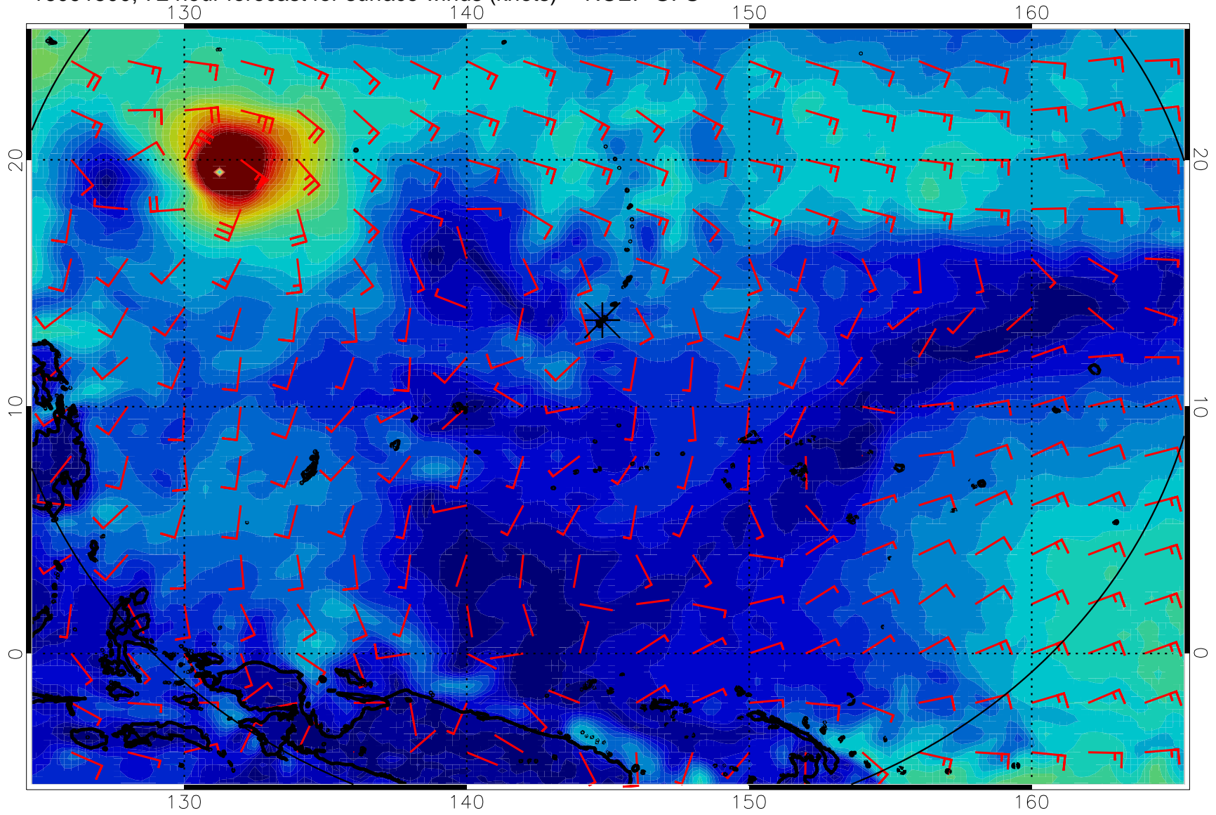
16091500, 72 hour forecast for surface winds (knots) -- NCEP GFS
