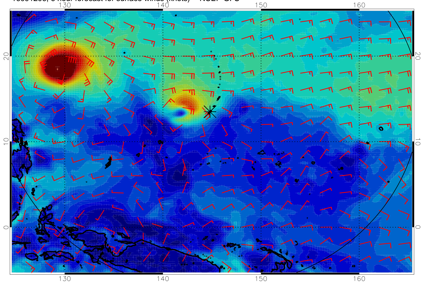
16091206, 6 hour forecast for surface winds (knots) -- NCEP GFS
