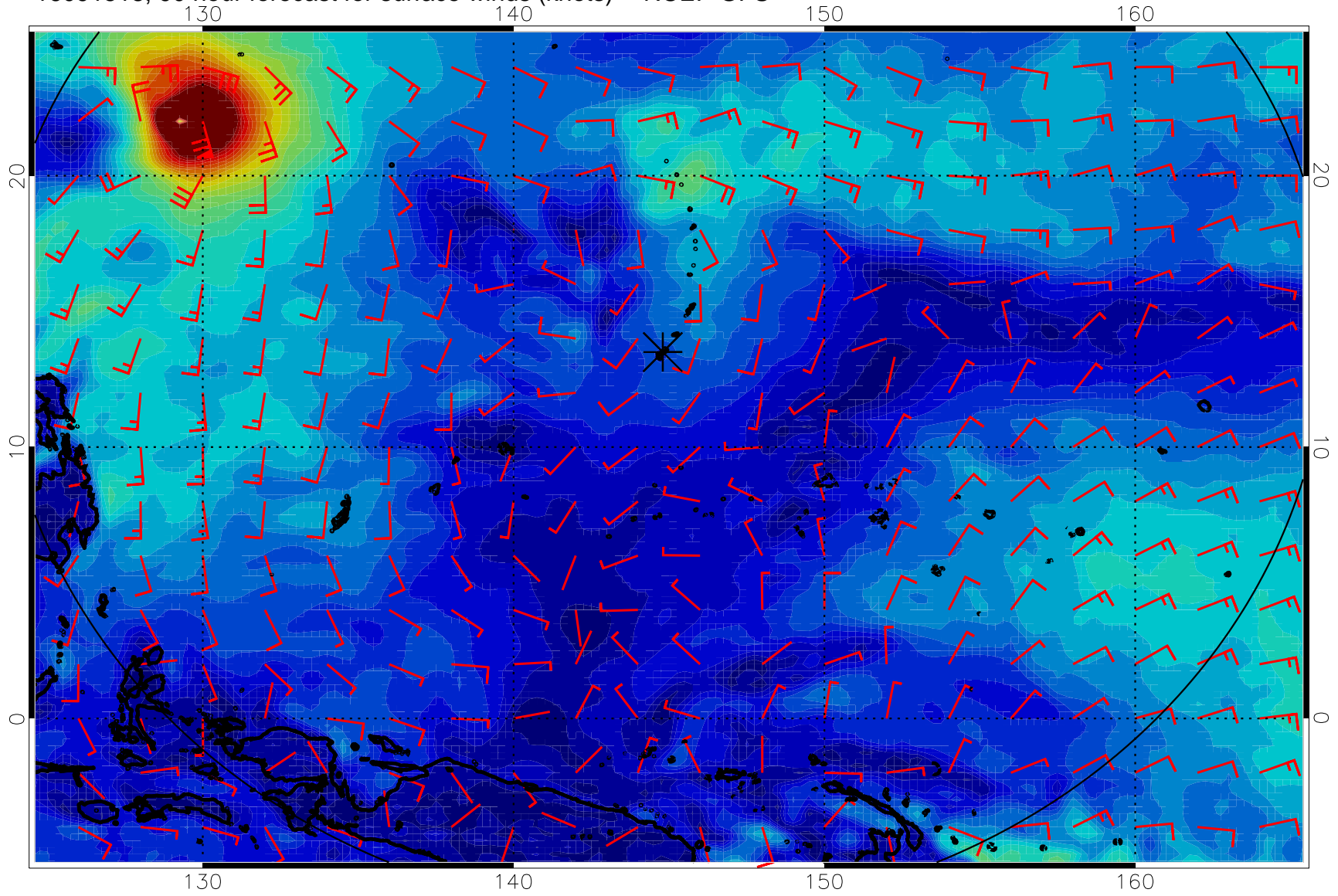
16091518, 90 hour forecast for surface winds (knots) -- NCEP GFS
