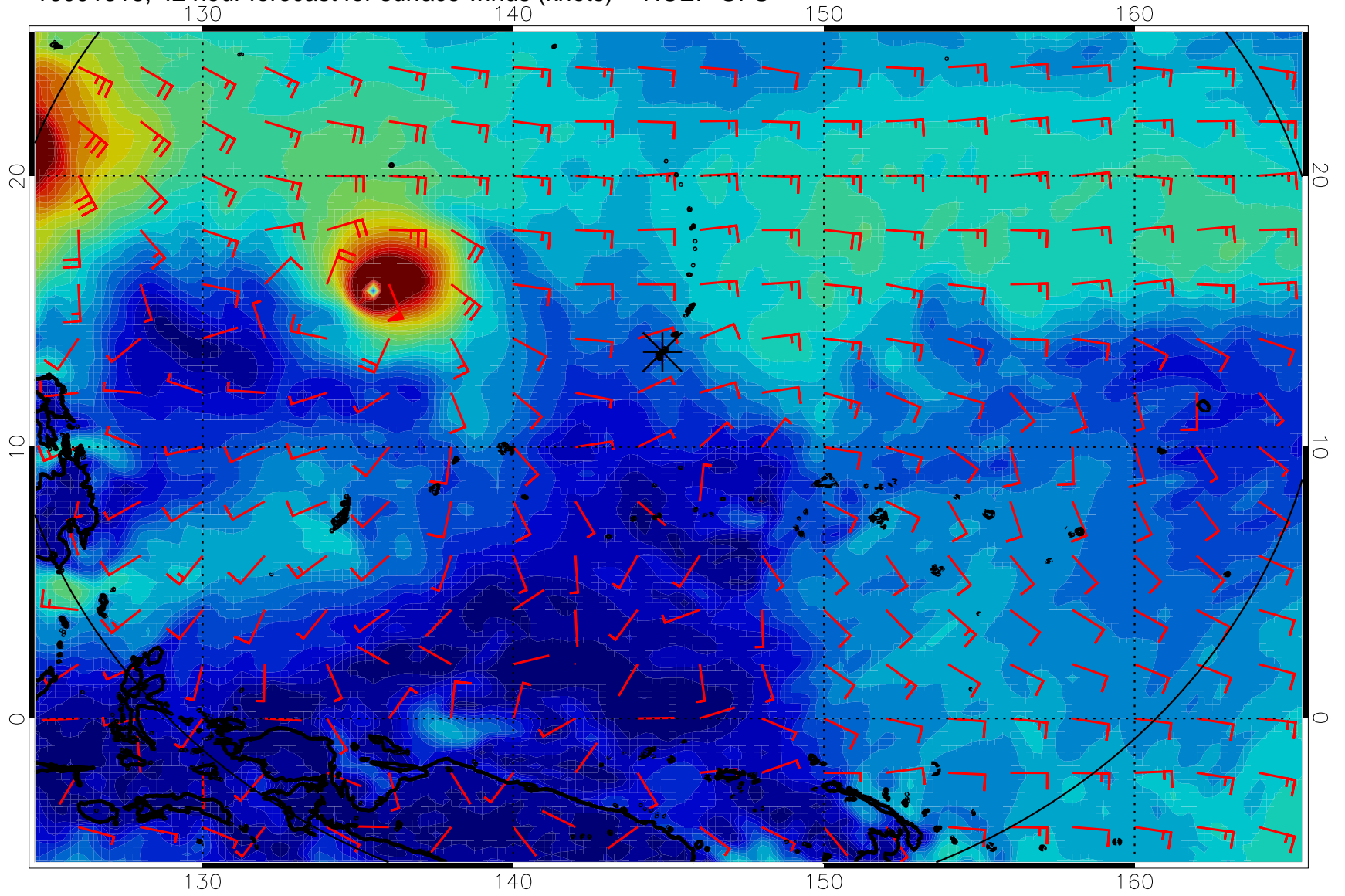
16091318, 42 hour forecast for surface winds (knots) -- NCEP GFS
