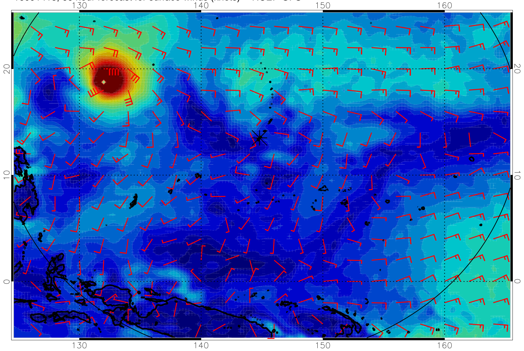
16091418, 66 hour forecast for surface winds (knots) -- NCEP GFS
