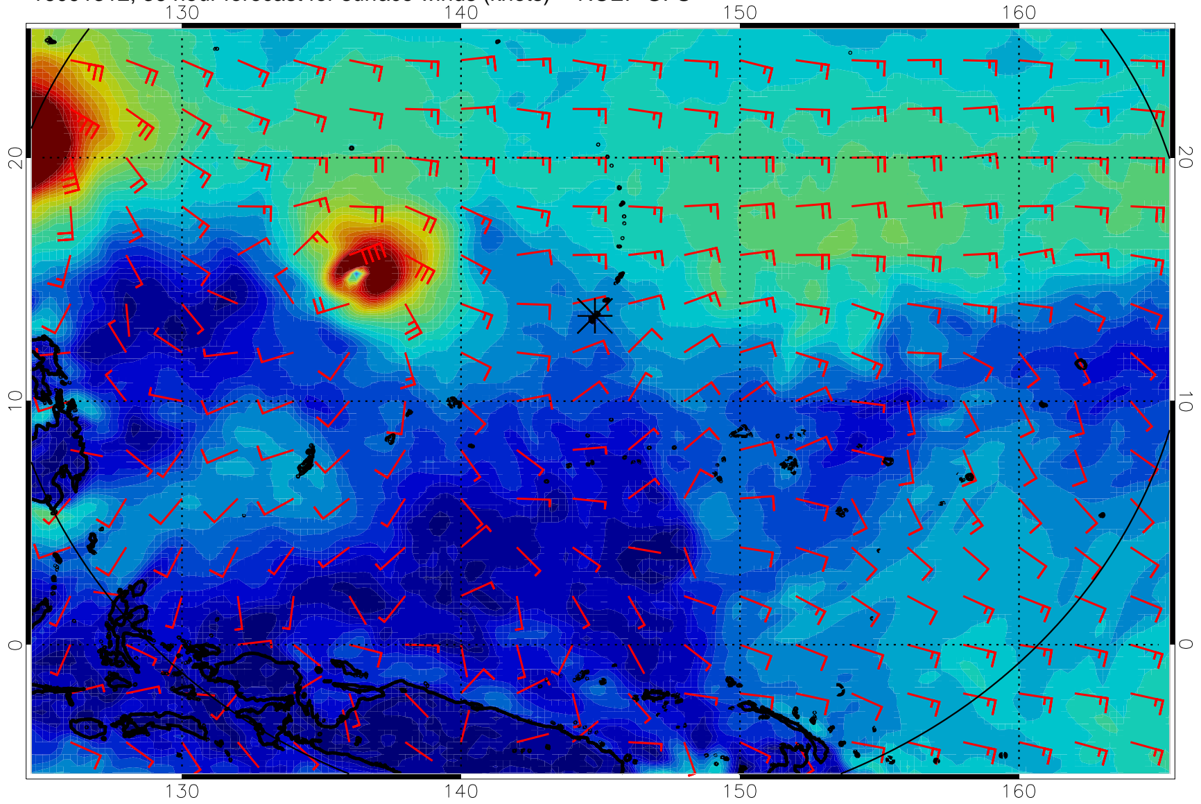
16091312, 36 hour forecast for surface winds (knots) -- NCEP GFS
