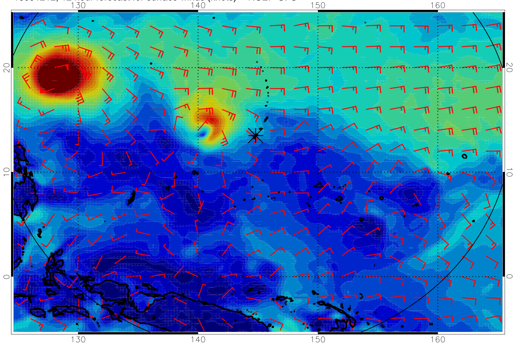
16091212, 12 hour forecast for surface winds (knots) -- NCEP GFS
