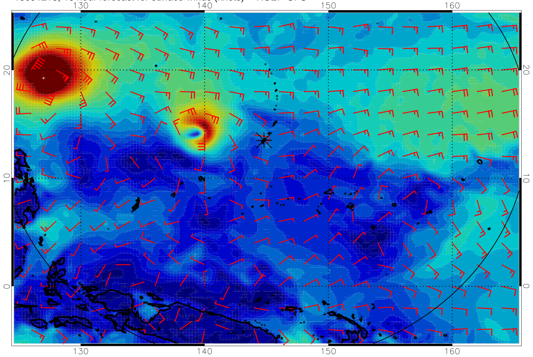
16091218, 18 hour forecast for surface winds (knots) -- NCEP GFS
