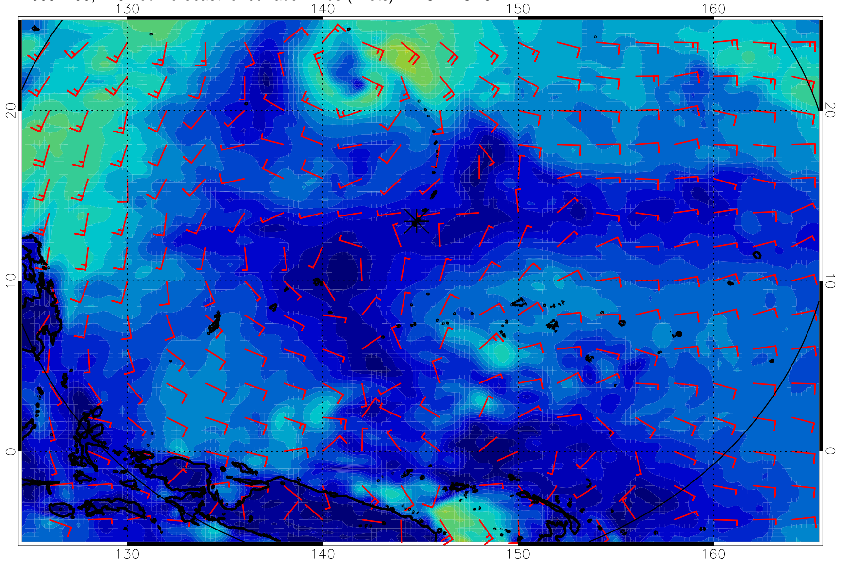
16091700, 120 hour forecast for surface winds (knots) -- NCEP GFS
