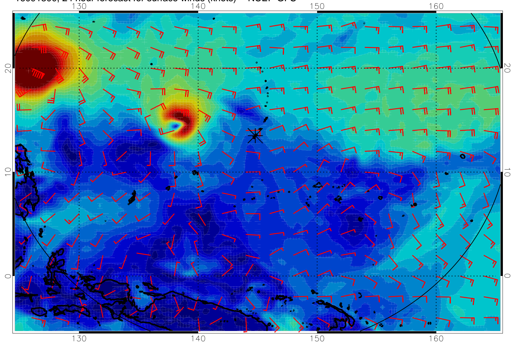
16091300, 24 hour forecast for surface winds (knots) -- NCEP GFS
