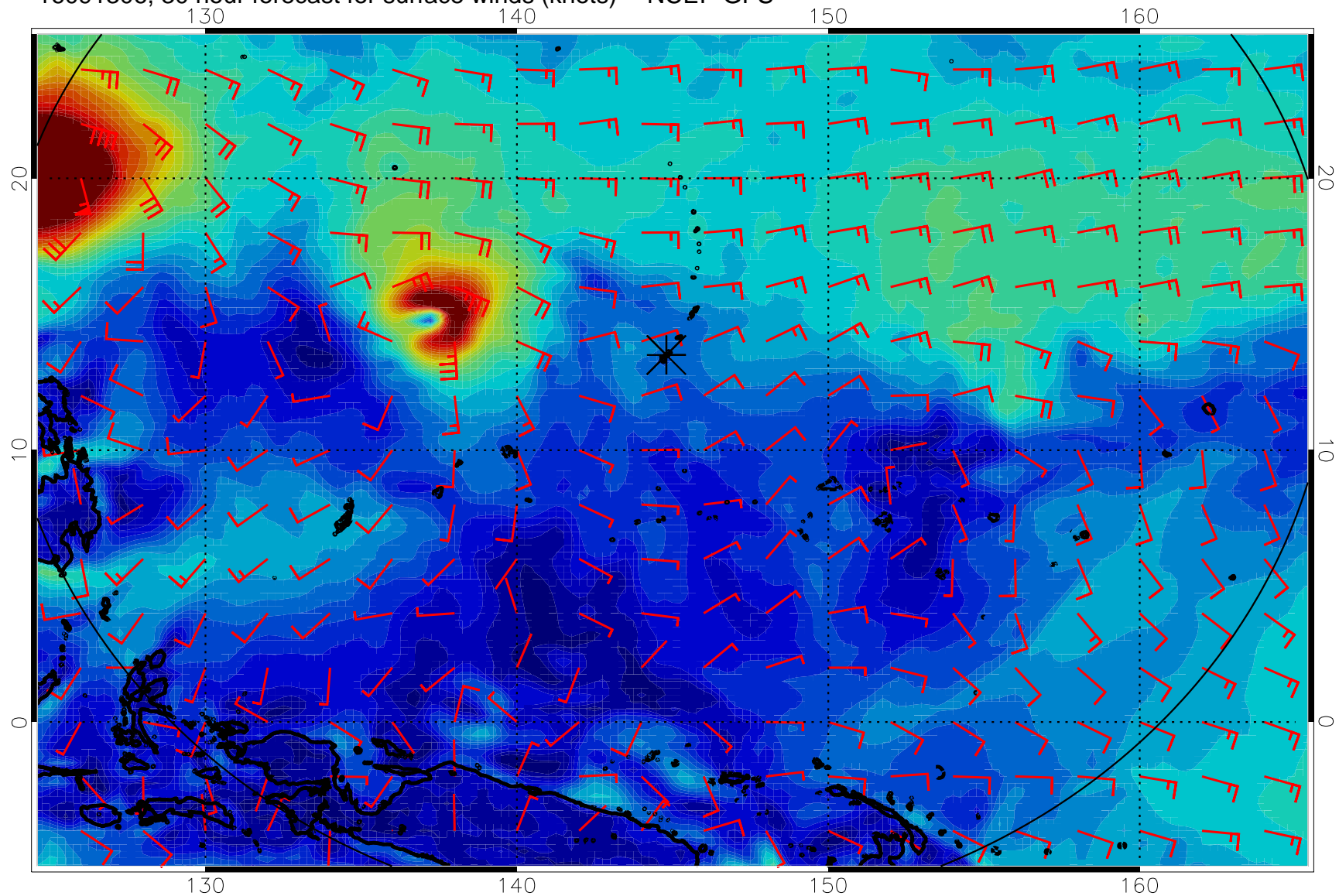
16091306, 30 hour forecast for surface winds (knots) -- NCEP GFS
