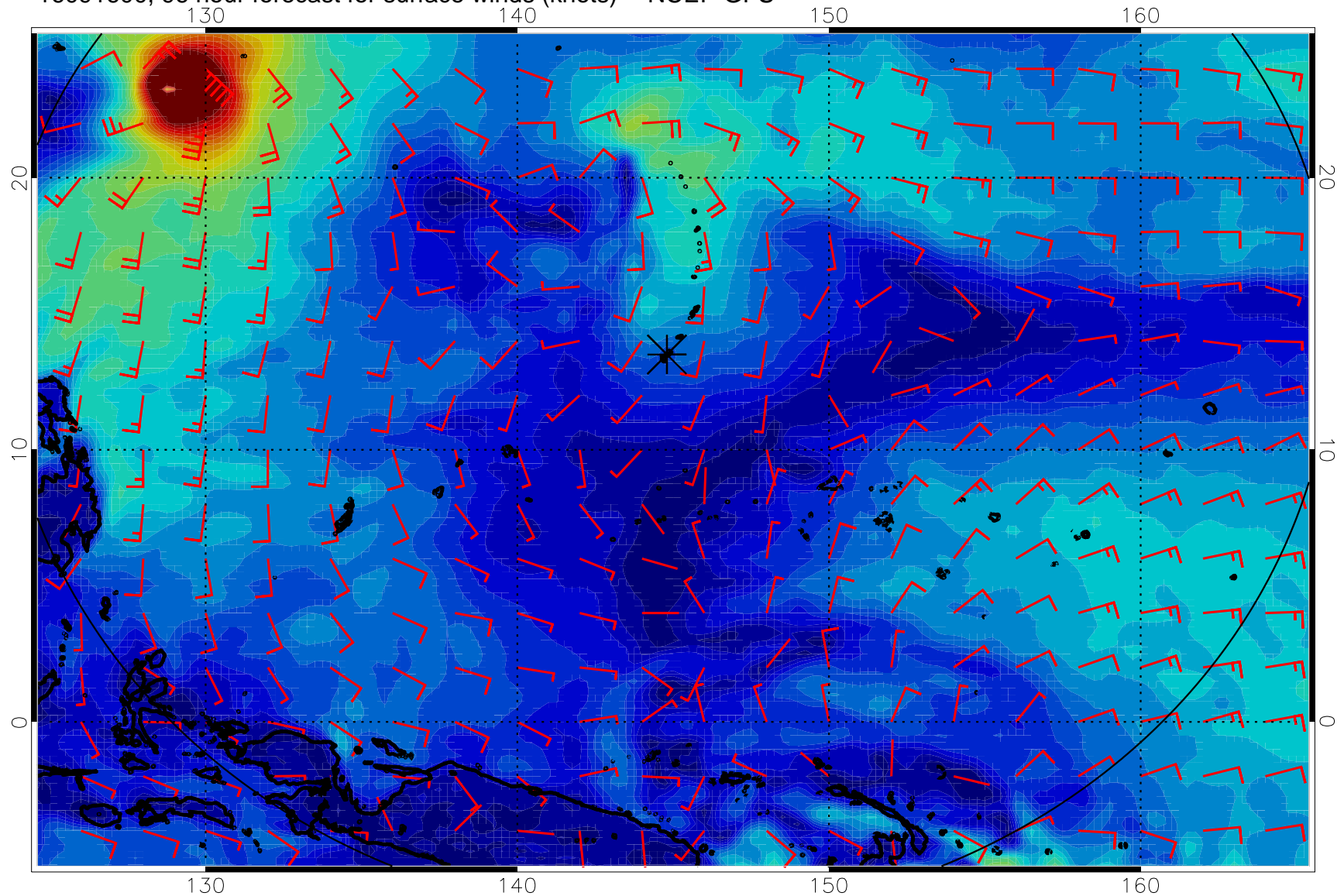
16091600, 96 hour forecast for surface winds (knots) -- NCEP GFS
