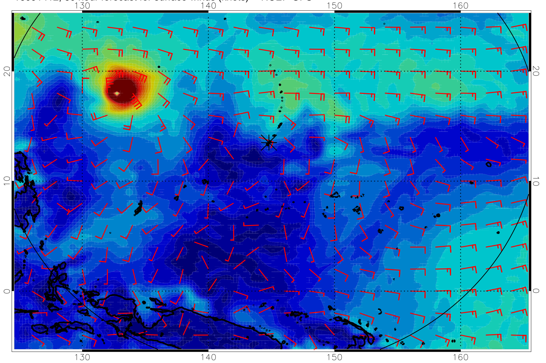
16091412, 60 hour forecast for surface winds (knots) -- NCEP GFS
