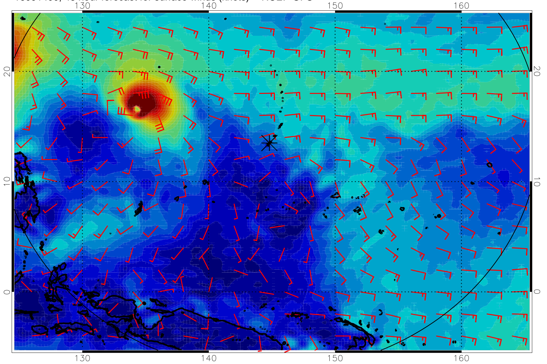
16091400, 48 hour forecast for surface winds (knots) -- NCEP GFS
