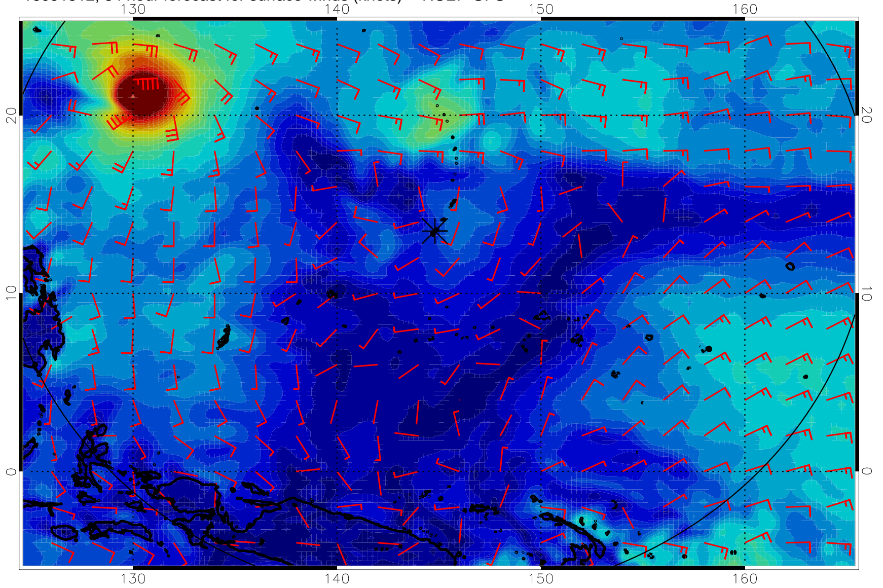
16091512, 84 hour forecast for surface winds (knots) -- NCEP GFS
