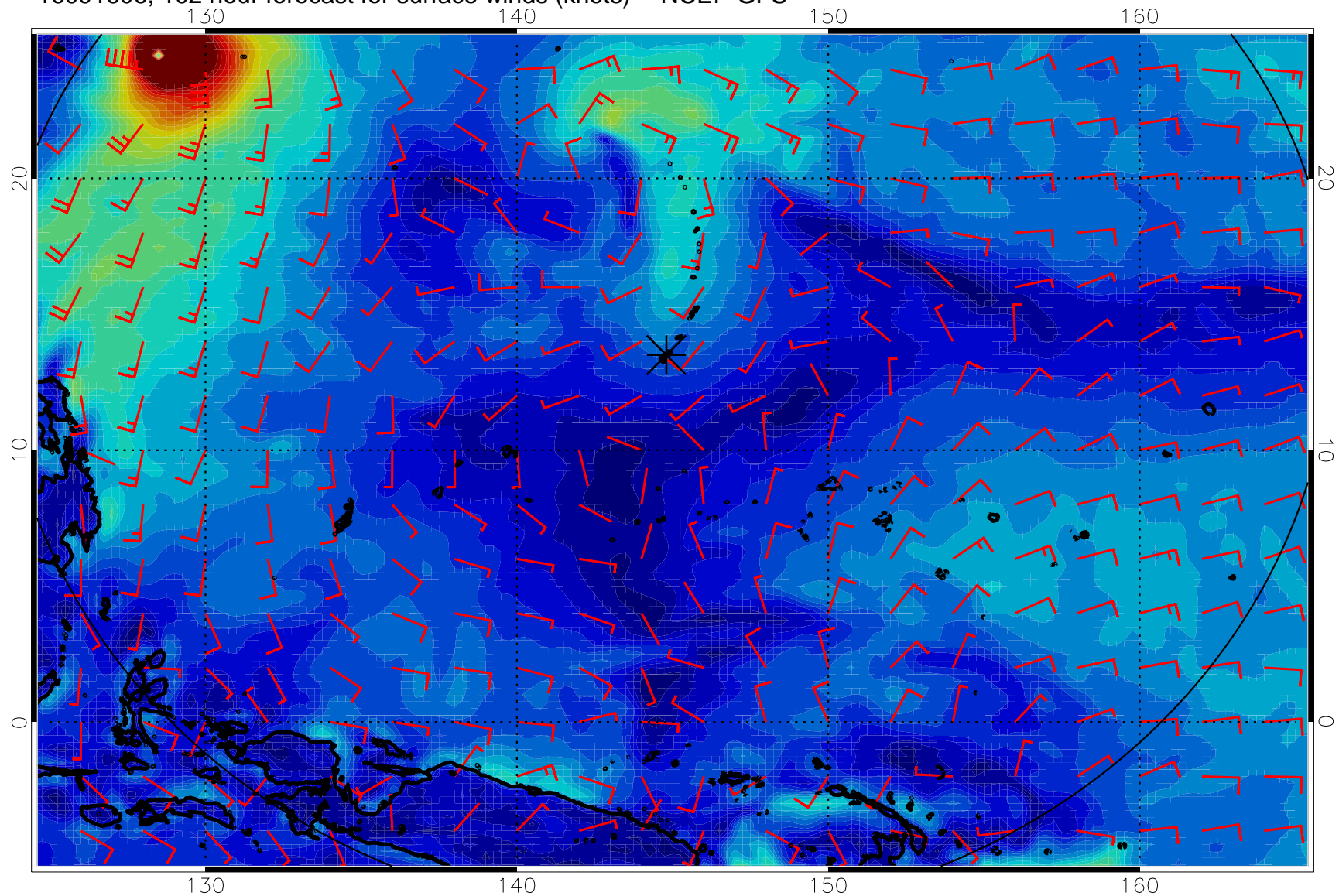
16091606, 102 hour forecast for surface winds (knots) -- NCEP GFS
