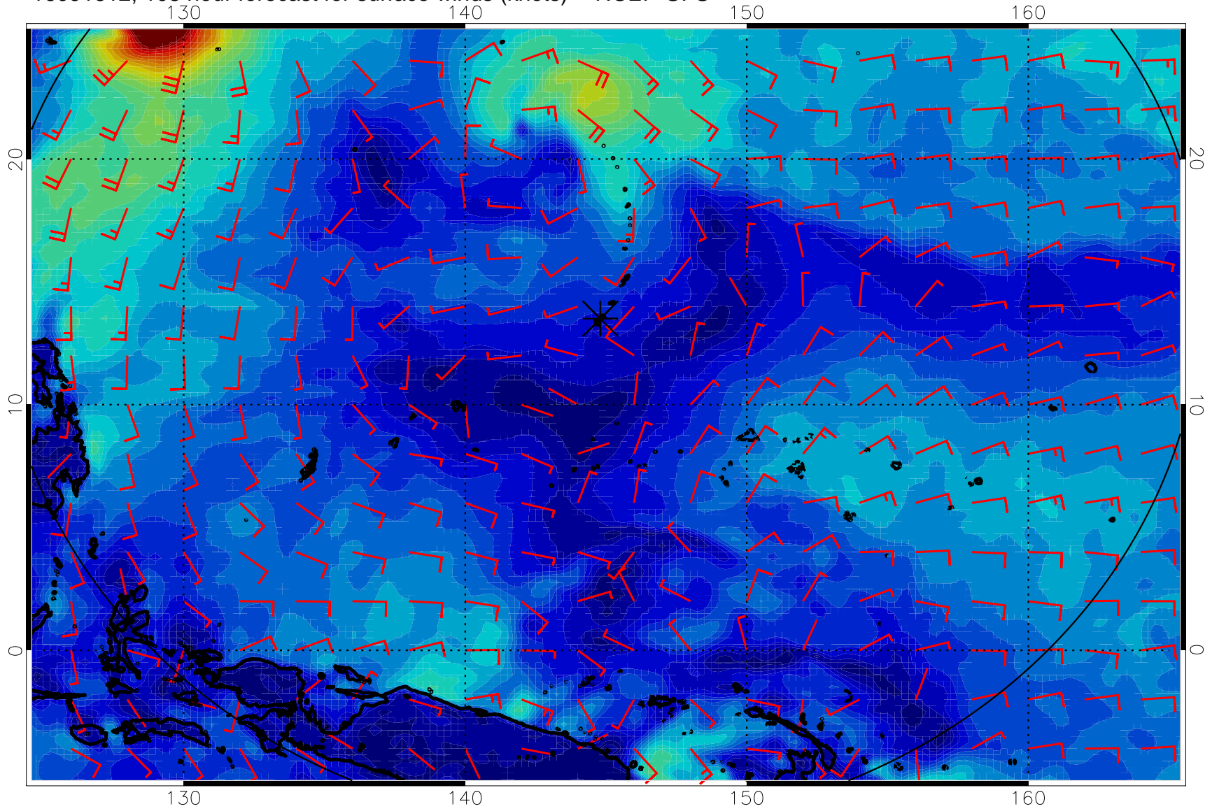
16091612, 108 hour forecast for surface winds (knots) -- NCEP GFS
