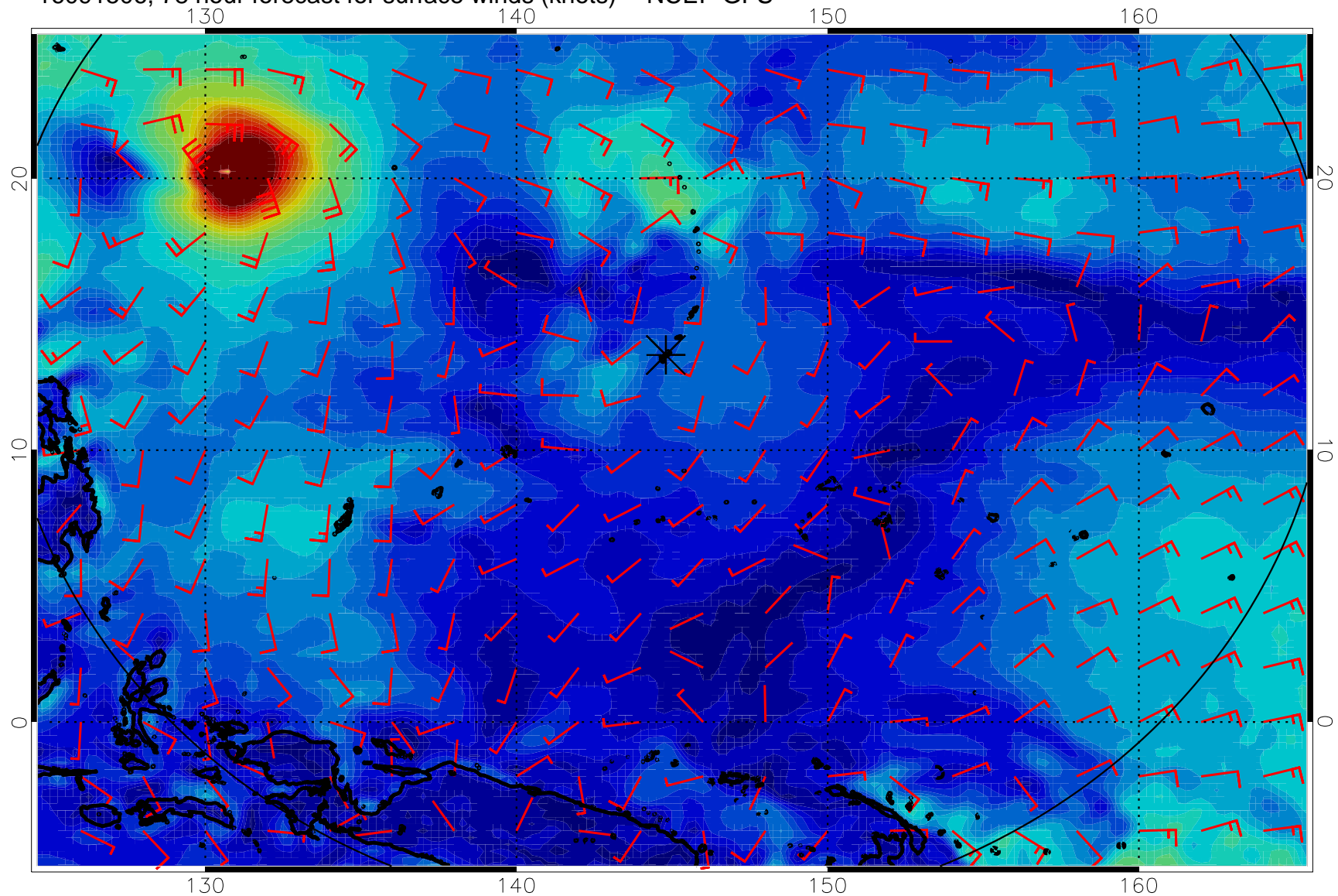
16091506, 78 hour forecast for surface winds (knots) -- NCEP GFS
