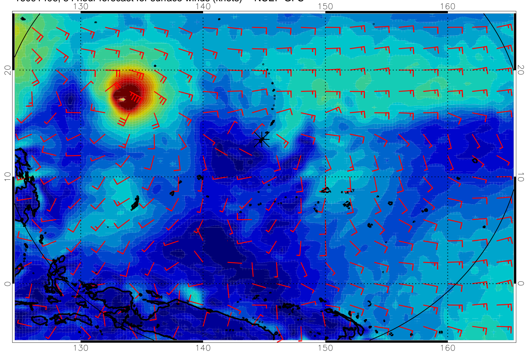
16091406, 54 hour forecast for surface winds (knots) -- NCEP GFS
