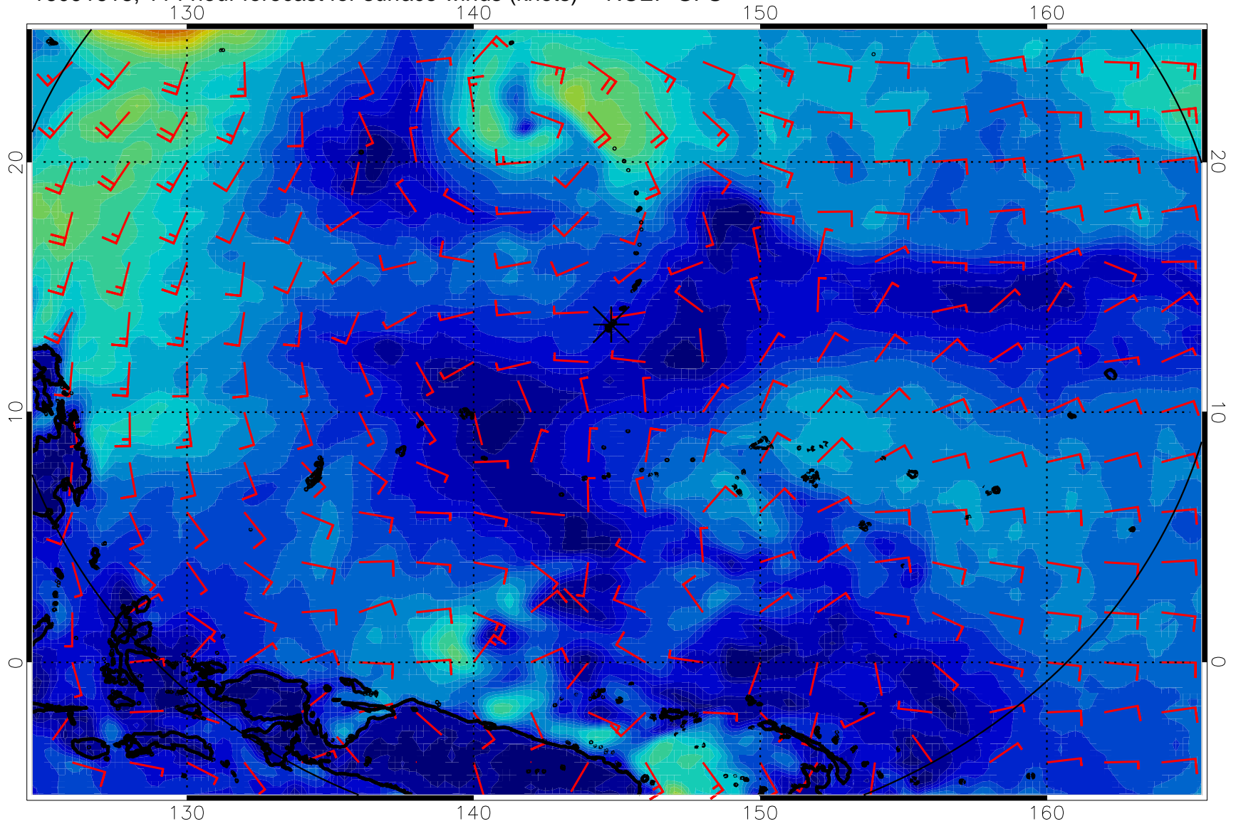
16091618, 114 hour forecast for surface winds (knots) -- NCEP GFS
