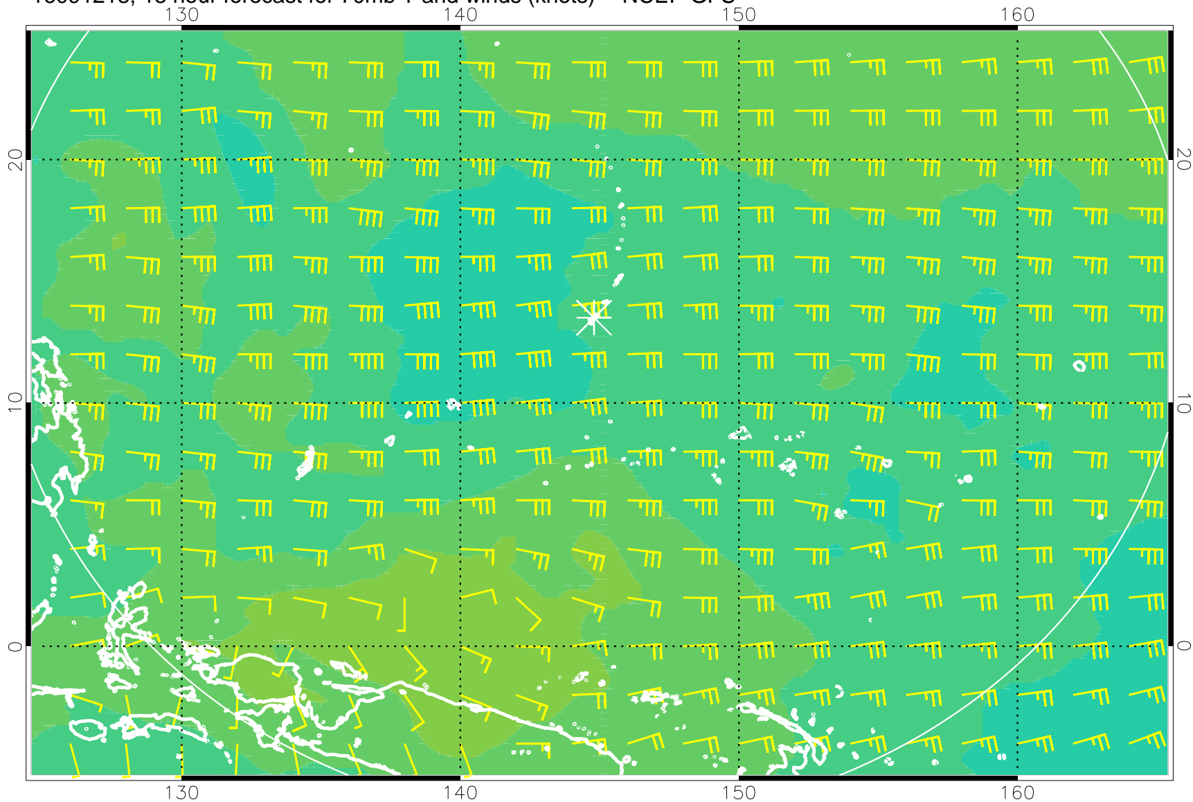
16091218, 18 hour forecast for 70mb T and winds (knots) -- NCEP GFS
