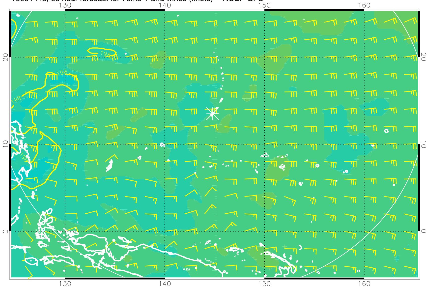
16091418, 66 hour forecast for 70mb T and winds (knots) -- NCEP GFS
