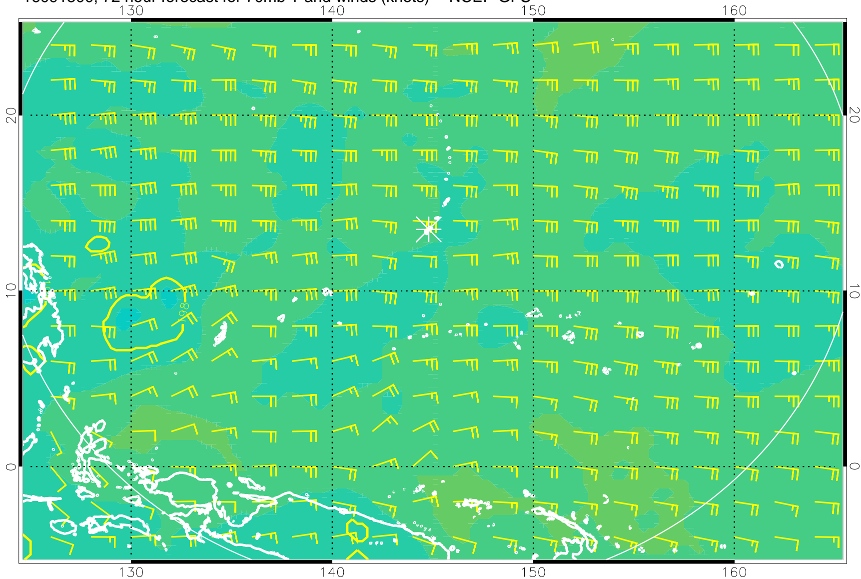
16091500, 72 hour forecast for 70mb T and winds (knots) -- NCEP GFS
