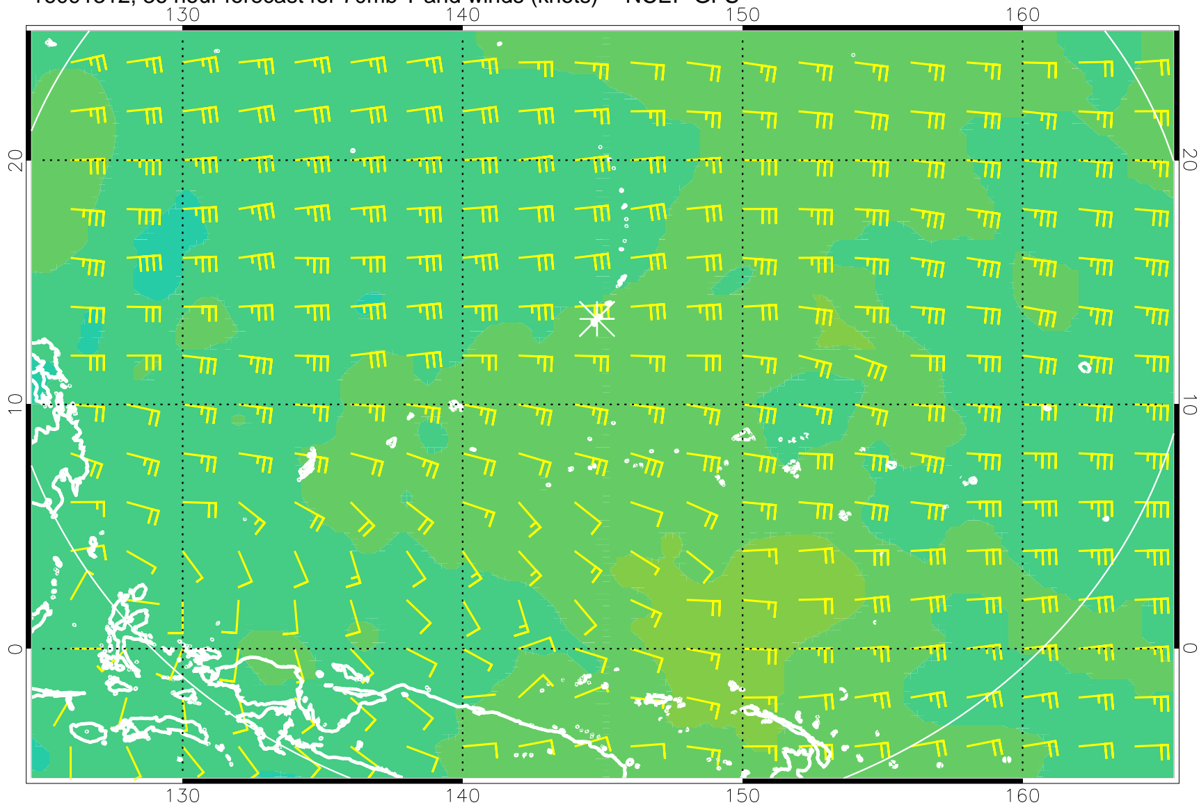
16091312, 36 hour forecast for 70mb T and winds (knots) -- NCEP GFS
