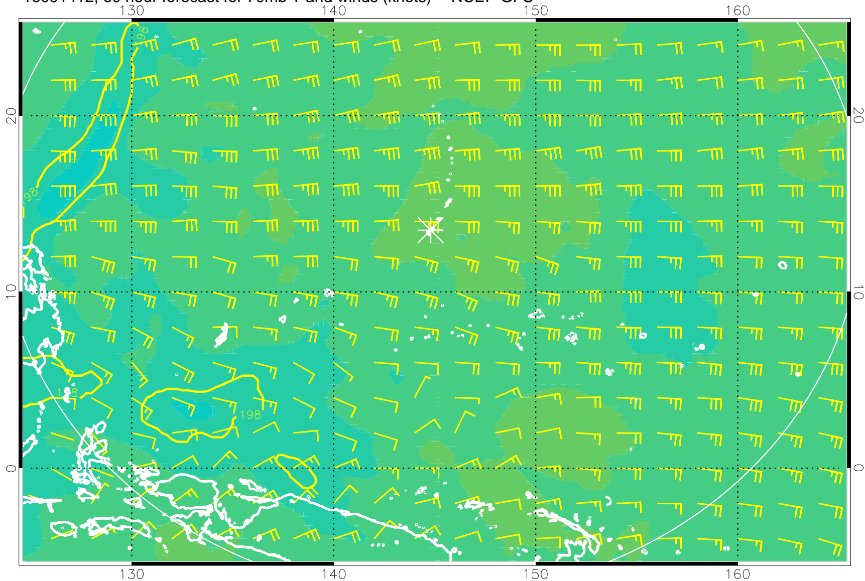
16091412, 60 hour forecast for 70mb T and winds (knots) -- NCEP GFS
