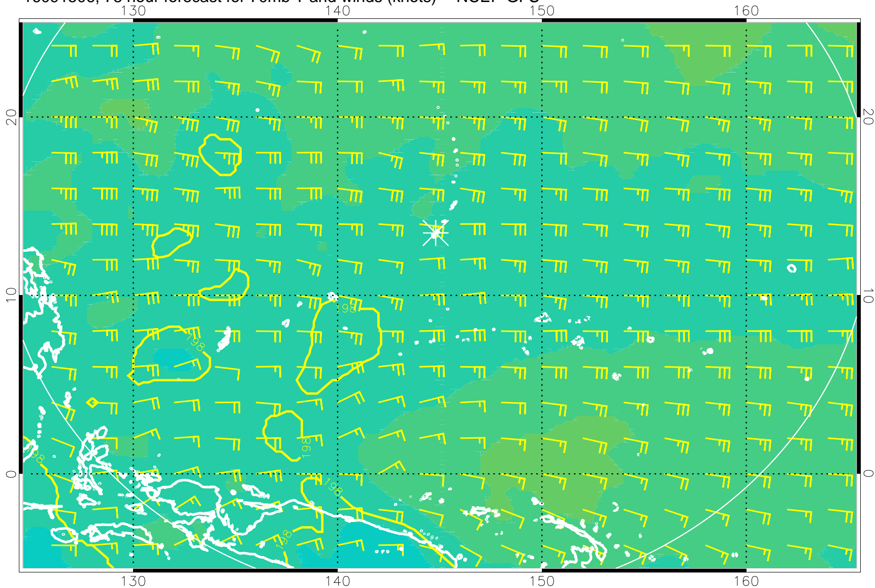
16091506, 78 hour forecast for 70mb T and winds (knots) -- NCEP GFS
