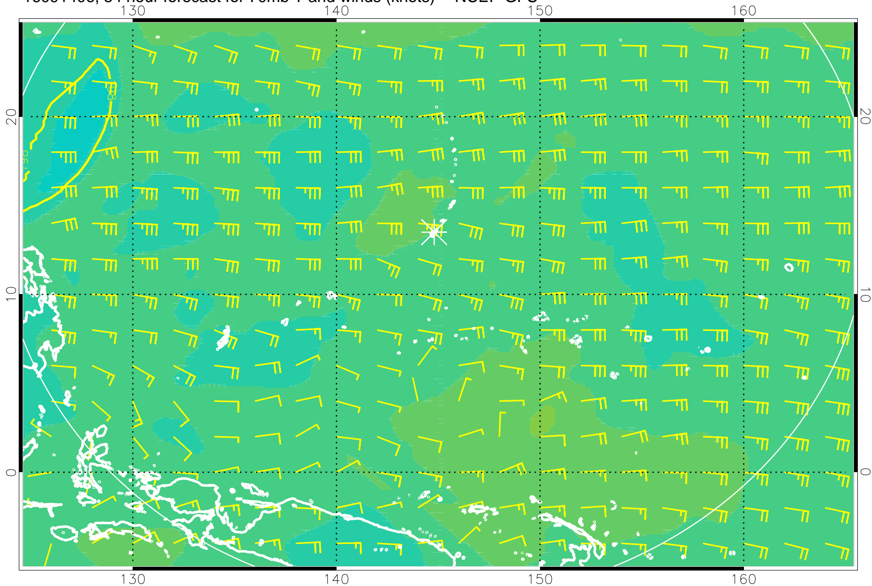
16091406, 54 hour forecast for 70mb T and winds (knots) -- NCEP GFS
