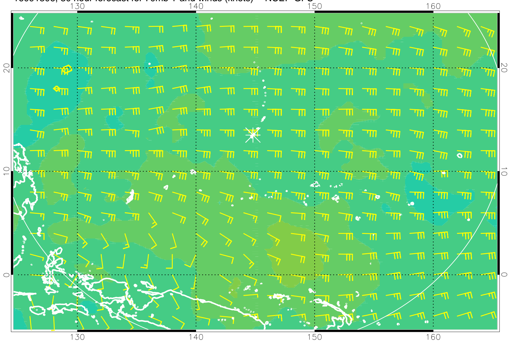
16091306, 30 hour forecast for 70mb T and winds (knots) -- NCEP GFS
