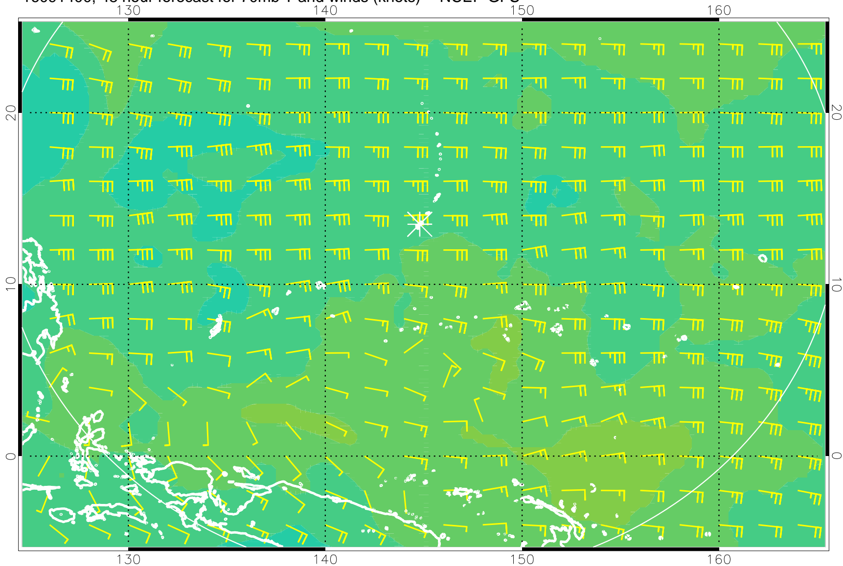
16091400, 48 hour forecast for 70mb T and winds (knots) -- NCEP GFS
