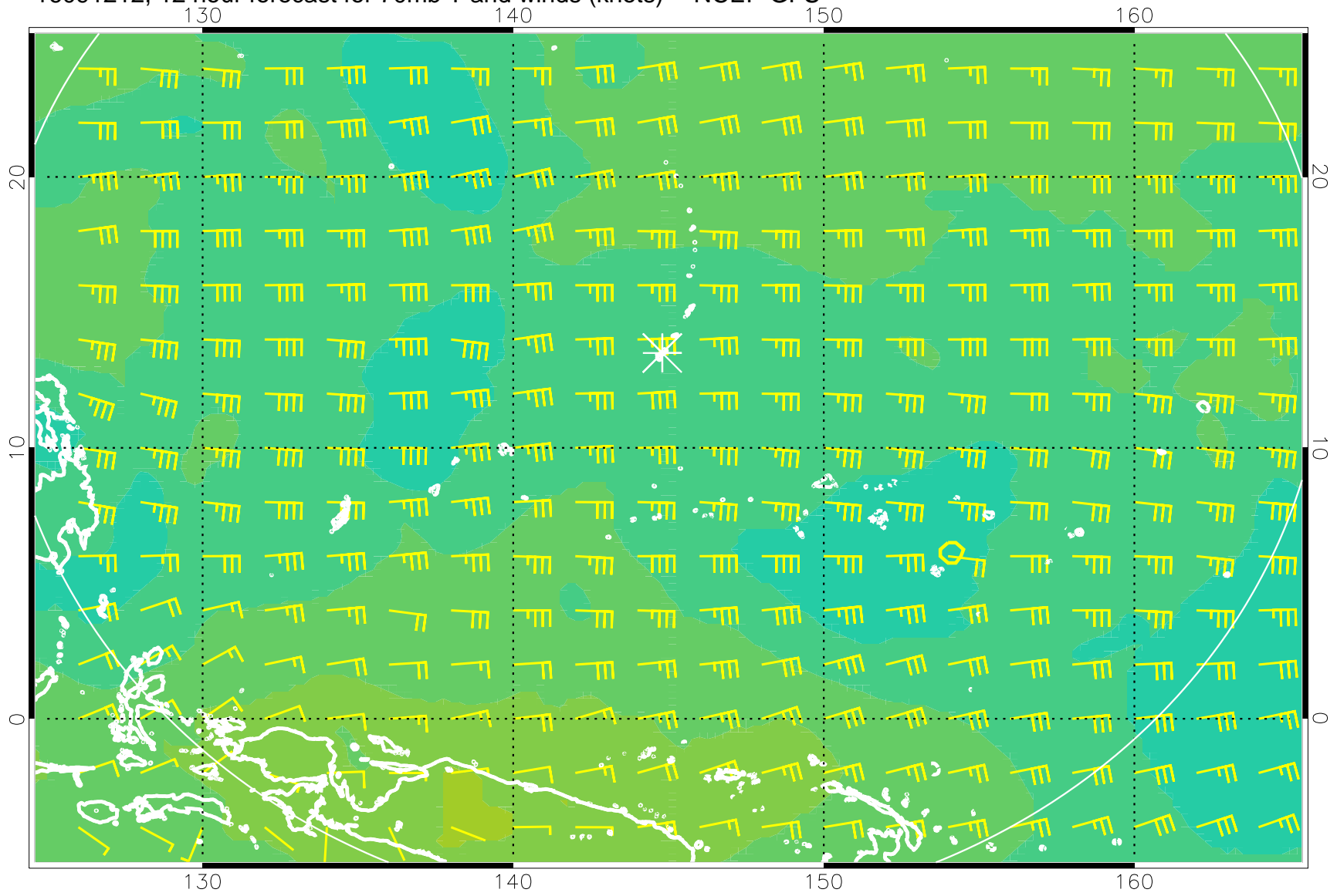
16091212, 12 hour forecast for 70mb T and winds (knots) -- NCEP GFS
