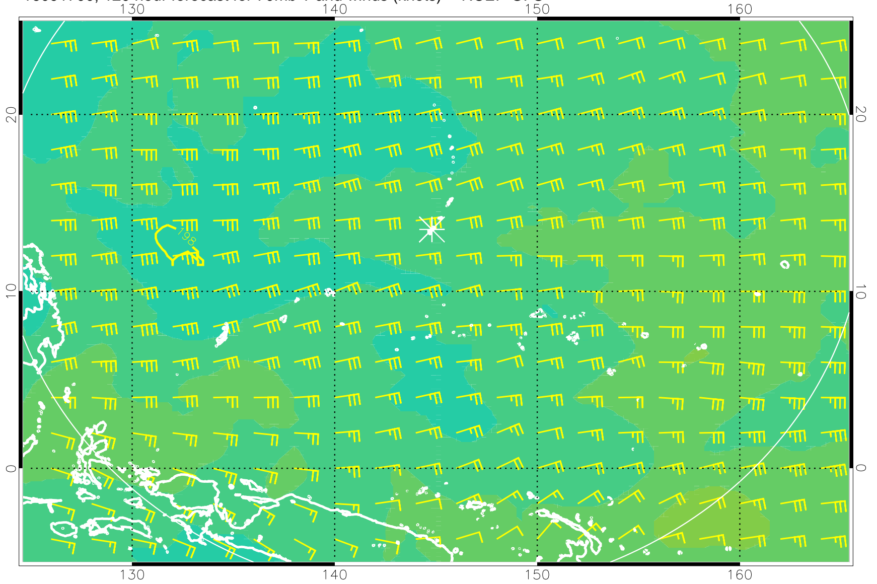
16091700, 120 hour forecast for 70mb T and winds (knots) -- NCEP GFS
