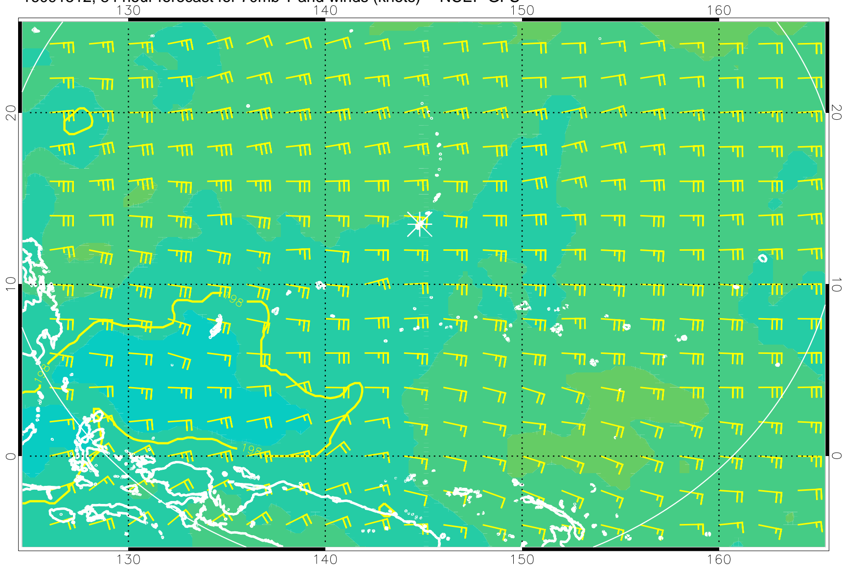
16091512, 84 hour forecast for 70mb T and winds (knots) -- NCEP GFS
