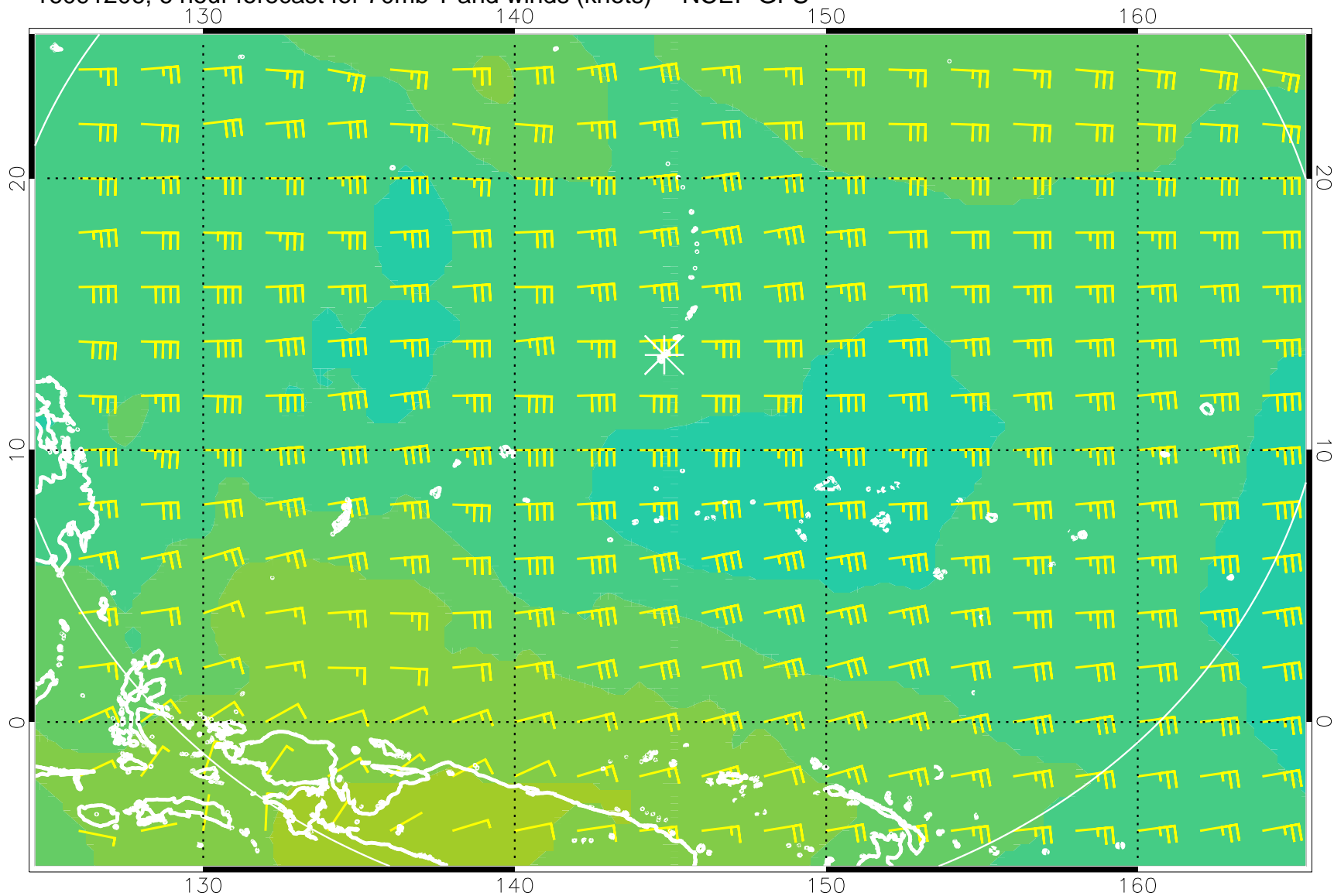
16091206, 6 hour forecast for 70mb T and winds (knots) -- NCEP GFS
