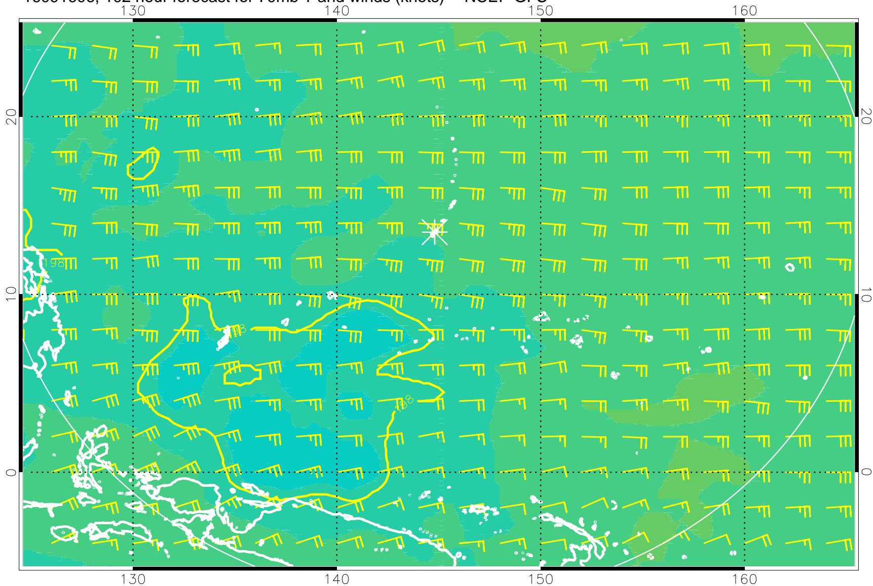
16091606, 102 hour forecast for 70mb T and winds (knots) -- NCEP GFS
