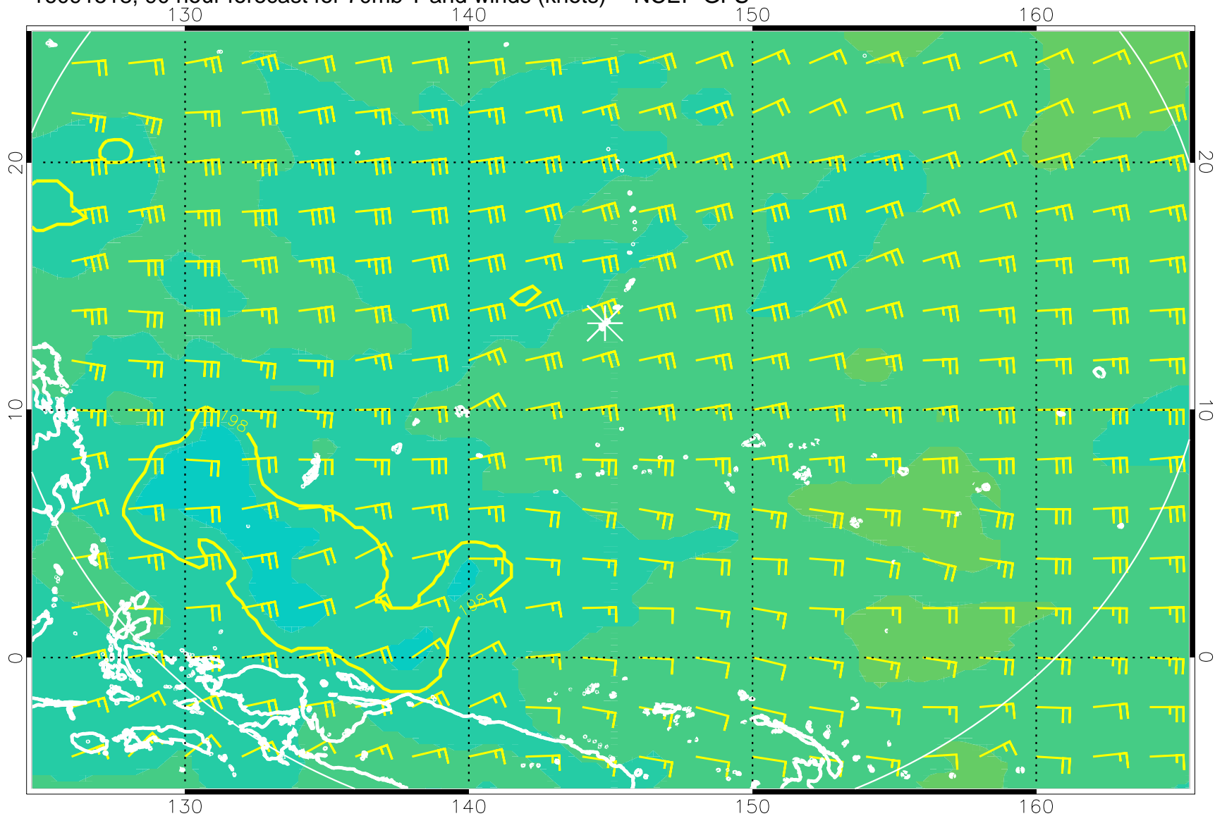
16091518, 90 hour forecast for 70mb T and winds (knots) -- NCEP GFS
