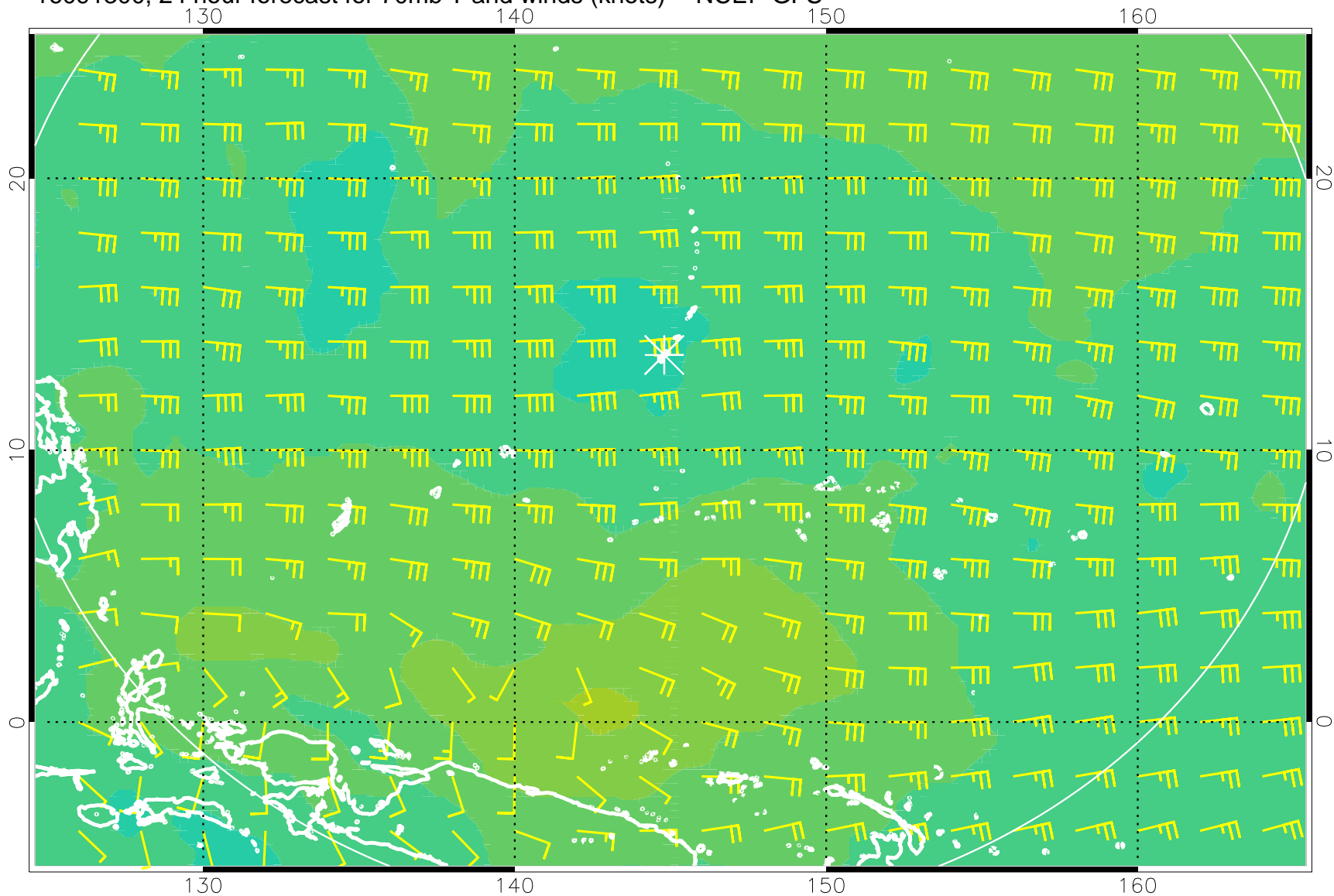
16091300, 24 hour forecast for 70mb T and winds (knots) -- NCEP GFS
