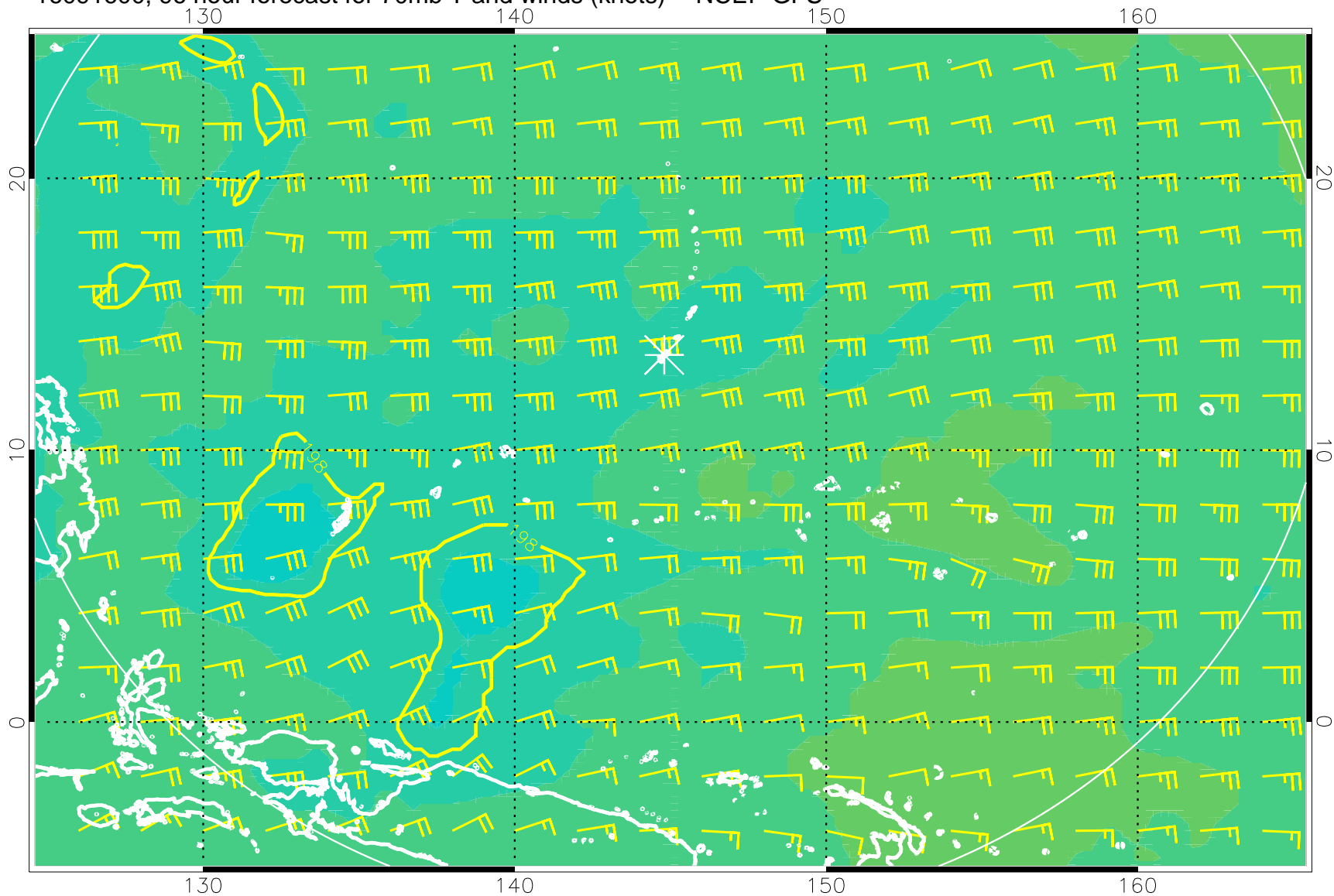
16091600, 96 hour forecast for 70mb T and winds (knots) -- NCEP GFS
