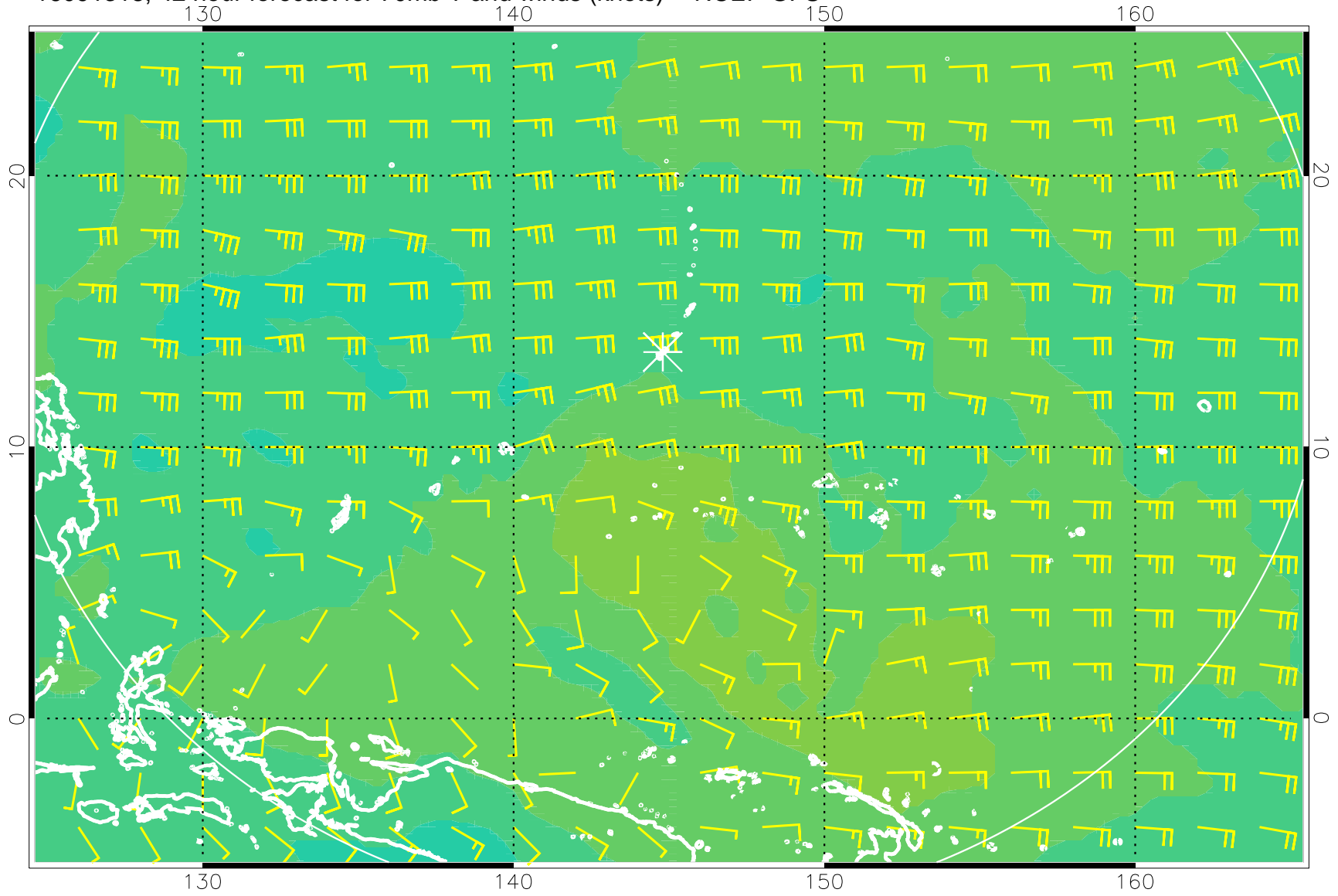
16091318, 42 hour forecast for 70mb T and winds (knots) -- NCEP GFS
