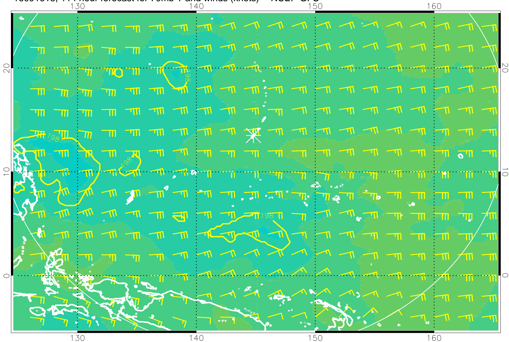
16091618, 114 hour forecast for 70mb T and winds (knots) -- NCEP GFS
