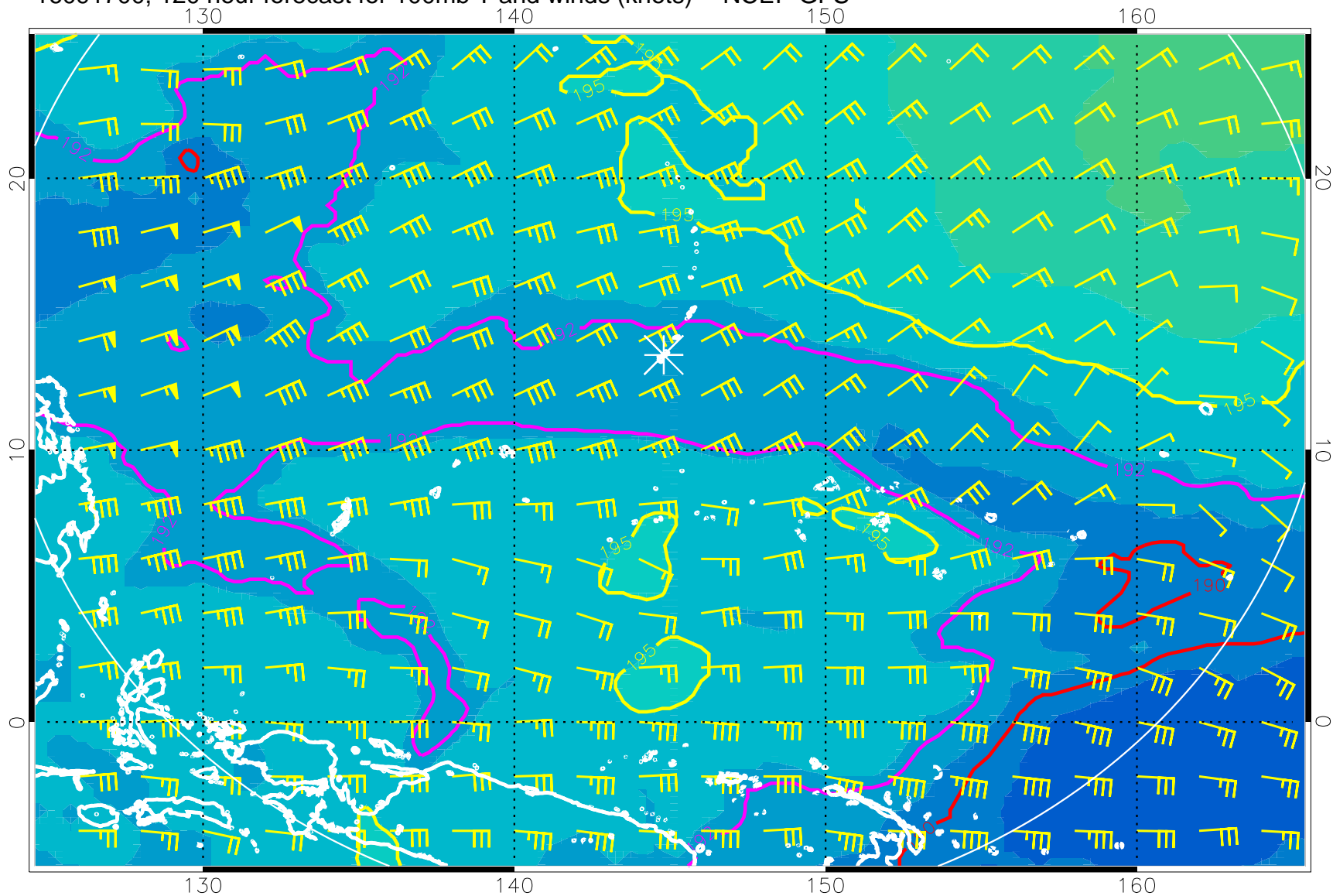
16091700, 120 hour forecast for 100mb T and winds (knots) -- NCEP GFS
