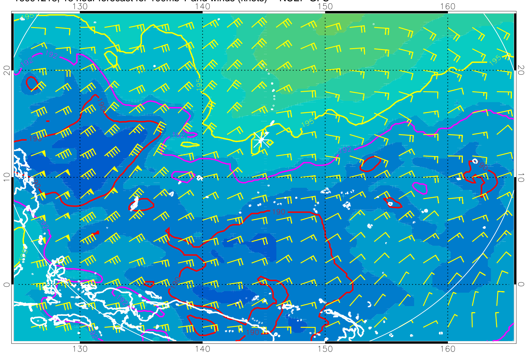
16091218, 18 hour forecast for 100mb T and winds (knots) -- NCEP GFS
