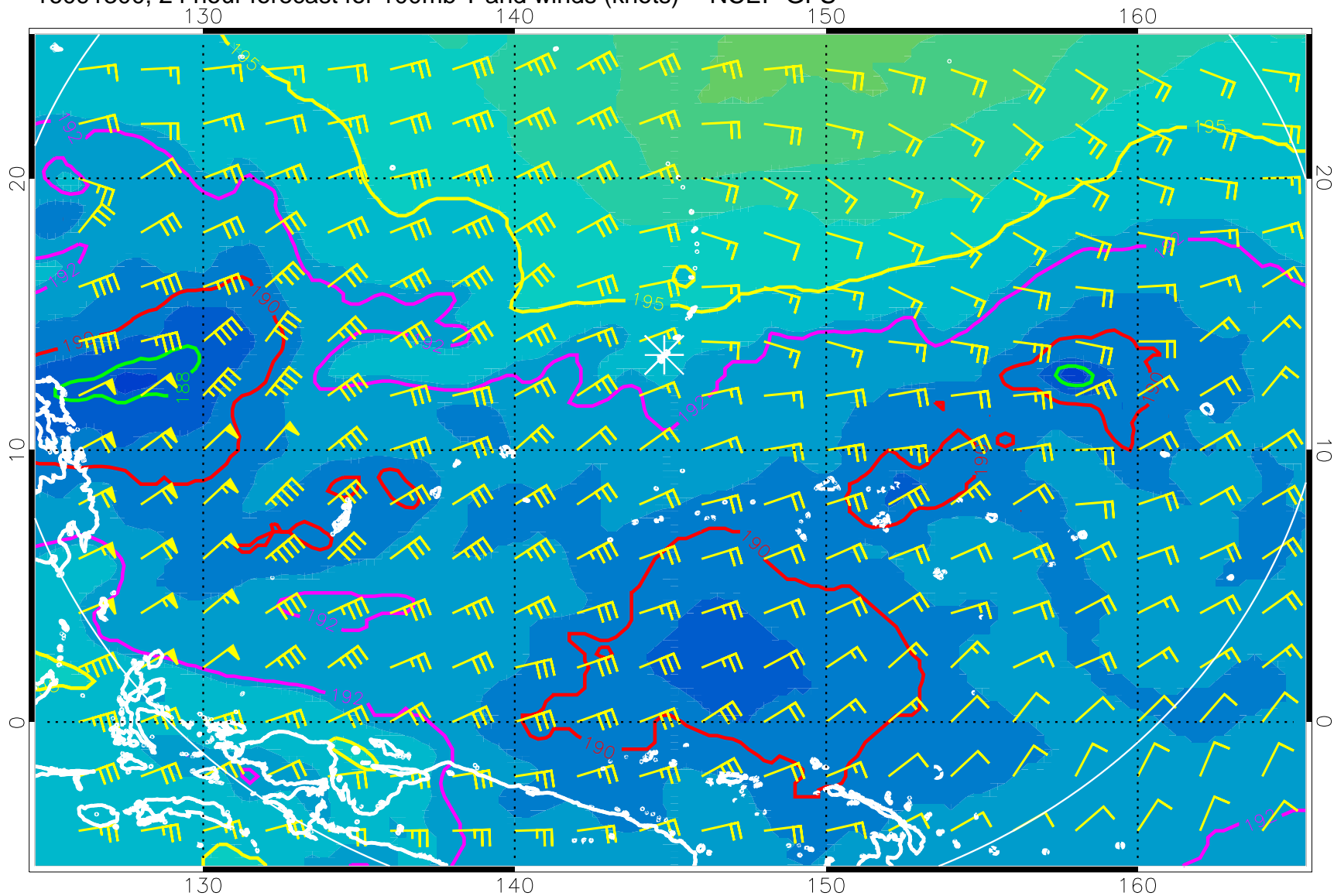
16091300, 24 hour forecast for 100mb T and winds (knots) -- NCEP GFS
