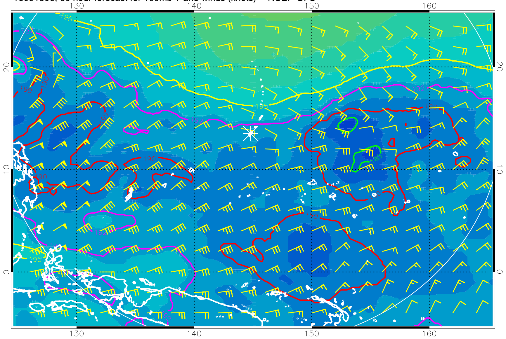
16091306, 30 hour forecast for 100mb T and winds (knots) -- NCEP GFS
