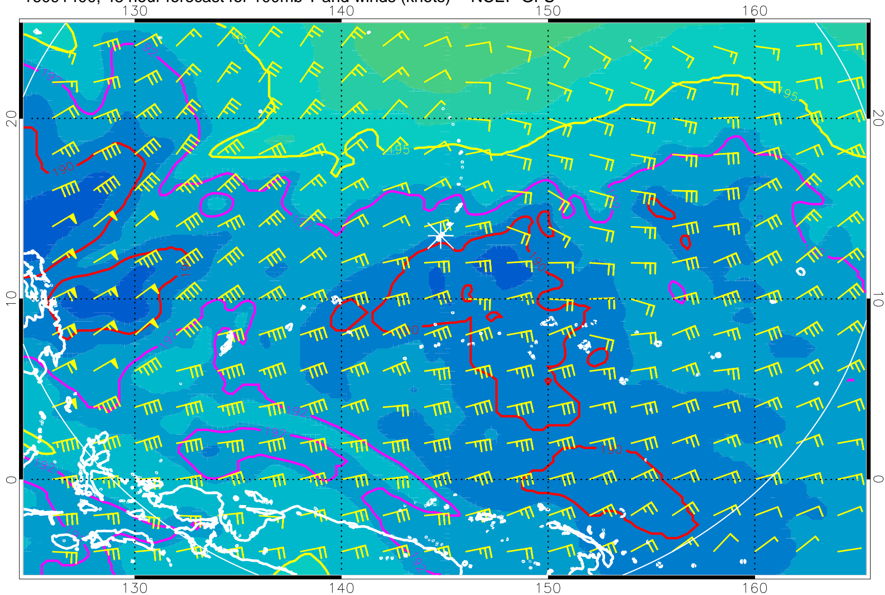
16091400, 48 hour forecast for 100mb T and winds (knots) -- NCEP GFS
