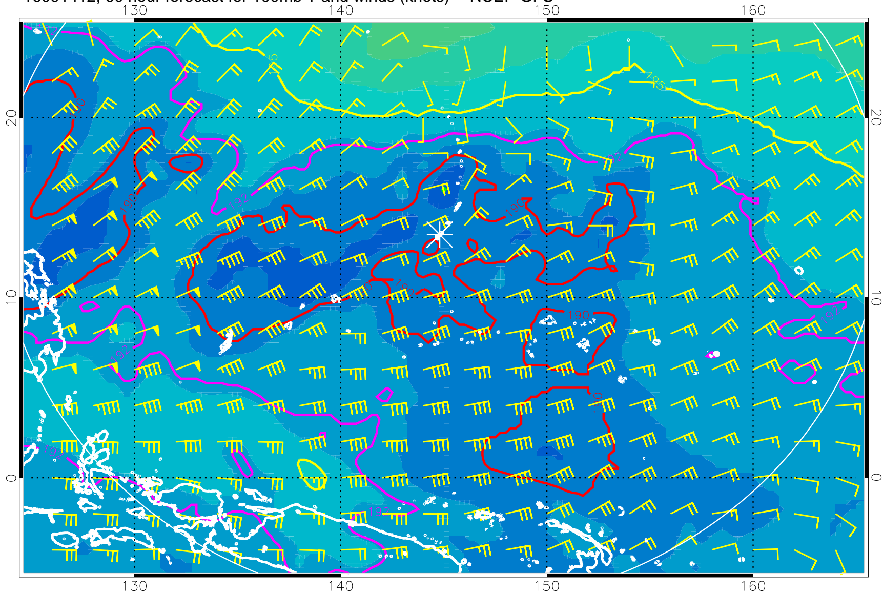
16091412, 60 hour forecast for 100mb T and winds (knots) -- NCEP GFS
