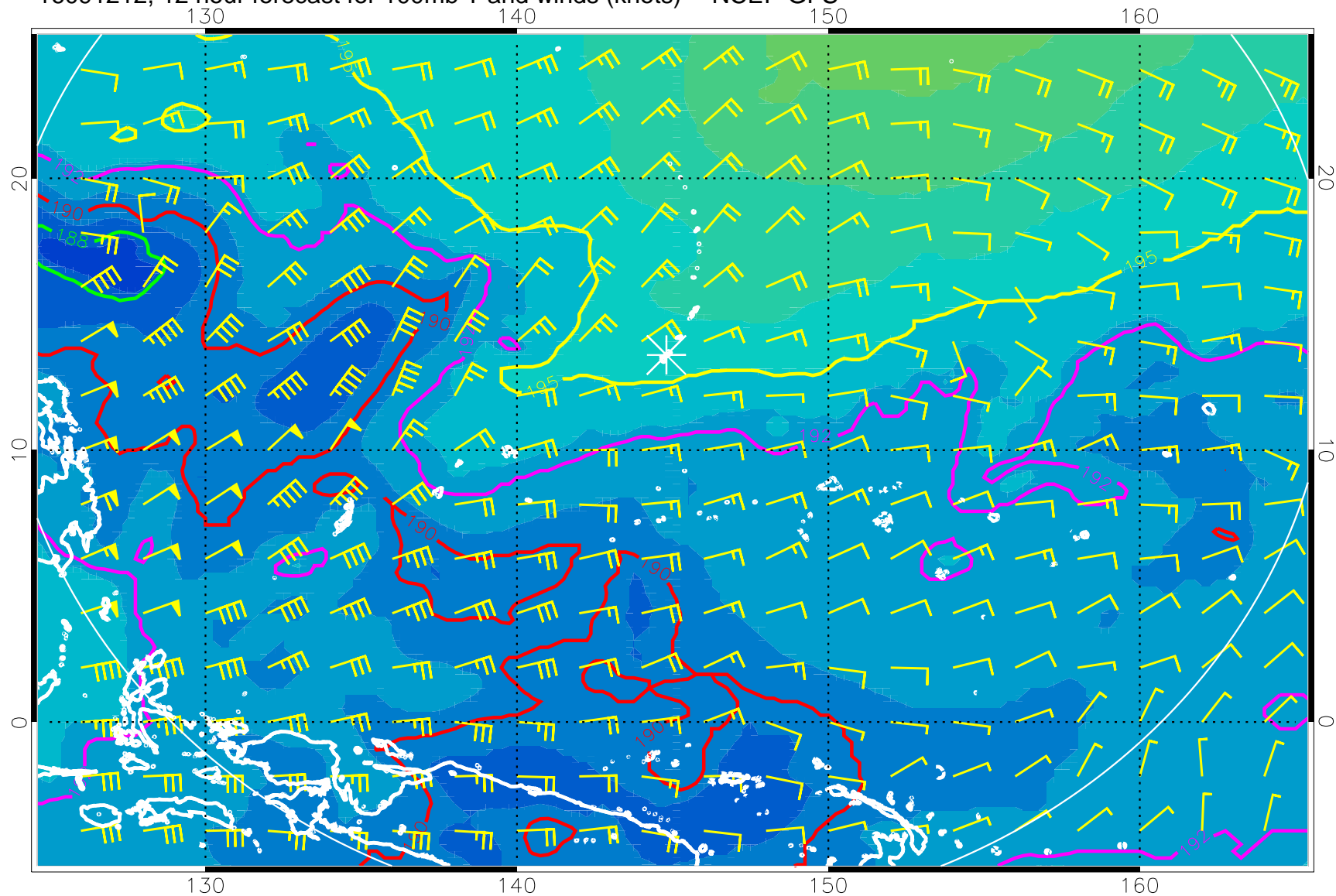
16091212, 12 hour forecast for 100mb T and winds (knots) -- NCEP GFS
