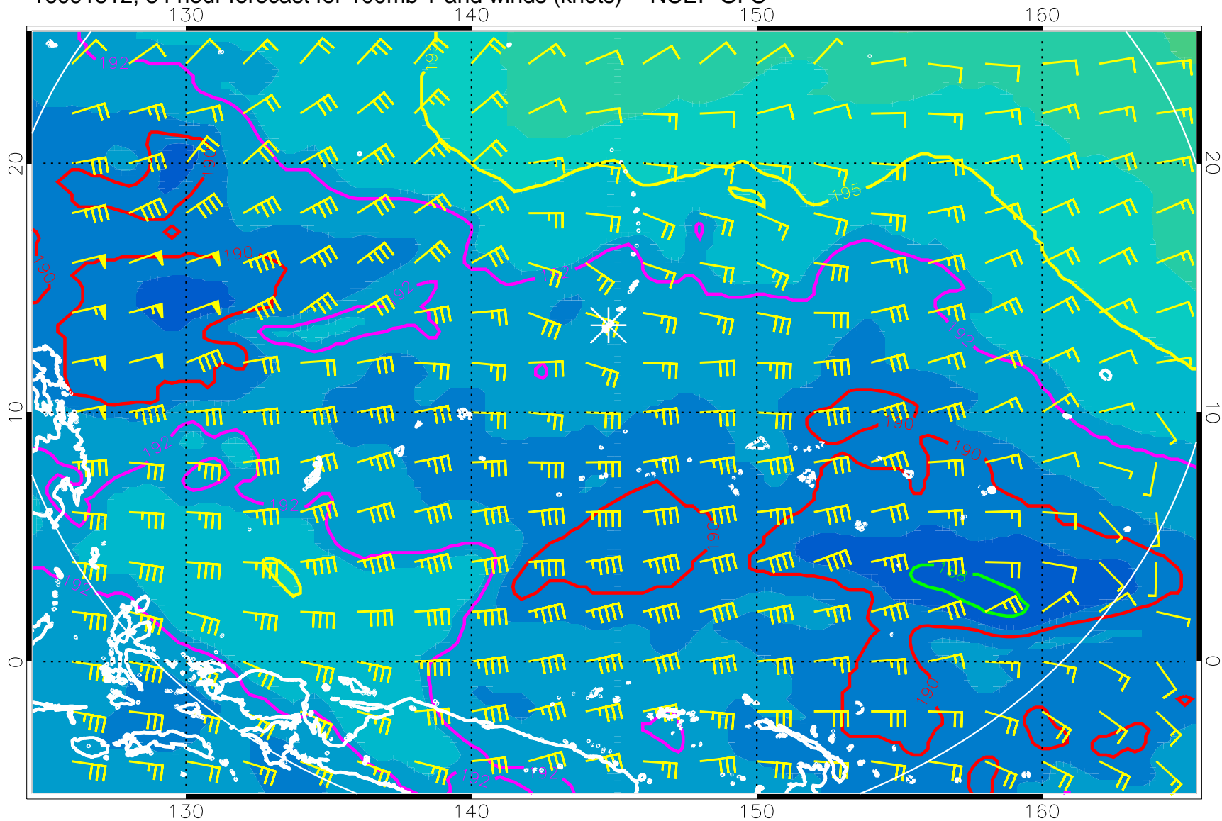
16091512, 84 hour forecast for 100mb T and winds (knots) -- NCEP GFS
