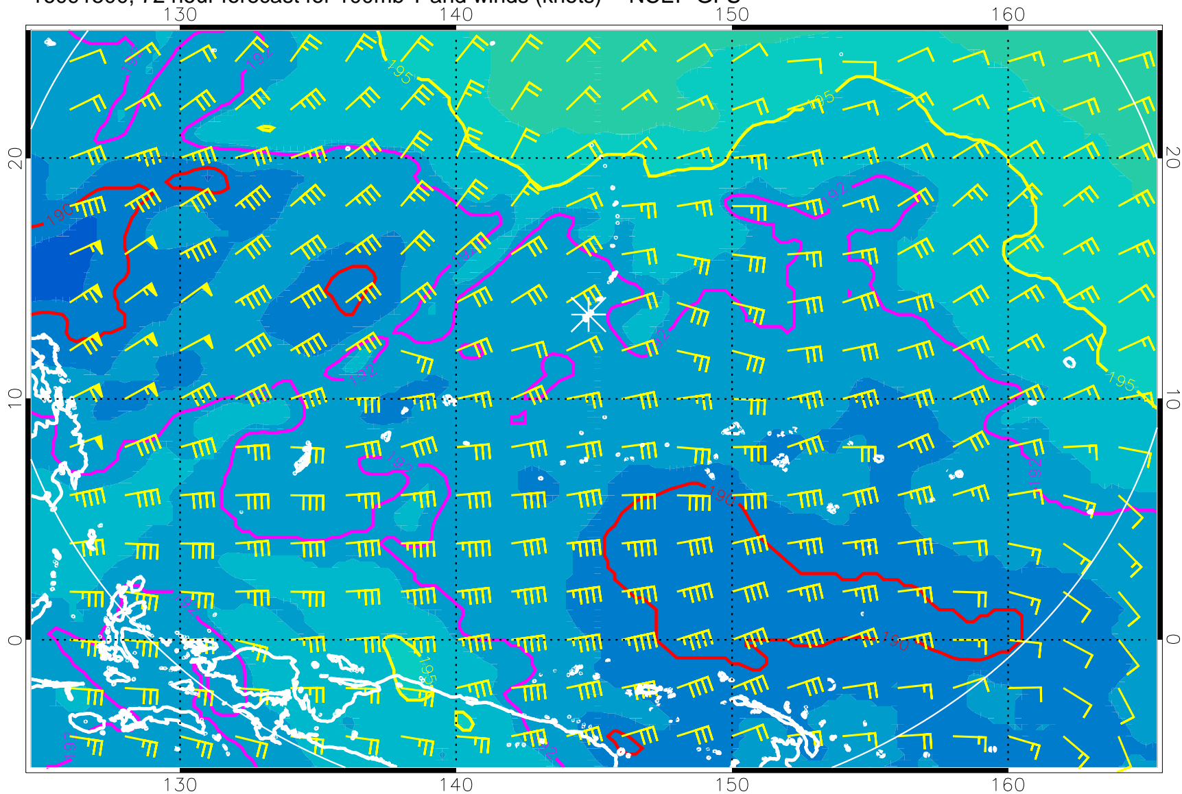
16091500, 72 hour forecast for 100mb T and winds (knots) -- NCEP GFS
