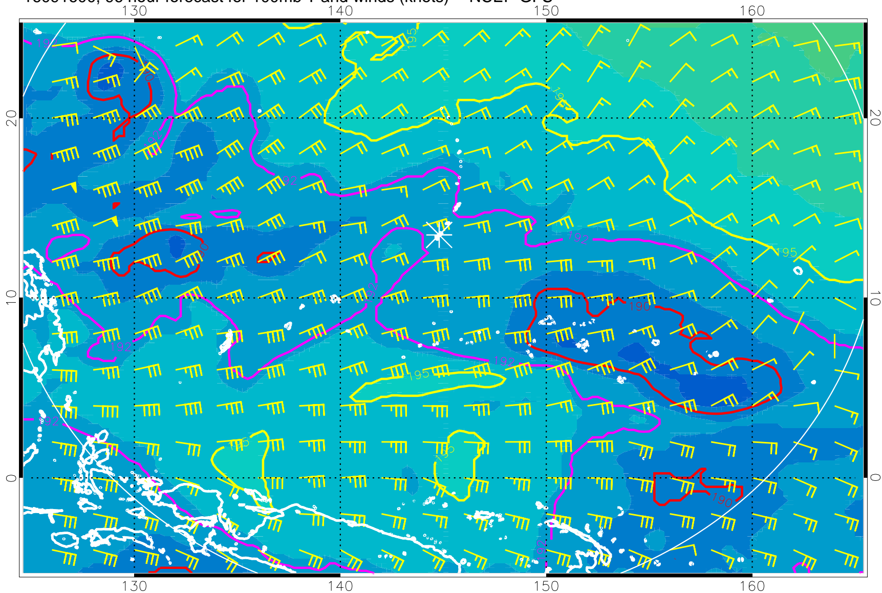
16091600, 96 hour forecast for 100mb T and winds (knots) -- NCEP GFS
