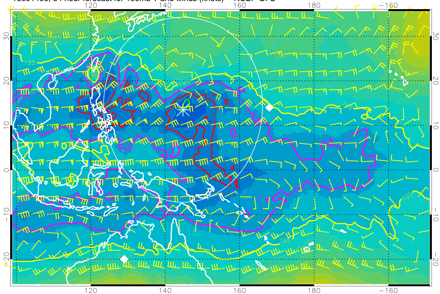
16091406, 54 hour forecast for 100mb T and winds (knots) -- NCEP GFS
