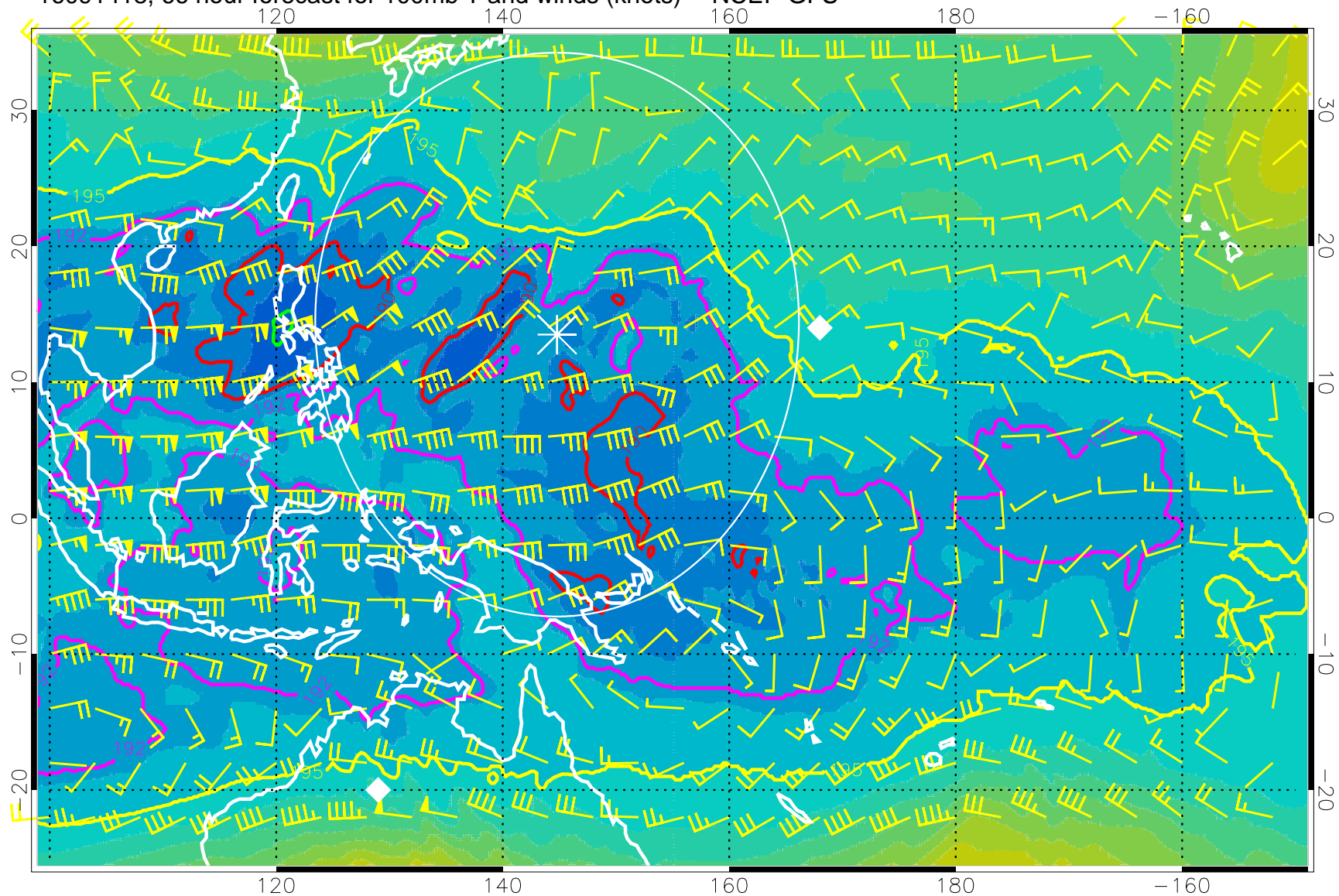
16091418, 66 hour forecast for 100mb T and winds (knots) -- NCEP GFS
