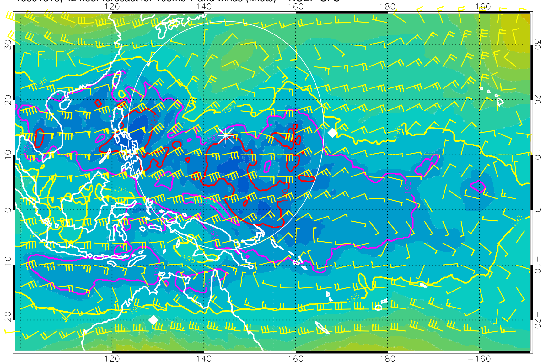
16091318, 42 hour forecast for 100mb T and winds (knots) -- NCEP GFS
