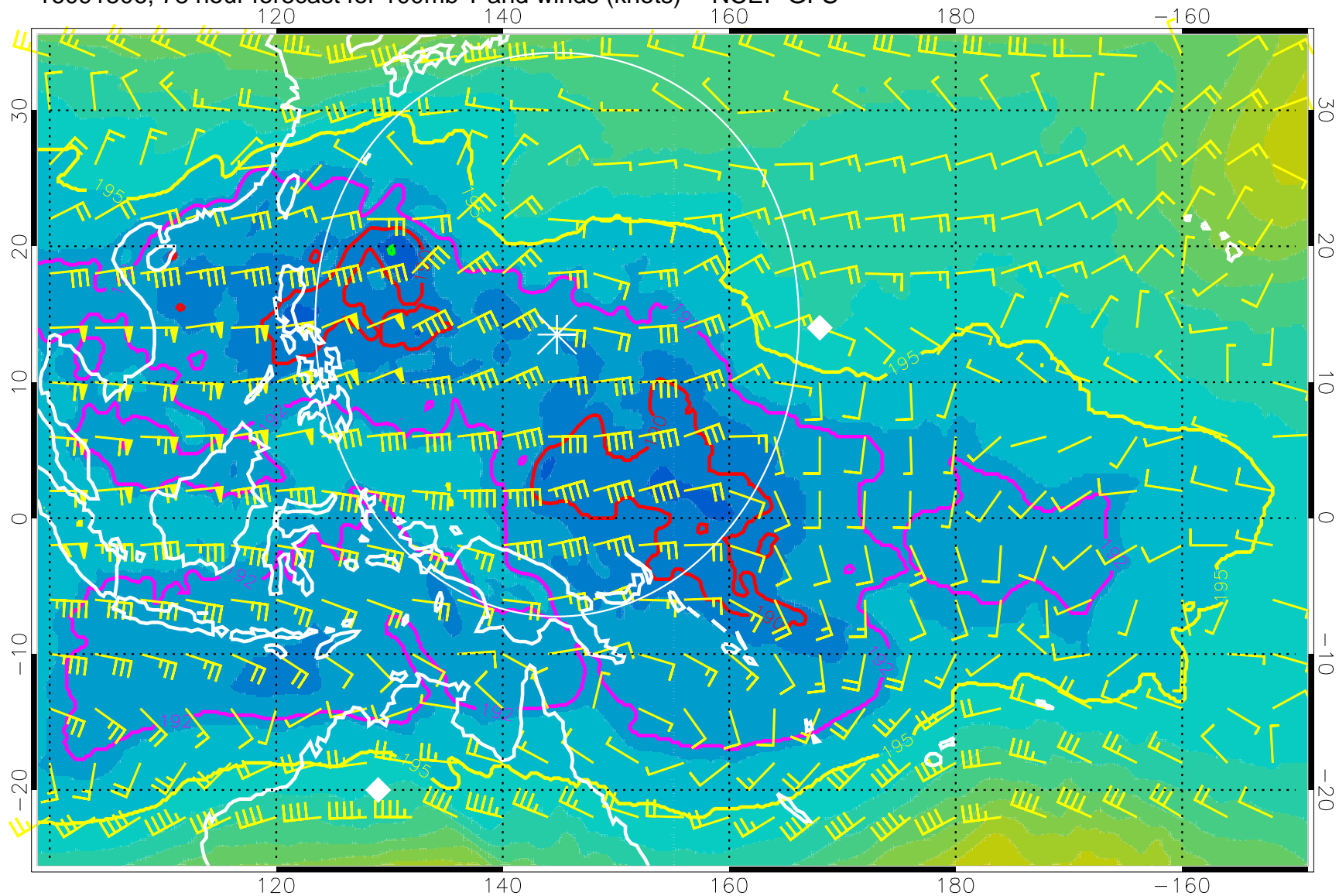
16091506, 78 hour forecast for 100mb T and winds (knots) -- NCEP GFS
