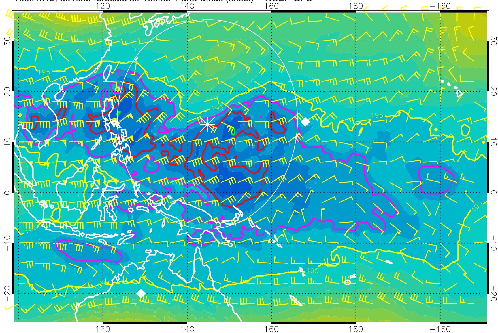
16091312, 36 hour forecast for 100mb T and winds (knots) -- NCEP GFS
