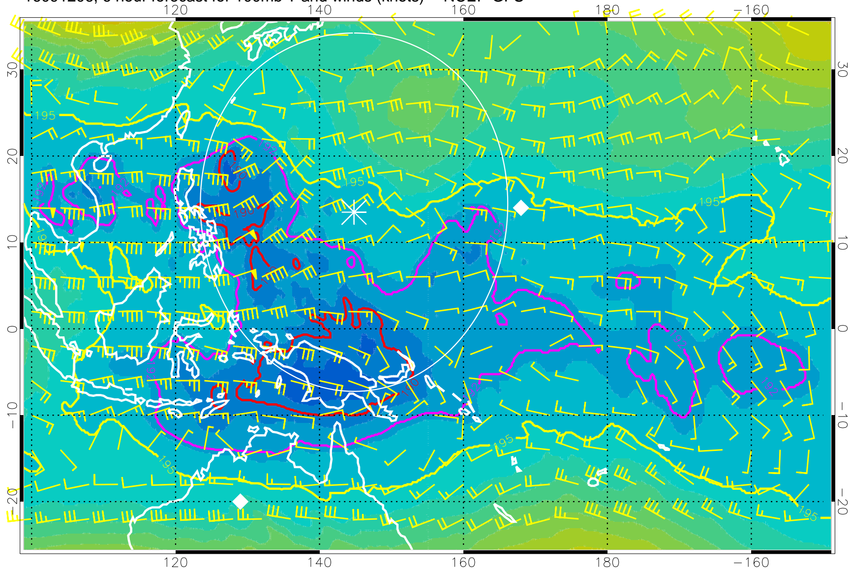
16091206, 6 hour forecast for 100mb T and winds (knots) -- NCEP GFS
