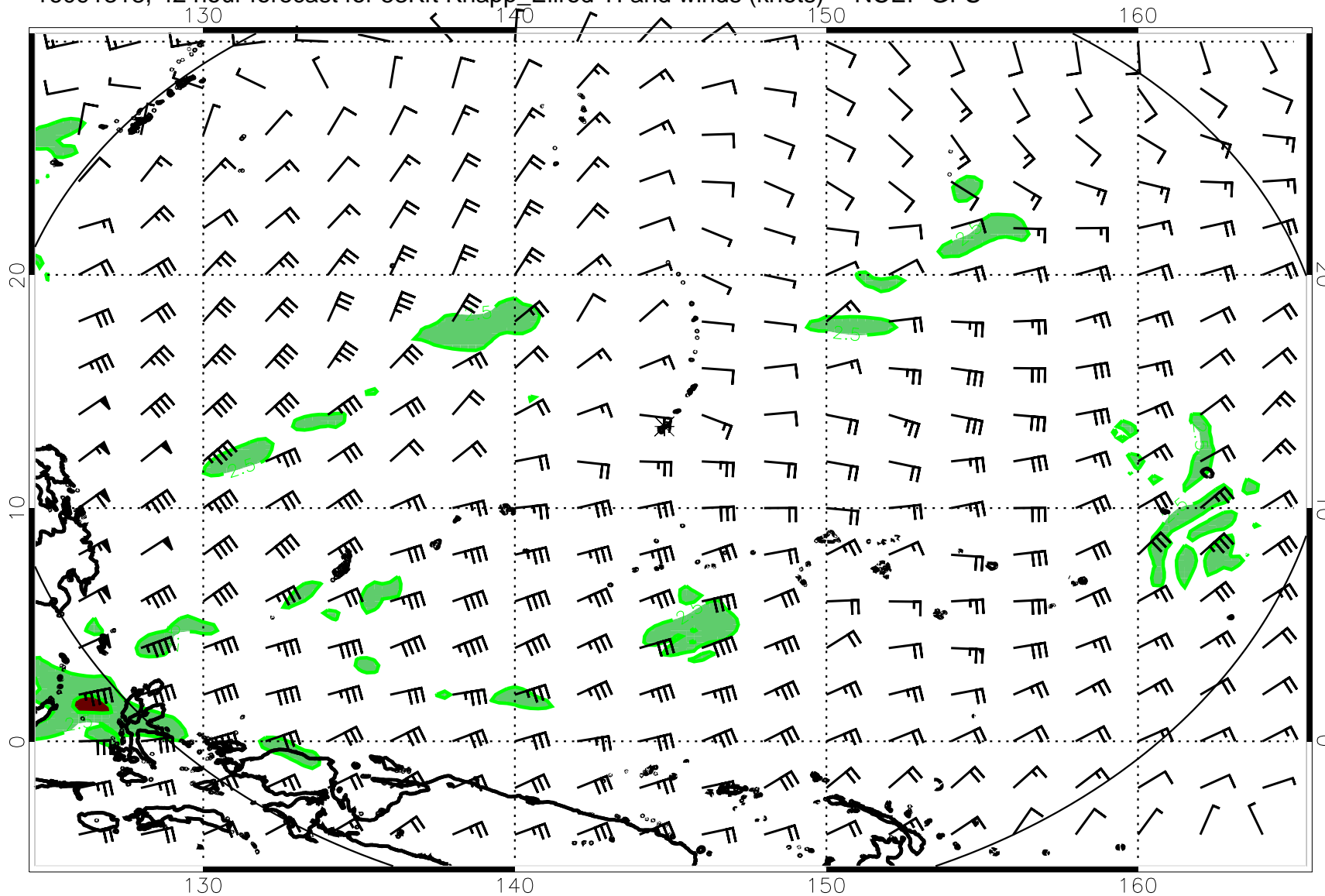
16091318, 42 hour forecast for 53Kft Knapp_Ellrod TI and winds (knots) -- NCEP GFS
