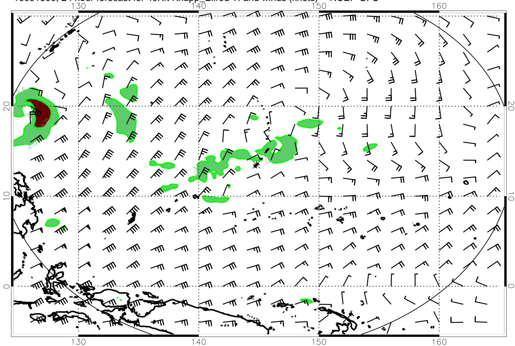
16091300, 24 hour forecast for 49Kft Knapp_Ellrod TI and winds (knots) -- NCEP GFS
