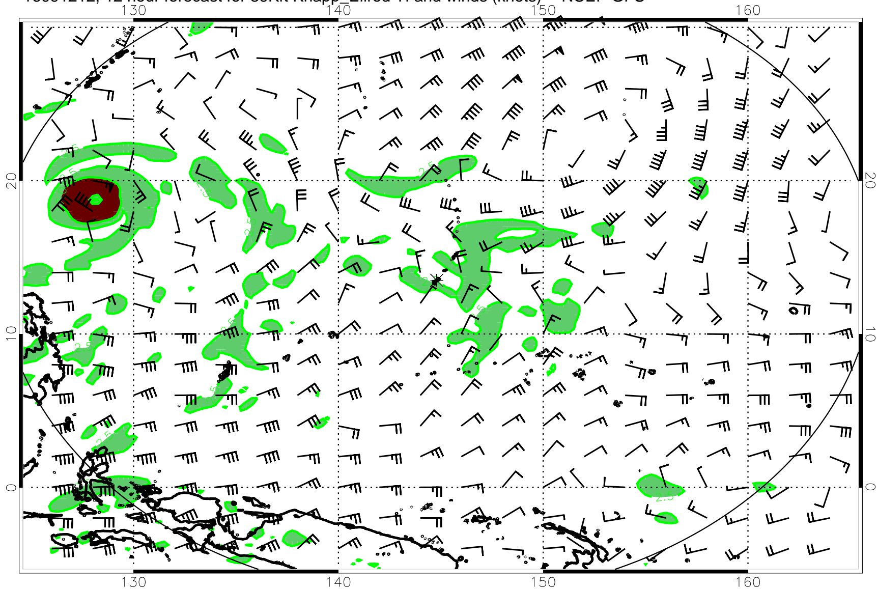
16091212, 12 hour forecast for 39Kft Knapp_Ellrod TI and winds (knots) -- NCEP GFS
