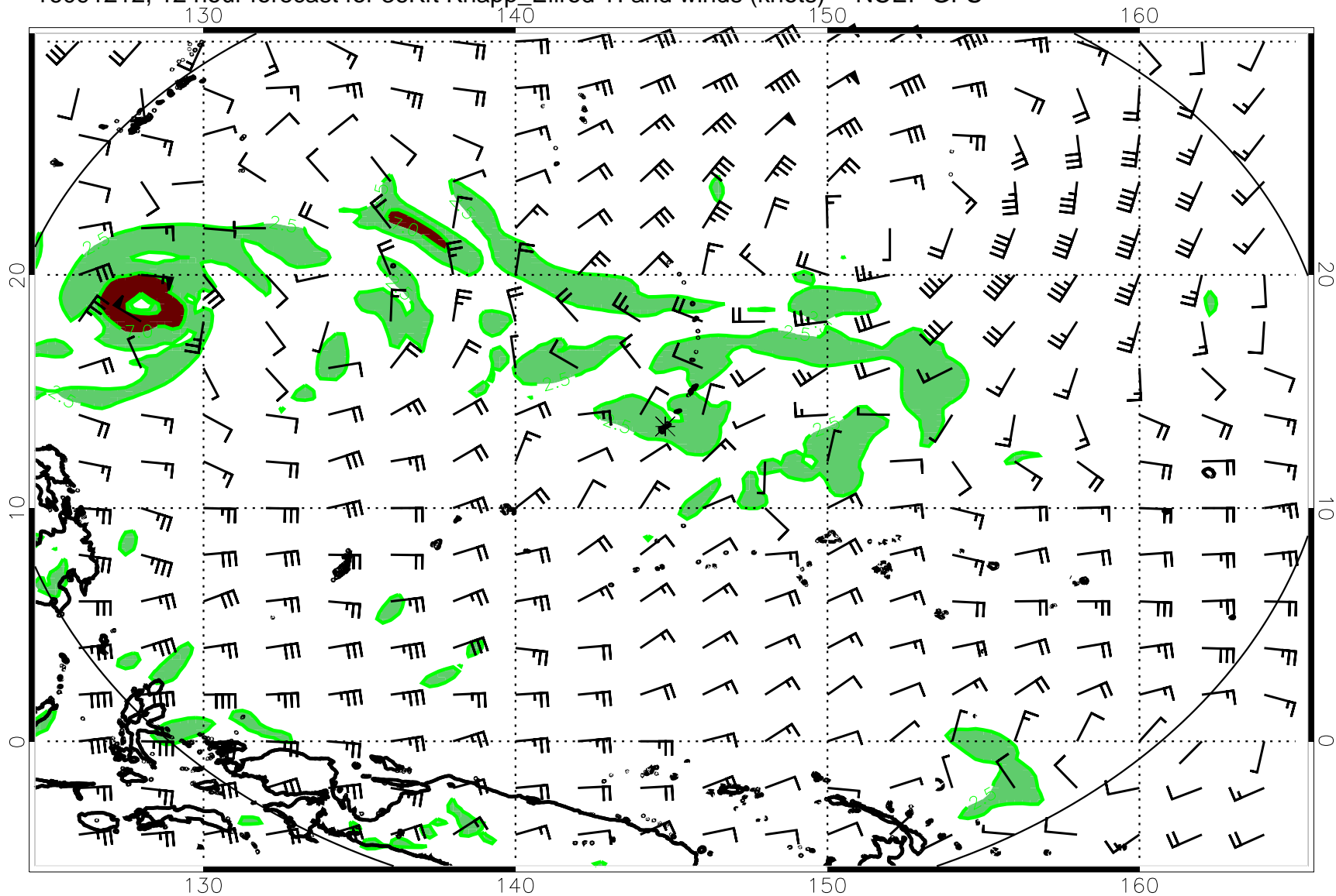
16091212, 12 hour forecast for 36Kft Knapp_Ellrod TI and winds (knots) -- NCEP GFS
