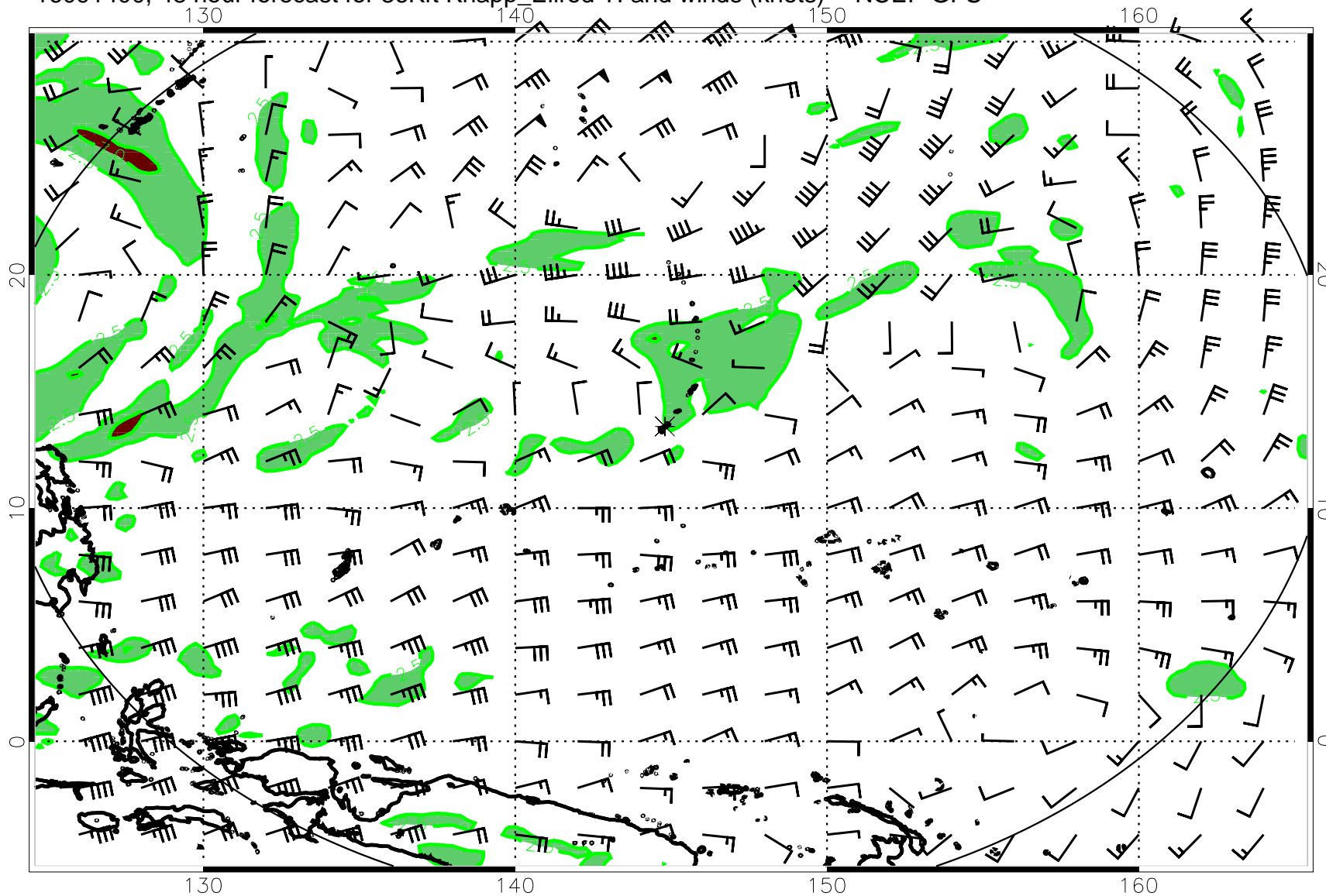
16091400, 48 hour forecast for 36Kft Knapp_Ellrod TI and winds (knots) -- NCEP GFS
