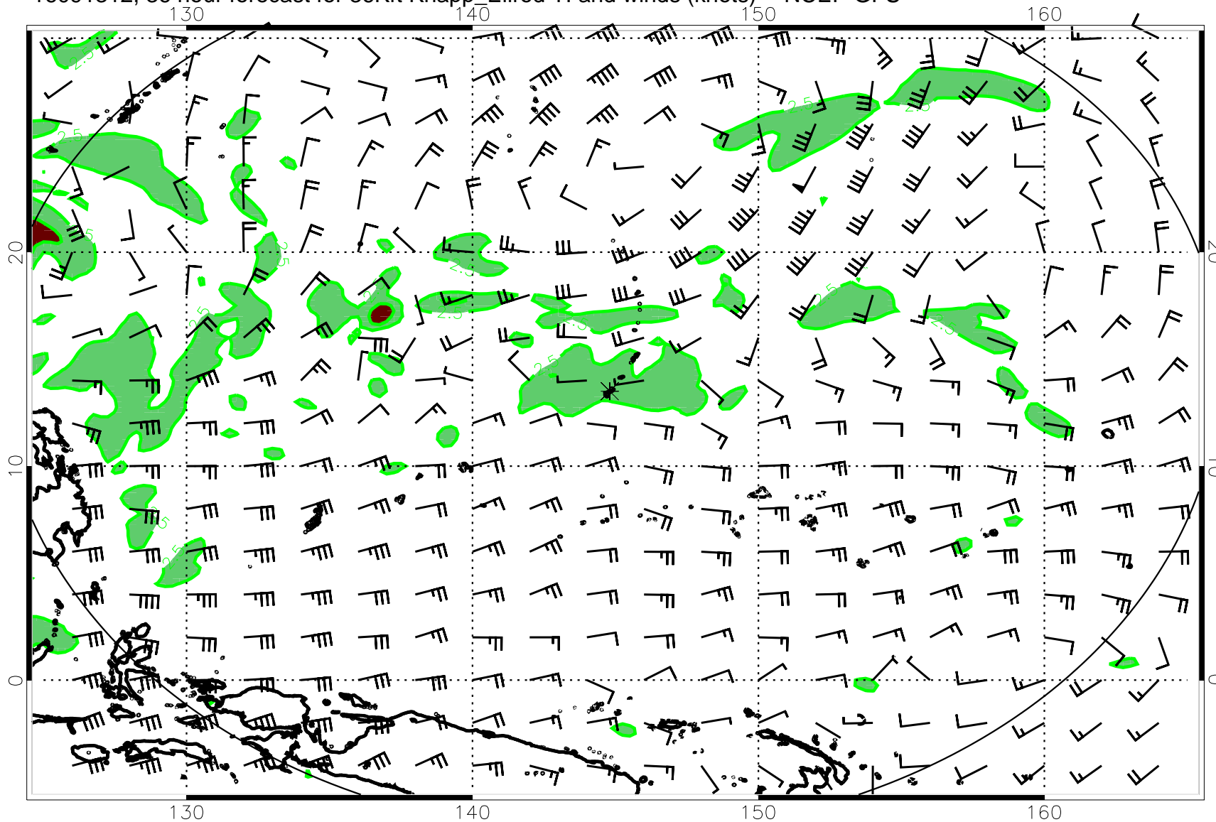
16091312, 36 hour forecast for 36Kft Knapp_Ellrod TI and winds (knots) -- NCEP GFS
