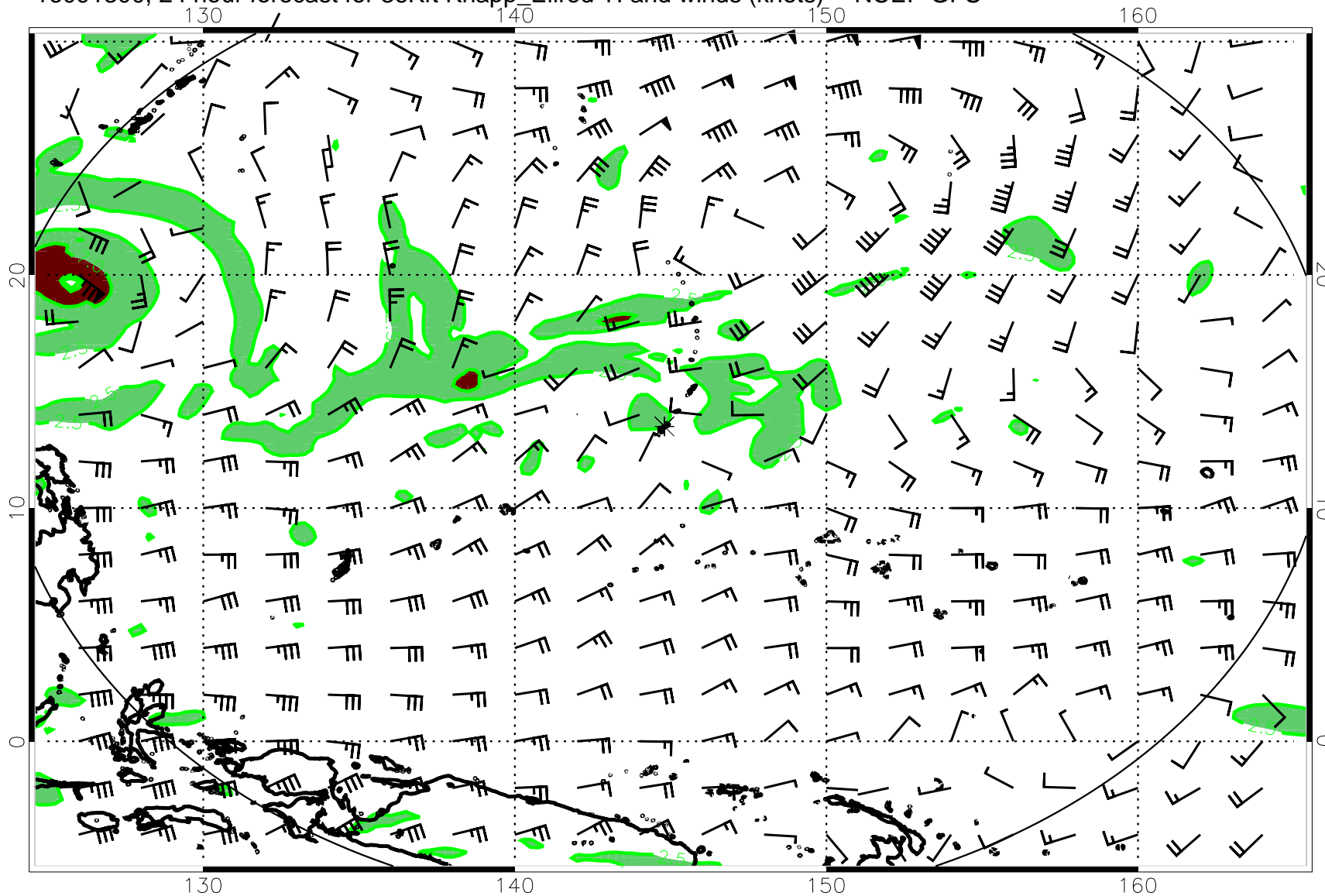
16091300, 24 hour forecast for 36Kft Knapp_Ellrod TI and winds (knots) -- NCEP GFS
