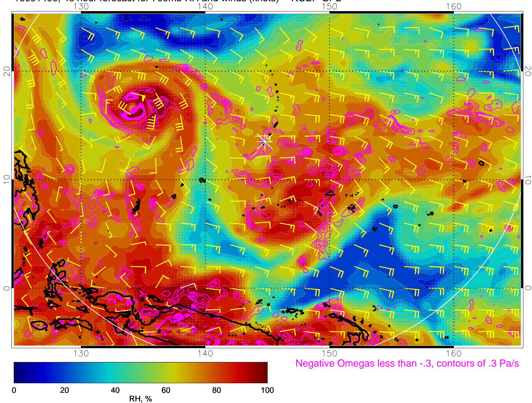
16091400, 48 hour forecast for 700mb RH and winds (knots) -- NCEP GFS
