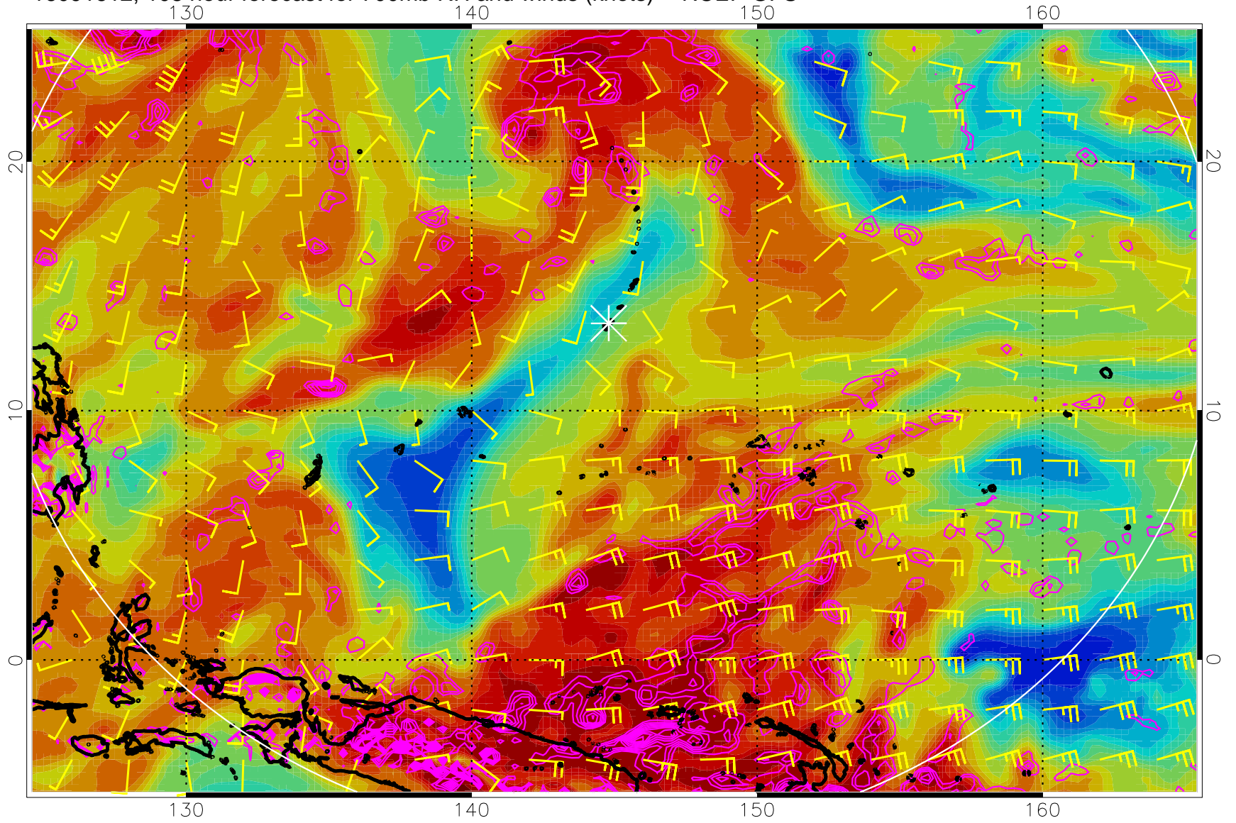
16091612, 108 hour forecast for 700mb RH and winds (knots) -- NCEP GFS
