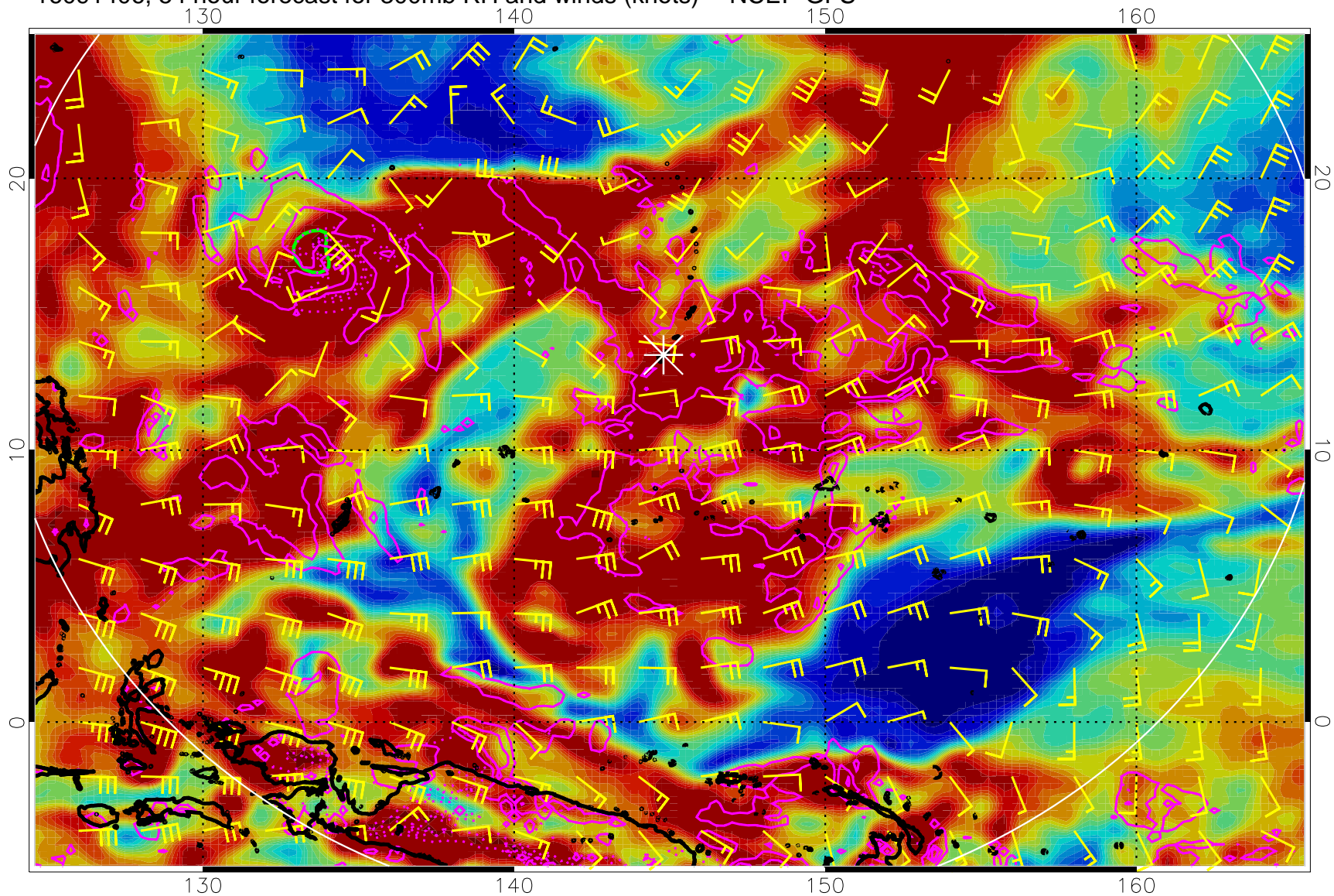
16091406, 54 hour forecast for 300mb RH and winds (knots) -- NCEP GFS
