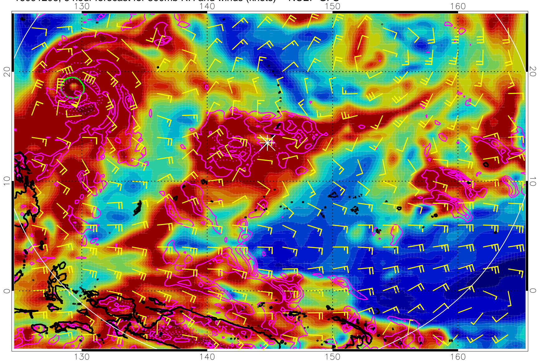
16091206, 6 hour forecast for 300mb RH and winds (knots) -- NCEP GFS
