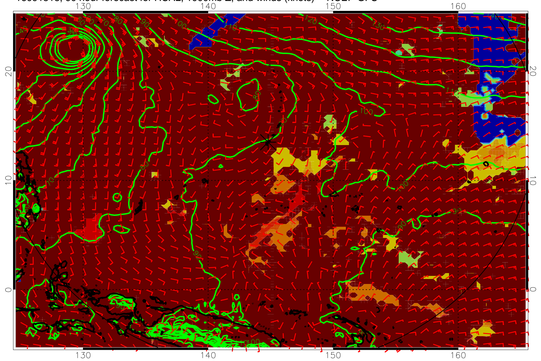
16091518, 90 hour forecast for HCAL, 1000mb Z, and winds (knots) -- NCEP GFS
