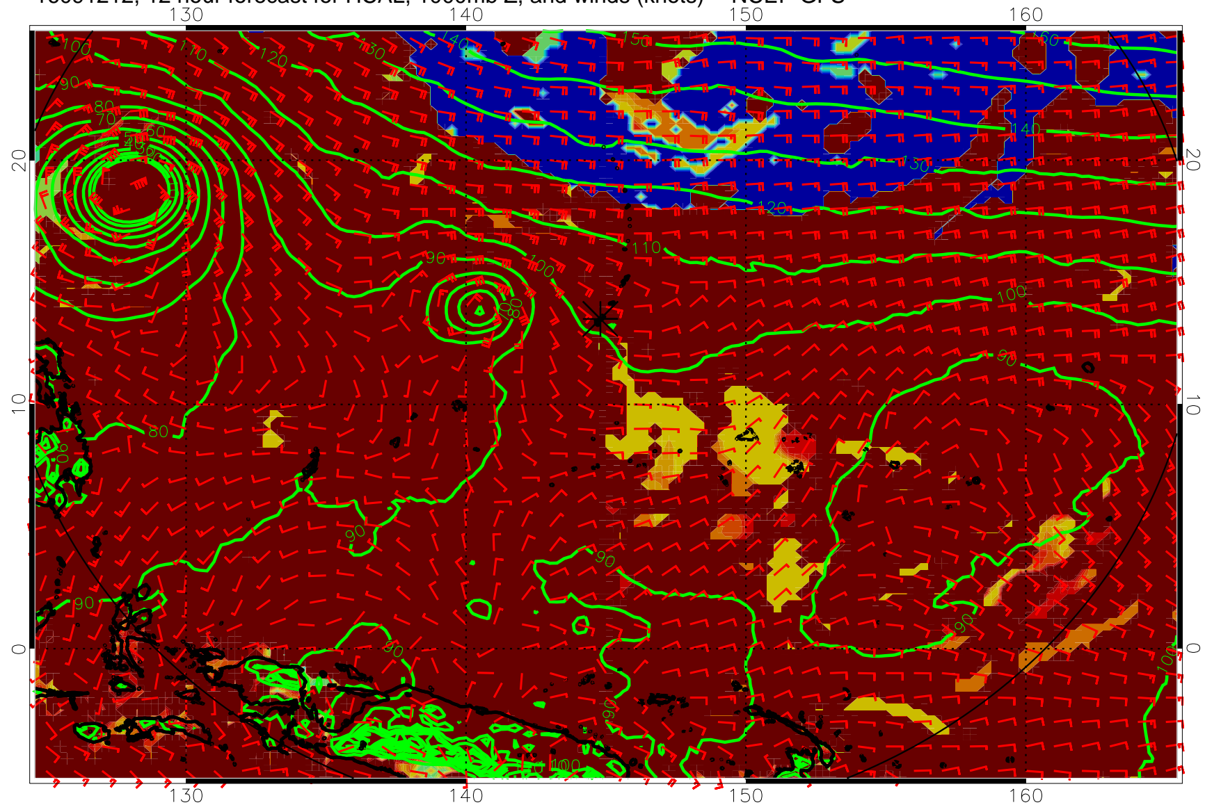
16091212, 12 hour forecast for HCAL, 1000mb Z, and winds (knots) -- NCEP GFS
