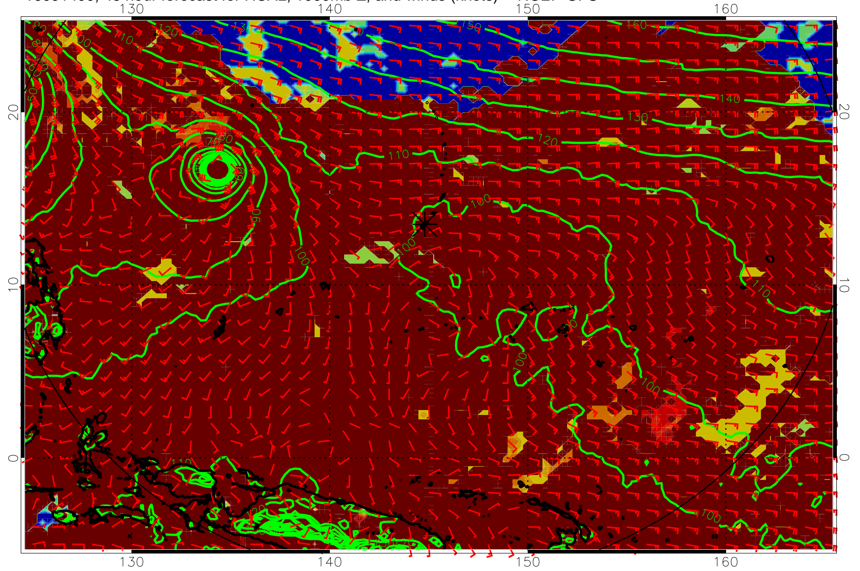
16091400, 48 hour forecast for HCAL, 1000mb Z, and winds (knots) -- NCEP GFS
