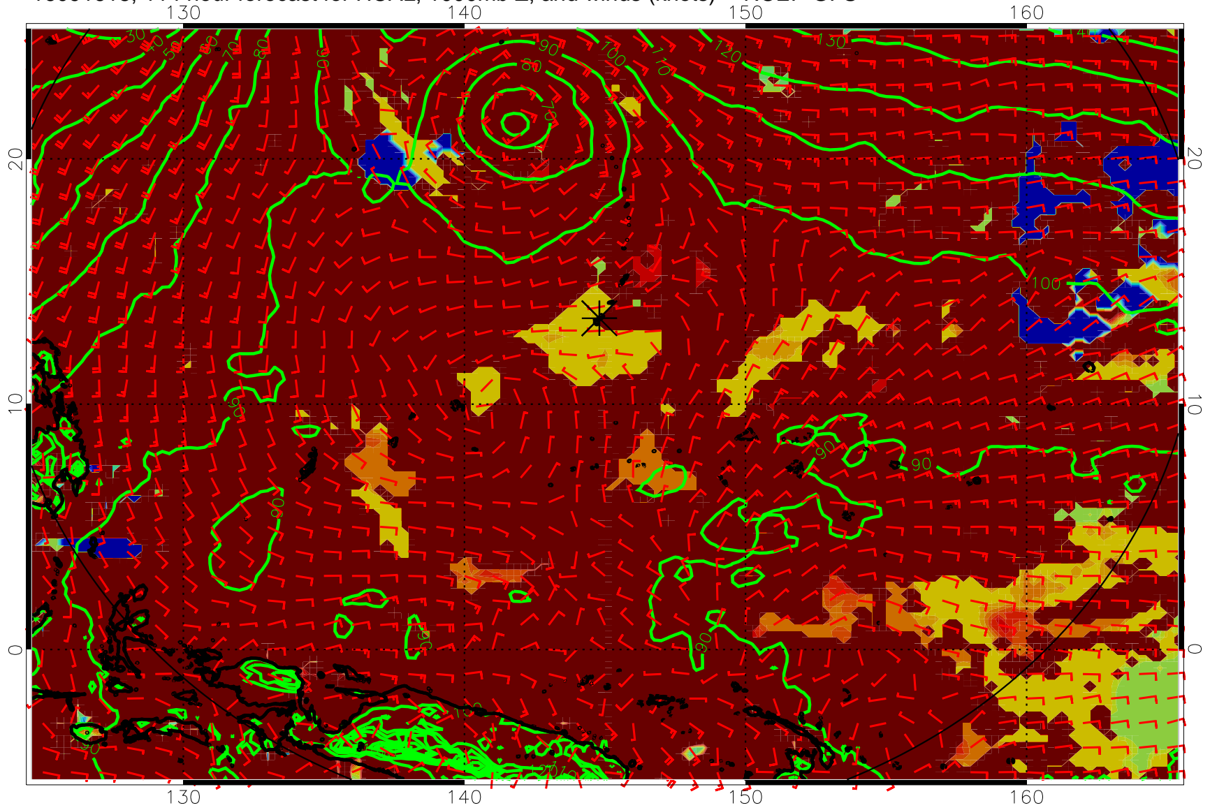
16091618, 114 hour forecast for HCAL, 1000mb Z, and winds (knots) -- NCEP GFS
