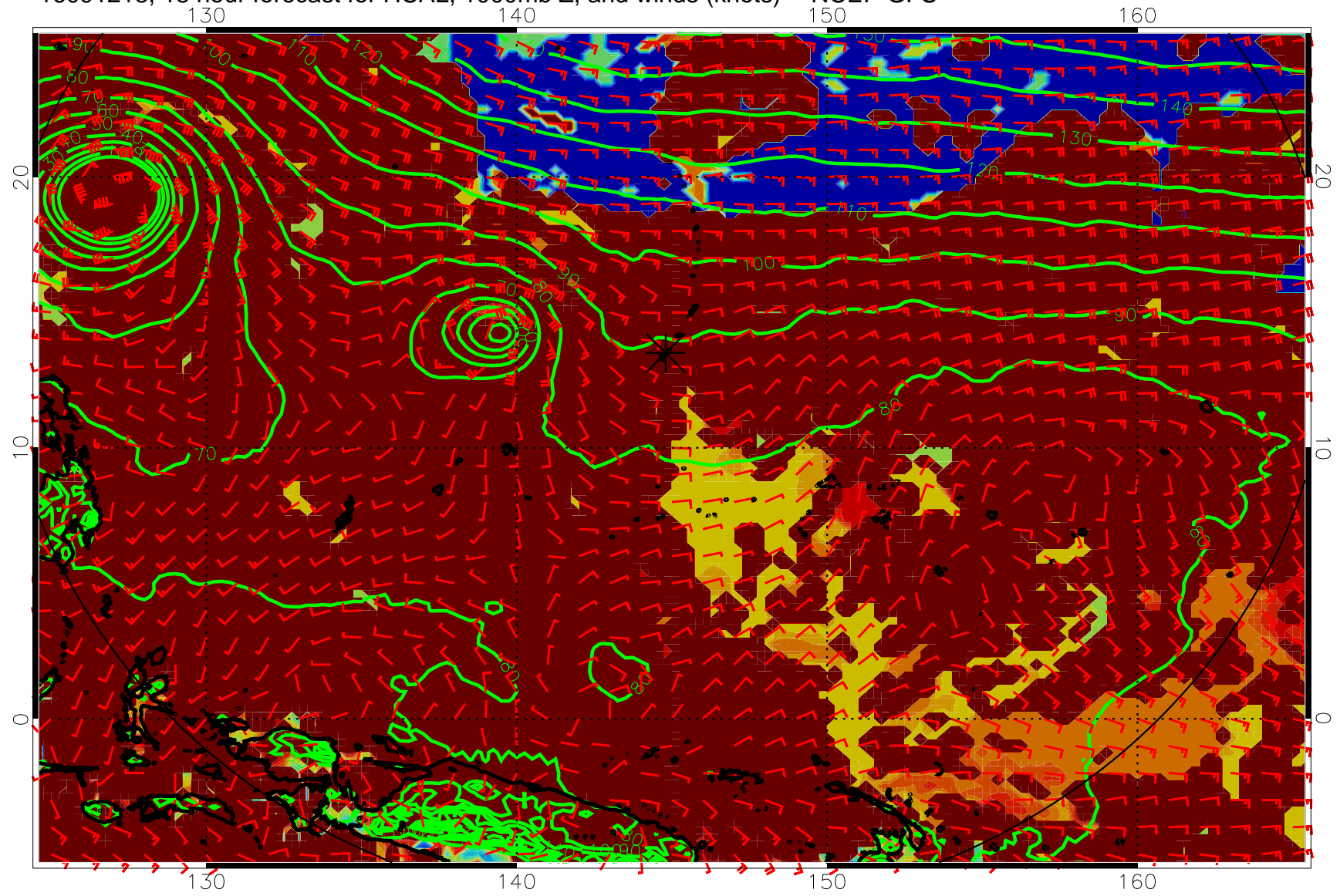
16091218, 18 hour forecast for HCAL, 1000mb Z, and winds (knots) -- NCEP GFS
