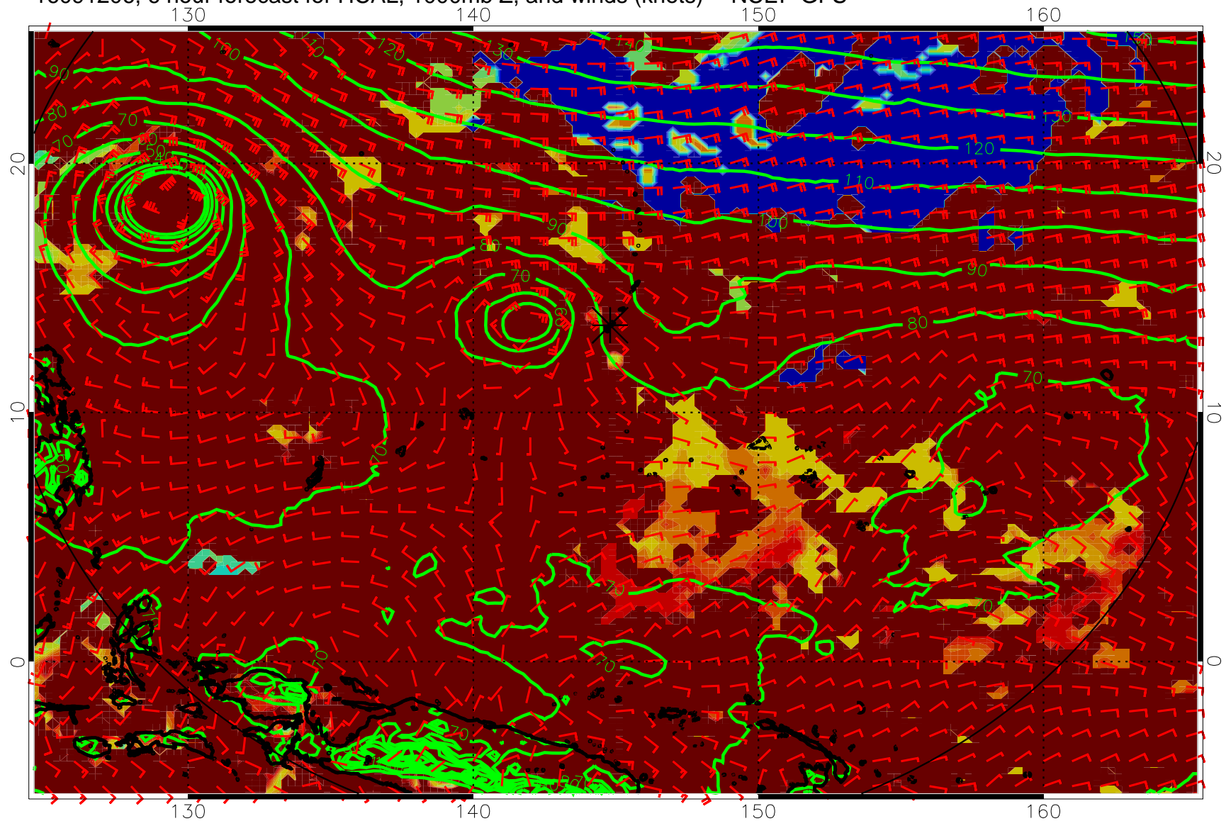
16091206, 6 hour forecast for HCAL, 1000mb Z, and winds (knots) -- NCEP GFS
