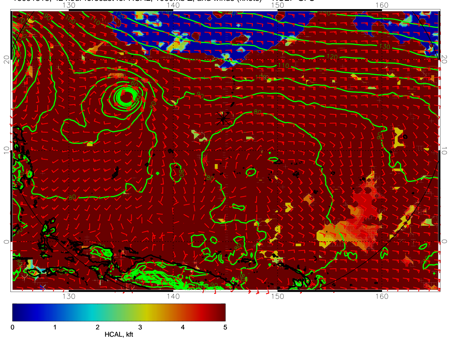
16091318, 42 hour forecast for HCAL, 1000mb Z, and winds (knots) -- NCEP GFS
