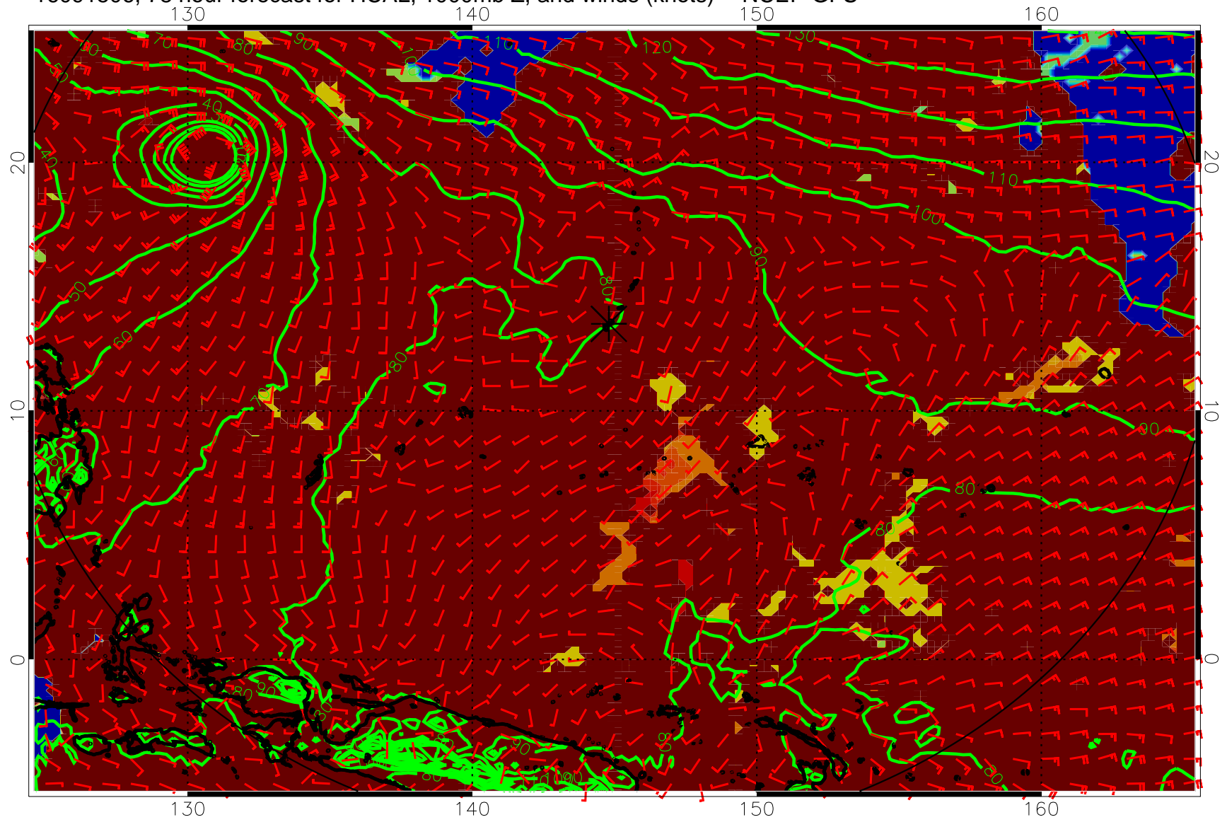
16091506, 78 hour forecast for HCAL, 1000mb Z, and winds (knots) -- NCEP GFS
