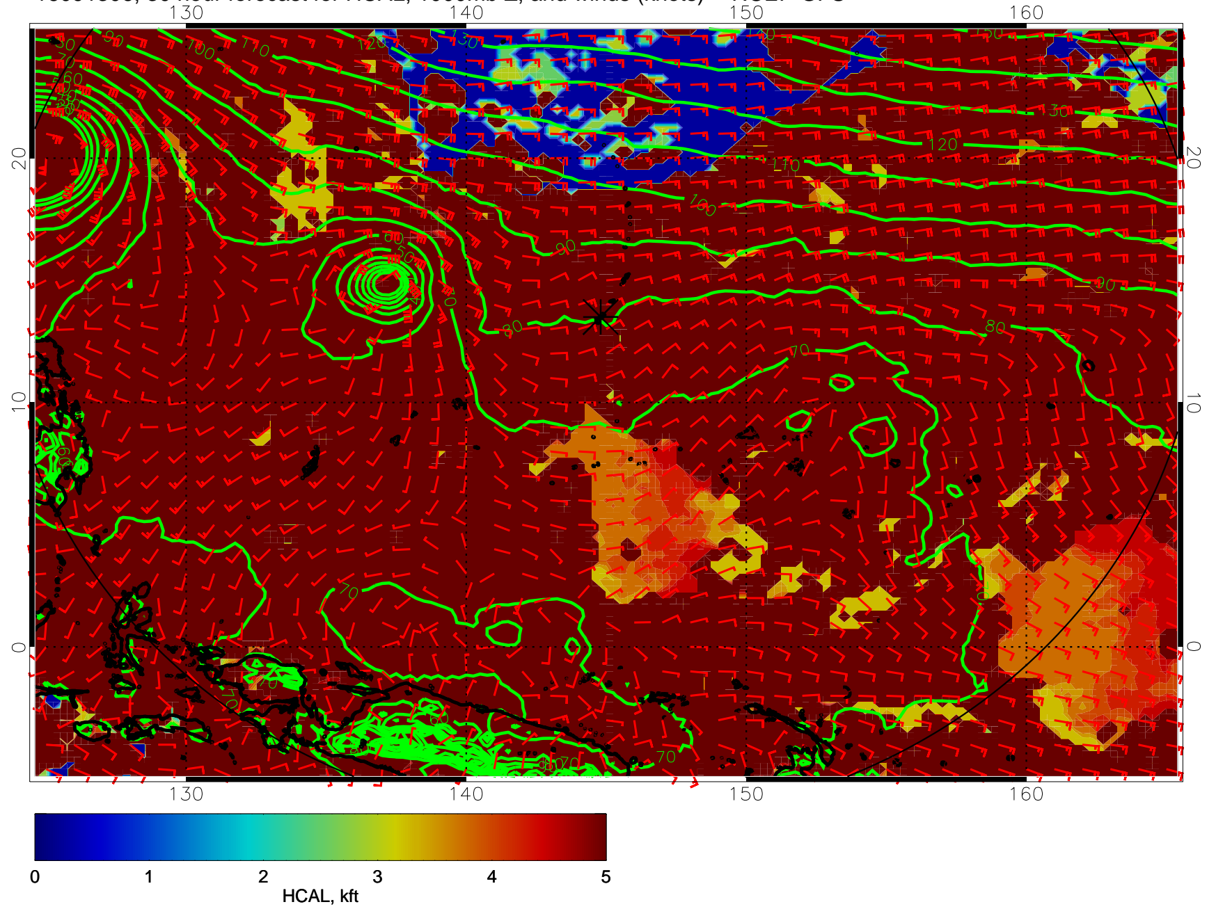
16091306, 30 hour forecast for HCAL, 1000mb Z, and winds (knots) -- NCEP GFS
