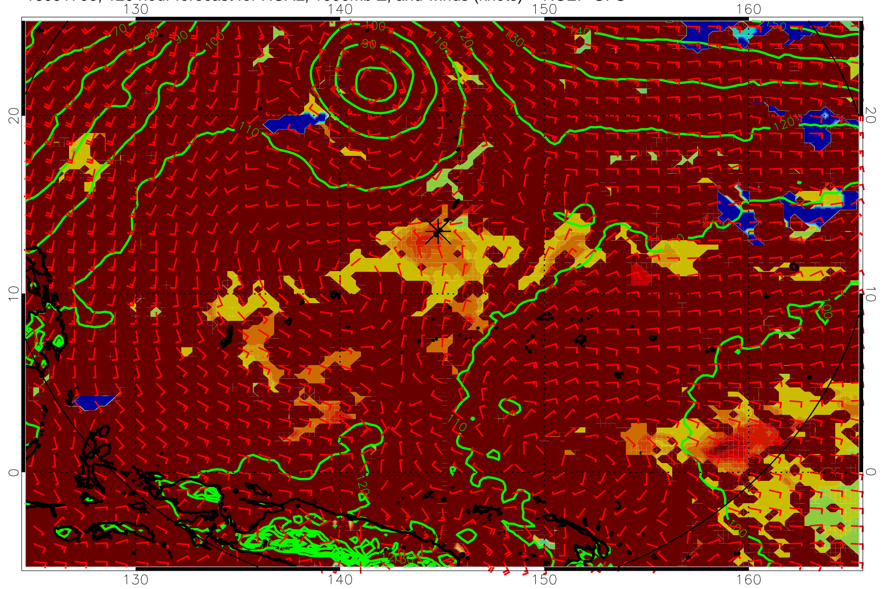
16091700, 120 hour forecast for HCAL, 1000mb Z, and winds (knots) -- NCEP GFS
