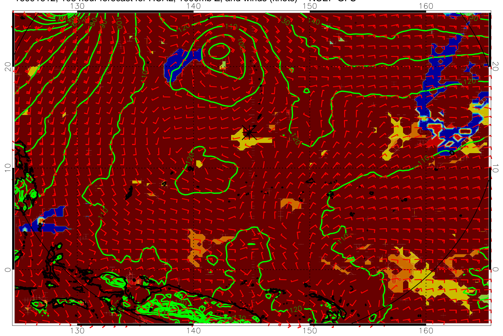
16091612, 108 hour forecast for HCAL, 1000mb Z, and winds (knots) -- NCEP GFS
