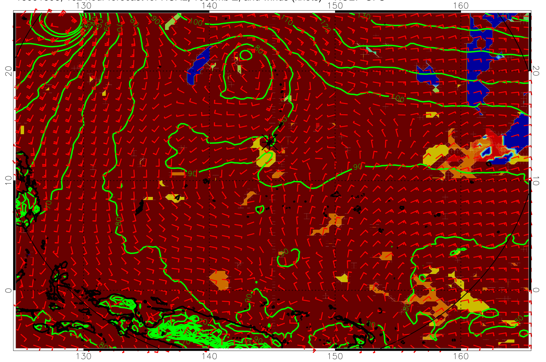
16091606, 102 hour forecast for HCAL, 1000mb Z, and winds (knots) -- NCEP GFS
