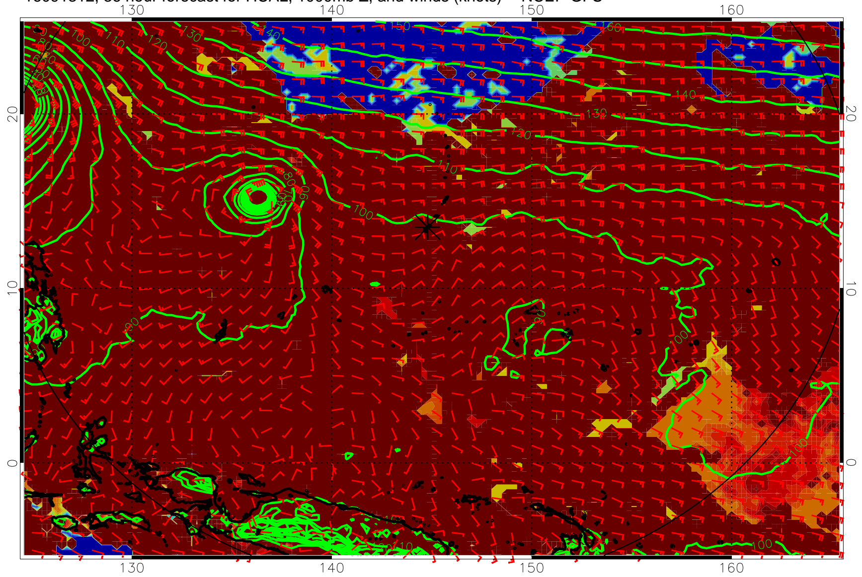
16091312, 36 hour forecast for HCAL, 1000mb Z, and winds (knots) -- NCEP GFS
