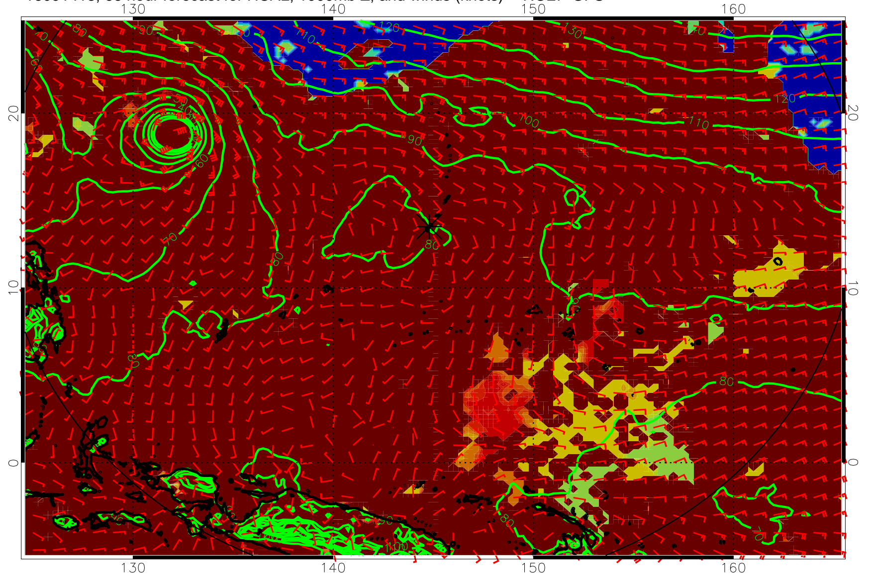
16091418, 66 hour forecast for HCAL, 1000mb Z, and winds (knots) -- NCEP GFS
