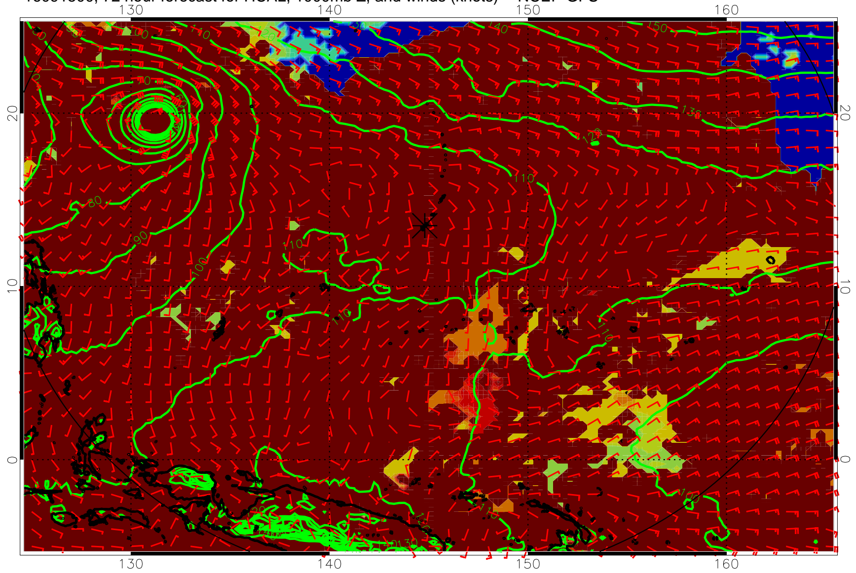
16091500, 72 hour forecast for HCAL, 1000mb Z, and winds (knots) -- NCEP GFS
