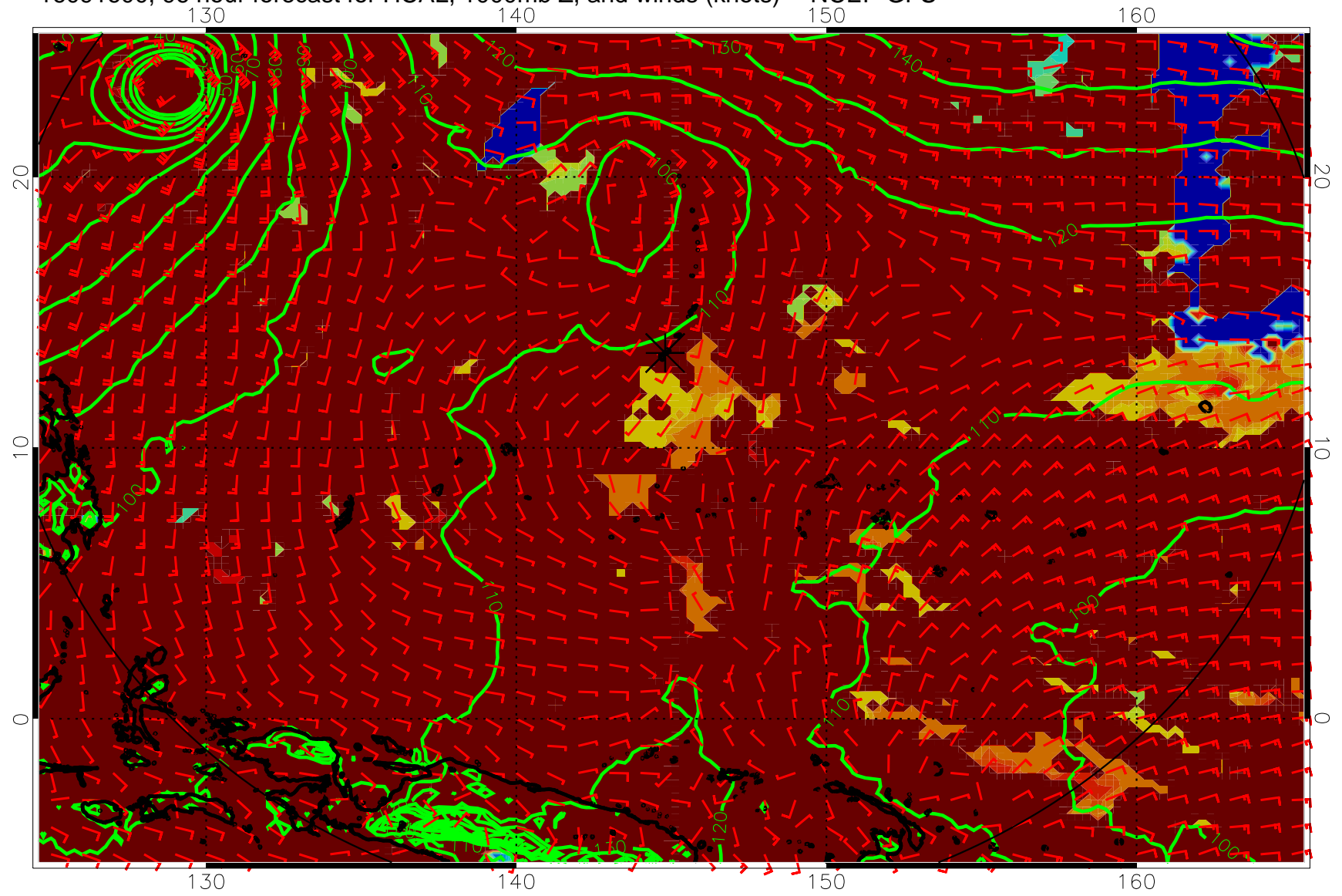
16091600, 96 hour forecast for HCAL, 1000mb Z, and winds (knots) -- NCEP GFS
