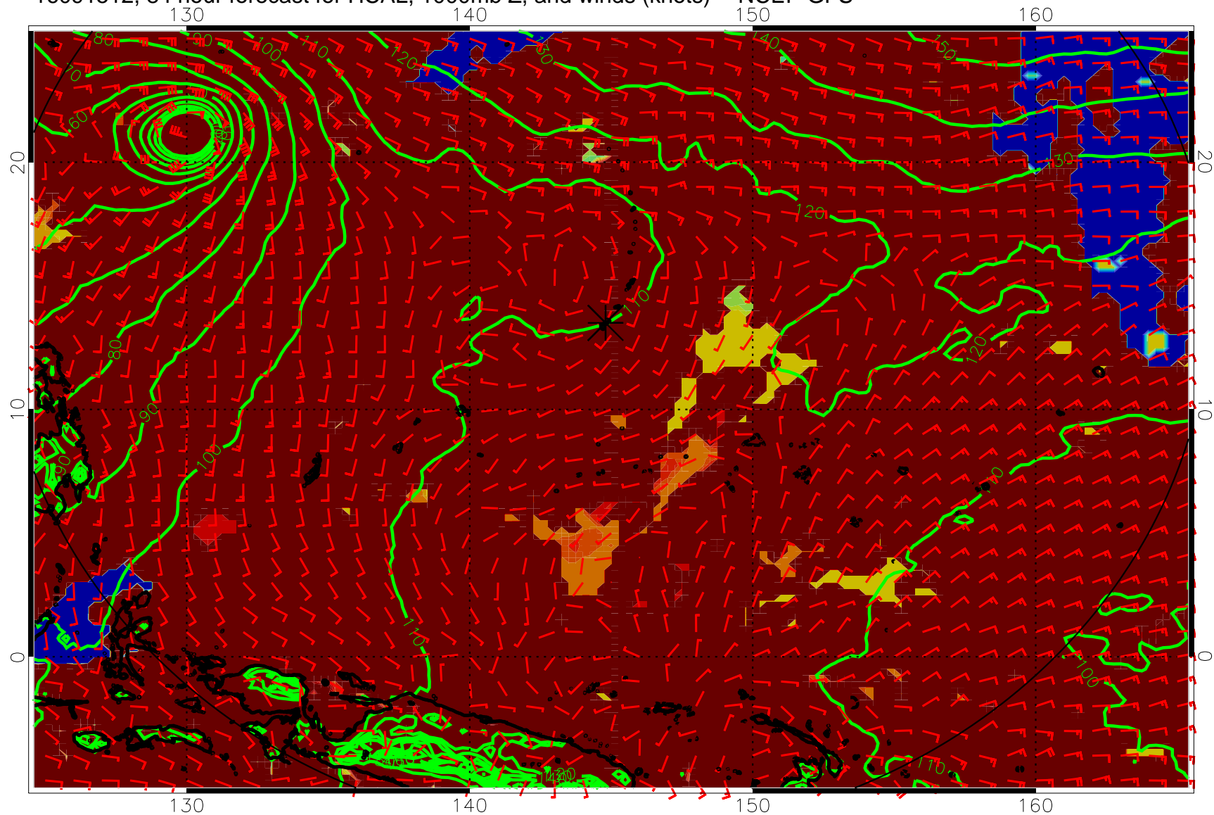
16091512, 84 hour forecast for HCAL, 1000mb Z, and winds (knots) -- NCEP GFS
