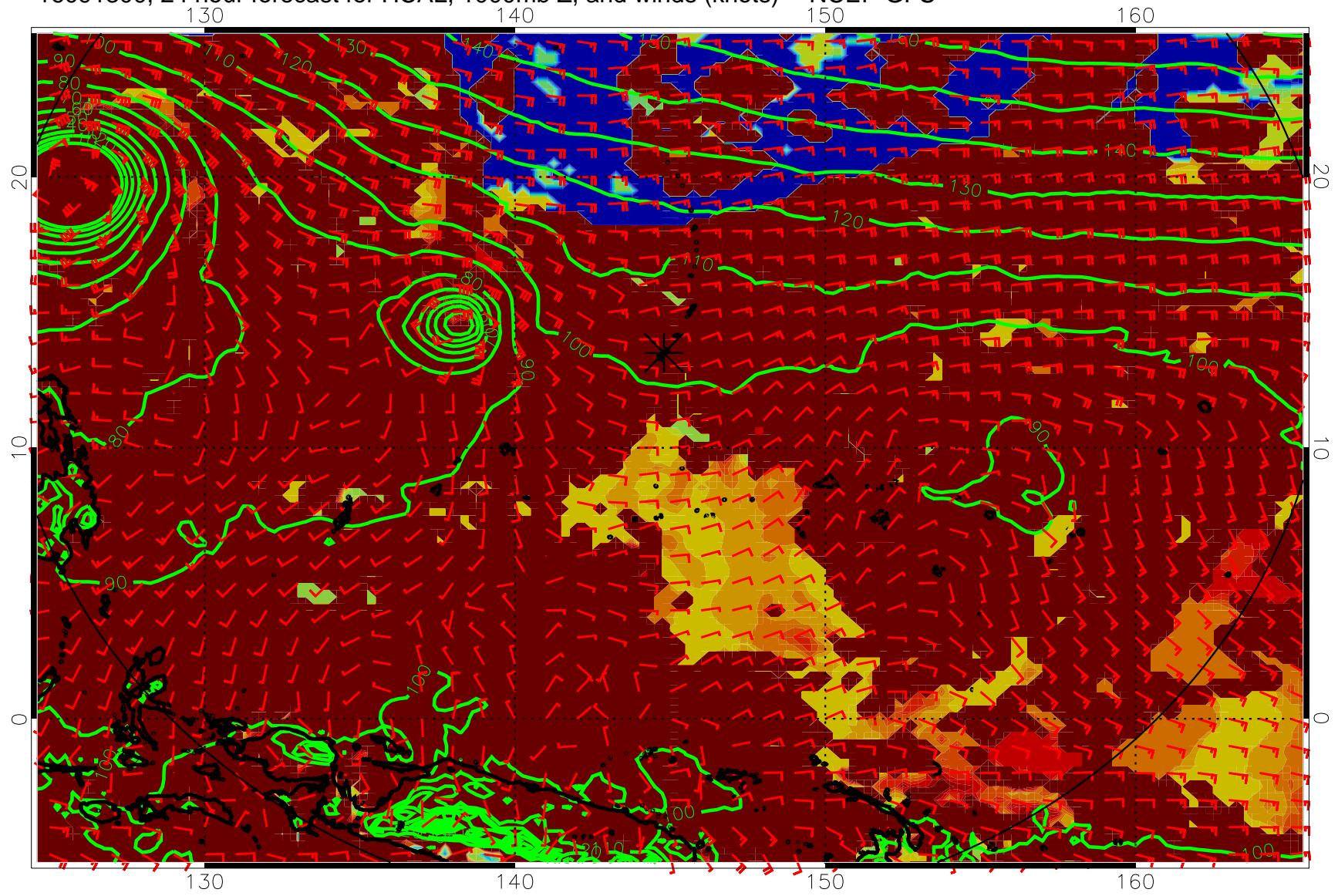
16091300, 24 hour forecast for HCAL, 1000mb Z, and winds (knots) -- NCEP GFS
