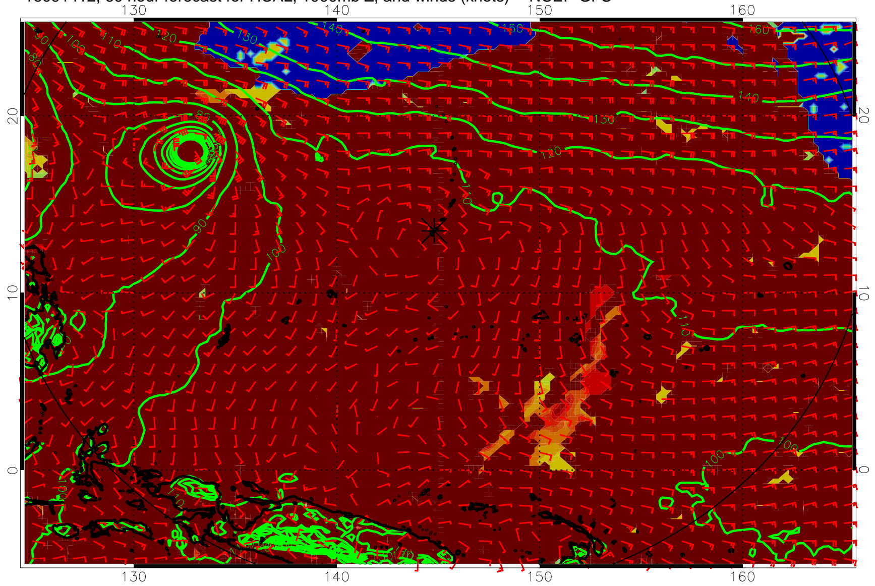
16091412, 60 hour forecast for HCAL, 1000mb Z, and winds (knots) -- NCEP GFS
