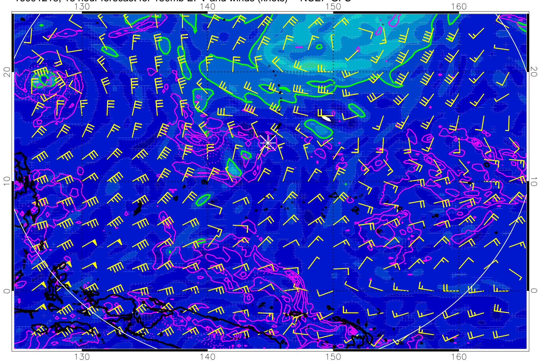
16091218, 18 hour forecast for 150mb EPV and winds (knots) -- NCEP GFS
