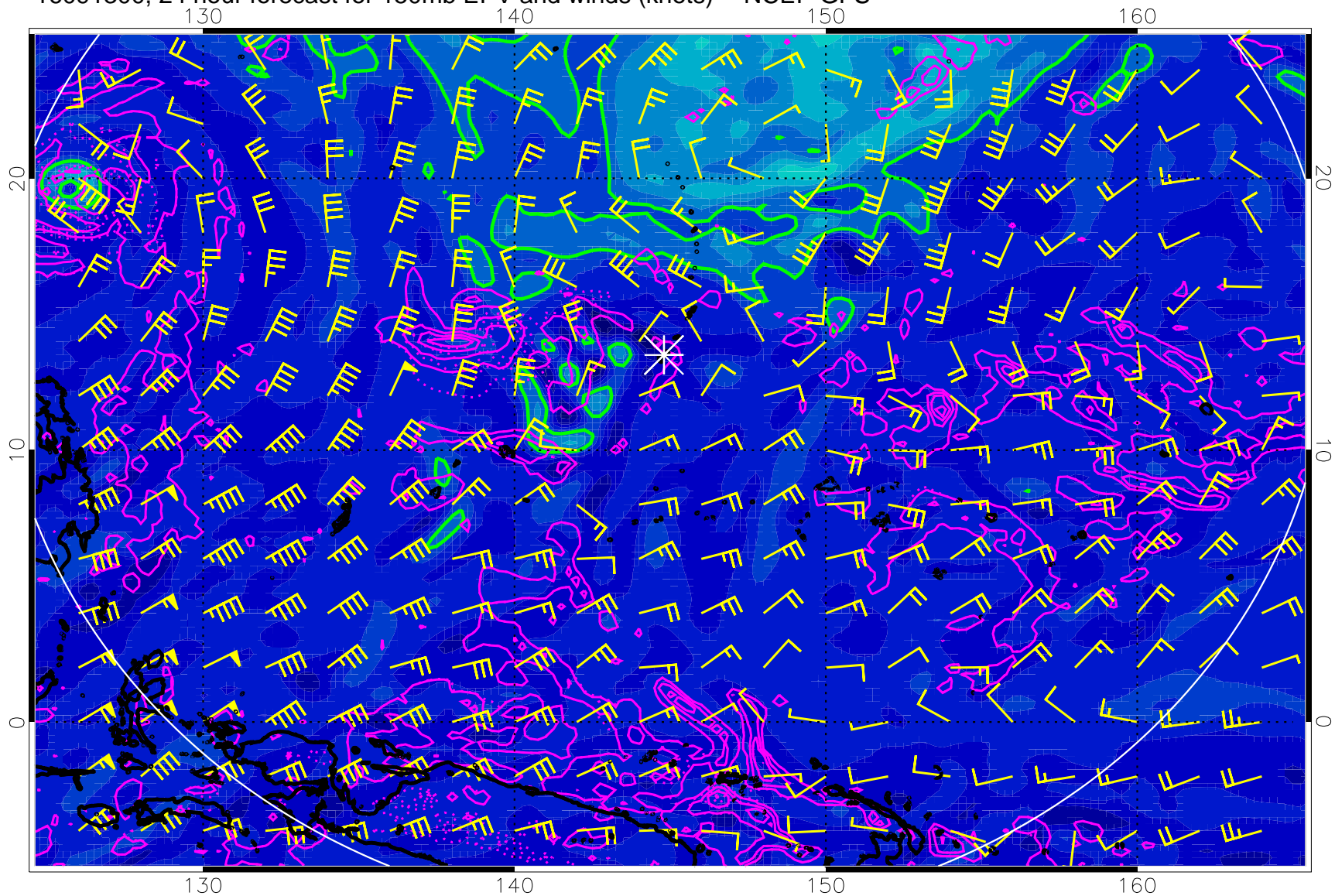
16091300, 24 hour forecast for 150mb EPV and winds (knots) -- NCEP GFS
