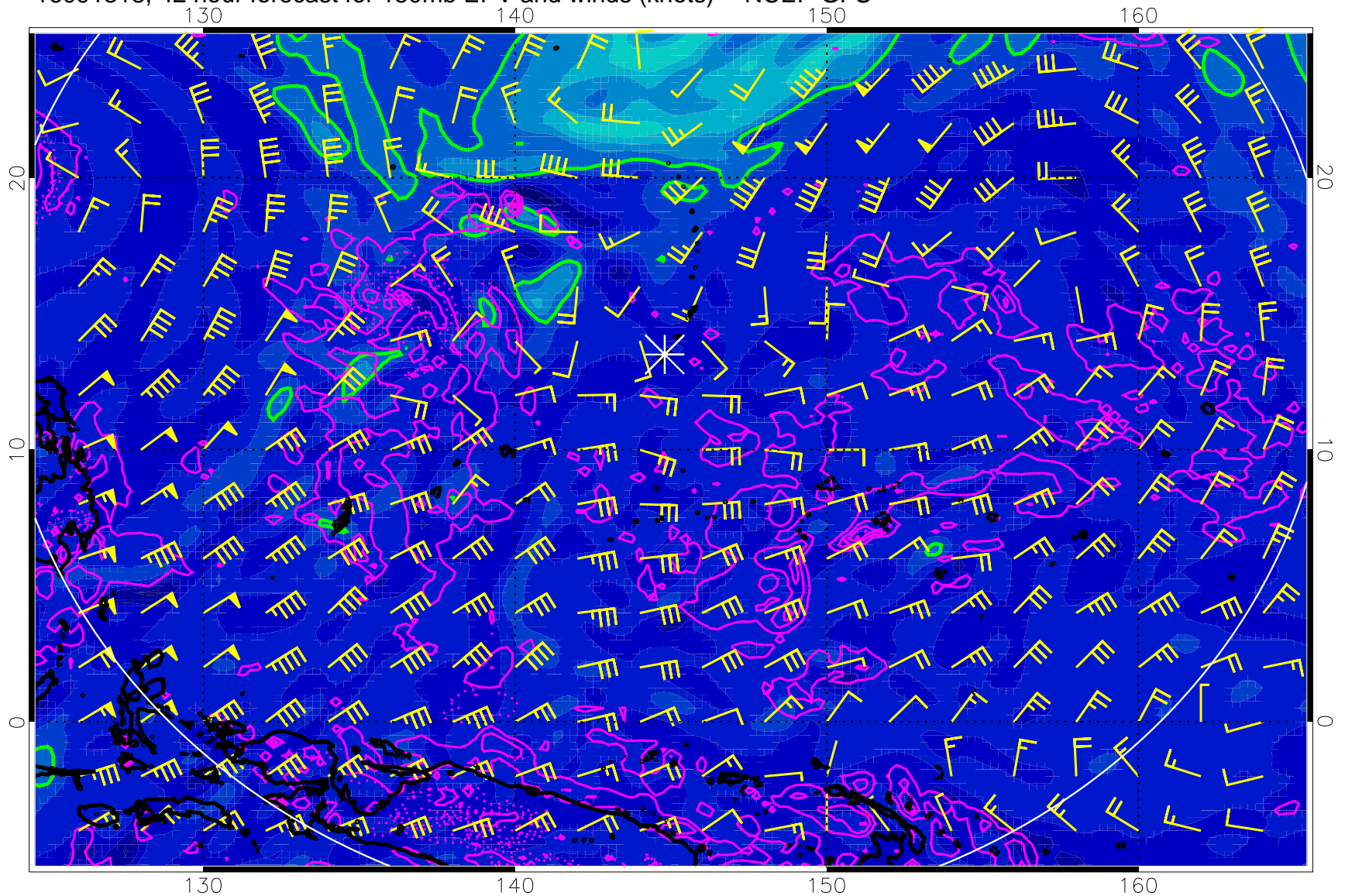
16091318, 42 hour forecast for 150mb EPV and winds (knots) -- NCEP GFS
