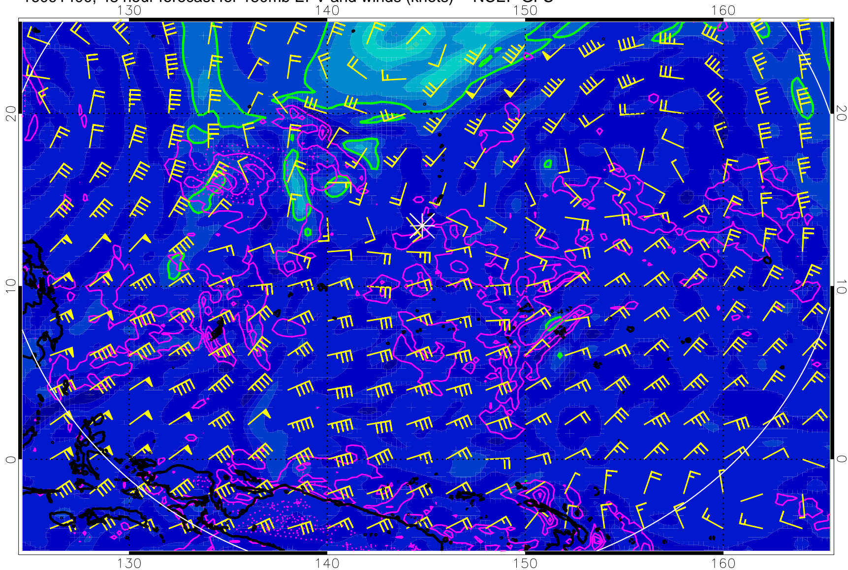
16091400, 48 hour forecast for 150mb EPV and winds (knots) -- NCEP GFS
