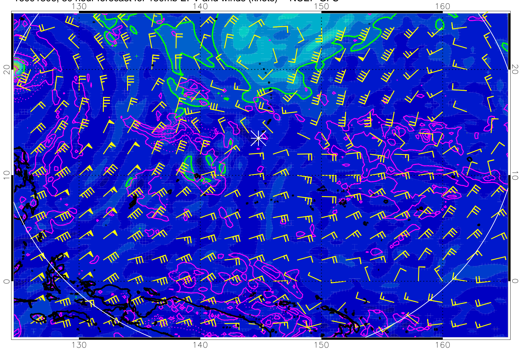
16091306, 30 hour forecast for 150mb EPV and winds (knots) -- NCEP GFS
