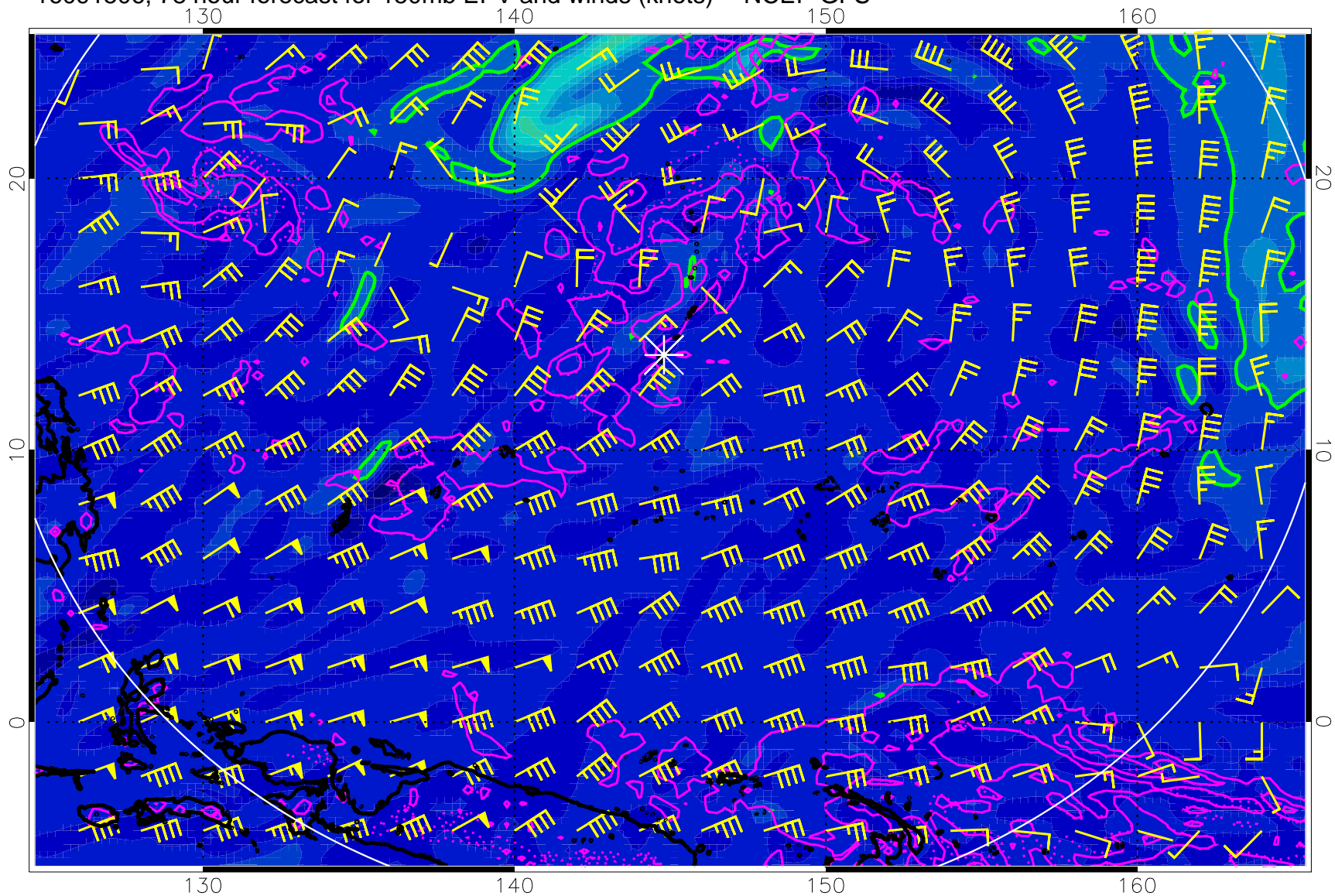
16091506, 78 hour forecast for 150mb EPV and winds (knots) -- NCEP GFS
