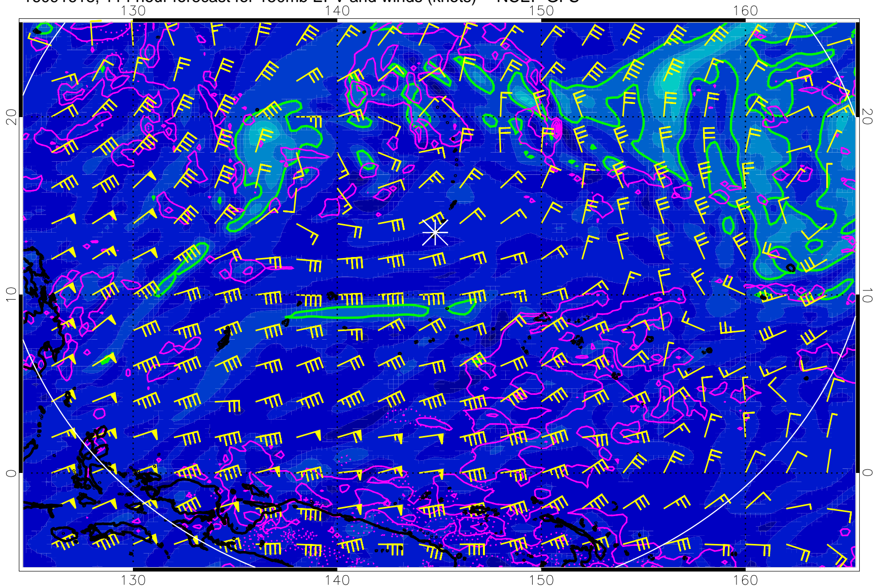
16091618, 114 hour forecast for 150mb EPV and winds (knots) -- NCEP GFS
