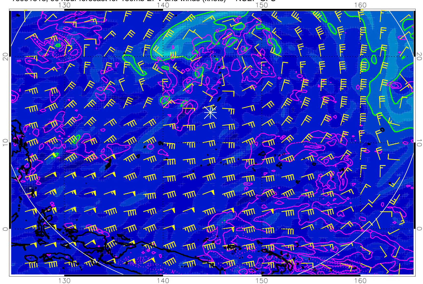
16091518, 90 hour forecast for 150mb EPV and winds (knots) -- NCEP GFS
