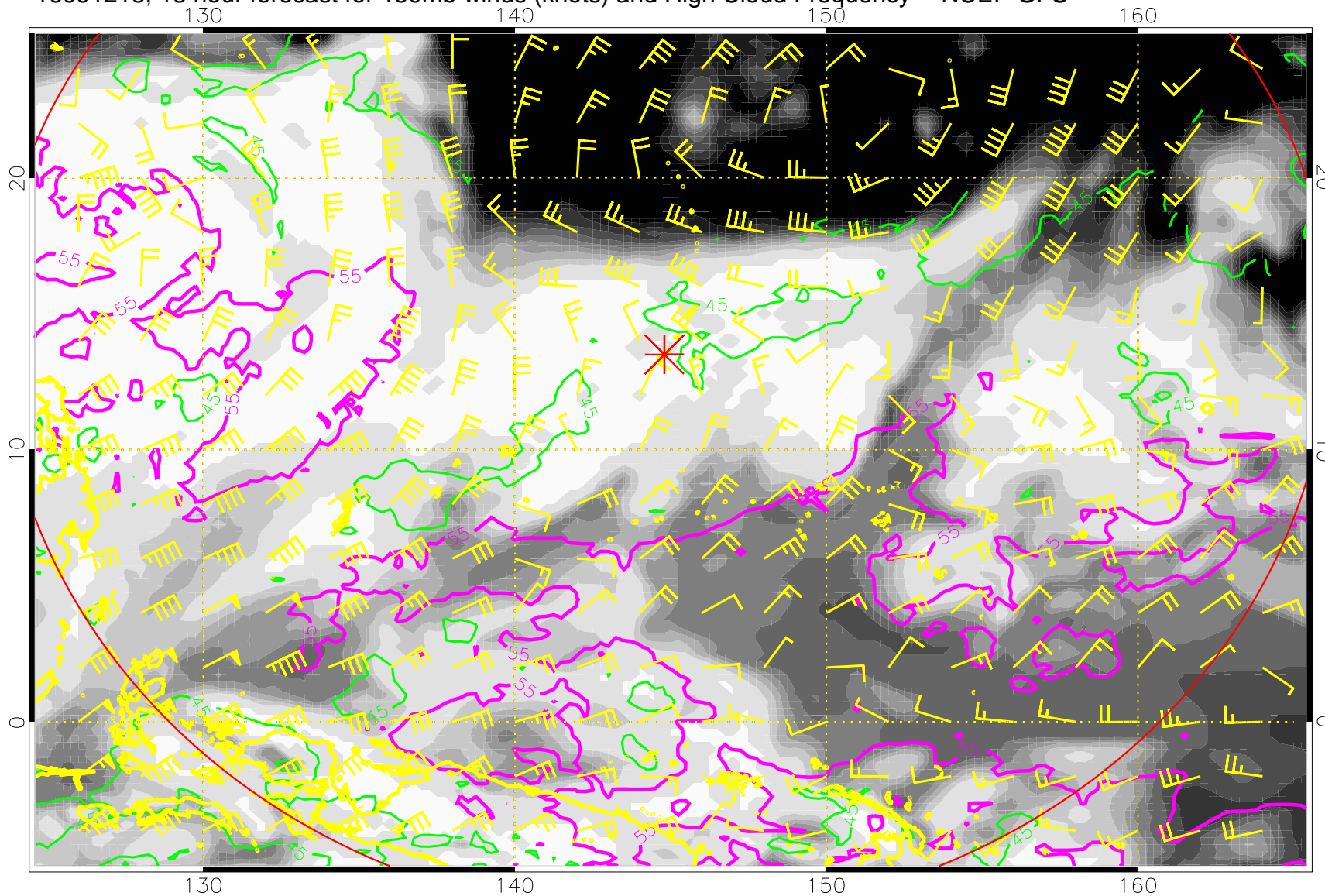
16091218, 18 hour forecast for 150mb winds (knots) and High Cloud Frequency -- NCEP GFS
