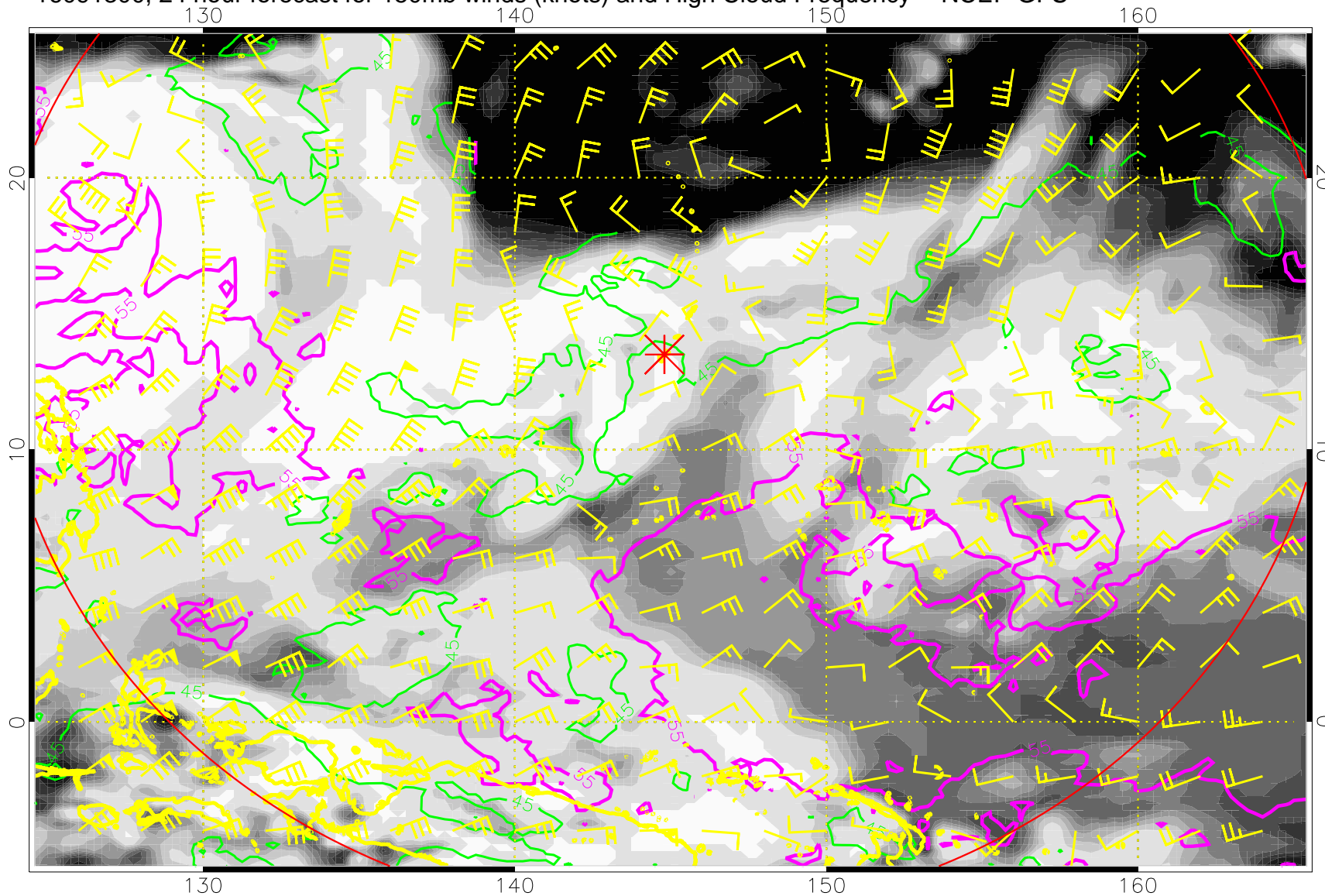
16091300, 24 hour forecast for 150mb winds (knots) and High Cloud Frequency -- NCEP GFS
