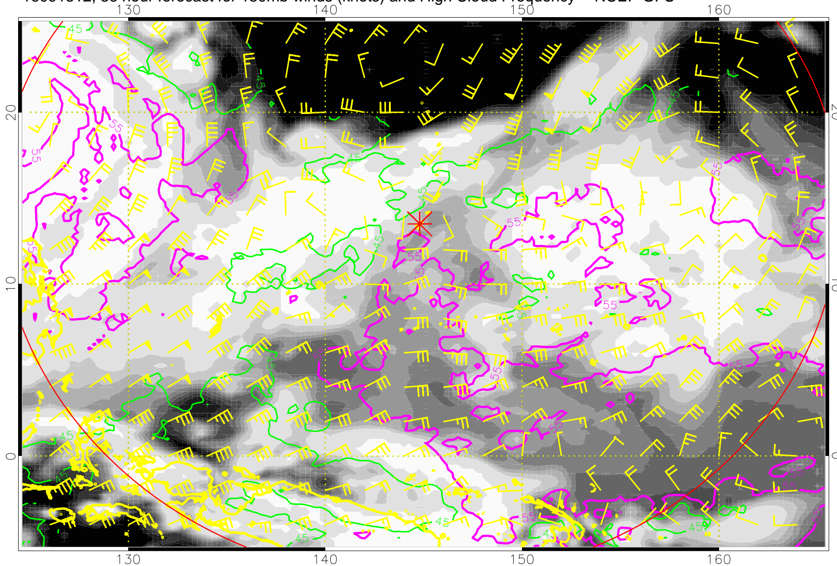
16091312, 36 hour forecast for 150mb winds (knots) and High Cloud Frequency -- NCEP GFS
