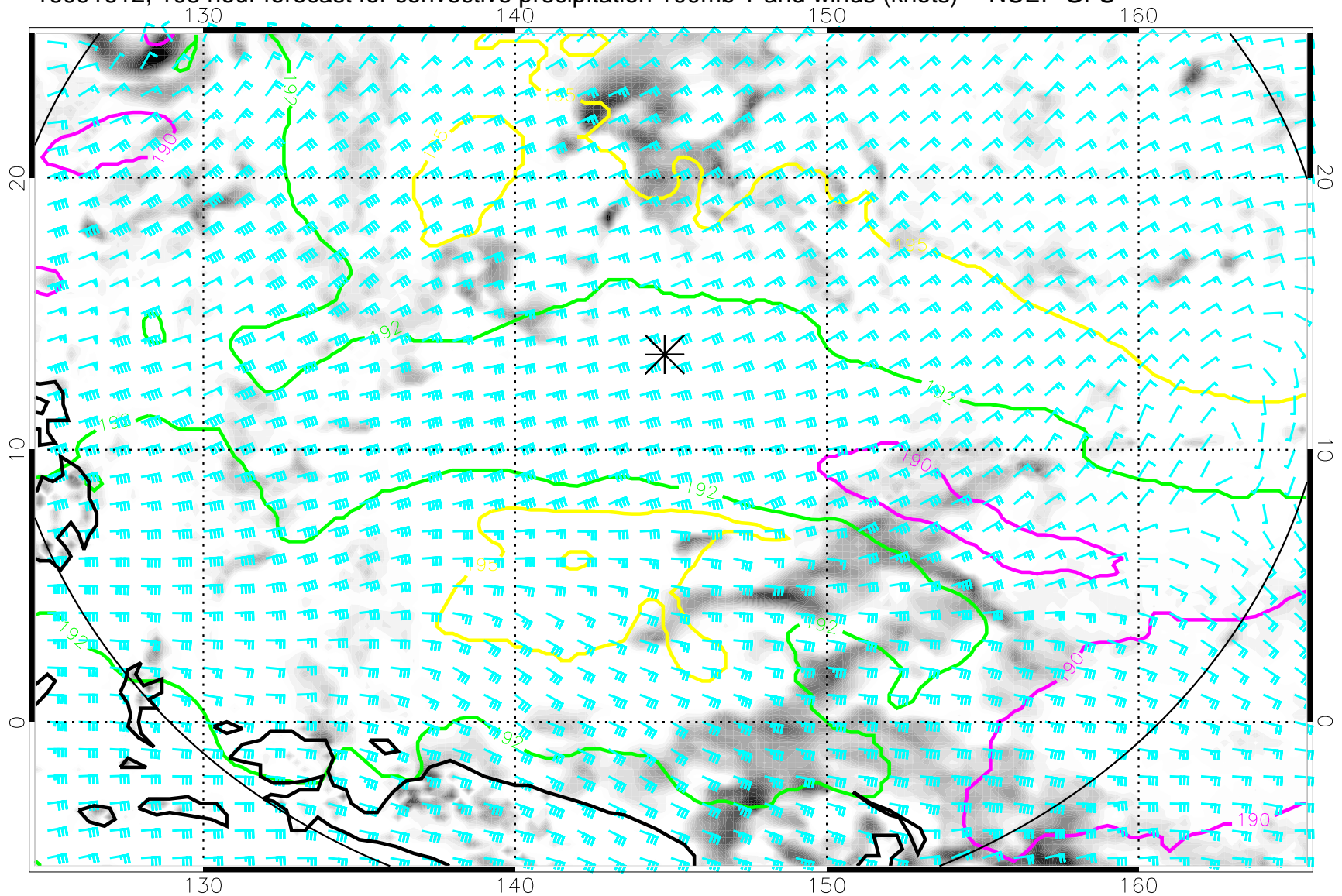
16091612, 108 hour forecast for convective precipitation 100mb T and winds (knots) -- NCEP GFS
