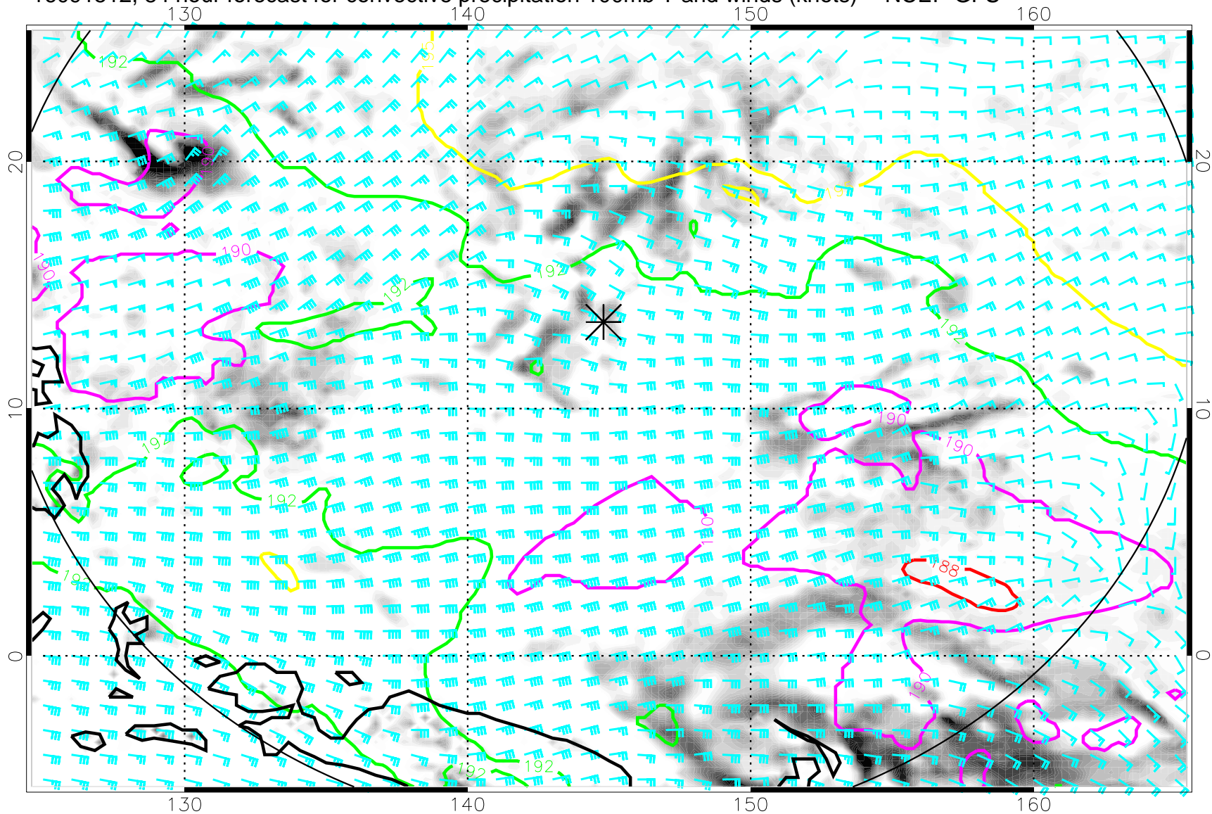
16091512, 84 hour forecast for convective precipitation 100mb T and winds (knots) -- NCEP GFS
