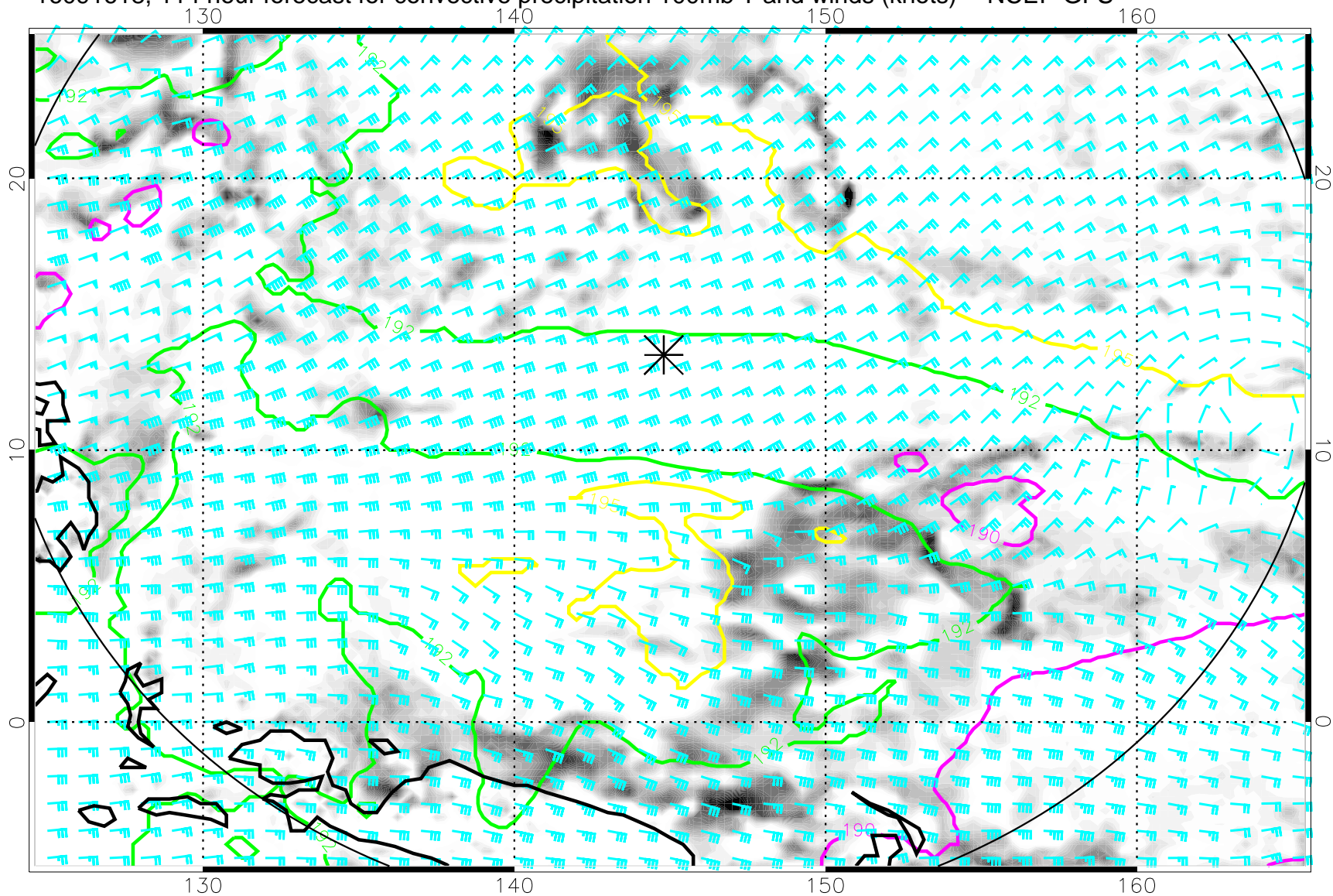
16091618, 114 hour forecast for convective precipitation 100mb T and winds (knots) -- NCEP GFS
