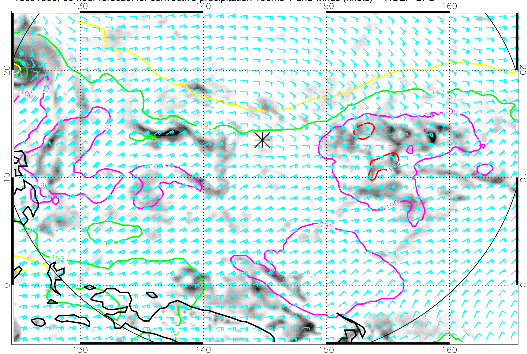
16091306, 30 hour forecast for convective precipitation 100mb T and winds (knots) -- NCEP GFS
