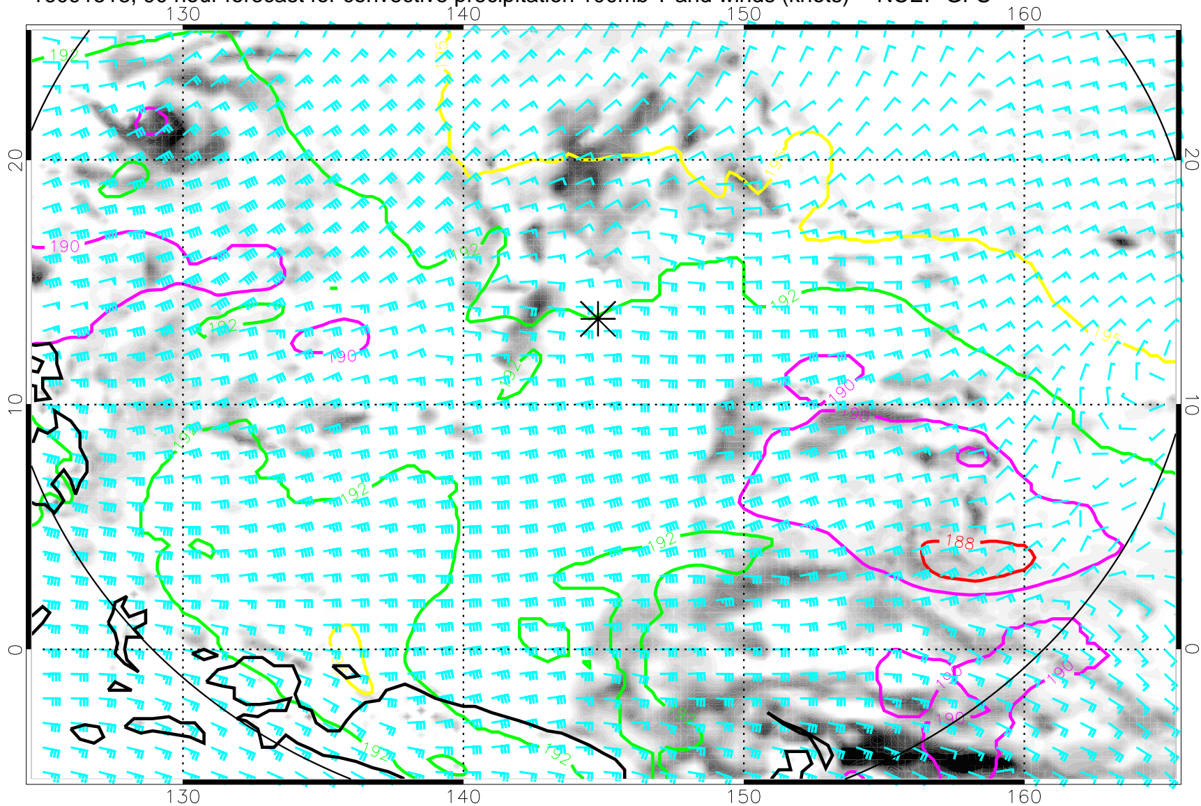
16091518, 90 hour forecast for convective precipitation 100mb T and winds (knots) -- NCEP GFS
