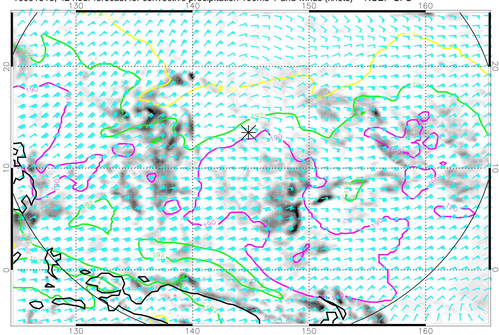
16091318, 42 hour forecast for convective precipitation 100mb T and winds (knots) -- NCEP GFS
