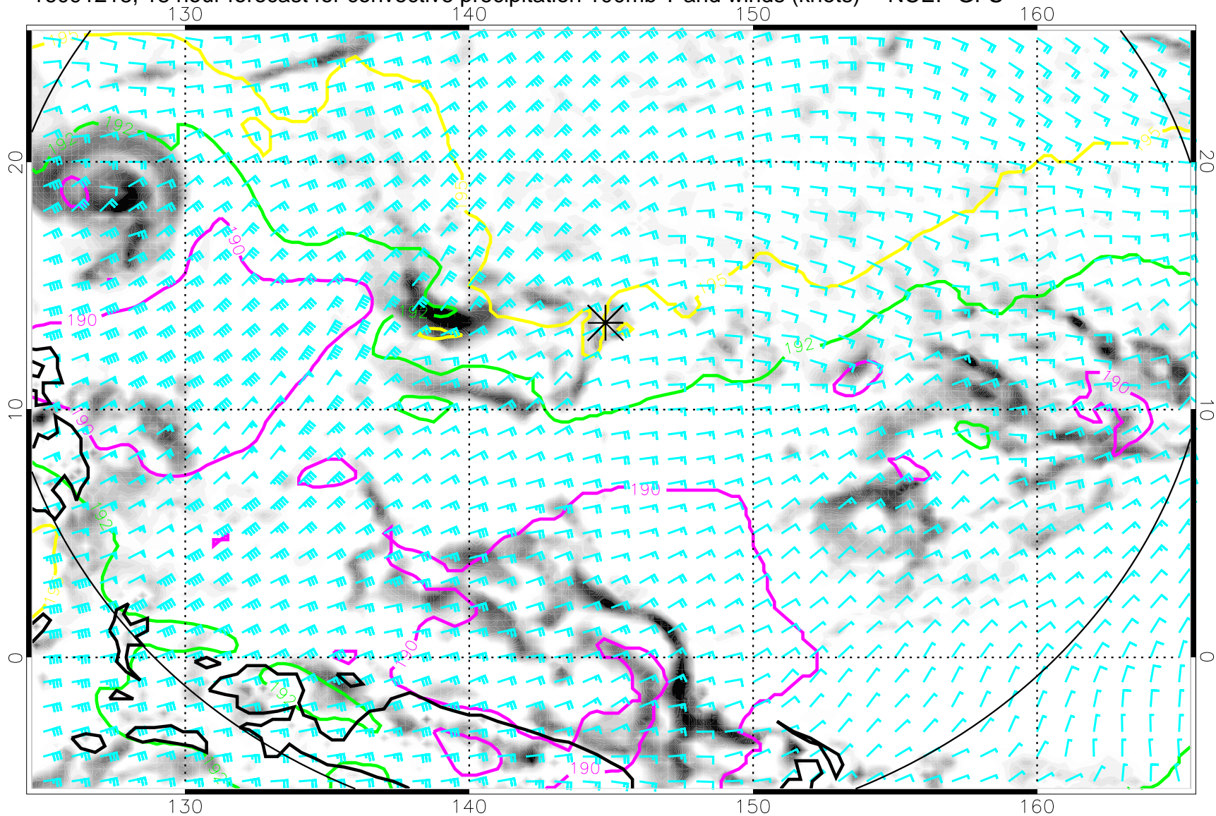
16091218, 18 hour forecast for convective precipitation 100mb T and winds (knots) -- NCEP GFS
