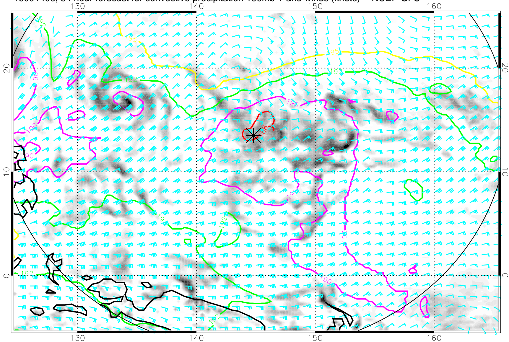
16091406, 54 hour forecast for convective precipitation 100mb T and winds (knots) -- NCEP GFS
