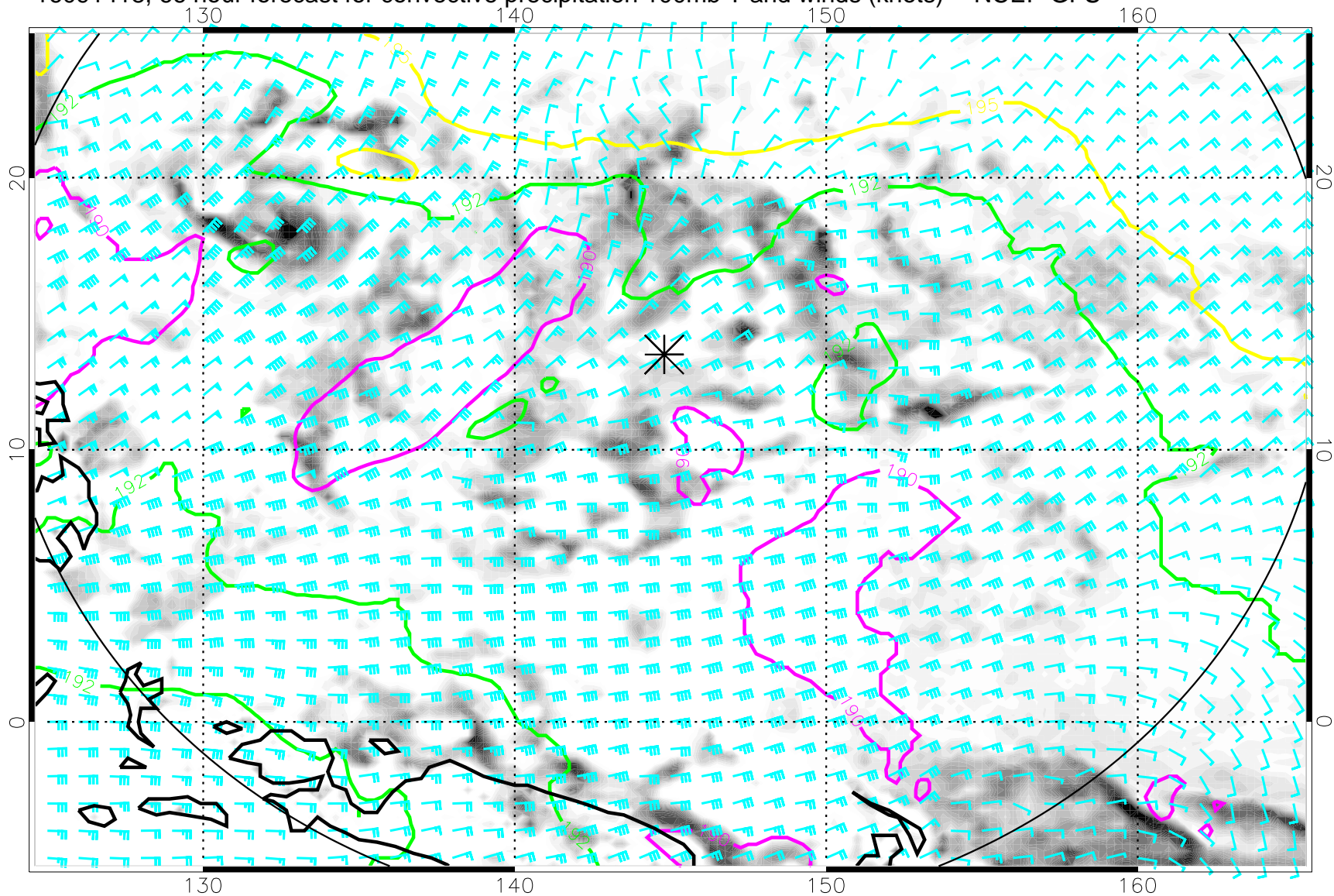
16091418, 66 hour forecast for convective precipitation 100mb T and winds (knots) -- NCEP GFS
