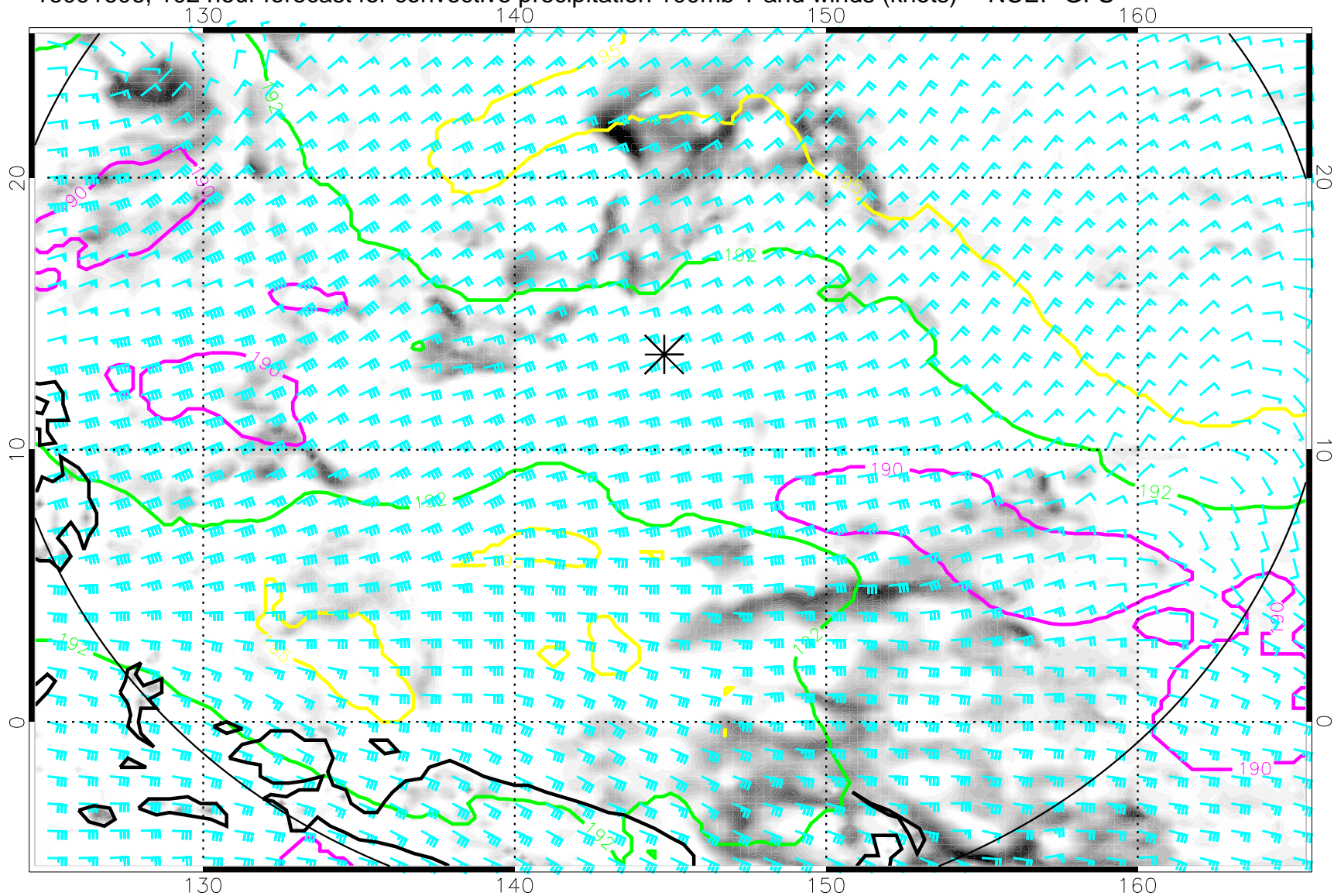
16091606, 102 hour forecast for convective precipitation 100mb T and winds (knots) -- NCEP GFS
