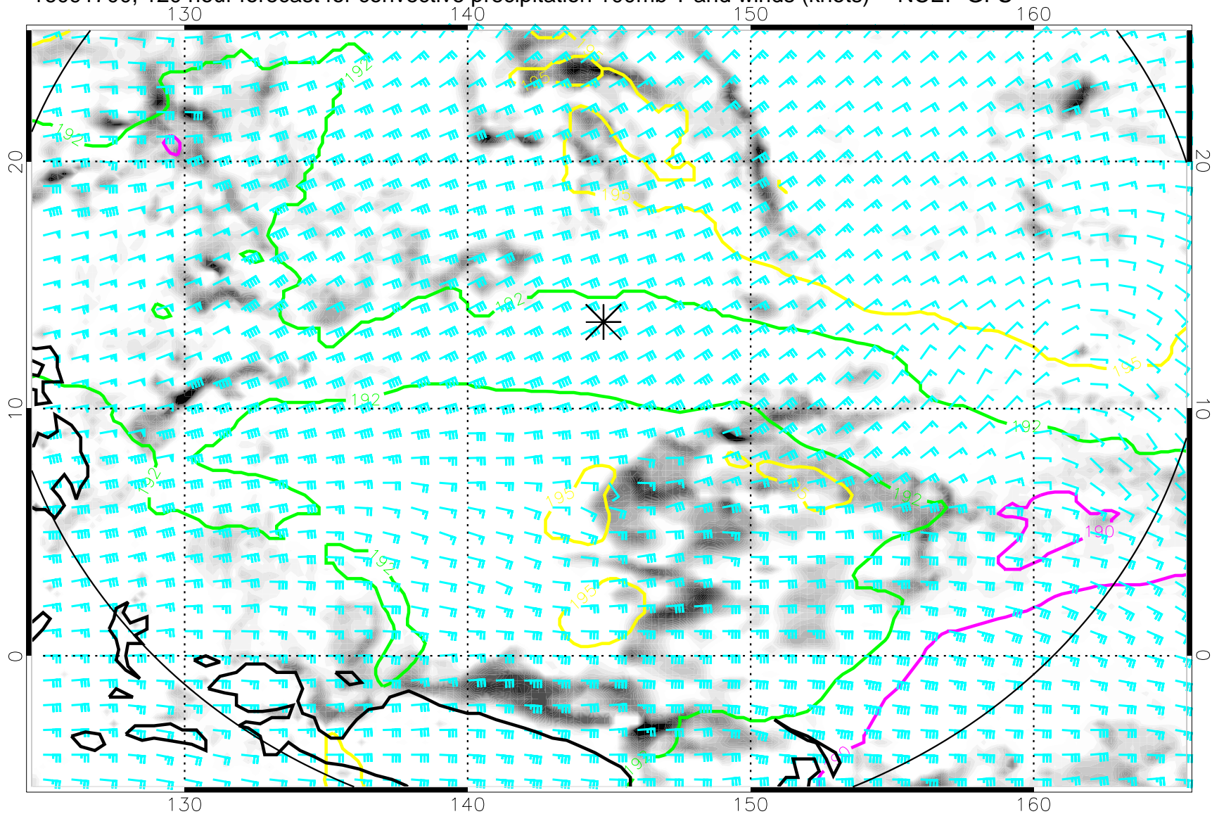
16091700, 120 hour forecast for convective precipitation 100mb T and winds (knots) -- NCEP GFS
