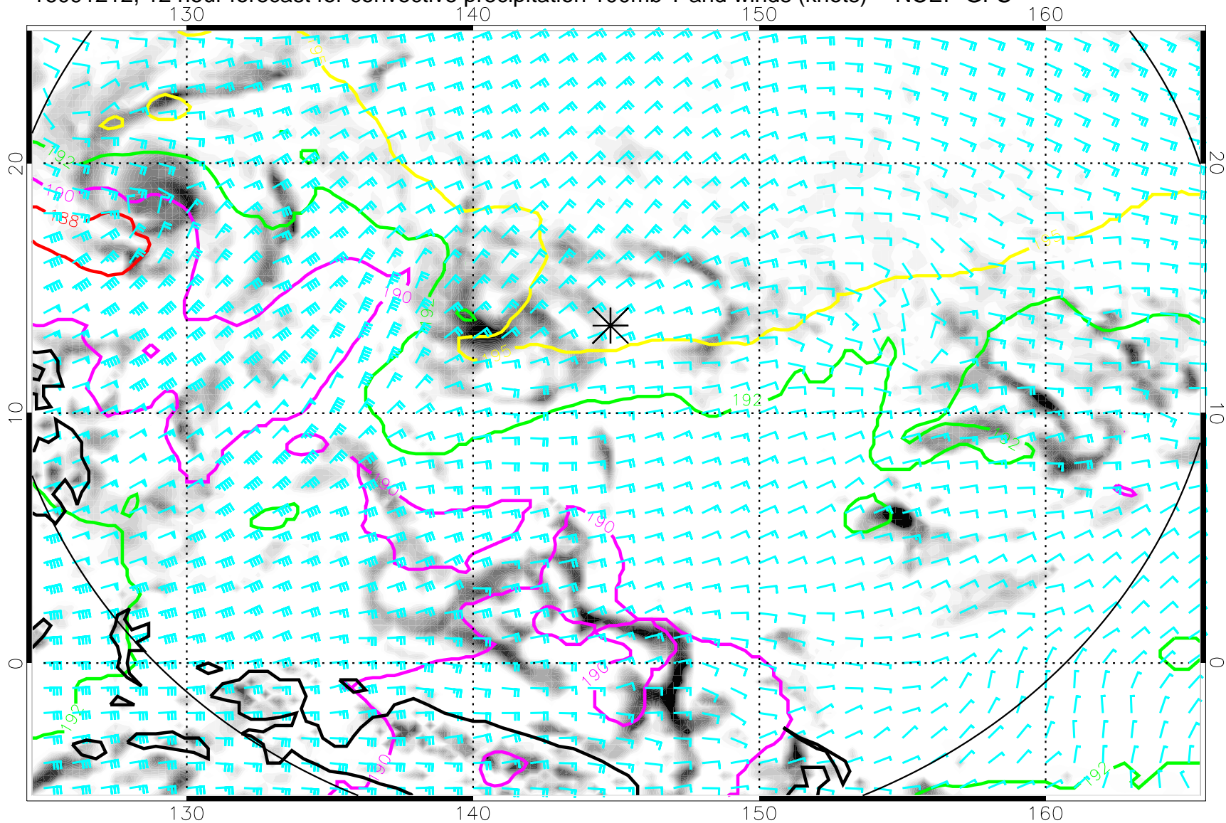
16091212, 12 hour forecast for convective precipitation 100mb T and winds (knots) -- NCEP GFS
