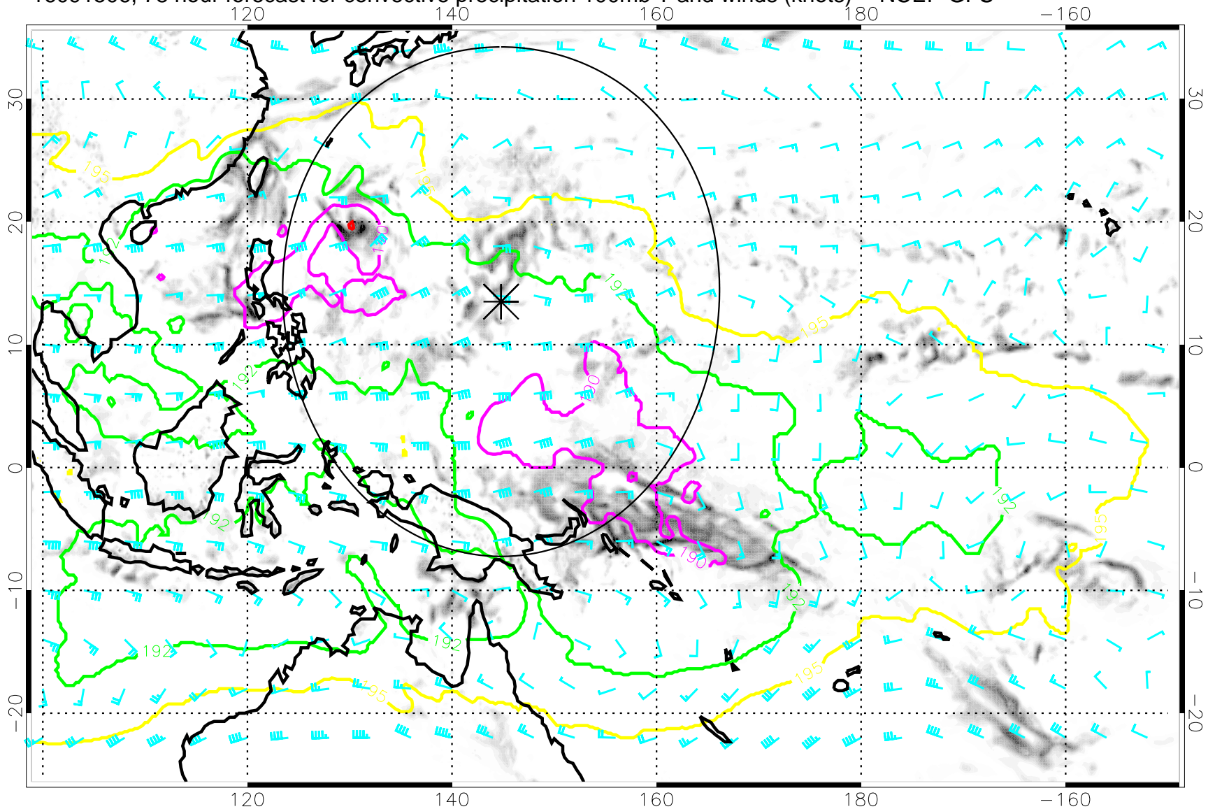
16091506, 78 hour forecast for convective precipitation 100mb T and winds (knots) -- NCEP GFS
