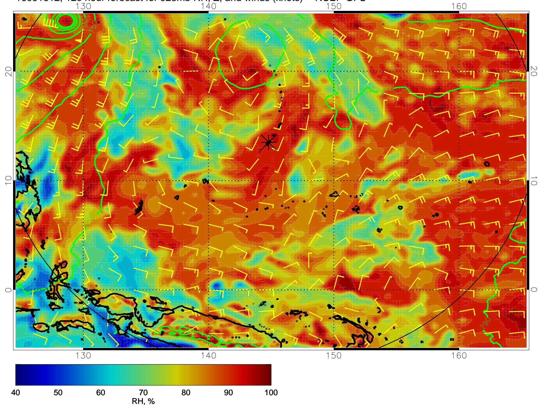
16091612, 120 hour forecast for 925mb RH, Z, and winds (knots) -- NCEP GFS
