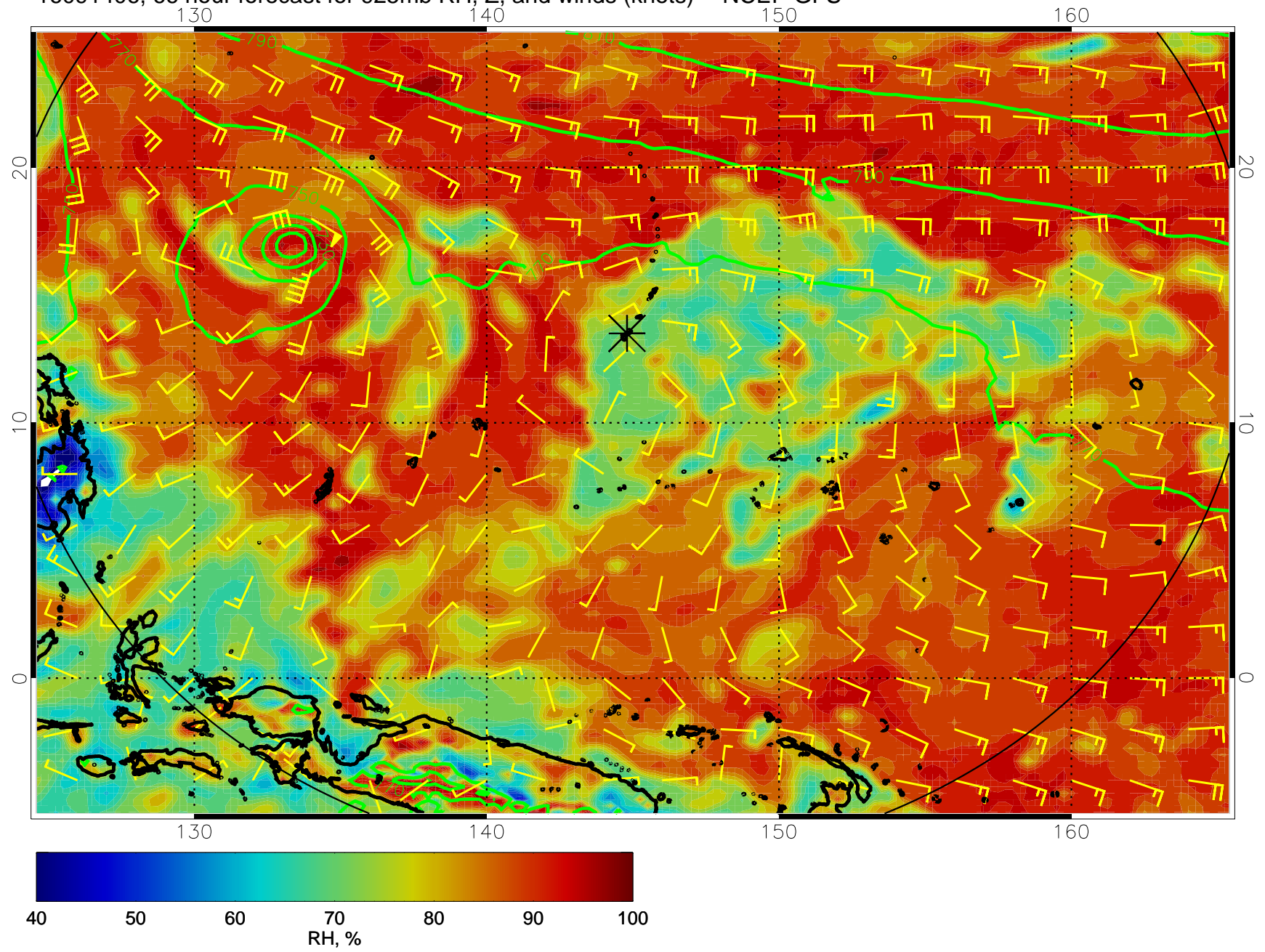
16091406, 66 hour forecast for 925mb RH, Z, and winds (knots) -- NCEP GFS
