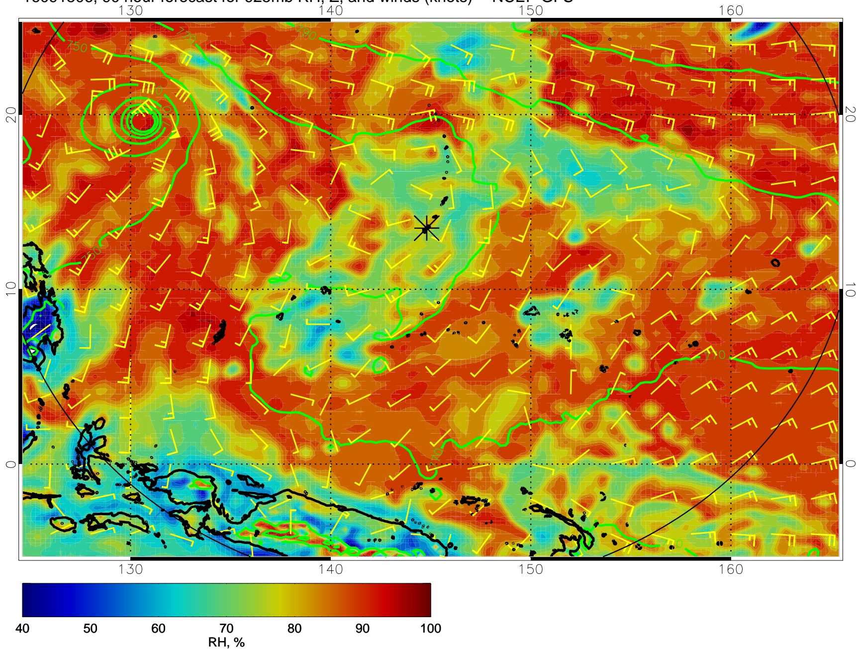
16091506, 90 hour forecast for 925mb RH, Z, and winds (knots) -- NCEP GFS
