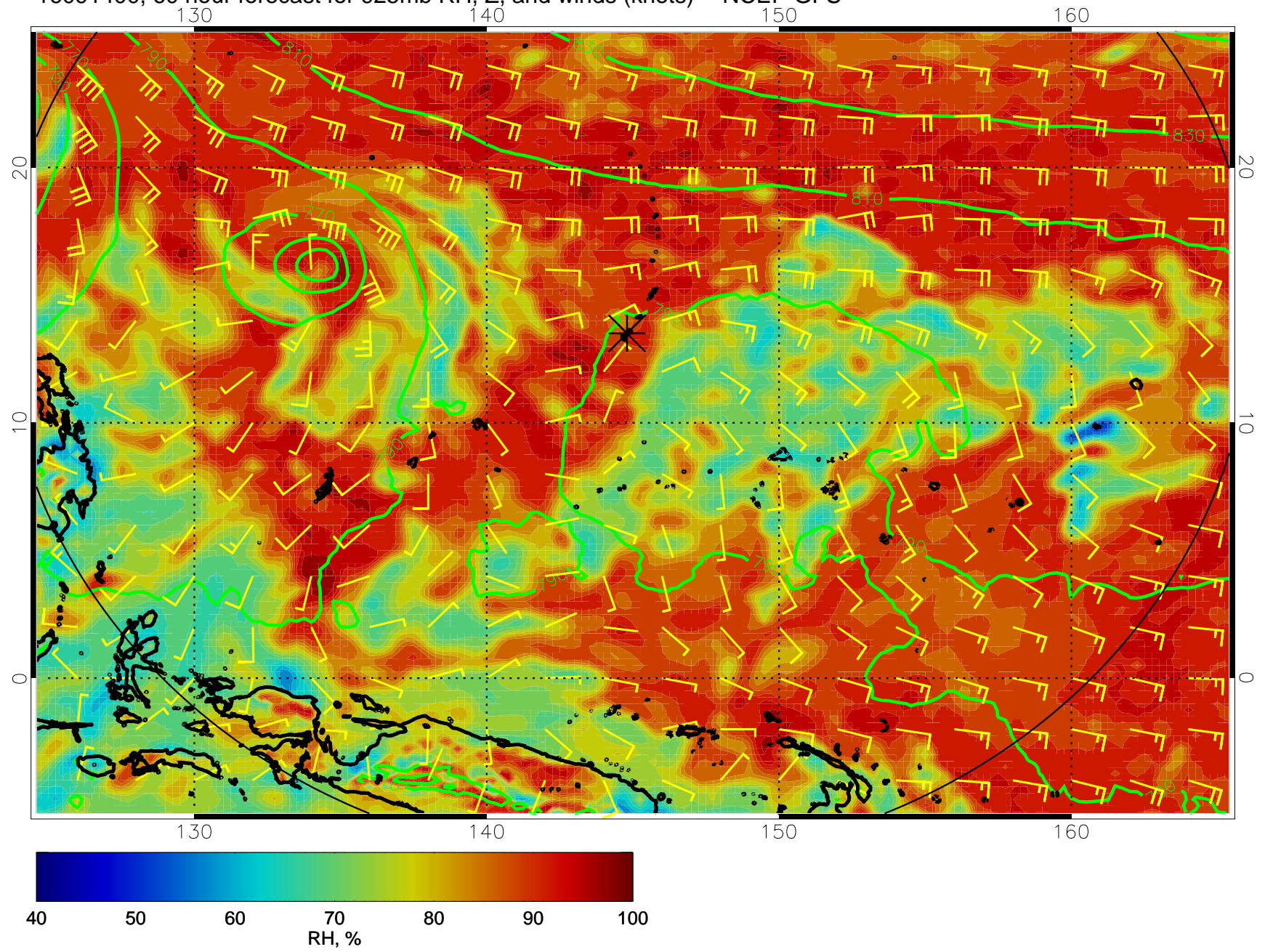
16091400, 60 hour forecast for 925mb RH, Z, and winds (knots) -- NCEP GFS
