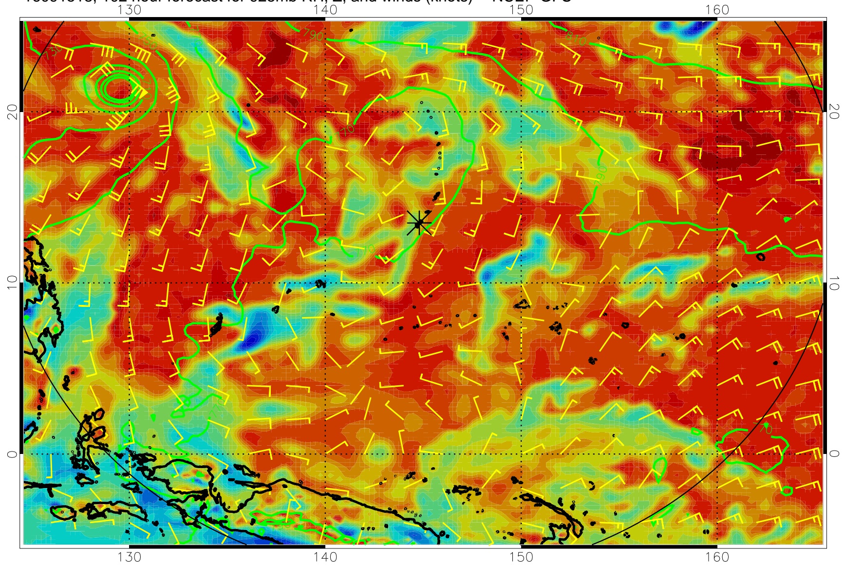
16091518, 102 hour forecast for 925mb RH, Z, and winds (knots) -- NCEP GFS
