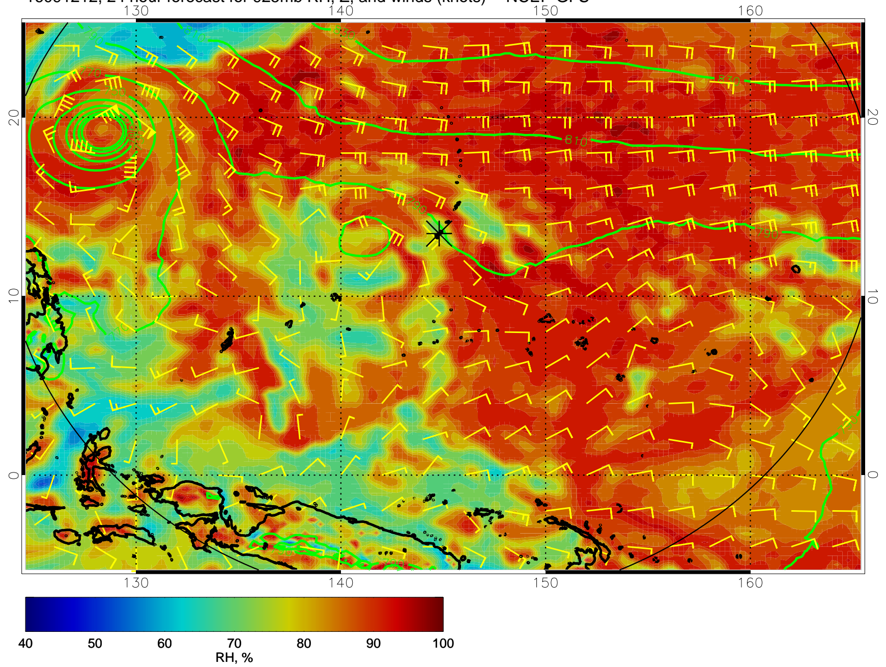
16091212, 24 hour forecast for 925mb RH, Z, and winds (knots) -- NCEP GFS
