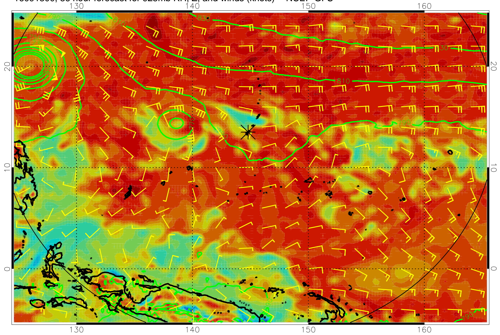
16091300, 36 hour forecast for 925mb RH, Z, and winds (knots) -- NCEP GFS
