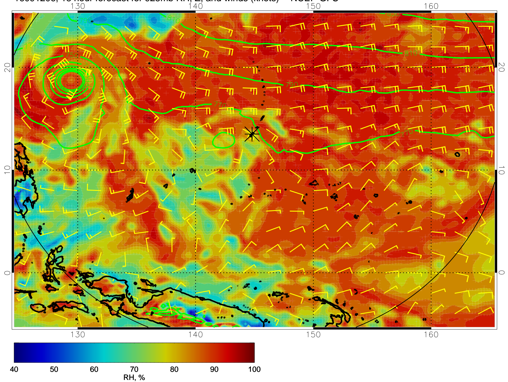
16091206, 18 hour forecast for 925mb RH, Z, and winds (knots) -- NCEP GFS
