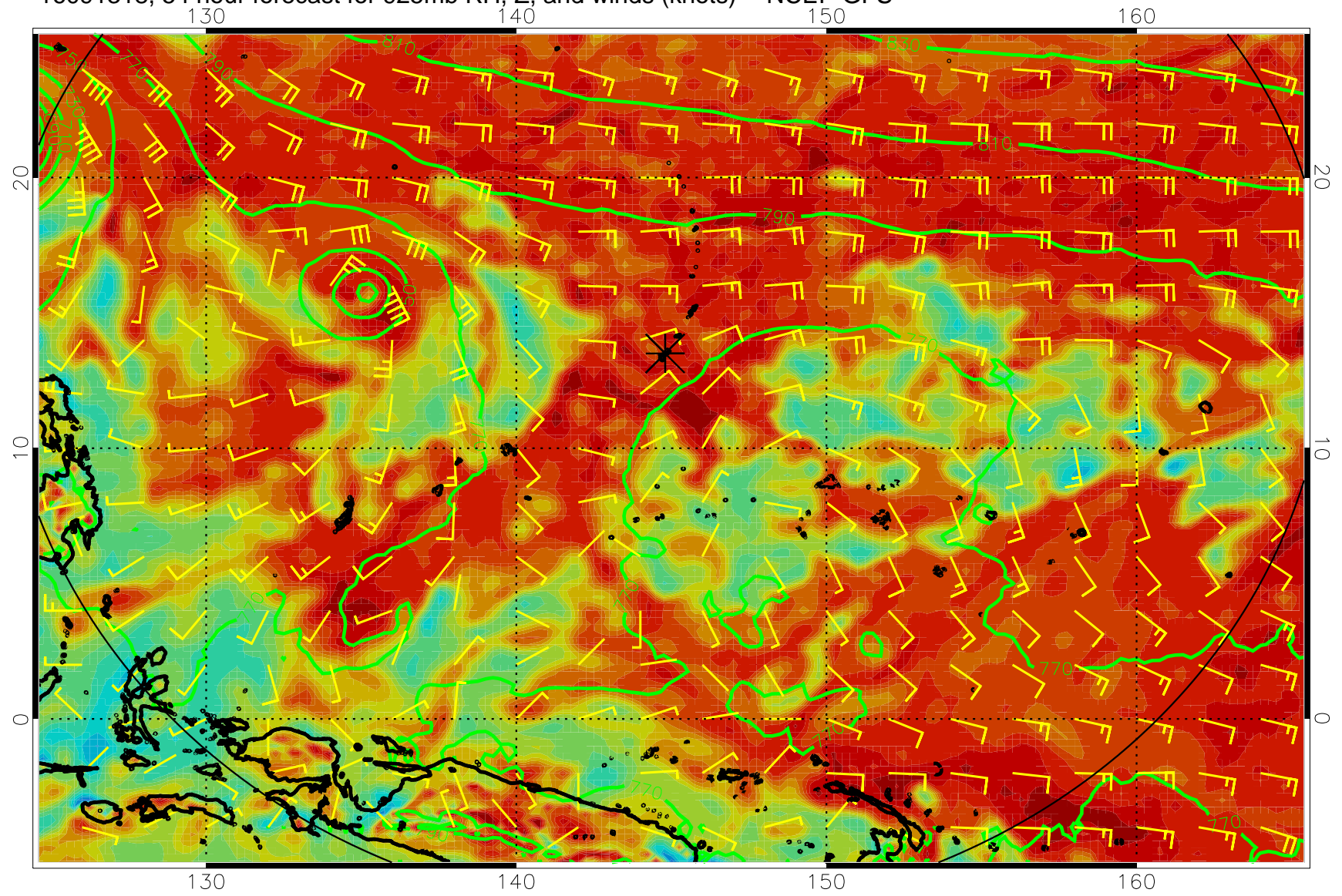
16091318, 54 hour forecast for 925mb RH, Z, and winds (knots) -- NCEP GFS
