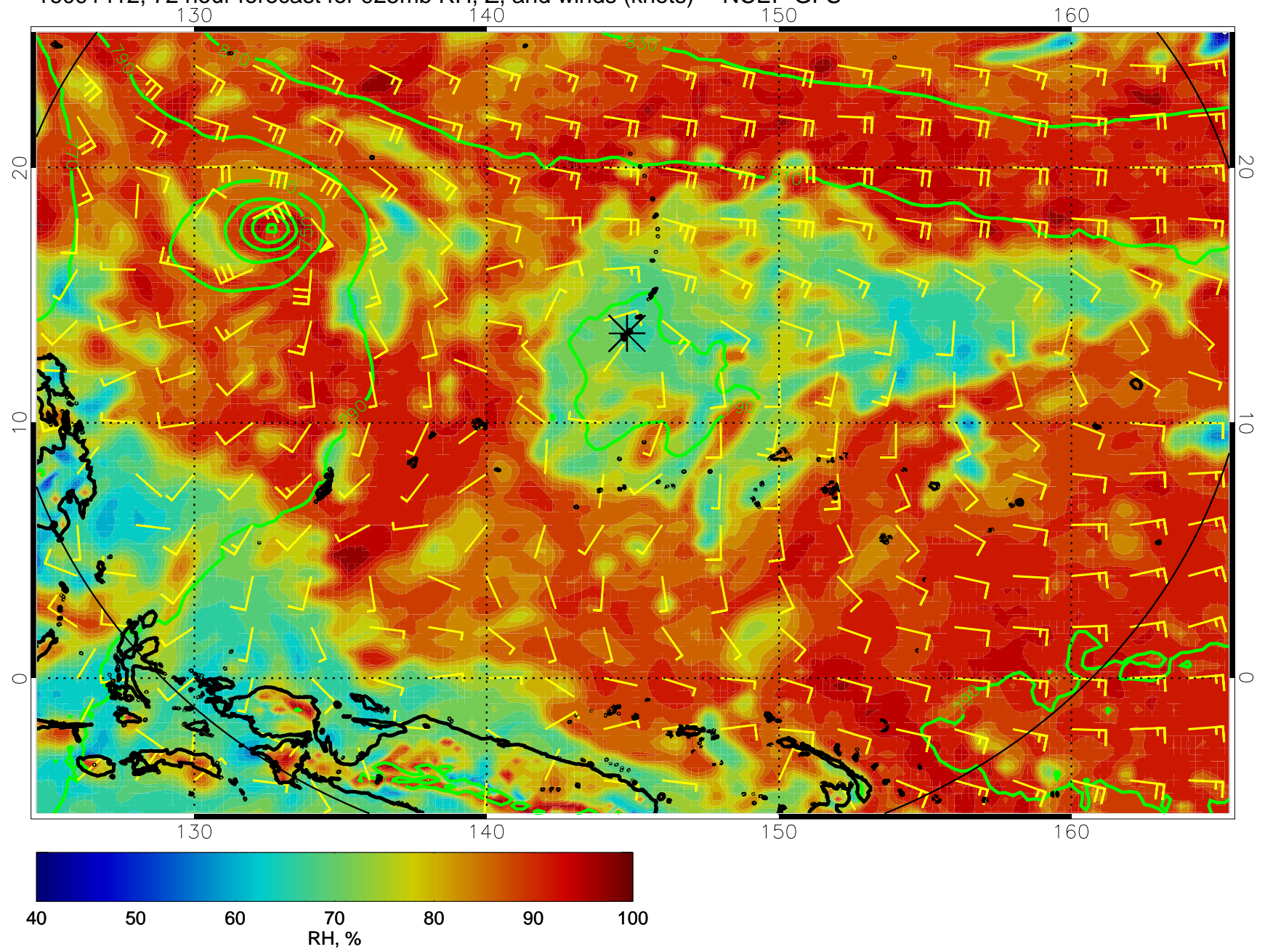
16091412, 72 hour forecast for 925mb RH, Z, and winds (knots) -- NCEP GFS
