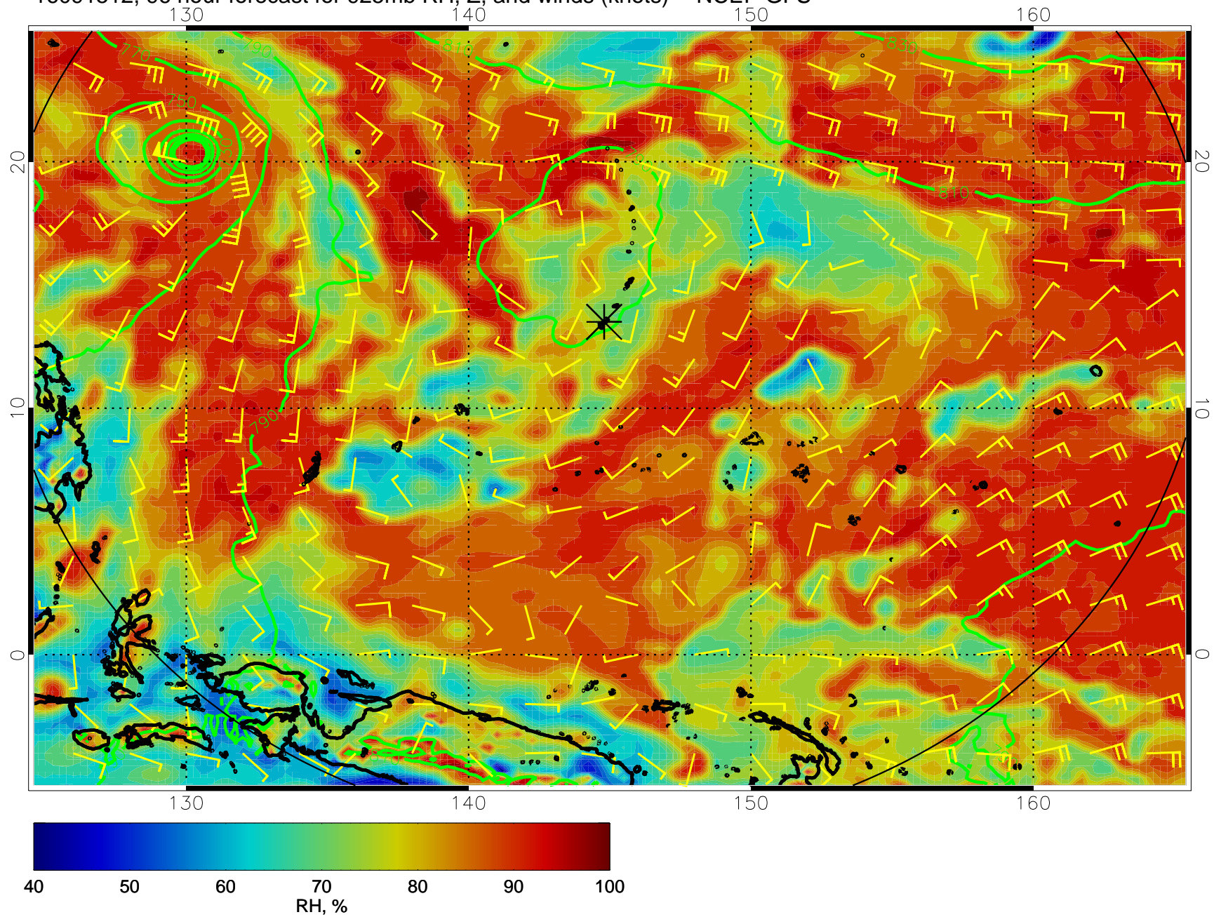
16091512, 96 hour forecast for 925mb RH, Z, and winds (knots) -- NCEP GFS
