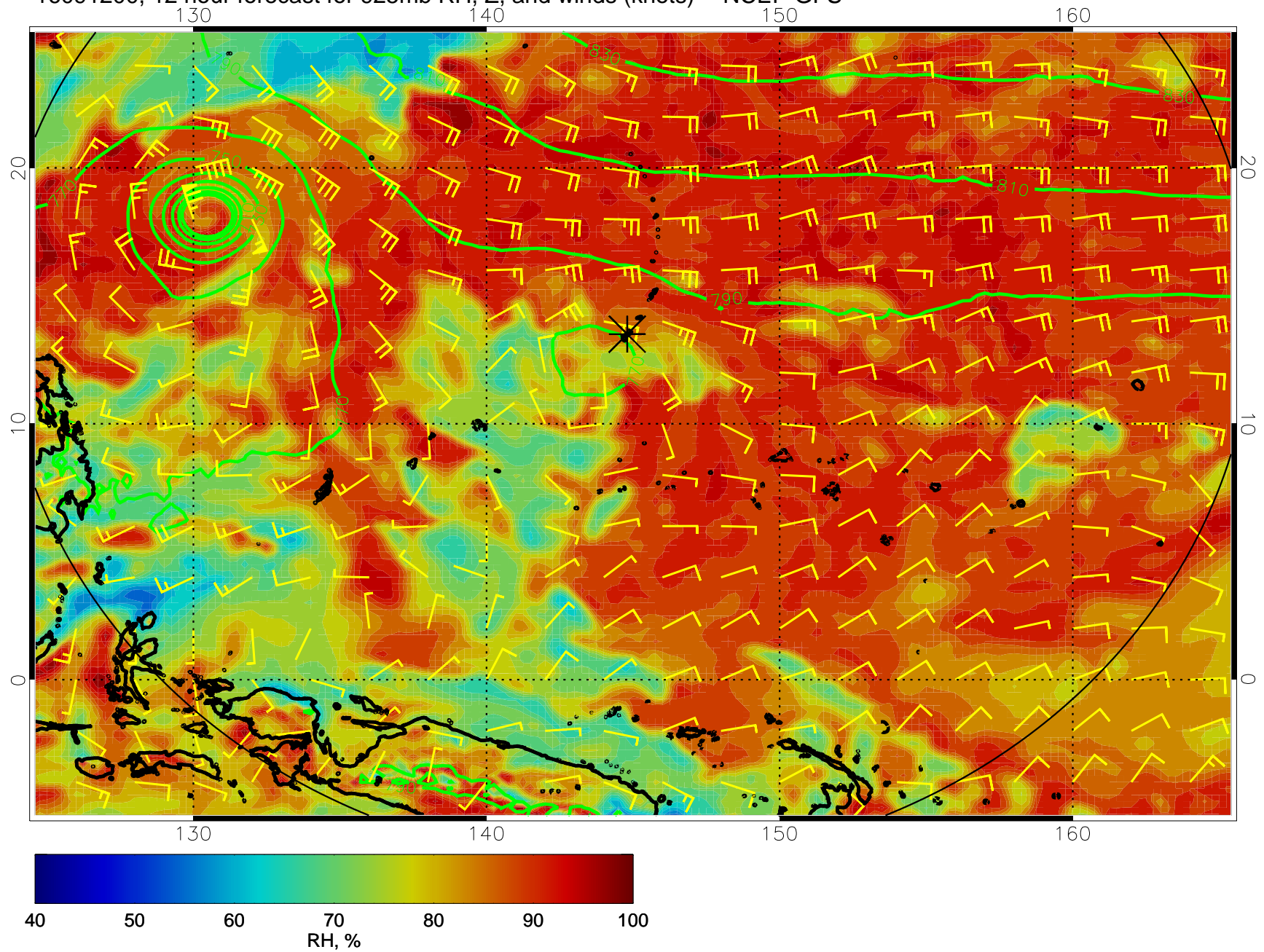
16091200, 12 hour forecast for 925mb RH, Z, and winds (knots) -- NCEP GFS
