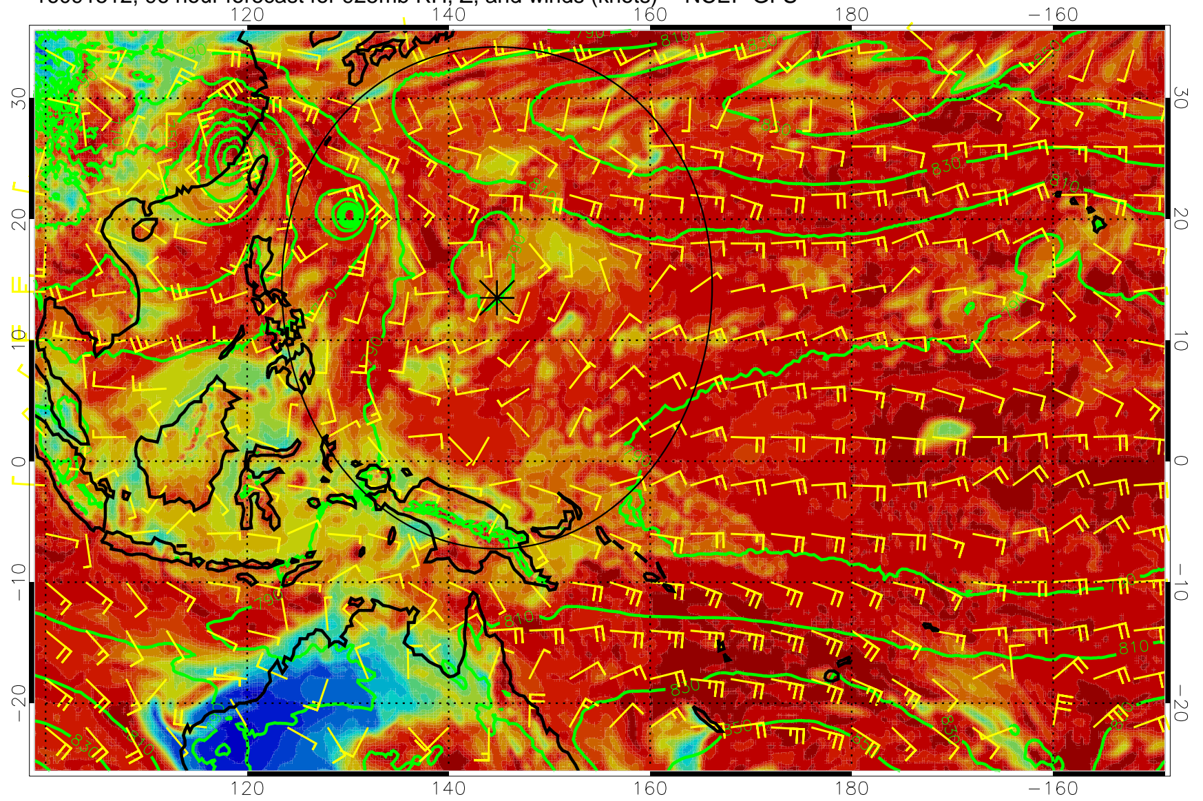
16091512, 96 hour forecast for 925mb RH, Z, and winds (knots) -- NCEP GFS
