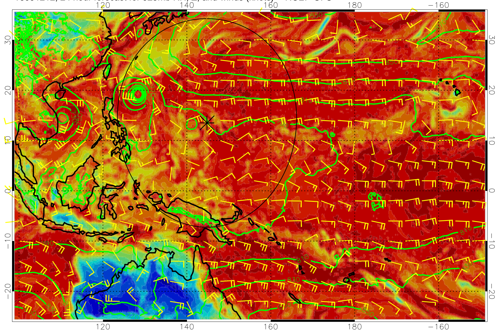
16091212, 24 hour forecast for 925mb RH, Z, and winds (knots) -- NCEP GFS
