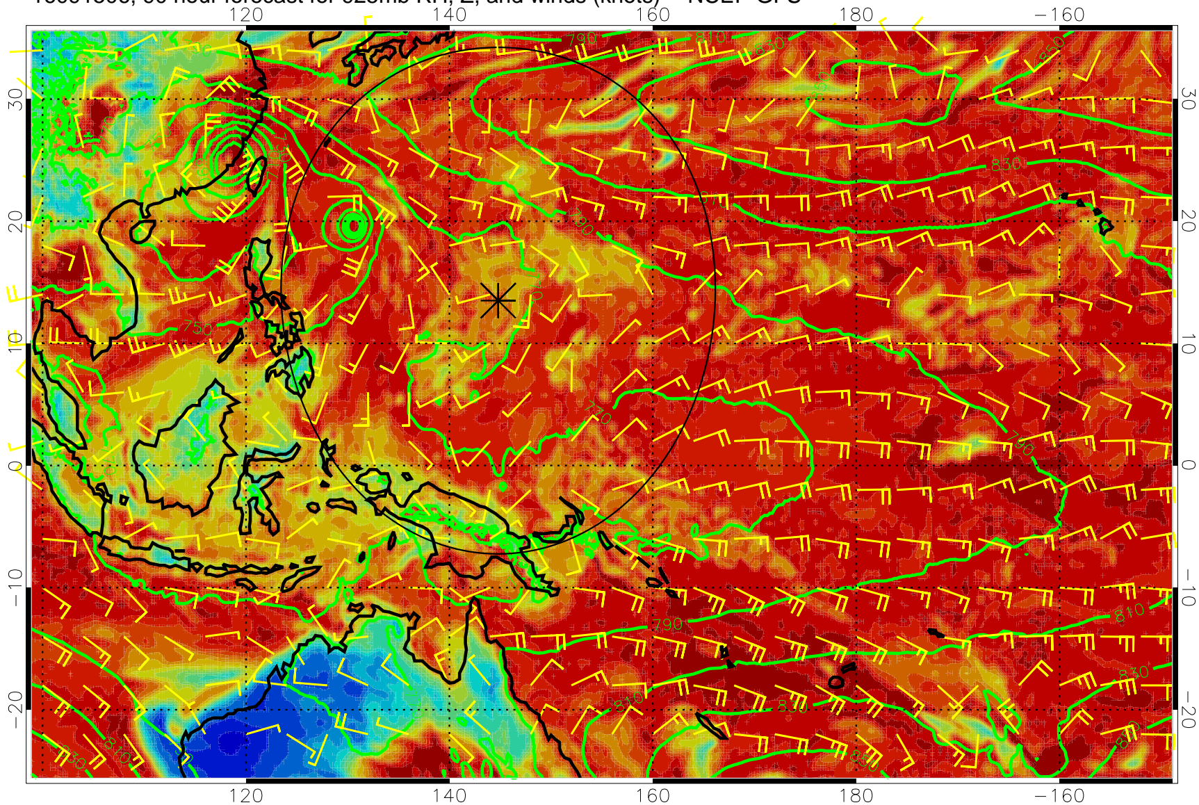
16091506, 90 hour forecast for 925mb RH, Z, and winds (knots) -- NCEP GFS
