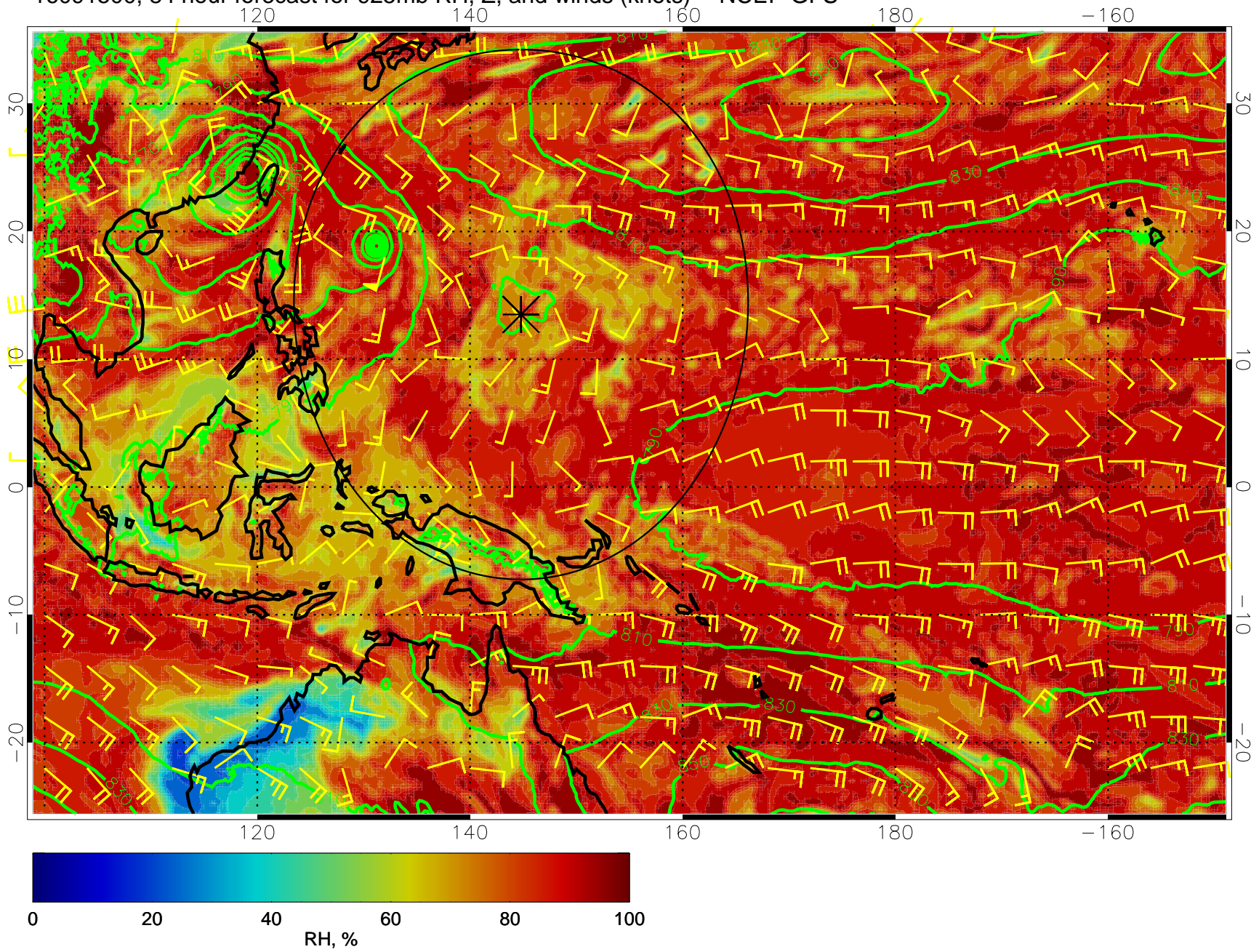
16091500, 84 hour forecast for 925mb RH, Z, and winds (knots) -- NCEP GFS
