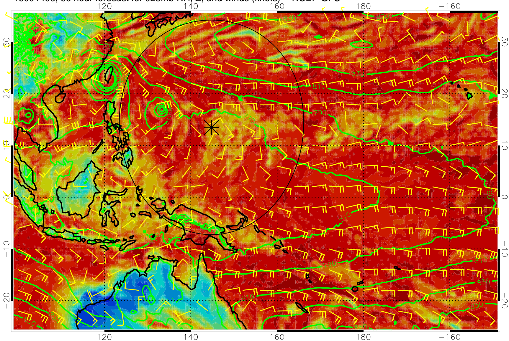
16091406, 66 hour forecast for 925mb RH, Z, and winds (knots) -- NCEP GFS
