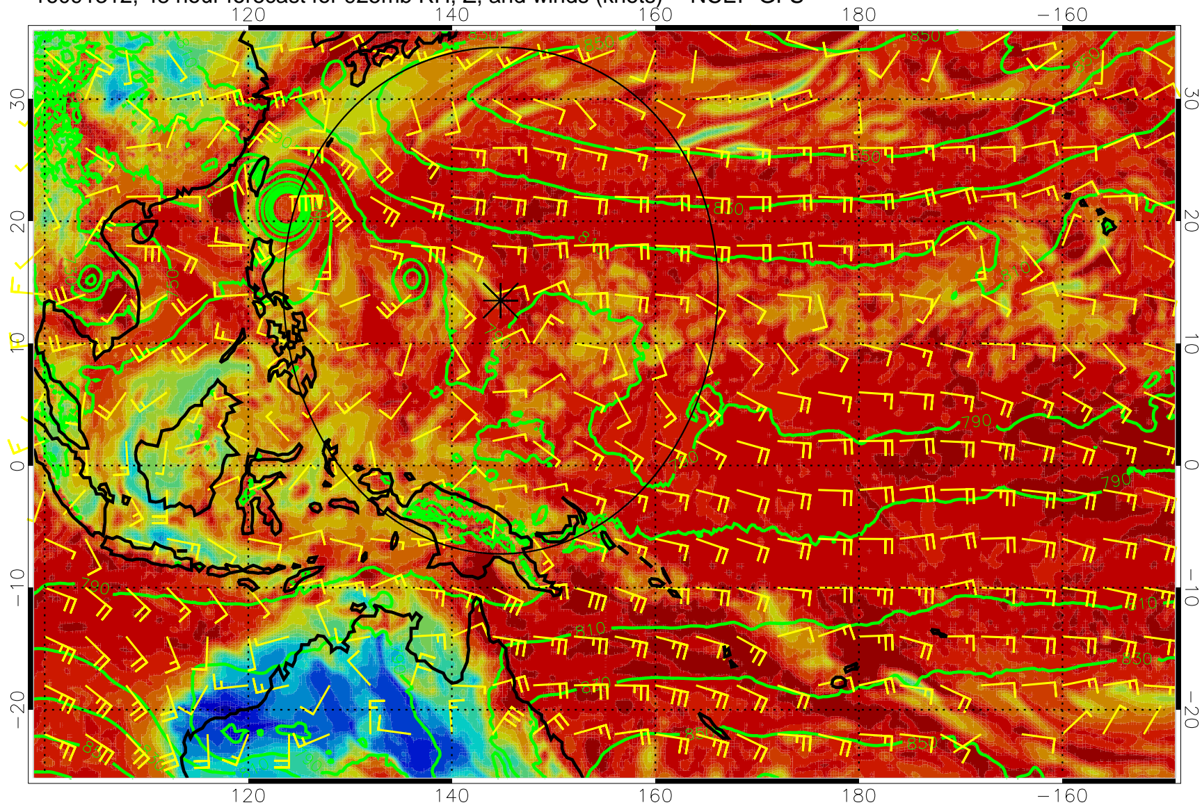
16091312, 48 hour forecast for 925mb RH, Z, and winds (knots) -- NCEP GFS
