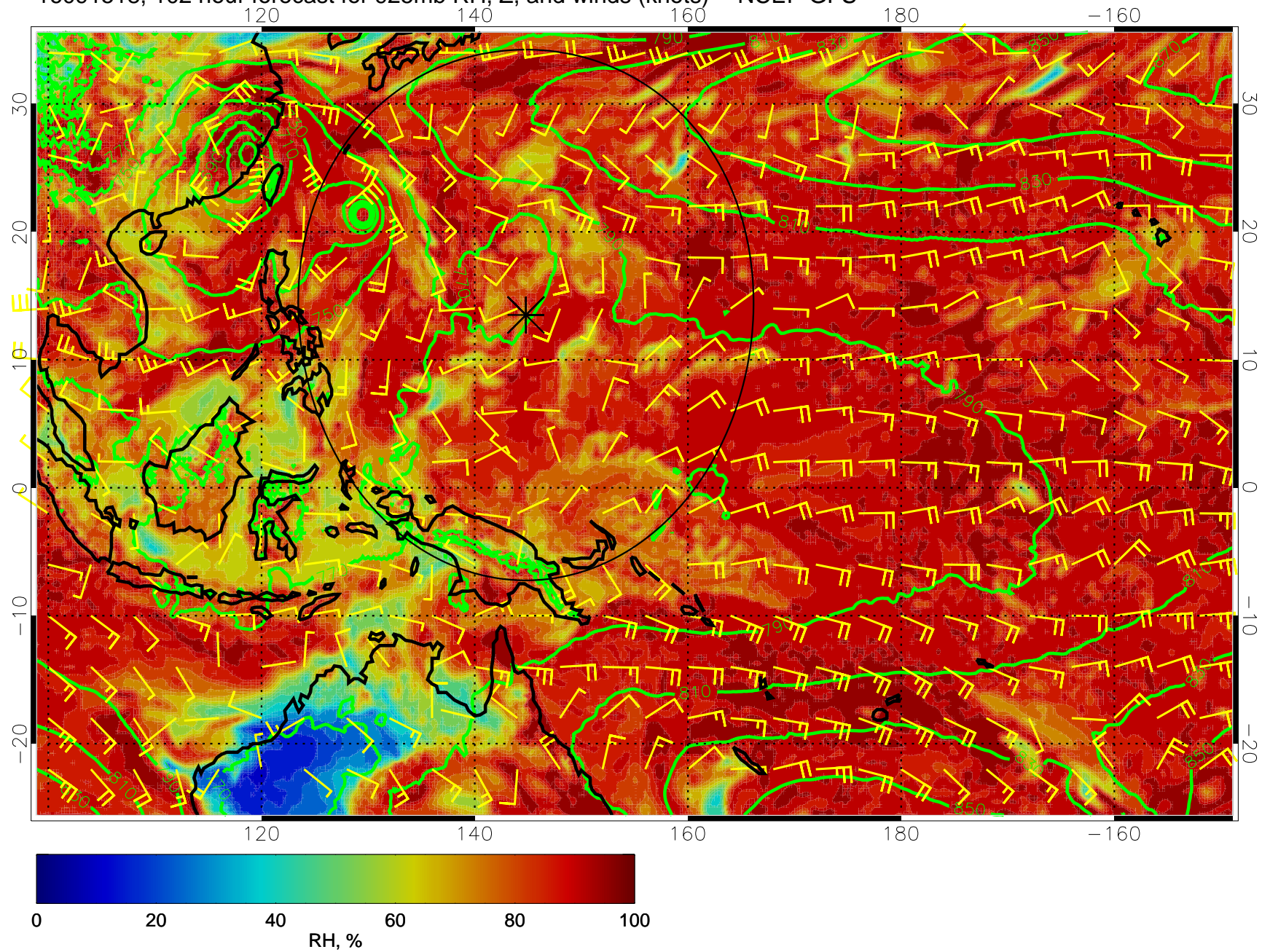
16091518, 102 hour forecast for 925mb RH, Z, and winds (knots) -- NCEP GFS
