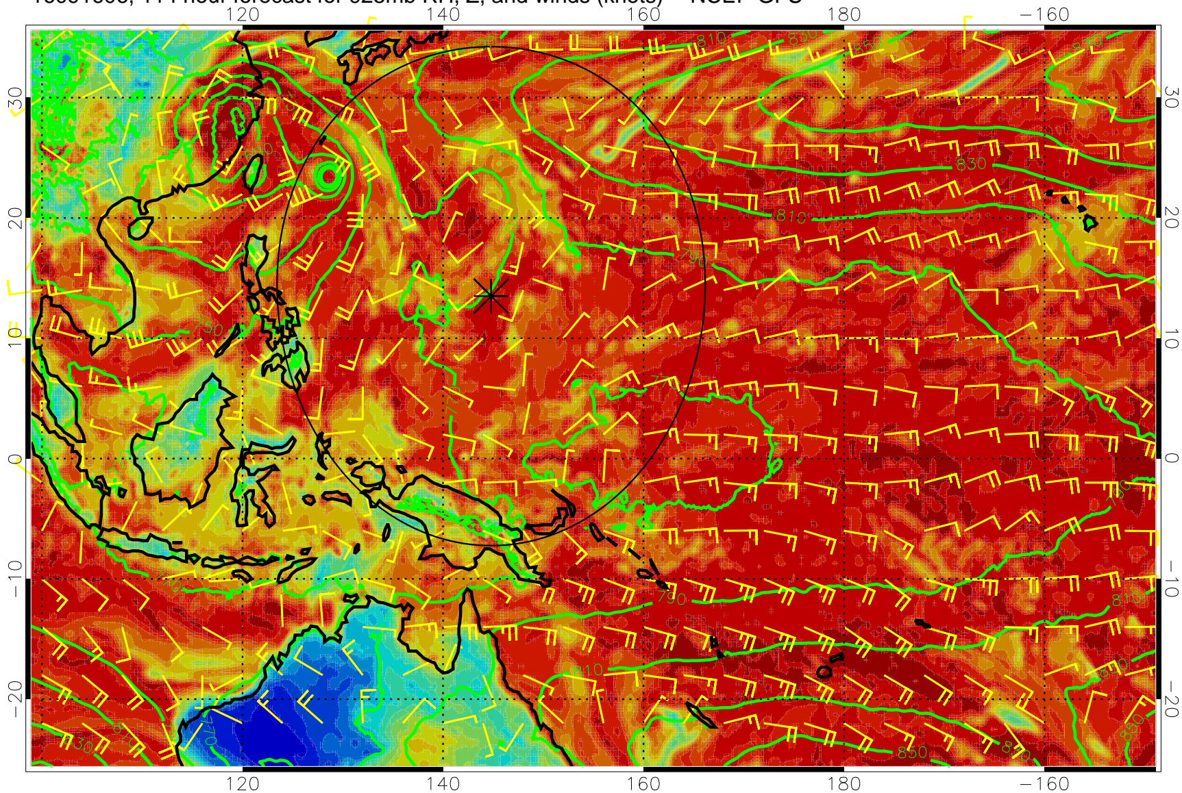
16091606, 114 hour forecast for 925mb RH, Z, and winds (knots) -- NCEP GFS
