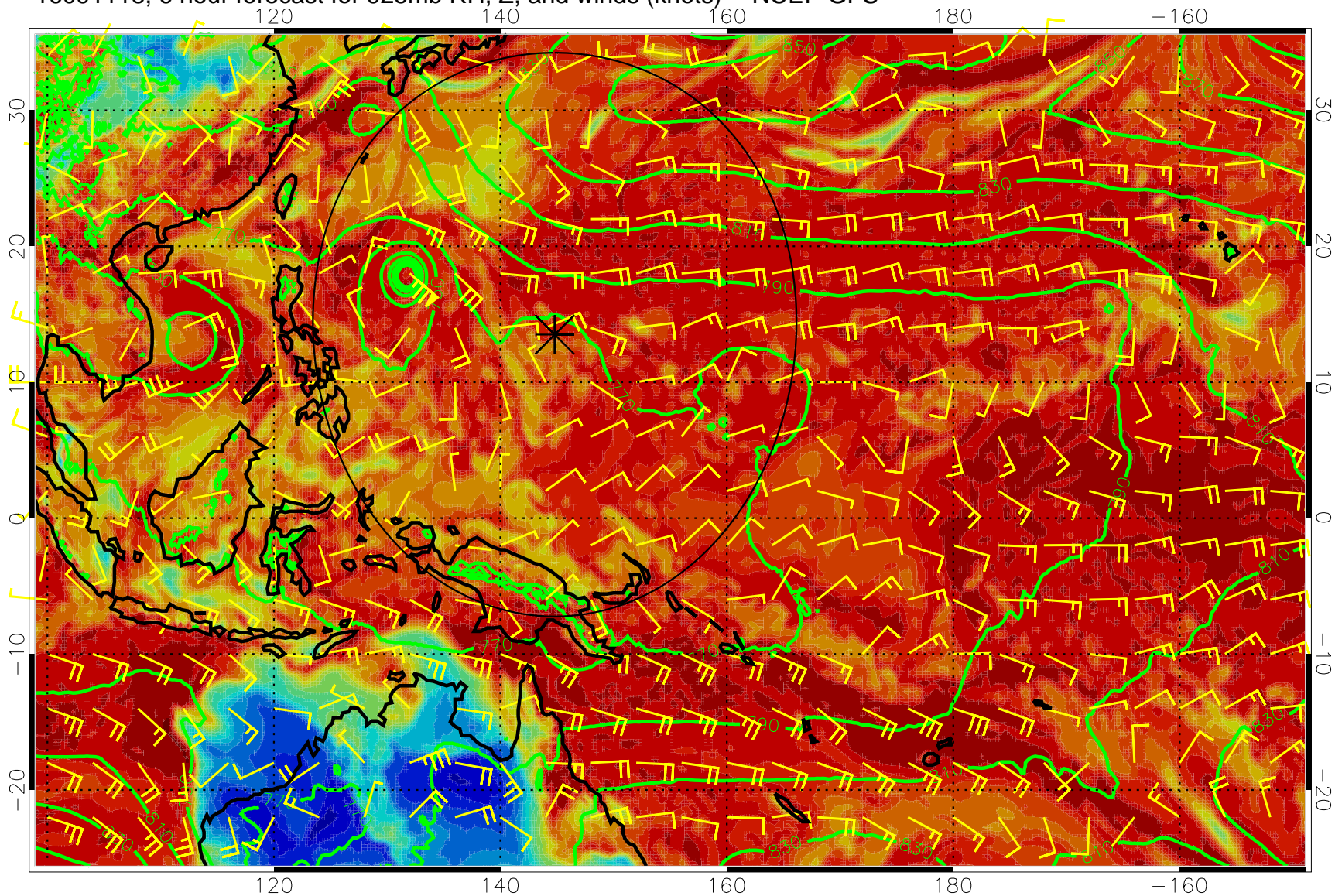
16091118, 6 hour forecast for 925mb RH, Z, and winds (knots) -- NCEP GFS
