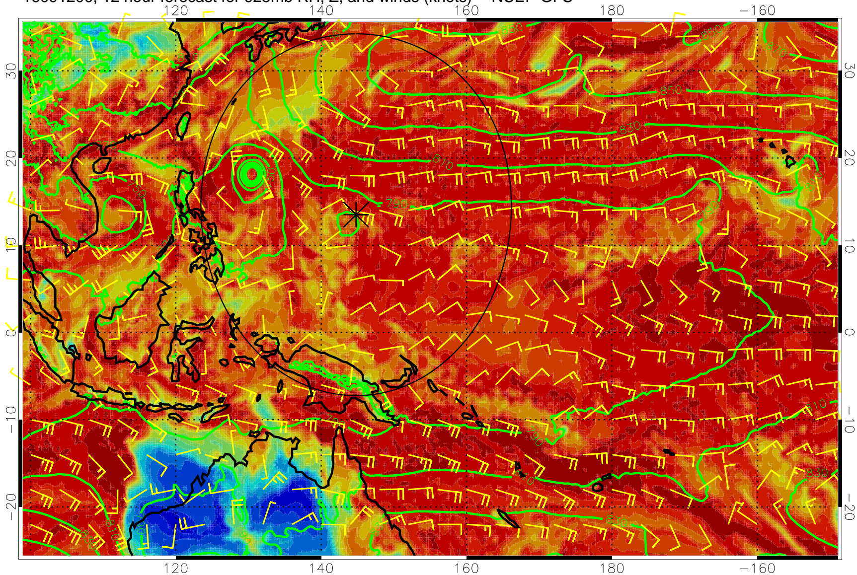
16091200, 12 hour forecast for 925mb RH, Z, and winds (knots) -- NCEP GFS
