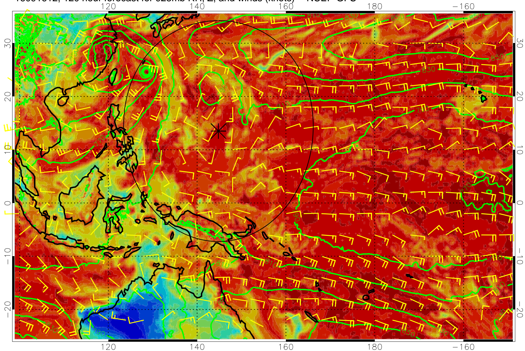
16091612, 120 hour forecast for 925mb RH, Z, and winds (knots) -- NCEP GFS
