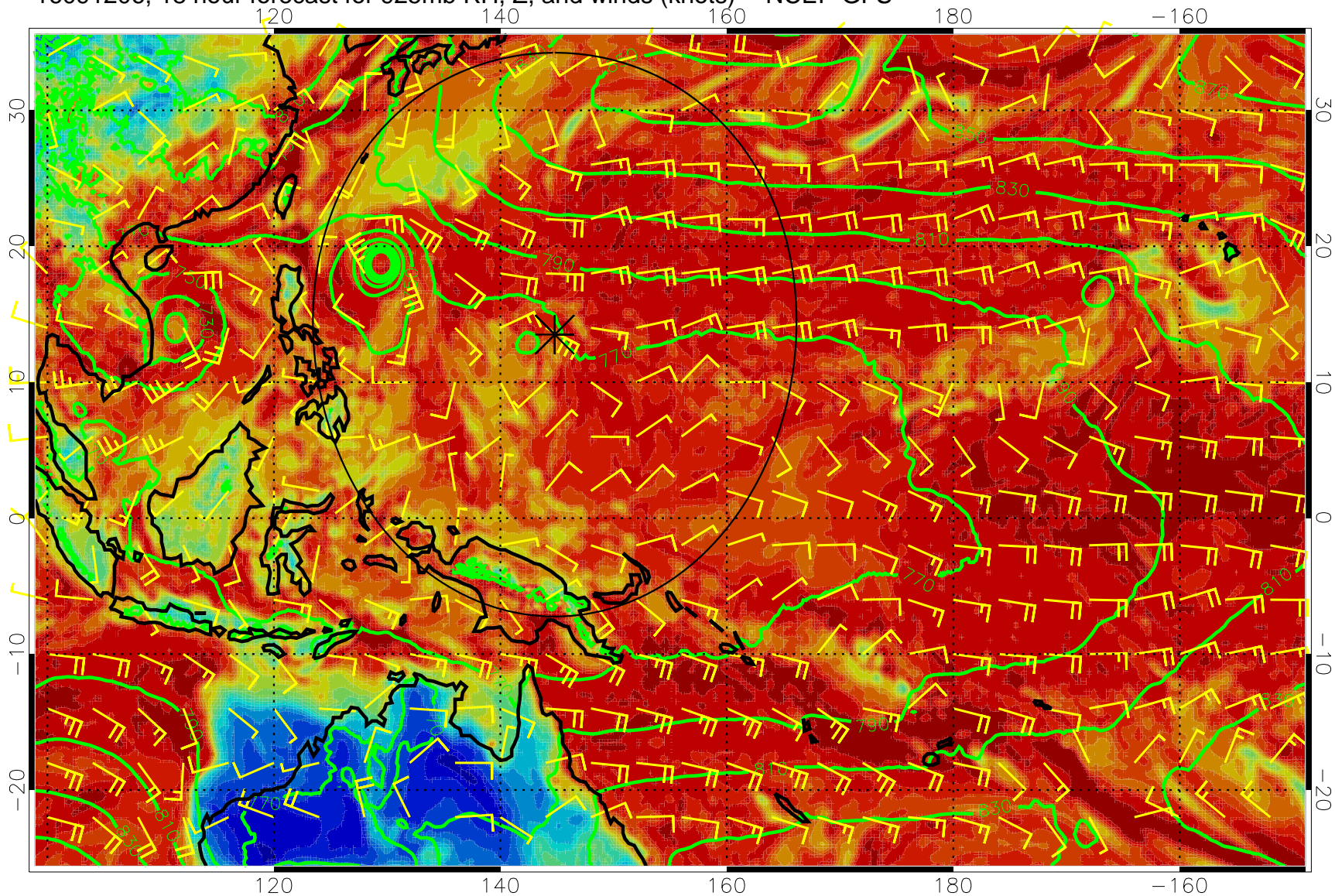
16091206, 18 hour forecast for 925mb RH, Z, and winds (knots) -- NCEP GFS
