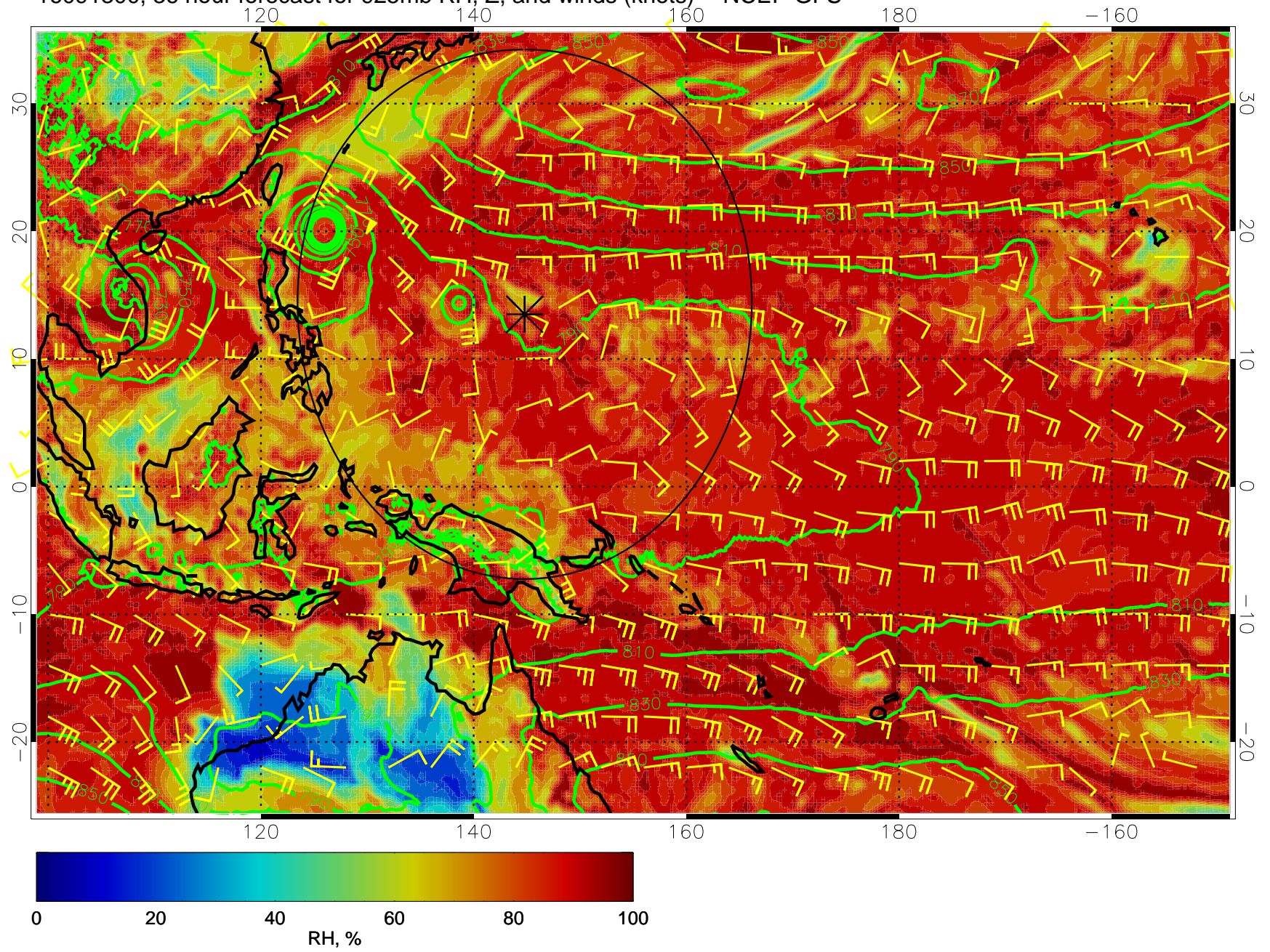
16091300, 36 hour forecast for 925mb RH, Z, and winds (knots) -- NCEP GFS
