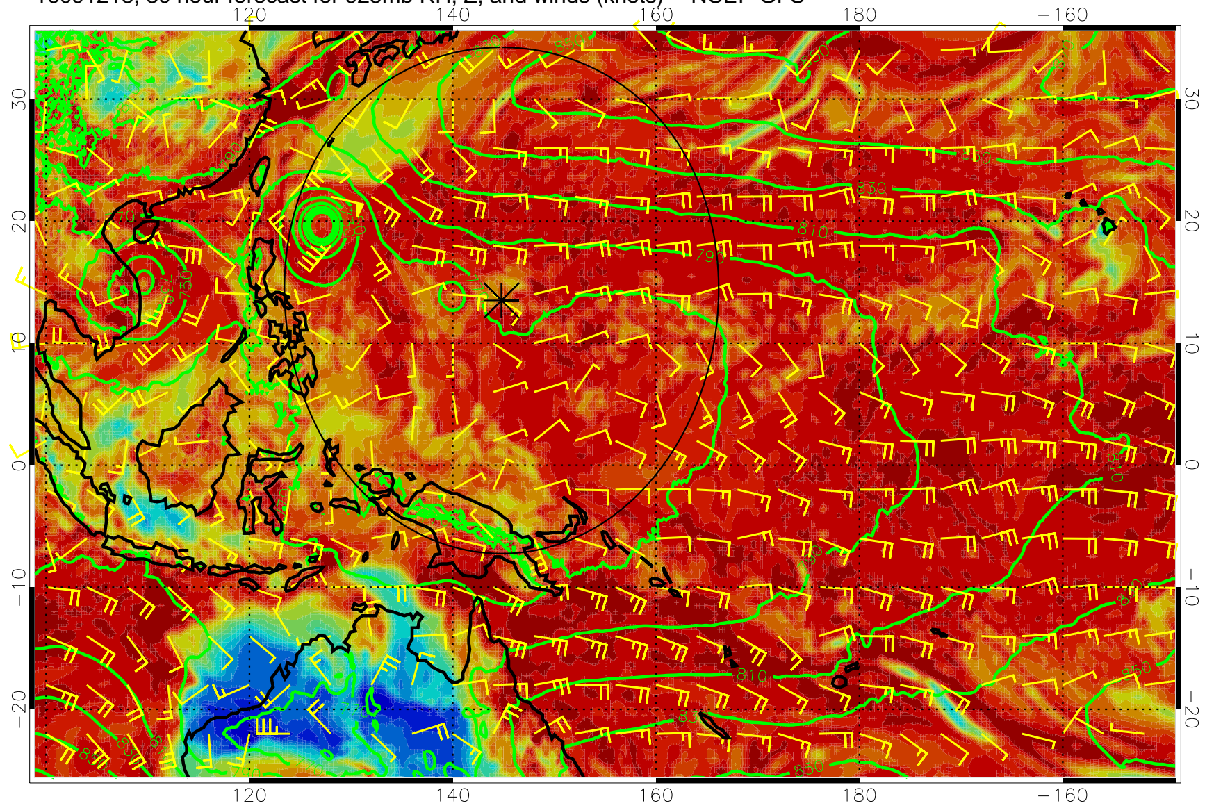
16091218, 30 hour forecast for 925mb RH, Z, and winds (knots) -- NCEP GFS
