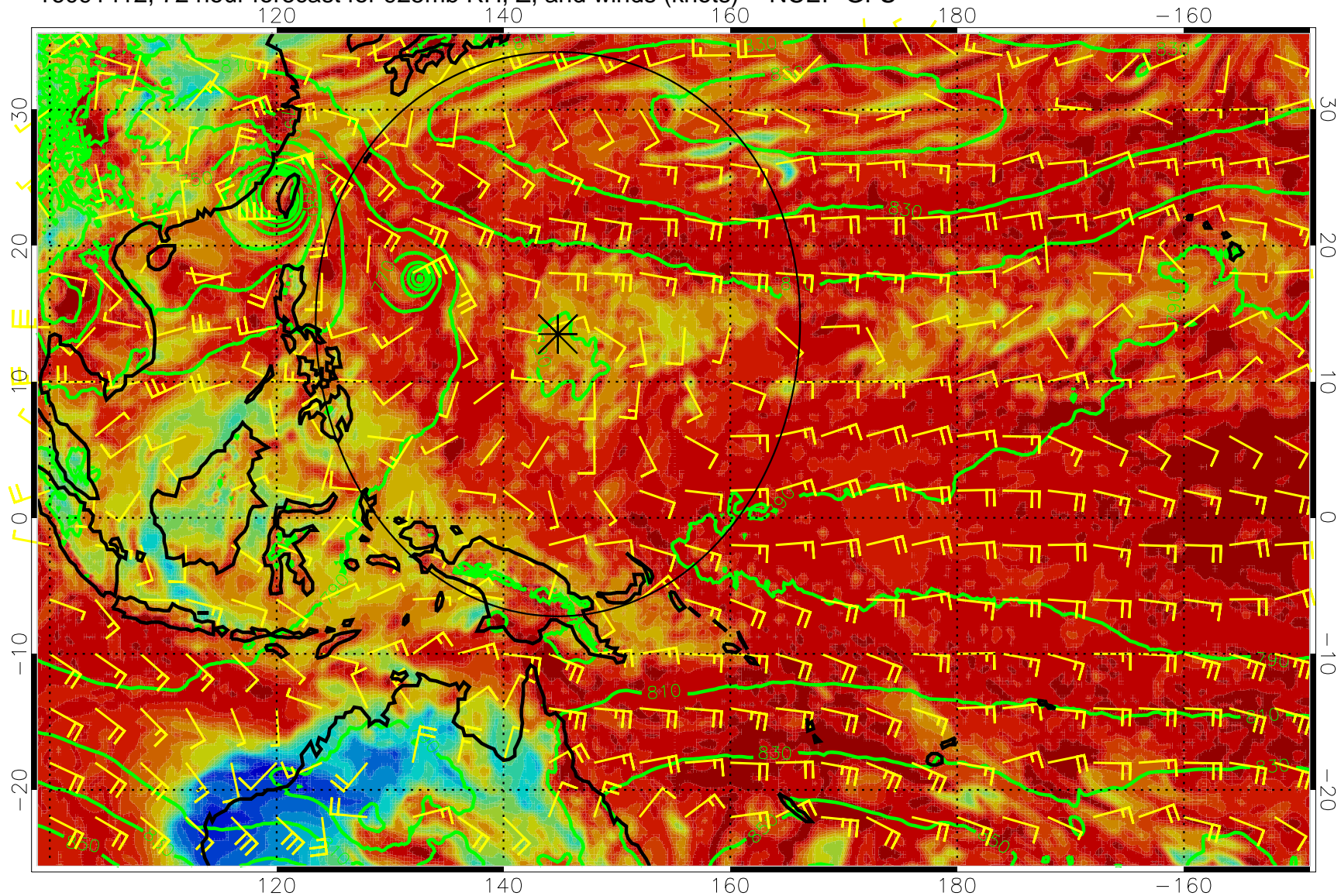
16091412, 72 hour forecast for 925mb RH, Z, and winds (knots) -- NCEP GFS
