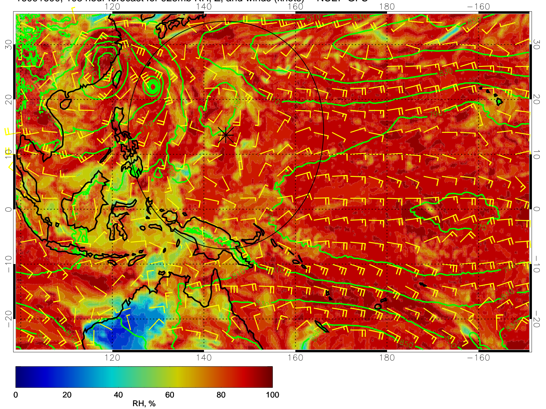
16091600, 108 hour forecast for 925mb RH, Z, and winds (knots) -- NCEP GFS
