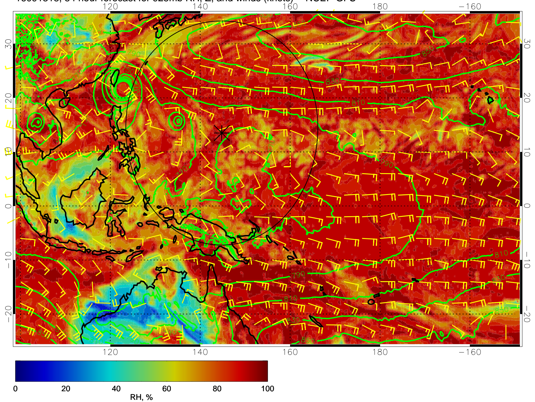
16091318, 54 hour forecast for 925mb RH, Z, and winds (knots) -- NCEP GFS
