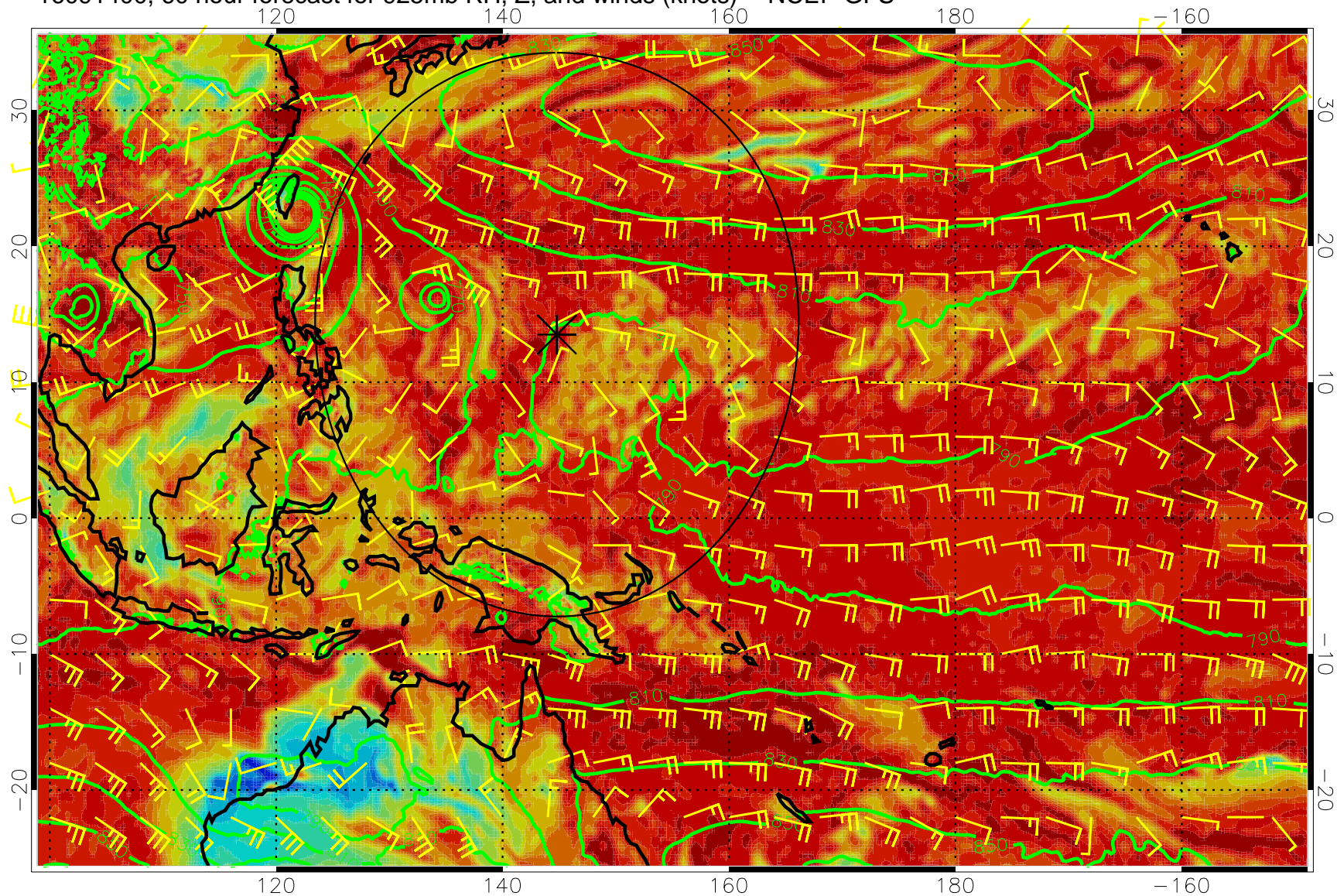
16091400, 60 hour forecast for 925mb RH, Z, and winds (knots) -- NCEP GFS
