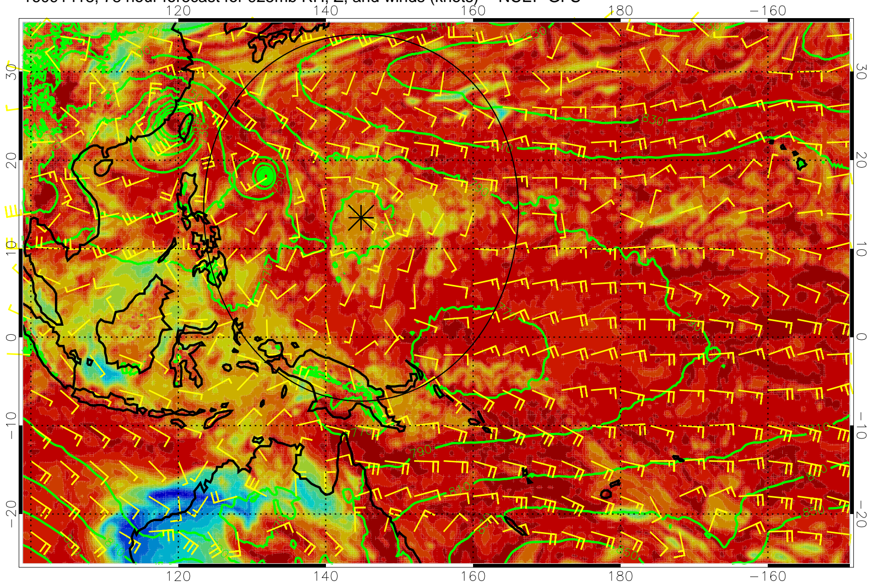
16091418, 78 hour forecast for 925mb RH, Z, and winds (knots) -- NCEP GFS
