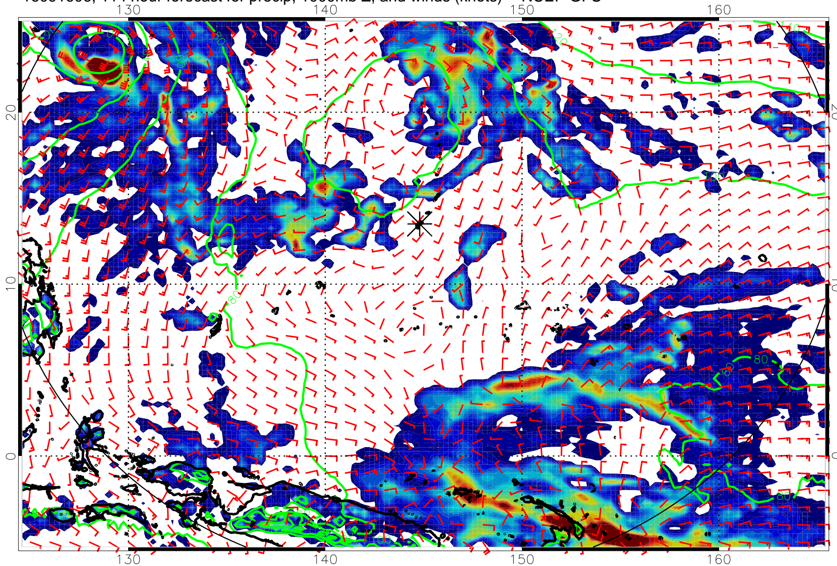
16091606, 114 hour forecast for precip, 1000mb Z, and winds (knots) -- NCEP GFS
