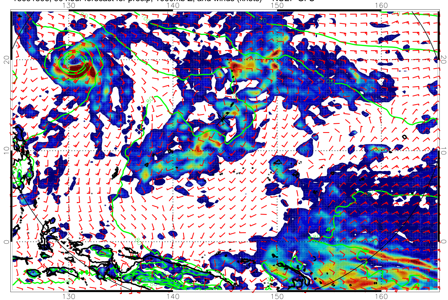
16091506, 90 hour forecast for precip, 1000mb Z, and winds (knots) -- NCEP GFS
