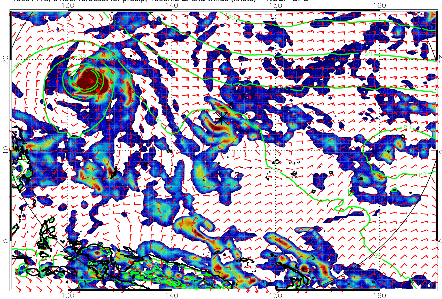
16091118, 6 hour forecast for precip, 1000mb Z, and winds (knots) -- NCEP GFS
