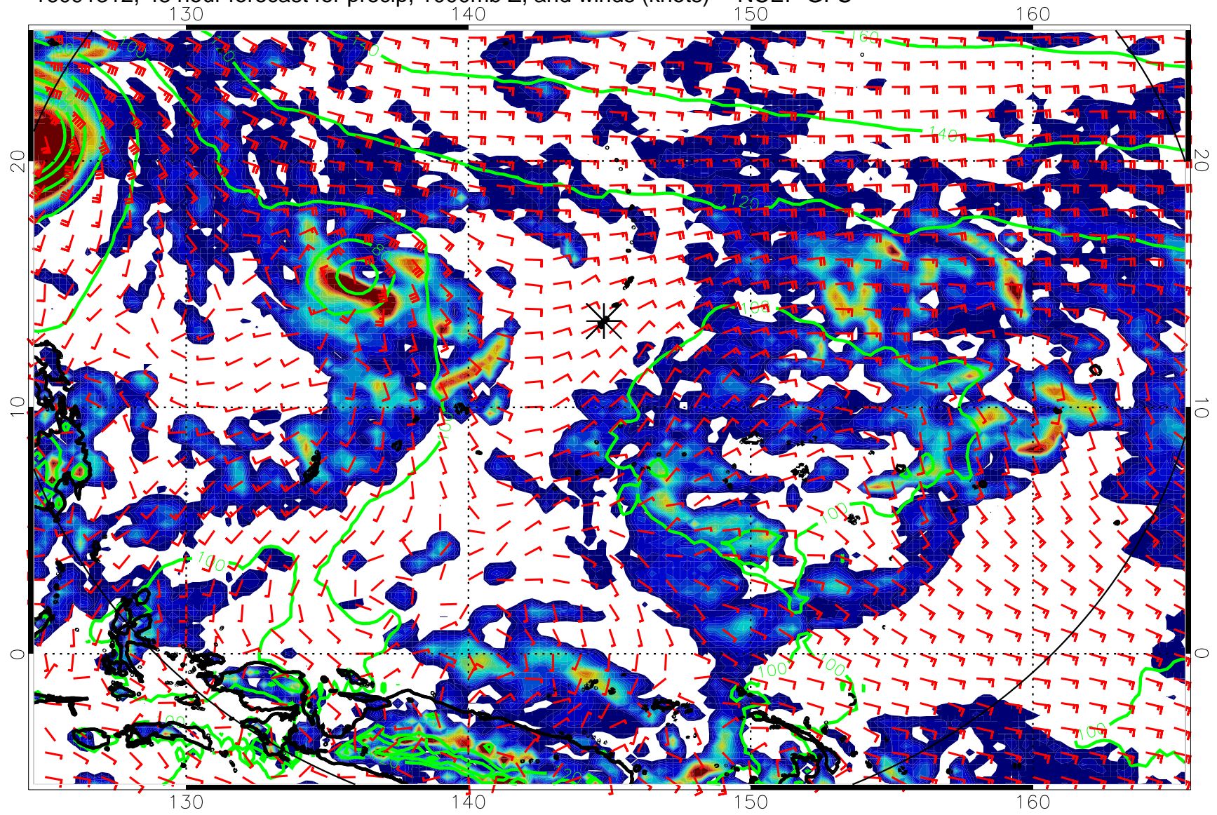
16091312, 48 hour forecast for precip, 1000mb Z, and winds (knots) -- NCEP GFS
