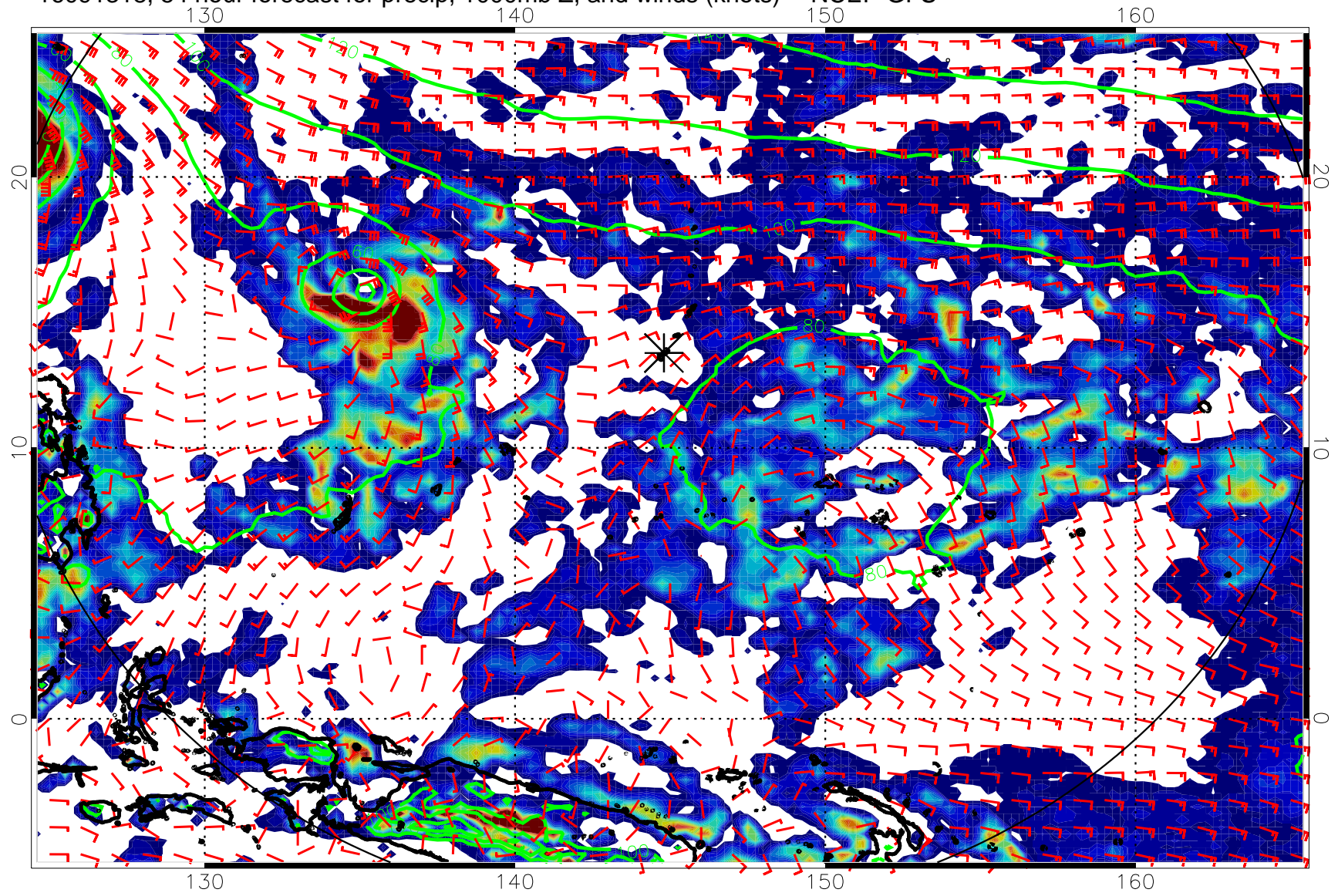
16091318, 54 hour forecast for precip, 1000mb Z, and winds (knots) -- NCEP GFS
