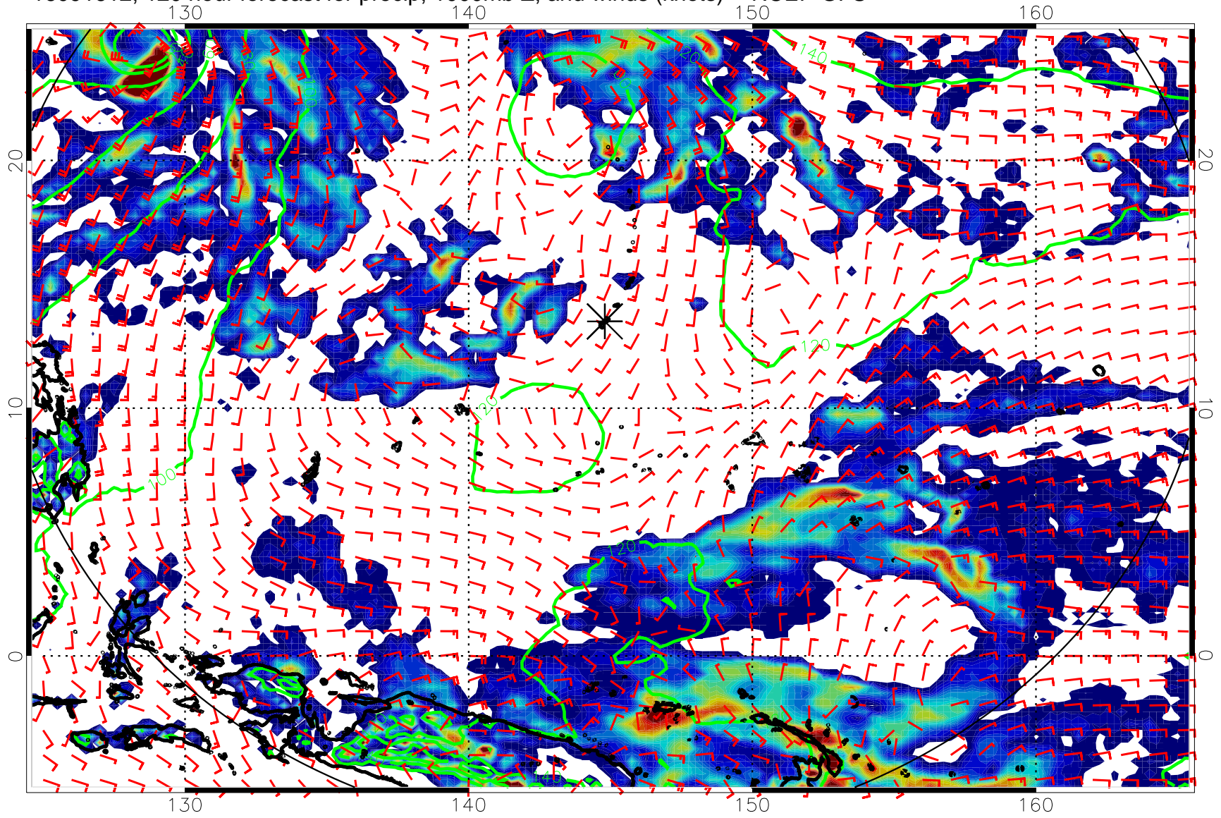
16091612, 120 hour forecast for precip, 1000mb Z, and winds (knots) -- NCEP GFS
