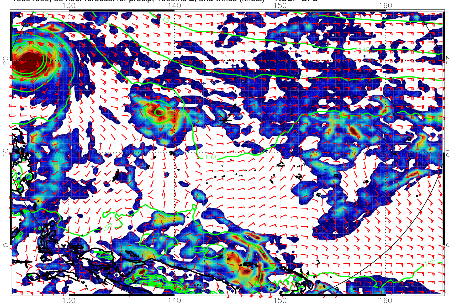
16091300, 36 hour forecast for precip, 1000mb Z, and winds (knots) -- NCEP GFS
