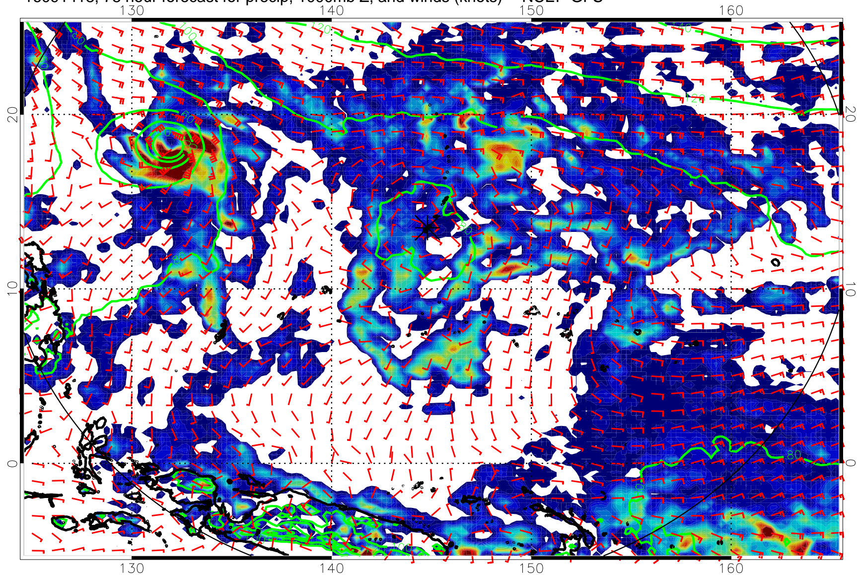
16091418, 78 hour forecast for precip, 1000mb Z, and winds (knots) -- NCEP GFS
