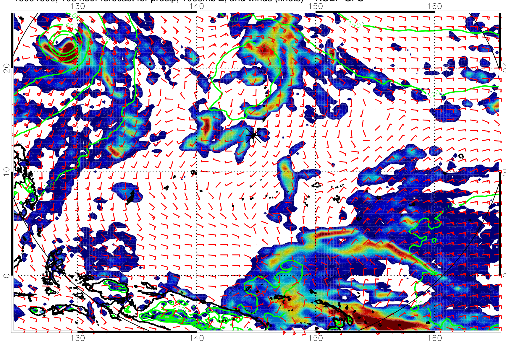
16091600, 108 hour forecast for precip, 1000mb Z, and winds (knots) -- NCEP GFS
