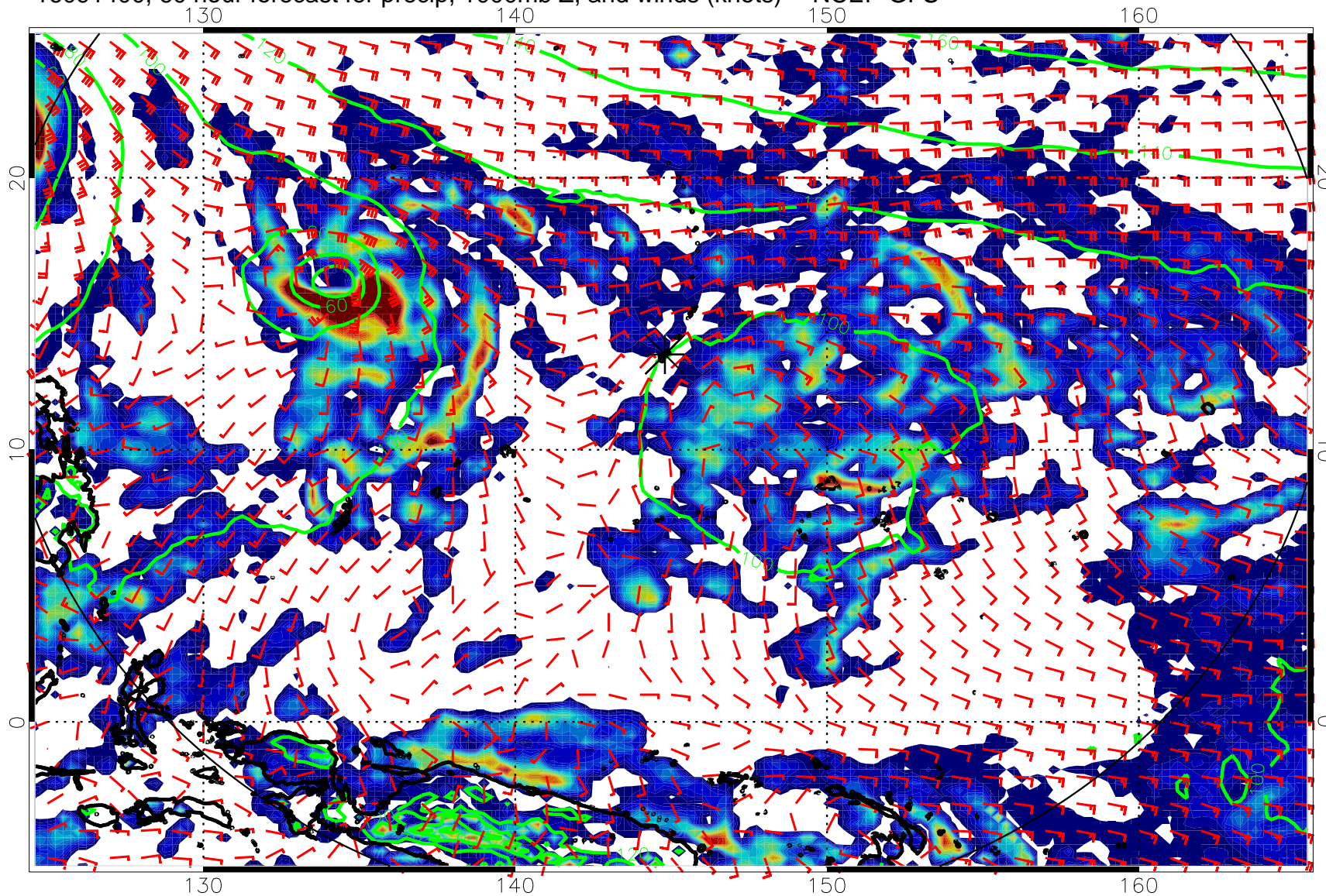
16091400, 60 hour forecast for precip, 1000mb Z, and winds (knots) -- NCEP GFS
