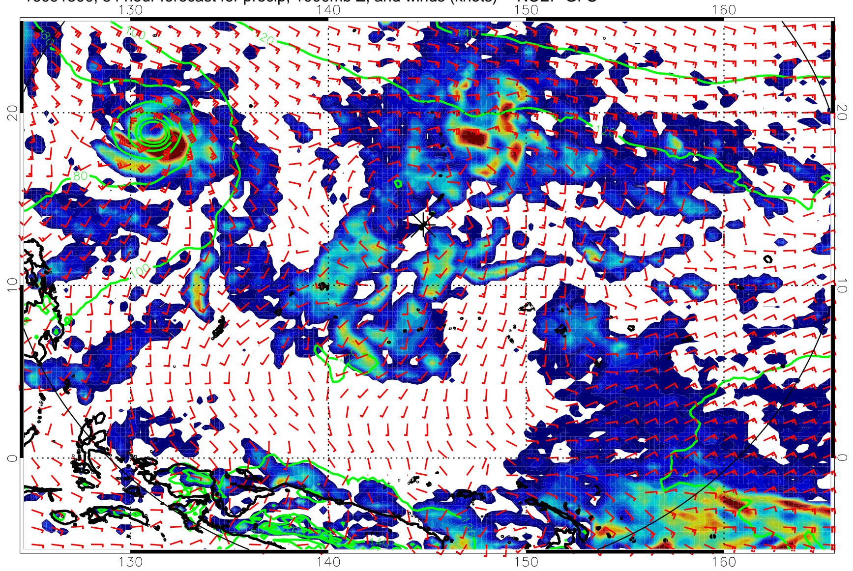
16091500, 84 hour forecast for precip, 1000mb Z, and winds (knots) -- NCEP GFS
