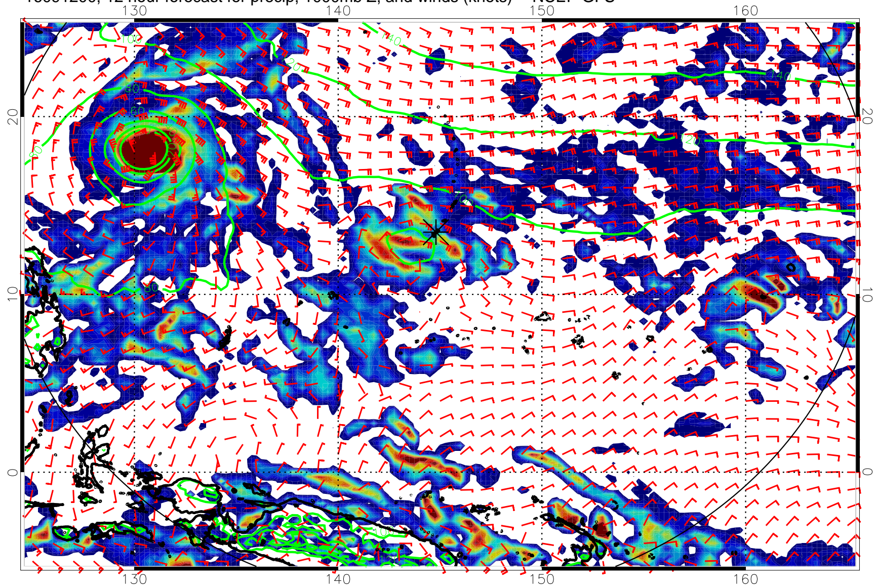
16091200, 12 hour forecast for precip, 1000mb Z, and winds (knots) -- NCEP GFS
