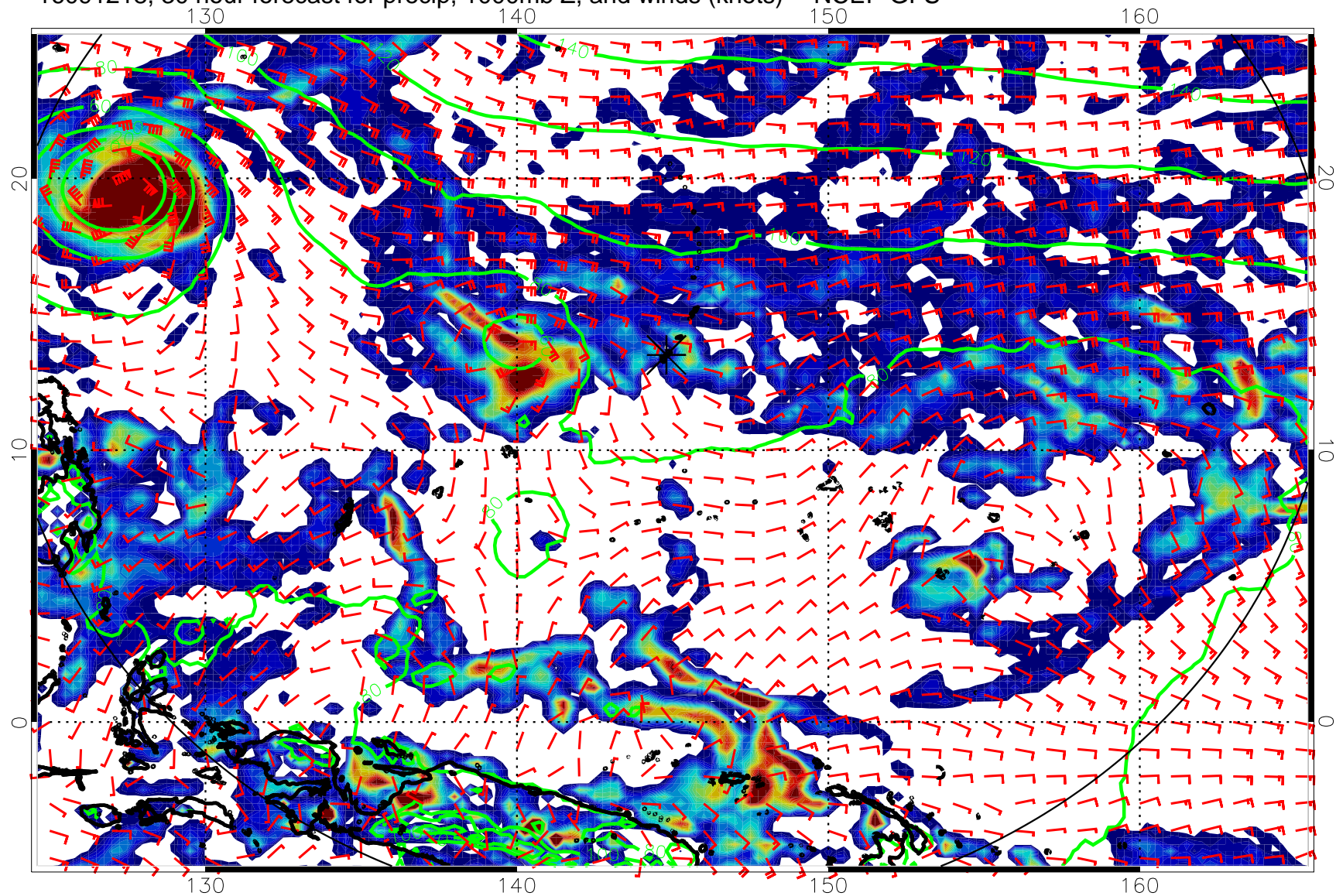
16091218, 30 hour forecast for precip, 1000mb Z, and winds (knots) -- NCEP GFS
