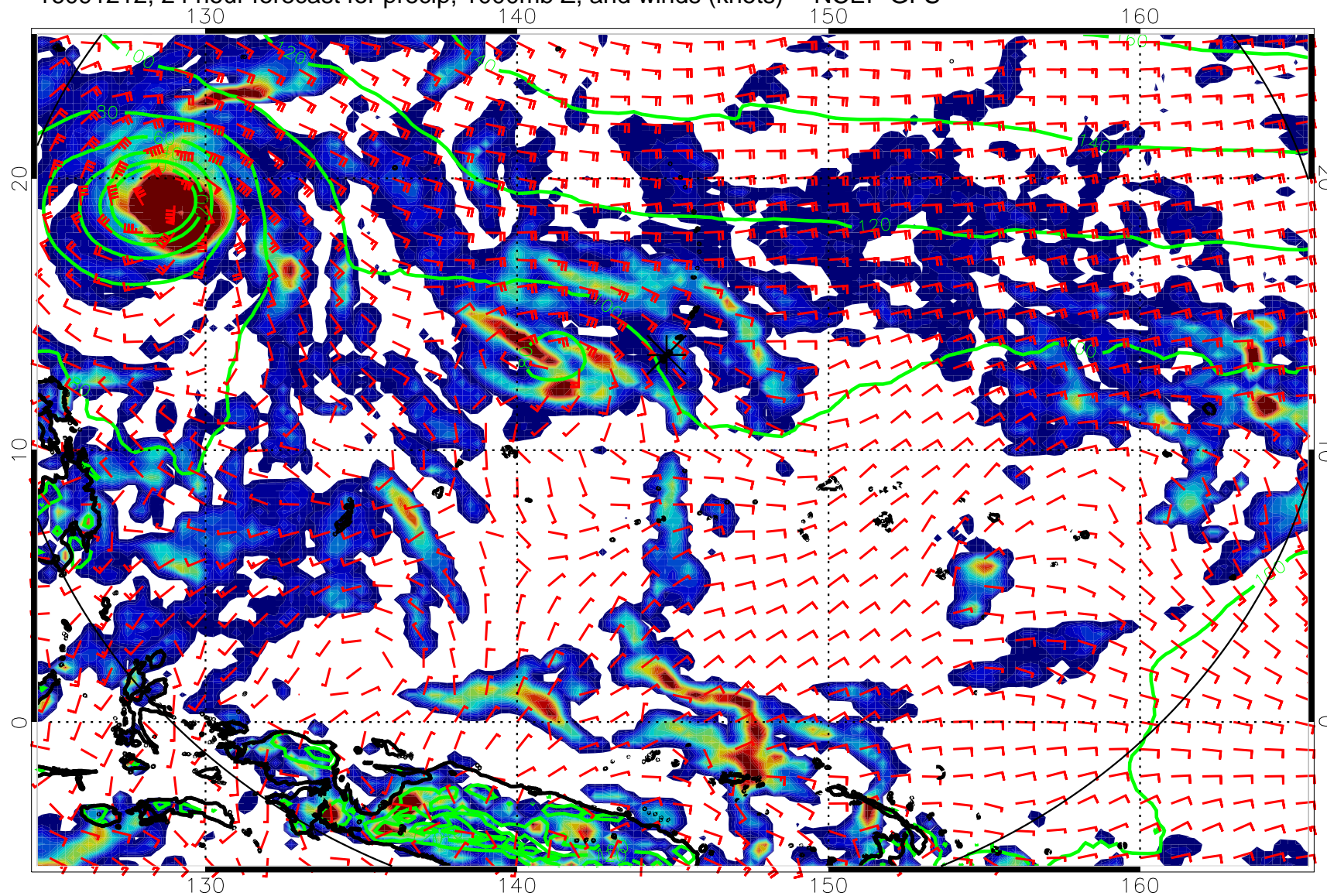
16091212, 24 hour forecast for precip, 1000mb Z, and winds (knots) -- NCEP GFS
