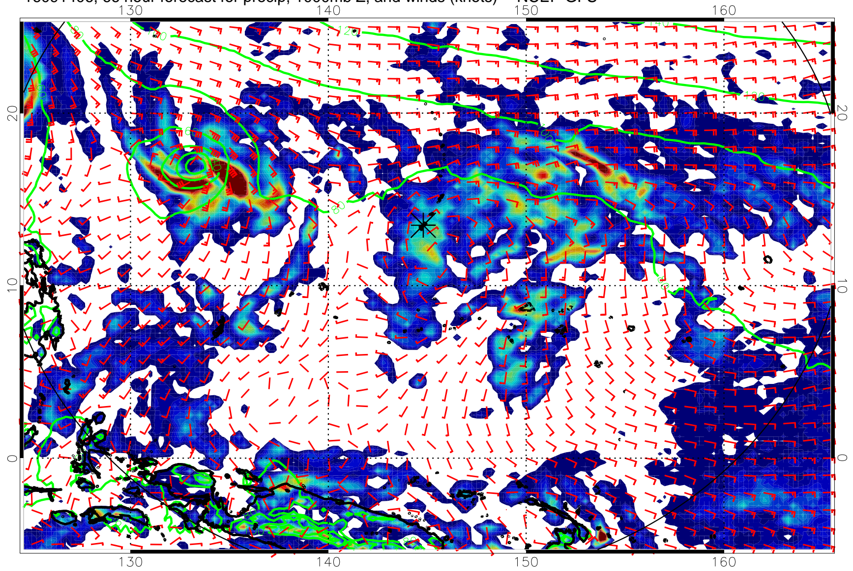
16091406, 66 hour forecast for precip, 1000mb Z, and winds (knots) -- NCEP GFS
