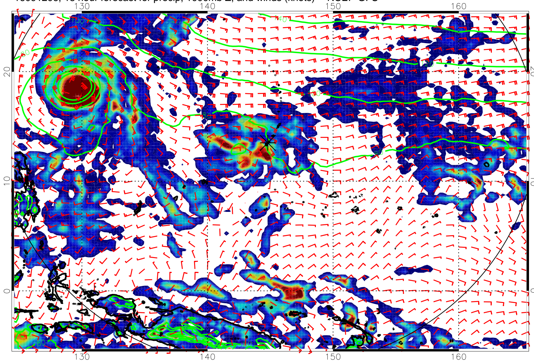
16091206, 18 hour forecast for precip, 1000mb Z, and winds (knots) -- NCEP GFS
