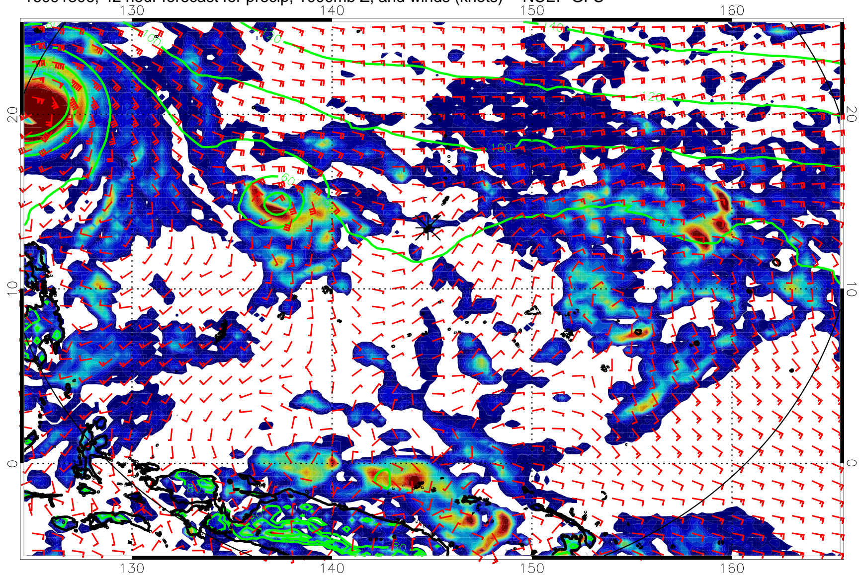
16091306, 42 hour forecast for precip, 1000mb Z, and winds (knots) -- NCEP GFS
