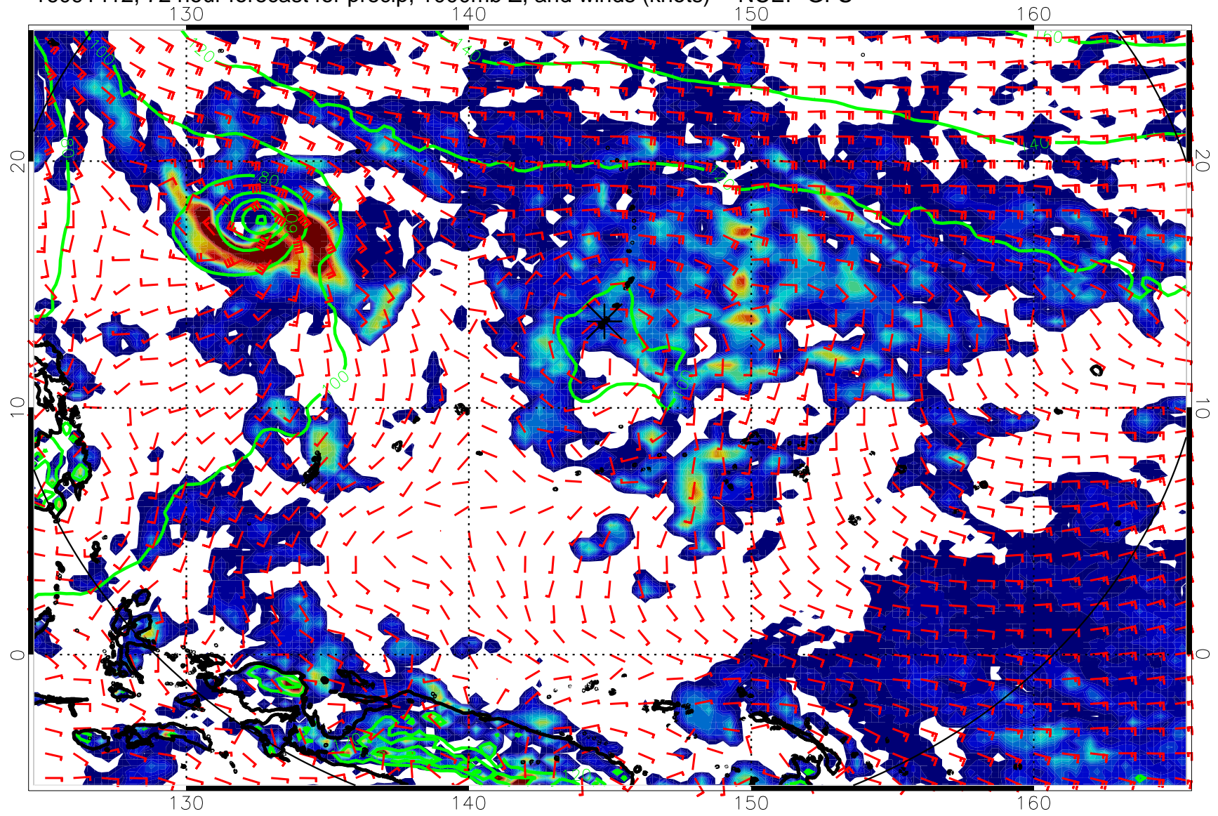
16091412, 72 hour forecast for precip, 1000mb Z, and winds (knots) -- NCEP GFS
