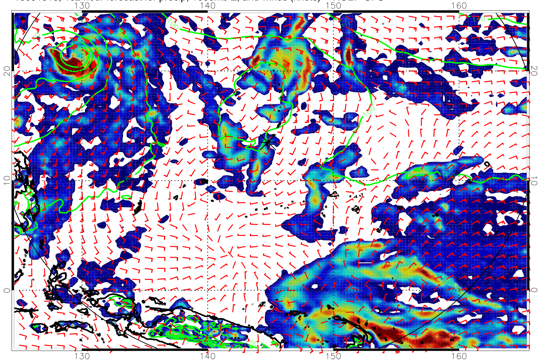
16091518, 102 hour forecast for precip, 1000mb Z, and winds (knots) -- NCEP GFS
