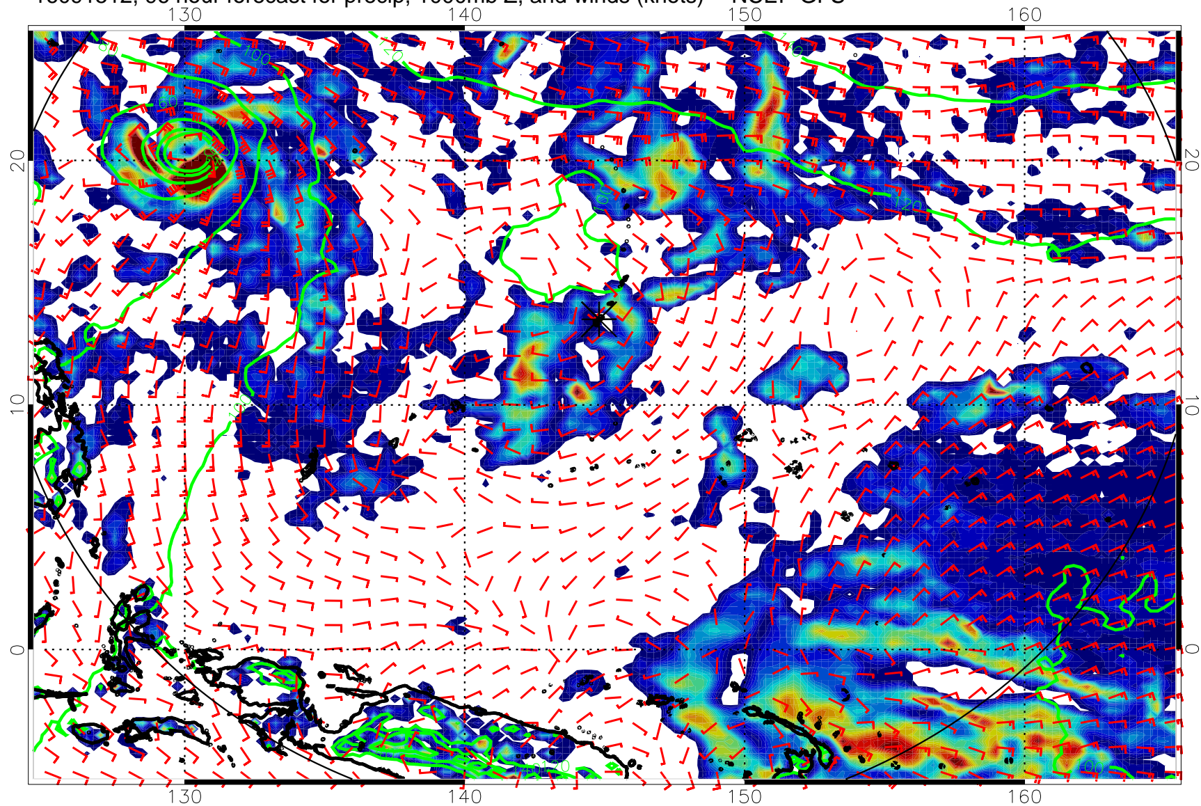
16091512, 96 hour forecast for precip, 1000mb Z, and winds (knots) -- NCEP GFS
